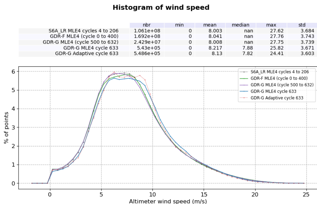
Figure 11: Altimeter Wind Speed histogram computed over cycle 633
