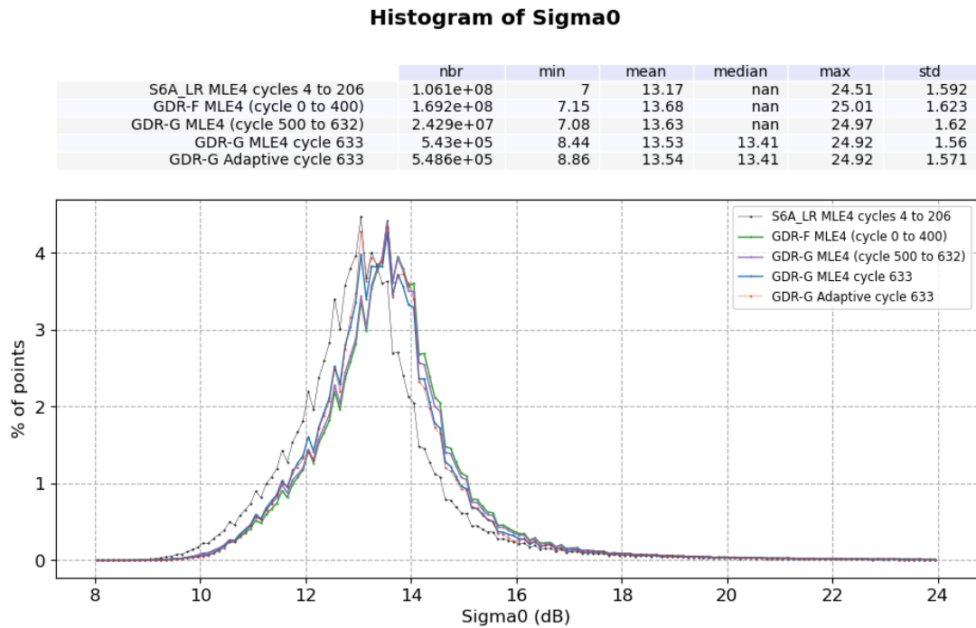
Figure 8: Ku-band Backscattering coefficient histogram computed over cycle 633
