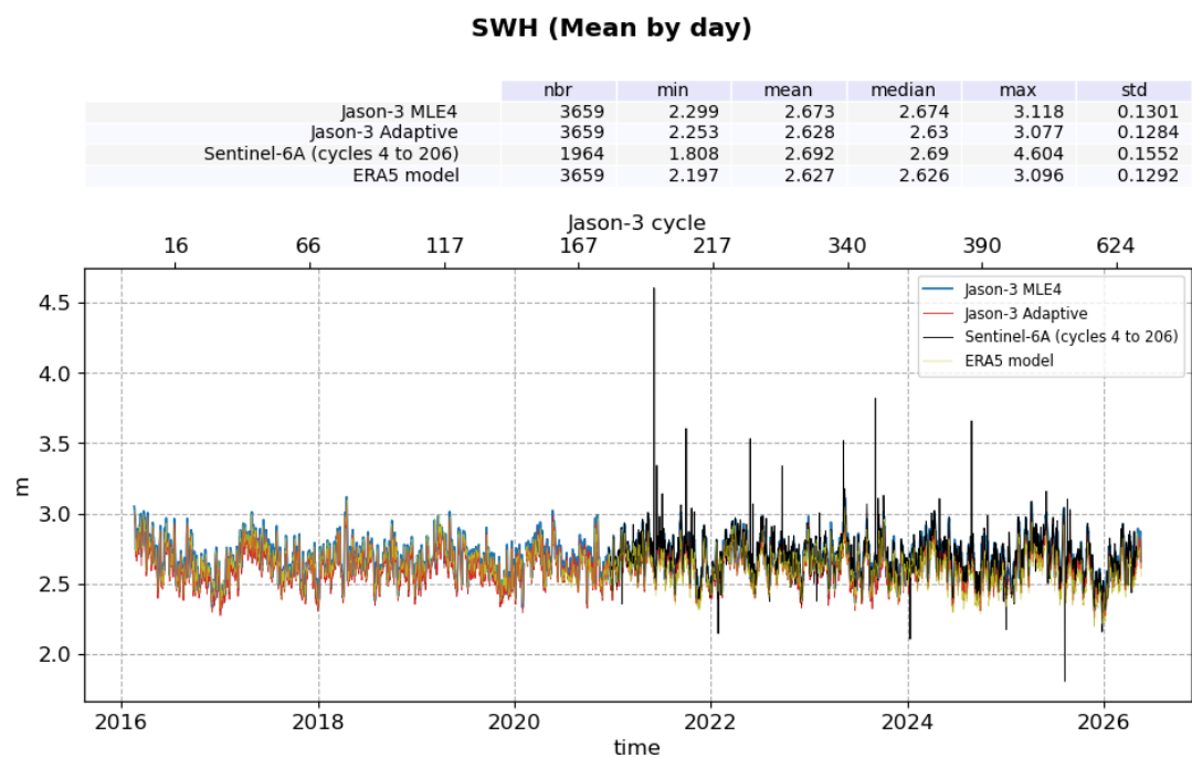
Figure 7: Ku-band Significant Wave Height daily monitoring from cycle 001 to 633, for Jason-3 and Sentinel-6A
