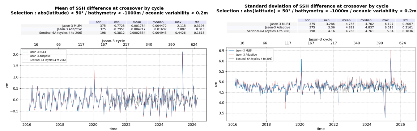
Figure 23: Monitoring of SSH difference at crossovers for Jason-3 MLE4 and Adaptive, and Sentinel-6A LR MLE4 : mean (left) and standard deviation (right), from cycle 001 to 633
