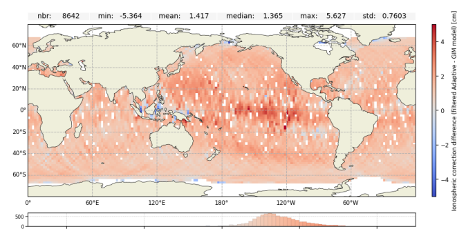
Figure 16: Ionospheric correction difference over cycle 633 for Jason-3 GDR : Filtered MLE4 - GIM model (left) and Filtered Adaptive - GIM model (right)
