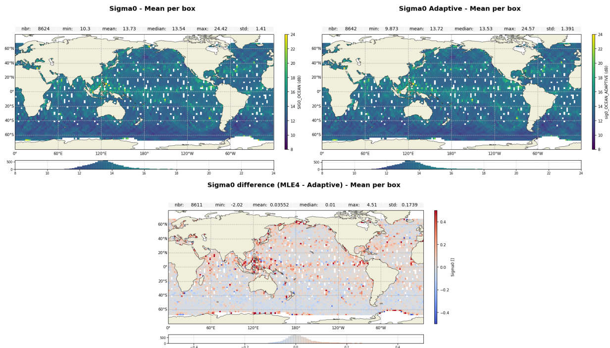
Figure 9: Map of Ku-band backscatter coefficient over cycle 633 for Jason-3 MLE4 (up left), Adaptive (up right) and difference MLE4-Adaptive (down)
