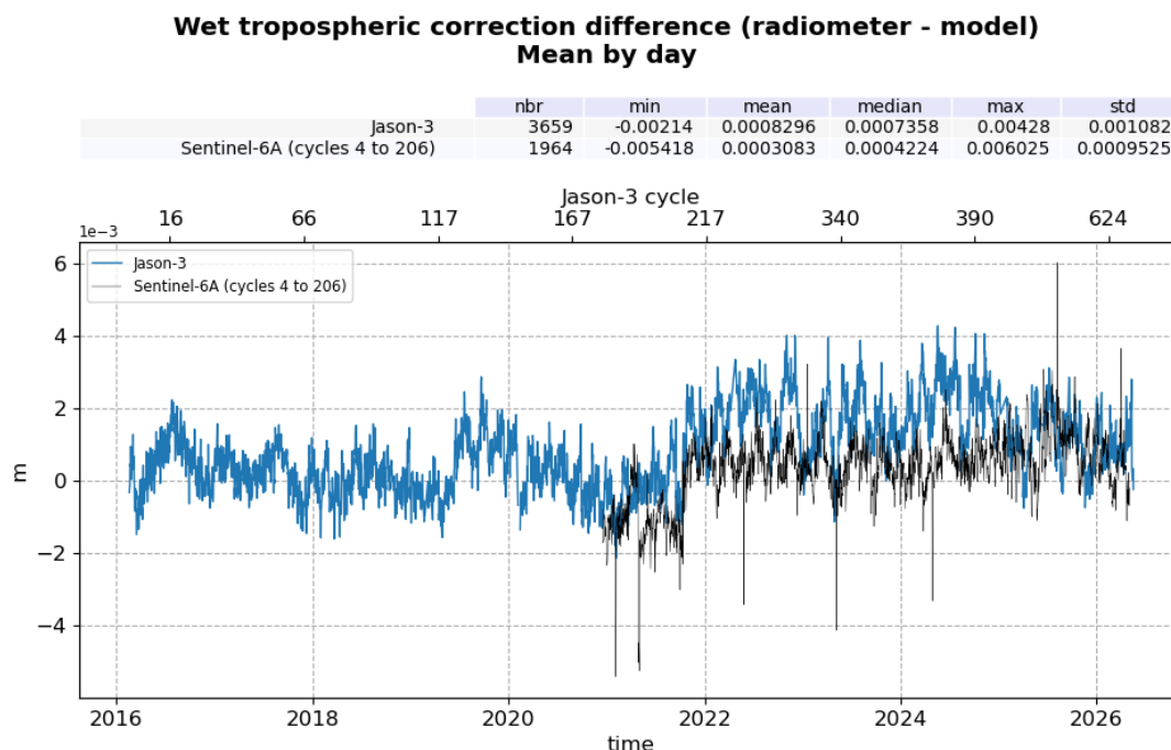
Figure 19: Daily monitoring of mean wet tropospheric correction difference computed from cycle 001 to cycle 633
