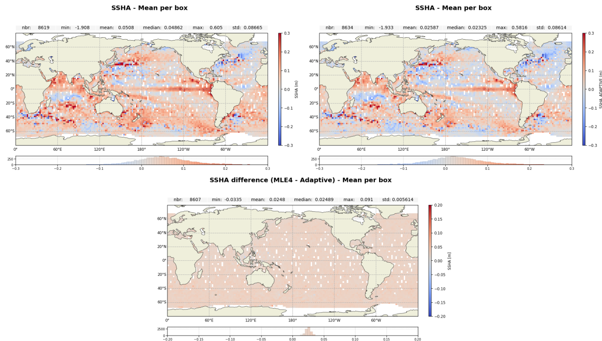
Figure 24: Along-track maps of SSHA over cycle 633 for Jason-3 MLE4 (up left), Adaptive (up right) and difference MLE4-Adaptive (down)
