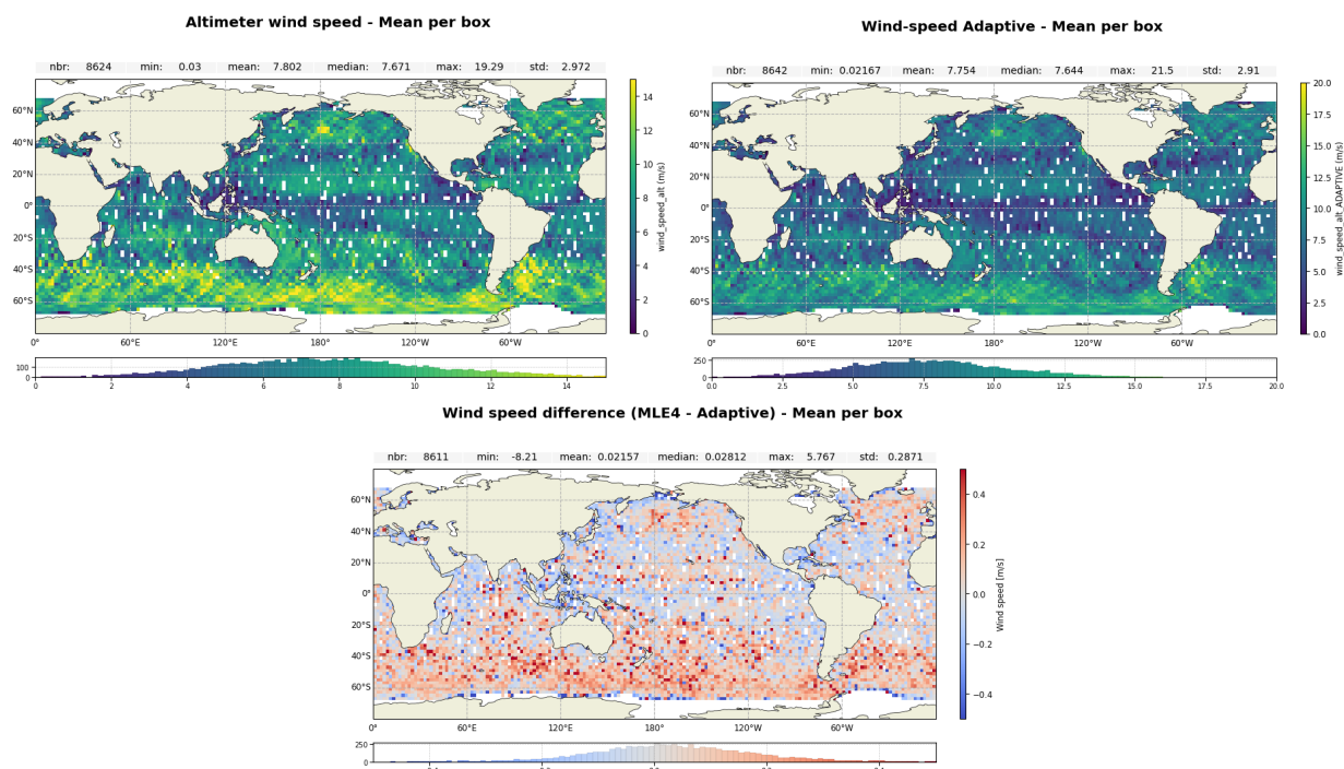
Figure 12: Map of Ku-band wind-speed over cycle 633 for Jason-3 MLE4 (up left), Adaptive (up right) and difference MLE4-Adaptive (down)
