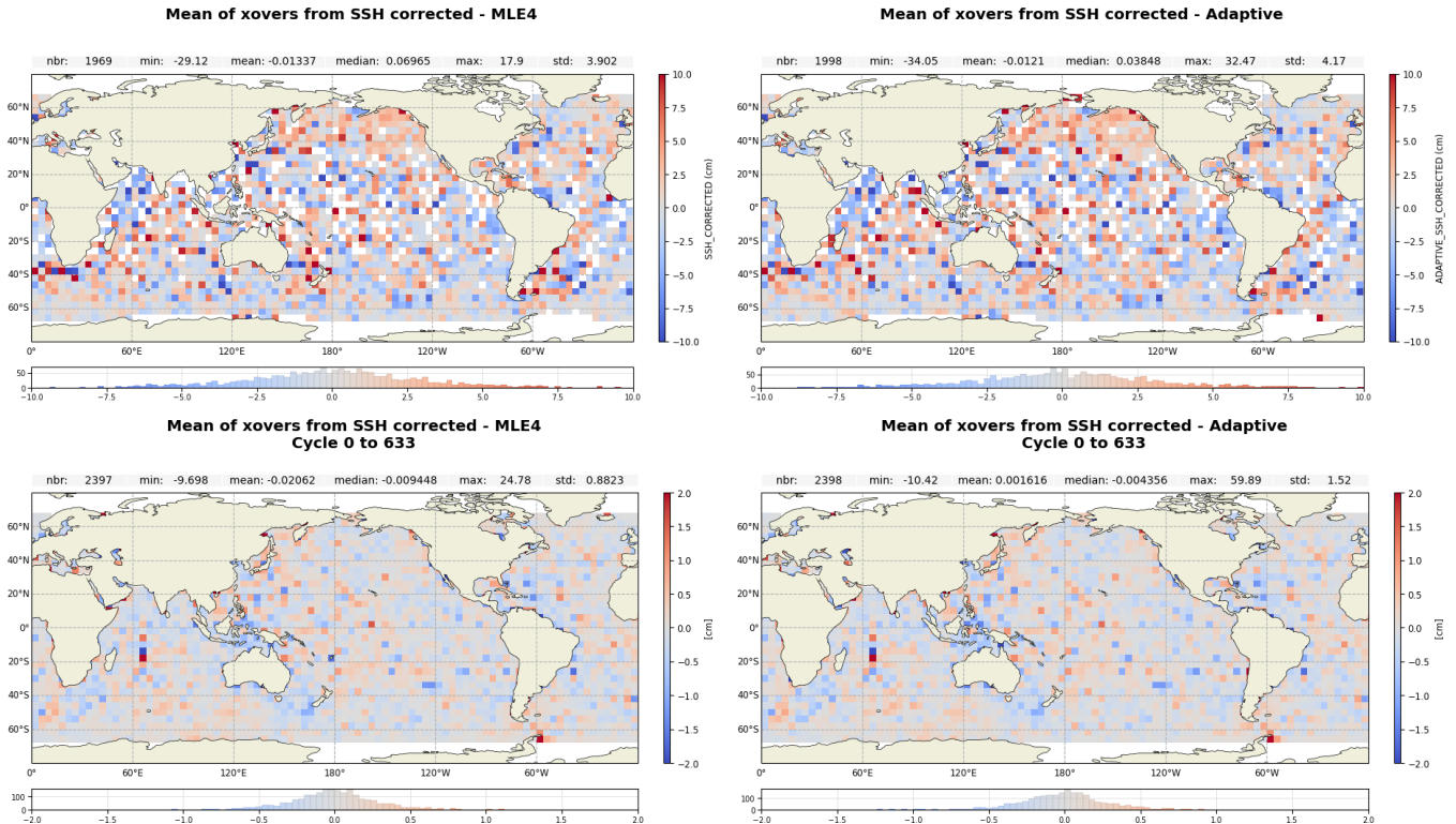
Figure 22: Mean SSH difference at crossovers for Jason-3 MLE4 (left) and Adaptive (right) cycle 633 (top) and from cycle 001 to cycle 633 (bottom)
