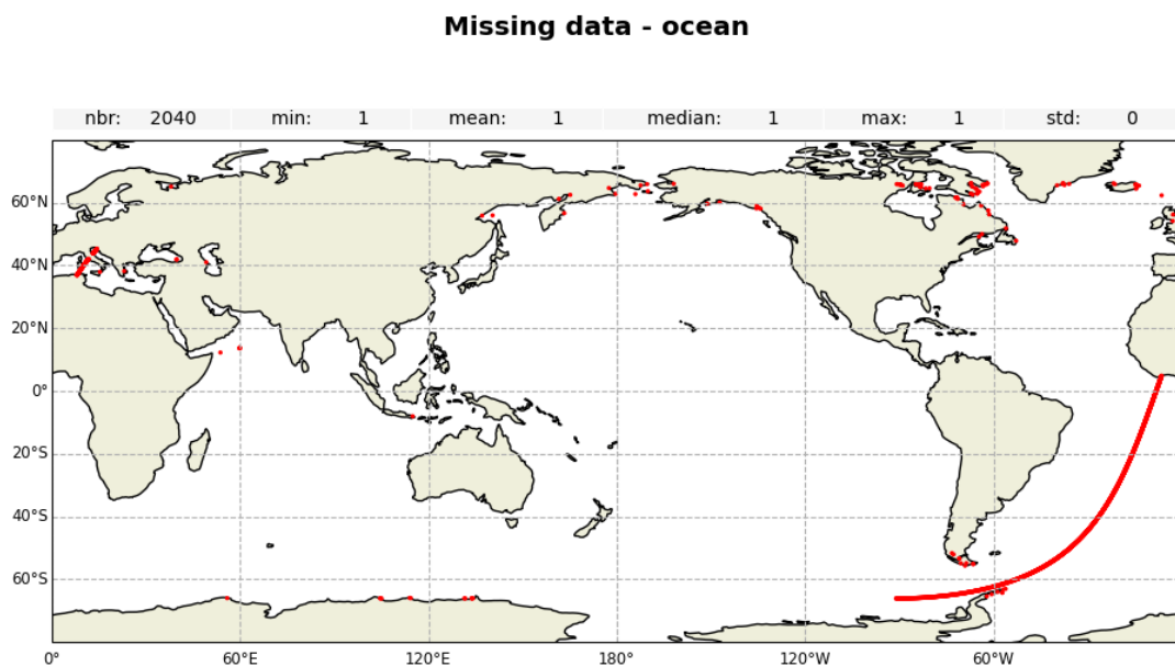
Figure 2: Map of missing measurements over ocean for Jason-3 GDR cycle 633
