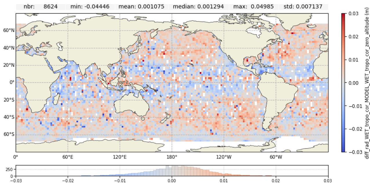
Figure 21: Map of wet tropospheric corrections differences over cycle 633 for Jason-3
