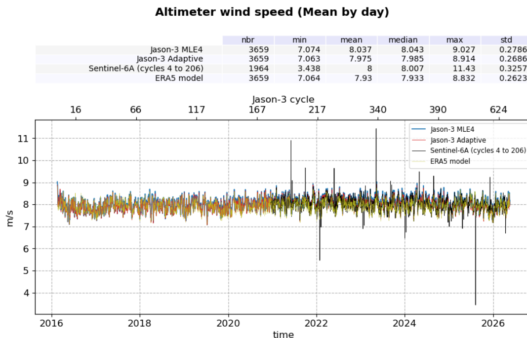
Figure 13: Wind Speed daily monitoring from cycle 001 to 633 for Jason-3 GDR, and Sentinel-6A (LR MLE4)
