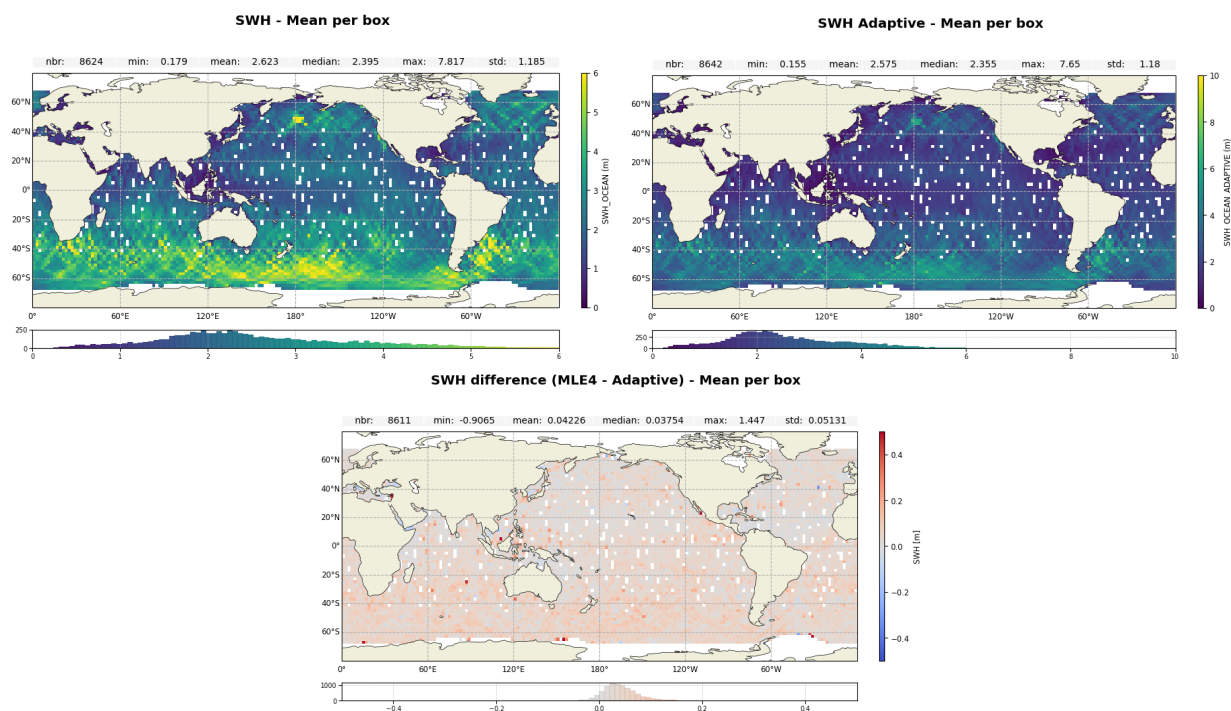
Figure 6: Map of Ku-band Significant Wave Height over cycle 633 for Jason-3 MLE4 (up left), Adaptive (up right) and difference MLE4-Adaptive (down)
