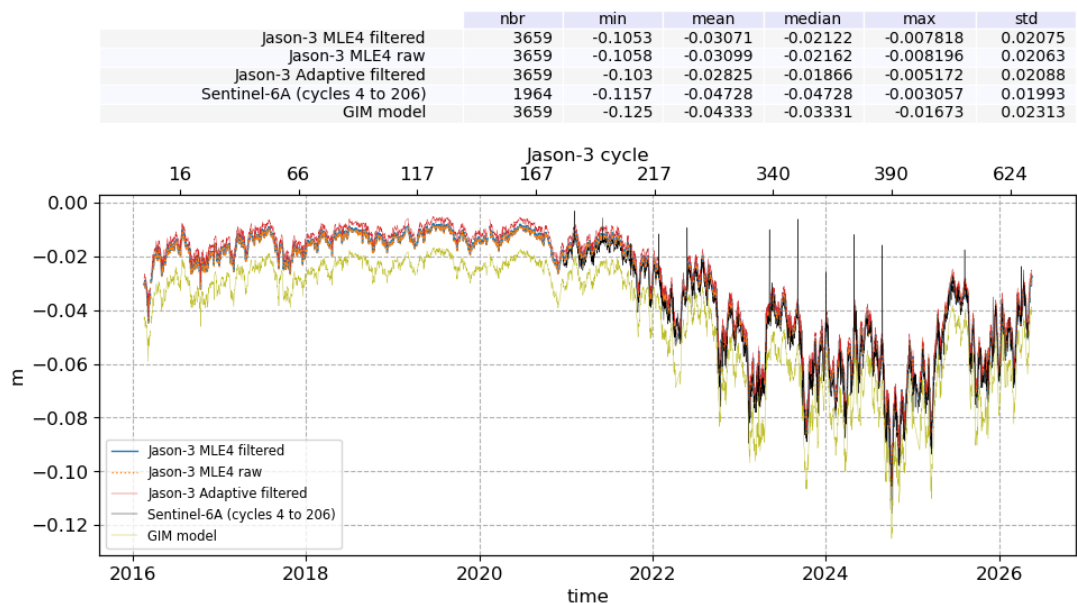
Figure 15: Daily mean of ionosphere correction over cycle 633 for Jason-3 MLE4 and Adaptive, and for Sentinel-6A
