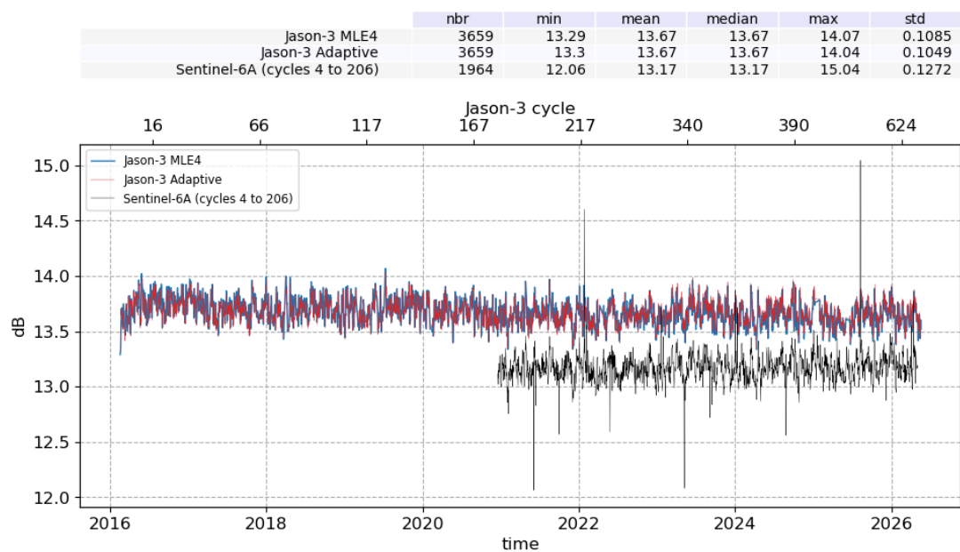
Figure 10: Ku-band Backscattering coefficient daily monitoring from cycle 001 to 633, for Jason-3 and Sentinel-6A
