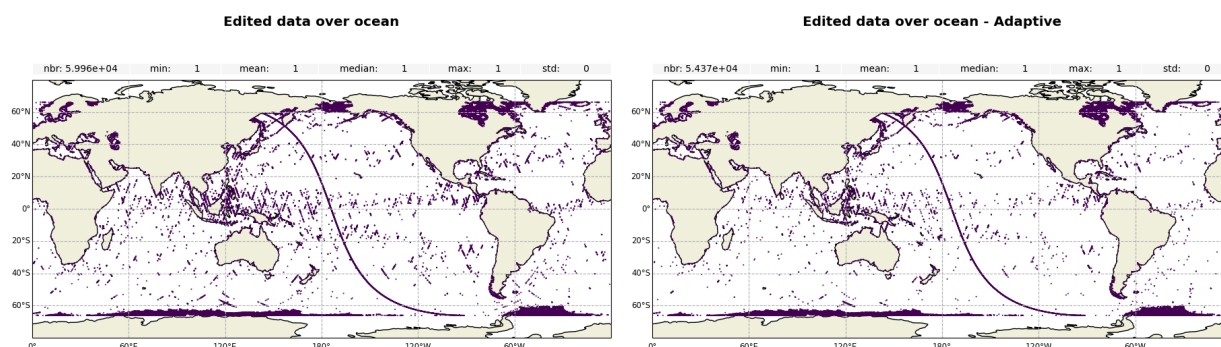
Figure 4: Edited measurements for Jason-3 over cycle 633 for MLE4 (left) and Adaptive (right)
