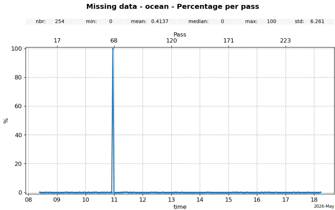
Figure 3: Monitoring of the percentage per pass of missing data over ocean for Jason-3 GDR cycle 633
