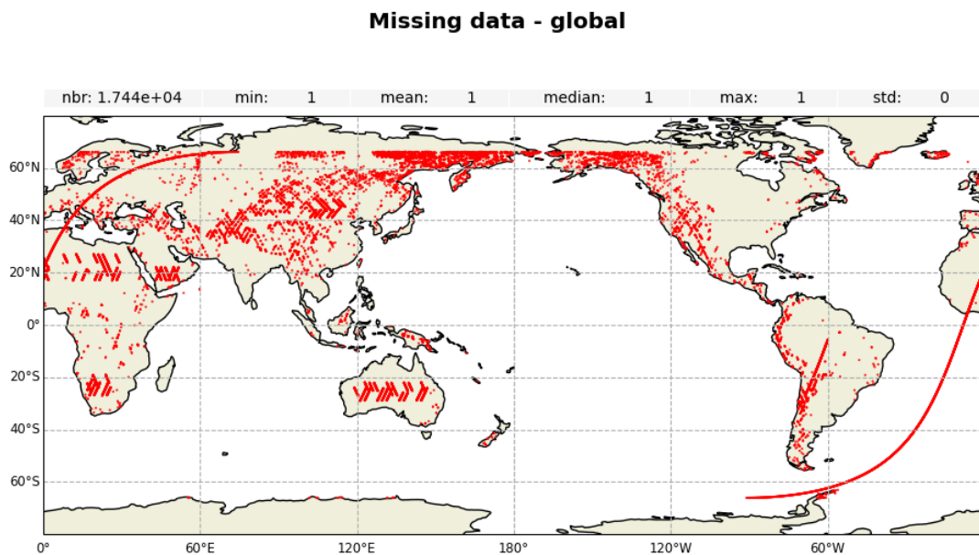
Figure 1: Map of missing measurements for Jason-3 GDR cycle 633
