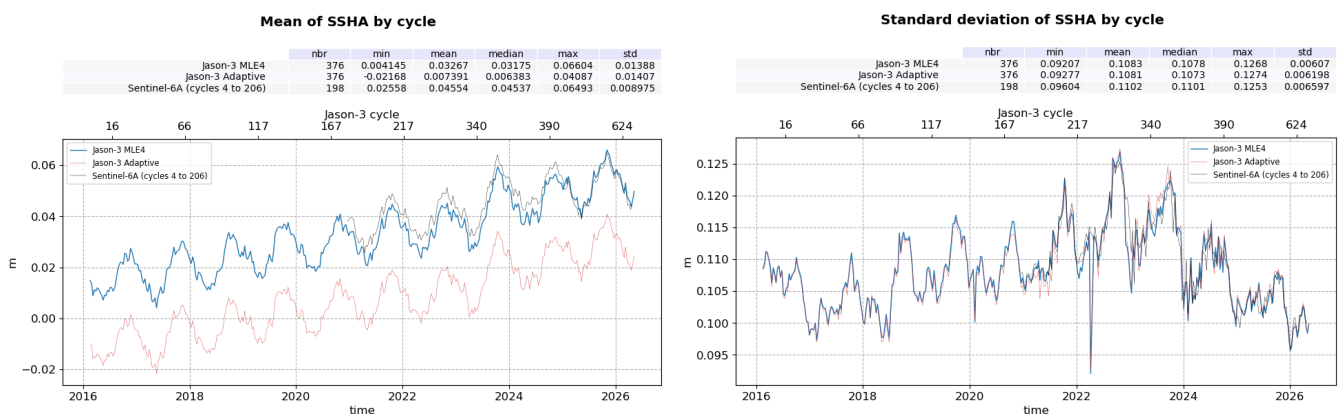
Figure 25: SSHA daily monitoring from cycle 001 to 633, for Jason-3 GDR
