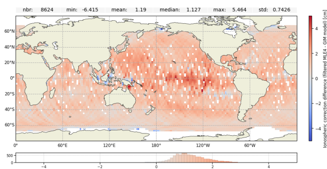
Figure 16: Ionospheric correction difference over cycle 633 for Jason-3 GDR : Filtered MLE4 - GIM model (left) and Filtered Adaptive - GIM model (right)
