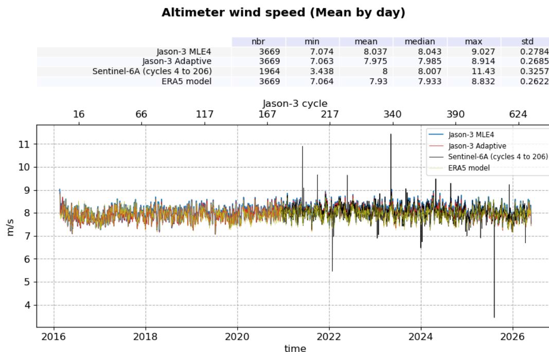
Figure 13: Wind Speed daily monitoring from cycle 001 to 634 for Jason-3 GDR, and Sentinel-6A (LR MLE4)
