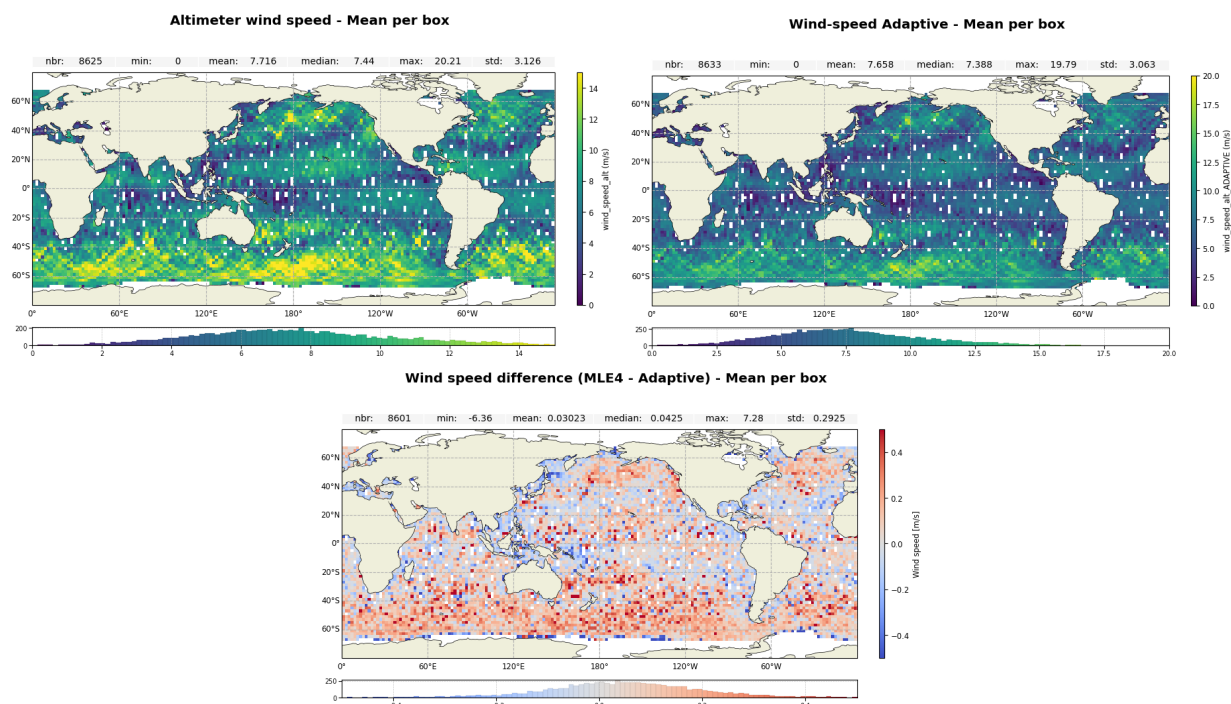
Figure 12: Map of Ku-band wind-speed over cycle 634 for Jason-3 MLE4 (up left), Adaptive (up right) and difference MLE4-Adaptive (down)
