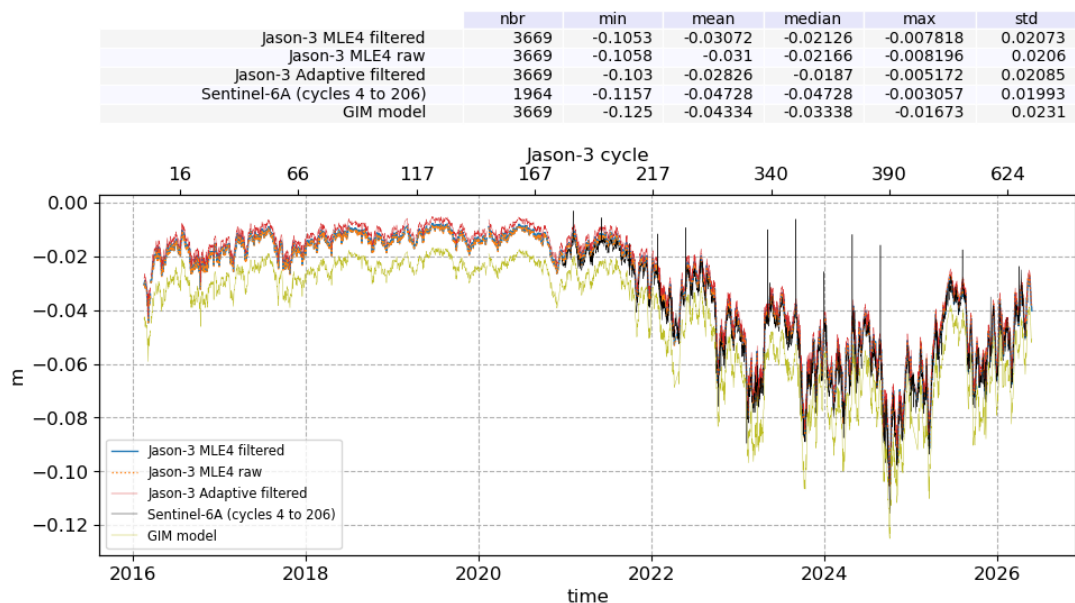
Figure 15: Daily mean of ionosphere correction over cycle 634 for Jason-3 MLE4 and Adaptive, and for Sentinel-6A
