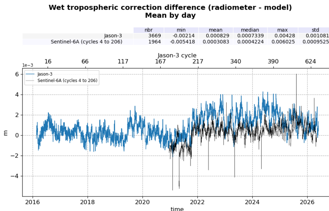
Figure 19: Daily monitoring of mean wet tropospheric correction difference computed from cycle 001 to cycle 634
