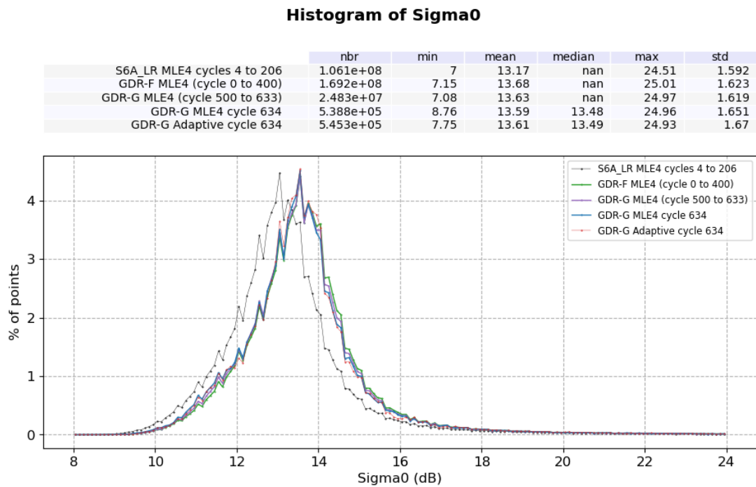
Figure 8: Ku-band Backscattering coefficient histogram computed over cycle 634
