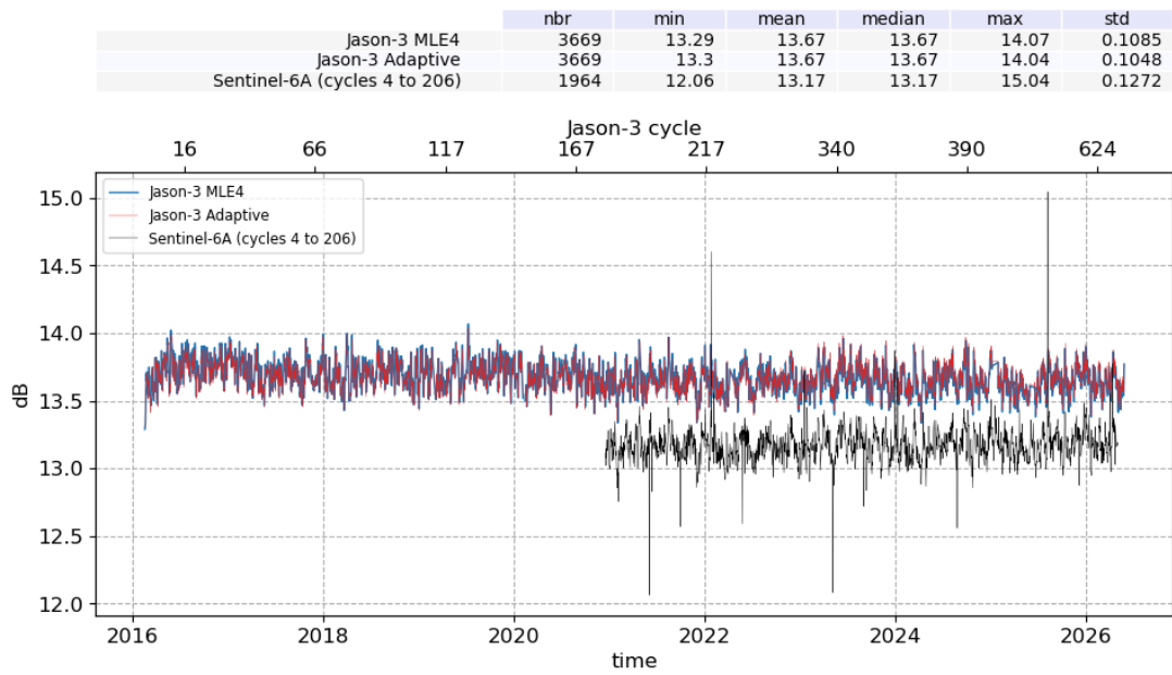
Figure 10: Ku-band Backscattering coefficient daily monitoring from cycle 001 to 634, for Jason-3 and Sentinel-6A
