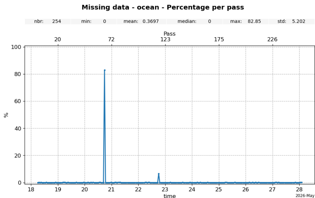
Figure 3: Monitoring of the percentage per pass of missing data over ocean for Jason-3 GDR cycle 634
