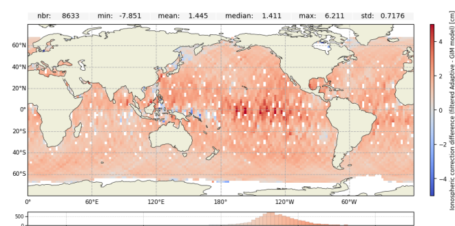
Figure 16: Ionospheric correction difference over cycle 634 for Jason-3 GDR : Filtered MLE4 - GIM model (left) and Filtered Adaptive - GIM model (right)
