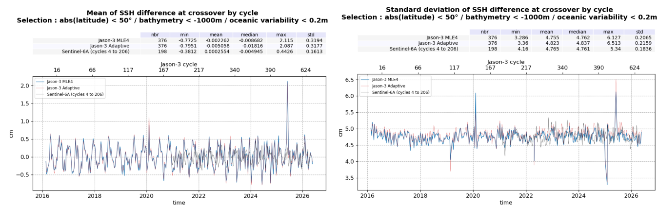
Figure 23: Monitoring of SSH difference at crossovers for Jason-3 MLE4 and Adaptive, and Sentinel-6A LR MLE4 : mean (left) and standard deviation (right), from cycle 001 to 634
