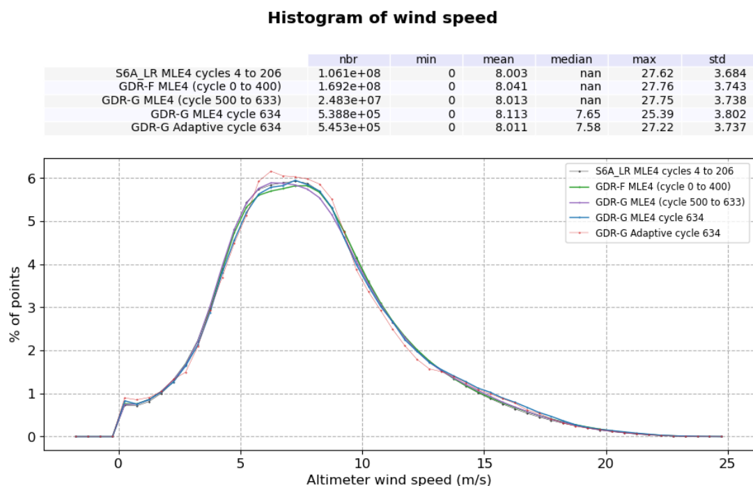
Figure 11: Altimeter Wind Speed histogram computed over cycle 634
