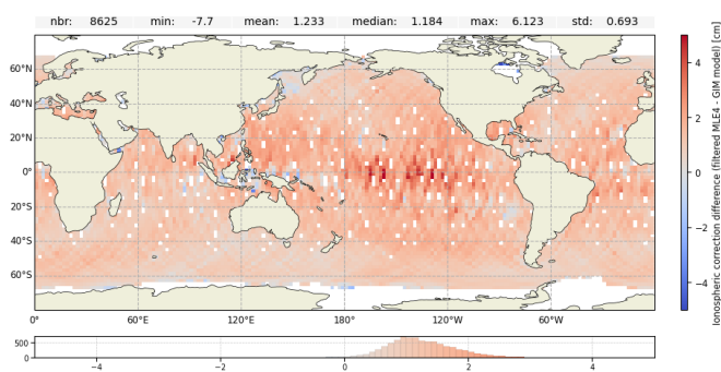
Figure 16: Ionospheric correction difference over cycle 634 for Jason-3 GDR : Filtered MLE4 - GIM model (left) and Filtered Adaptive - GIM model (right)
