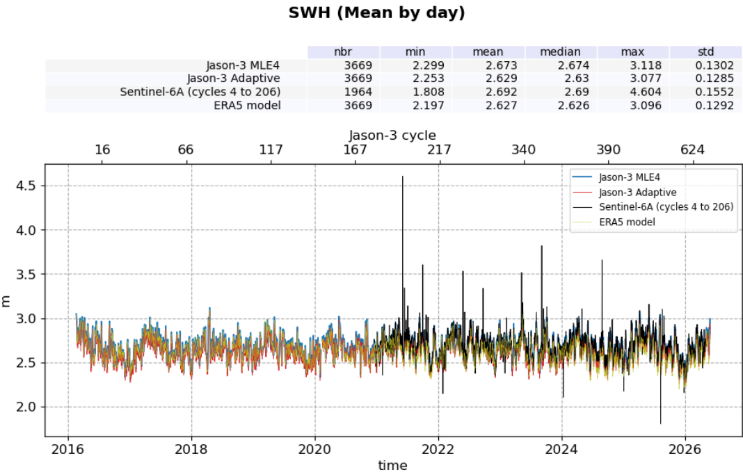
Figure 7: Ku-band Significant Wave Height daily monitoring from cycle 001 to 634, for Jason-3 and Sentinel-6A
