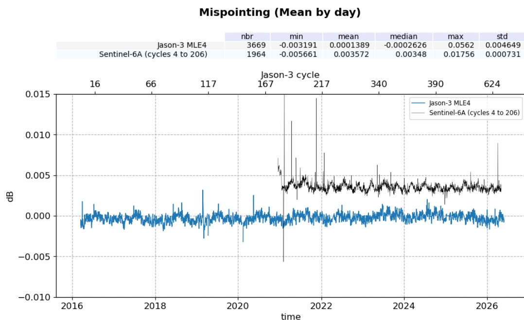
Figure 18: Mispointing daily monitoring from cycle 001 to 634 for Jason-3 GDR and Sentinel-6A
