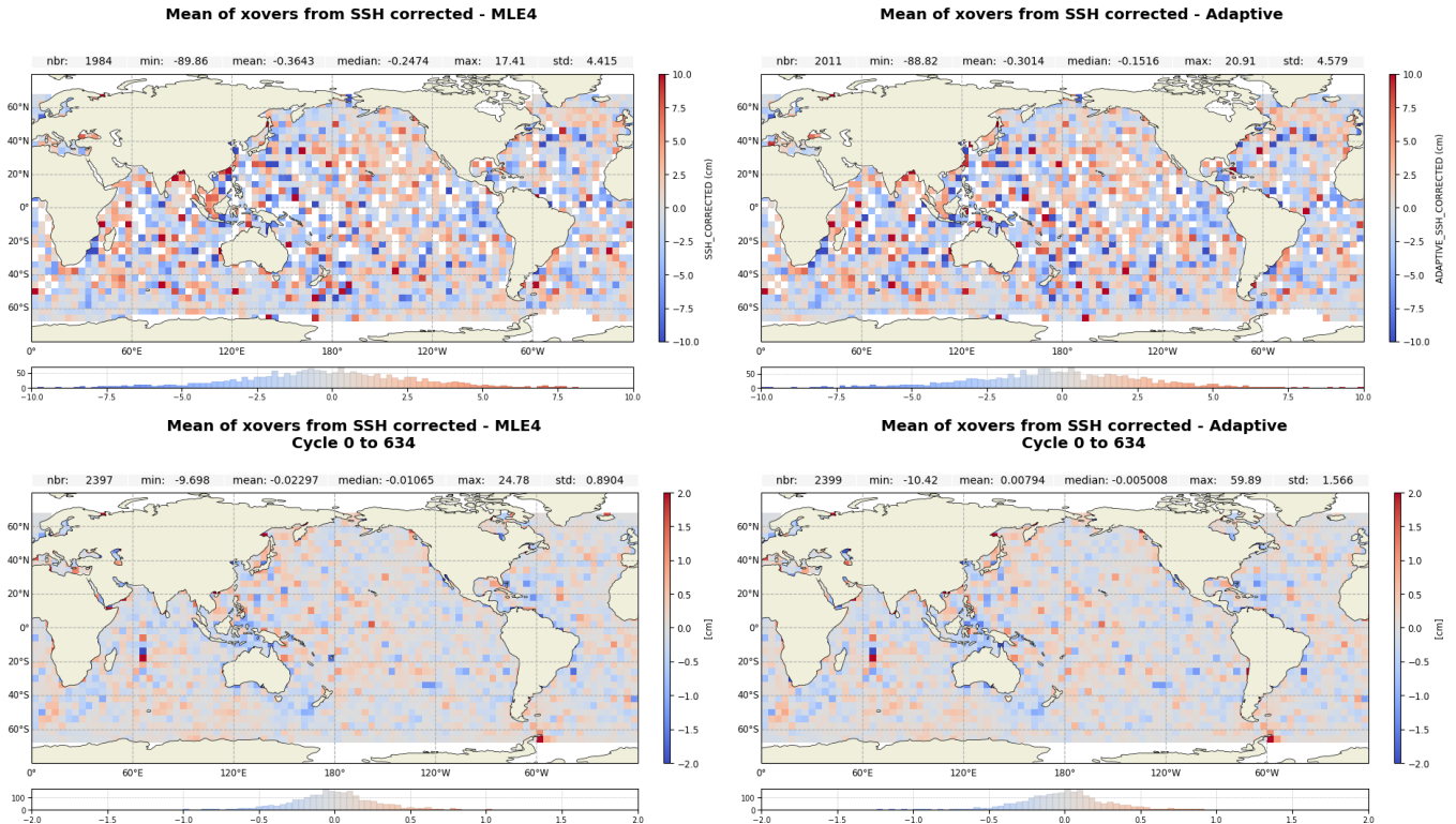
Figure 22: Mean SSH difference at crossovers for Jason-3 MLE4 (left) and Adaptive (right) cycle 634 (top) and from cycle 001 to cycle 634 (bottom)
