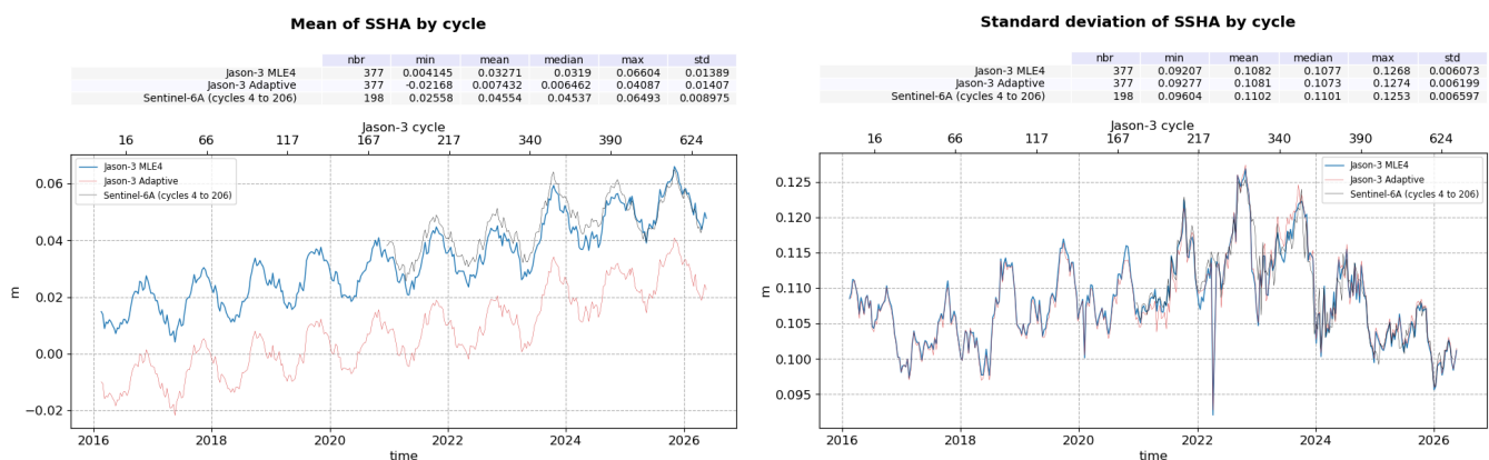
Figure 25: SSHA daily monitoring from cycle 001 to 634, for Jason-3 GDR
