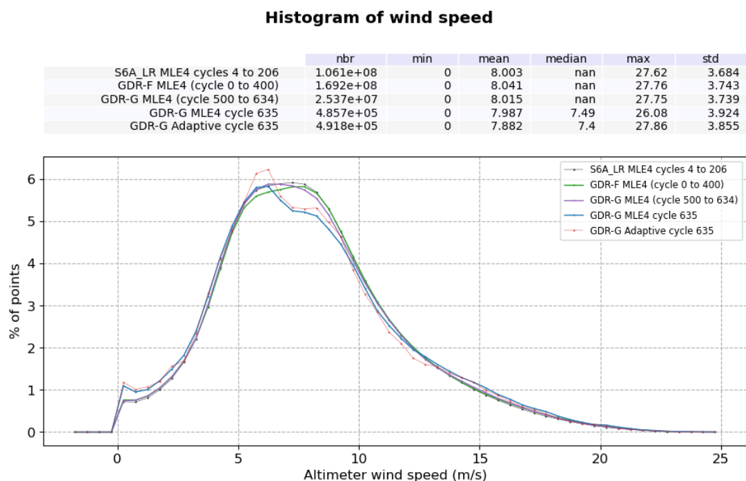
Figure 11: Altimeter Wind Speed histogram computed over cycle 635
