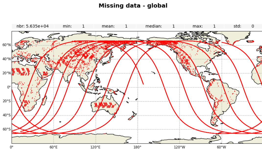
Figure 1: Map of missing measurements for Jason-3 GDR cycle 635
