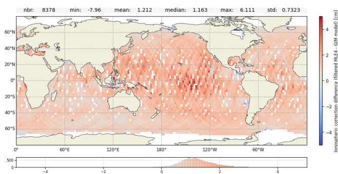
Figure 16: Ionospheric correction difference over cycle 635 for Jason-3 GDR : Filtered MLE4 - GIM model (left) and Filtered Adaptive - GIM model (right)
