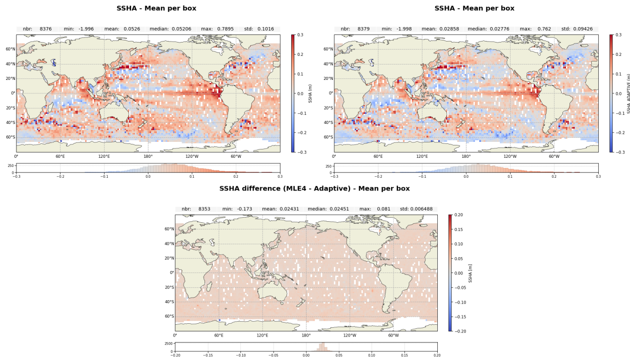
Figure 24: Along-track maps of SSHA over cycle 635 for Jason-3 MLE4 (up left), Adaptive (up right) and difference MLE4-Adaptive (down)
