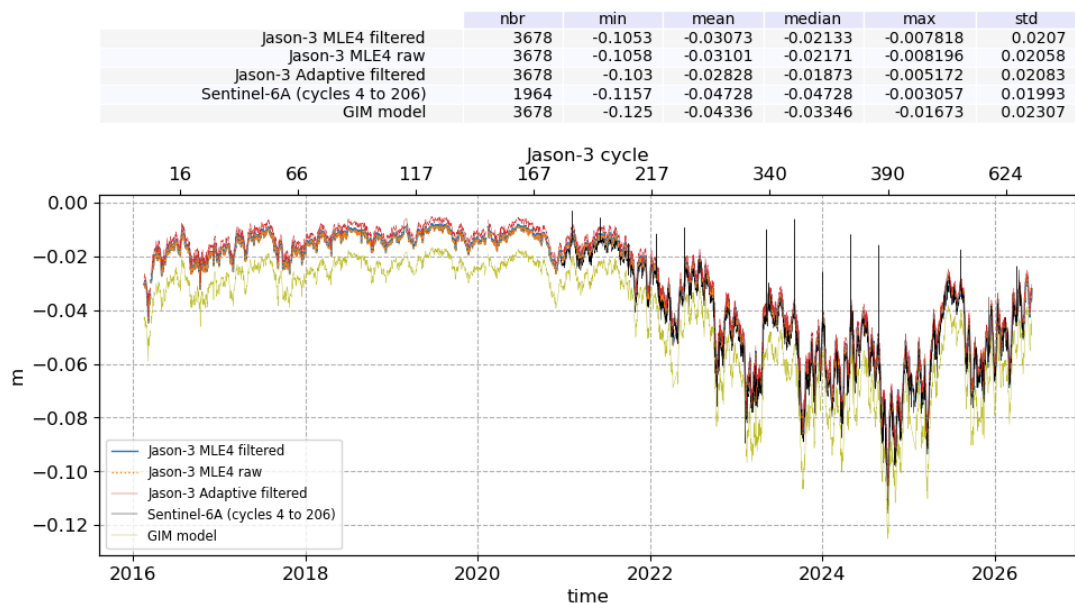
Figure 15: Daily mean of ionosphere correction over cycle 635 for Jason-3 MLE4 and Adaptive, and for Sentinel-6A
