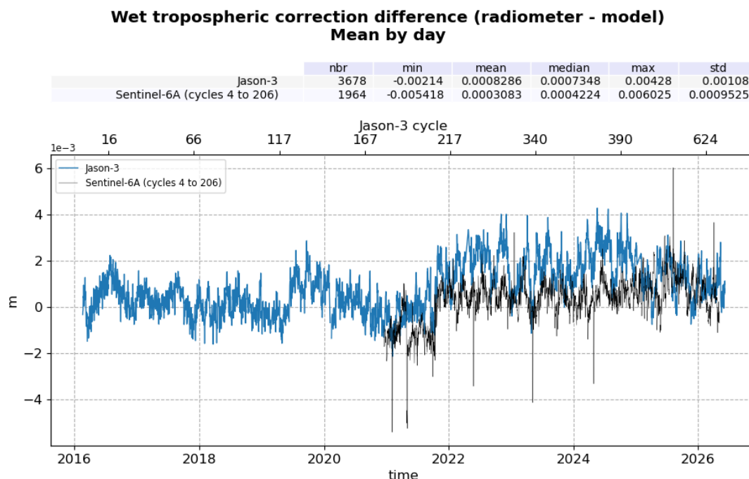
Figure 19: Daily monitoring of mean wet tropospheric correction difference computed from cycle 001 to cycle 635
