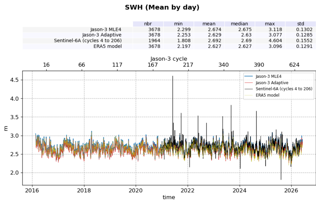
Figure 7: Ku-band Significant Wave Height daily monitoring from cycle 001 to 635, for Jason-3 and Sentinel-6A
