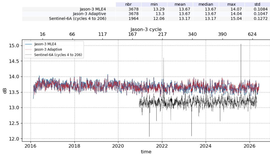
Figure 10: Ku-band Backscattering coefficient daily monitoring from cycle 001 to 635, for Jason-3 and Sentinel-6A
