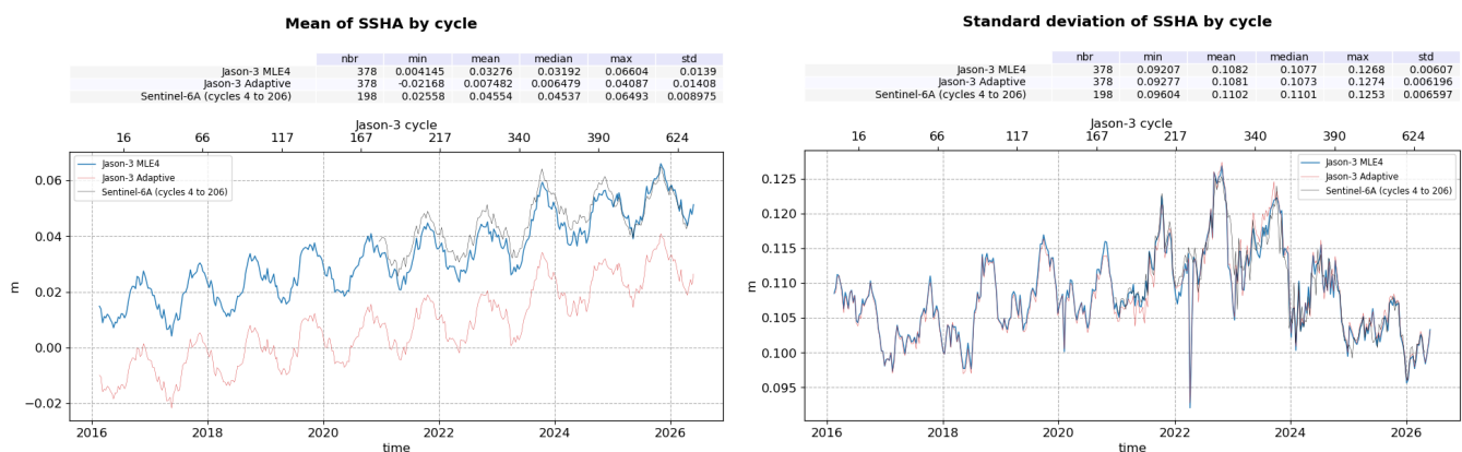
Figure 25: SSHA daily monitoring from cycle 001 to 635, for Jason-3 GDR
