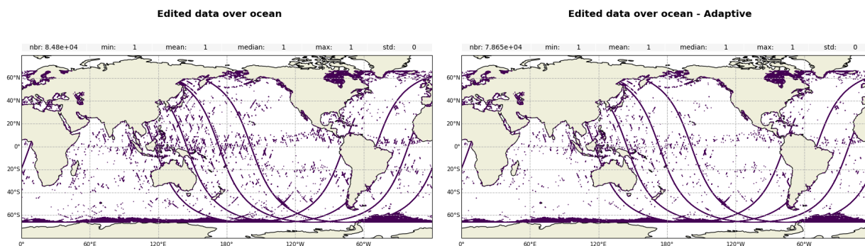
Figure 4: Edited measurements for Jason-3 over cycle 635 for MLE4 (left) and Adaptive (right)
