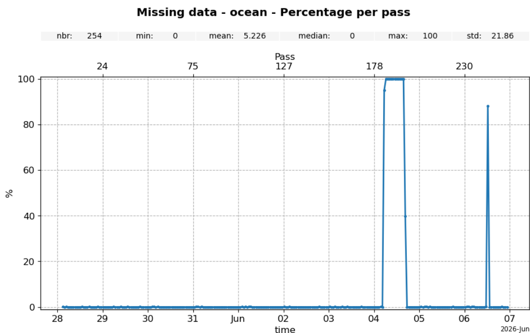
Figure 3: Monitoring of the percentage per pass of missing data over ocean for Jason-3 GDR cycle 635
