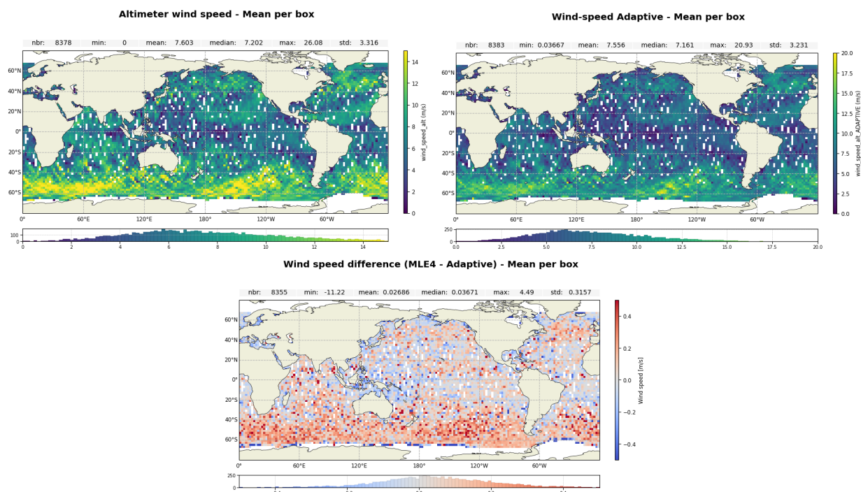
Figure 12: Map of Ku-band wind-speed over cycle 635 for Jason-3 MLE4 (up left), Adaptive (up right) and difference MLE4-Adaptive (down)
