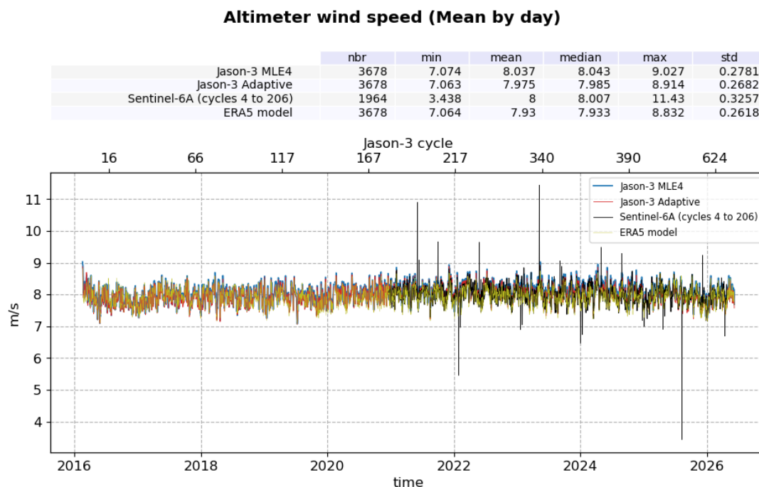
Figure 13: Wind Speed daily monitoring from cycle 001 to 635 for Jason-3 GDR, and Sentinel-6A (LR MLE4)
