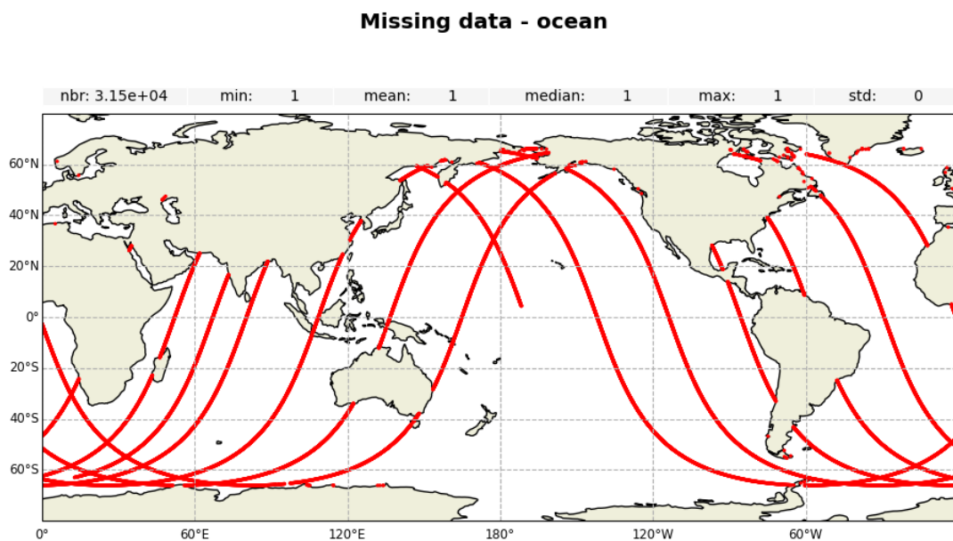
Figure 2: Map of missing measurements over ocean for Jason-3 GDR cycle 635
