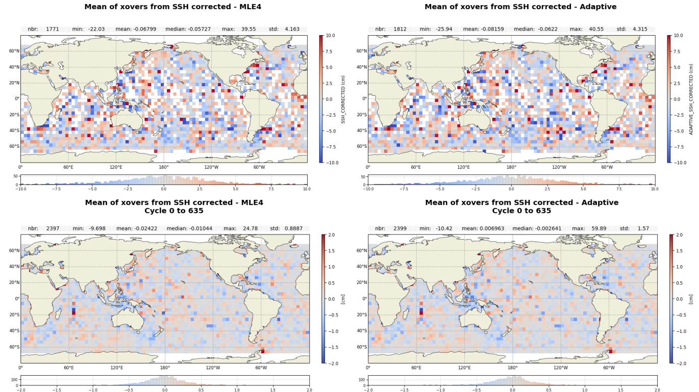
Figure 22: Mean SSH difference at crossovers for Jason-3 MLE4 (left) and Adaptive (right) cycle 635 (top) and from cycle 001 to cycle 635 (bottom)
