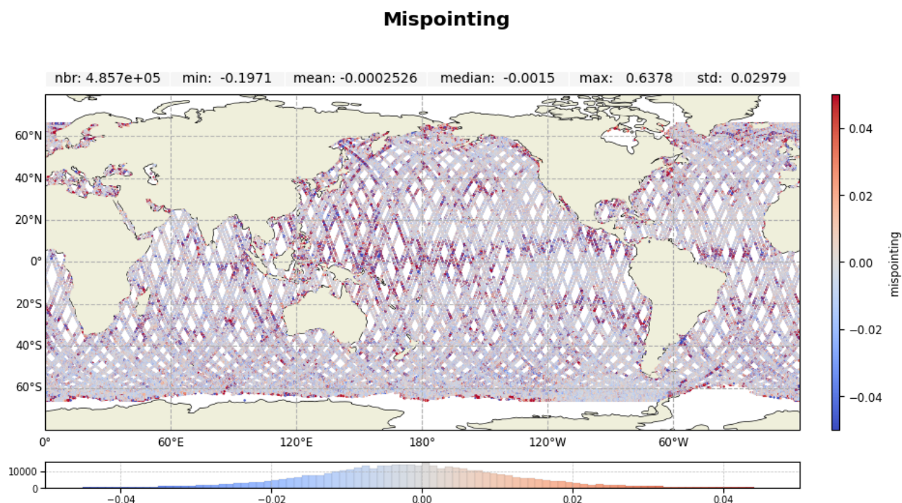
Figure 17: Along-track map of mispointing over cycle 635 for Jason-3 MLE4
