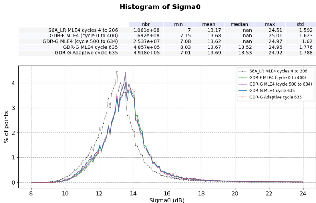
Figure 8: Ku-band Backscattering coefficient histogram computed over cycle 635
