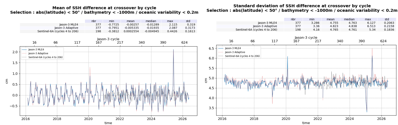
Figure 23: Monitoring of SSH difference at crossovers for Jason-3 MLE4 and Adaptive, and Sentinel-6A LR MLE4 : mean (left) and standard deviation (right), from cycle 001 to 635
