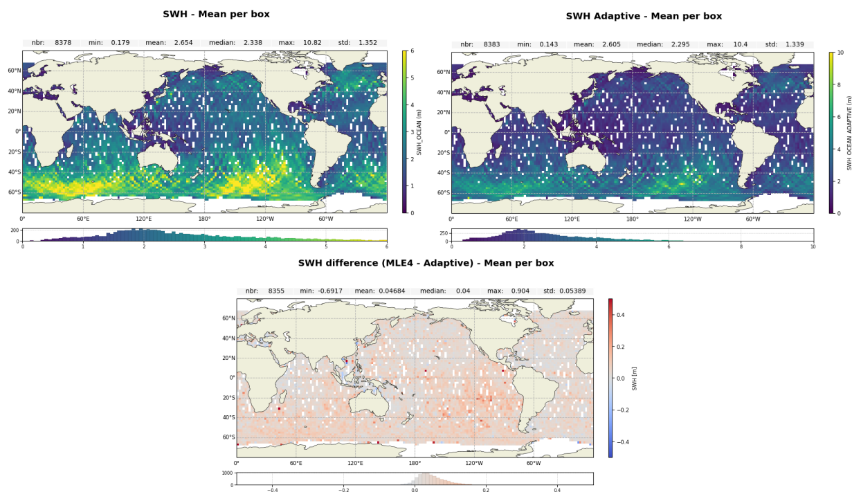
Figure 6: Map of Ku-band Significant Wave Height over cycle 635 for Jason-3 MLE4 (up left), Adaptive (up right) and difference MLE4-Adaptive (down)
