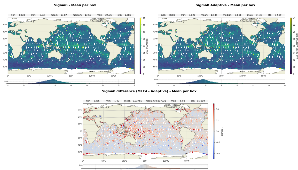
Figure 9: Map of Ku-band backscatter coefficient over cycle 635 for Jason-3 MLE4 (up left), Adaptive (up right) and difference MLE4-Adaptive (down)
