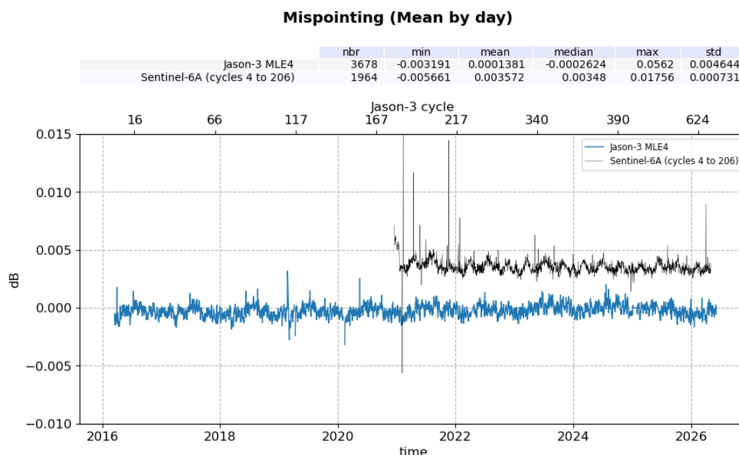
Figure 18: Mispointing daily monitoring from cycle 001 to 635 for Jason-3 GDR and Sentinel-6A
