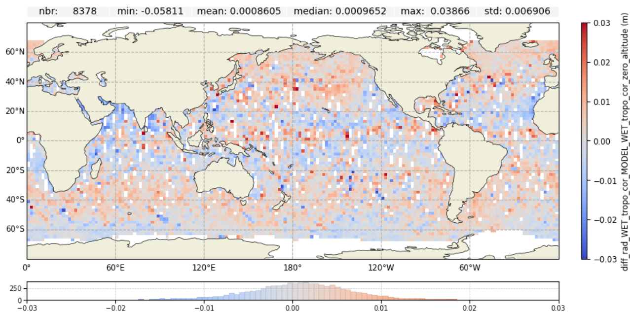
Figure 21: Map of wet tropospheric corrections differences over cycle 635 for Jason-3
