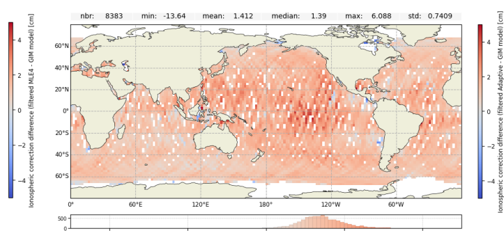
Figure 16: Ionospheric correction difference over cycle 635 for Jason-3 GDR : Filtered MLE4 - GIM model (left) and Filtered Adaptive - GIM model (right)
