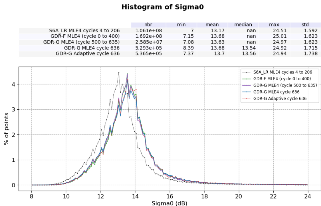
Figure 8: Ku-band Backscattering coefficient histogram computed over cycle 636
