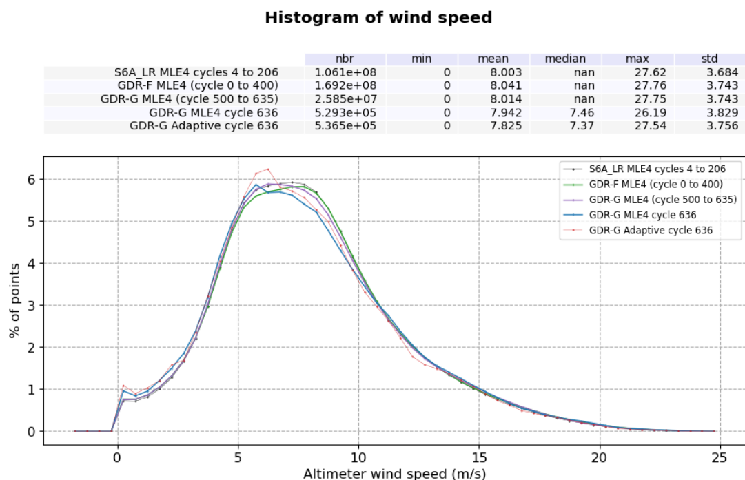
Figure 11: Altimeter Wind Speed histogram computed over cycle 636
