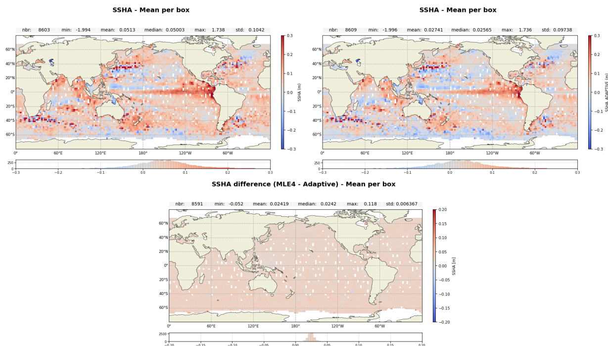
Figure 24: Along-track maps of SSHA over cycle 636 for Jason-3 MLE4 (up left), Adaptive (up right) and difference MLE4-Adaptive (down)
