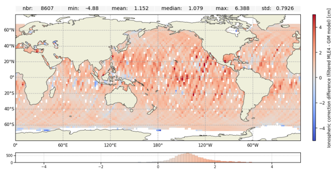
Figure 16: Ionospheric correction difference over cycle 636 for Jason-3 GDR : Filtered MLE4 - GIM model (left) and Filtered Adaptive - GIM model (right)
