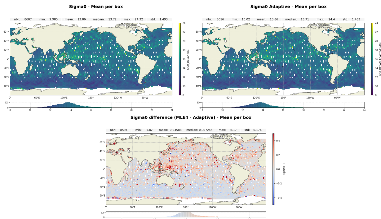
Figure 9: Map of Ku-band backscatter coefficient over cycle 636 for Jason-3 MLE4 (up left), Adaptive (up right) and difference MLE4-Adaptive (down)
