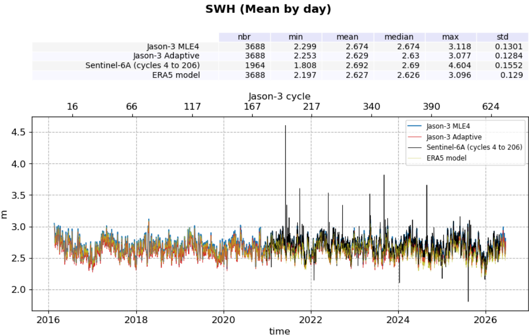
Figure 7: Ku-band Significant Wave Height daily monitoring from cycle 001 to 636, for Jason-3 and Sentinel-6A
