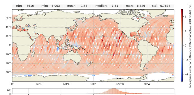
Figure 16: Ionospheric correction difference over cycle 636 for Jason-3 GDR : Filtered MLE4 - GIM model (left) and Filtered Adaptive - GIM model (right)
