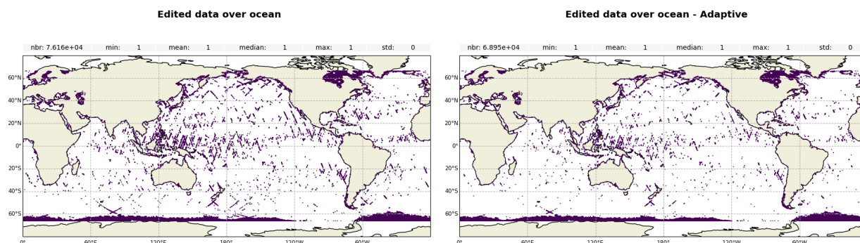
Figure 4: Edited measurements for Jason-3 over cycle 636 for MLE4 (left) and Adaptive (right)
