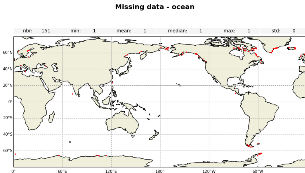
Figure 2: Map of missing measurements over ocean for Jason-3 GDR cycle 636
