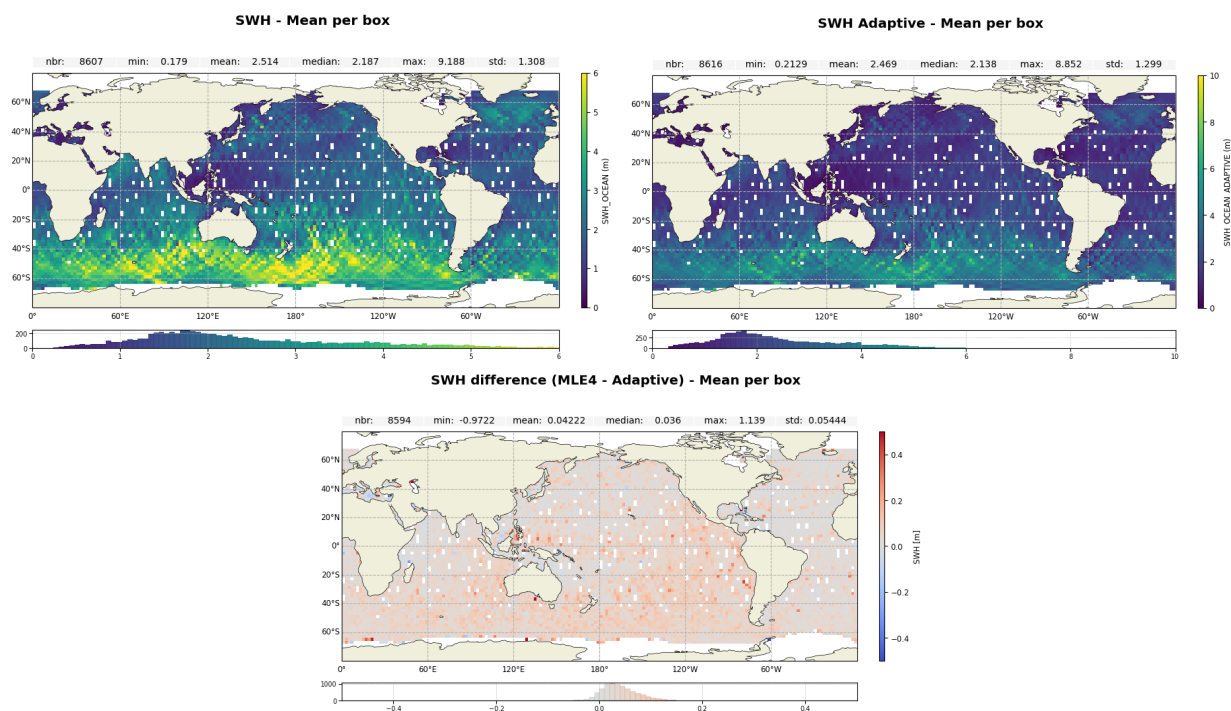
Figure 6: Map of Ku-band Significant Wave Height over cycle 636 for Jason-3 MLE4 (up left), Adaptive (up right) and difference MLE4-Adaptive (down)
