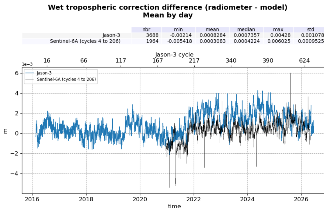
Figure 19: Daily monitoring of mean wet tropospheric correction difference computed from cycle 001 to cycle 636
