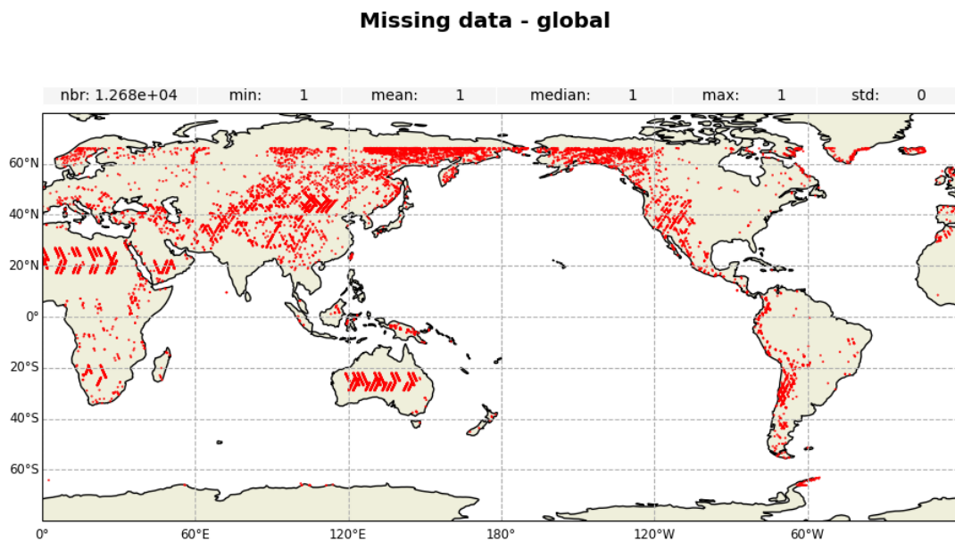
Figure 1: Map of missing measurements for Jason-3 GDR cycle 636
