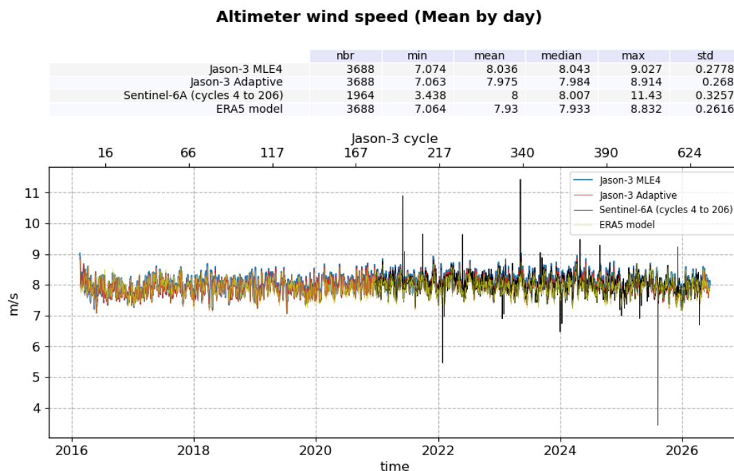
Figure 13: Wind Speed daily monitoring from cycle 001 to 636 for Jason-3 GDR, and Sentinel-6A (LR MLE4)
