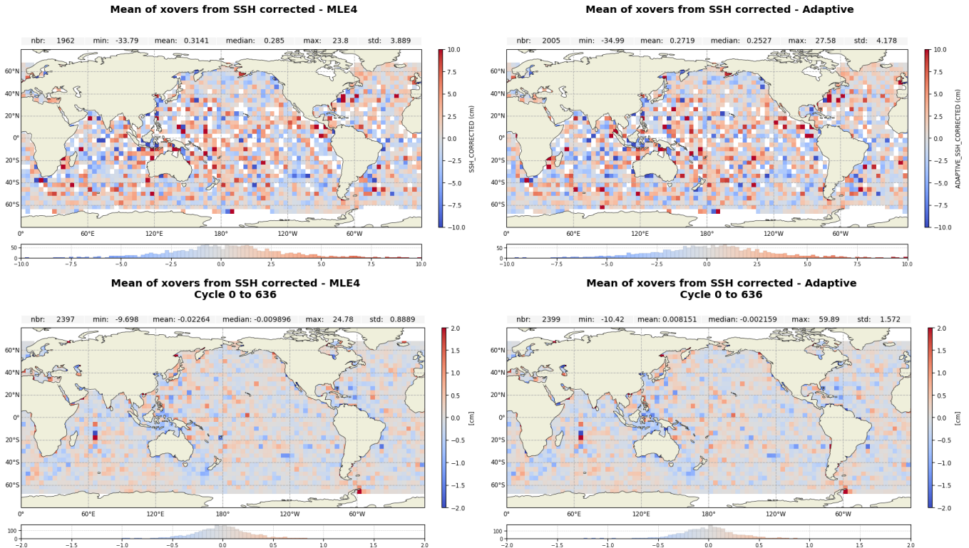
Figure 22: Mean SSH difference at crossovers for Jason-3 MLE4 (left) and Adaptive (right) cycle 636 (top) and from cycle 001 to cycle 636 (bottom)
