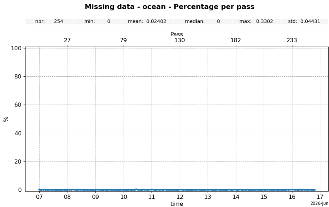
Figure 3: Monitoring of the percentage per pass of missing data over ocean for Jason-3 GDR cycle 636
