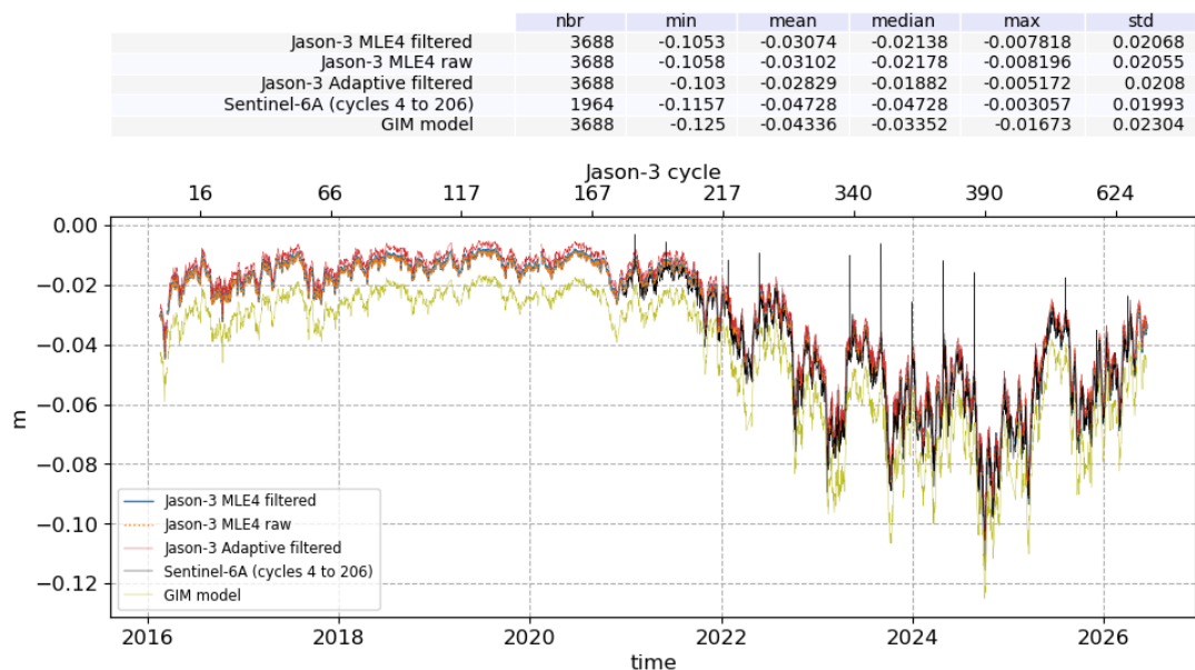
Figure 15: Daily mean of ionosphere correction over cycle 636 for Jason-3 MLE4 and Adaptive, and for Sentinel-6A
