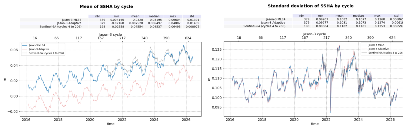
Figure 25: SSHA daily monitoring from cycle 001 to 636, for Jason-3 GDR
