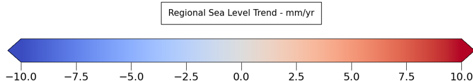
Figure 27: Regional MSL trends from 1999 onwards.
