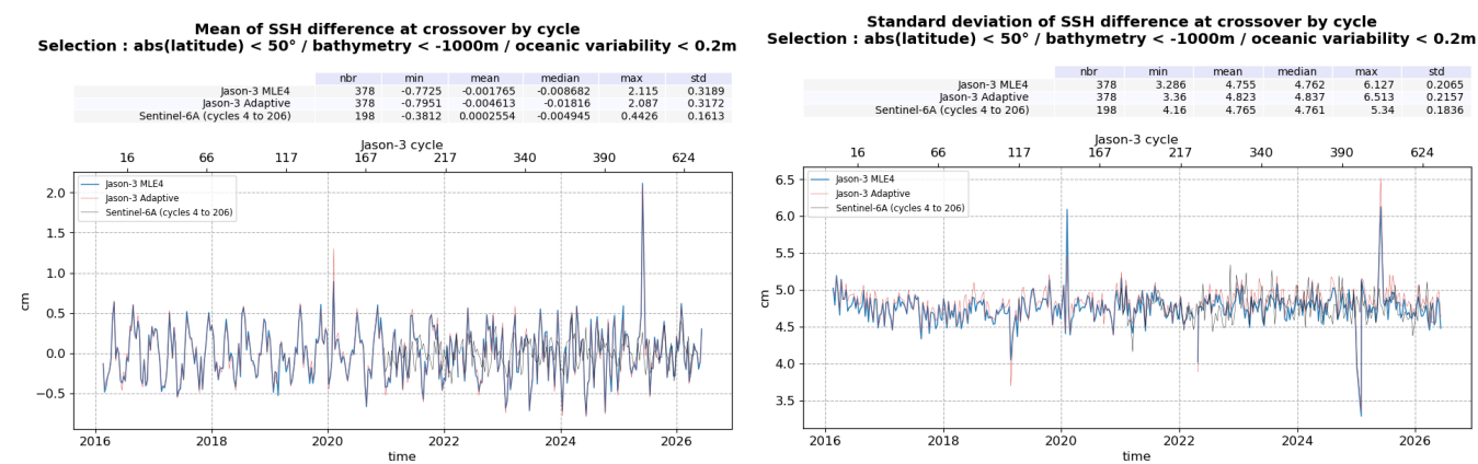
Figure 23: Monitoring of SSH difference at crossovers for Jason-3 MLE4 and Adaptive, and Sentinel-6A LR MLE4 : mean (left) and standard deviation (right), from cycle 001 to 636
