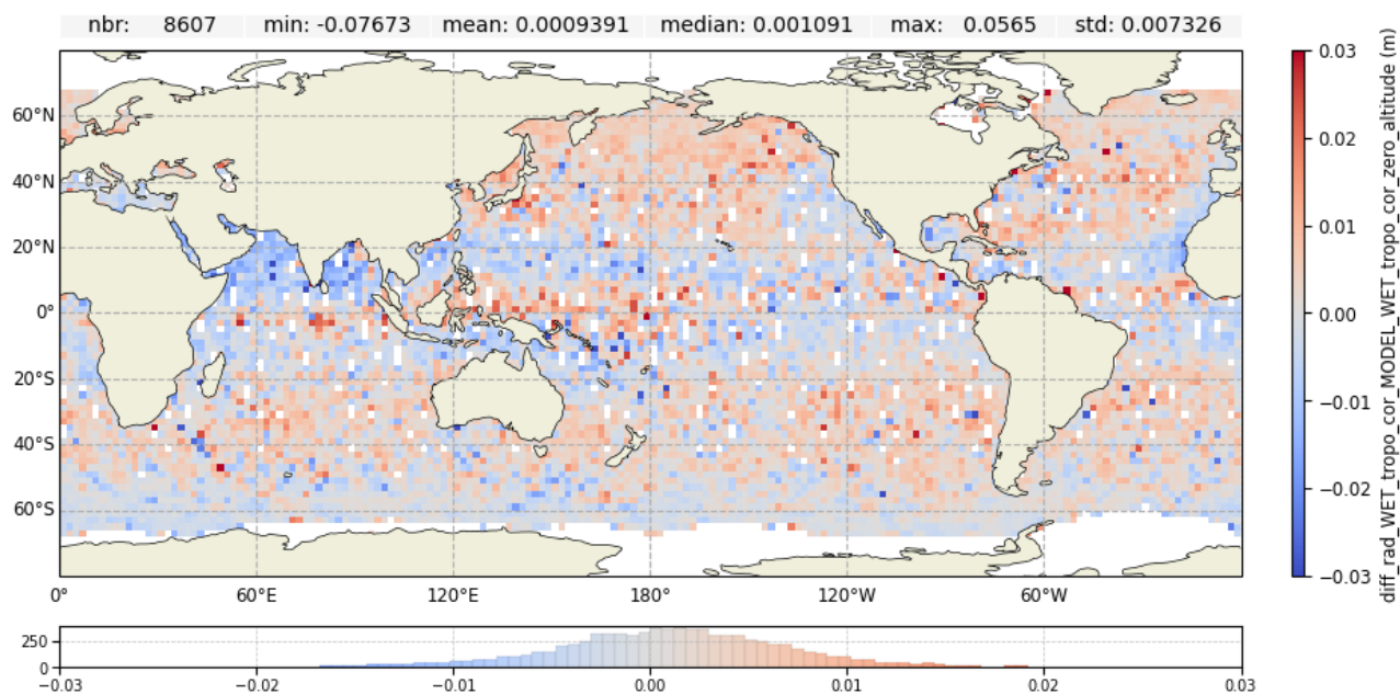
Figure 21: Map of wet tropospheric corrections differences over cycle 636 for Jason-3
