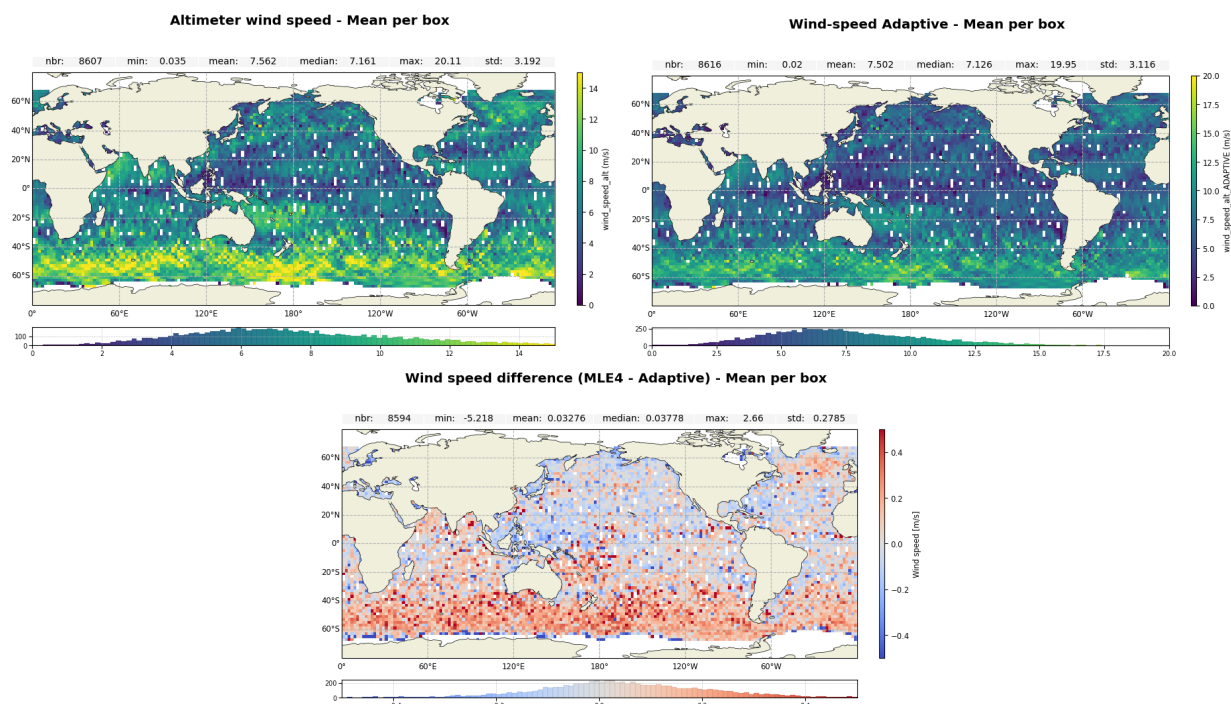
Figure 12: Map of Ku-band wind-speed over cycle 636 for Jason-3 MLE4 (up left), Adaptive (up right) and difference MLE4-Adaptive (down)
