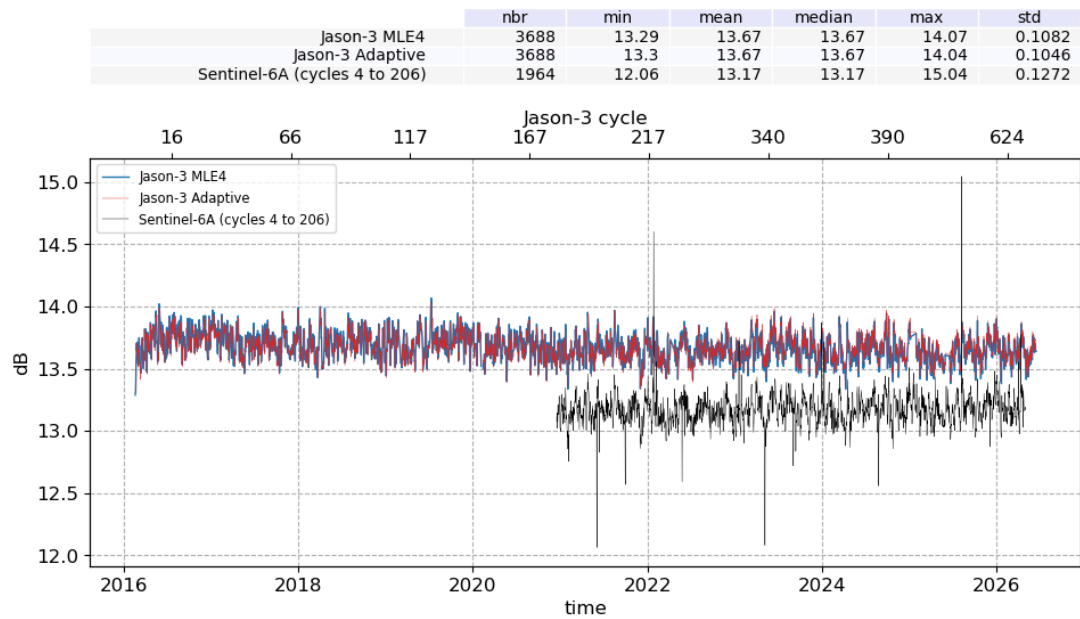
Figure 10: Ku-band Backscattering coefficient daily monitoring from cycle 001 to 636, for Jason-3 and Sentinel-6A
