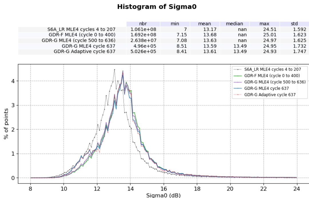
Figure 8: Ku-band Backscattering coefficient histogram computed over cycle 637
