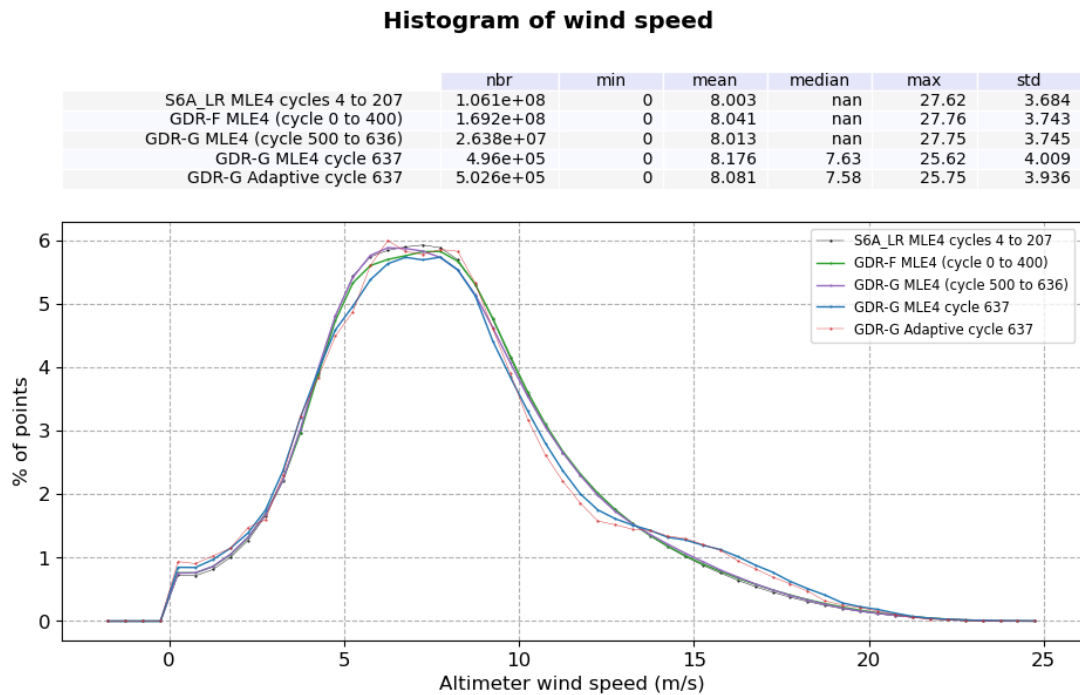
Figure 11: Altimeter Wind Speed histogram computed over cycle 637
