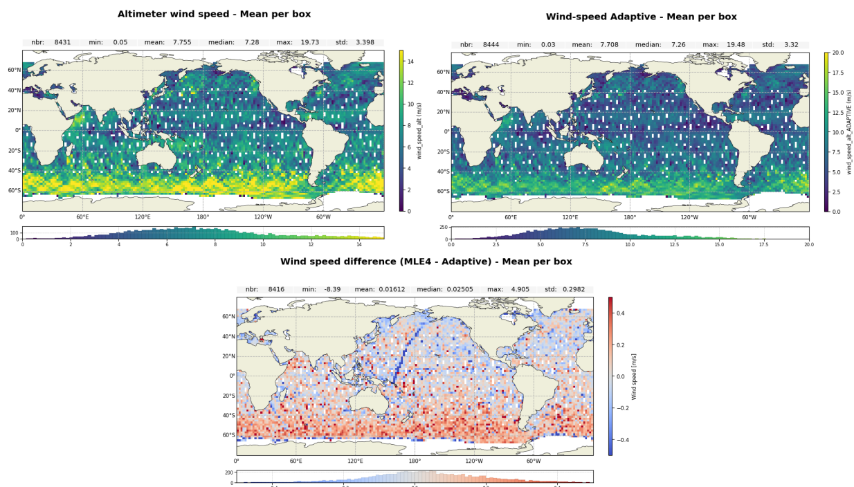
Figure 12: Map of Ku-band wind-speed over cycle 637 for Jason-3 MLE4 (up left), Adaptive (up right) and difference MLE4-Adaptive (down)
