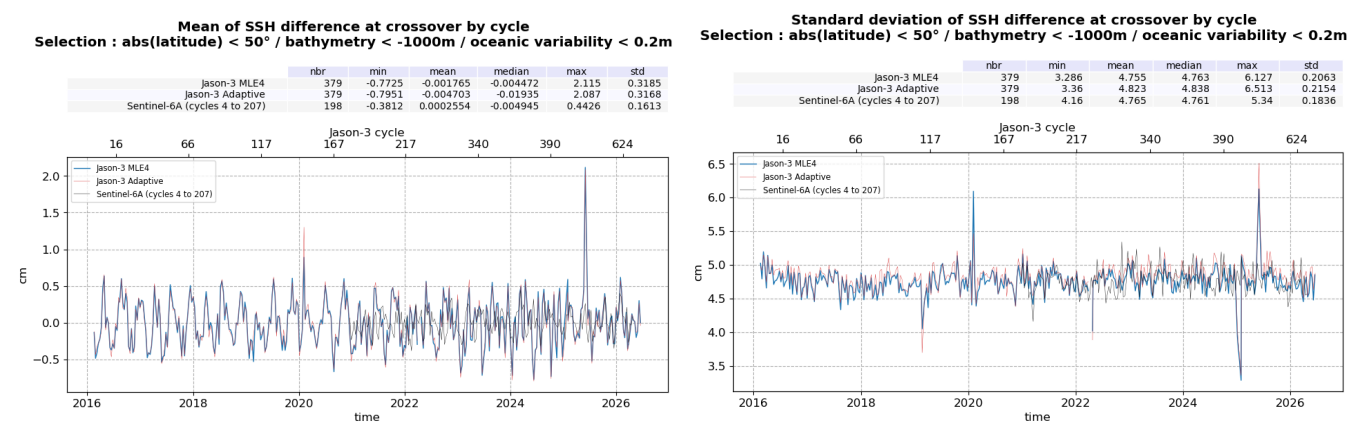
Figure 23: Monitoring of SSH difference at crossovers for Jason-3 MLE4 and Adaptive, and Sentinel-6A LR MLE4 : mean (left) and standard deviation (right), from cycle 001 to 637
