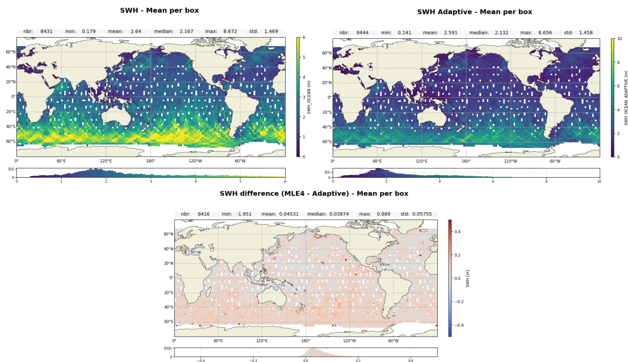
Figure 6: Map of Ku-band Significant Wave Height over cycle 637 for Jason-3 MLE4 (up left), Adaptive (up right) and difference MLE4-Adaptive (down)
