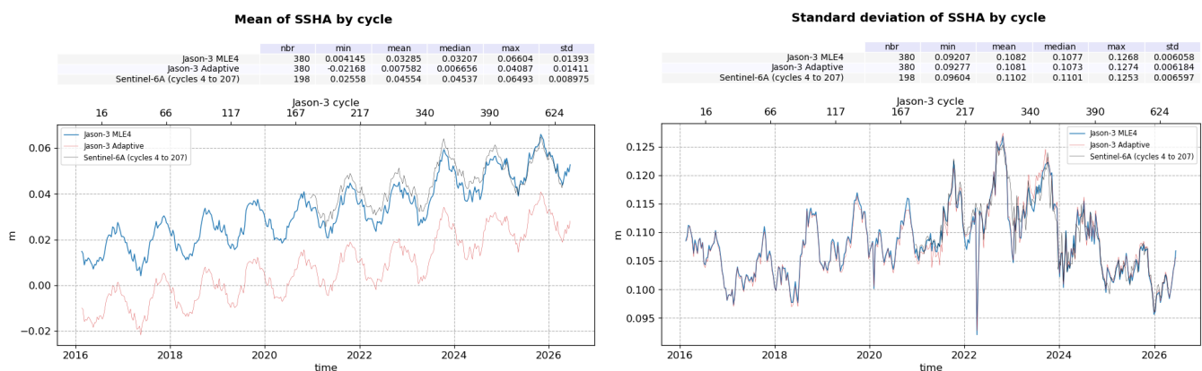
Figure 25: SSHA daily monitoring from cycle 001 to 637, for Jason-3 GDR
