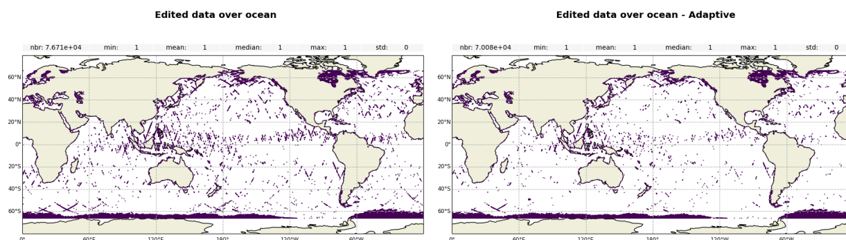
Figure 4: Edited measurements for Jason-3 over cycle 637 for MLE4 (left) and Adaptive (right)
