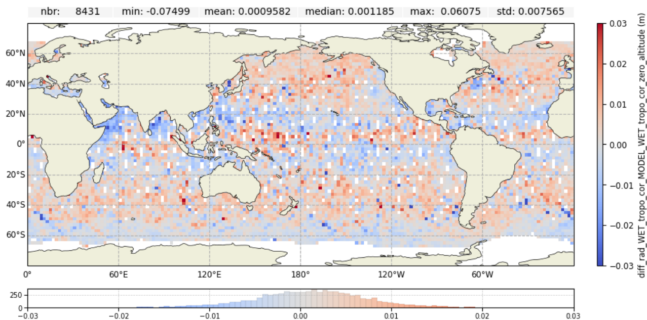
Figure 21: Map of wet tropospheric corrections differences over cycle 637 for Jason-3
