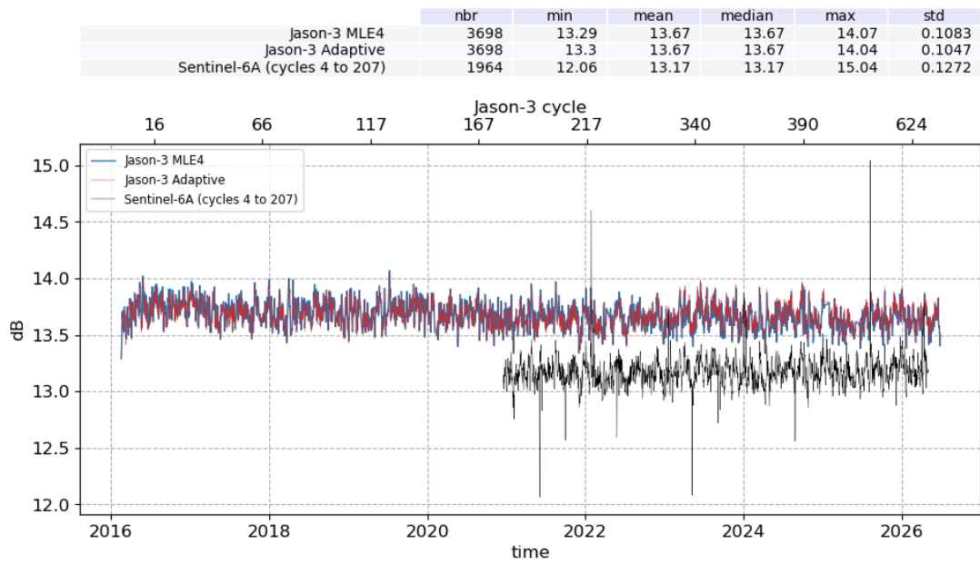
Figure 10: Ku-band Backscattering coefficient daily monitoring from cycle 001 to 637, for Jason-3 and Sentinel-6A
