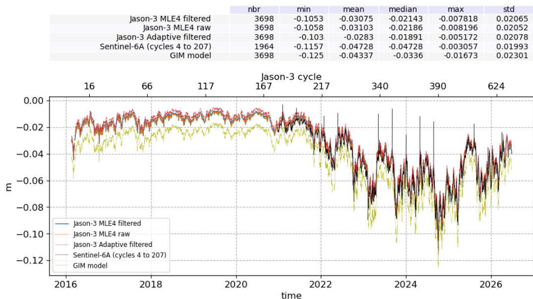
Figure 15: Daily mean of ionosphere correction over cycle 637 for Jason-3 MLE4 and Adaptive, and for Sentinel-6A
