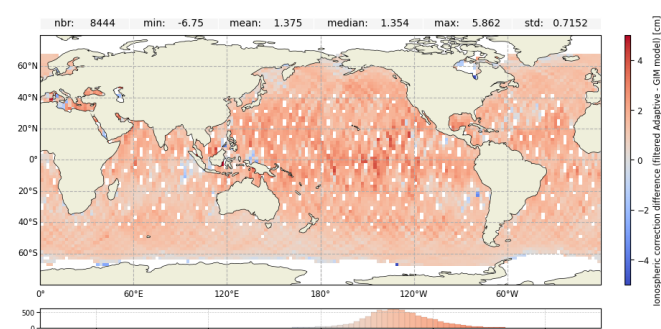
Figure 16: Ionospheric correction difference over cycle 637 for Jason-3 GDR : Filtered MLE4 - GIM model (left) and Filtered Adaptive - GIM model (right)
