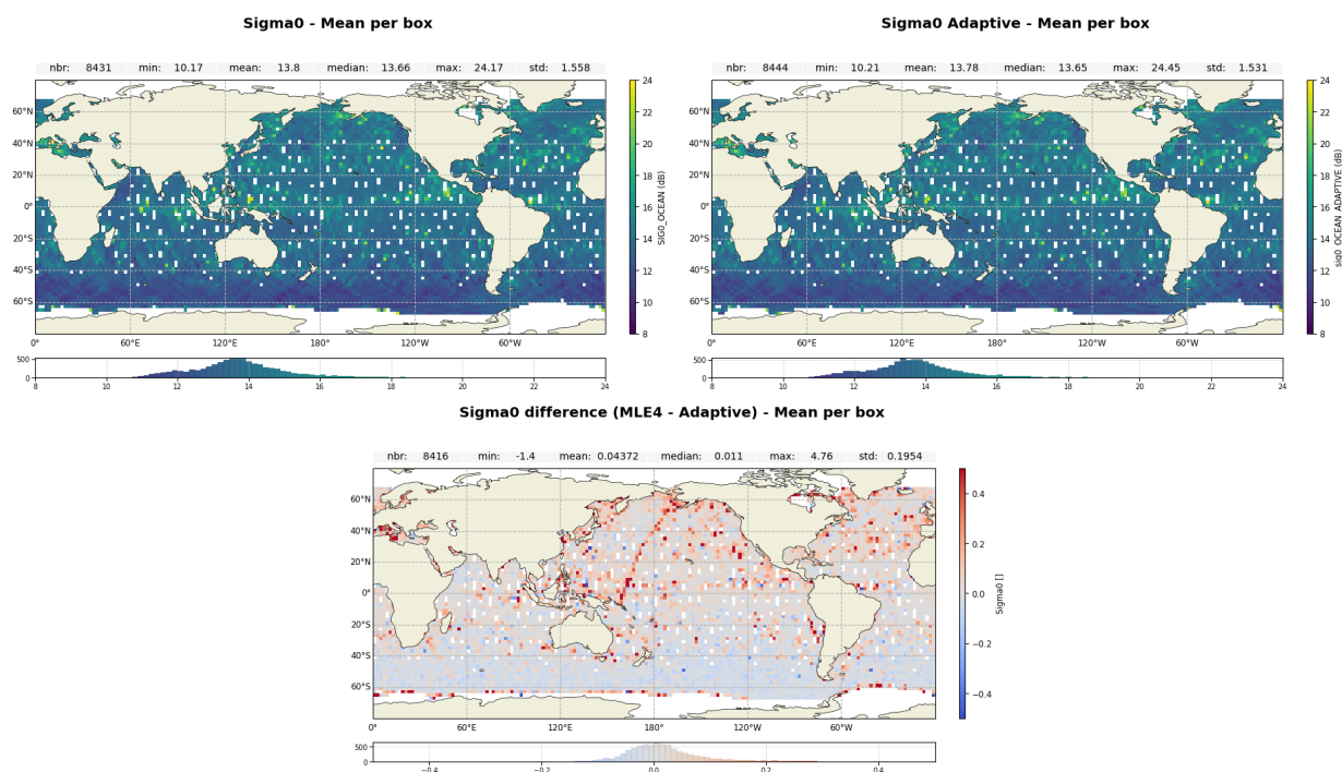
Figure 9: Map of Ku-band backscatter coefficient over cycle 637 for Jason-3 MLE4 (up left), Adaptive (up right) and difference MLE4-Adaptive (down)
