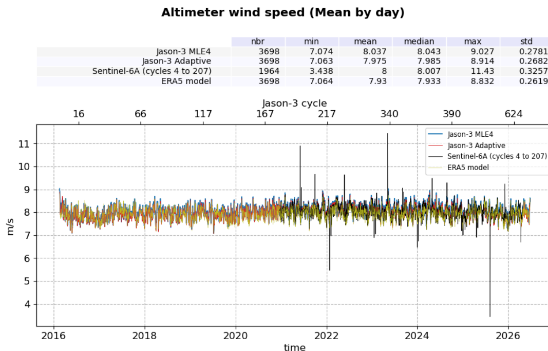
Figure 13: Wind Speed daily monitoring from cycle 001 to 637 for Jason-3 GDR, and Sentinel-6A (LR MLE4)
