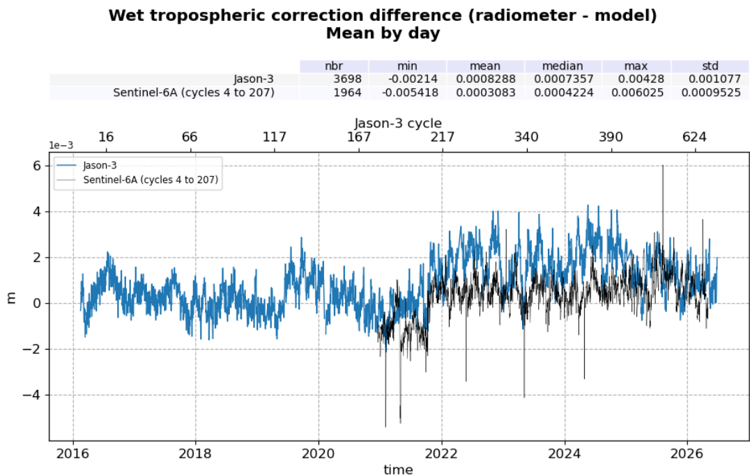
Figure 19: Daily monitoring of mean wet tropospheric correction difference computed from cycle 001 to cycle 637
