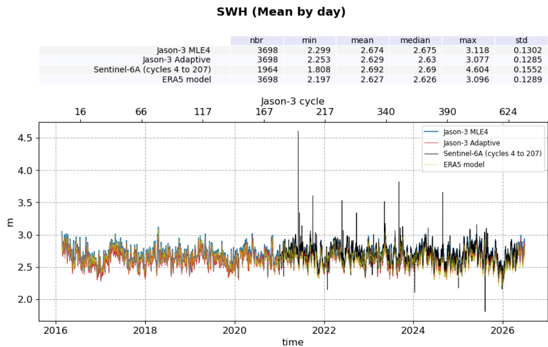
Figure 7: Ku-band Significant Wave Height daily monitoring from cycle 001 to 637, for Jason-3 and Sentinel-6A
