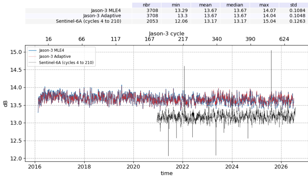
Figure 10: Ku-band Backscattering coefficient daily monitoring from cycle 001 to 700, for Jason-3 and Sentinel-6A
