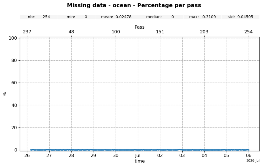
Figure 3: Monitoring of the percentage per pass of missing data over ocean for Jason-3 GDR cycle 700
