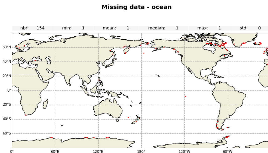
Figure 2: Map of missing measurements over ocean for Jason-3 GDR cycle 700
