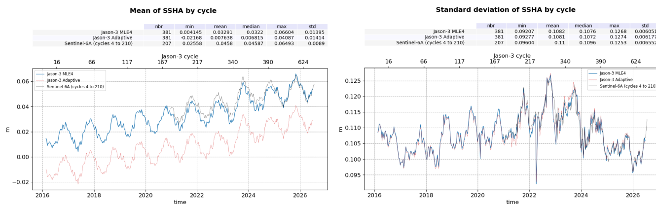
Figure 25: SSHA daily monitoring from cycle 001 to 700, for Jason-3 GDR
