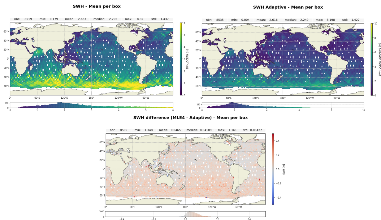
Figure 6: Map of Ku-band Significant Wave Height over cycle 700 for Jason-3 MLE4 (up left), Adaptive (up right) and difference MLE4-Adaptive (down)
