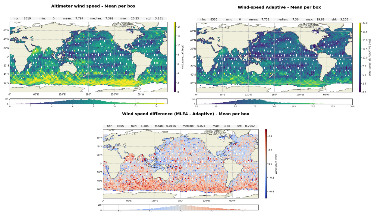
Figure 12: Map of Ku-band wind-speed over cycle 700 for Jason-3 MLE4 (up left), Adaptive (up right) and difference MLE4-Adaptive (down)
