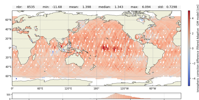
Figure 16: Ionospheric correction difference over cycle 700 for Jason-3 GDR : Filtered MLE4 - GIM model (left) and Filtered Adaptive - GIM model (right)
