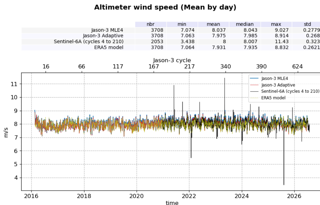
Figure 13: Wind Speed daily monitoring from cycle 001 to 700 for Jason-3 GDR, and Sentinel-6A (LR MLE4)
