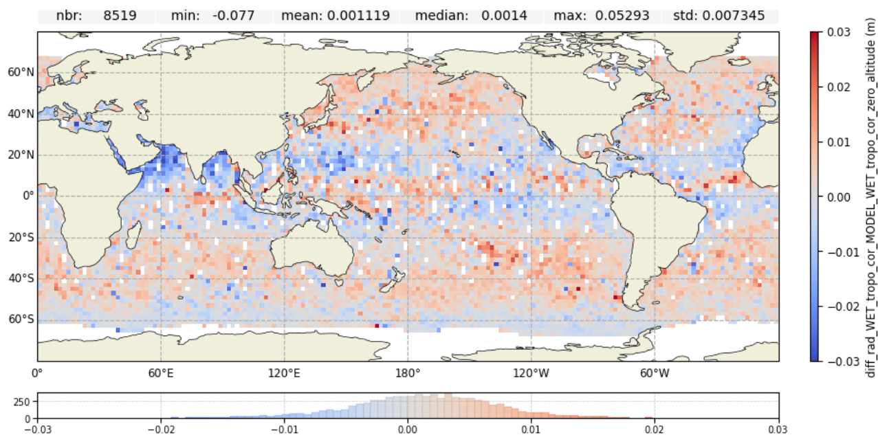
Figure 21: Map of wet tropospheric corrections differences over cycle 700 for Jason-3
