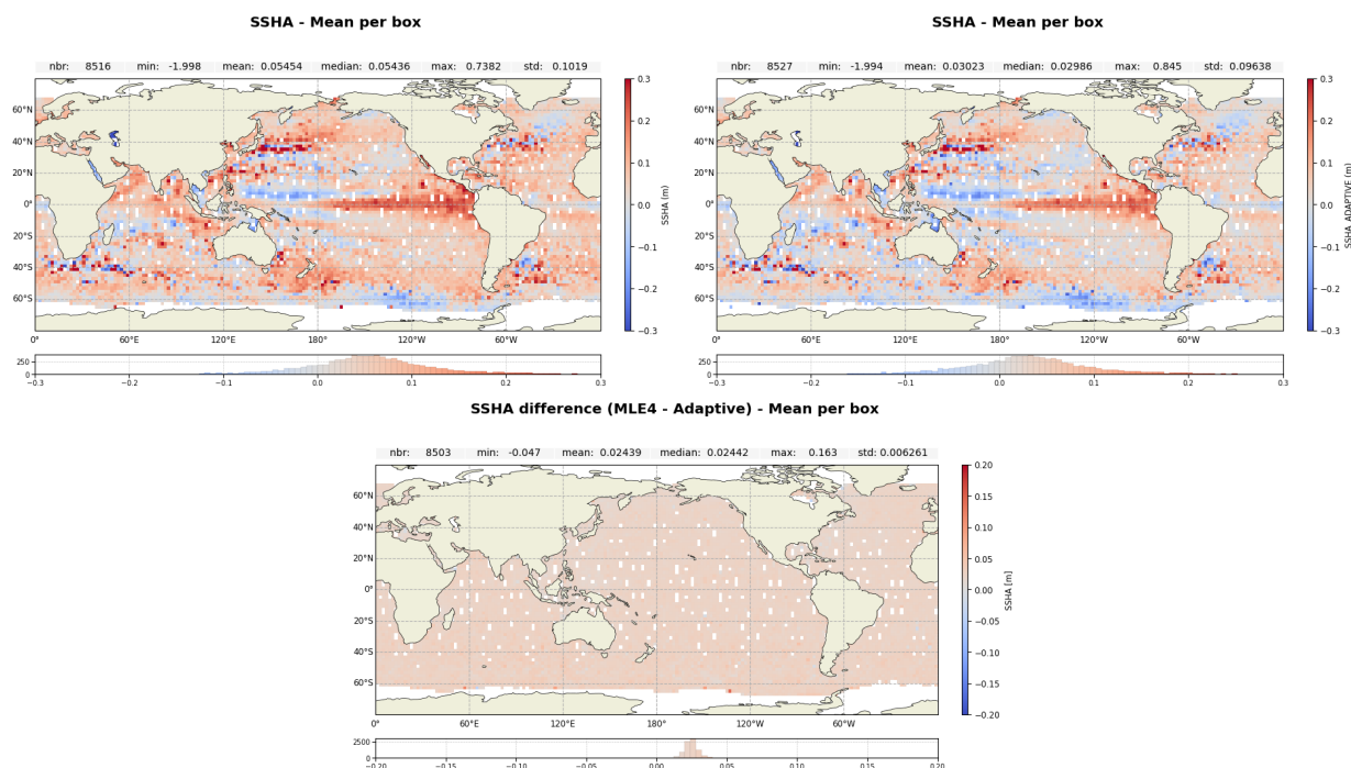
Figure 24: Along-track maps of SSHA over cycle 700 for Jason-3 MLE4 (up left), Adaptive (up right) and difference MLE4-Adaptive (down)
