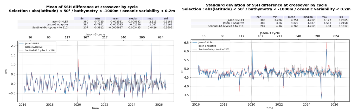
Figure 23: Monitoring of SSH difference at crossovers for Jason-3 MLE4 and Adaptive, and Sentinel-6A LR MLE4 : mean (left) and standard deviation (right), from cycle 001 to 700
