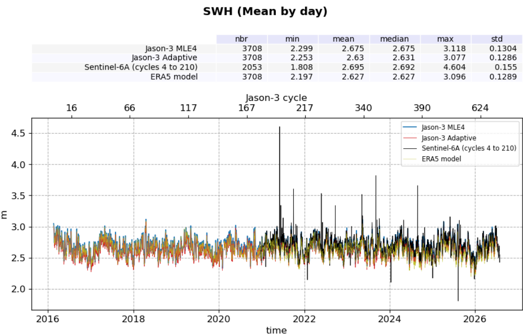
Figure 7: Ku-band Significant Wave Height daily monitoring from cycle 001 to 700, for Jason-3 and Sentinel-6A
