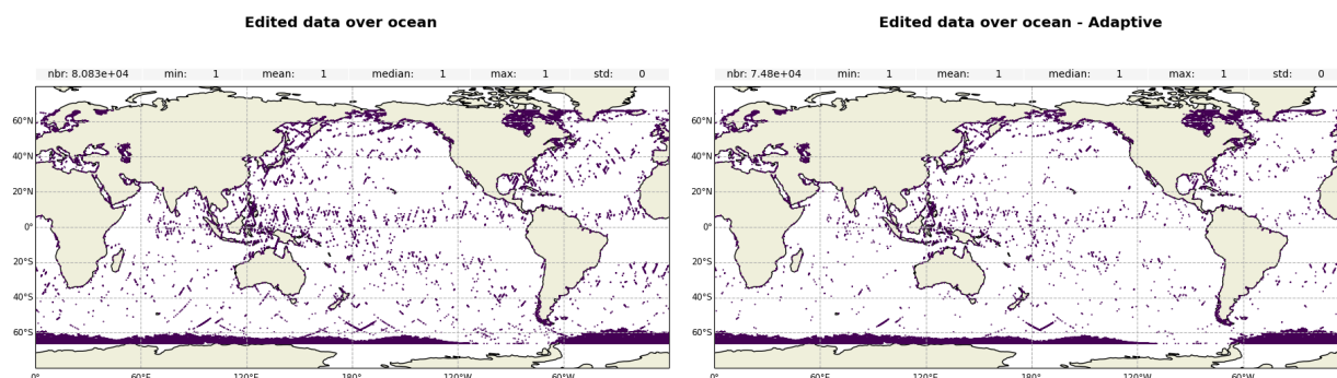
Figure 4: Edited measurements for Jason-3 over cycle 700 for MLE4 (left) and Adaptive (right)
