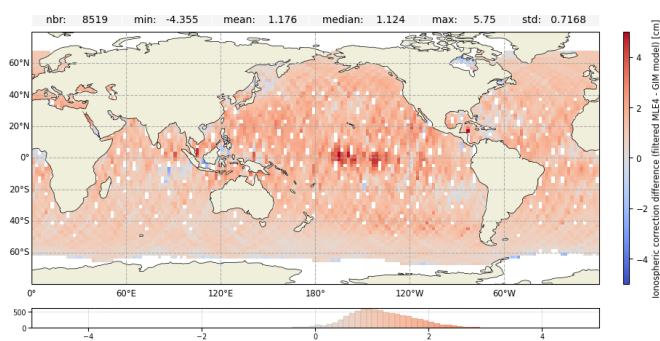
Figure 16: Ionospheric correction difference over cycle 700 for Jason-3 GDR : Filtered MLE4 - GIM model (left) and Filtered Adaptive - GIM model (right)
