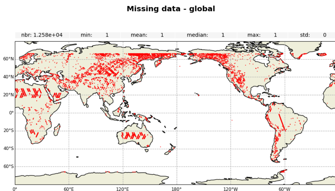
Figure 1: Map of missing measurements for Jason-3 GDR cycle 700
