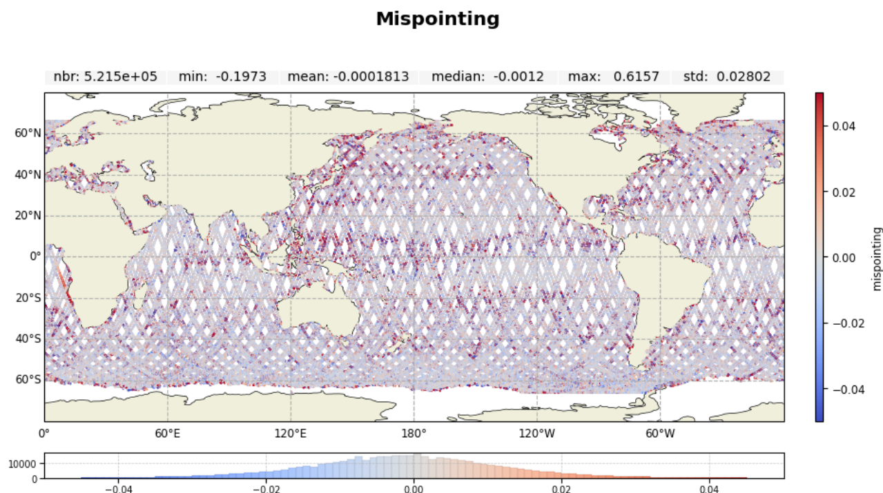
Figure 17: Along-track map of mispointing over cycle 700 for Jason-3 MLE4
