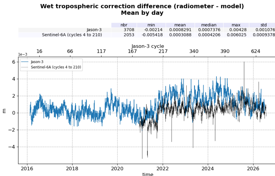
Figure 19: Daily monitoring of mean wet tropospheric correction difference computed from cycle 001 to cycle 700
