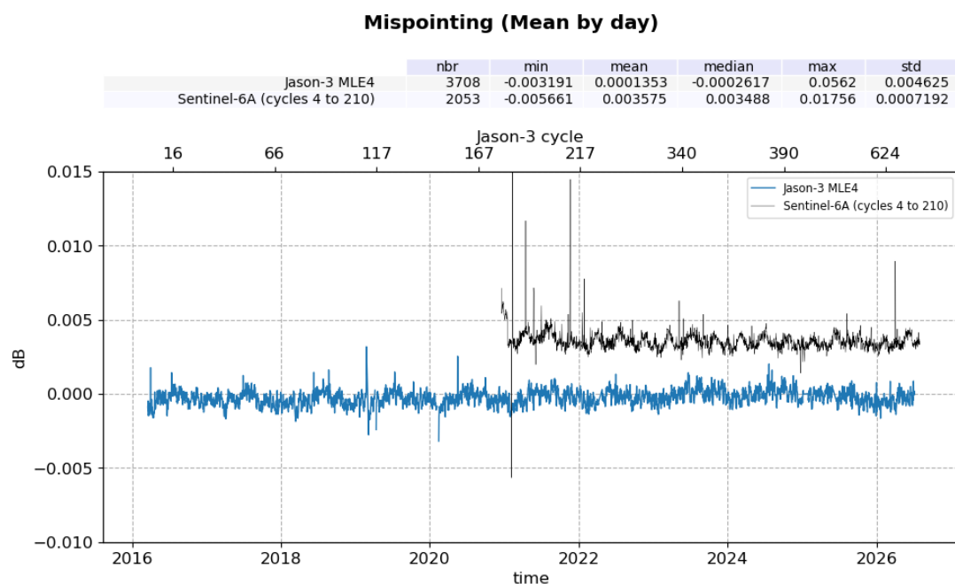
Figure 18: Mispointing daily monitoring from cycle 001 to 700 for Jason-3 GDR and Sentinel-6A
