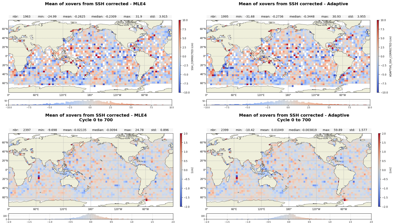
Figure 22: Mean SSH difference at crossovers for Jason-3 MLE4 (left) and Adaptive (right) cycle 700 (top) and from cycle 001 to cycle 700 (bottom)
