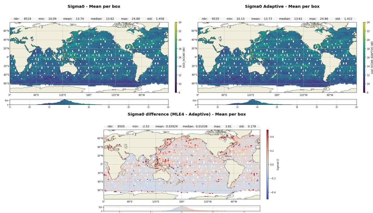
Figure 9: Map of Ku-band backscatter coefficient over cycle 700 for Jason-3 MLE4 (up left), Adaptive (up right) and difference MLE4-Adaptive (down)
