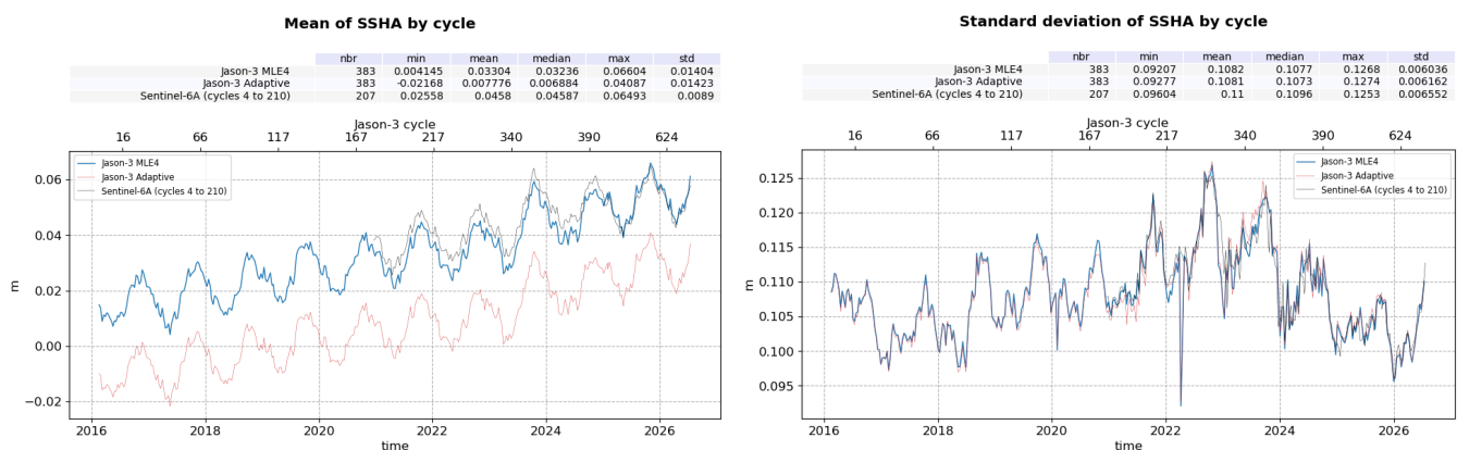
Figure 25: SSHA daily monitoring from cycle 001 to 702, for Jason-3 GDR
