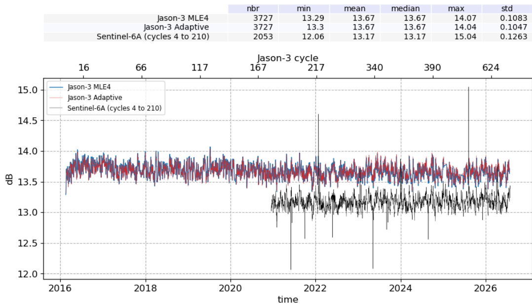
Figure 10: Ku-band Backscattering coefficient daily monitoring from cycle 001 to 702, for Jason-3 and Sentinel-6A
