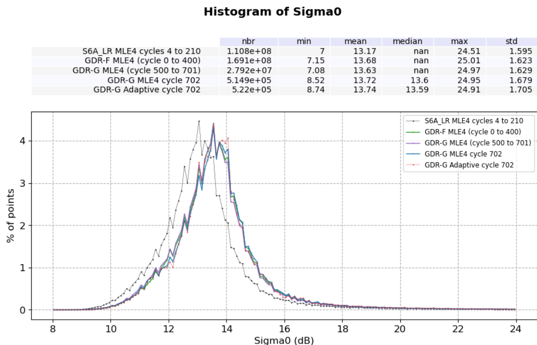
Figure 8: Ku-band Backscattering coefficient histogram computed over cycle 702
