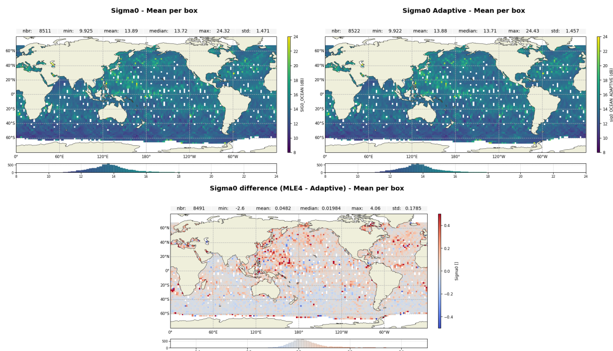
Figure 9: Map of Ku-band backscatter coefficient over cycle 702 for Jason-3 MLE4 (up left), Adaptive (up right) and difference MLE4-Adaptive (down)
