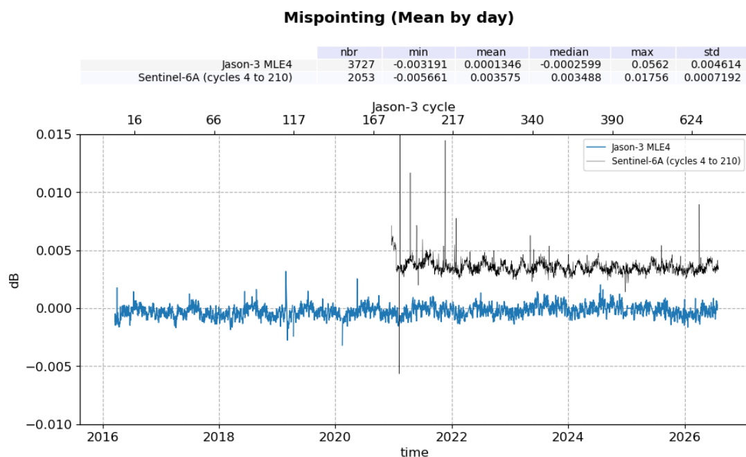
Figure 18: Mispointing daily monitoring from cycle 001 to 702 for Jason-3 GDR and Sentinel-6A
