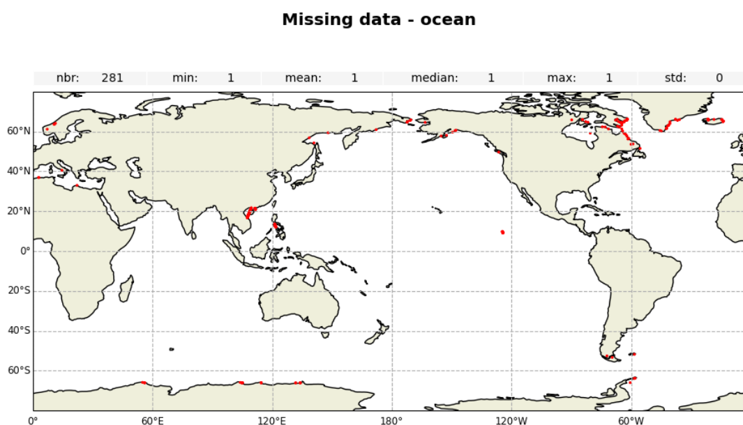
Figure 2: Map of missing measurements over ocean for Jason-3 GDR cycle 702
