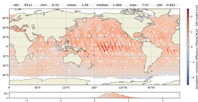
Figure 16: Ionospheric correction difference over cycle 702 for Jason-3 GDR : Filtered MLE4 - GIM model (left) and Filtered Adaptive - GIM model (right)
