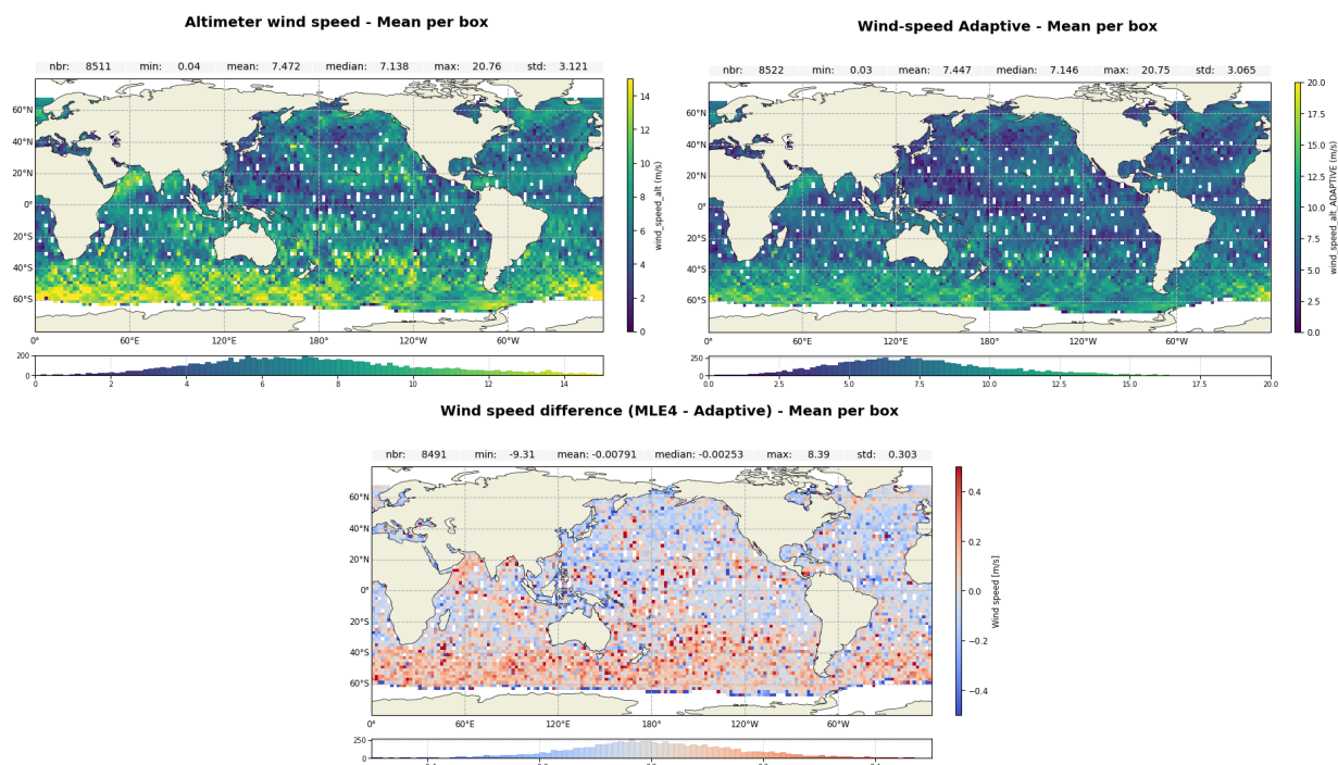
Figure 12: Map of Ku-band wind-speed over cycle 702 for Jason-3 MLE4 (up left), Adaptive (up right) and difference MLE4-Adaptive (down)
