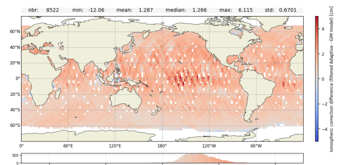
Figure 16: Ionospheric correction difference over cycle 702 for Jason-3 GDR : Filtered MLE4 - GIM model (left) and Filtered Adaptive - GIM model (right)
