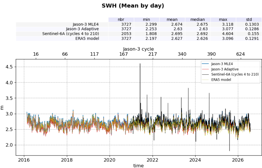
Figure 7: Ku-band Significant Wave Height daily monitoring from cycle 001 to 702, for Jason-3 and Sentinel-6A
