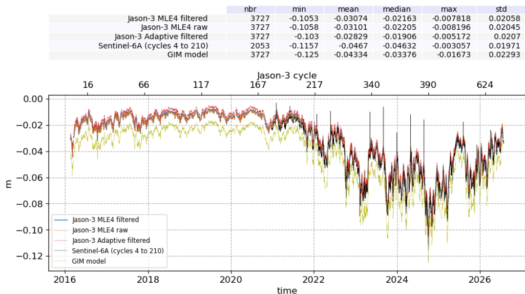
Figure 15: Daily mean of ionosphere correction over cycle 702 for Jason-3 MLE4 and Adaptive, and for Sentinel-6A
