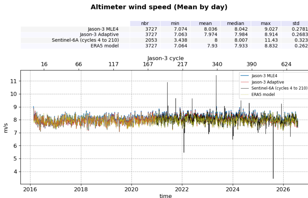
Figure 13: Wind Speed daily monitoring from cycle 001 to 702 for Jason-3 GDR, and Sentinel-6A (LR MLE4)
