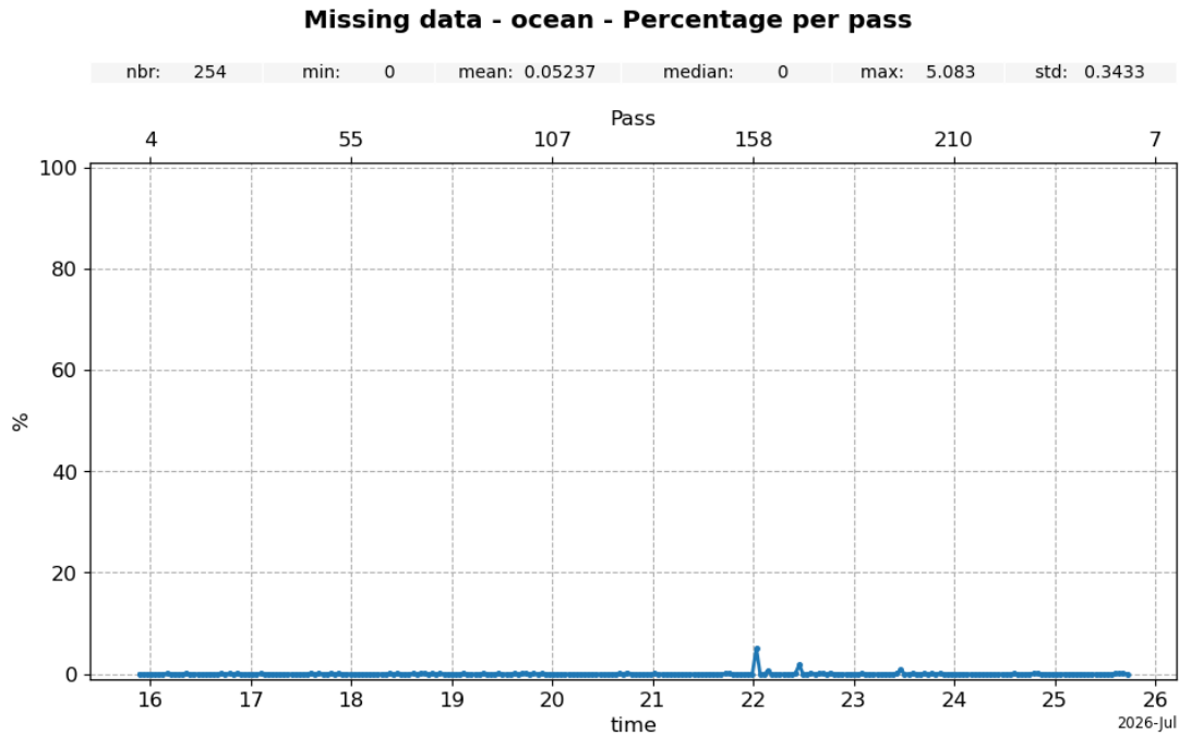
Figure 3: Monitoring of the percentage per pass of missing data over ocean for Jason-3 GDR cycle 702
