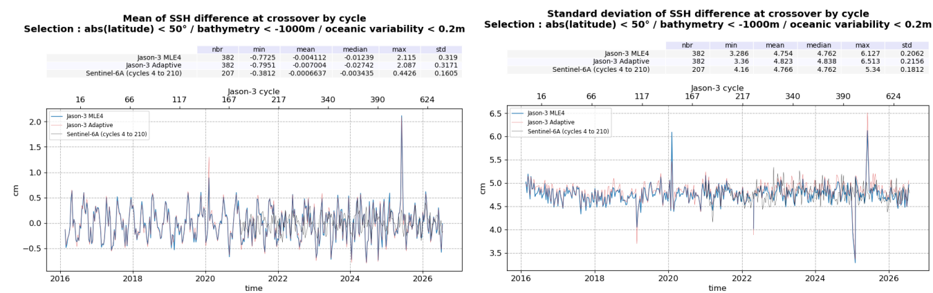
Figure 23: Monitoring of SSH difference at crossovers for Jason-3 MLE4 and Adaptive, and Sentinel-6A LR MLE4 : mean (left) and standard deviation (right), from cycle 001 to 702
