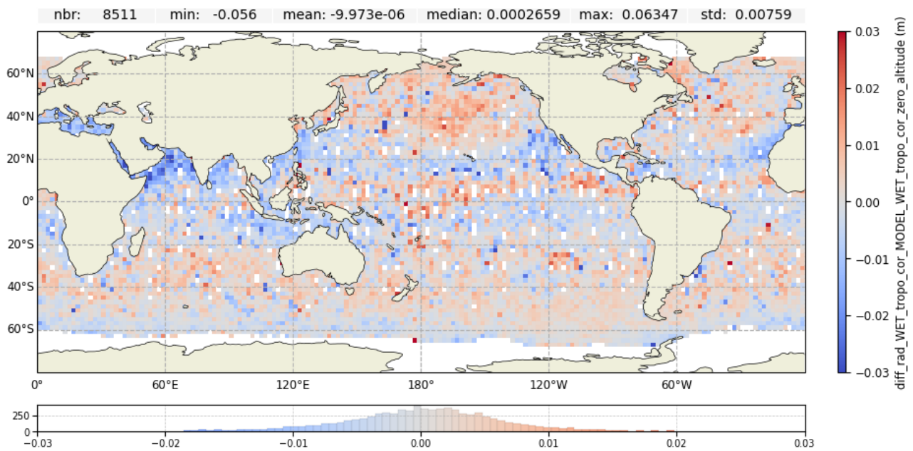
Figure 21: Map of wet tropospheric corrections differences over cycle 702 for Jason-3
