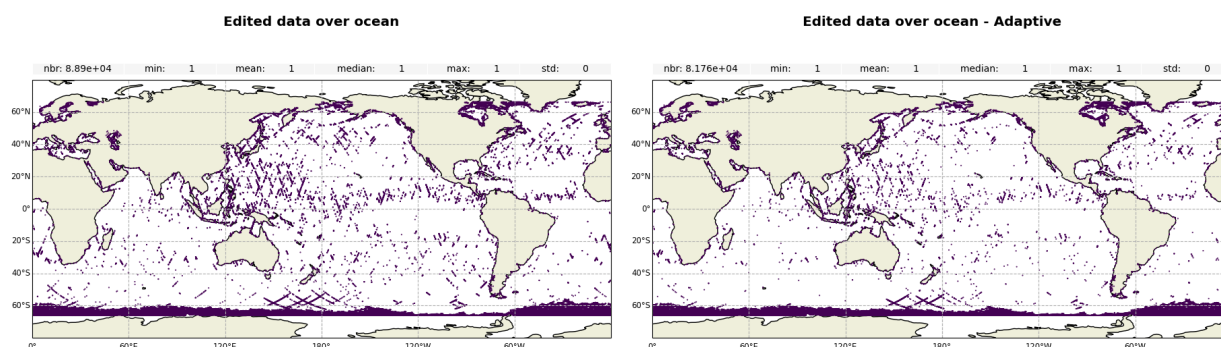
Figure 4: Edited measurements for Jason-3 over cycle 702 for MLE4 (left) and Adaptive (right)
