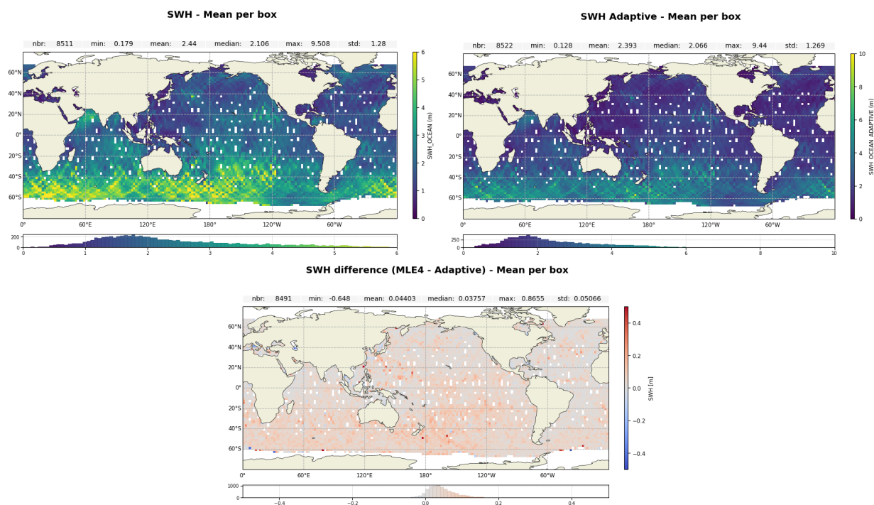
Figure 6: Map of Ku-band Significant Wave Height over cycle 702 for Jason-3 MLE4 (up left), Adaptive (up right) and difference MLE4-Adaptive (down)
