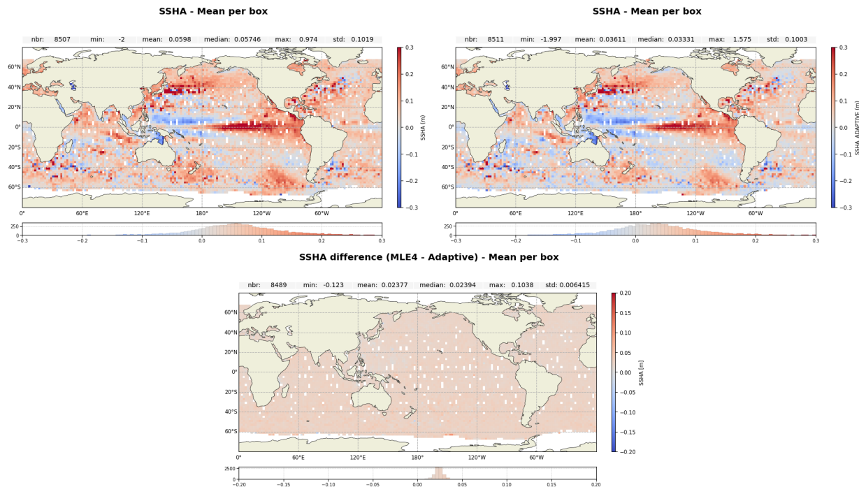
Figure 24: Along-track maps of SSHA over cycle 702 for Jason-3 MLE4 (up left), Adaptive (up right) and difference MLE4-Adaptive (down)
