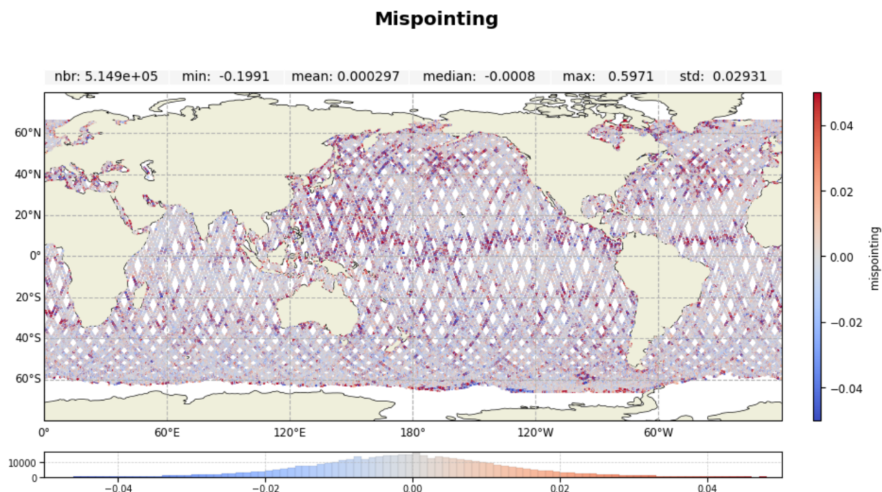
Figure 17: Along-track map of mispointing over cycle 702 for Jason-3 MLE4
