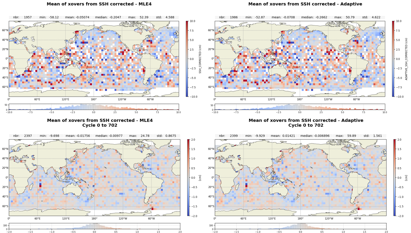
Figure 22: Mean SSH difference at crossovers for Jason-3 MLE4 (left) and Adaptive (right) cycle 702 (top) and from cycle 001 to cycle 702 (bottom)
