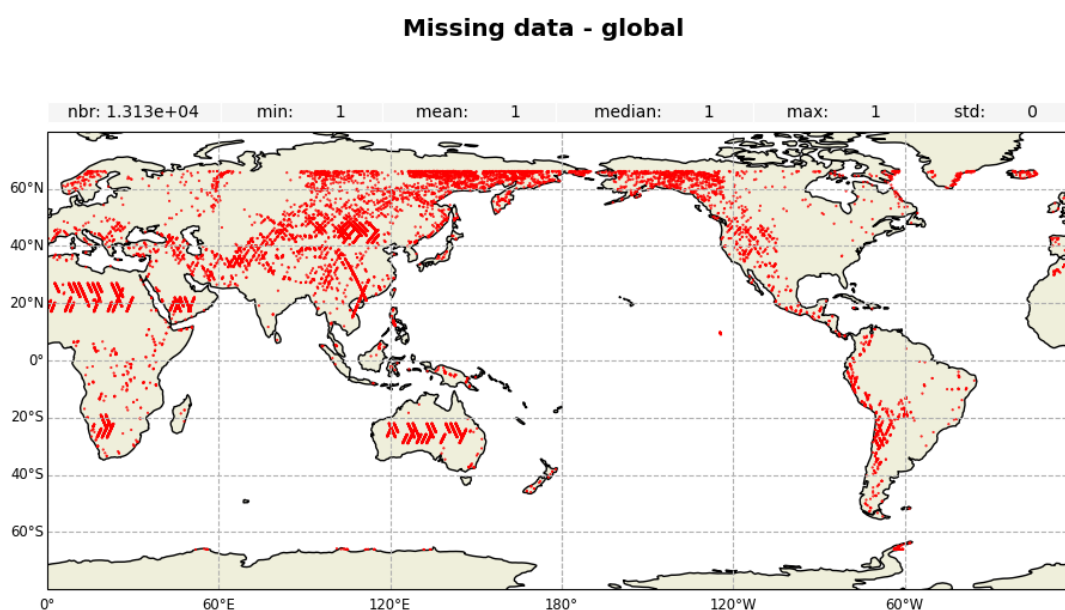
Figure 1: Map of missing measurements for Jason-3 GDR cycle 702
