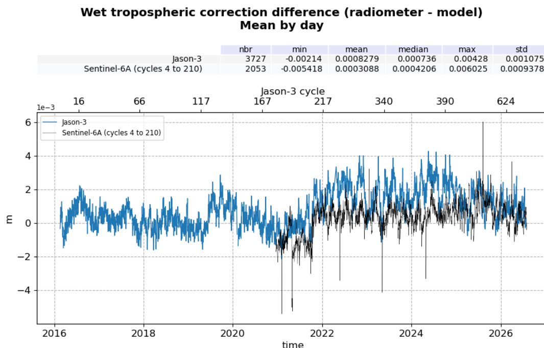
Figure 19: Daily monitoring of mean wet tropospheric correction difference computed from cycle 001 to cycle 702
