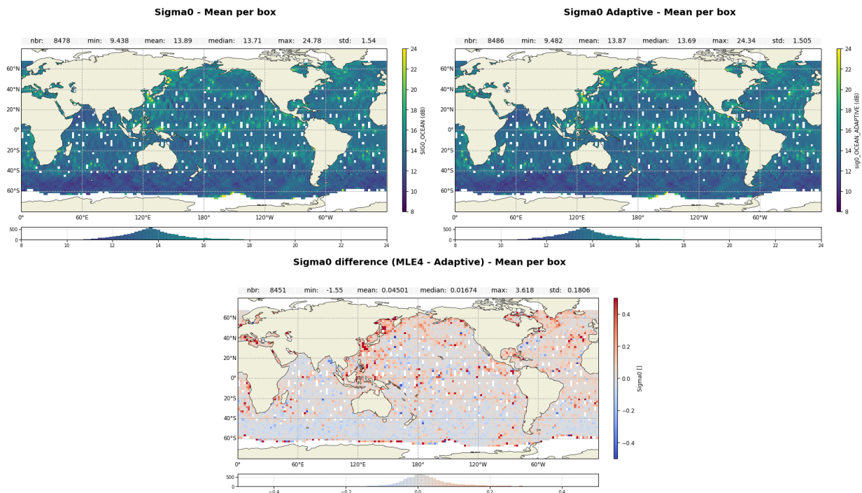
Figure 9: Map of Ku-band backscatter coefficient over cycle 703 for Jason-3 MLE4 (up left), Adaptive (up right) and difference MLE4-Adaptive (down)
