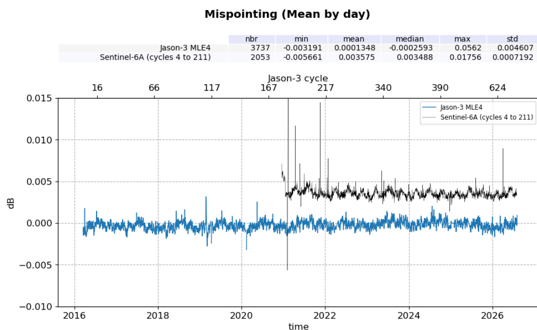
Figure 18: Mispointing daily monitoring from cycle 001 to 703 for Jason-3 GDR and Sentinel-6A
