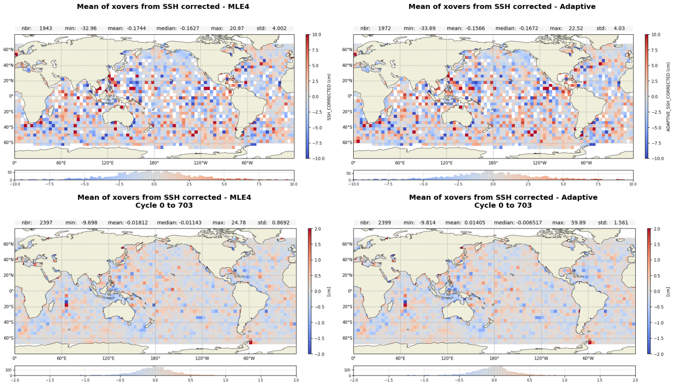
Figure 22: Mean SSH difference at crossovers for Jason-3 MLE4 (left) and Adaptive (right) cycle 703 (top) and from cycle 001 to cycle 703 (bottom)
