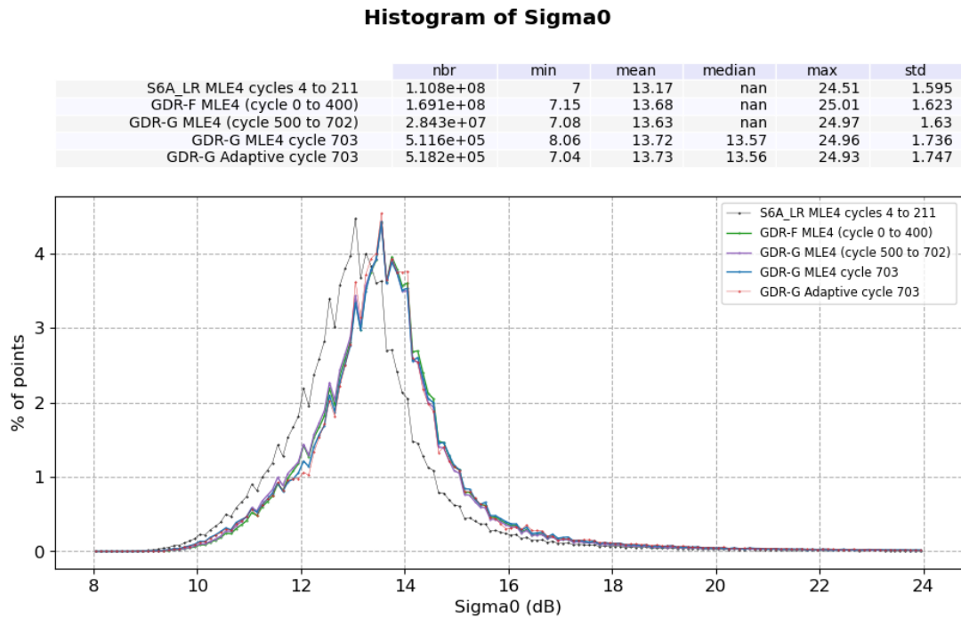
Figure 8: Ku-band Backscattering coefficient histogram computed over cycle 703
