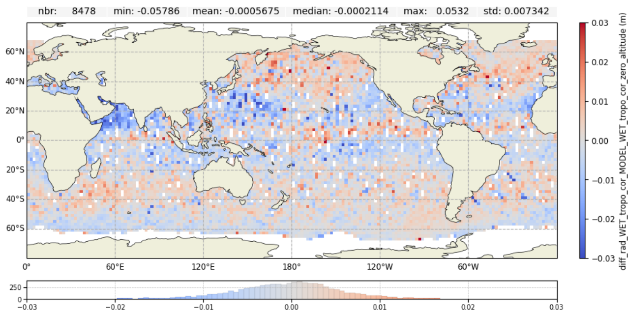
Figure 21: Map of wet tropospheric corrections differences over cycle 703 for Jason-3
