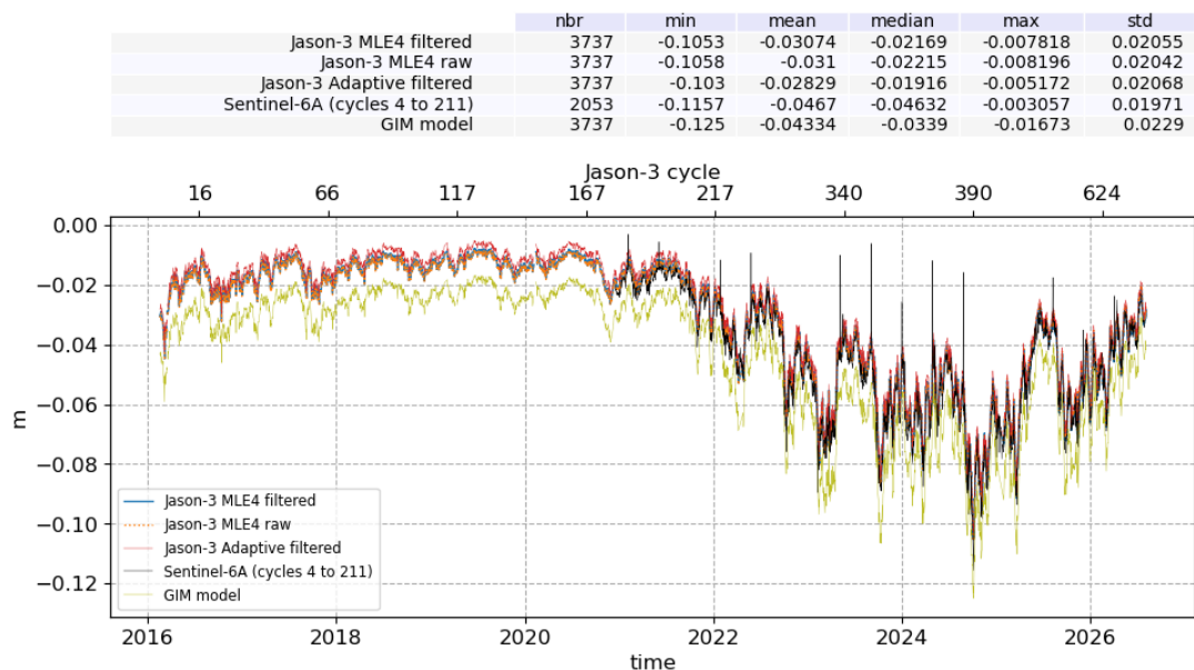
Figure 15: Daily mean of ionosphere correction over cycle 703 for Jason-3 MLE4 and Adaptive, and for Sentinel-6A
