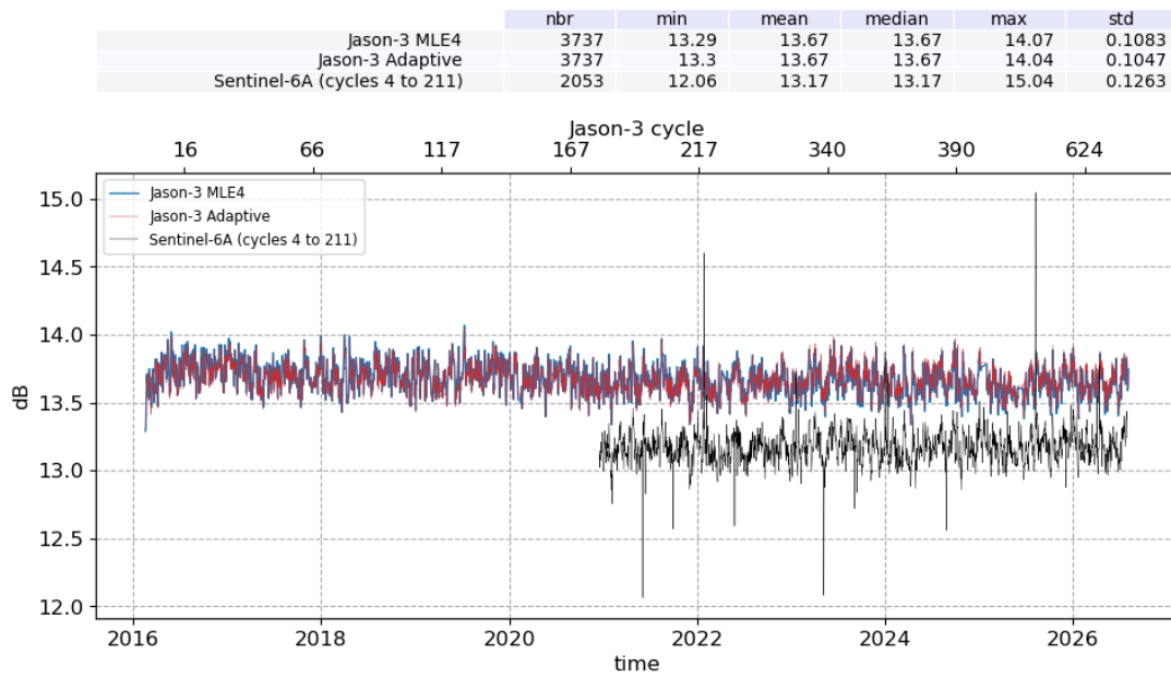
Figure 10: Ku-band Backscattering coefficient daily monitoring from cycle 001 to 703, for Jason-3 and Sentinel-6A
