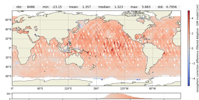
Figure 16: Ionospheric correction difference over cycle 703 for Jason-3 GDR : Filtered MLE4 - GIM model (left) and Filtered Adaptive - GIM model (right)
