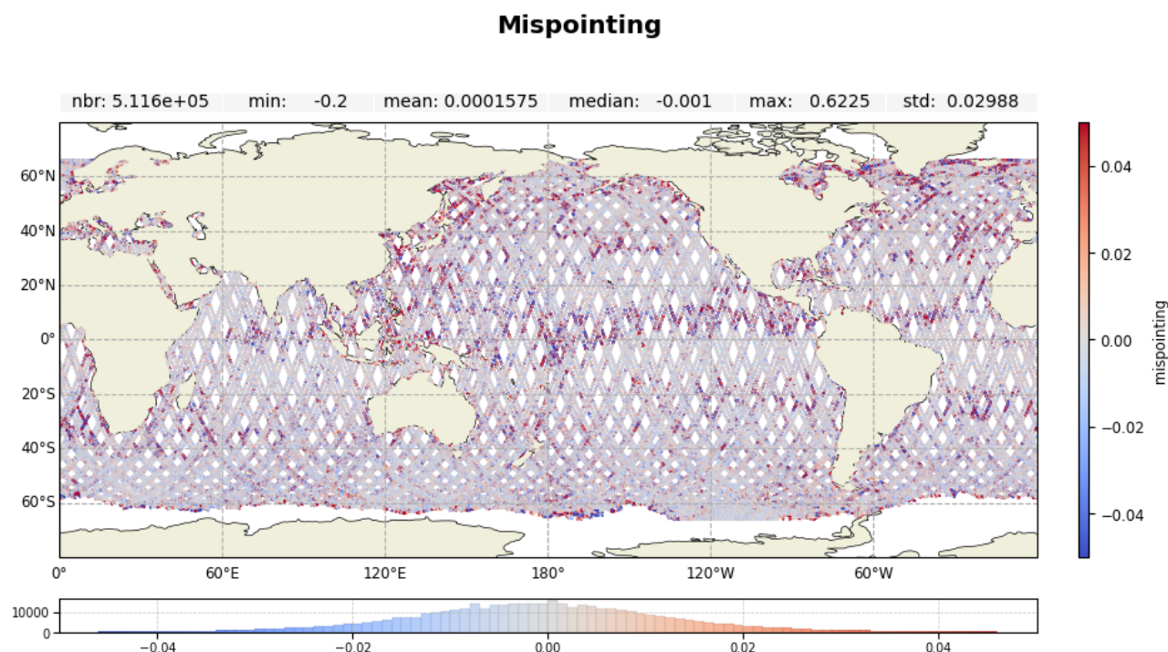
Figure 17: Along-track map of mispointing over cycle 703 for Jason-3 MLE4
