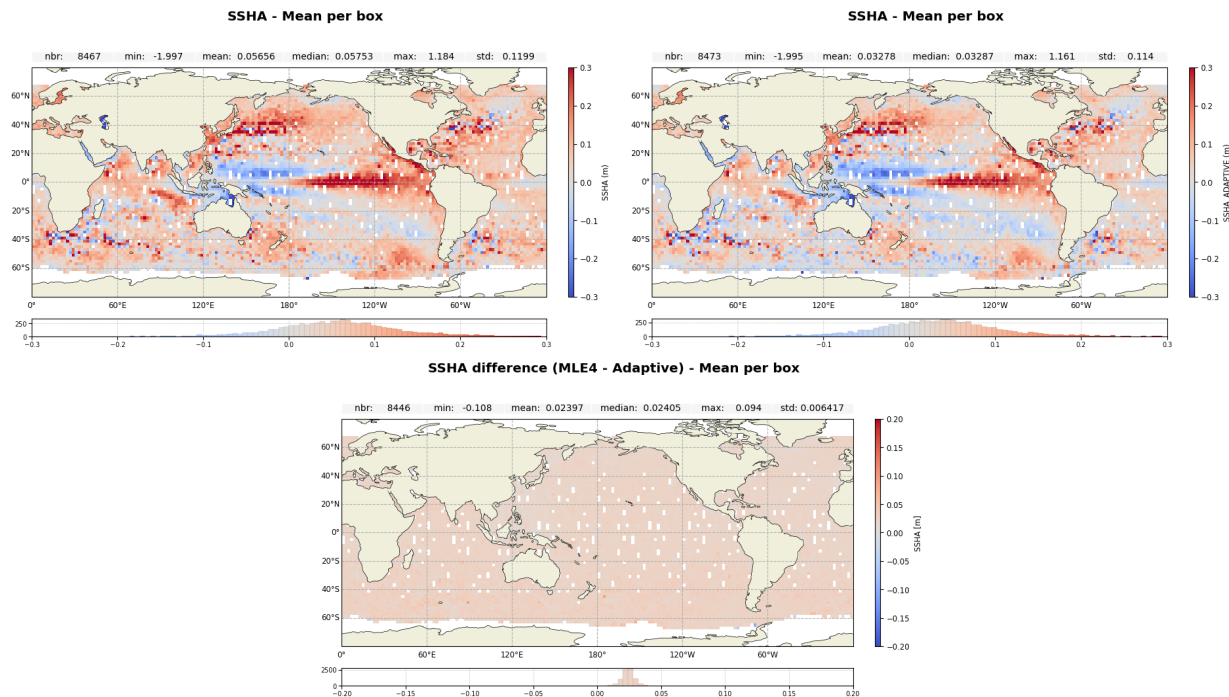
Figure 24: Along-track maps of SSHA over cycle 703 for Jason-3 MLE4 (up left), Adaptive (up right) and difference MLE4-Adaptive (down)
