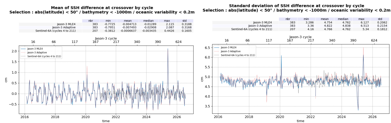
Figure 23: Monitoring of SSH difference at crossovers for Jason-3 MLE4 and Adaptive, and Sentinel-6A LR MLE4 : mean (left) and standard deviation (right), from cycle 001 to 703
