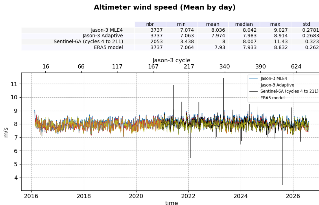
Figure 13: Wind Speed daily monitoring from cycle 001 to 703 for Jason-3 GDR, and Sentinel-6A (LR MLE4)
