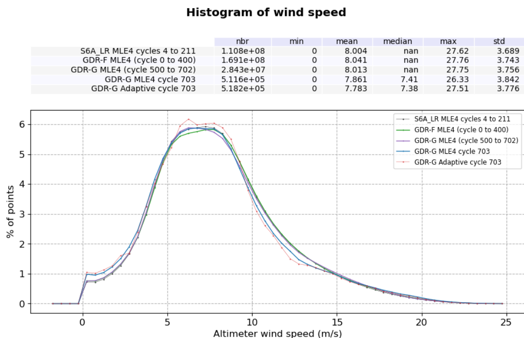
Figure 11: Altimeter Wind Speed histogram computed over cycle 703
