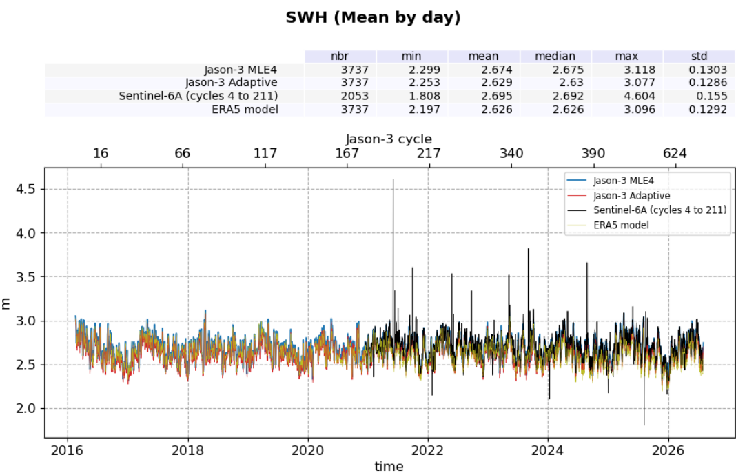
Figure 7: Ku-band Significant Wave Height daily monitoring from cycle 001 to 703, for Jason-3 and Sentinel-6A
