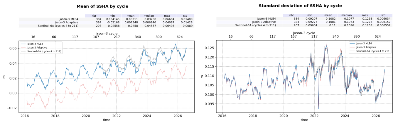
Figure 25: SSHA daily monitoring from cycle 001 to 703, for Jason-3 GDR
