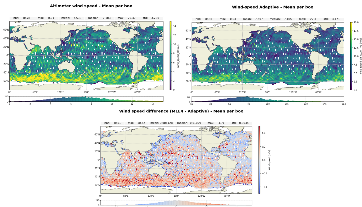
Figure 12: Map of Ku-band wind-speed over cycle 703 for Jason-3 MLE4 (up left), Adaptive (up right) and difference MLE4-Adaptive (down)
