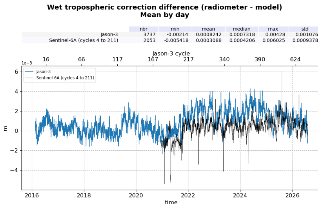
Figure 19: Daily monitoring of mean wet tropospheric correction difference computed from cycle 001 to cycle 703
