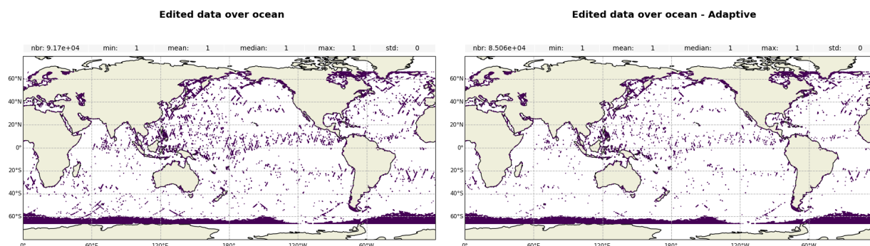
Figure 4: Edited measurements for Jason-3 over cycle 703 for MLE4 (left) and Adaptive (right)
