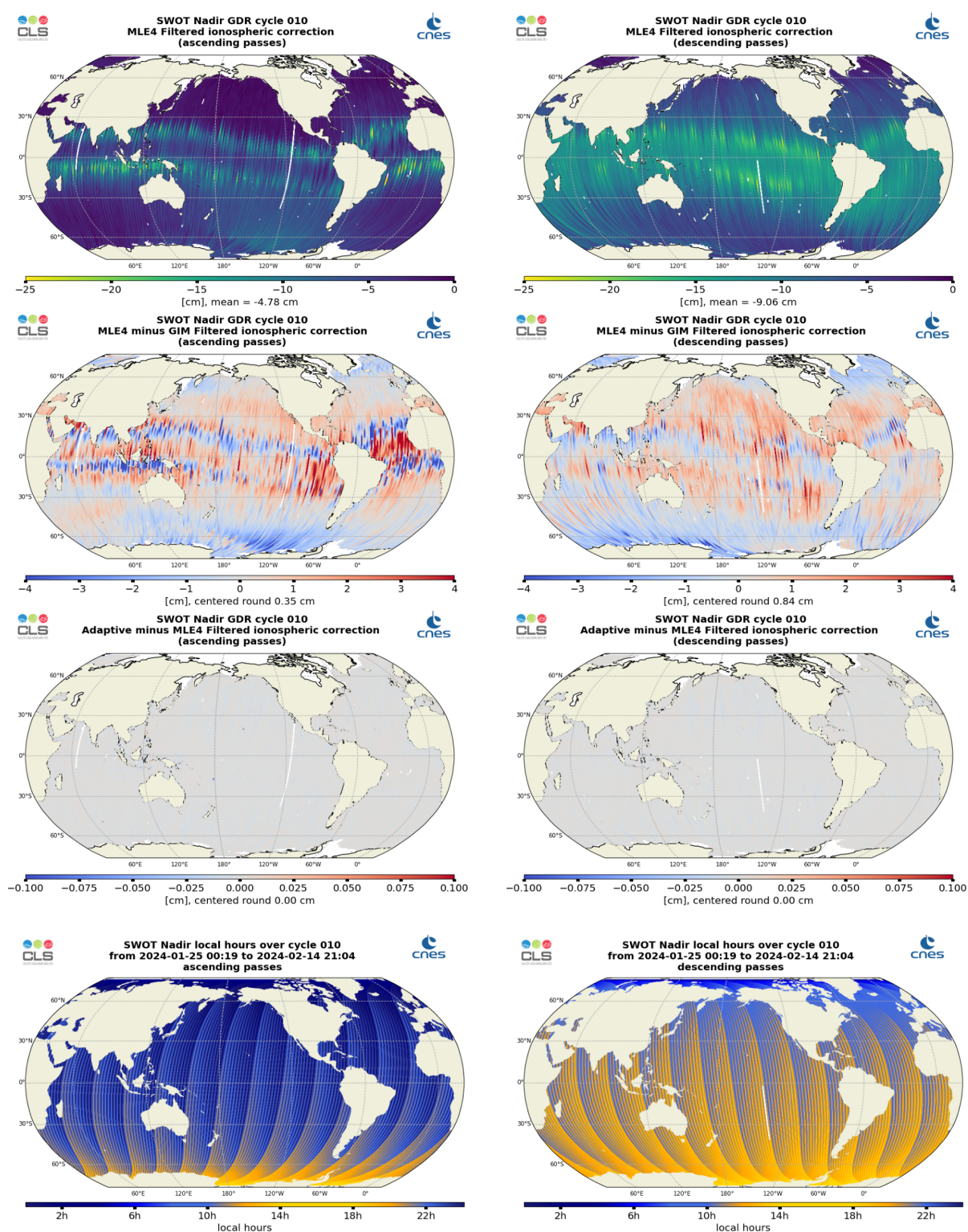
Figure 14: Along-track maps of filtered ionosphere correction over cycle 010 for SWOT Nadir MLE4 (top), MLE4 minus GIM (middle top) or Adaptive minus MLE4 (middle bottom), and local hours (bottom), for ascending passes (left) and descending passes (right)
