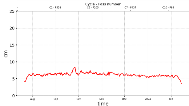
Figure 28: Daily monitoring of SSH difference at crossovers between SWOT Nadir MLE4 and Sentinel-6 MF LR MLE4 from cycle 001 onwards : mean (left) and standard deviation (right)
