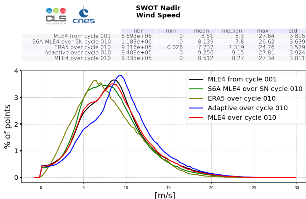
Figure 10: Altimeter Wind Speed histogram computed over cycle 010 (red line for SWOT Nadir MLE4 and blue line for SWOT Nadir Adaptive, green for Sentinel-6A-MF (LR MLE4)) and from cycle 001 (SWOT Nadir, MLE4 only, black line)
