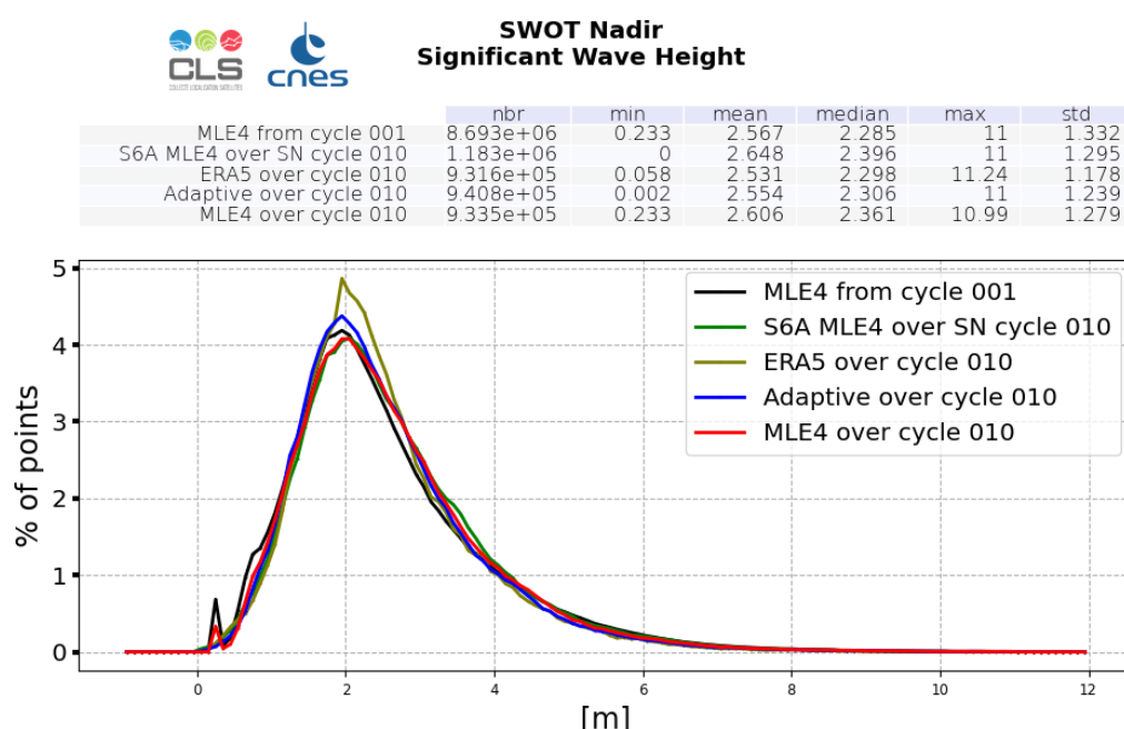
Figure 4: Ku-band Significant Wave Height histogram computed over cycle 010 (red line for SWOT Nadir MLE4 and blue line for SWOT Nadir Adaptive, green for Sentinel-6A-MF (LR MLE4) and dark green for ERA5) and from cycle 001 (SWOT Nadir, MLE4 only, black line)
