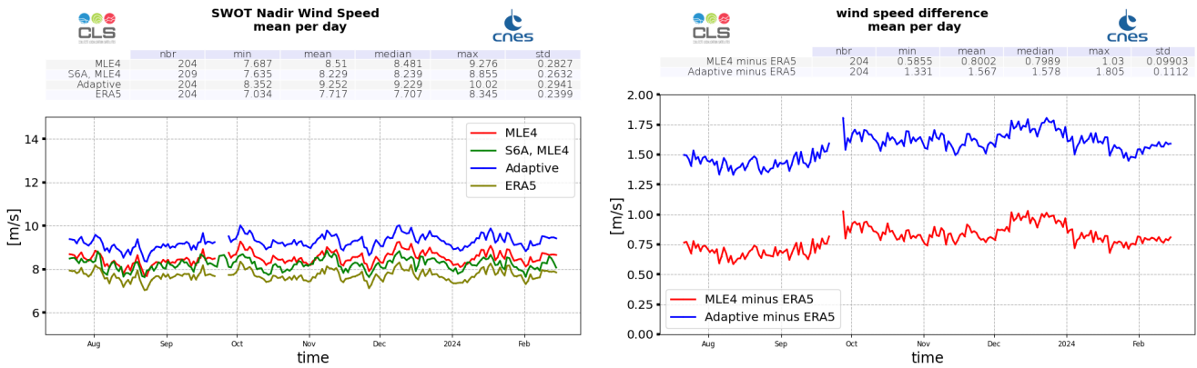
Figure 12: Wind Speed daily monitoring from cycle 001 to 010 for SWOT Nadir GDR, ERA5 model, and Sentinel-6A-MF (LR MLE4) (left), and daily mean difference with ERA5 (right)
