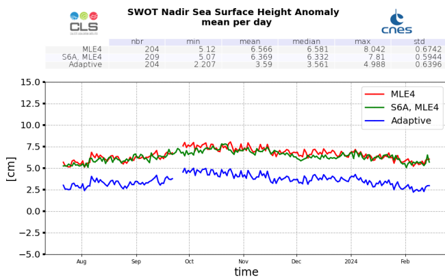
Figure 24: SSHA daily monitoring from cycle 001 to 010, for SWOT Nadir GDR
