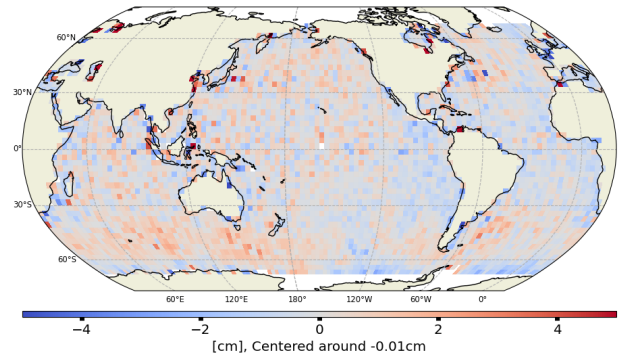
Figure 27: Mean SSH difference at crossovers between SWOT Nadir MLE4 and Sentinel-6 MF LR MLE4 over cycle 010 (left) and from cycle 001 onwards (right)
