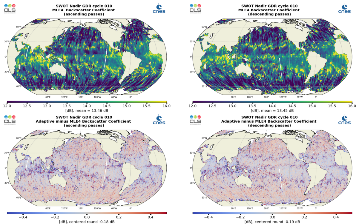
Figure 8: Along-track maps of Ku-band backscatter coefficient \sigma_0 over cycle 010 for SWOT Nadir MLE4 (top) or Adaptive minus MLE4 difference (bottom), ascending passes (left) and descending passes (right)
