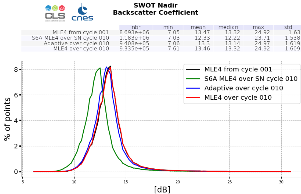
Figure 7: Ku-band Backscattering coefficient histogram computed over cycle 010 (red line for SWOT Nadir MLE4 and blue line for SWOT Nadir Adaptive, green for Sentinel-6A-MF (LR MLE4)) and from cycle 001 (SWOT Nadir, MLE4 only, black line)
