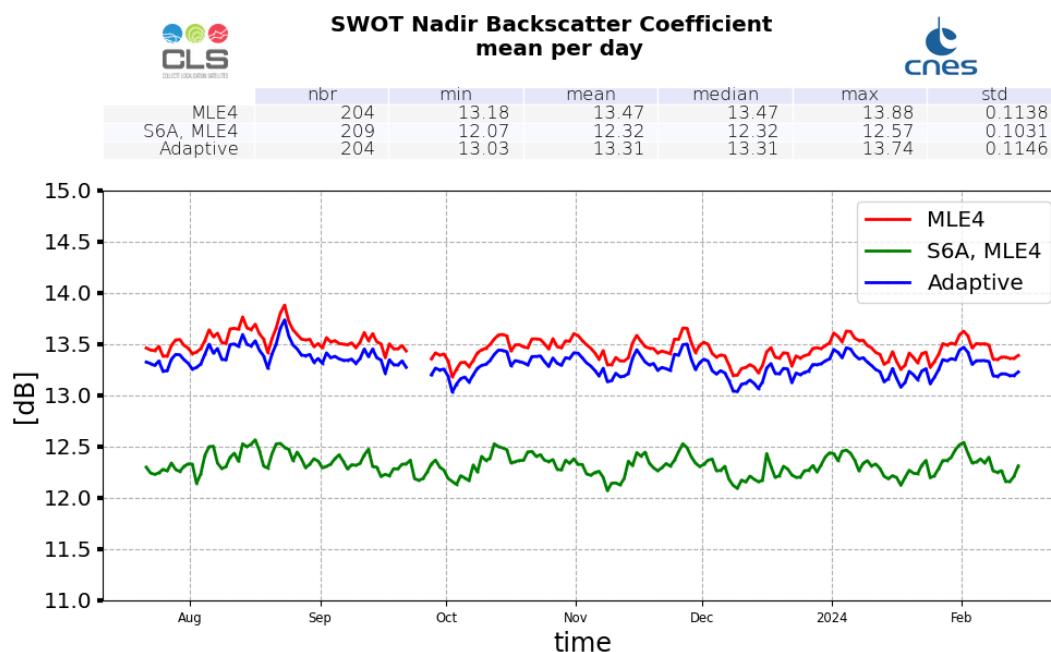
Figure 9: Ku-band Backscattering coefficient daily monitoring from cycle 001 to 010, for SWOT Nadir and Sentinel-6A-MF
