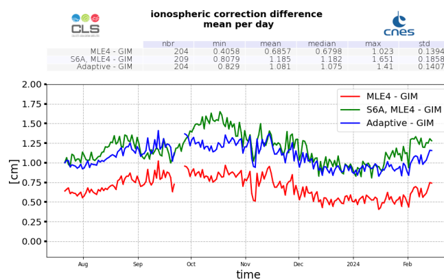
Figure 15: SWOT Nadir MLE4 (red), Adaptive (blue) and Sentinel-6A-MF (LR MLE4) (green) filtered ionosphere correction daily monitoring from cycle 001 to 010 (left) and difference with GIM model (right)
