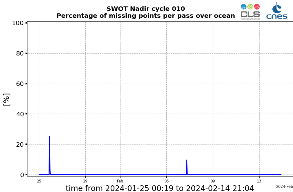
Figure 2: Monitoring of the percentage per pass of missing data over ocean, for SWOT Nadir GDR cycle 010
