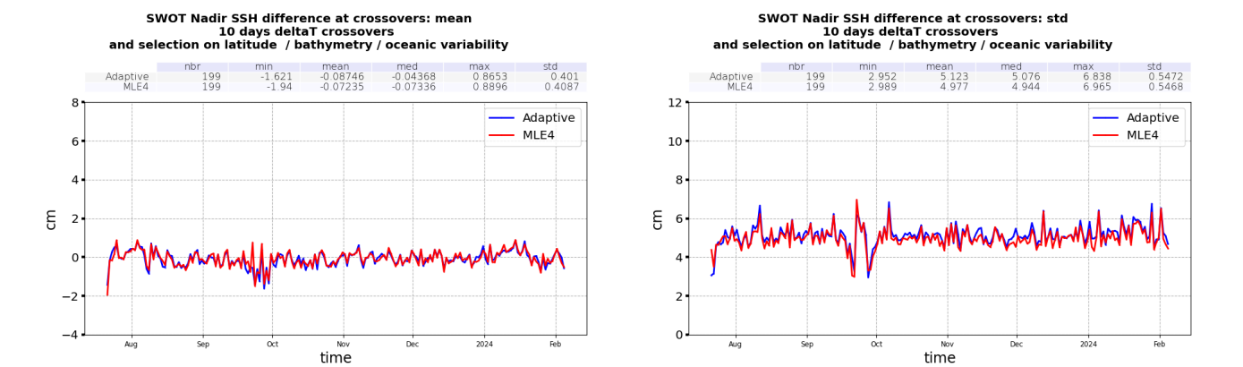
Figure 26: Monitoring of SSH difference at crossovers for SWOT Nadir MLE4 (red) and Adaptive (blue) : mean (left) and standard deviation (right), from cycle 001 to 010
