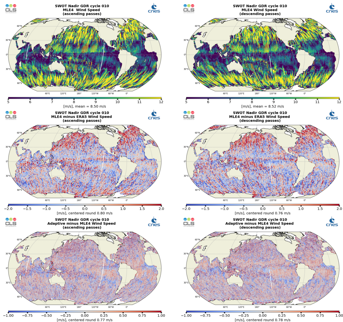
Figure 11: Along-track maps of Altimeter Wind Speed over cycle 010 for SWOT Nadir MLE4 (top), MLE4 minus ERA5 (middle) or Adaptive minus MLE4 (bottom), ascending passes (left) and descending passes (right)
