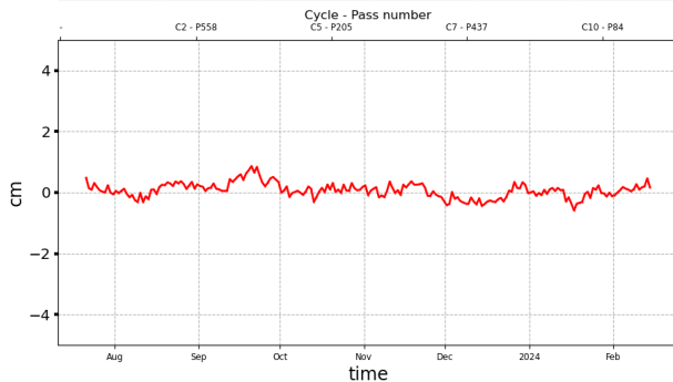
Figure 28: Daily monitoring of SSH difference at crossovers between SWOT Nadir MLE4 and Sentinel-6 MF LR MLE4 from cycle 001 onwards : mean (left) and standard deviation (right)
