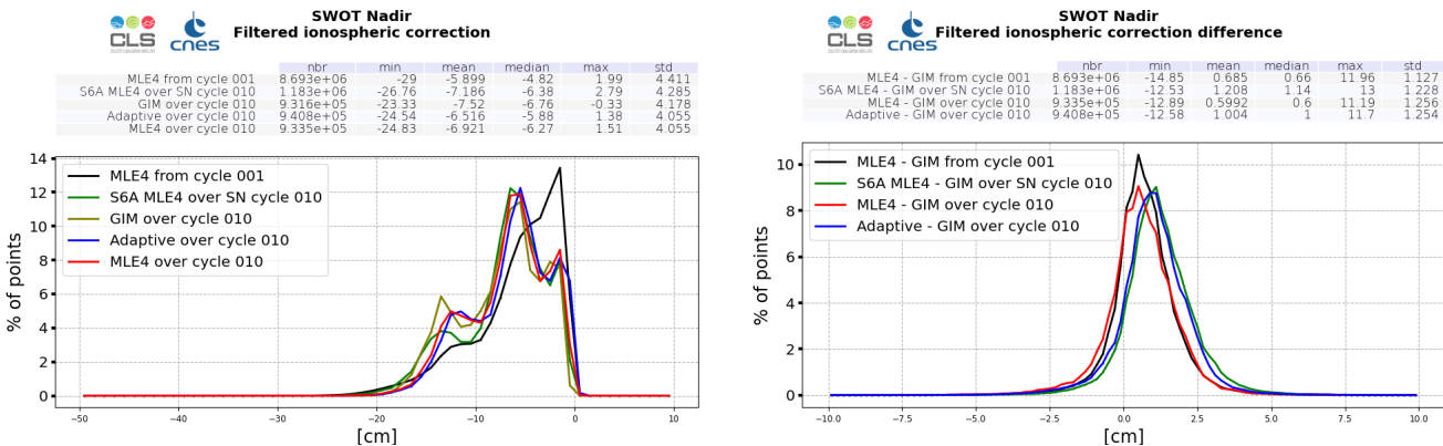
Figure 13: GIM model (dark green) and altimeter filtered ionosphere correction histogram computed over cycle 010 (red line for SWOT Nadir MLE4 and blue line for SWOT Nadir Adaptive, green for Sentinel-6A-MF (LR MLE4)) and from cycle 001 (SWOT Nadir, MLE4 only, black line) (left). Difference between filtered altimeter and GIM model (right).
