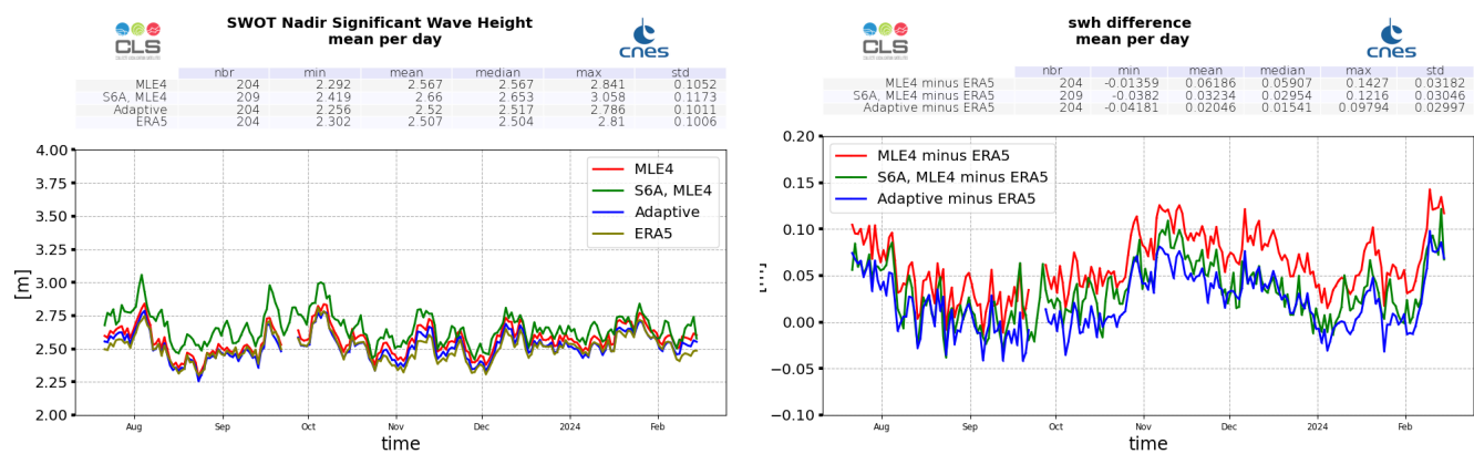
Figure 6: Ku-band Significant Wave Height daily monitoring from cycle 001 to 010, for SWOT Nadir, ERA5 model estimated at SWOT locations, and Sentinel-6A-MF (LR MLE4) (left), and difference with ERA5 model (right)
