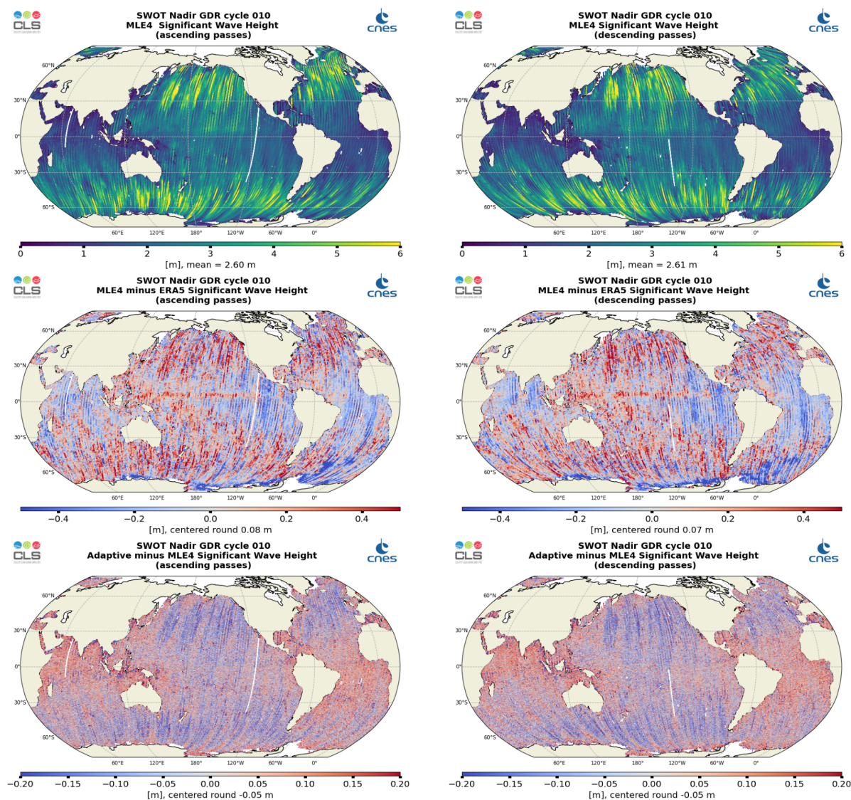
Figure 5: Along-track maps of Ku-band Significant Wave Height over cycle 010 for SWOT Nadir MLE4 (top), MLE4 minus model (middle) or Adaptive minus MLE4 (bottom), ascending passes (left) and descending passes (right)
