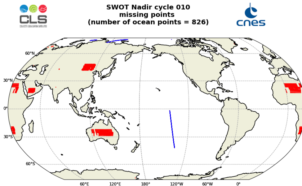
Figure 1: Map of missing measurements for SWOT Nadir GDR cycle 010
