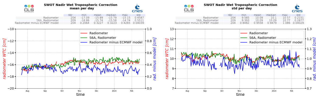
Figure 21: Daily monitoring of mean (left) and standard deviation (right) of the interpolated to Nadir AMRs wet tropospheric corrections (red) and radiometer minus ECMWF model difference of wet tropospheric corrections (blue), computed from cycle 001 to 010. Sentinel-6A-MF radiometer monitoring in green.
