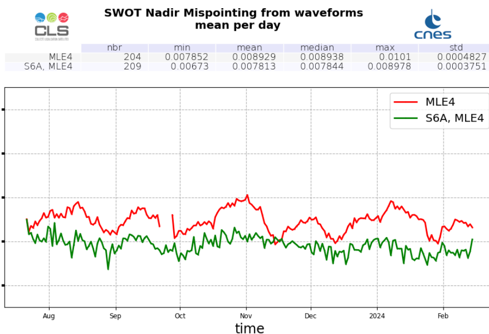
Figure 18: Mispointing daily monitoring from SWOT cycle 001 to 010 for SWOT Nadir GDR (red) and Sentinel-6A-MF (green)
