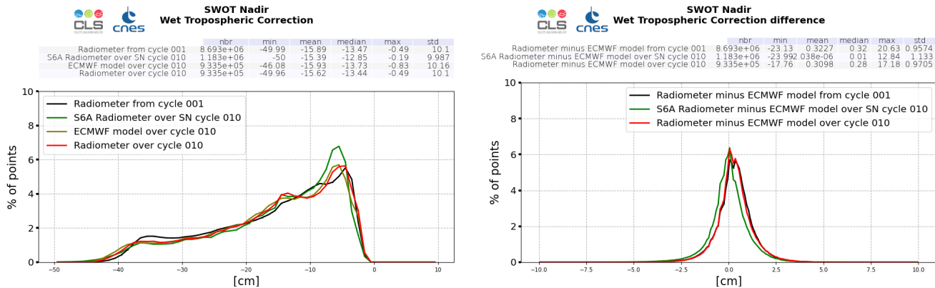
Figure 19: Histogram of wet troposphere corrections : SWOT Nadir radiometer (left) and difference with ECMWF model (right), computed over cycle 010 and from cycle 001 (black line)
