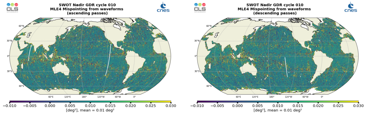
Figure 17: Along-track maps of mispointing over cycle 010 for SWOT Nadir MLE4, ascending passes (left) and descending passes (right)
