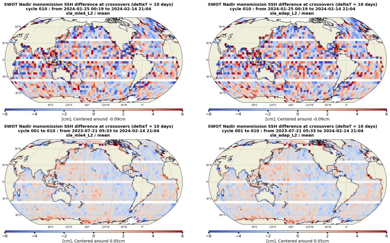
Figure 25: Mean SSH difference at crossovers for SWOT Nadir MLE4 (left) and Adaptive (right) cycle 010(top) and from cycle 001 to cycle 010 (bottom)
