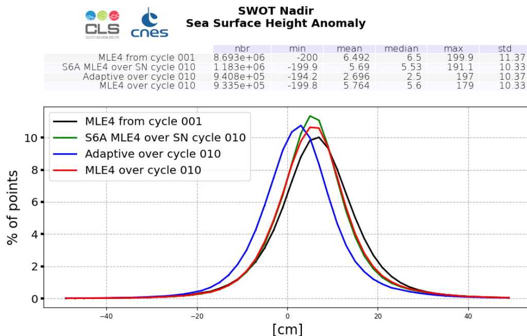
Figure 22: SSHA histogram computed over cycle 010 (red line for SWOT Nadir MLE4 and blue line for SWOT Nadir Adaptive, green for Sentinel-6A-MF (LR MLE4)) and from cycle 001 (SWOT Nadir, MLE4 only, black line)
