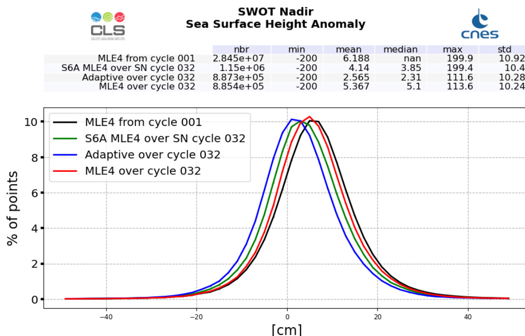
Figure 25: SSHA histogram computed over cycle 032 (red line for SWOT Nadir MLE4 and blue line for SWOT Nadir Adaptive, green for Sentinel-6A-MF (LR MLE4)) and from cycle 001 (SWOT Nadir, MLE4 only, black line)
