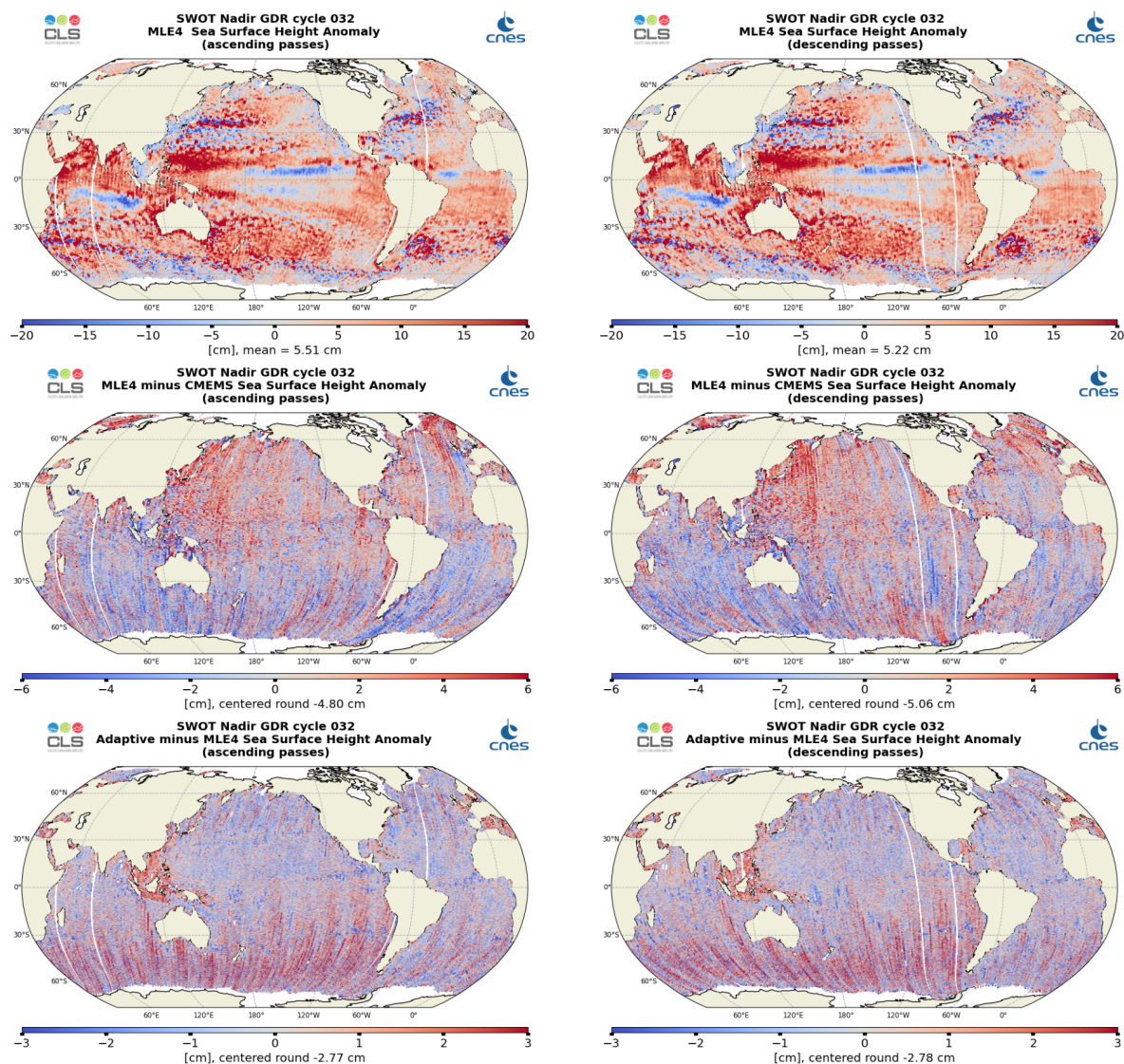
Figure 26: Along-track maps of SSHA over cycle 032 for SWOT Nadir MLE4 (top), MLE4 minus CMEMS (middle) or Adaptive minus MLE4 (bottom), ascending passes (left) and descending passes (right)
