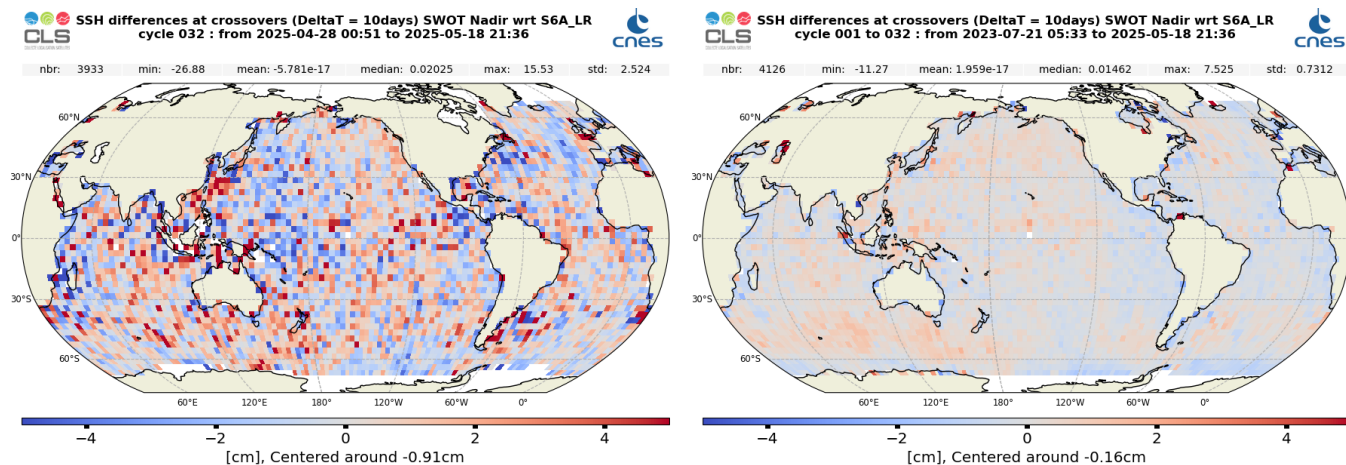
Figure 30: Mean SSH difference at crossovers between SWOT Nadir MLE4 and Sentinel-6 MF LR MLE4 over cycle 032 (left) and from cycle 001 onwards (right)
