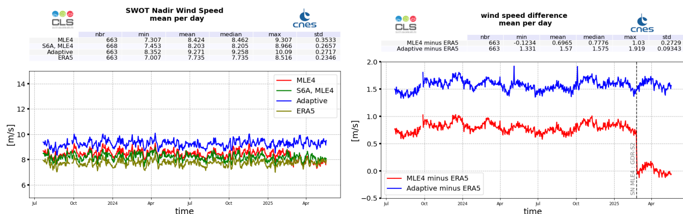
Figure 12: Wind Speed daily monitoring from cycle 001 to 032 for SWOT Nadir GDR, ERA5 model, and Sentinel-6A-MF (LR MLE4) (left), and daily mean difference with ERA5 (right)
