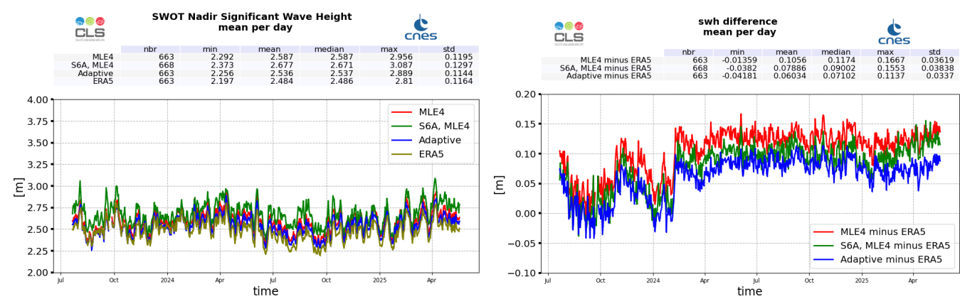
Figure 6: Ku-band Significant Wave Height daily monitoring from cycle 001 to 032, for SWOT Nadir, ERA5 model estimated at SWOT locations, and Sentinel-6A-MF (LR MLE4) (left), and difference with ERA5 model (right)
