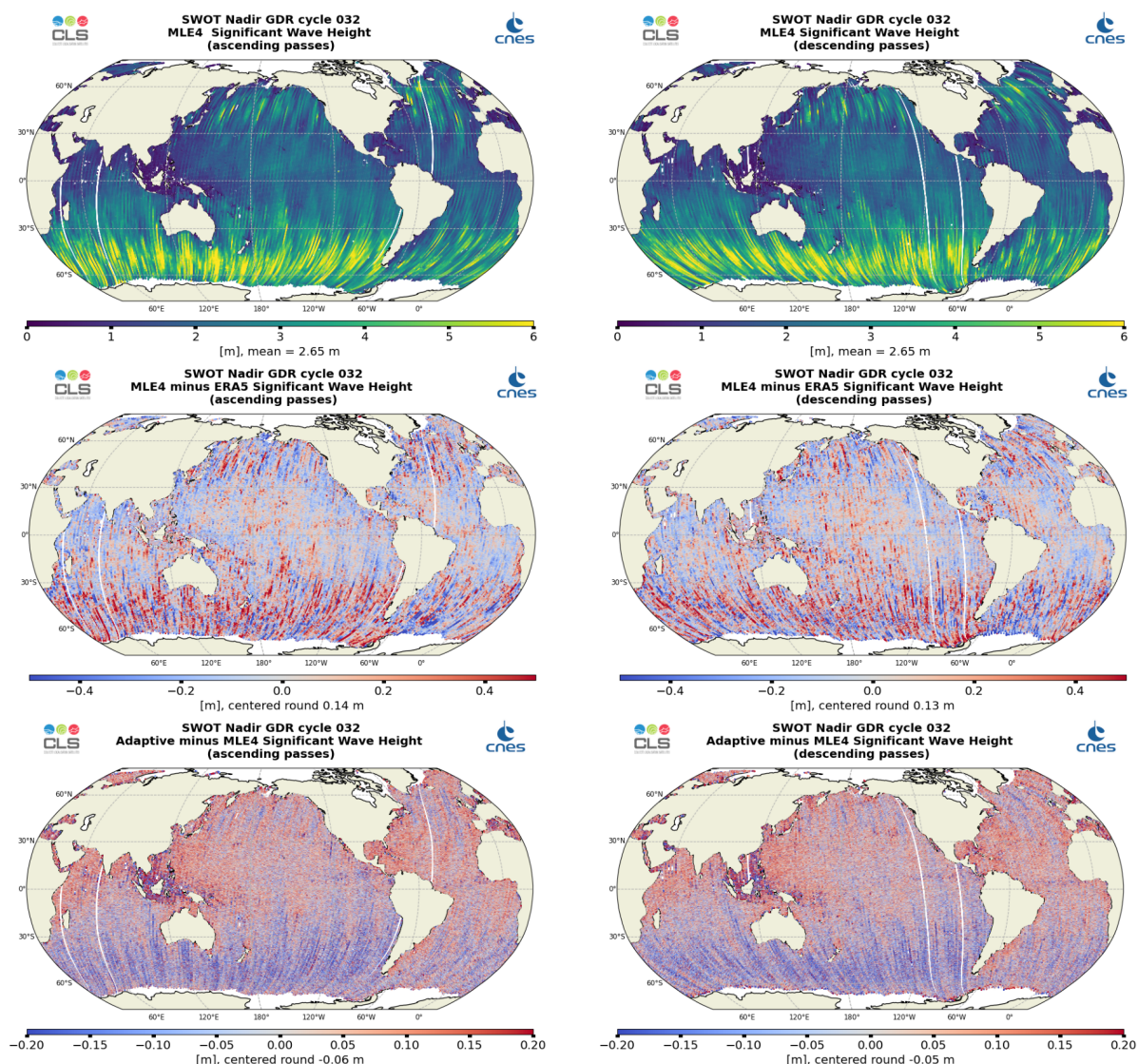
Figure 5: Along-track maps of Ku-band Significant Wave Height over cycle 032 for SWOT Nadir MLE4 (top), MLE4 minus model (middle) or Adaptive minus MLE4 (bottom), ascending passes (left) and descending passes (right)
