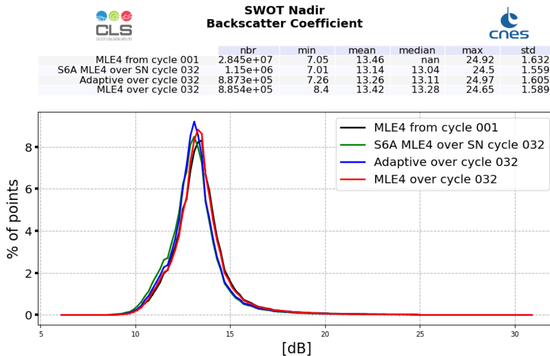
Figure 7: Ku-band Backscattering coefficient histogram computed over cycle 032 (red line for SWOT Nadir MLE4 and blue line for SWOT Nadir Adaptive, green for Sentinel-6A-MF (LR MLE4)) and from cycle 001 (SWOT Nadir, MLE4 only, black line)
