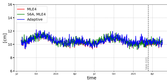
Figure 27: SSHA daily monitoring from cycle 001 to 032, for SWOT Nadir GDR
