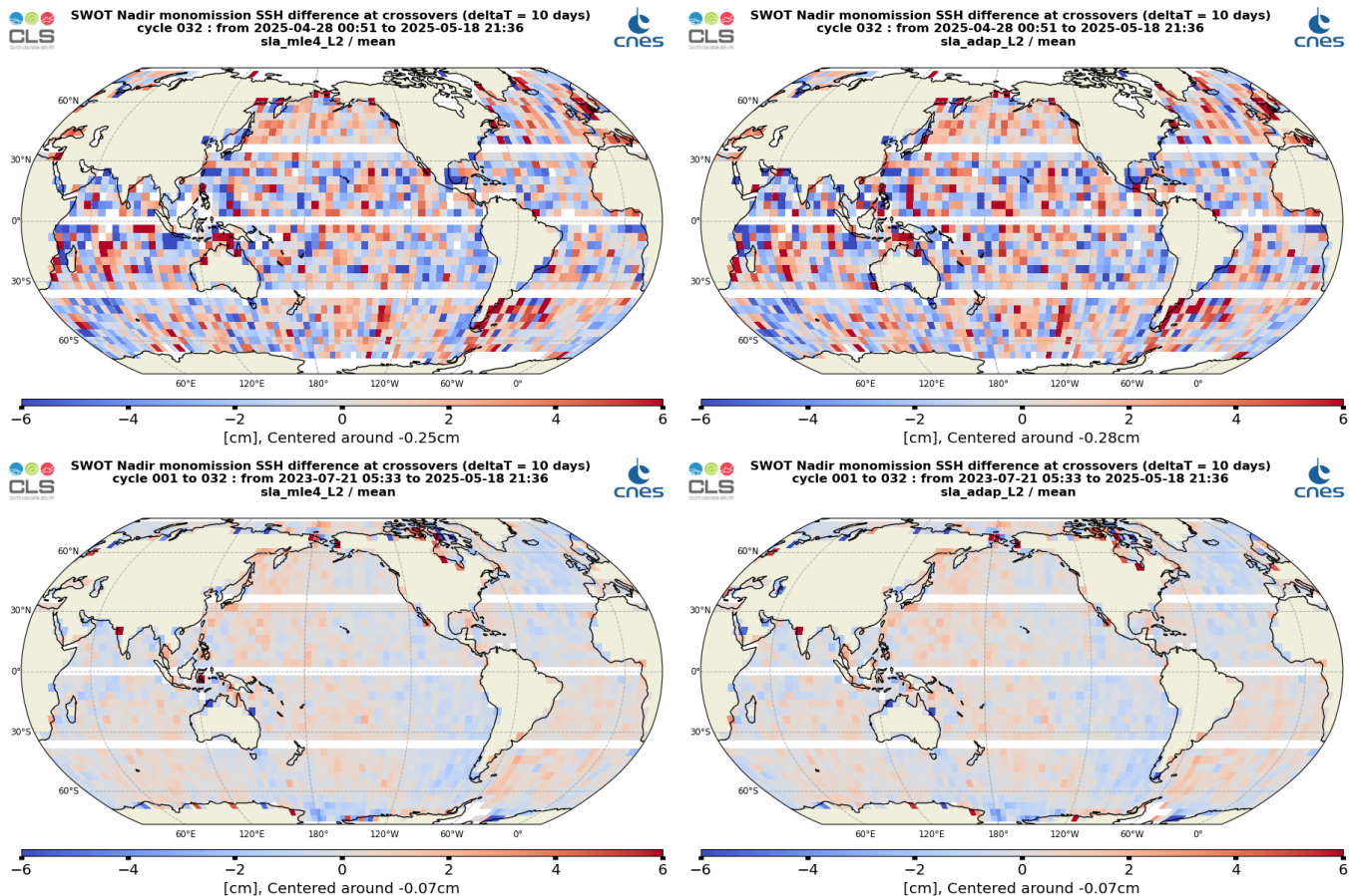
Figure 28: Mean SSH difference at crossovers for SWOT Nadir MLE4 (left) and Adaptive (right) cycle 032(top) and from cycle 001 to cycle 032 (bottom)
