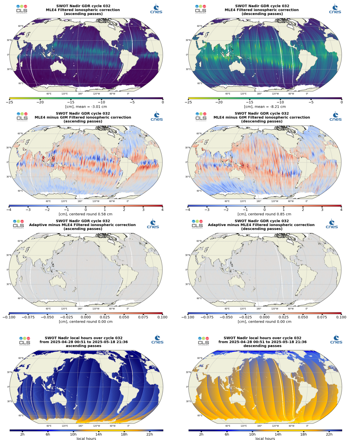
Figure 14: Along-track maps of filtered ionosphere correction over cycle 032 for SWOT Nadir MLE4 (top), MLE4 minus GIM (middle top) or Adaptive minus MLE4 (middle bottom), and local hours (bottom), for ascending passes (left) and descending passes (right)
