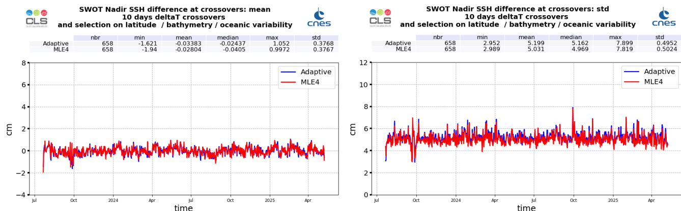
Figure 29: Monitoring of SSH difference at crossovers for SWOT Nadir MLE4 (red) and Adaptive (blue) : mean (left) and standard deviation (right), from cycle 001 to 032
