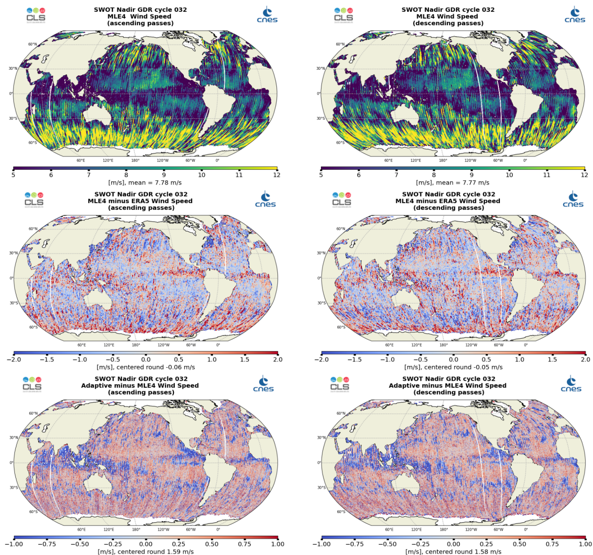
Figure 11: Along-track maps of Altimeter Wind Speed over cycle 032 for SWOT Nadir MLE4 (top), MLE4 minus ERA5 (middle) or Adaptive minus MLE4 (bottom), ascending passes (left) and descending passes (right)
