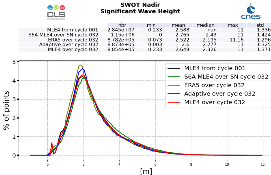
Figure 4: Ku-band Significant Wave Height histogram computed over cycle 032 (red line for SWOT Nadir MLE4 and blue line for SWOT Nadir Adaptive, green for Sentinel-6A-MF (LR MLE4) and dark green for ERA5) and from cycle 001 (SWOT Nadir, MLE4 only, black line)
