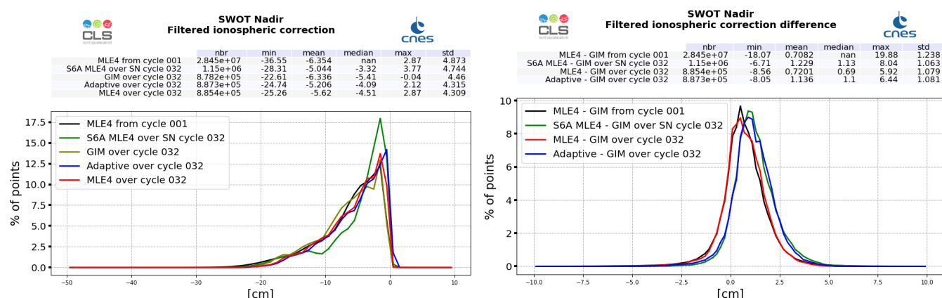
Figure 13: GIM model (dark green) and altimeter filtered ionosphere correction histogram computed over cycle 032 (red line for SWOT Nadir MLE4 and blue line for SWOT Nadir Adaptive, green for Sentinel-6A-MF (LR MLE4)) and from cycle 001 (SWOT Nadir, MLE4 only, black line) (left). Difference between filtered altimeter and GIM model (right).
