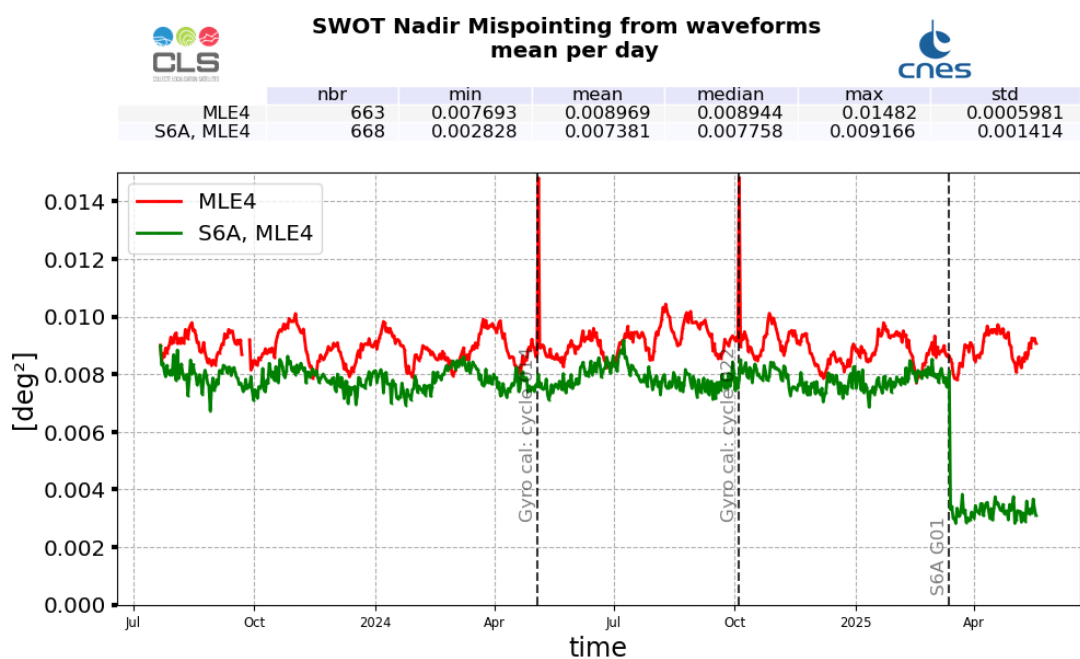
Figure 18: Mispointing daily monitoring from SWOT cycle 001 to 032 for SWOT Nadir GDR (red) and Sentinel-6A-MF (green)
