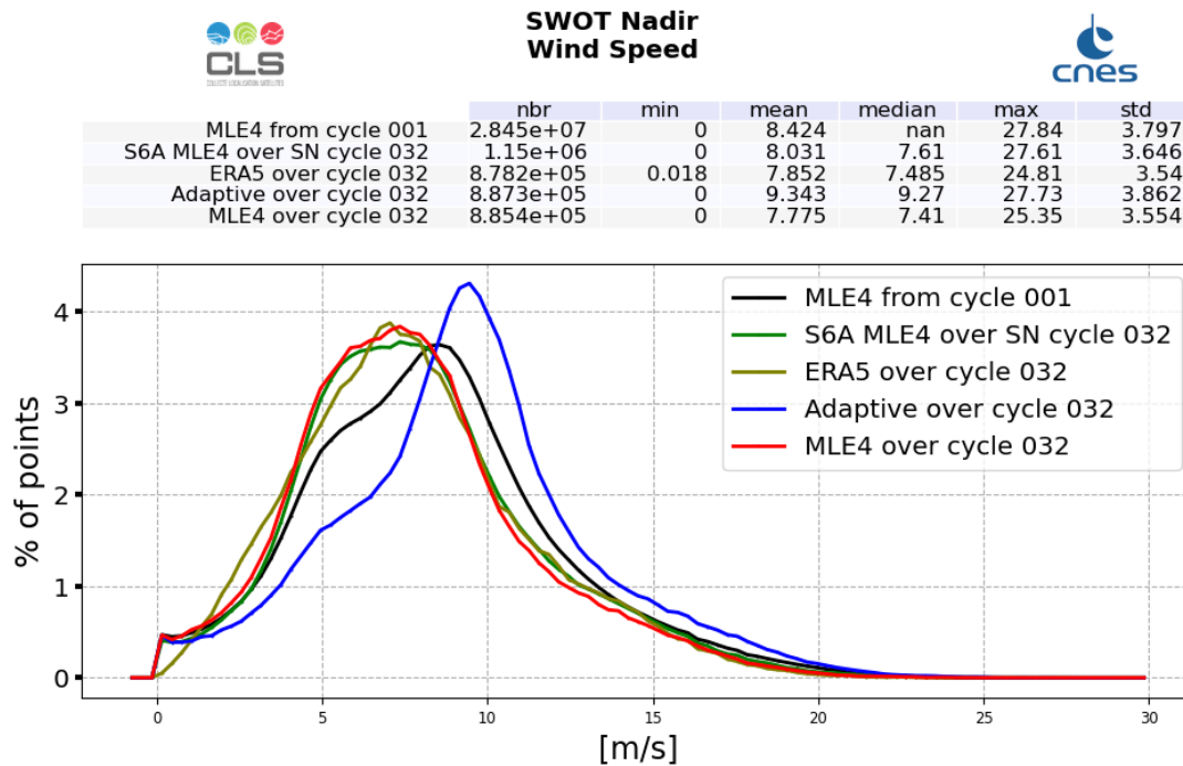
Figure 10: Altimeter Wind Speed histogram computed over cycle 032 (red line for SWOT Nadir MLE4 and blue line for SWOT Nadir Adaptive, green for Sentinel-6A-MF (LR MLE4)) and from cycle 001 (SWOT Nadir, MLE4 only, black line)
