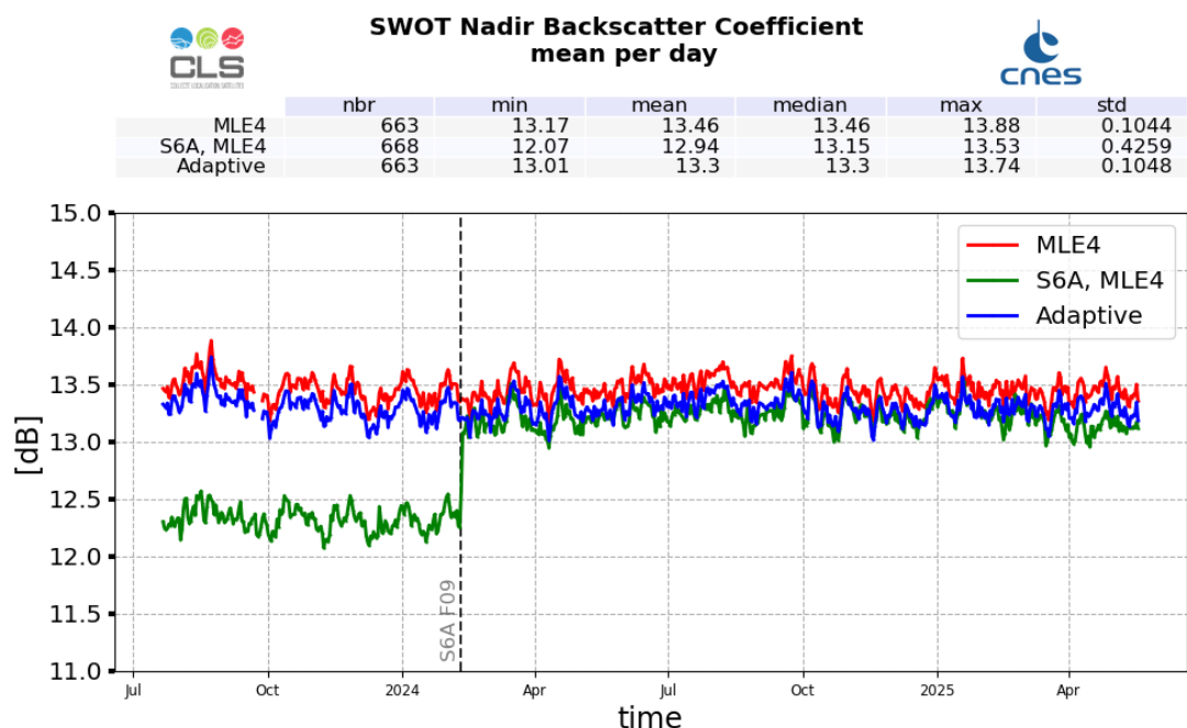
Figure 9: Ku-band Backscattering coefficient daily monitoring from cycle 001 to 032, for SWOT Nadir and Sentinel-6A-MF
