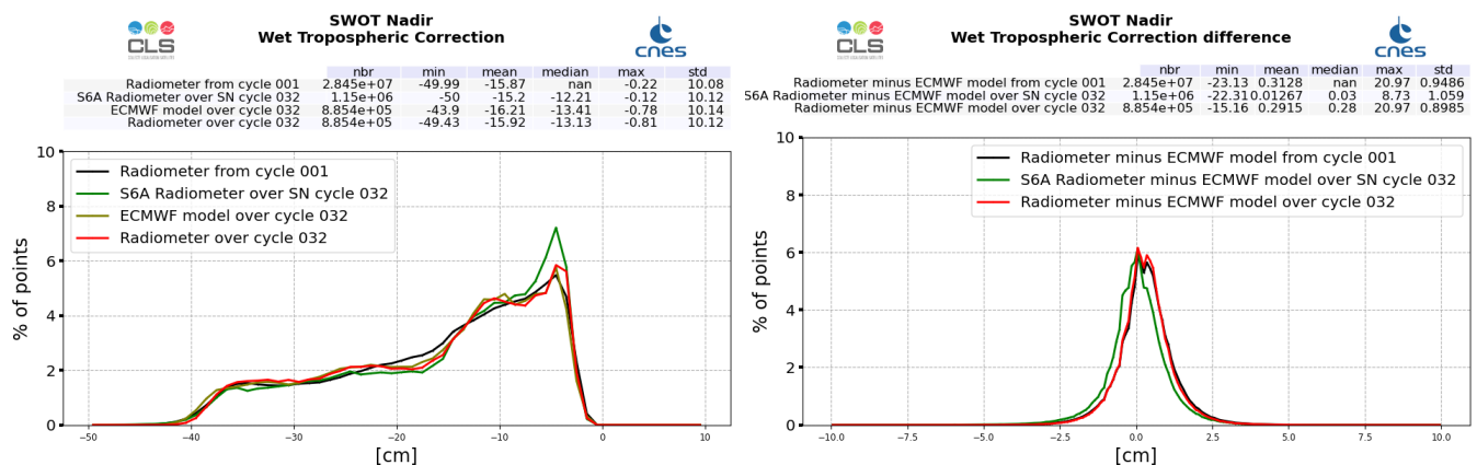
Figure 21: Histogram of wet troposphere corrections : SWOT Nadir radiometer (left) and difference with ECMWF model (right), computed over cycle 032 and from cycle 001 (black line)
