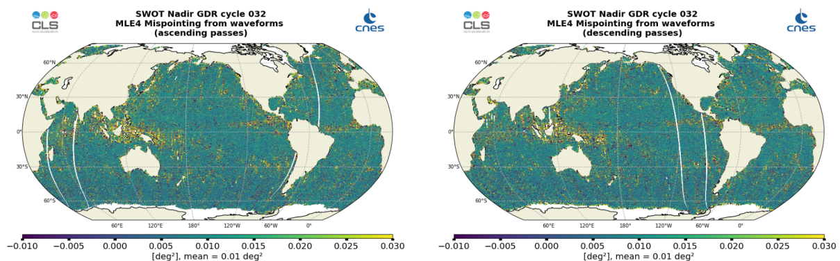
Figure 17: Along-track maps of mispointing over cycle 032 for SWOT Nadir MLE4, ascending passes (left) and descending passes (right)
