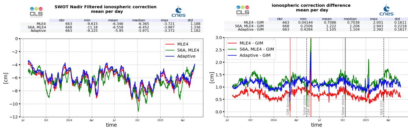
Figure 15: SWOT Nadir MLE4 (red), Adaptive (blue) and Sentinel-6A-MF (LR MLE4) (green) filtered ionosphere correction daily monitoring from cycle 001 to 032 (left) and difference with GIM model (right)
