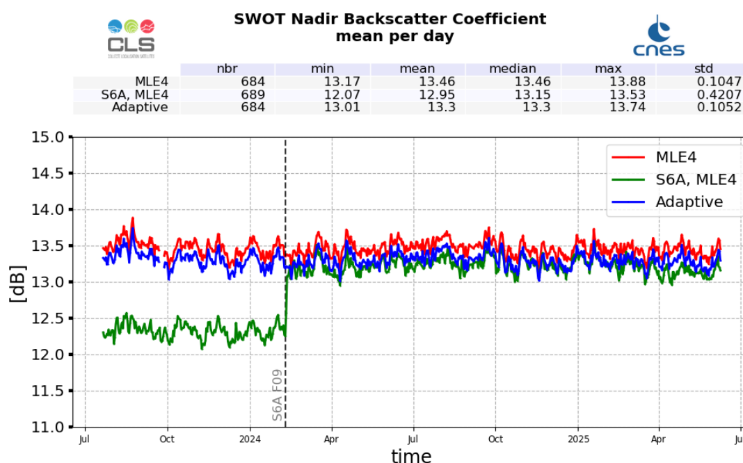
Figure 9: Ku-band Backscattering coefficient daily monitoring from cycle 001 to 033, for SWOT Nadir and Sentinel-6A-MF
