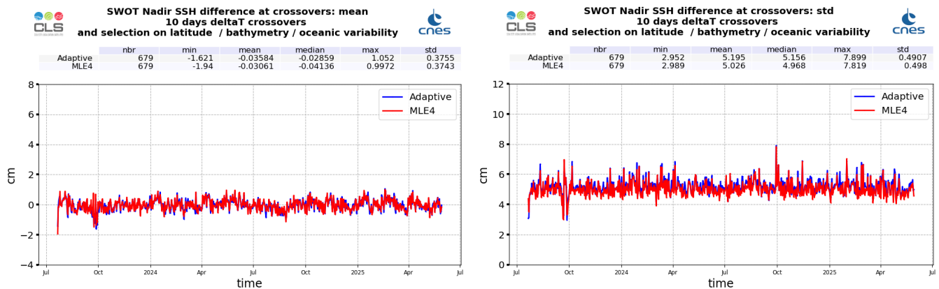
Figure 29: Monitoring of SSH difference at crossovers for SWOT Nadir MLE4 (red) and Adaptive (blue) : mean (left) and standard deviation (right), from cycle 001 to 033
