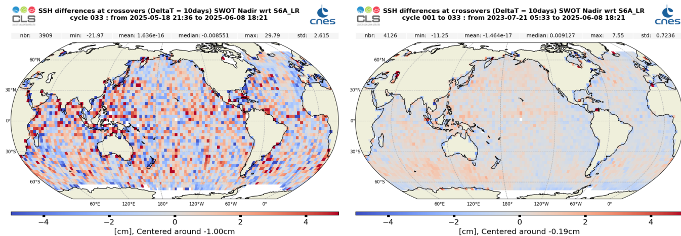
Figure 30: Mean SSH difference at crossovers between SWOT Nadir MLE4 and Sentinel-6 MF LR MLE4 over cycle 033 (left) and from cycle 001 onwards (right)
