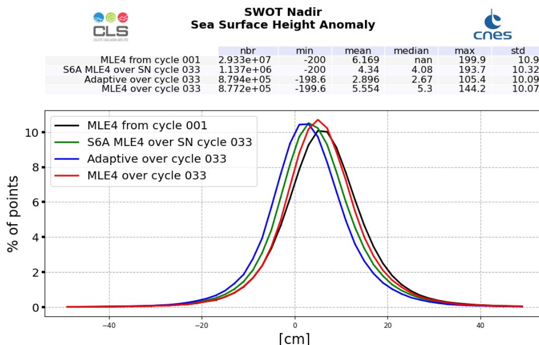
Figure 25: SSHA histogram computed over cycle 033 (red line for SWOT Nadir MLE4 and blue line for SWOT Nadir Adaptive, green for Sentinel-6A-MF (LR MLE4)) and from cycle 001 (SWOT Nadir, MLE4 only, black line)
