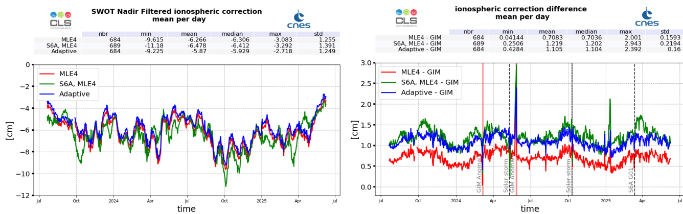
Figure 15: SWOT Nadir MLE4 (red), Adaptive (blue) and Sentinel-6A-MF (LR MLE4) (green) filtered ionosphere correction daily monitoring from cycle 001 to 033 (left) and difference with GIM model (right)
