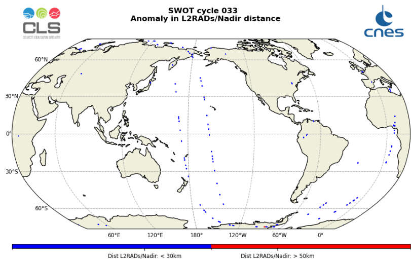
Figure 24: Map of the anomalies detected in the L2RADs/Nadir distance over the cycle 033
