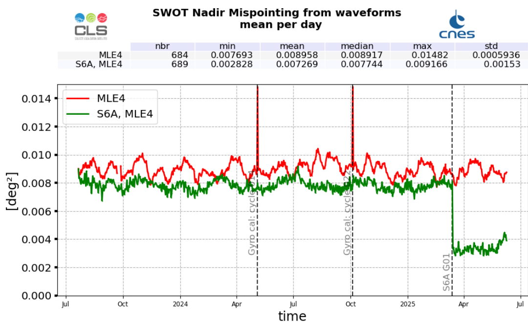
Figure 18: Mispointing daily monitoring from SWOT cycle 001 to 033 for SWOT Nadir GDR (red) and Sentinel-6A-MF (green)
