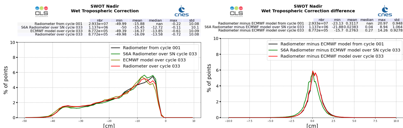
Figure 21: Histogram of wet troposphere corrections : SWOT Nadir radiometer (left) and difference with ECMWF model (right), computed over cycle 033 and from cycle 001 (black line)
