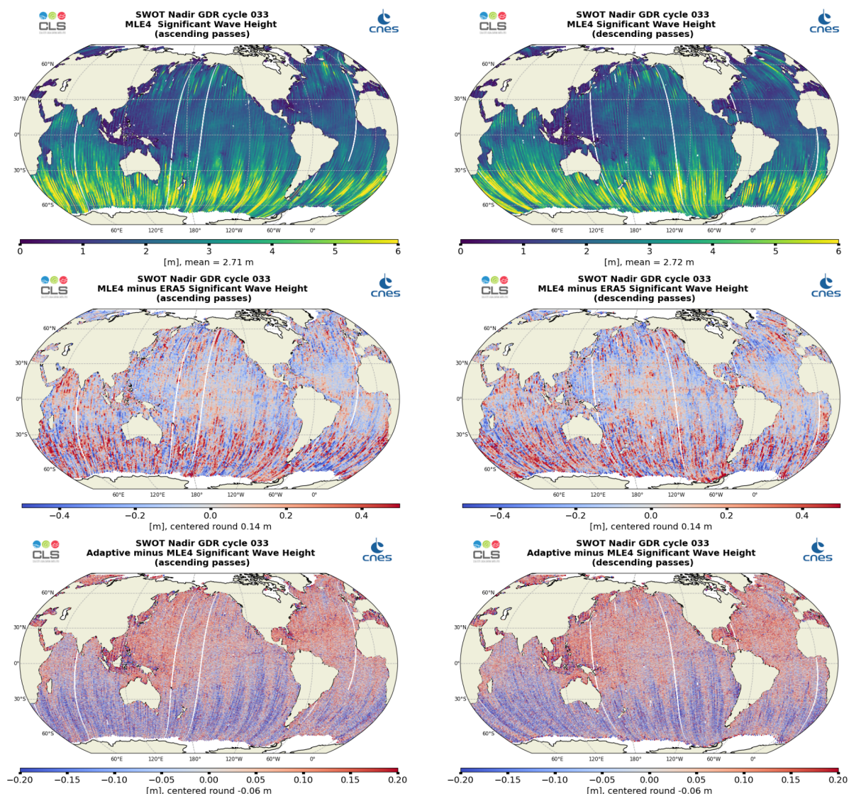
Figure 5: Along-track maps of Ku-band Significant Wave Height over cycle 033 for SWOT Nadir MLE4 (top), MLE4 minus model (middle) or Adaptive minus MLE4 (bottom), ascending passes (left) and descending passes (right)
