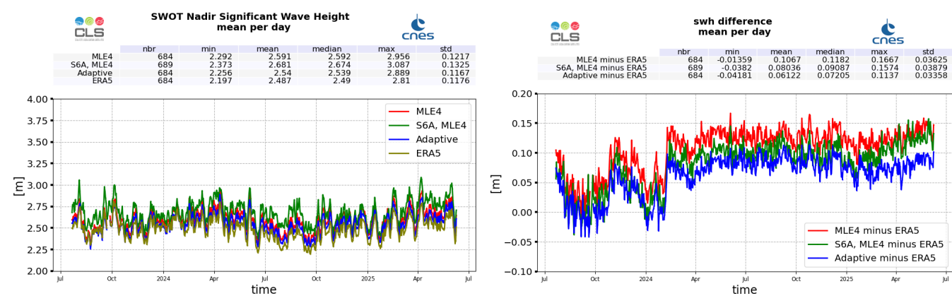
Figure 6: Ku-band Significant Wave Height daily monitoring from cycle 001 to 033, for SWOT Nadir, ERA5 model estimated at SWOT locations, and Sentinel-6A-MF (LR MLE4) (left), and difference with ERA5 model (right)
