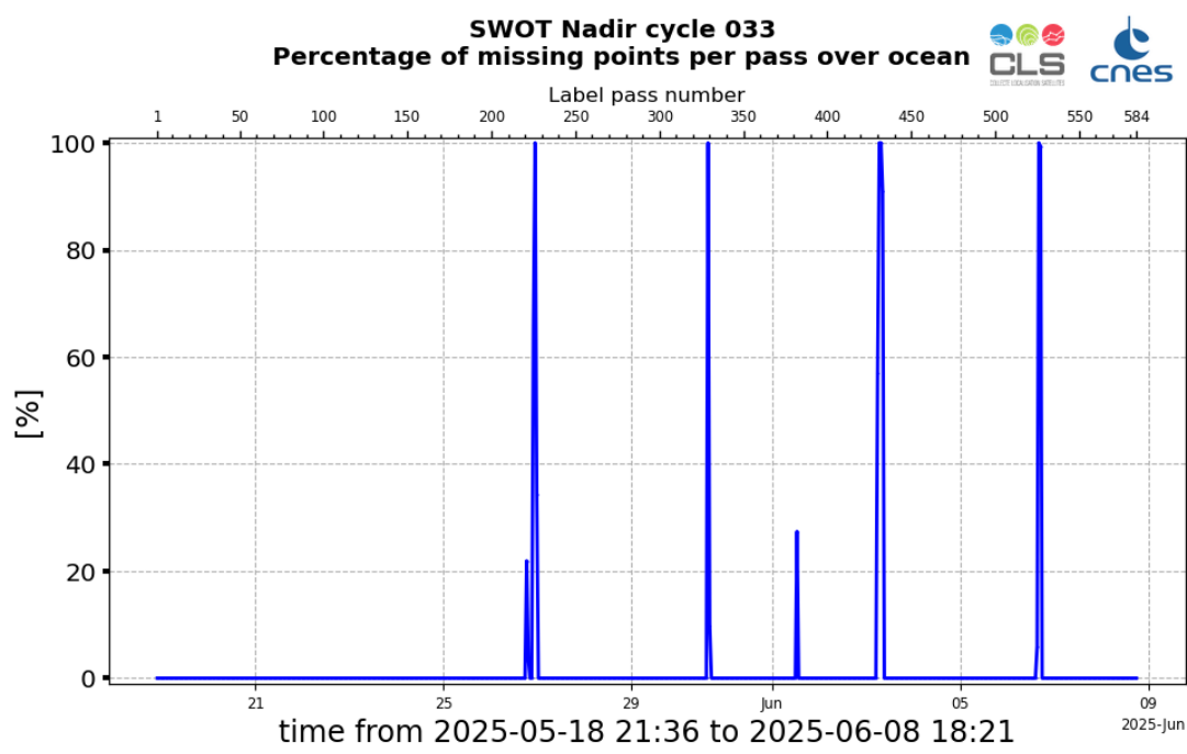
Figure 2: Monitoring of the percentage per pass of missing data over ocean, for SWOT Nadir GDR cycle 033
