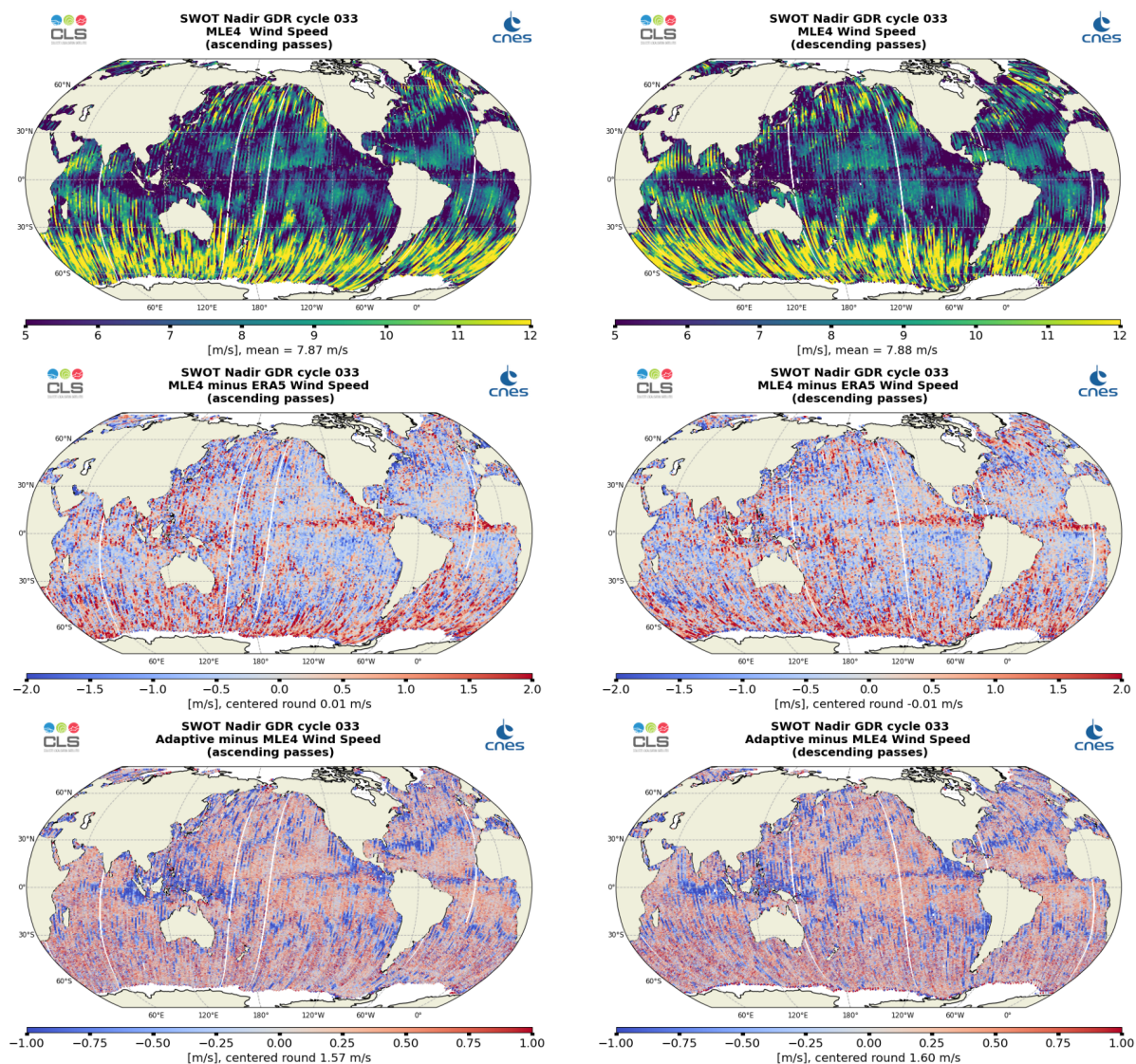
Figure 11: Along-track maps of Altimeter Wind Speed over cycle 033 for SWOT Nadir MLE4 (top), MLE4 minus ERA5 (middle) or Adaptive minus MLE4 (bottom), ascending passes (left) and descending passes (right)
