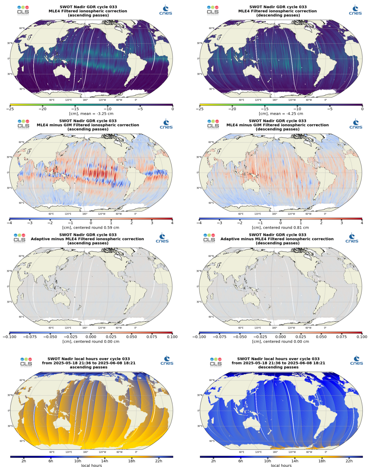
Figure 14: Along-track maps of filtered ionosphere correction over cycle 033 for SWOT Nadir MLE4 (top), MLE4 minus GIM (middle top) or Adaptive minus MLE4 (middle bottom), and local hours (bottom), for ascending passes (left) and descending passes (right)
