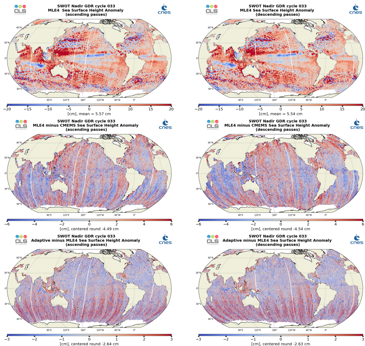
Figure 26: Along-track maps of SSHA over cycle 033 for SWOT Nadir MLE4 (top), MLE4 minus CMEMS (middle) or Adaptive minus MLE4 (bottom), ascending passes (left) and descending passes (right)
