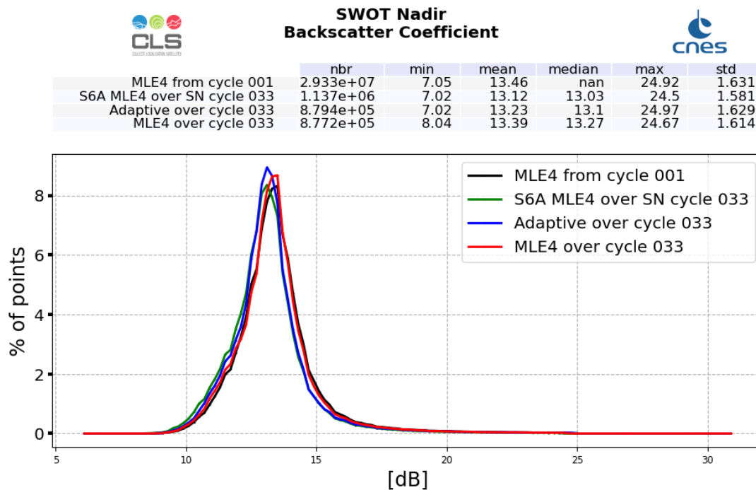
Figure 7: Ku-band Backscattering coefficient histogram computed over cycle 033 (red line for SWOT Nadir MLE4 and blue line for SWOT Nadir Adaptive, green for Sentinel-6A-MF (LR MLE4)) and from cycle 001 (SWOT Nadir, MLE4 only, black line)
