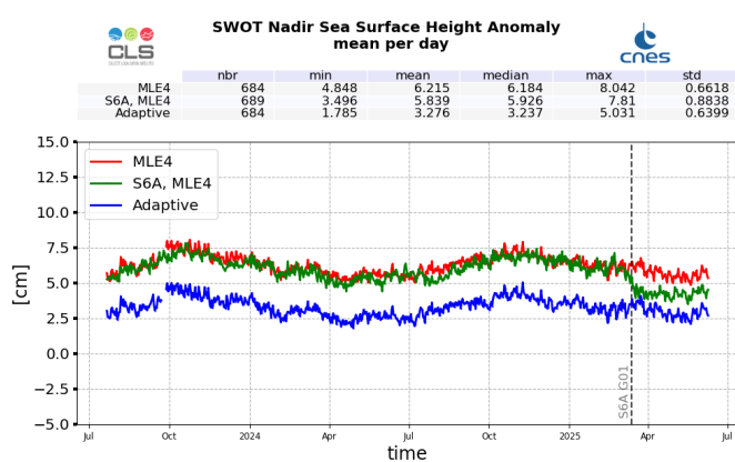
Figure 27: SSHA daily monitoring from cycle 001 to 033, for SWOT Nadir GDR
