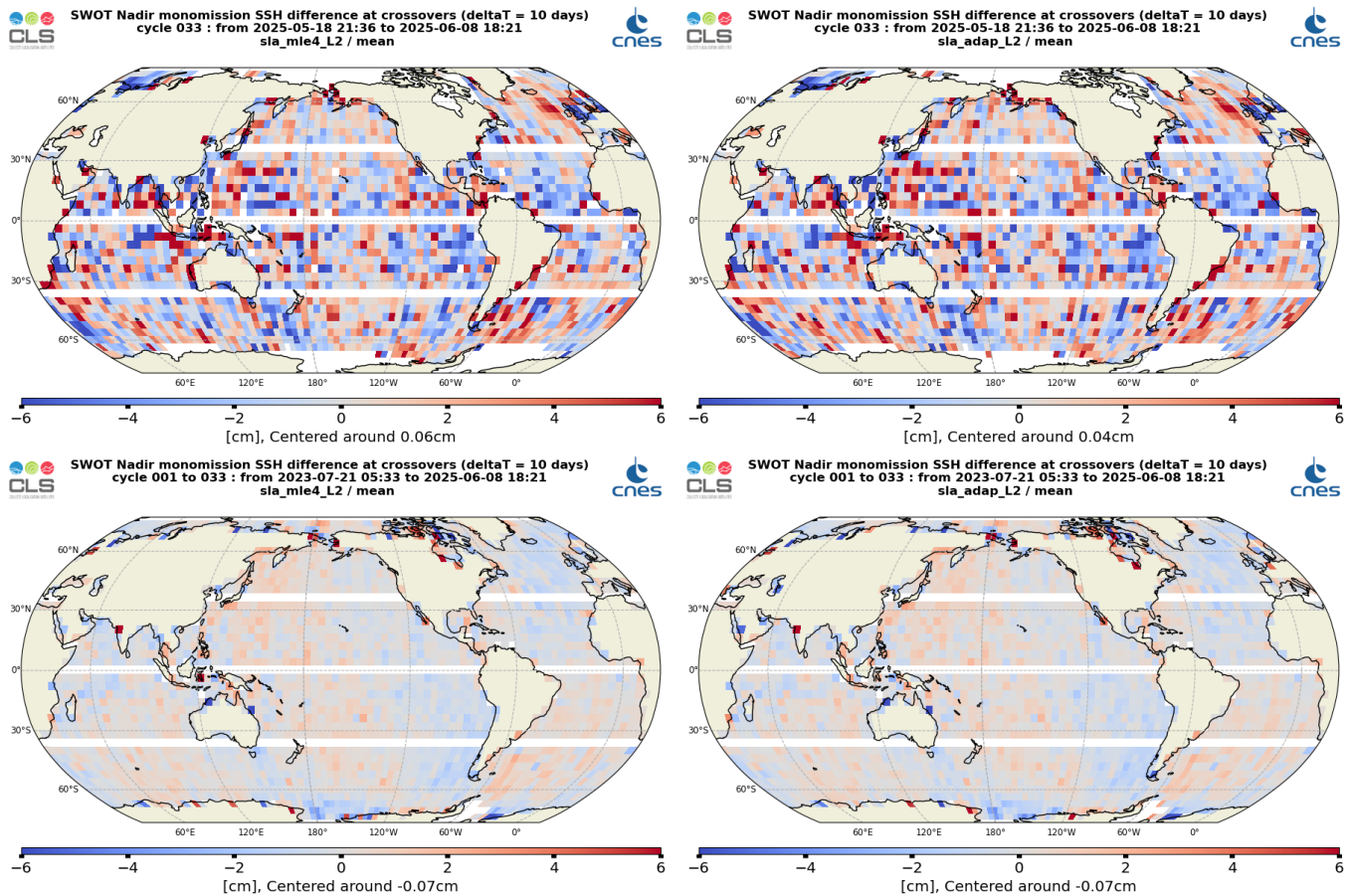
Figure 28: Mean SSH difference at crossovers for SWOT Nadir MLE4 (left) and Adaptive (right) cycle 033(top) and from cycle 001 to cycle 033 (bottom)
