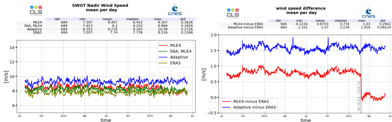
Figure 12: Wind Speed daily monitoring from cycle 001 to 033 for SWOT Nadir GDR, ERA5 model, and Sentinel-6A-MF (LR MLE4) (left), and daily mean difference with ERA5 (right)
