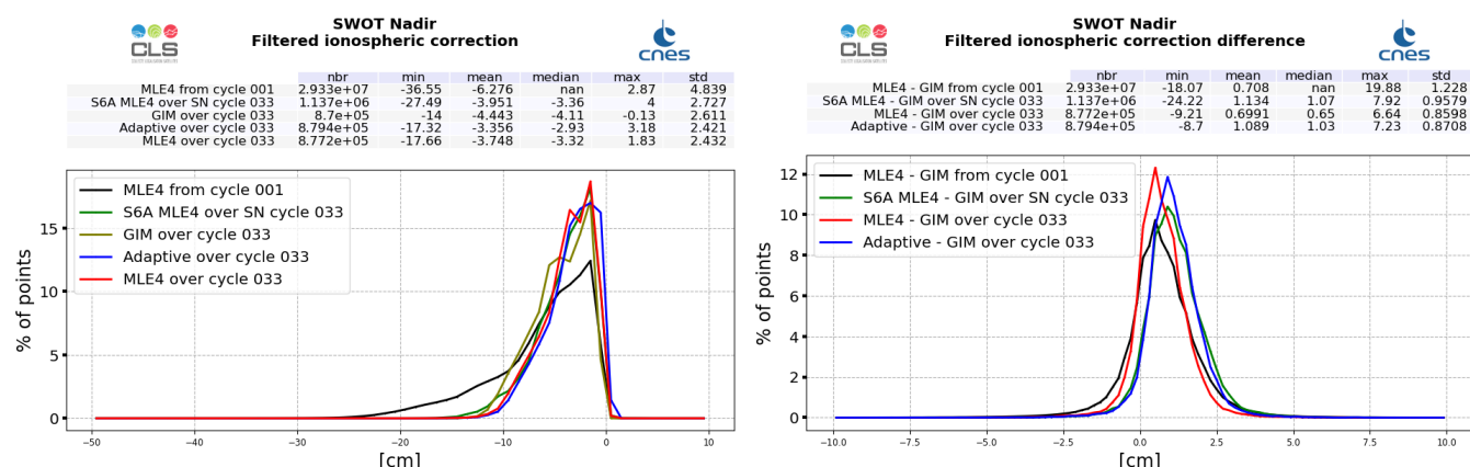
Figure 13: GIM model (dark green) and altimeter filtered ionosphere correction histogram computed over cycle 033 (red line for SWOT Nadir MLE4 and blue line for SWOT Nadir Adaptive, green for Sentinel-6A-MF (LR MLE4)) and from cycle 001 (SWOT Nadir, MLE4 only, black line) (left). Difference between filtered altimeter and GIM model (right).
