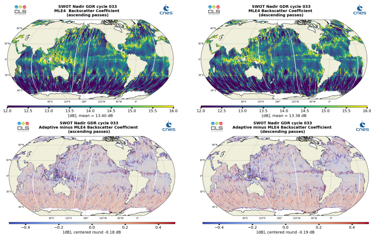
Figure 8: Along-track maps of Ku-band backscatter coefficient \sigma_0 over cycle 033 for SWOT Nadir MLE4 (top) or Adaptive minus MLE4 difference (bottom), ascending passes (left) and descending passes (right)
