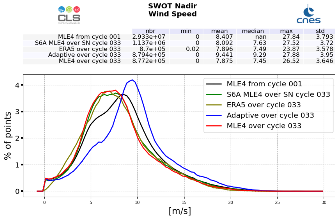
Figure 10: Altimeter Wind Speed histogram computed over cycle 033 (red line for SWOT Nadir MLE4 and blue line for SWOT Nadir Adaptive, green for Sentinel-6A-MF (LR MLE4)) and from cycle 001 (SWOT Nadir, MLE4 only, black line)
