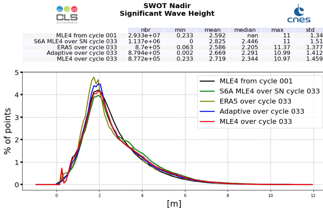
Figure 4: Ku-band Significant Wave Height histogram computed over cycle 033 (red line for SWOT Nadir MLE4 and blue line for SWOT Nadir Adaptive, green for Sentinel-6A-MF (LR MLE4) and dark green for ERA5) and from cycle 001 (SWOT Nadir, MLE4 only, black line)
