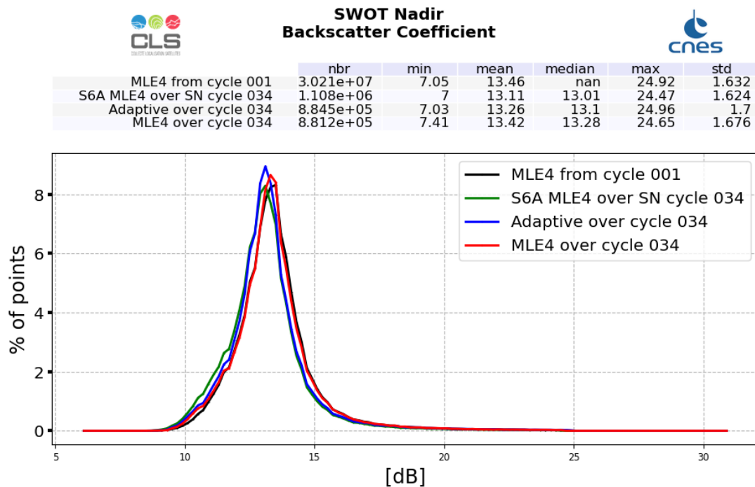
Figure 7: Ku-band Backscattering coefficient histogram computed over cycle 034 (red line for SWOT Nadir MLE4 and blue line for SWOT Nadir Adaptive, green for Sentinel-6A-MF (LR MLE4)) and from cycle 001 (SWOT Nadir, MLE4 only, black line)
