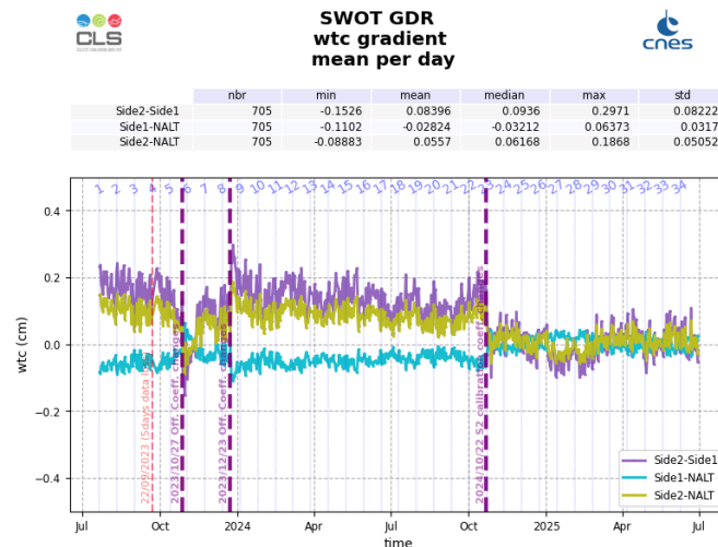
Figure 20: Daily monitoring of the wet tropospheric correction gradient between AMR Side 1 and AMR Side 2 (purple), AMR Side 1 and Nadir (cyan), and AMR Side 2 and Nadir (yellow), from Cycle 001 to 034
