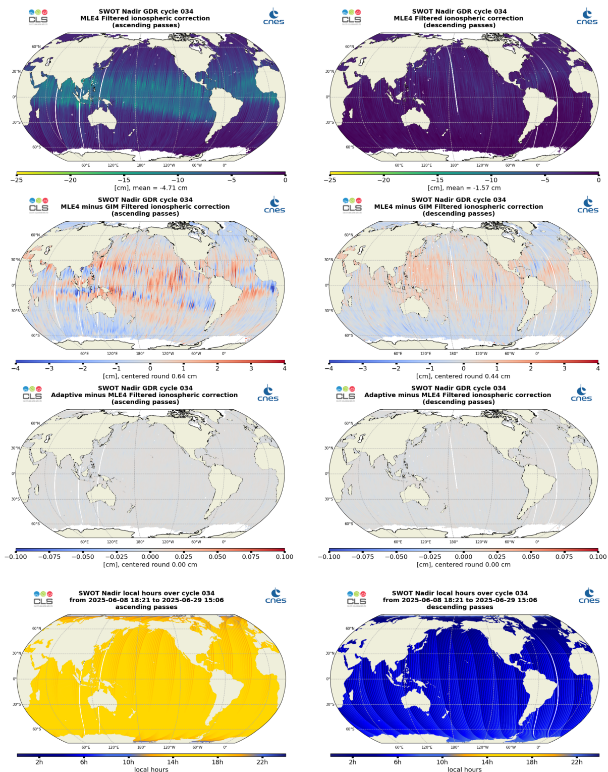
Figure 14: Along-track maps of filtered ionosphere correction over cycle 034 for SWOT Nadir MLE4 (top), MLE4 minus GIM (middle top) or Adaptive minus MLE4 (middle bottom), and local hours (bottom), for ascending passes (left) and descending passes (right)
