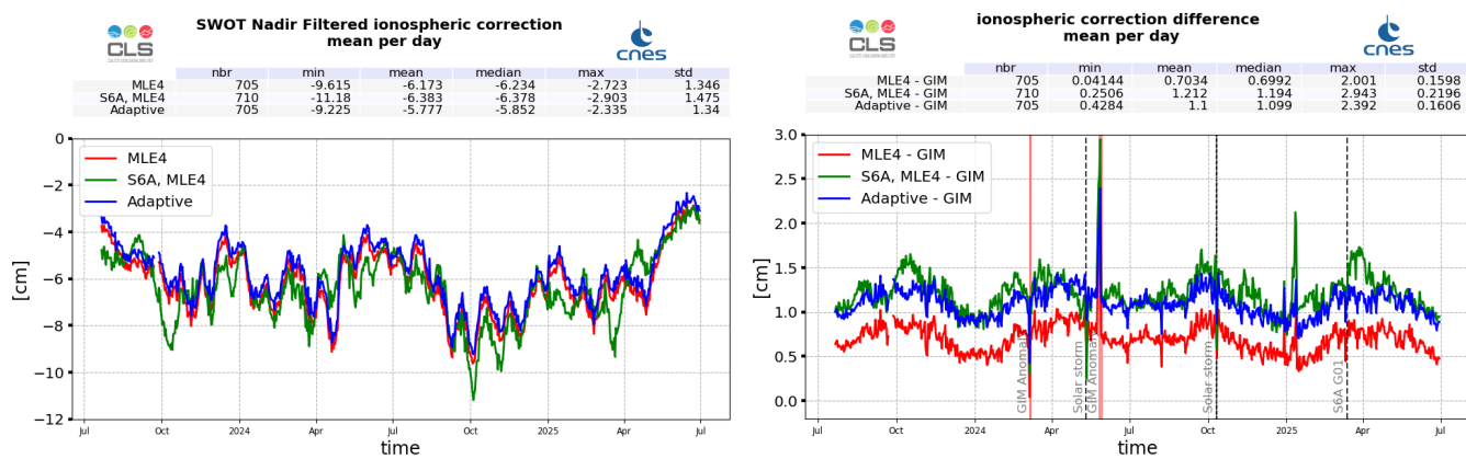
Figure 15: SWOT Nadir MLE4 (red), Adaptive (blue) and Sentinel-6A-MF (LR MLE4) (green) filtered ionosphere correction daily monitoring from cycle 001 to 034 (left) and difference with GIM model (right)
