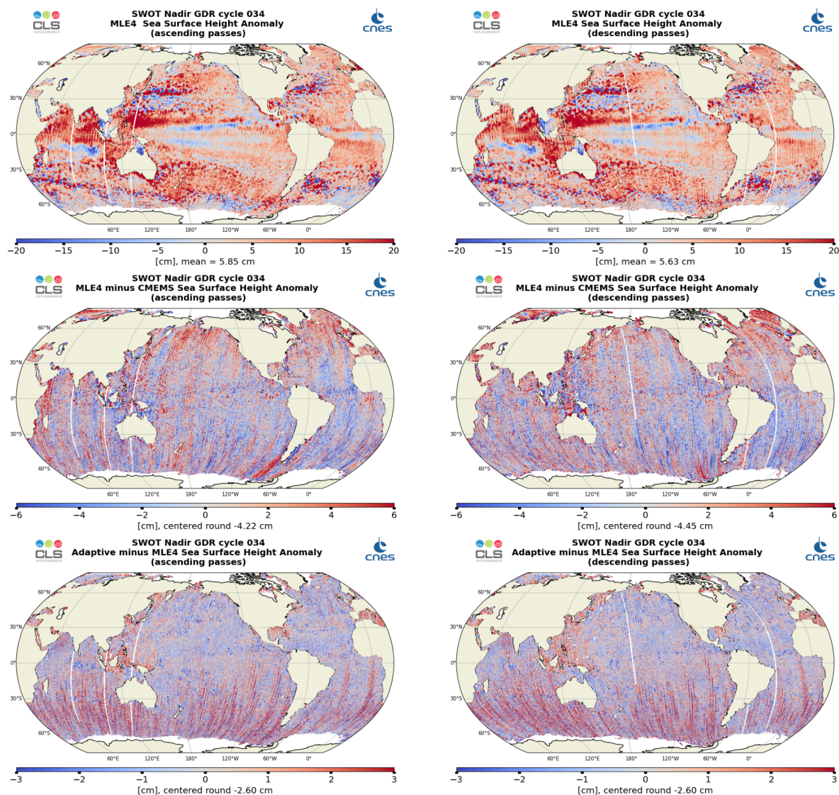
Figure 26: Along-track maps of SSHA over cycle 034 for SWOT Nadir MLE4 (top), MLE4 minus CMEMS (middle) or Adaptive minus MLE4 (bottom), ascending passes (left) and descending passes (right)
