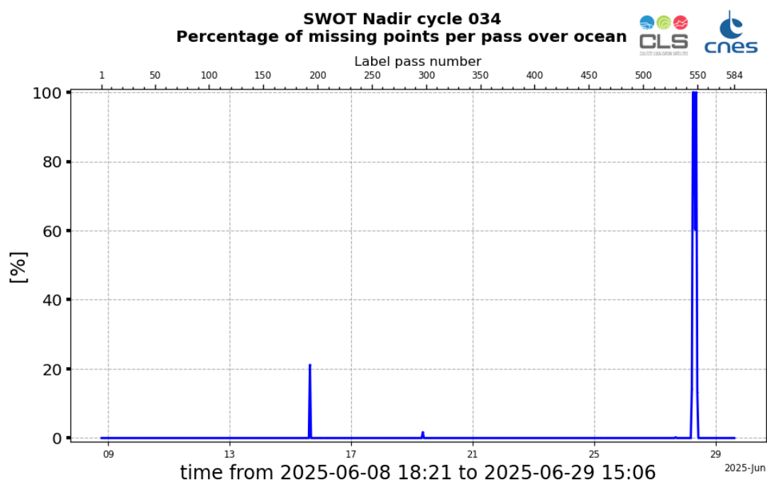
Figure 2: Monitoring of the percentage per pass of missing data over ocean, for SWOT Nadir GDR cycle 034
