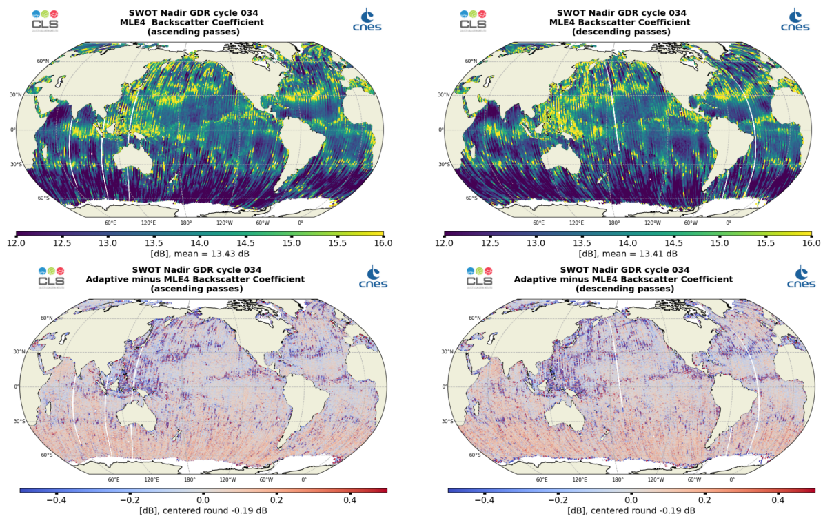
Figure 8: Along-track maps of Ku-band backscatter coefficient \sigma_0 over cycle 034 for SWOT Nadir MLE4 (top) or Adaptive minus MLE4 difference (bottom), ascending passes (left) and descending passes (right)
