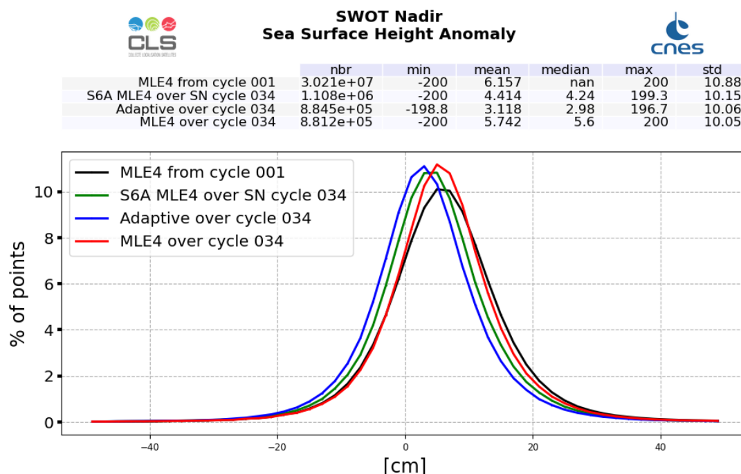
Figure 25: SSHA histogram computed over cycle 034 (red line for SWOT Nadir MLE4 and blue line for SWOT Nadir Adaptive, green for Sentinel-6A-MF (LR MLE4)) and from cycle 001 (SWOT Nadir, MLE4 only, black line)
