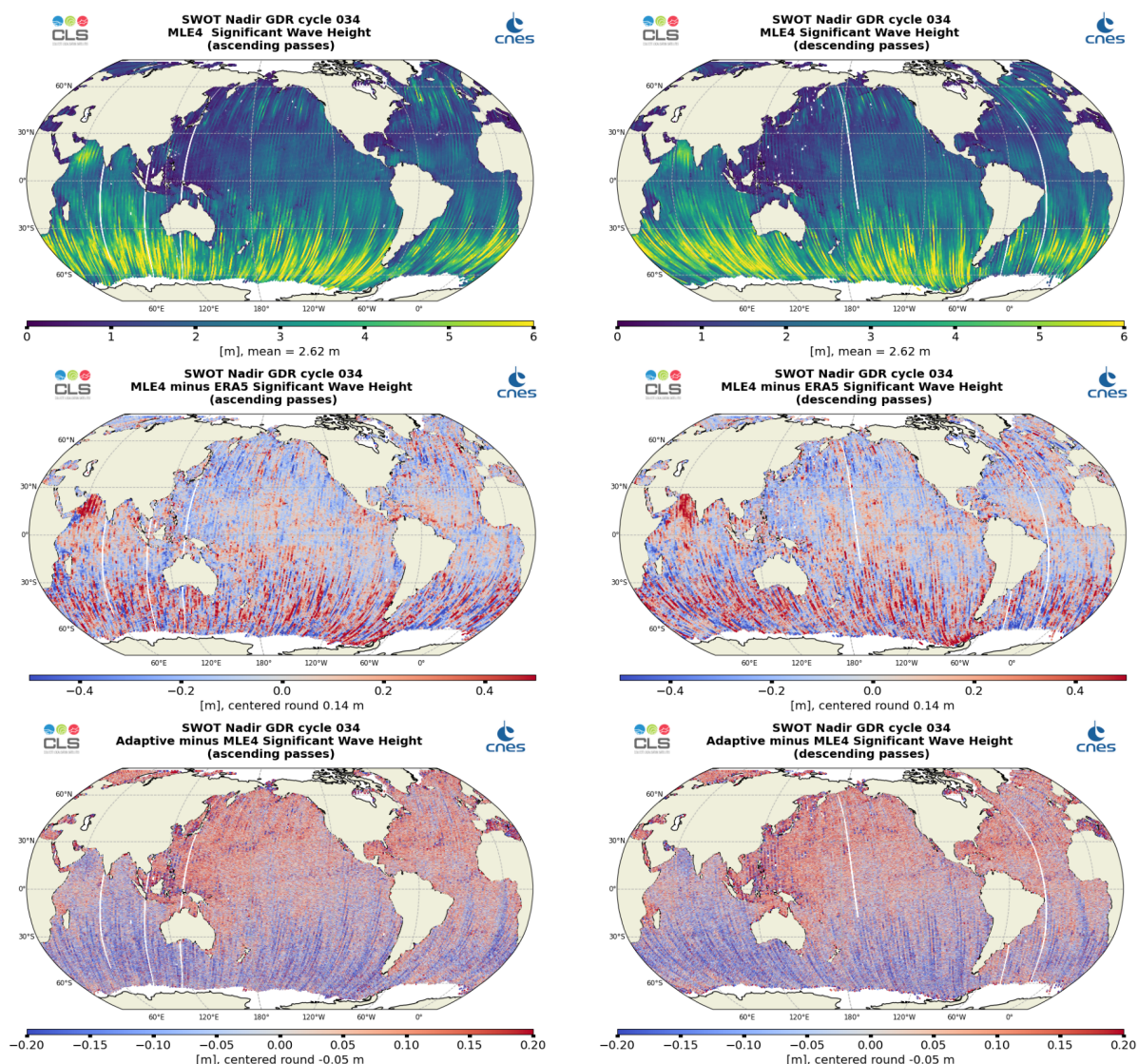
Figure 5: Along-track maps of Ku-band Significant Wave Height over cycle 034 for SWOT Nadir MLE4 (top), MLE4 minus model (middle) or Adaptive minus MLE4 (bottom), ascending passes (left) and descending passes (right)
