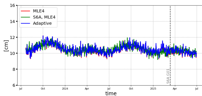
Figure 27: SSHA daily monitoring from cycle 001 to 034, for SWOT Nadir GDR
