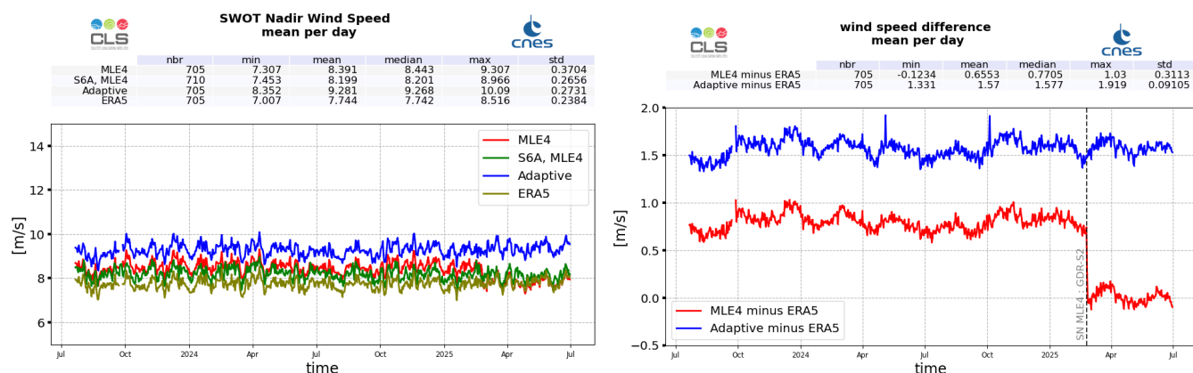
Figure 12: Wind Speed daily monitoring from cycle 001 to 034 for SWOT Nadir GDR, ERA5 model, and Sentinel-6A-MF (LR MLE4) (left), and daily mean difference with ERA5 (right)
