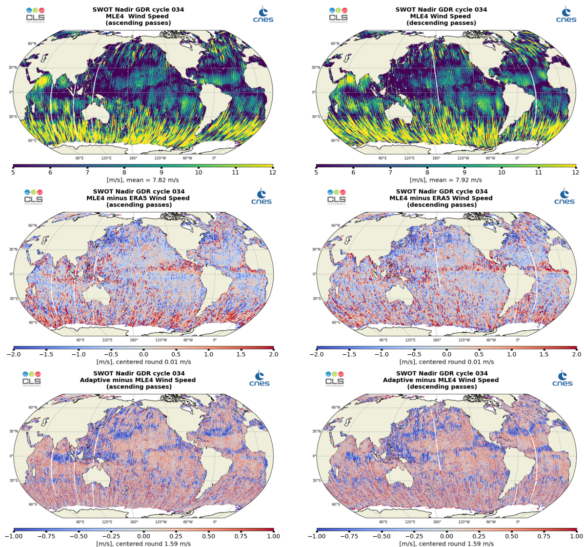
Figure 11: Along-track maps of Altimeter Wind Speed over cycle 034 for SWOT Nadir MLE4 (top), MLE4 minus ERA5 (middle) or Adaptive minus MLE4 (bottom), ascending passes (left) and descending passes (right)
