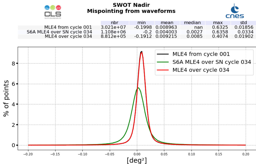
Figure 16: Mispointing histogram computed over cycle 034 (solid line) and from cycle 4 (dashed line)
