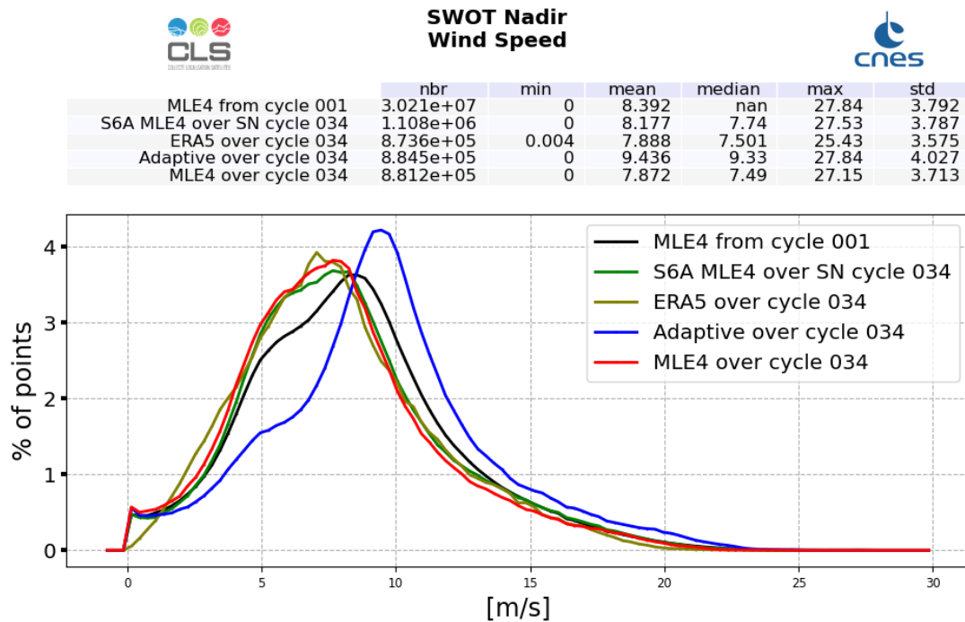
Figure 10: Altimeter Wind Speed histogram computed over cycle 034 (red line for SWOT Nadir MLE4 and blue line for SWOT Nadir Adaptive, green for Sentinel-6A-MF (LR MLE4)) and from cycle 001 (SWOT Nadir, MLE4 only, black line)
