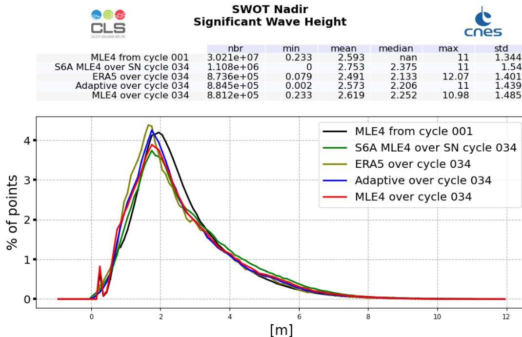
Figure 4: Ku-band Significant Wave Height histogram computed over cycle 034 (red line for SWOT Nadir MLE4 and blue line for SWOT Nadir Adaptive, green for Sentinel-6A-MF (LR MLE4) and dark green for ERA5) and from cycle 001 (SWOT Nadir, MLE4 only, black line)
