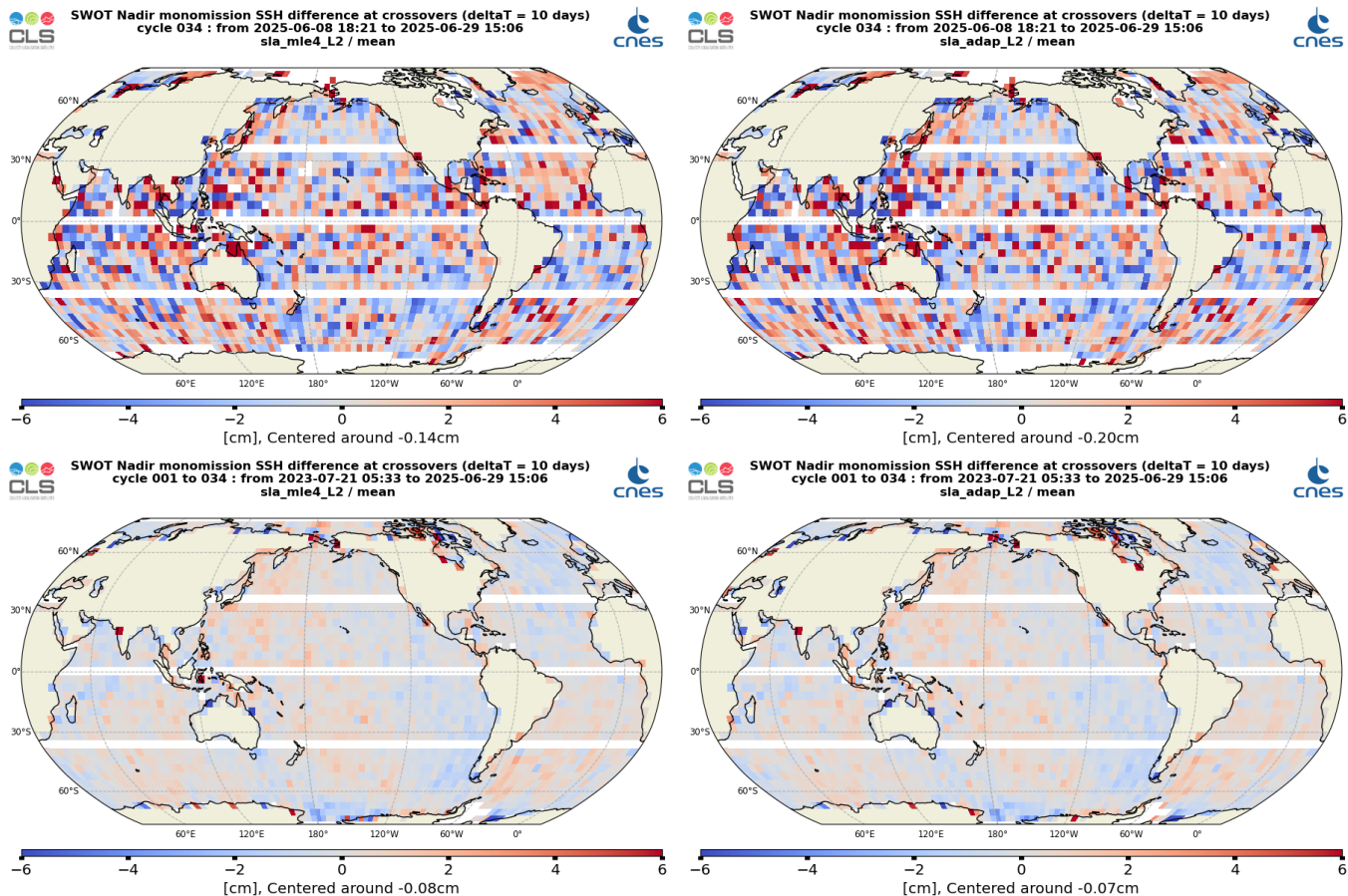
Figure 28: Mean SSH difference at crossovers for SWOT Nadir MLE4 (left) and Adaptive (right) cycle 034(top) and from cycle 001 to cycle 034 (bottom)
