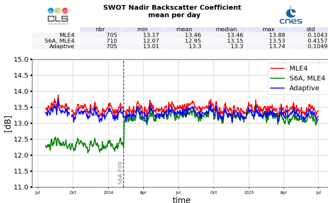
Figure 9: Ku-band Backscattering coefficient daily monitoring from cycle 001 to 034, for SWOT Nadir and Sentinel-6A-MF
