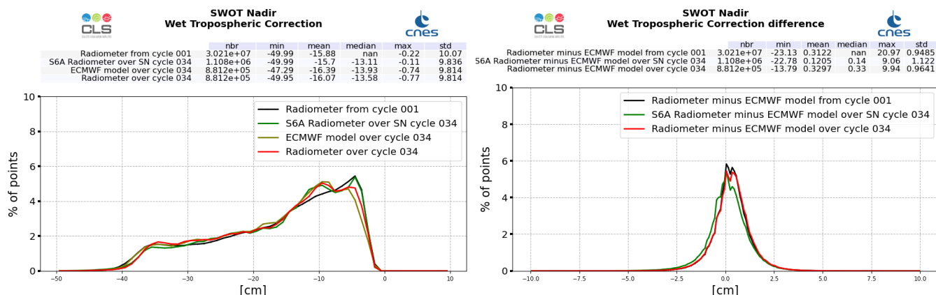
Figure 21: Histogram of wet troposphere corrections : SWOT Nadir radiometer (left) and difference with ECMWF model (right), computed over cycle 034 and from cycle 001 (black line)
