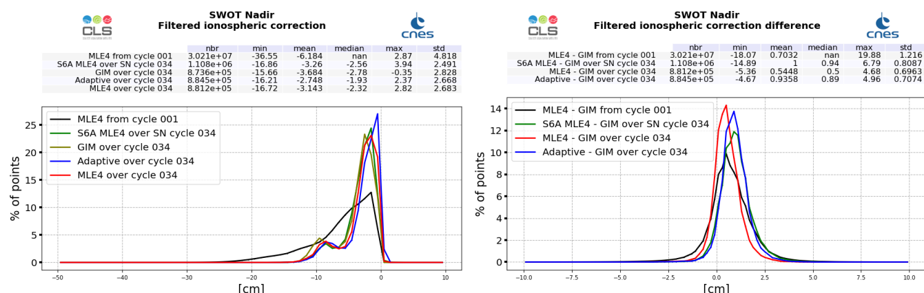
Figure 13: GIM model (dark green) and altimeter filtered ionosphere correction histogram computed over cycle 034 (red line for SWOT Nadir MLE4 and blue line for SWOT Nadir Adaptive, green for Sentinel-6A-MF (LR MLE4)) and from cycle 001 (SWOT Nadir, MLE4 only, black line) (left). Difference between filtered altimeter and GIM model (right).
