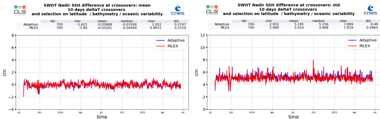
Figure 29: Monitoring of SSH difference at crossovers for SWOT Nadir MLE4 (red) and Adaptive (blue) : mean (left) and standard deviation (right), from cycle 001 to 034
