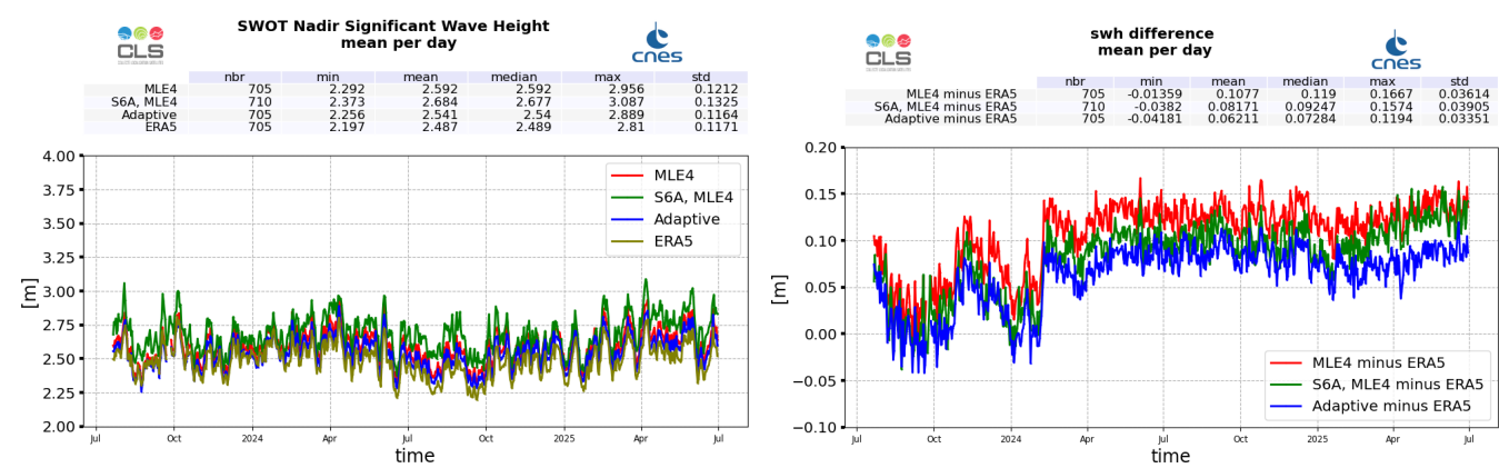
Figure 6: Ku-band Significant Wave Height daily monitoring from cycle 001 to 034, for SWOT Nadir, ERA5 model estimated at SWOT locations, and Sentinel-6A-MF (LR MLE4) (left), and difference with ERA5 model (right)
