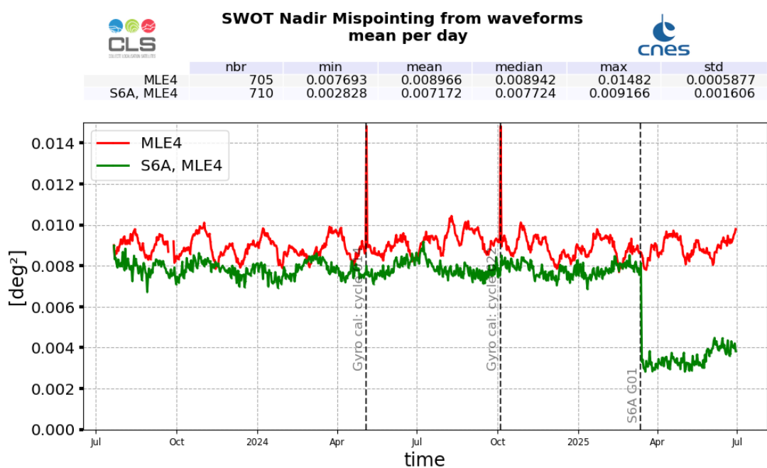
Figure 18: Mispointing daily monitoring from SWOT cycle 001 to 034 for SWOT Nadir GDR (red) and Sentinel-6A-MF (green)
