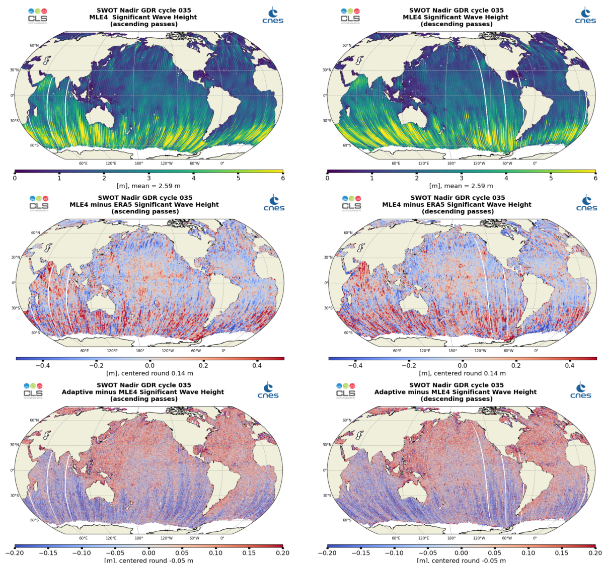
Figure 5: Along-track maps of Ku-band Significant Wave Height over cycle 035 for SWOT Nadir MLE4 (top), MLE4 minus model (middle) or Adaptive minus MLE4 (bottom), ascending passes (left) and descending passes (right)
