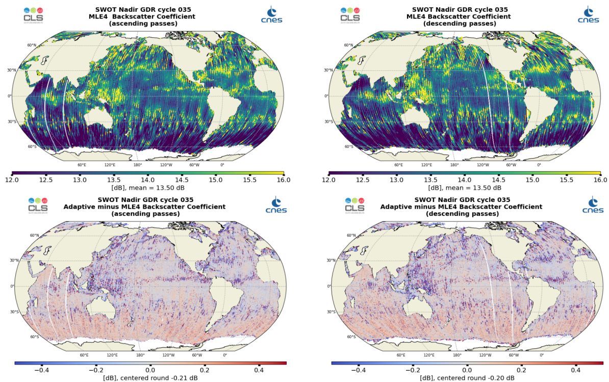
Figure 8: Along-track maps of Ku-band backscatter coefficient \sigma_0 over cycle 035 for SWOT Nadir MLE4 (top) or Adaptive minus MLE4 difference (bottom), ascending passes (left) and descending passes (right)
