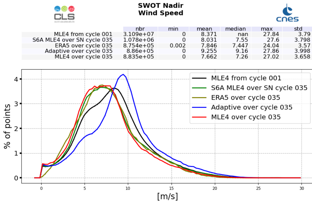
Figure 10: Altimeter Wind Speed histogram computed over cycle 035 (red line for SWOT Nadir MLE4 and blue line for SWOT Nadir Adaptive, green for Sentinel-6A-MF (LR MLE4)) and from cycle 001 (SWOT Nadir, MLE4 only, black line)
