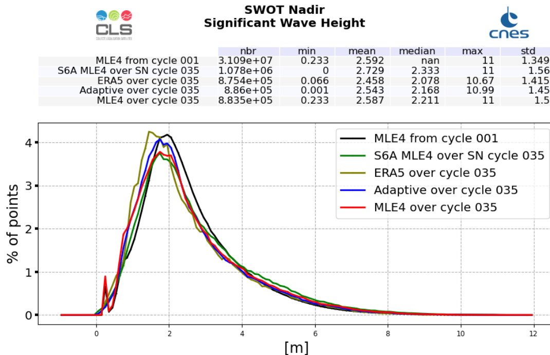
Figure 4: Ku-band Significant Wave Height histogram computed over cycle 035 (red line for SWOT Nadir MLE4 and blue line for SWOT Nadir Adaptive, green for Sentinel-6A-MF (LR MLE4) and dark green for ERA5) and from cycle 001 (SWOT Nadir, MLE4 only, black line)
