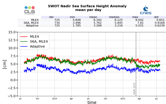
Figure 27: SSHA daily monitoring from cycle 001 to 035, for SWOT Nadir GDR
