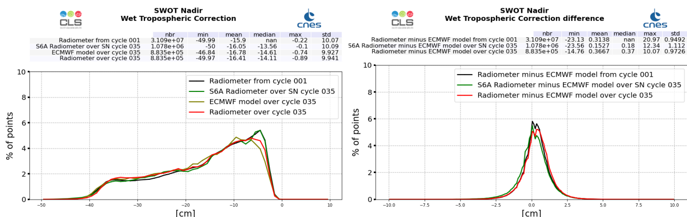
Figure 21: Histogram of wet troposphere corrections : SWOT Nadir radiometer (left) and difference with ECMWF model (right), computed over cycle 035 and from cycle 001 (black line)
