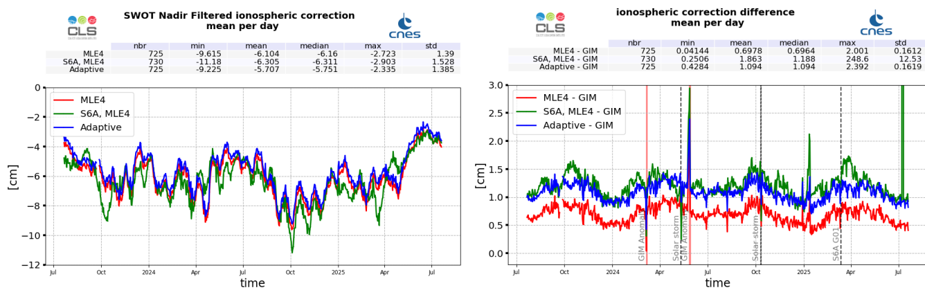
Figure 15: SWOT Nadir MLE4 (red), Adaptive (blue) and Sentinel-6A-MF (LR MLE4) (green) filtered ionosphere correction daily monitoring from cycle 001 to 035 (left) and difference with GIM model (right)
