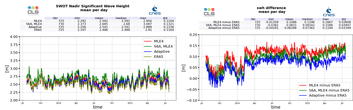
Figure 6: Ku-band Significant Wave Height daily monitoring from cycle 001 to 035, for SWOT Nadir, ERA5 model estimated at SWOT locations, and Sentinel-6A-MF (LR MLE4) (left), and difference with ERA5 model (right)
