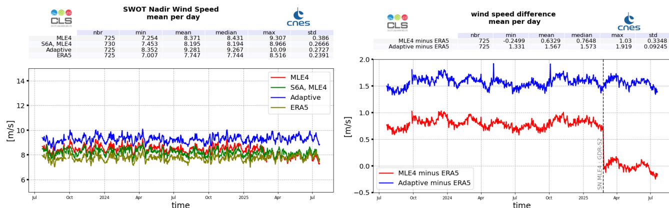
Figure 12: Wind Speed daily monitoring from cycle 001 to 035 for SWOT Nadir GDR, ERA5 model, and Sentinel-6A-MF (LR MLE4) (left), and daily mean difference with ERA5 (right)
