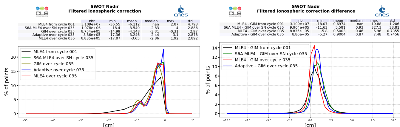
Figure 13: GIM model (dark green) and altimeter filtered ionosphere correction histogram computed over cycle 035 (red line for SWOT Nadir MLE4 and blue line for SWOT Nadir Adaptive, green for Sentinel-6A-MF (LR MLE4)) and from cycle 001 (SWOT Nadir, MLE4 only, black line) (left). Difference between filtered altimeter and GIM model (right).
