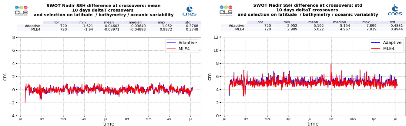
Figure 29: Monitoring of SSH difference at crossovers for SWOT Nadir MLE4 (red) and Adaptive (blue) : mean (left) and standard deviation (right), from cycle 001 to 035
