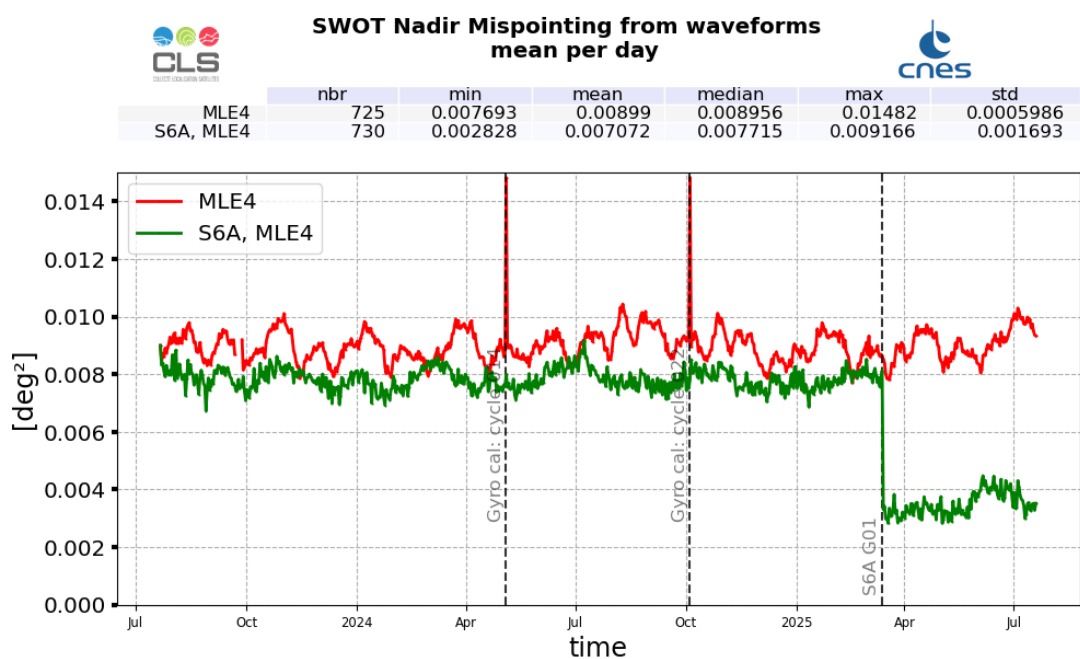
Figure 18: Mispointing daily monitoring from SWOT cycle 001 to 035 for SWOT Nadir GDR (red) and Sentinel-6A-MF (green)
