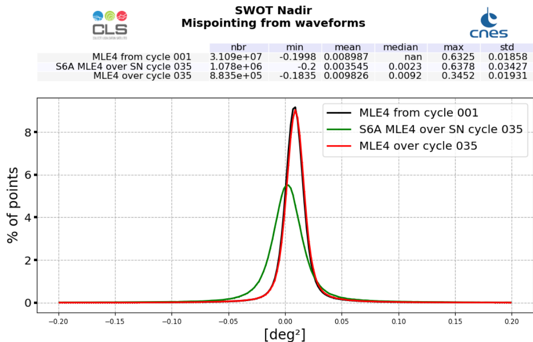
Figure 16: Mispointing histogram computed over cycle 035 (solid line) and from cycle 4 (dashed line)
