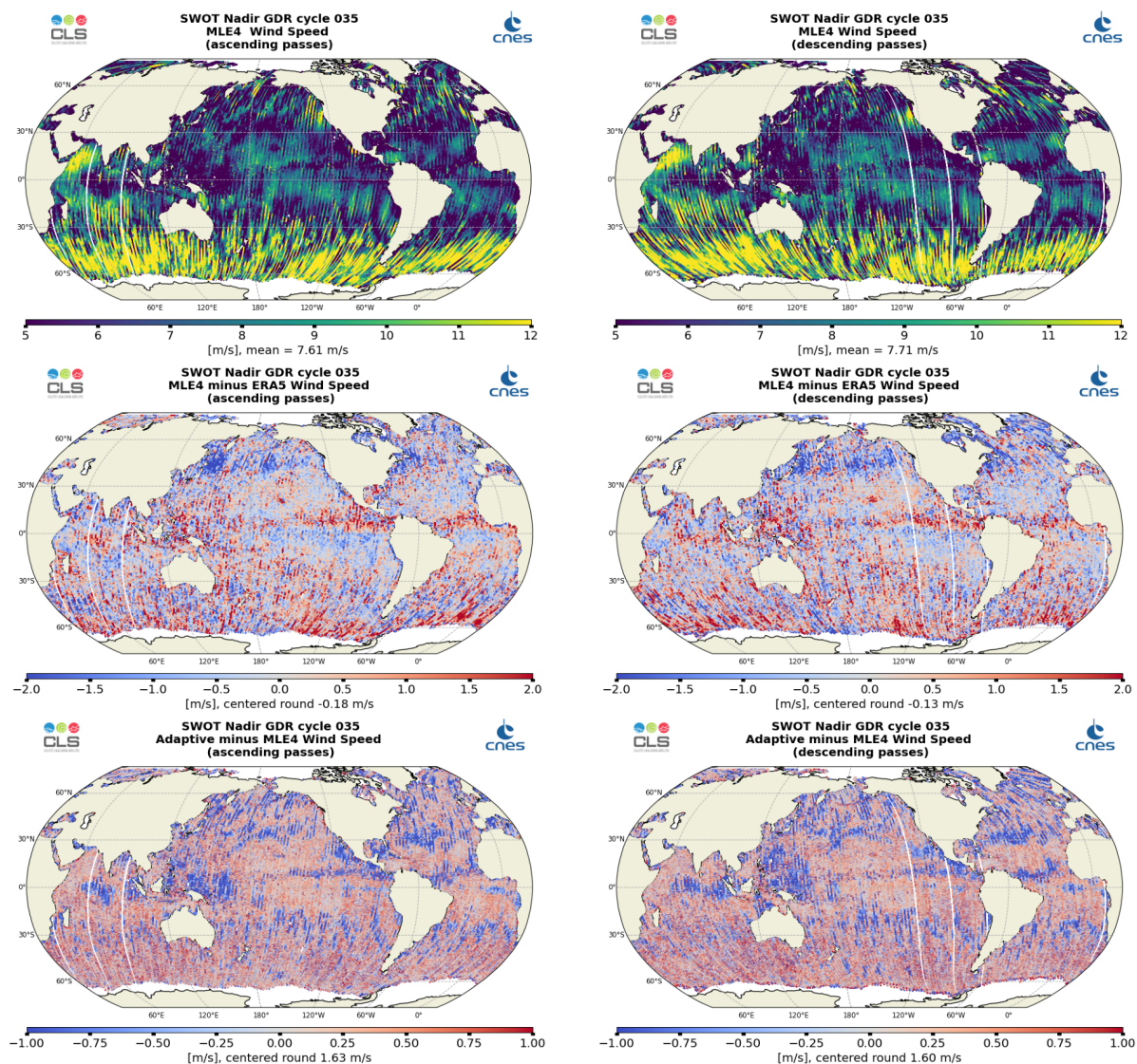
Figure 11: Along-track maps of Altimeter Wind Speed over cycle 035 for SWOT Nadir MLE4 (top), MLE4 minus ERA5 (middle) or Adaptive minus MLE4 (bottom), ascending passes (left) and descending passes (right)
