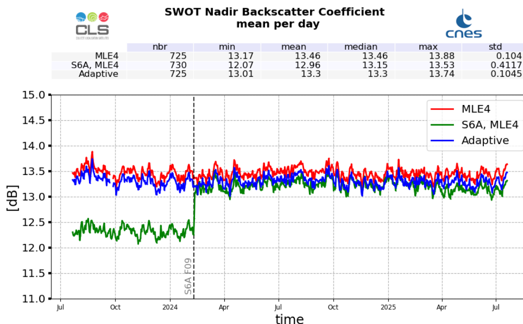
Figure 9: Ku-band Backscattering coefficient daily monitoring from cycle 001 to 035, for SWOT Nadir and Sentinel-6A-MF
