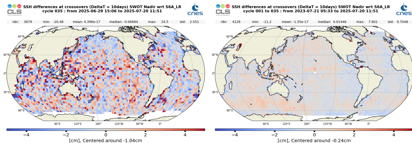
Figure 30: Mean SSH difference at crossovers between SWOT Nadir MLE4 and Sentinel-6 MF LR MLE4 over cycle 035 (left) and from cycle 001 onwards (right)
