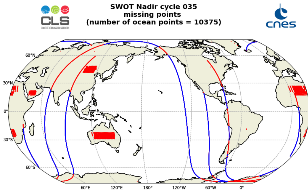
Figure 1: Map of missing measurements for SWOT Nadir GDR cycle 035
