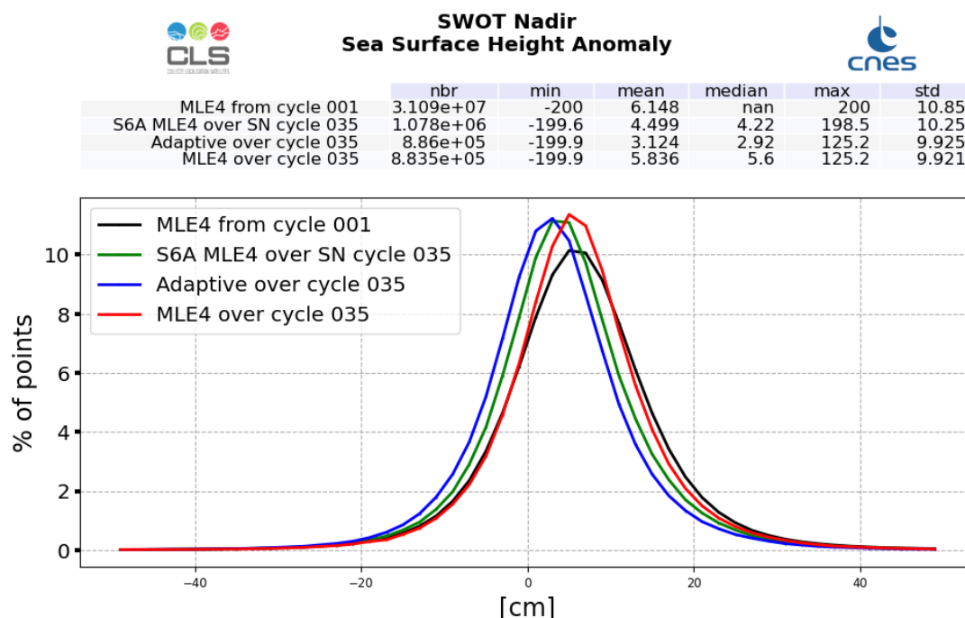
Figure 25: SSHA histogram computed over cycle 035 (red line for SWOT Nadir MLE4 and blue line for SWOT Nadir Adaptive, green for Sentinel-6A-MF (LR MLE4)) and from cycle 001 (SWOT Nadir, MLE4 only, black line)
