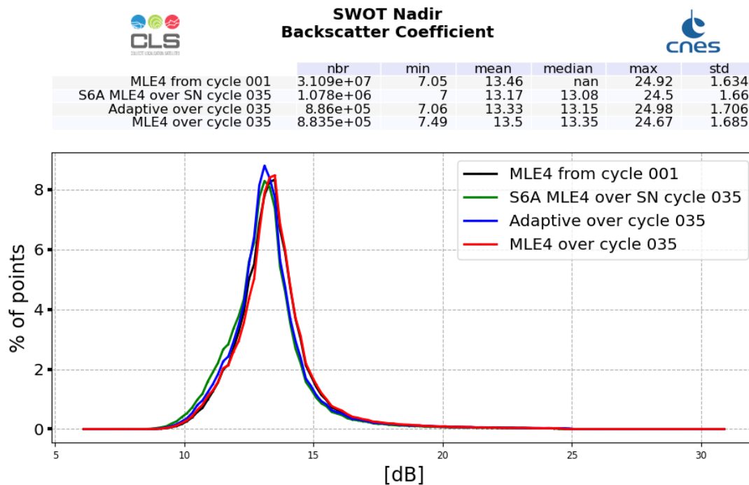
Figure 7: Ku-band Backscattering coefficient histogram computed over cycle 035 (red line for SWOT Nadir MLE4 and blue line for SWOT Nadir Adaptive, green for Sentinel-6A-MF (LR MLE4)) and from cycle 001 (SWOT Nadir, MLE4 only, black line)
