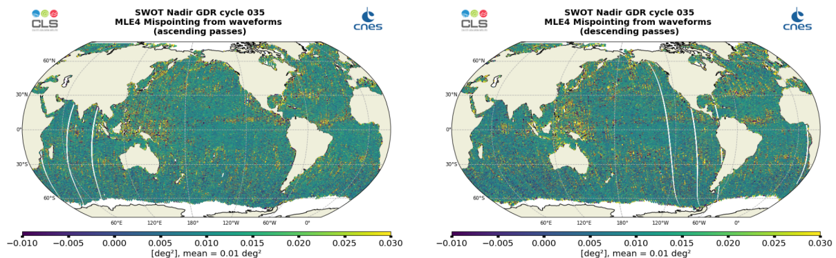
Figure 17: Along-track maps of mispointing over cycle 035 for SWOT Nadir MLE4, ascending passes (left) and descending passes (right)
