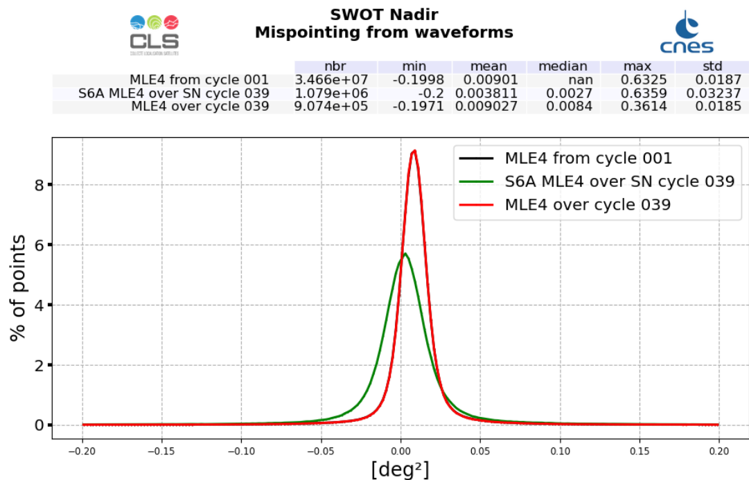
Figure 16: Mispointing histogram computed over cycle 039 (solid line) and from cycle 4 (dashed line)
