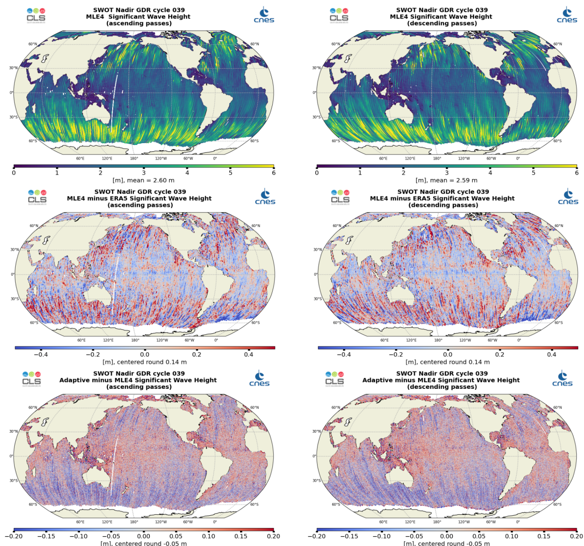
Figure 5: Along-track maps of Ku-band Significant Wave Height over cycle 039 for SWOT Nadir MLE4 (top), MLE4 minus model (middle) or Adaptive minus MLE4 (bottom), ascending passes (left) and descending passes (right)
