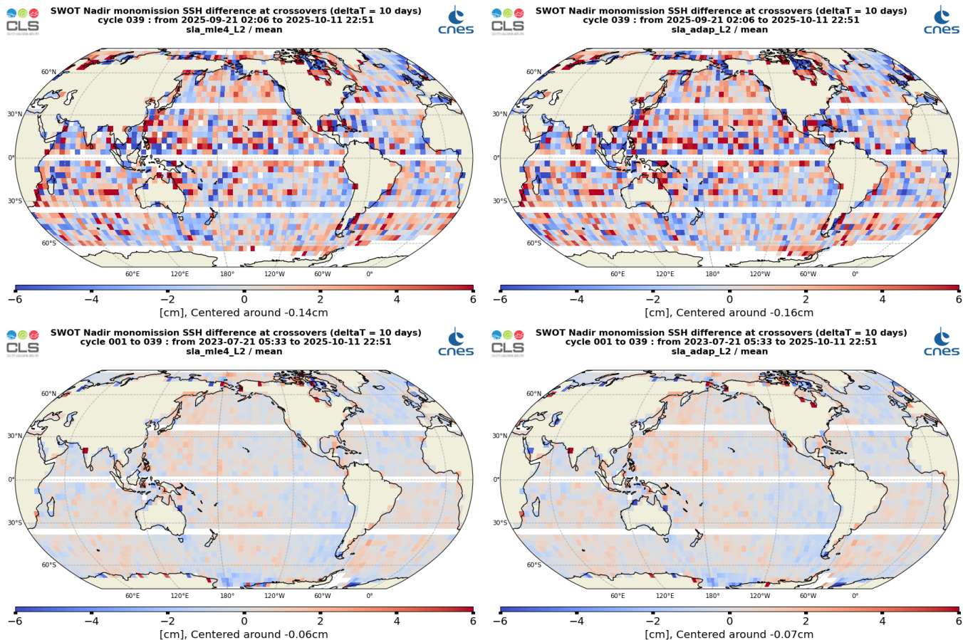
Figure 28: Mean SSH difference at crossovers for SWOT Nadir MLE4 (left) and Adaptive (right) cycle 039(top) and from cycle 001 to cycle 039 (bottom)
