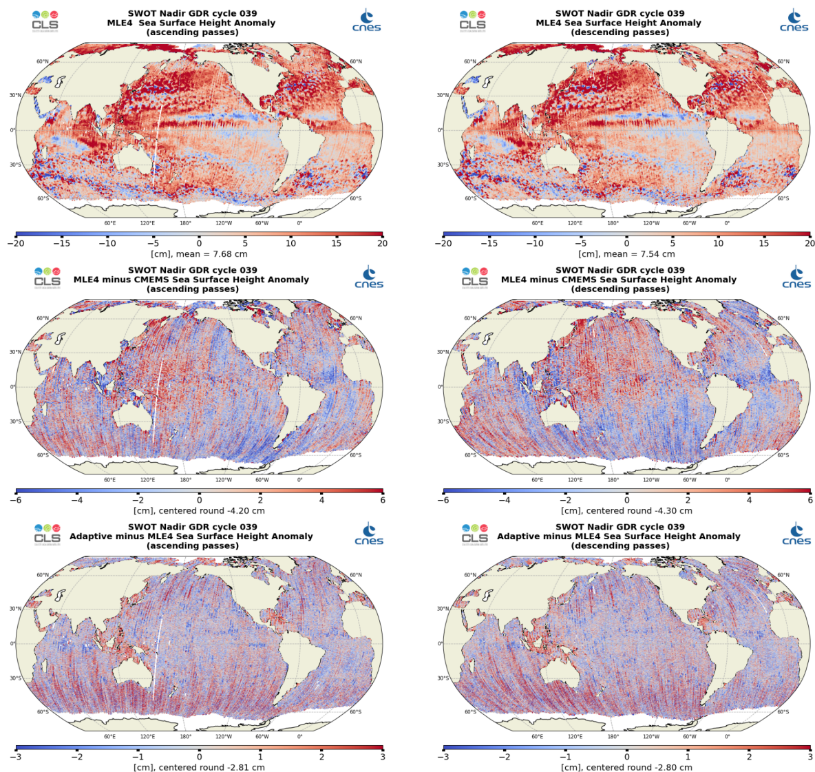
Figure 26: Along-track maps of SSHA over cycle 039 for SWOT Nadir MLE4 (top), MLE4 minus CMEMS (middle) or Adaptive minus MLE4 (bottom), ascending passes (left) and descending passes (right)
