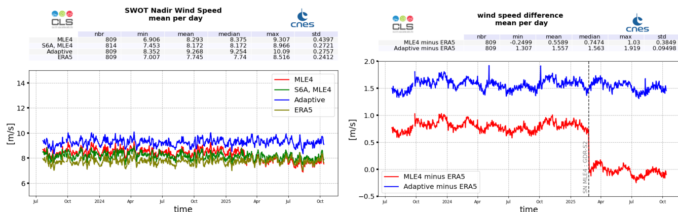
Figure 12: Wind Speed daily monitoring from cycle 001 to 039 for SWOT Nadir GDR, ERA5 model, and Sentinel-6A-MF (LR MLE4) (left), and daily mean difference with ERA5 (right)
