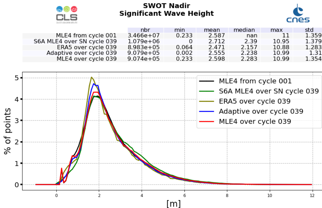
Figure 4: Ku-band Significant Wave Height histogram computed over cycle 039 (red line for SWOT Nadir MLE4 and blue line for SWOT Nadir Adaptive, green for Sentinel-6A-MF (LR MLE4) and dark green for ERA5) and from cycle 001 (SWOT Nadir, MLE4 only, black line)
