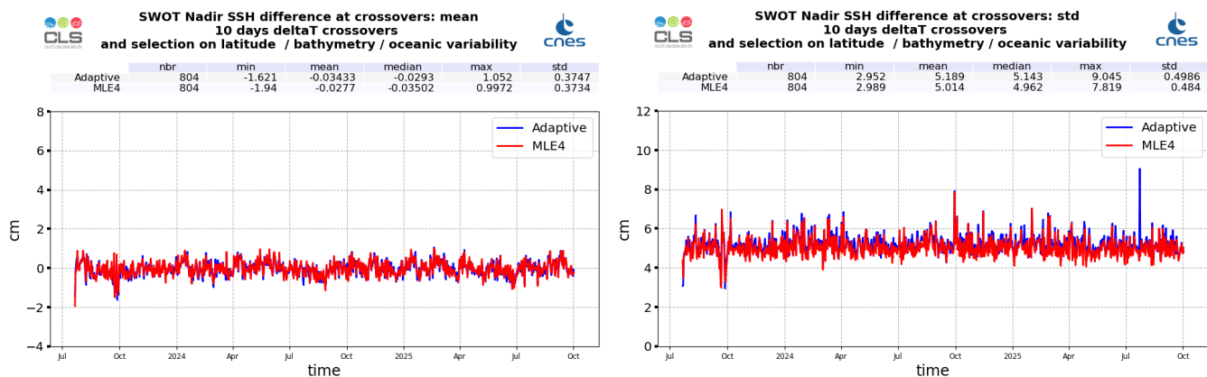
Figure 29: Monitoring of SSH difference at crossovers for SWOT Nadir MLE4 (red) and Adaptive (blue) : mean (left) and standard deviation (right), from cycle 001 to 039
