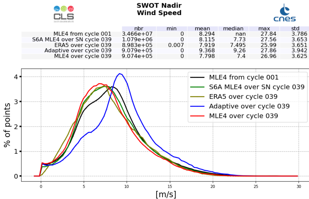
Figure 10: Altimeter Wind Speed histogram computed over cycle 039 (red line for SWOT Nadir MLE4 and blue line for SWOT Nadir Adaptive, green for Sentinel-6A-MF (LR MLE4)) and from cycle 001 (SWOT Nadir, MLE4 only, black line)
