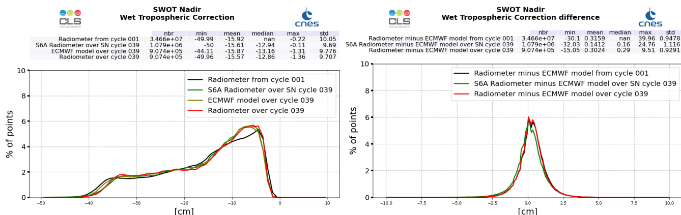
Figure 21: Histogram of wet troposphere corrections : SWOT Nadir radiometer (left) and difference with ECMWF model (right), computed over cycle 039 and from cycle 001 (black line)
