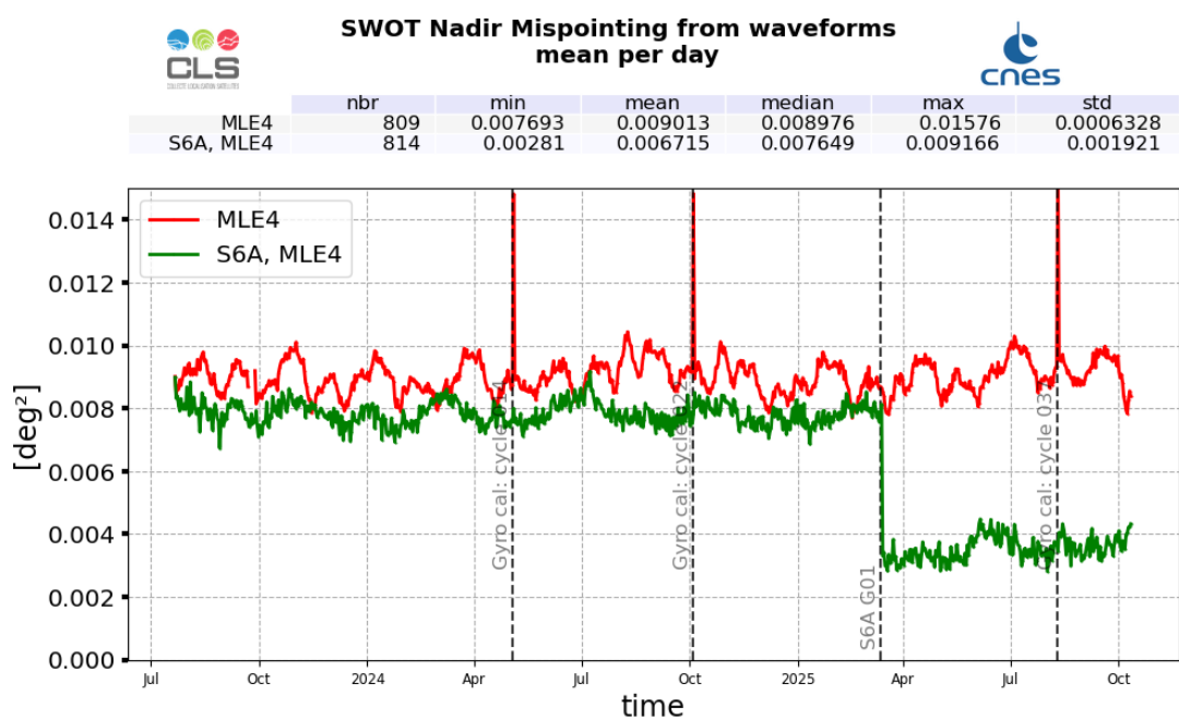
Figure 18: Mispointing daily monitoring from SWOT cycle 001 to 039 for SWOT Nadir GDR (red) and Sentinel-6A-MF (green)
