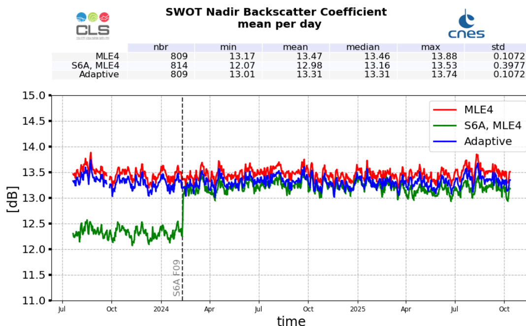
Figure 9: Ku-band Backscattering coefficient daily monitoring from cycle 001 to 039, for SWOT Nadir and Sentinel-6A-MF
