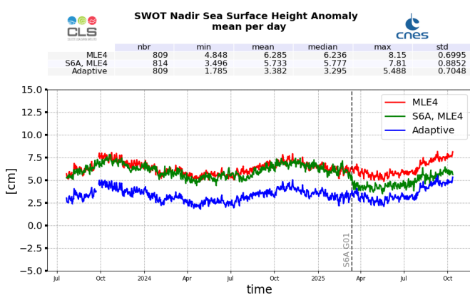
Figure 27: SSHA daily monitoring from cycle 001 to 039, for SWOT Nadir GDR
