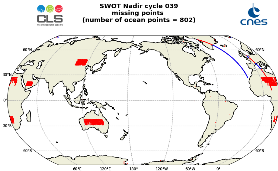
Figure 1: Map of missing measurements for SWOT Nadir GDR cycle 039
