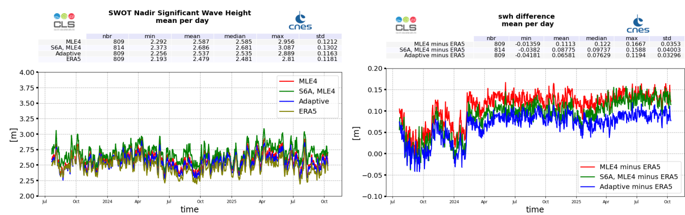
Figure 6: Ku-band Significant Wave Height daily monitoring from cycle 001 to 039, for SWOT Nadir, ERA5 model estimated at SWOT locations, and Sentinel-6A-MF (LR MLE4) (left), and difference with ERA5 model (right)
