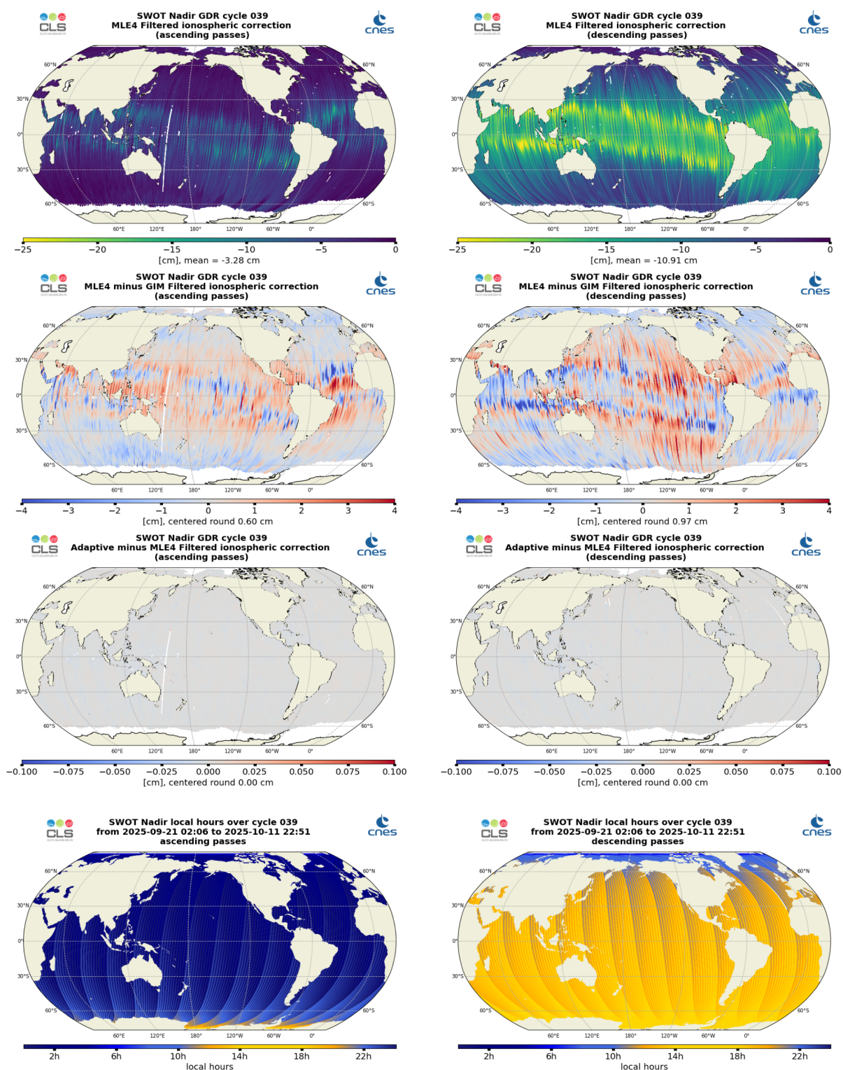
Figure 14: Along-track maps of filtered ionosphere correction over cycle 039 for SWOT Nadir MLE4 (top), MLE4 minus GIM (middle top) or Adaptive minus MLE4 (middle bottom), and local hours (bottom), for ascending passes (left) and descending passes (right)
