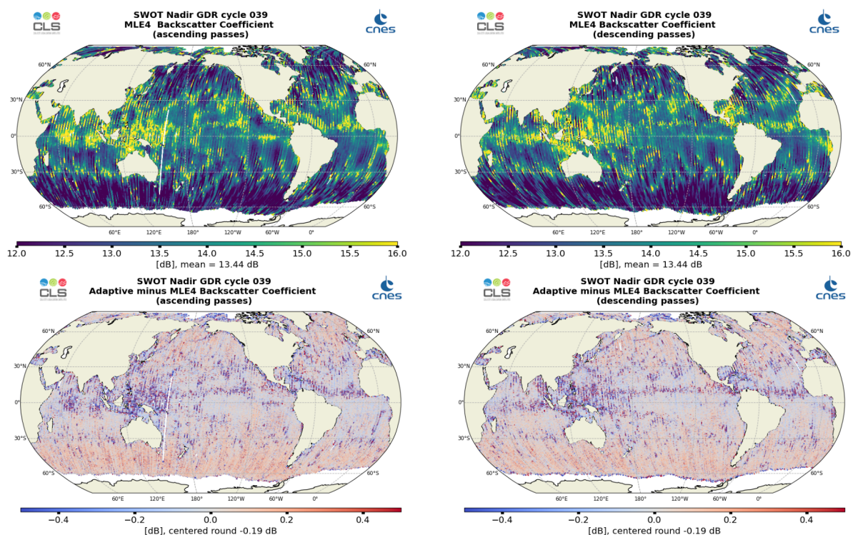
Figure 8: Along-track maps of Ku-band backscatter coefficient \sigma_0 over cycle 039 for SWOT Nadir MLE4 (top) or Adaptive minus MLE4 difference (bottom), ascending passes (left) and descending passes (right)
