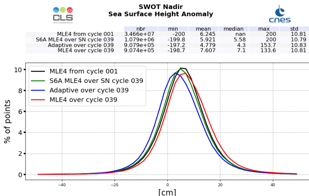
Figure 25: SSHA histogram computed over cycle 039 (red line for SWOT Nadir MLE4 and blue line for SWOT Nadir Adaptive, green for Sentinel-6A-MF (LR MLE4)) and from cycle 001 (SWOT Nadir, MLE4 only, black line)
