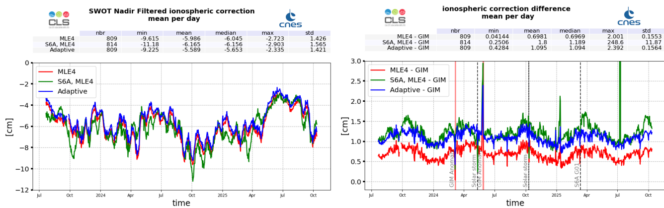
Figure 15: SWOT Nadir MLE4 (red), Adaptive (blue) and Sentinel-6A-MF (LR MLE4) (green) filtered ionosphere correction daily monitoring from cycle 001 to 039 (left) and difference with GIM model (right)
