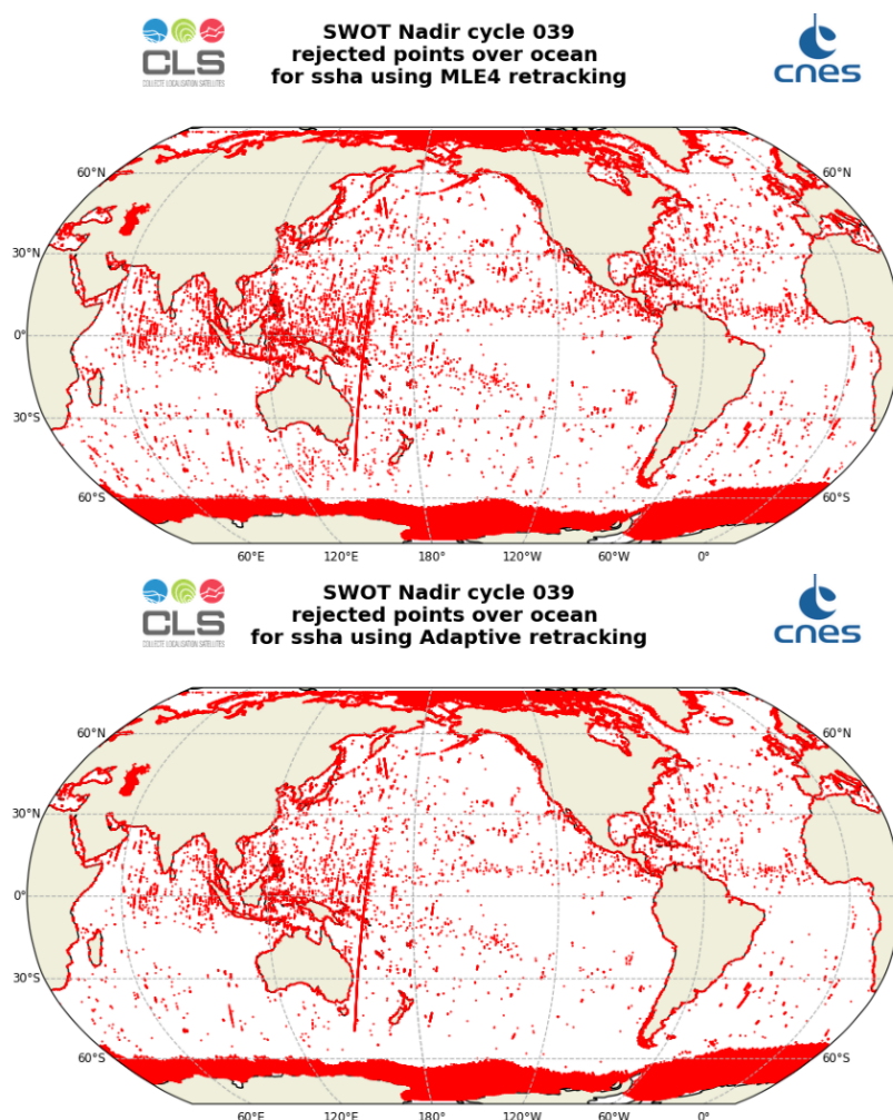
Figure 3: Edited measurements for SWOT Nadir over cycle 039
