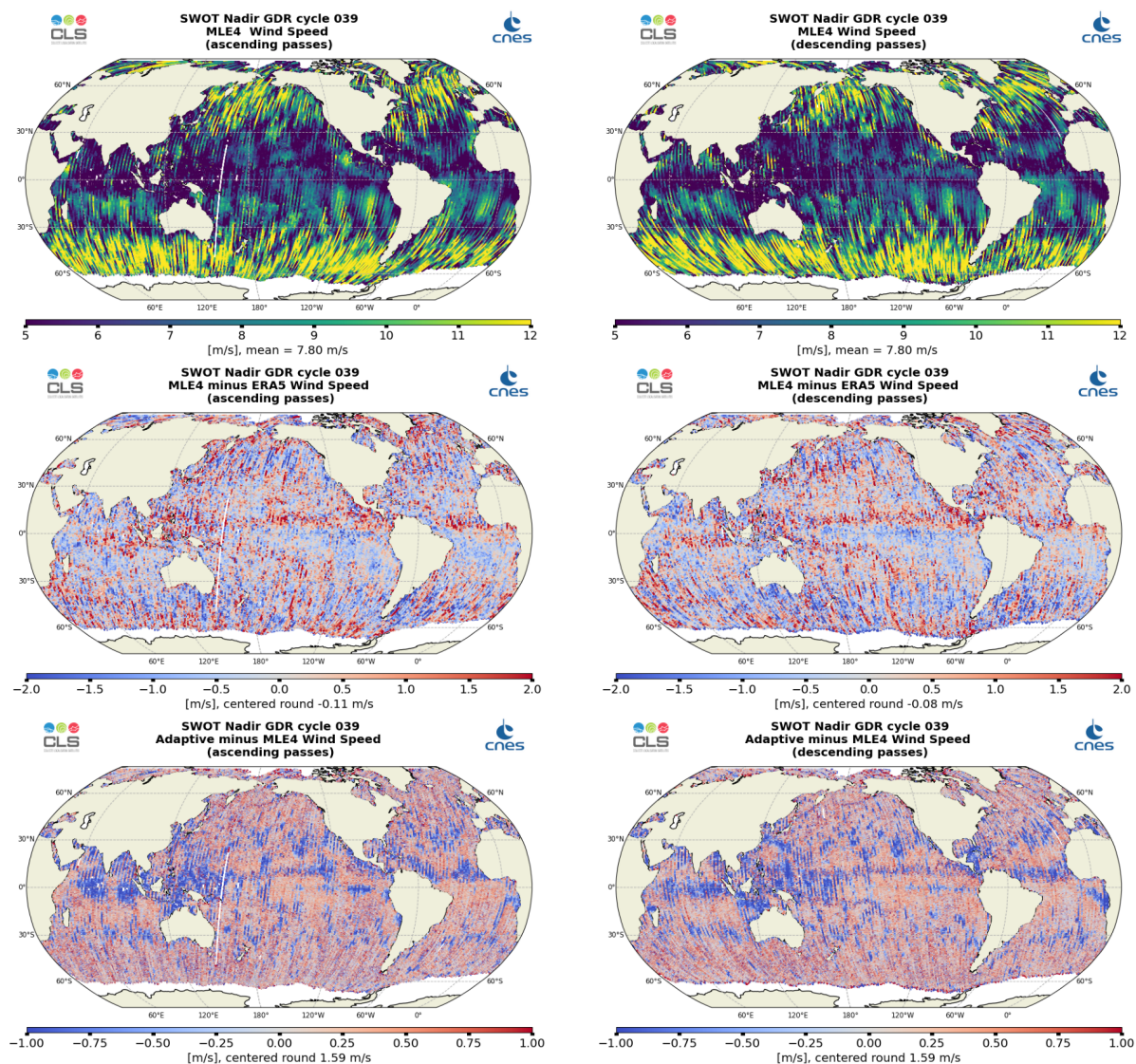
Figure 11: Along-track maps of Altimeter Wind Speed over cycle 039 for SWOT Nadir MLE4 (top), MLE4 minus ERA5 (middle) or Adaptive minus MLE4 (bottom), ascending passes (left) and descending passes (right)
