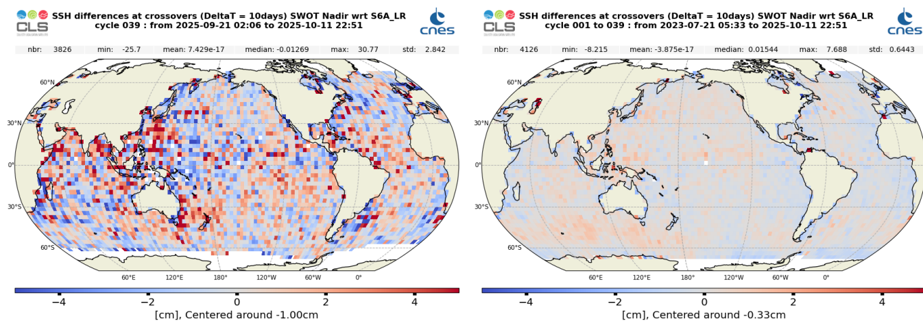
Figure 30: Mean SSH difference at crossovers between SWOT Nadir MLE4 and Sentinel-6 MF LR MLE4 over cycle 039 (left) and from cycle 001 onwards (right)
