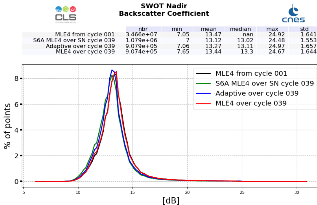
Figure 7: Ku-band Backscattering coefficient histogram computed over cycle 039 (red line for SWOT Nadir MLE4 and blue line for SWOT Nadir Adaptive, green for Sentinel-6A-MF (LR MLE4)) and from cycle 001 (SWOT Nadir, MLE4 only, black line)
