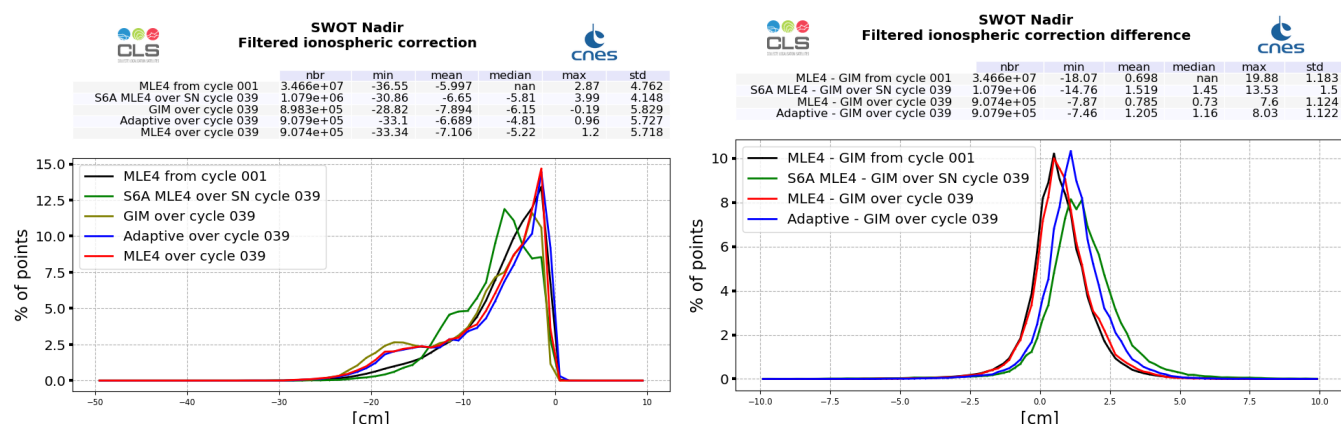
Figure 13: GIM model (dark green) and altimeter filtered ionosphere correction histogram computed over cycle 039 (red line for SWOT Nadir MLE4 and blue line for SWOT Nadir Adaptive, green for Sentinel-6A-MF (LR MLE4)) and from cycle 001 (SWOT Nadir, MLE4 only, black line) (left). Difference between filtered altimeter and GIM model (right).
