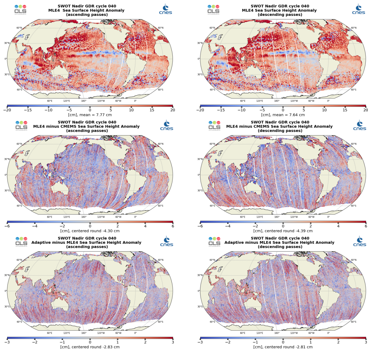
Figure 26: Along-track maps of SSHA over cycle 040 for SWOT Nadir MLE4 (top), MLE4 minus CMEMS (middle) or Adaptive minus MLE4 (bottom), ascending passes (left) and descending passes (right)
