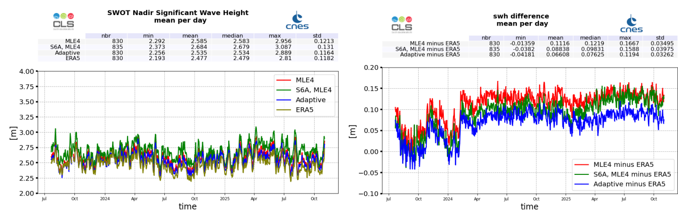
Figure 6: Ku-band Significant Wave Height daily monitoring from cycle 001 to 040, for SWOT Nadir, ERA5 model estimated at SWOT locations, and Sentinel-6A-MF (LR MLE4) (left), and difference with ERA5 model (right)
