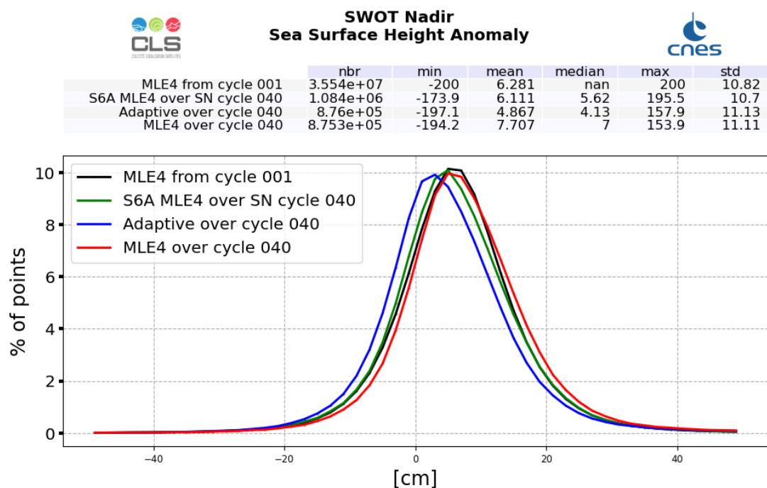
Figure 25: SSHA histogram computed over cycle 040 (red line for SWOT Nadir MLE4 and blue line for SWOT Nadir Adaptive, green for Sentinel-6A-MF (LR MLE4)) and from cycle 001 (SWOT Nadir, MLE4 only, black line)
