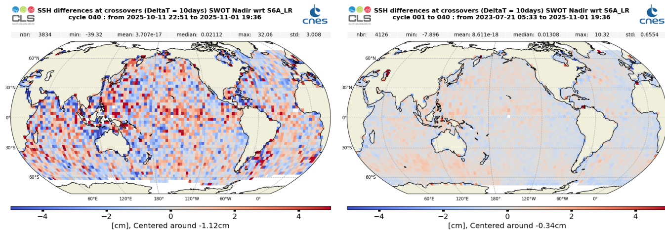
Figure 30: Mean SSH difference at crossovers between SWOT Nadir MLE4 and Sentinel-6 MF LR MLE4 over cycle 040 (left) and from cycle 001 onwards (right)
