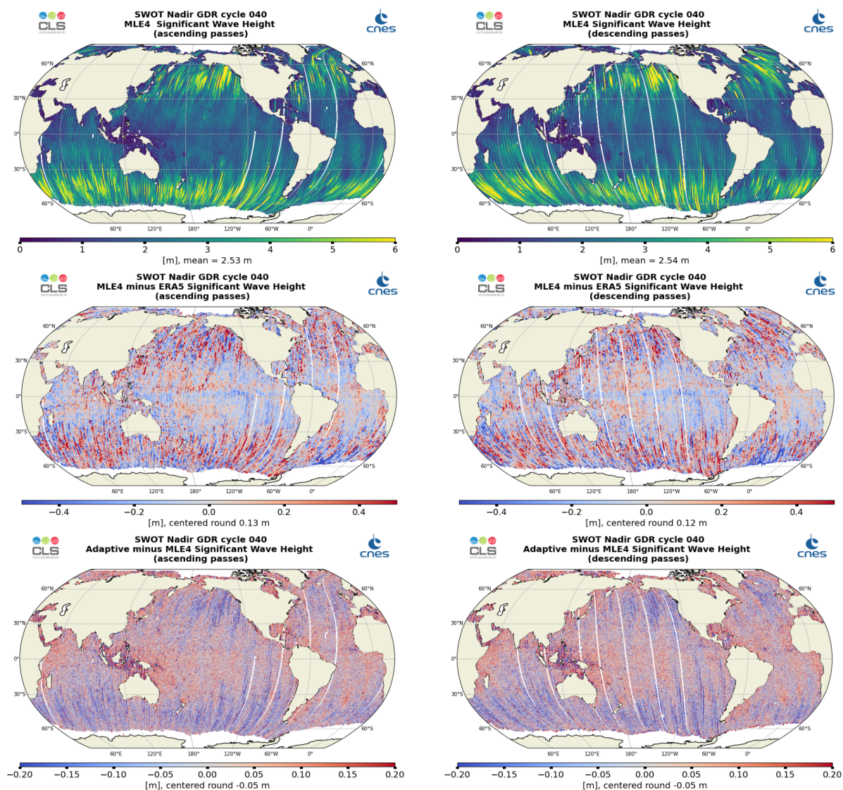
Figure 5: Along-track maps of Ku-band Significant Wave Height over cycle 040 for SWOT Nadir MLE4 (top), MLE4 minus model (middle) or Adaptive minus MLE4 (bottom), ascending passes (left) and descending passes (right)
