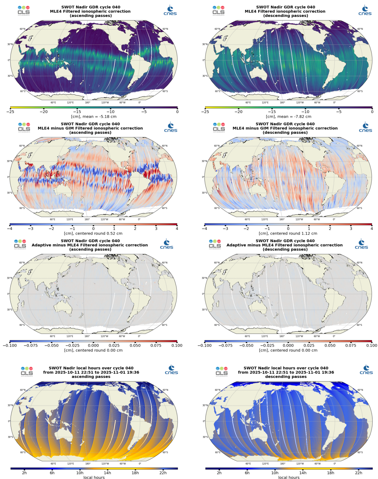
Figure 14: Along-track maps of filtered ionosphere correction over cycle 040 for SWOT Nadir MLE4 (top), MLE4 minus GIM (middle top) or Adaptive minus MLE4 (middle bottom), and local hours (bottom), for ascending passes (left) and descending passes (right)
