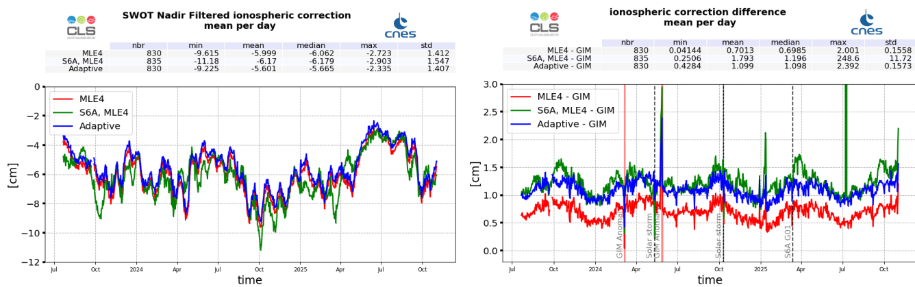
Figure 15: SWOT Nadir MLE4 (red), Adaptive (blue) and Sentinel-6A-MF (LR MLE4) (green) filtered ionosphere correction daily monitoring from cycle 001 to 040 (left) and difference with GIM model (right)
