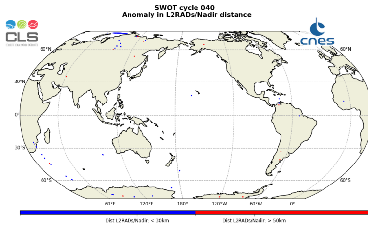
Figure 24: Map of the anomalies detected in the L2RADs/Nadir distance over the cycle 040
