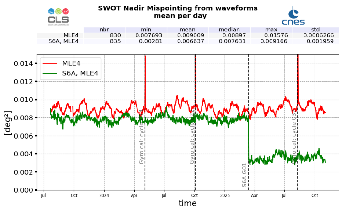
Figure 18: Mispointing daily monitoring from SWOT cycle 001 to 040 for SWOT Nadir GDR (red) and Sentinel-6A-MF (green)
