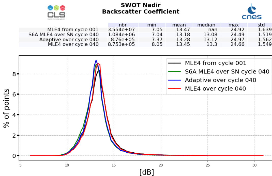
Figure 7: Ku-band Backscattering coefficient histogram computed over cycle 040 (red line for SWOT Nadir MLE4 and blue line for SWOT Nadir Adaptive, green for Sentinel-6A-MF (LR MLE4)) and from cycle 001 (SWOT Nadir, MLE4 only, black line)
