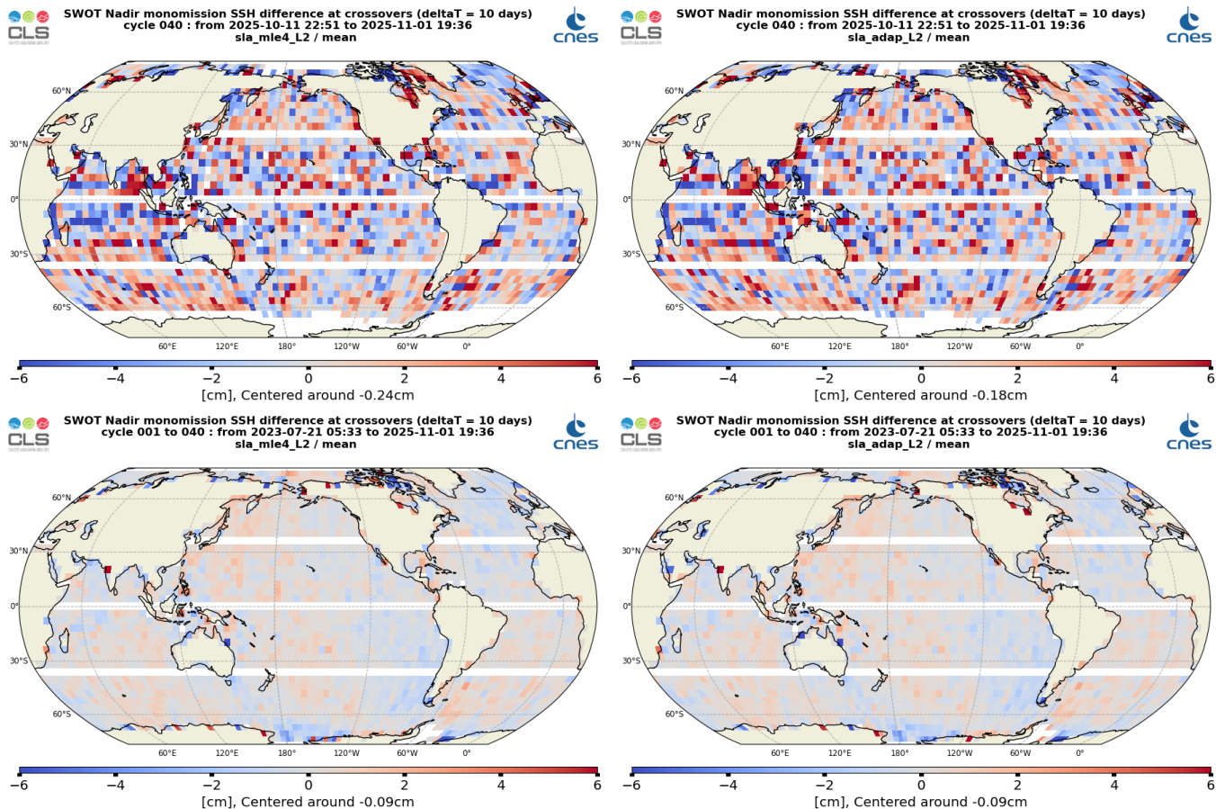
Figure 28: Mean SSH difference at crossovers for SWOT Nadir MLE4 (left) and Adaptive (right) cycle 040(top) and from cycle 001 to cycle 040 (bottom)
