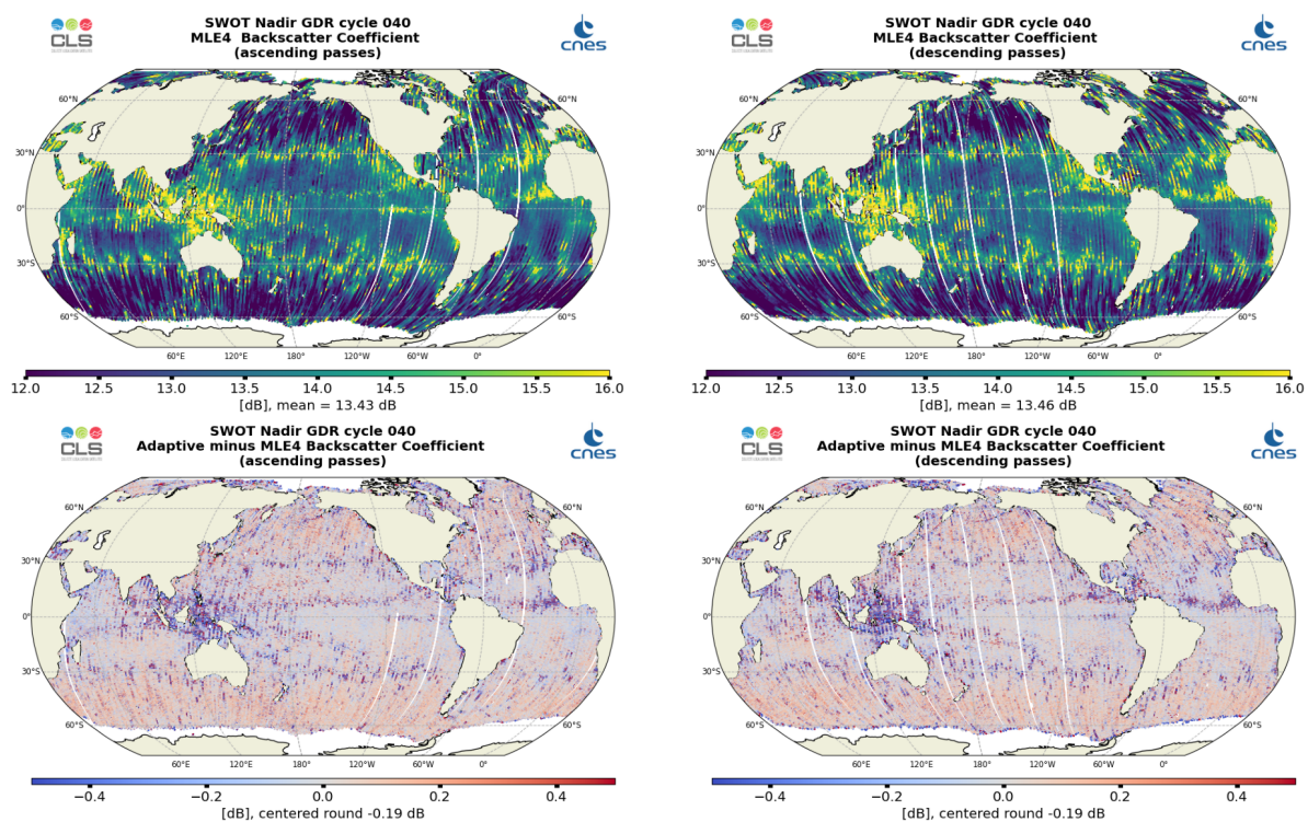
Figure 8: Along-track maps of Ku-band backscatter coefficient \sigma_0 over cycle 040 for SWOT Nadir MLE4 (top) or Adaptive minus MLE4 difference (bottom), ascending passes (left) and descending passes (right)
