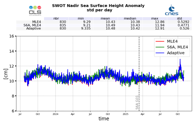
Figure 27: SSHA daily monitoring from cycle 001 to 040, for SWOT Nadir GDR
