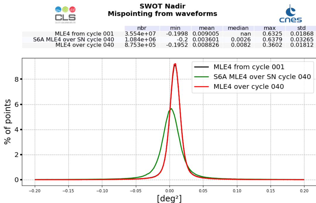
Figure 16: Mispointing histogram computed over cycle 040 (solid line) and from cycle 4 (dashed line)
