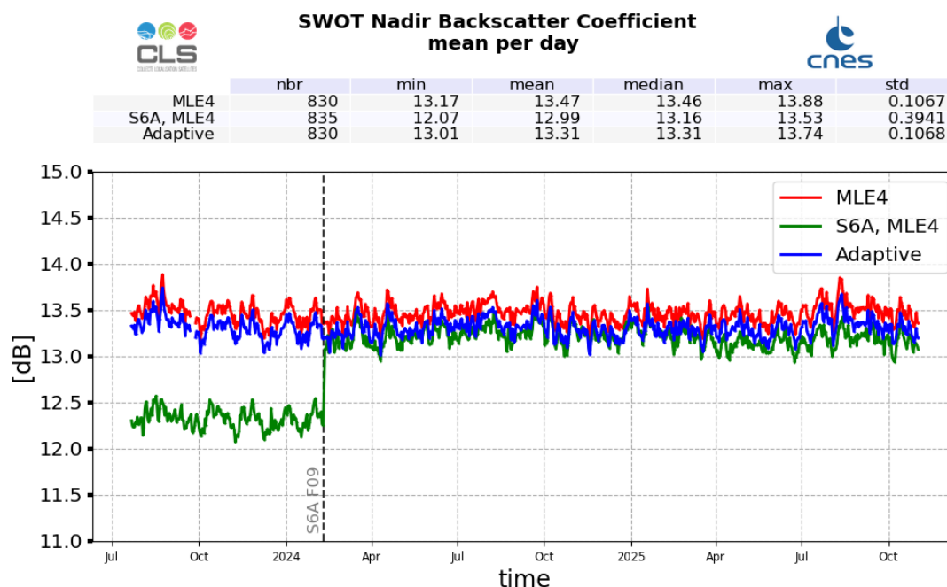
Figure 9: Ku-band Backscattering coefficient daily monitoring from cycle 001 to 040, for SWOT Nadir and Sentinel-6A-MF
