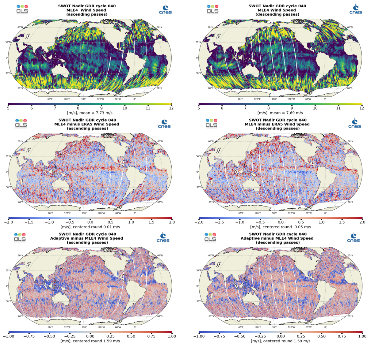
Figure 11: Along-track maps of Altimeter Wind Speed over cycle 040 for SWOT Nadir MLE4 (top), MLE4 minus ERA5 (middle) or Adaptive minus MLE4 (bottom), ascending passes (left) and descending passes (right)
