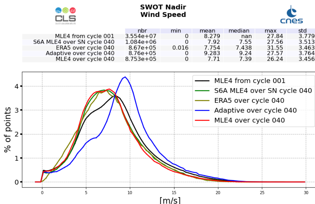
Figure 10: Altimeter Wind Speed histogram computed over cycle 040 (red line for SWOT Nadir MLE4 and blue line for SWOT Nadir Adaptive, green for Sentinel-6A-MF (LR MLE4)) and from cycle 001 (SWOT Nadir, MLE4 only, black line)
