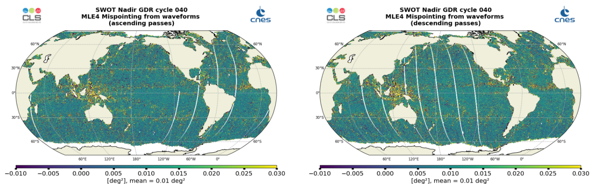
Figure 17: Along-track maps of mispointing over cycle 040 for SWOT Nadir MLE4, ascending passes (left) and descending passes (right)
