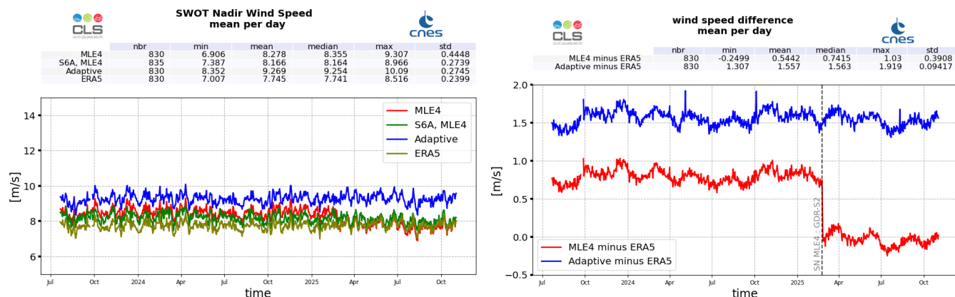
Figure 12: Wind Speed daily monitoring from cycle 001 to 040 for SWOT Nadir GDR, ERA5 model, and Sentinel-6A-MF (LR MLE4) (left), and daily mean difference with ERA5 (right)
