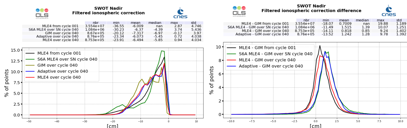
Figure 13: GIM model (dark green) and altimeter filtered ionosphere correction histogram computed over cycle 040 (red line for SWOT Nadir MLE4 and blue line for SWOT Nadir Adaptive, green for Sentinel-6A-MF (LR MLE4)) and from cycle 001 (SWOT Nadir, MLE4 only, black line) (left). Difference between filtered altimeter and GIM model (right).
