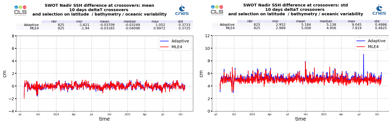
Figure 29: Monitoring of SSH difference at crossovers for SWOT Nadir MLE4 (red) and Adaptive (blue) : mean (left) and standard deviation (right), from cycle 001 to 040
