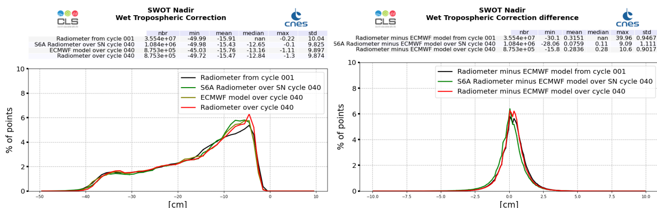
Figure 21: Histogram of wet troposphere corrections : SWOT Nadir radiometer (left) and difference with ECMWF model (right), computed over cycle 040 and from cycle 001 (black line)
