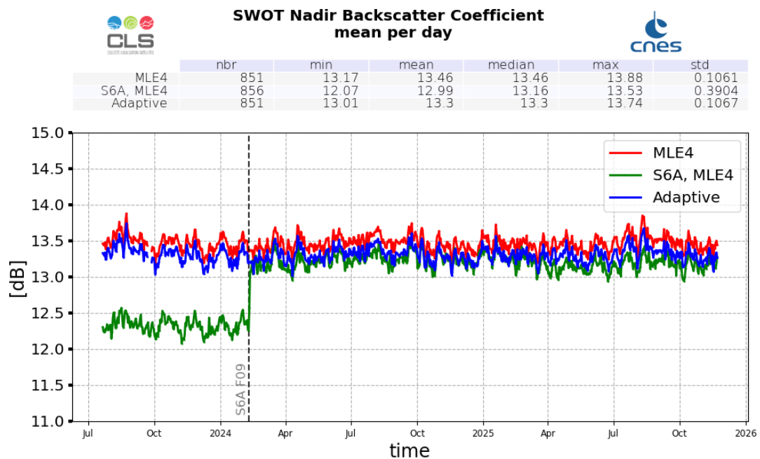
Figure 9: Ku-band Backscattering coefficient daily monitoring from cycle 001 to 041, for SWOT Nadir and Sentinel-6A-MF
