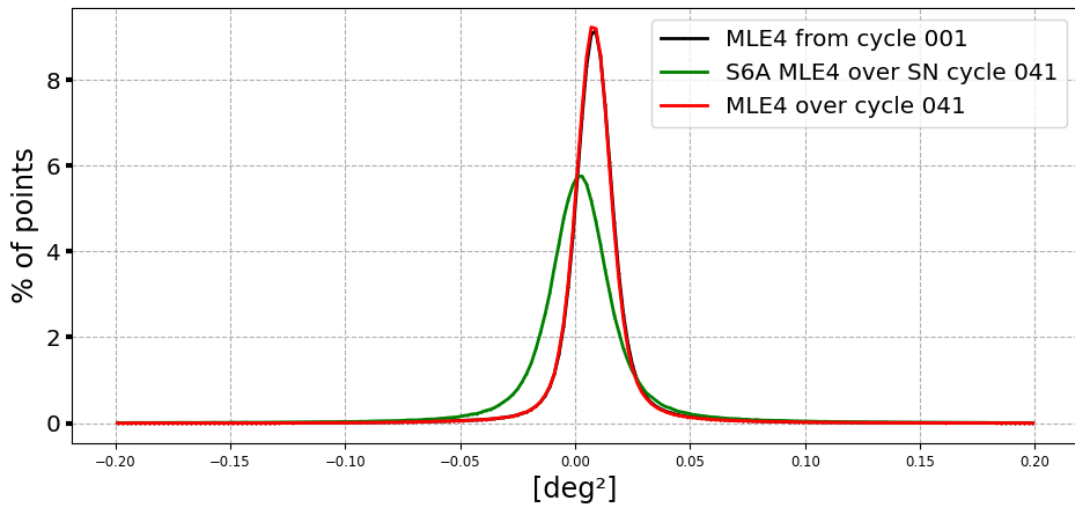
Figure 16: Mispointing histogram computed over cycle 041 (solid line) and from cycle 4 (dashed line)
