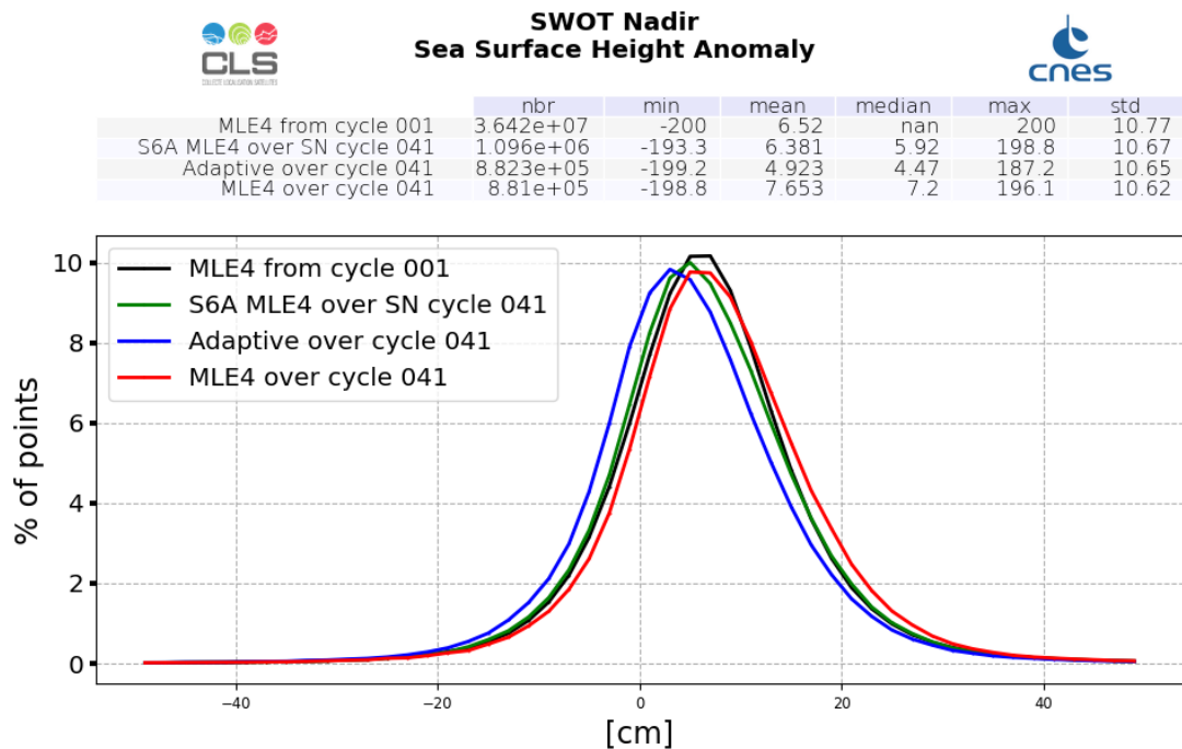
Figure 25: SSHA histogram computed over cycle 041 (red line for SWOT Nadir MLE4 and blue line for SWOT Nadir Adaptive, green for Sentinel-6A-MF (LR MLE4)) and from cycle 001 (SWOT Nadir, MLE4 only, black line)
