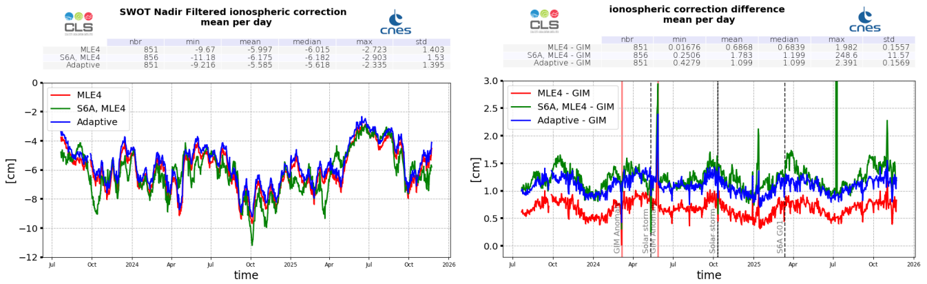
Figure 15: SWOT Nadir MLE4 (red), Adaptive (blue) and Sentinel-6A-MF (LR MLE4) (green) filtered ionosphere correction daily monitoring from cycle 001 to 041 (left) and difference with GIM model (right)
