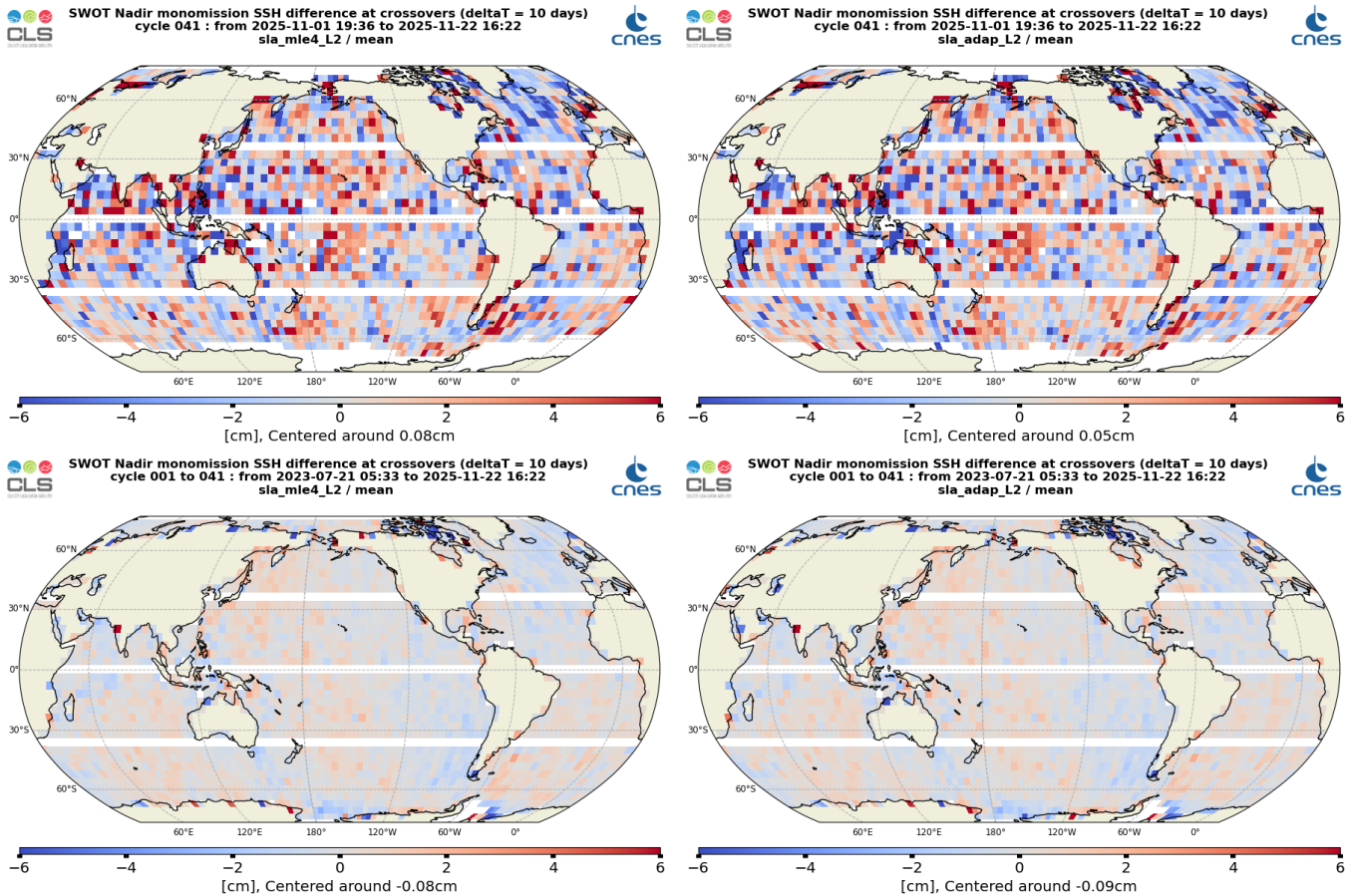
Figure 28: Mean SSH difference at crossovers for SWOT Nadir MLE4 (left) and Adaptive (right) cycle 041(top) and from cycle 001 to cycle 041 (bottom)
