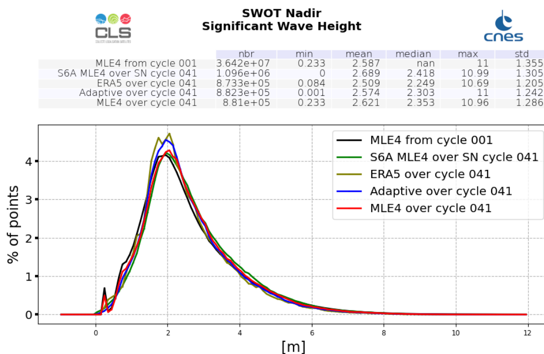
Figure 4: Ku-band Significant Wave Height histogram computed over cycle 041 (red line for SWOT Nadir MLE4 and blue line for SWOT Nadir Adaptive, green for Sentinel-6A-MF (LR MLE4) and dark green for ERA5) and from cycle 001 (SWOT Nadir, MLE4 only, black line)
