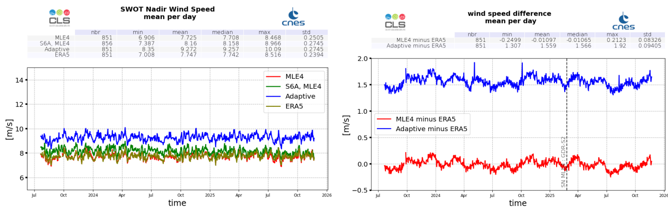
Figure 12: Wind Speed daily monitoring from cycle 001 to 041 for SWOT Nadir GDR, ERA5 model, and Sentinel-6A-MF (LR MLE4) (left), and daily mean difference with ERA5 (right)
