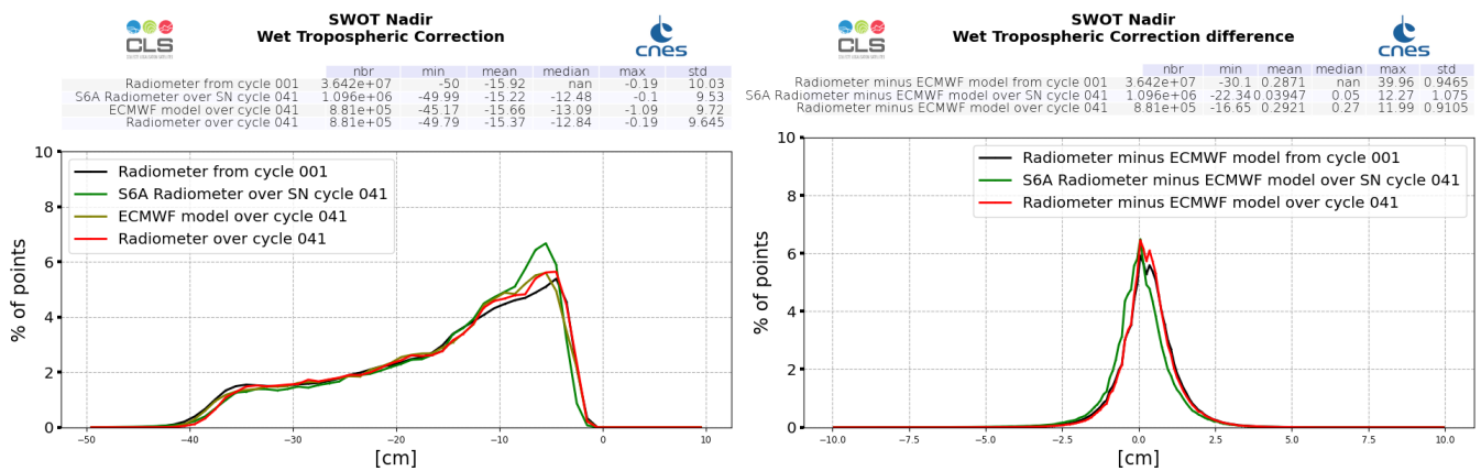
Figure 21: Histogram of wet troposphere corrections : SWOT Nadir radiometer (left) and difference with ECMWF model (right), computed over cycle 041 and from cycle 001 (black line)
