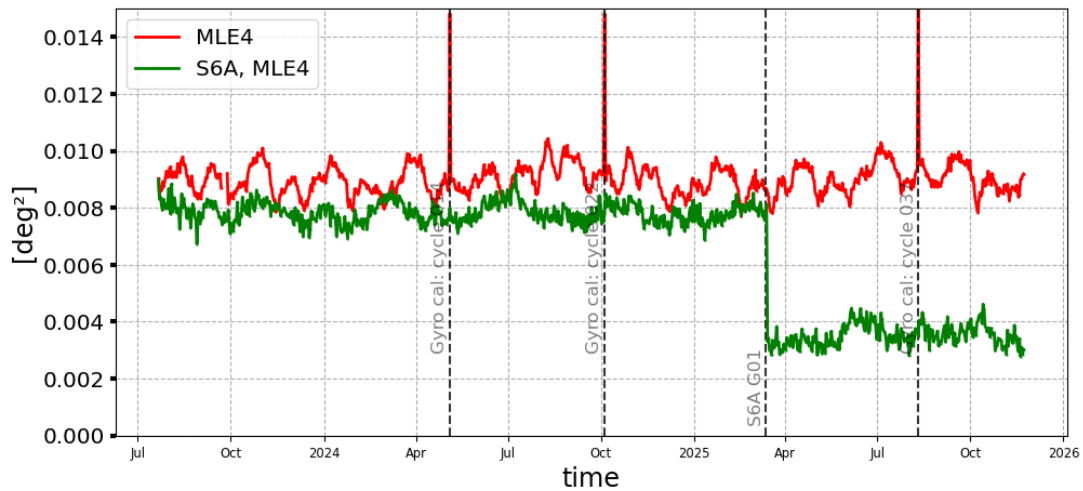
Figure 18: Mispointing daily monitoring from SWOT cycle 001 to 041 for SWOT Nadir GDR (red) and Sentinel-6A-MF (green)
