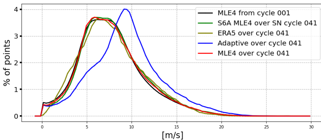
Figure 10: Altimeter Wind Speed histogram computed over cycle 041 (red line for SWOT Nadir MLE4 and blue line for SWOT Nadir Adaptive, green for Sentinel-6A-MF (LR MLE4)) and from cycle 001 (SWOT Nadir, MLE4 only, black line)
