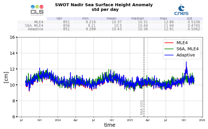
Figure 27: SSHA daily monitoring from cycle 001 to 041, for SWOT Nadir GDR
