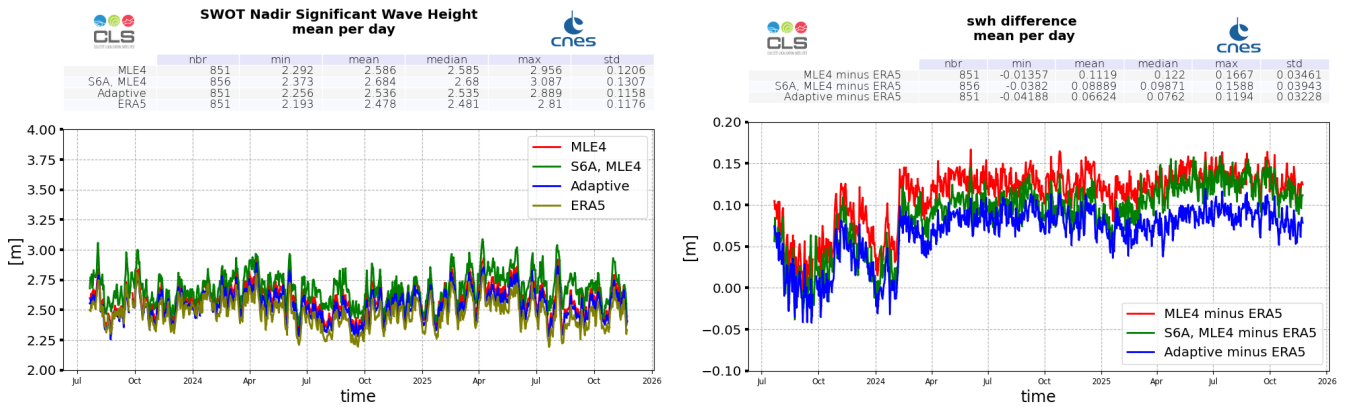
Figure 6: Ku-band Significant Wave Height daily monitoring from cycle 001 to 041, for SWOT Nadir, ERA5 model estimated at SWOT locations, and Sentinel-6A-MF (LR MLE4) (left), and difference with ERA5 model (right)
