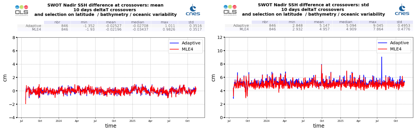
Figure 29: Monitoring of SSH difference at crossovers for SWOT Nadir MLE4 (red) and Adaptive (blue) : mean (left) and standard deviation (right), from cycle 001 to 041
