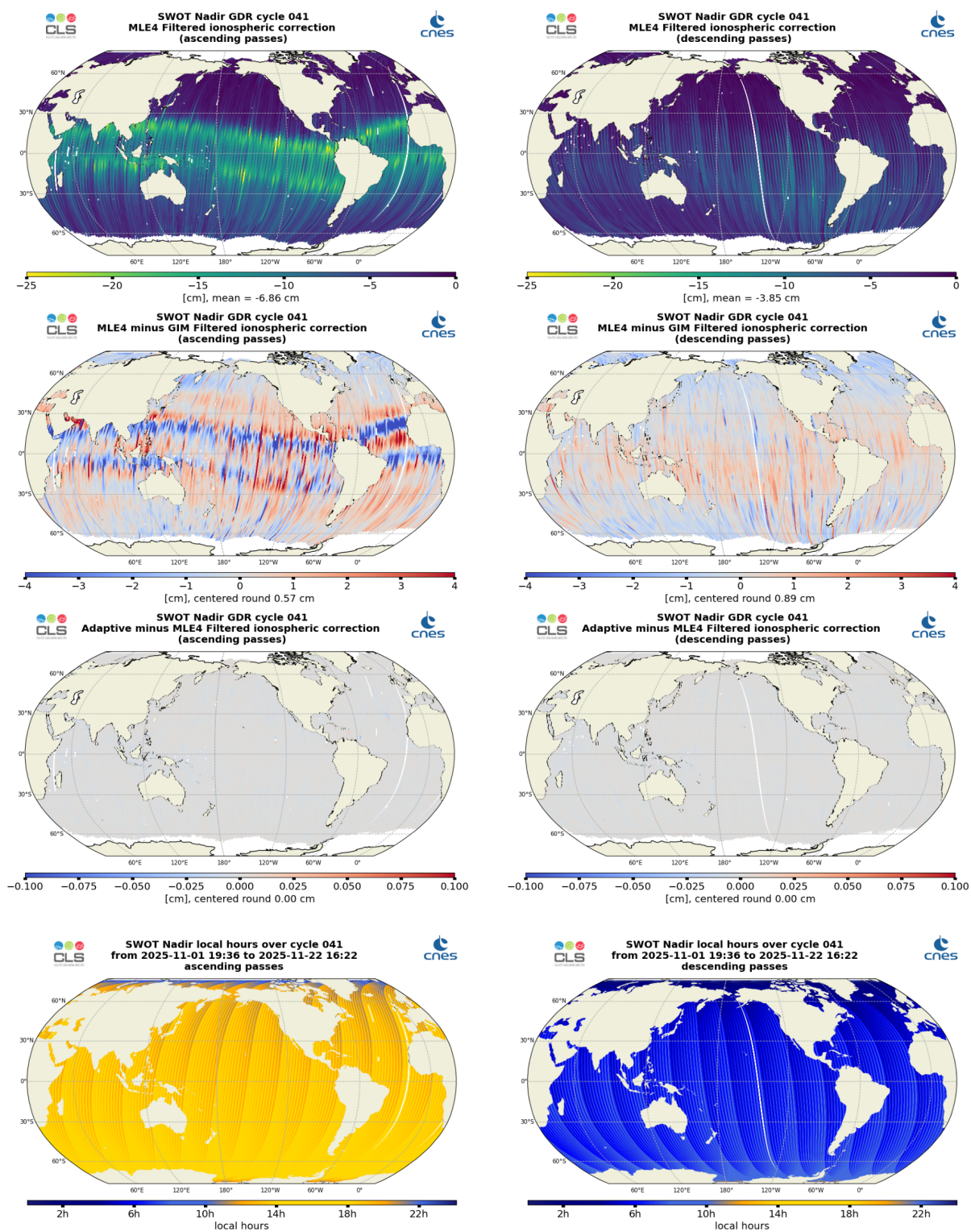
Figure 14: Along-track maps of filtered ionosphere correction over cycle 041 for SWOT Nadir MLE4 (top), MLE4 minus GIM (middle top) or Adaptive minus MLE4 (middle bottom), and local hours (bottom), for ascending passes (left) and descending passes (right)
