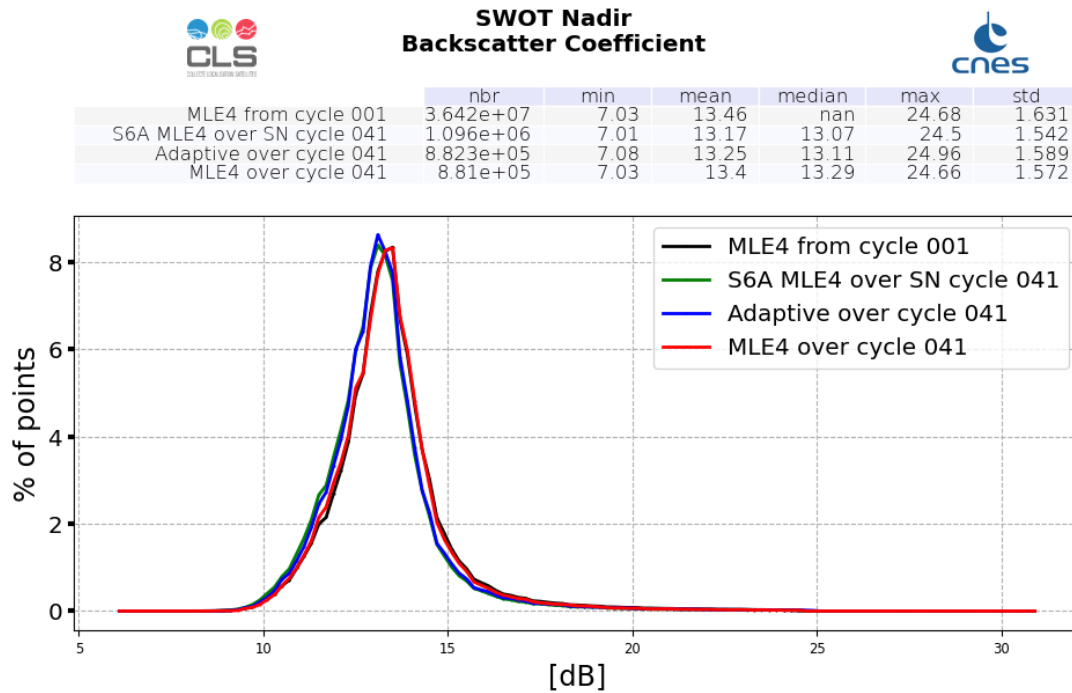
Figure 7: Ku-band Backscattering coefficient histogram computed over cycle 041 (red line for SWOT Nadir MLE4 and blue line for SWOT Nadir Adaptive, green for Sentinel-6A-MF (LR MLE4)) and from cycle 001 (SWOT Nadir, MLE4 only, black line)
