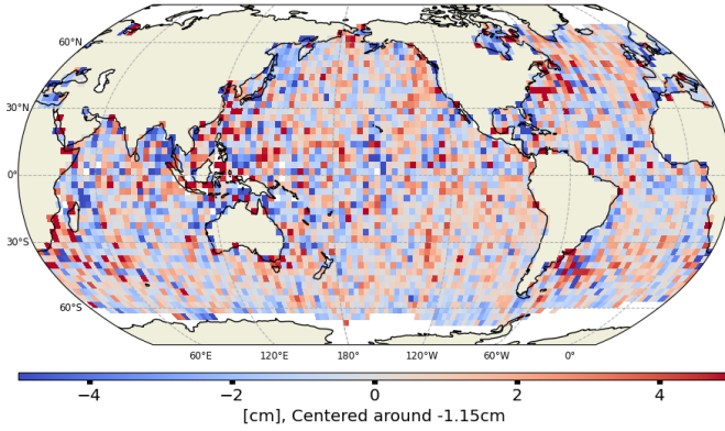
Figure 30: Mean SSH difference at crossovers between SWOT Nadir MLE4 and Sentinel-6 MF LR MLE4 over cycle 041 (left) and from cycle 001 onwards (right)
