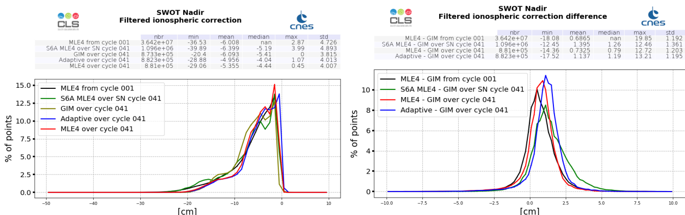
Figure 13: GIM model (dark green) and altimeter filtered ionosphere correction histogram computed over cycle 041 (red line for SWOT Nadir MLE4 and blue line for SWOT Nadir Adaptive, green for Sentinel-6A-MF (LR MLE4)) and from cycle 001 (SWOT Nadir, MLE4 only, black line) (left). Difference between filtered altimeter and GIM model (right).
