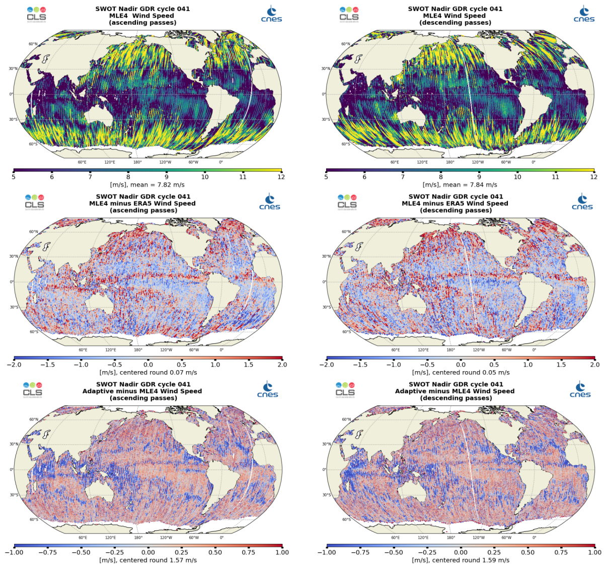
Figure 11: Along-track maps of Altimeter Wind Speed over cycle 041 for SWOT Nadir MLE4 (top), MLE4 minus ERA5 (middle) or Adaptive minus MLE4 (bottom), ascending passes (left) and descending passes (right)
