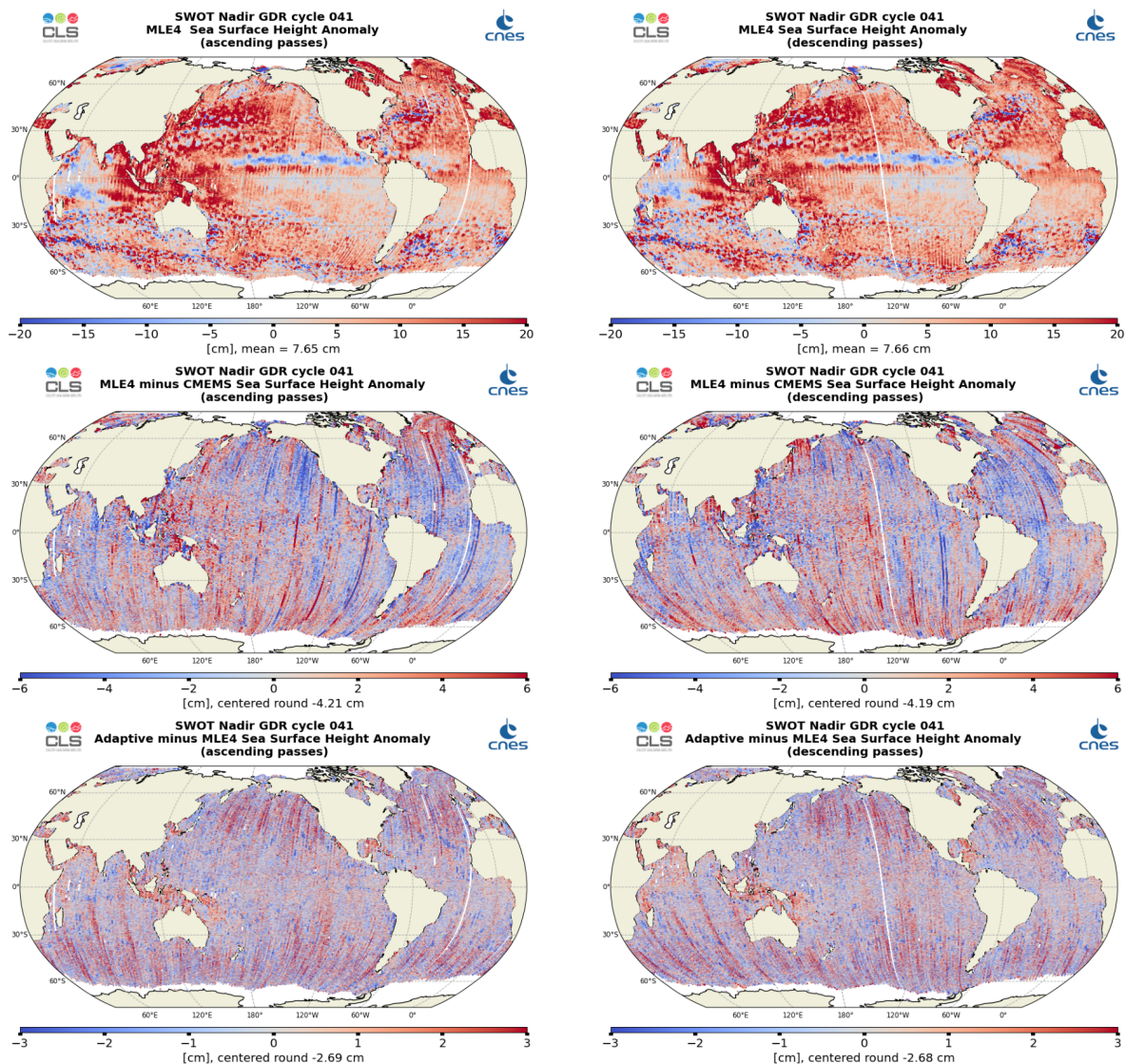
Figure 26: Along-track maps of SSHA over cycle 041 for SWOT Nadir MLE4 (top), MLE4 minus CMEMS (middle) or Adaptive minus MLE4 (bottom), ascending passes (left) and descending passes (right)
