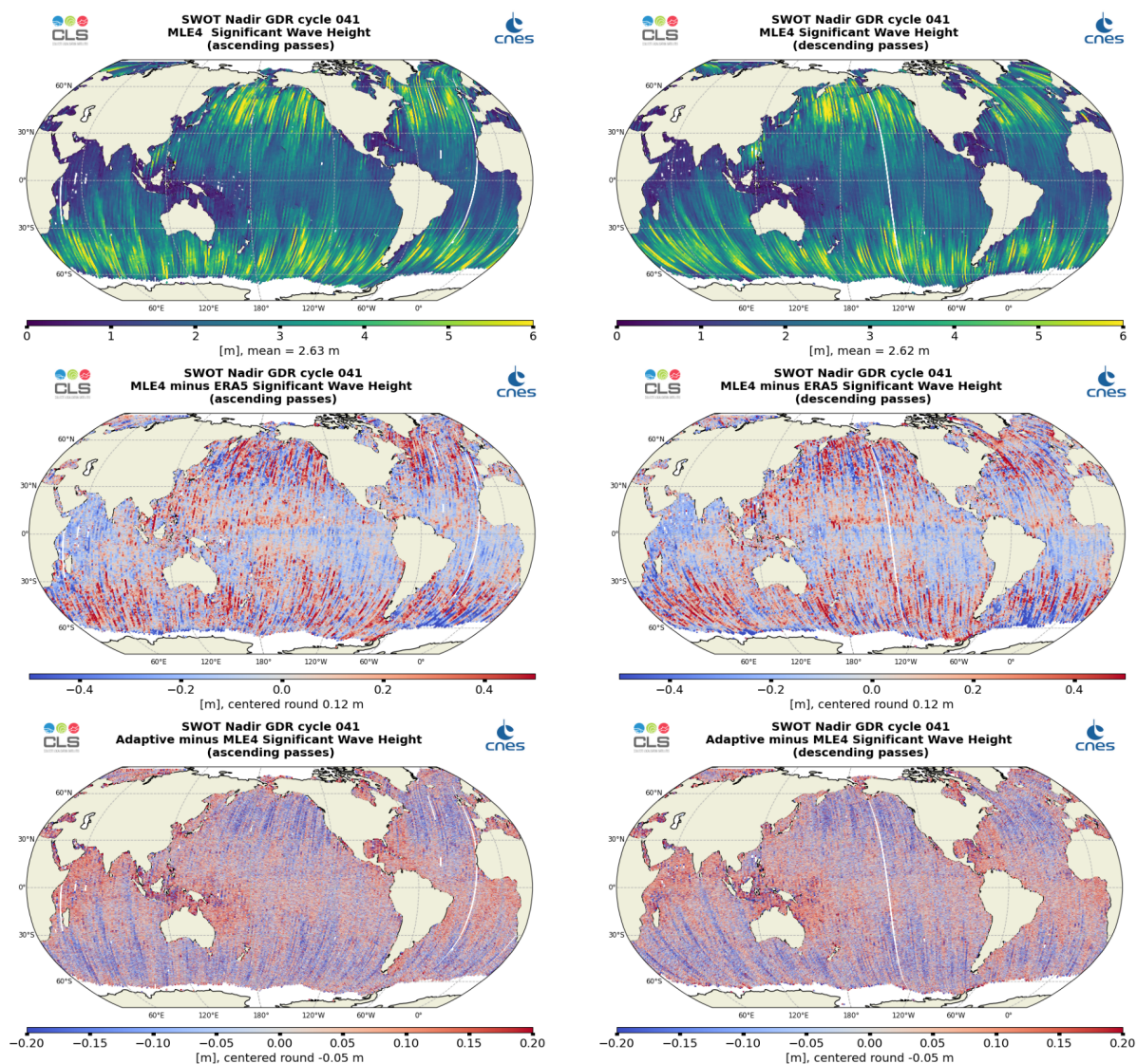
Figure 5: Along-track maps of Ku-band Significant Wave Height over cycle 041 for SWOT Nadir MLE4 (top), MLE4 minus model (middle) or Adaptive minus MLE4 (bottom), ascending passes (left) and descending passes (right)
