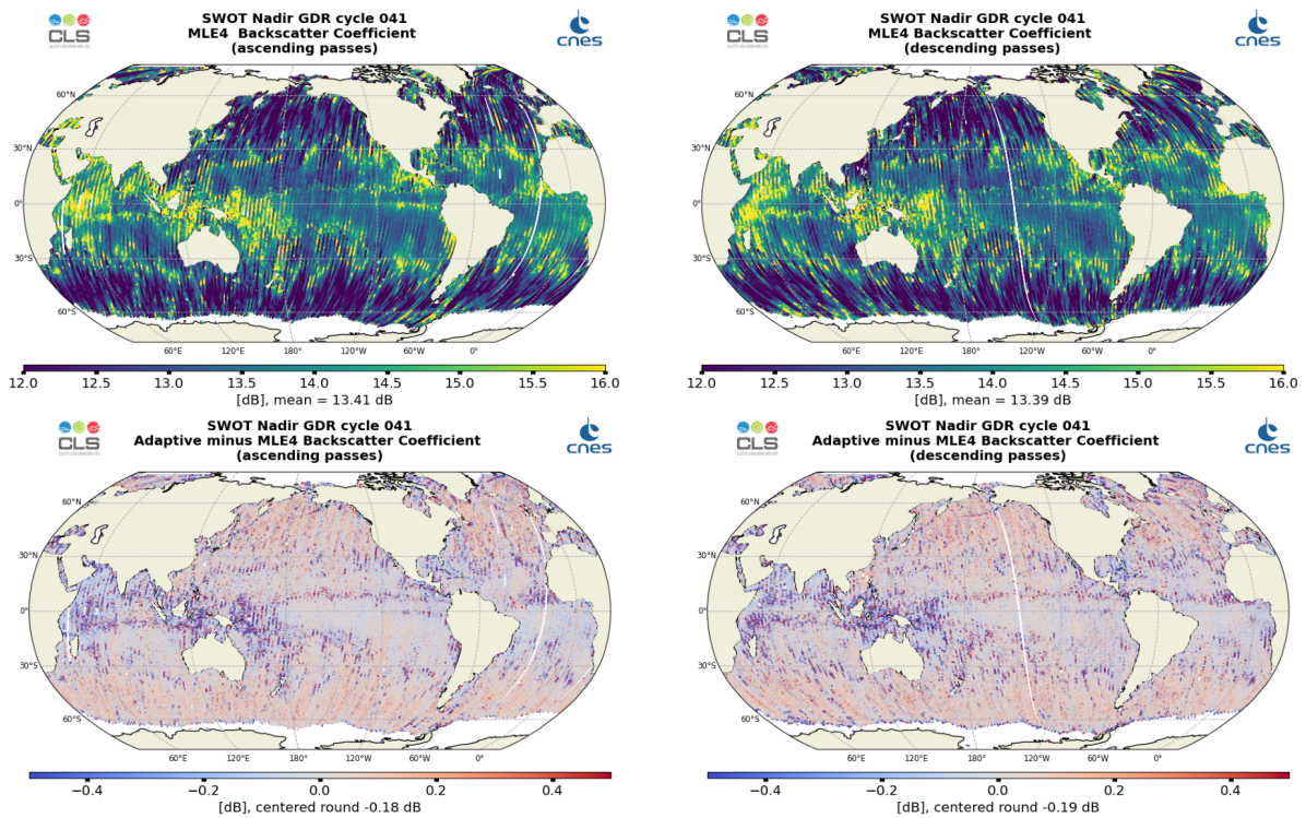
Figure 8: Along-track maps of Ku-band backscatter coefficient \sigma_0 over cycle 041 for SWOT Nadir MLE4 (top) or Adaptive minus MLE4 difference (bottom), ascending passes (left) and descending passes (right)
