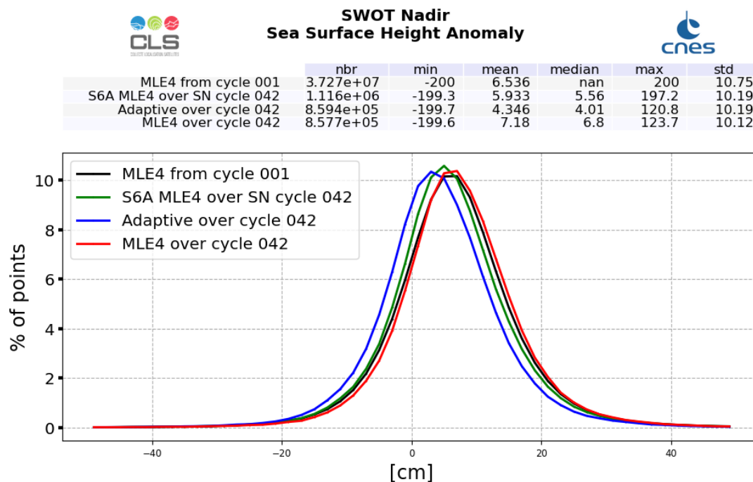
Figure 25: SSHA histogram computed over cycle 042 (red line for SWOT Nadir MLE4 and blue line for SWOT Nadir Adaptive, green for Sentinel-6A-MF (LR MLE4)) and from cycle 001 (SWOT Nadir, MLE4 only, black line)
