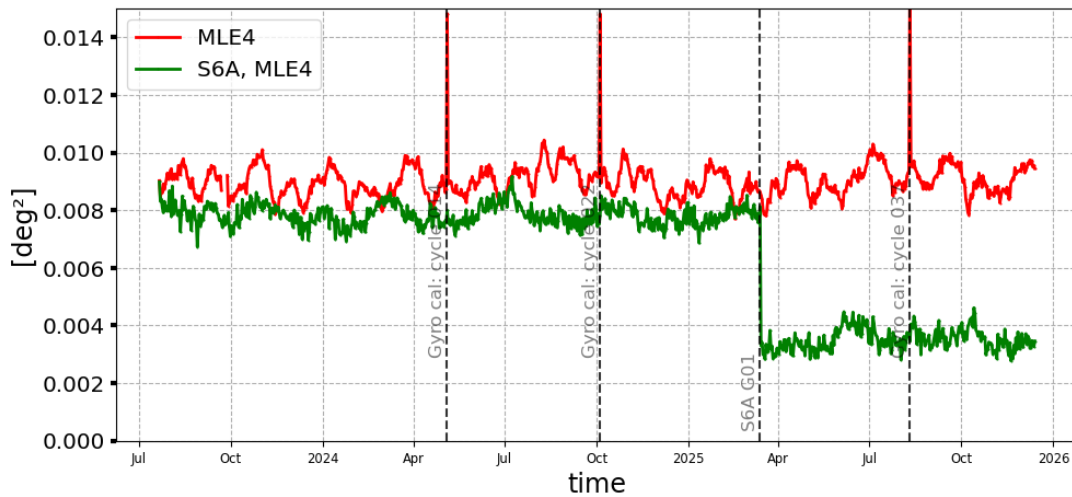
Figure 18: Mispointing daily monitoring from SWOT cycle 001 to 042 for SWOT Nadir GDR (red) and Sentinel-6A-MF (green)
