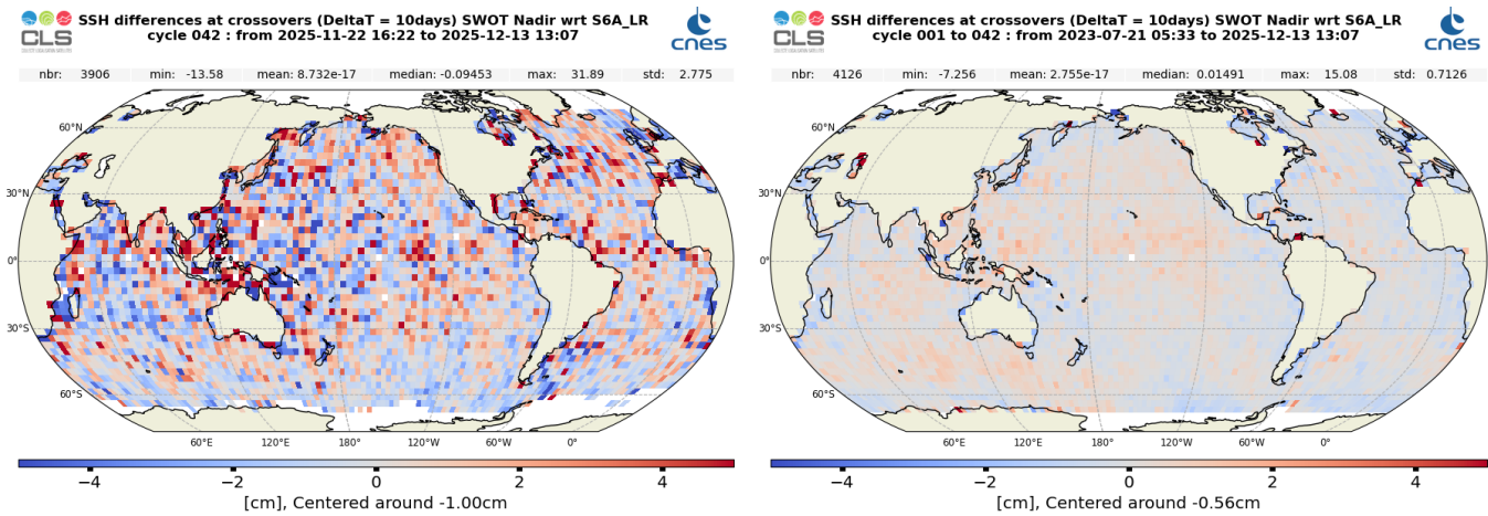
Figure 30: Mean SSH difference at crossovers between SWOT Nadir MLE4 and Sentinel-6 MF LR MLE4 over cycle 042 (left) and from cycle 001 onwards (right)
