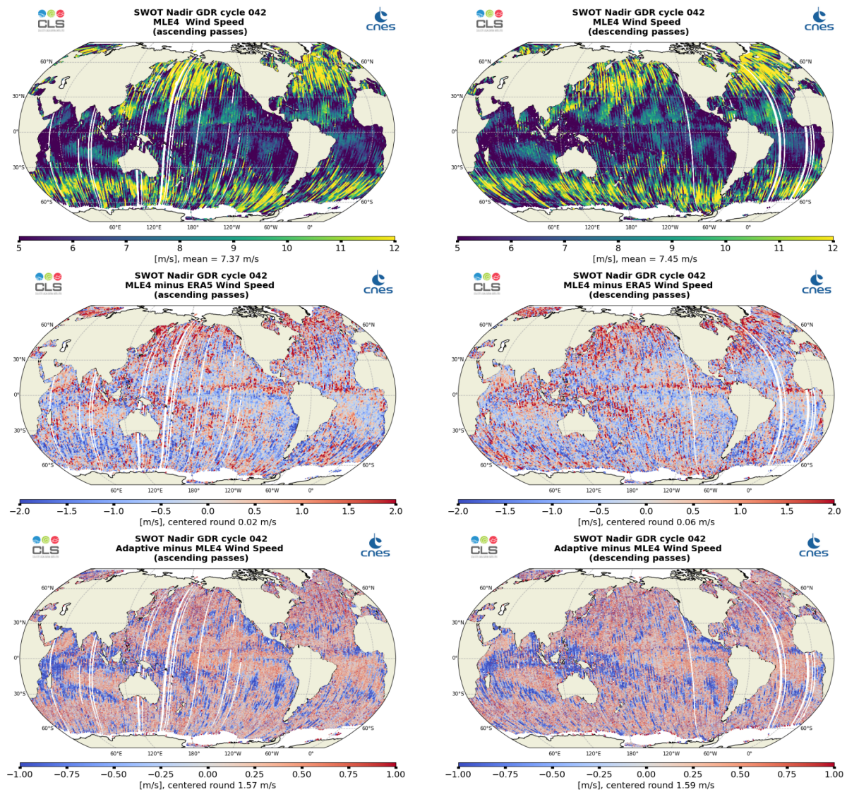
Figure 11: Along-track maps of Altimeter Wind Speed over cycle 042 for SWOT Nadir MLE4 (top), MLE4 minus ERA5 (middle) or Adaptive minus MLE4 (bottom), ascending passes (left) and descending passes (right)
