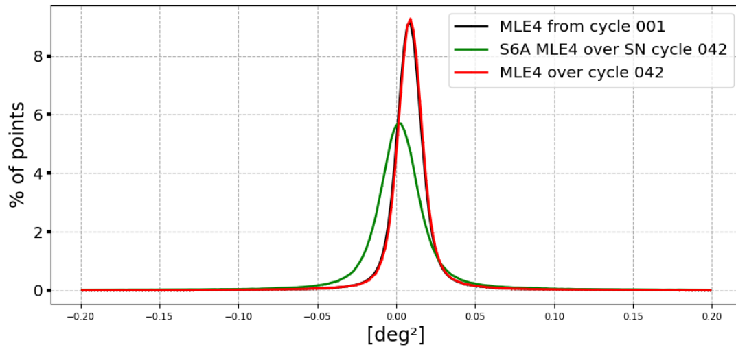
Figure 16: Mispointing histogram computed over cycle 042 (solid line) and from cycle 4 (dashed line)
