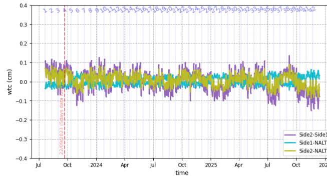
Figure 20: Daily monitoring of the wet tropospheric correction gradient between AMR Side 1 and AMR Side 2 (purple), AMR Side 1 and Nadir (cyan), and AMR Side 2 and Nadir (yellow), from Cycle 001 to 042
