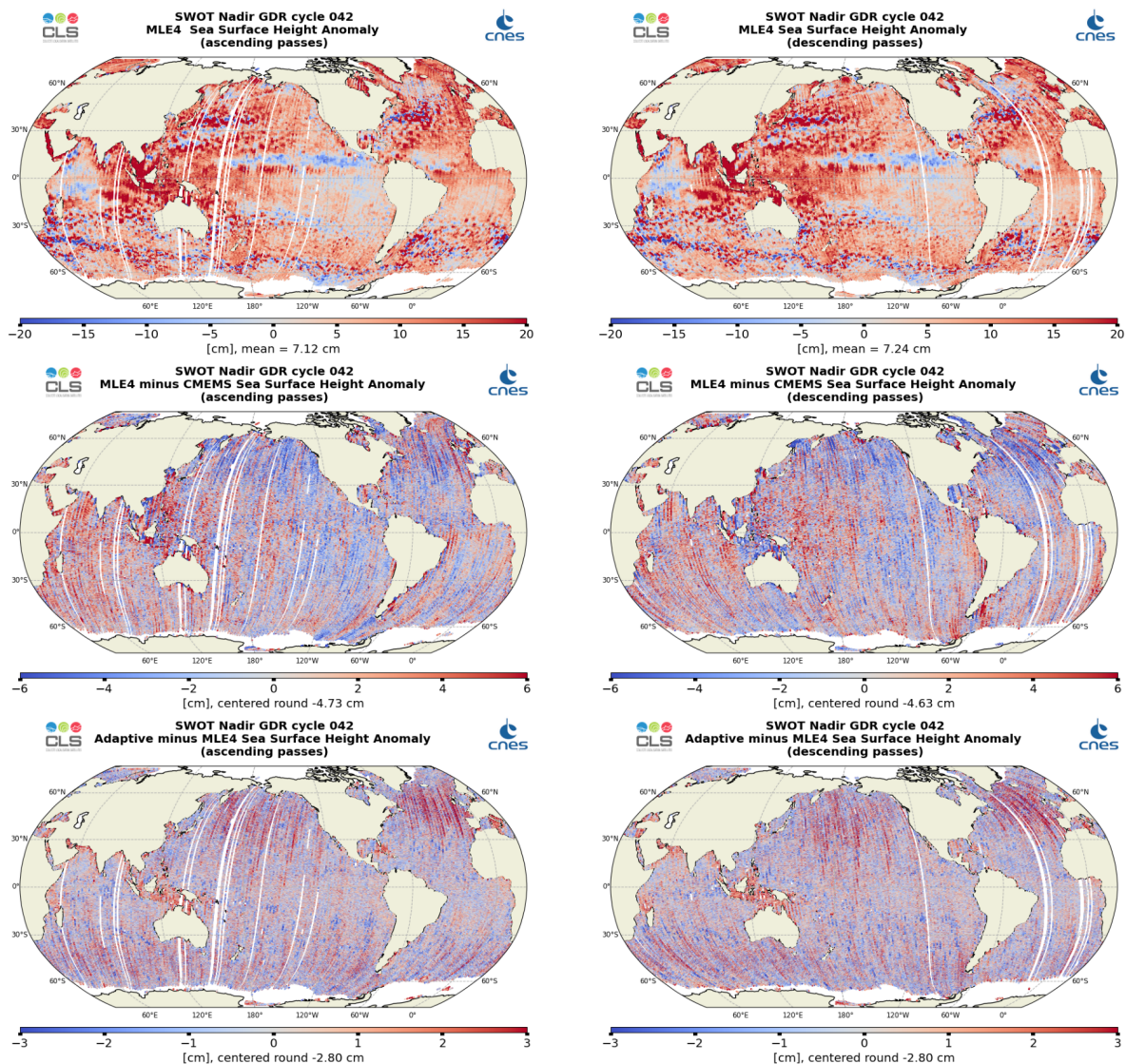
Figure 26: Along-track maps of SSHA over cycle 042 for SWOT Nadir MLE4 (top), MLE4 minus CMEMS (middle) or Adaptive minus MLE4 (bottom), ascending passes (left) and descending passes (right)
