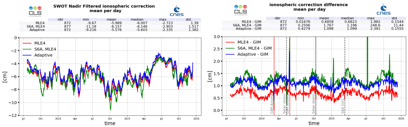
Figure 15: SWOT Nadir MLE4 (red), Adaptive (blue) and Sentinel-6A-MF (LR MLE4) (green) filtered ionosphere correction daily monitoring from cycle 001 to 042 (left) and difference with GIM model (right)
