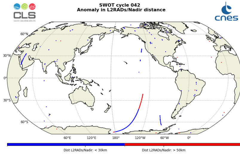
Figure 24: Map of the anomalies detected in the L2RADs/Nadir distance over the cycle 042
