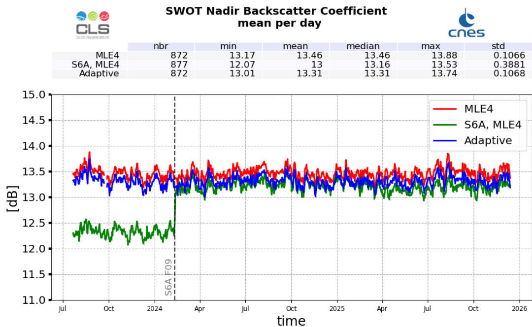
Figure 9: Ku-band Backscattering coefficient daily monitoring from cycle 001 to 042, for SWOT Nadir and Sentinel-6A-MF
