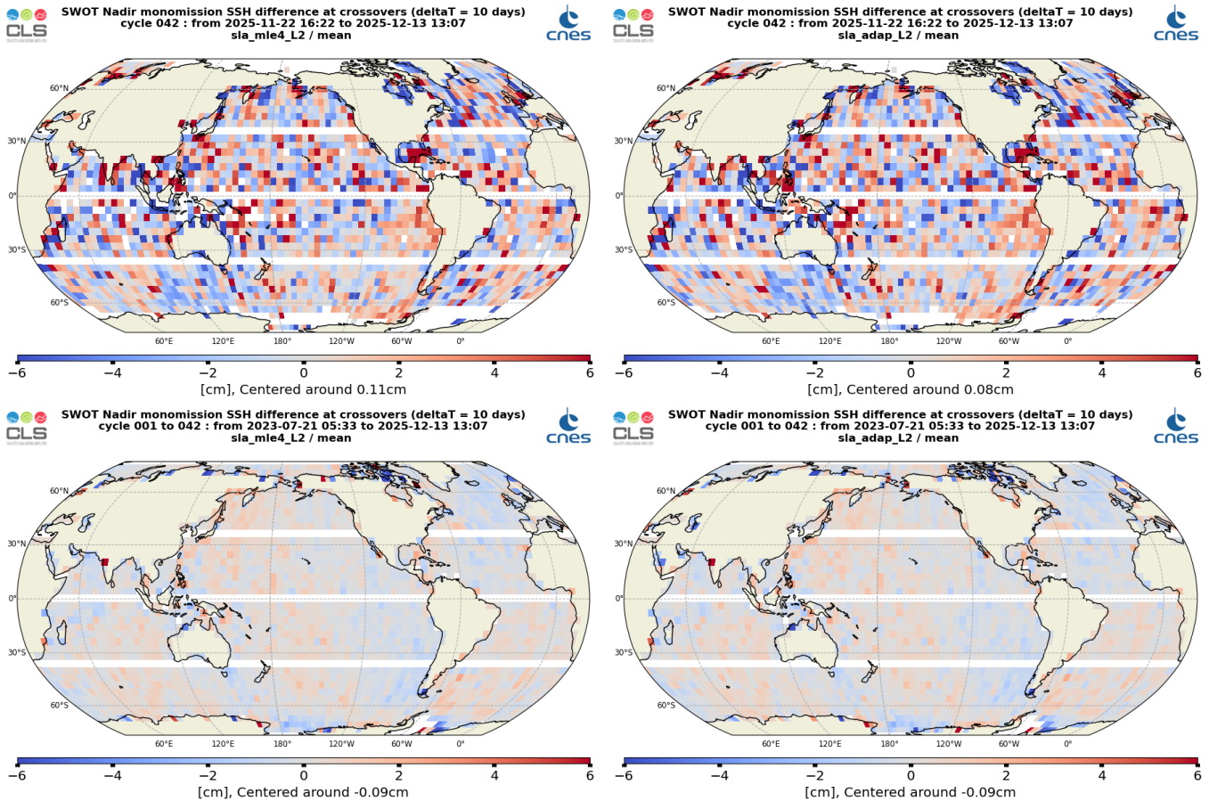
Figure 28: Mean SSH difference at crossovers for SWOT Nadir MLE4 (left) and Adaptive (right) cycle 042(top) and from cycle 001 to cycle 042 (bottom)
