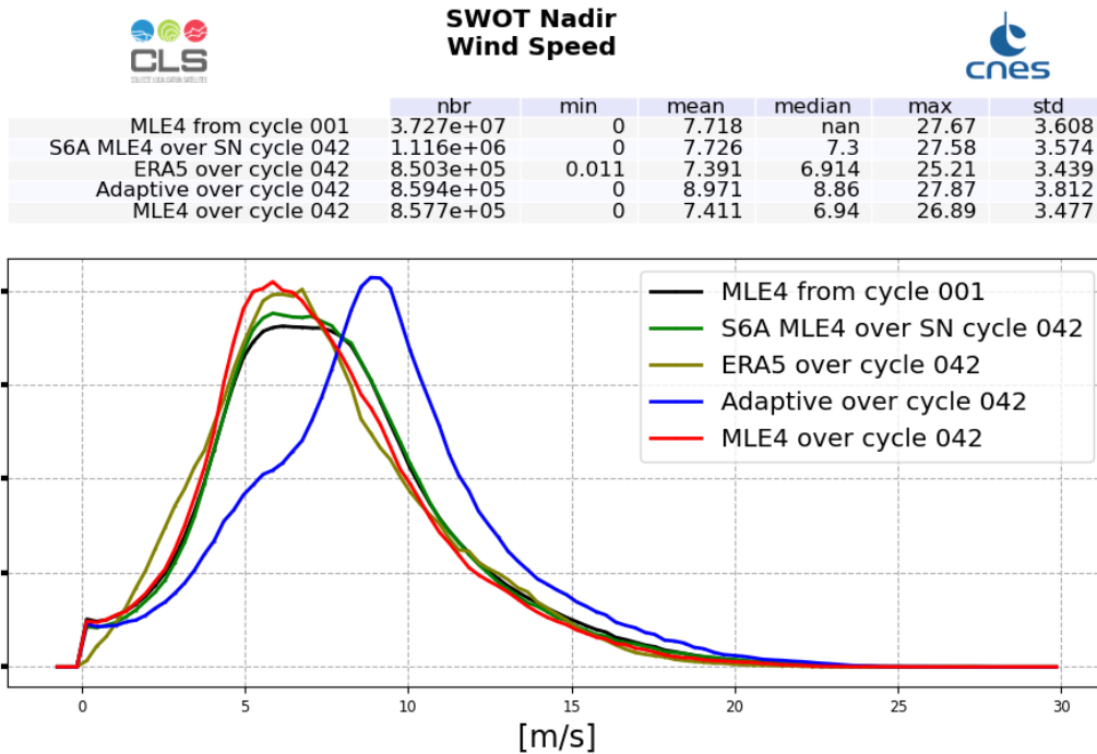
Figure 10: Altimeter Wind Speed histogram computed over cycle 042 (red line for SWOT Nadir MLE4 and blue line for SWOT Nadir Adaptive, green for Sentinel-6A-MF (LR MLE4)) and from cycle 001 (SWOT Nadir, MLE4 only, black line)
