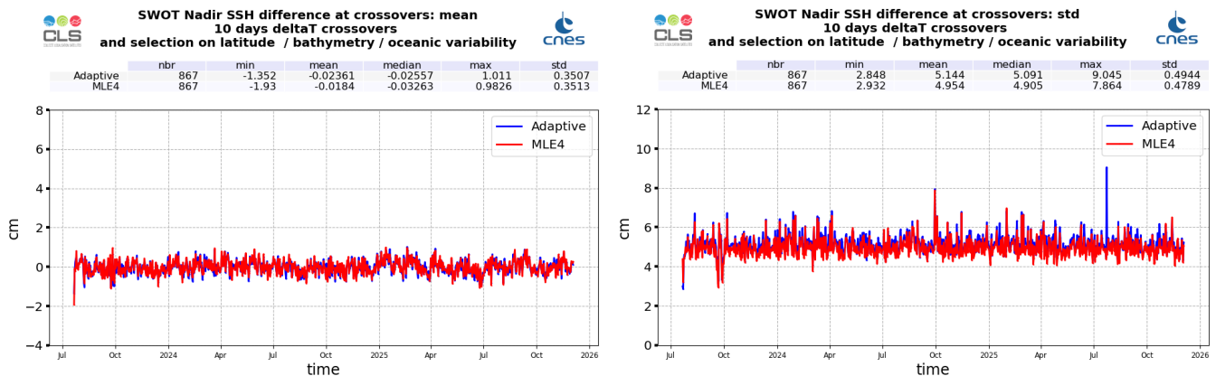
Figure 29: Monitoring of SSH difference at crossovers for SWOT Nadir MLE4 (red) and Adaptive (blue) : mean (left) and standard deviation (right), from cycle 001 to 042
