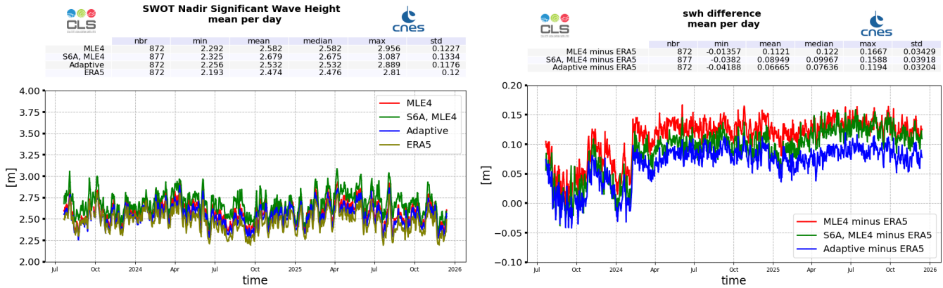
Figure 6: Ku-band Significant Wave Height daily monitoring from cycle 001 to 042, for SWOT Nadir, ERA5 model estimated at SWOT locations, and Sentinel-6A-MF (LR MLE4) (left), and difference with ERA5 model (right)
