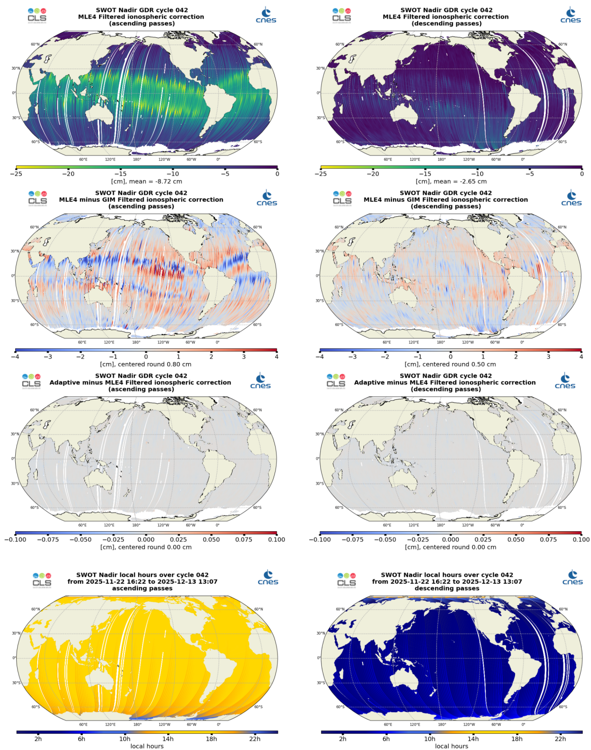
Figure 14: Along-track maps of filtered ionosphere correction over cycle 042 for SWOT Nadir MLE4 (top), MLE4 minus GIM (middle top) or Adaptive minus MLE4 (middle bottom), and local hours (bottom), for ascending passes (left) and descending passes (right)
