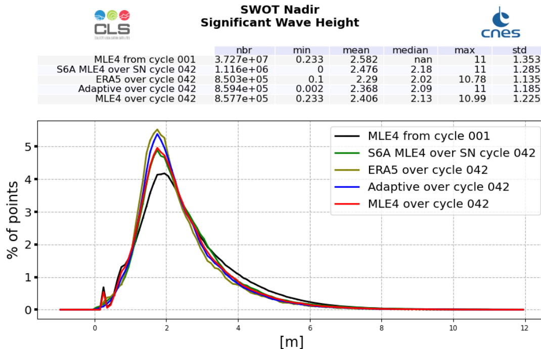
Figure 4: Ku-band Significant Wave Height histogram computed over cycle 042 (red line for SWOT Nadir MLE4 and blue line for SWOT Nadir Adaptive, green for Sentinel-6A-MF (LR MLE4) and dark green for ERA5) and from cycle 001 (SWOT Nadir, MLE4 only, black line)
