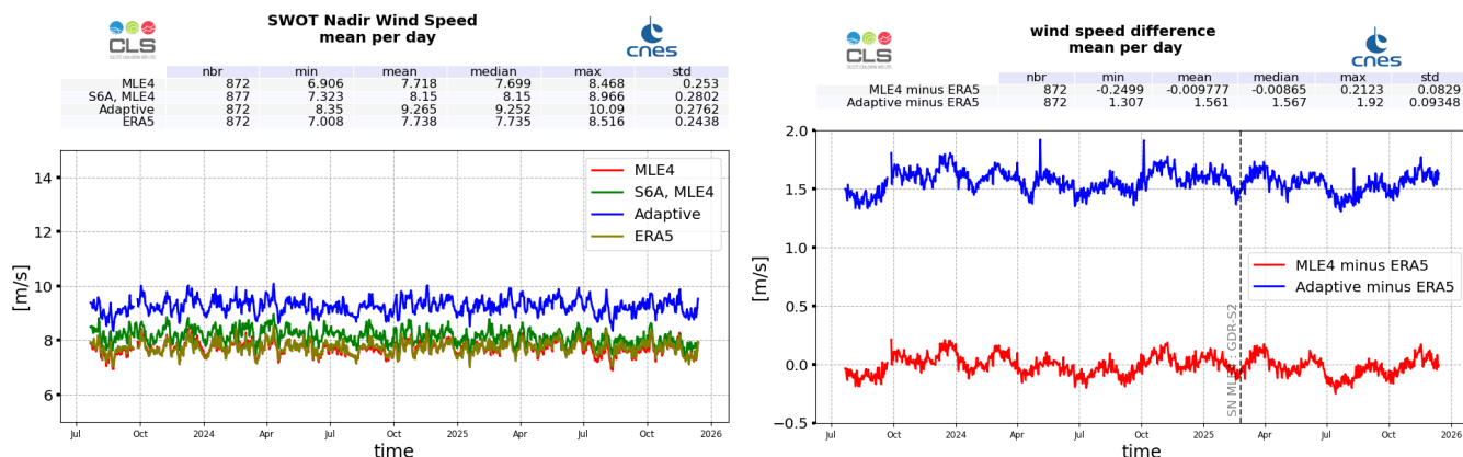
Figure 12: Wind Speed daily monitoring from cycle 001 to 042 for SWOT Nadir GDR, ERA5 model, and Sentinel-6A-MF (LR MLE4) (left), and daily mean difference with ERA5 (right)
