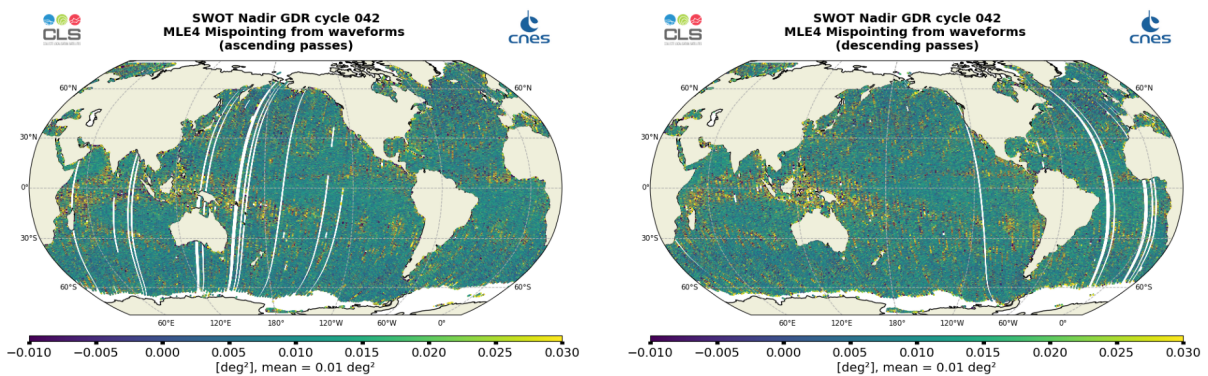
Figure 17: Along-track maps of mispointing over cycle 042 for SWOT Nadir MLE4, ascending passes (left) and descending passes (right)
