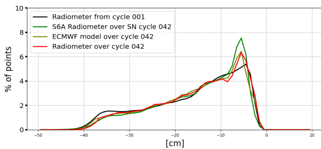
Figure 21: Histogram of wet troposphere corrections : SWOT Nadir radiometer (left) and difference with ECMWF model (right), computed over cycle 042 and from cycle 001 (black line)
