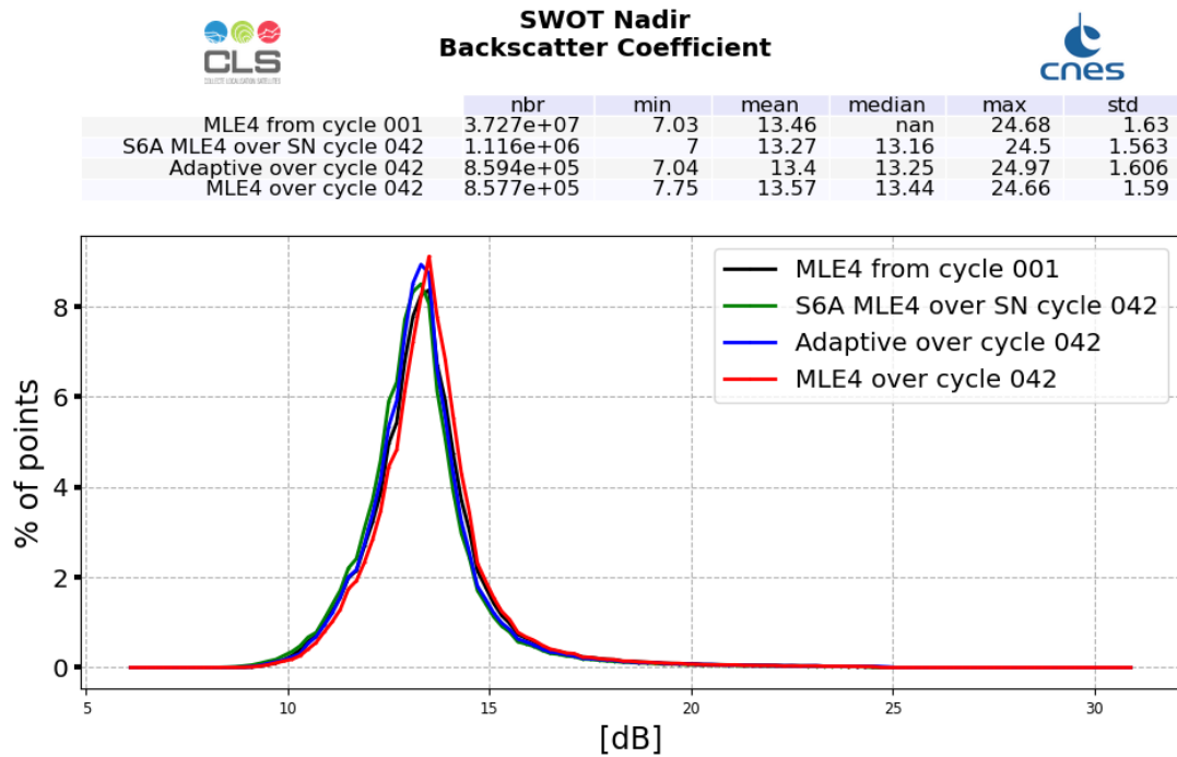
Figure 7: Ku-band Backscattering coefficient histogram computed over cycle 042 (red line for SWOT Nadir MLE4 and blue line for SWOT Nadir Adaptive, green for Sentinel-6A-MF (LR MLE4)) and from cycle 001 (SWOT Nadir, MLE4 only, black line)
