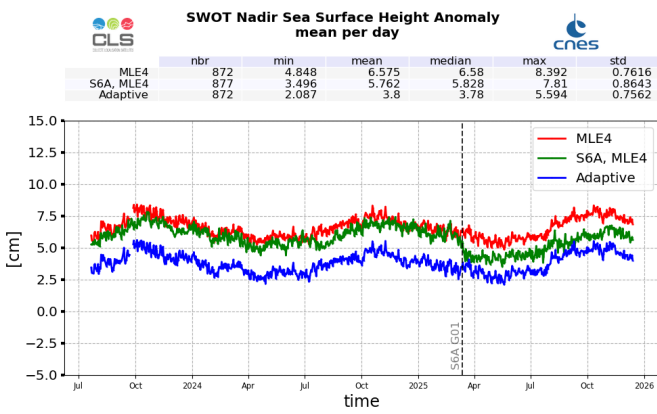
Figure 27: SSHA daily monitoring from cycle 001 to 042, for SWOT Nadir GDR
