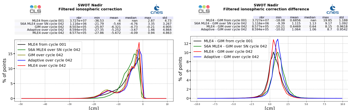
Figure 13: GIM model (dark green) and altimeter filtered ionosphere correction histogram computed over cycle 042 (red line for SWOT Nadir MLE4 and blue line for SWOT Nadir Adaptive, green for Sentinel-6A-MF (LR MLE4)) and from cycle 001 (SWOT Nadir, MLE4 only, black line) (left). Difference between filtered altimeter and GIM model (right).
