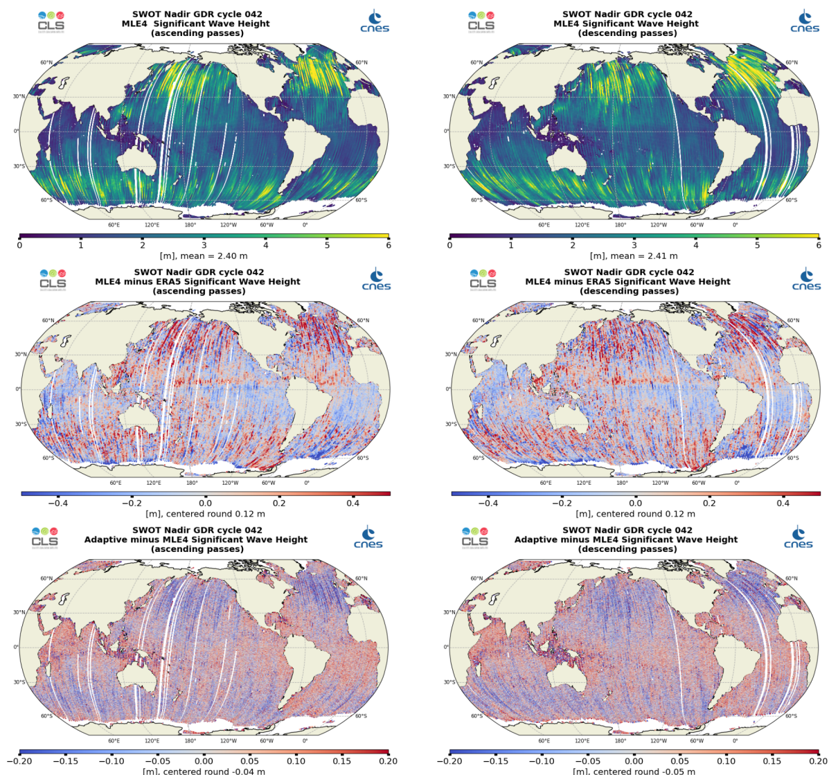
Figure 5: Along-track maps of Ku-band Significant Wave Height over cycle 042 for SWOT Nadir MLE4 (top), MLE4 minus model (middle) or Adaptive minus MLE4 (bottom), ascending passes (left) and descending passes (right)
