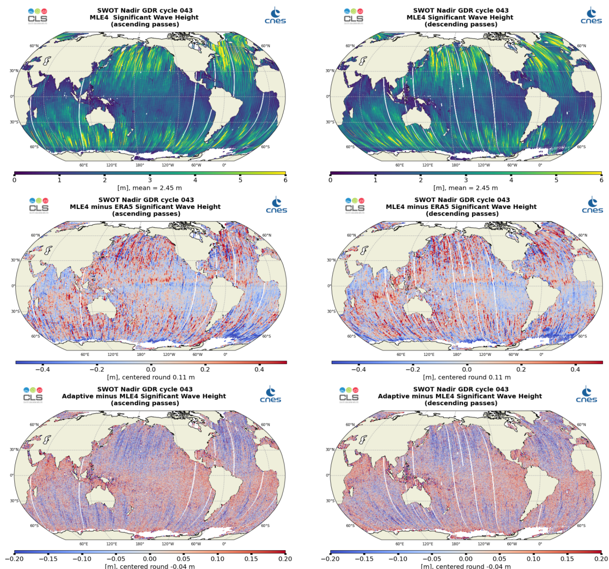
Figure 5: Along-track maps of Ku-band Significant Wave Height over cycle 043 for SWOT Nadir MLE4 (top), MLE4 minus model (middle) or Adaptive minus MLE4 (bottom), ascending passes (left) and descending passes (right)
