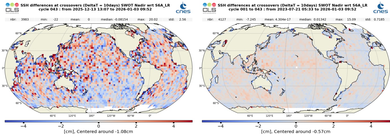
Figure 30: Mean SSH difference at crossovers between SWOT Nadir MLE4 and Sentinel-6 MF LR MLE4 over cycle 043 (left) and from cycle 001 onwards (right)
