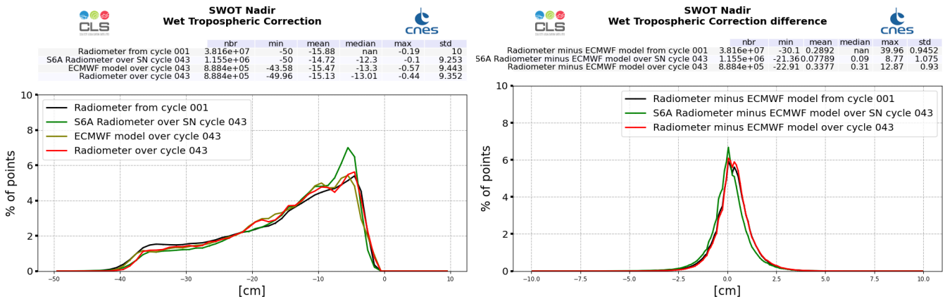
Figure 21: Histogram of wet troposphere corrections : SWOT Nadir radiometer (left) and difference with ECMWF model (right), computed over cycle 043 and from cycle 001 (black line)
