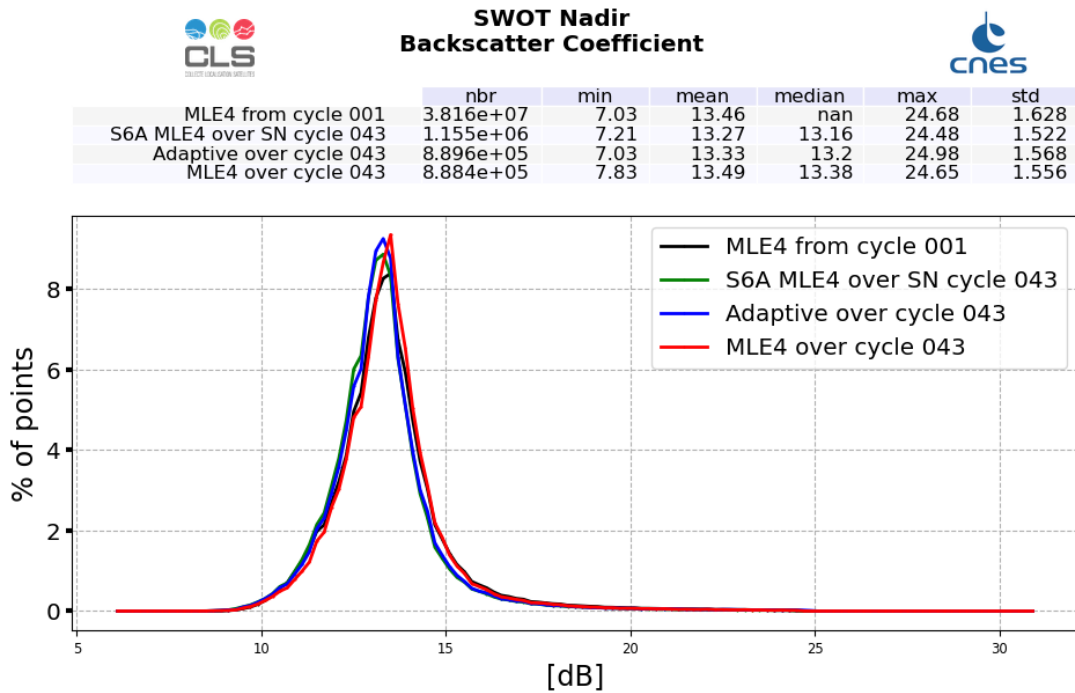
Figure 7: Ku-band Backscattering coefficient histogram computed over cycle 043 (red line for SWOT Nadir MLE4 and blue line for SWOT Nadir Adaptive, green for Sentinel-6A-MF (LR MLE4)) and from cycle 001 (SWOT Nadir, MLE4 only, black line)
