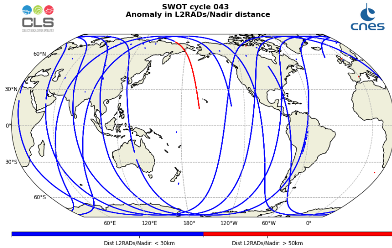
Figure 24: Map of the anomalies detected in the L2RADs/Nadir distance over the cycle 043
