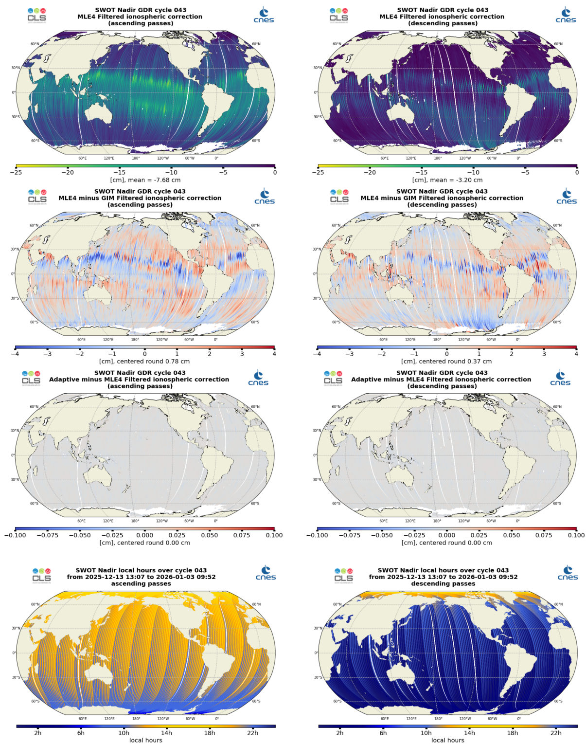
Figure 14: Along-track maps of filtered ionosphere correction over cycle 043 for SWOT Nadir MLE4 (top), MLE4 minus GIM (middle top) or Adaptive minus MLE4 (middle bottom), and local hours (bottom), for ascending passes (left) and descending passes (right)
