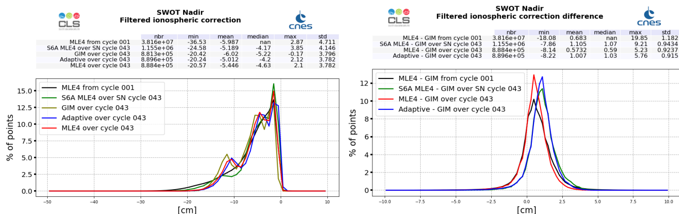
Figure 13: GIM model (dark green) and altimeter filtered ionosphere correction histogram computed over cycle 043 (red line for SWOT Nadir MLE4 and blue line for SWOT Nadir Adaptive, green for Sentinel-6A-MF (LR MLE4)) and from cycle 001 (SWOT Nadir, MLE4 only, black line) (left). Difference between filtered altimeter and GIM model (right).
