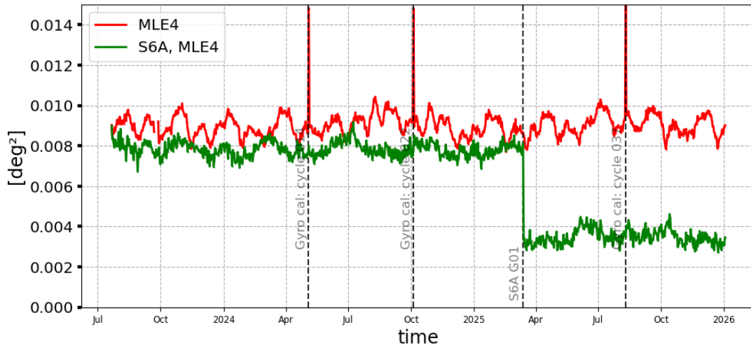
Figure 18: Mispointing daily monitoring from SWOT cycle 001 to 043 for SWOT Nadir GDR (red) and Sentinel-6A-MF (green)
