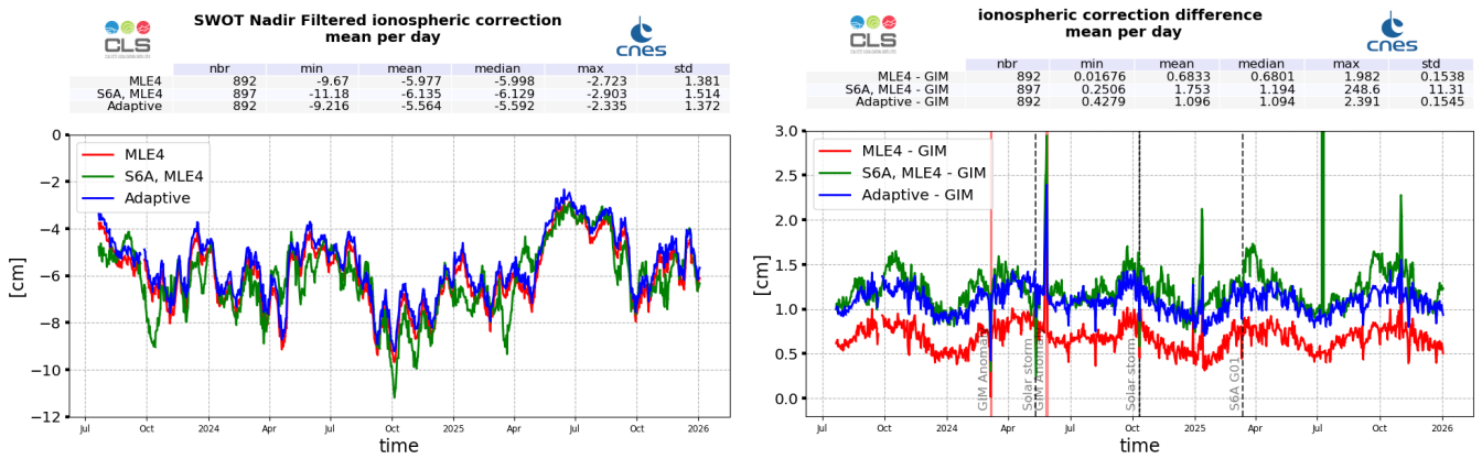
Figure 15: SWOT Nadir MLE4 (red), Adaptive (blue) and Sentinel-6A-MF (LR MLE4) (green) filtered ionosphere correction daily monitoring from cycle 001 to 043 (left) and difference with GIM model (right)
