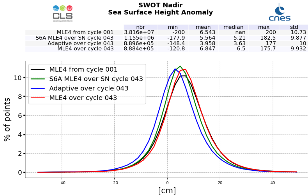
Figure 25: SSHA histogram computed over cycle 043 (red line for SWOT Nadir MLE4 and blue line for SWOT Nadir Adaptive, green for Sentinel-6A-MF (LR MLE4)) and from cycle 001 (SWOT Nadir, MLE4 only, black line)
