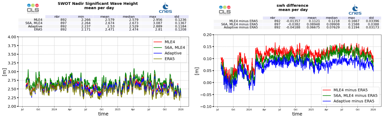
Figure 6: Ku-band Significant Wave Height daily monitoring from cycle 001 to 043, for SWOT Nadir, ERA5 model estimated at SWOT locations, and Sentinel-6A-MF (LR MLE4) (left), and difference with ERA5 model (right)
