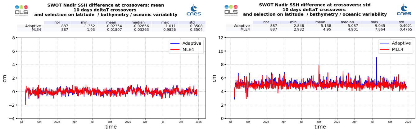
Figure 29: Monitoring of SSH difference at crossovers for SWOT Nadir MLE4 (red) and Adaptive (blue) : mean (left) and standard deviation (right), from cycle 001 to 043
