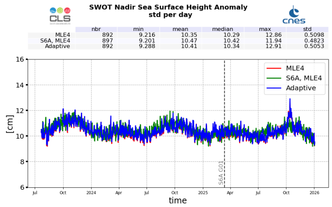
Figure 27: SSHA daily monitoring from cycle 001 to 043, for SWOT Nadir GDR
