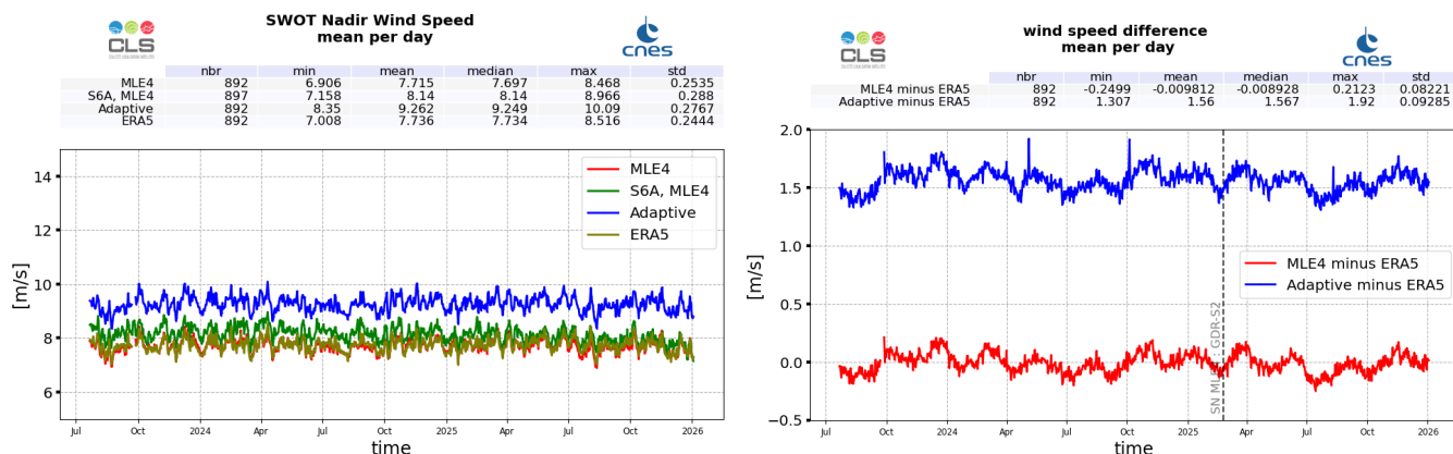
Figure 12: Wind Speed daily monitoring from cycle 001 to 043 for SWOT Nadir GDR, ERA5 model, and Sentinel-6A-MF (LR MLE4) (left), and daily mean difference with ERA5 (right)
