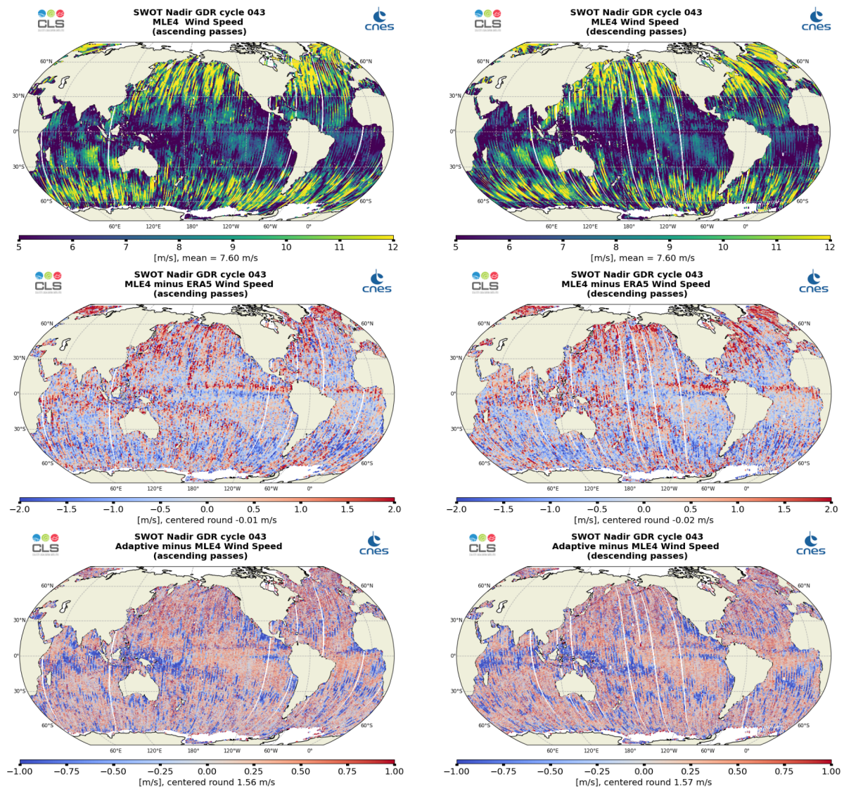
Figure 11: Along-track maps of Altimeter Wind Speed over cycle 043 for SWOT Nadir MLE4 (top), MLE4 minus ERA5 (middle) or Adaptive minus MLE4 (bottom), ascending passes (left) and descending passes (right)
