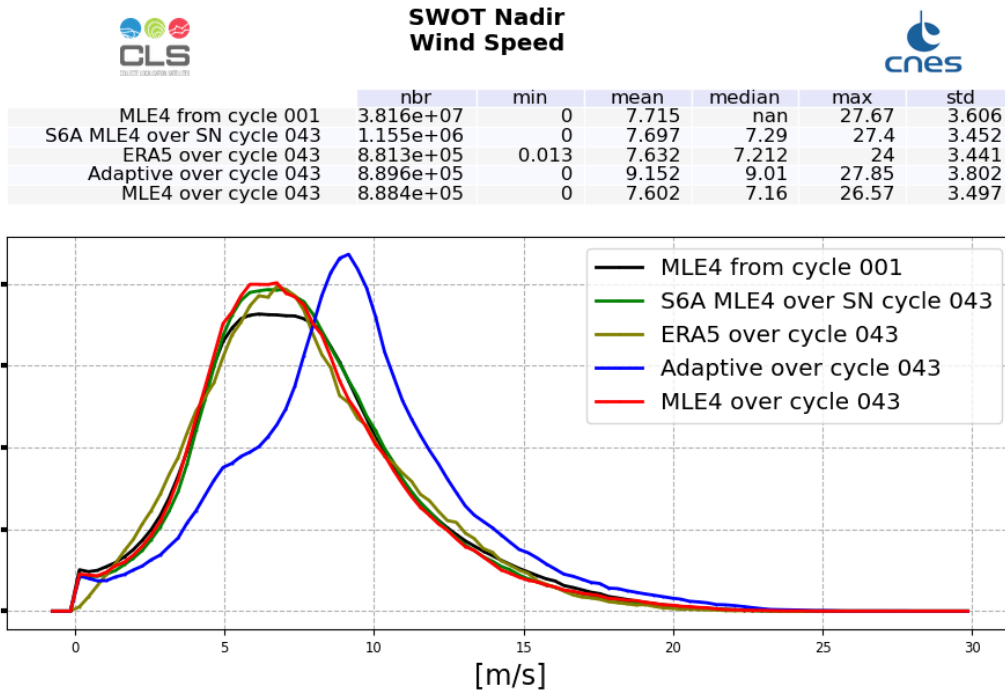
Figure 10: Altimeter Wind Speed histogram computed over cycle 043 (red line for SWOT Nadir MLE4 and blue line for SWOT Nadir Adaptive, green for Sentinel-6A-MF (LR MLE4)) and from cycle 001 (SWOT Nadir, MLE4 only, black line)
