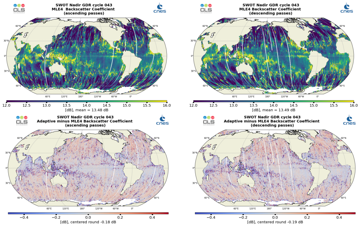
Figure 8: Along-track maps of Ku-band backscatter coefficient \sigma_0 over cycle 043 for SWOT Nadir MLE4 (top) or Adaptive minus MLE4 difference (bottom), ascending passes (left) and descending passes (right)
