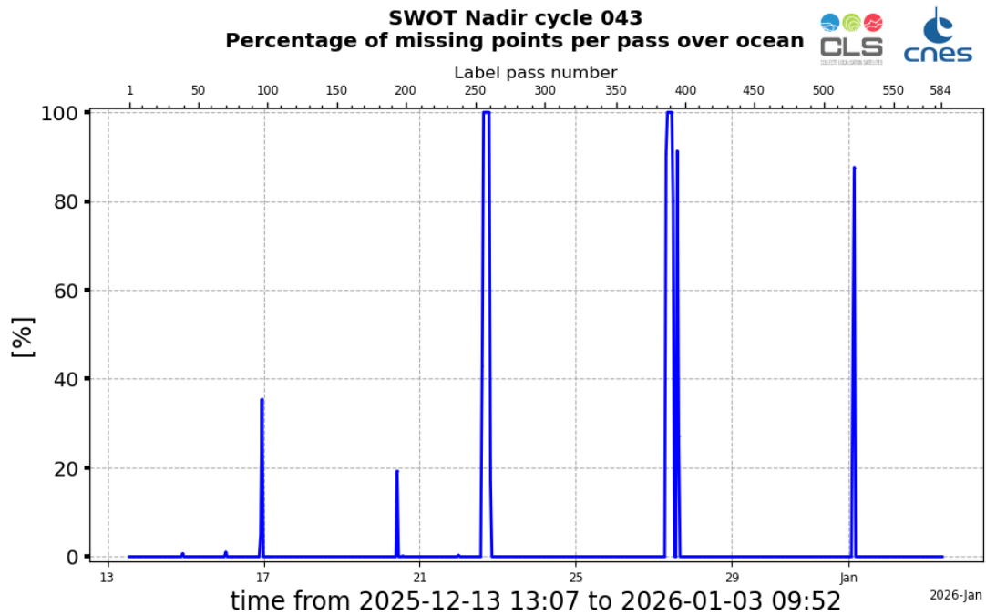
Figure 2: Monitoring of the percentage per pass of missing data over ocean, for SWOT Nadir GDR cycle 043
