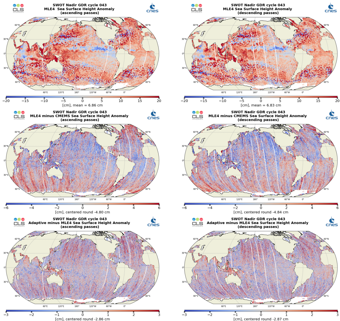
Figure 26: Along-track maps of SSHA over cycle 043 for SWOT Nadir MLE4 (top), MLE4 minus CMEMS (middle) or Adaptive minus MLE4 (bottom), ascending passes (left) and descending passes (right)
