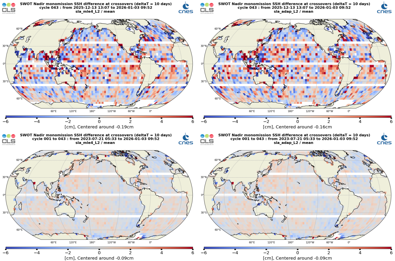
Figure 28: Mean SSH difference at crossovers for SWOT Nadir MLE4 (left) and Adaptive (right) cycle 043(top) and from cycle 001 to cycle 043 (bottom)
