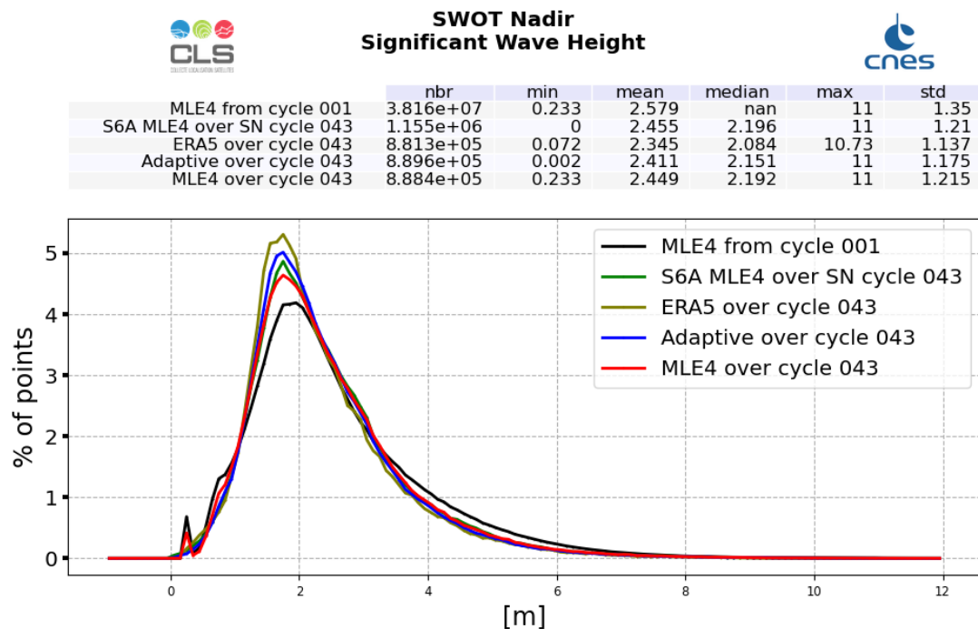
Figure 4: Ku-band Significant Wave Height histogram computed over cycle 043 (red line for SWOT Nadir MLE4 and blue line for SWOT Nadir Adaptive, green for Sentinel-6A-MF (LR MLE4) and dark green for ERA5) and from cycle 001 (SWOT Nadir, MLE4 only, black line)
