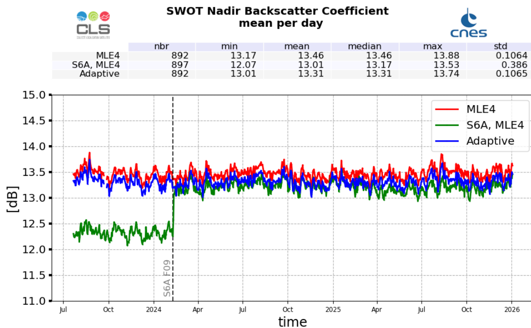
Figure 9: Ku-band Backscattering coefficient daily monitoring from cycle 001 to 043, for SWOT Nadir and Sentinel-6A-MF
