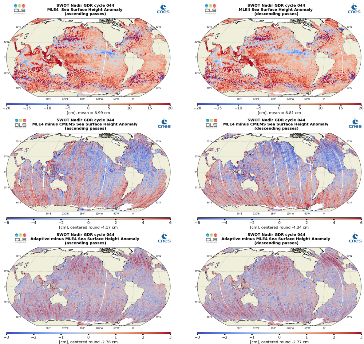
Figure 26: Along-track maps of SSHA over cycle 044 for SWOT Nadir MLE4 (top), MLE4 minus CMEMS (middle) or Adaptive minus MLE4 (bottom), ascending passes (left) and descending passes (right)
