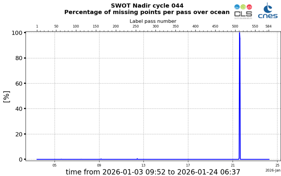
Figure 2: Monitoring of the percentage per pass of missing data over ocean, for SWOT Nadir GDR cycle 044
