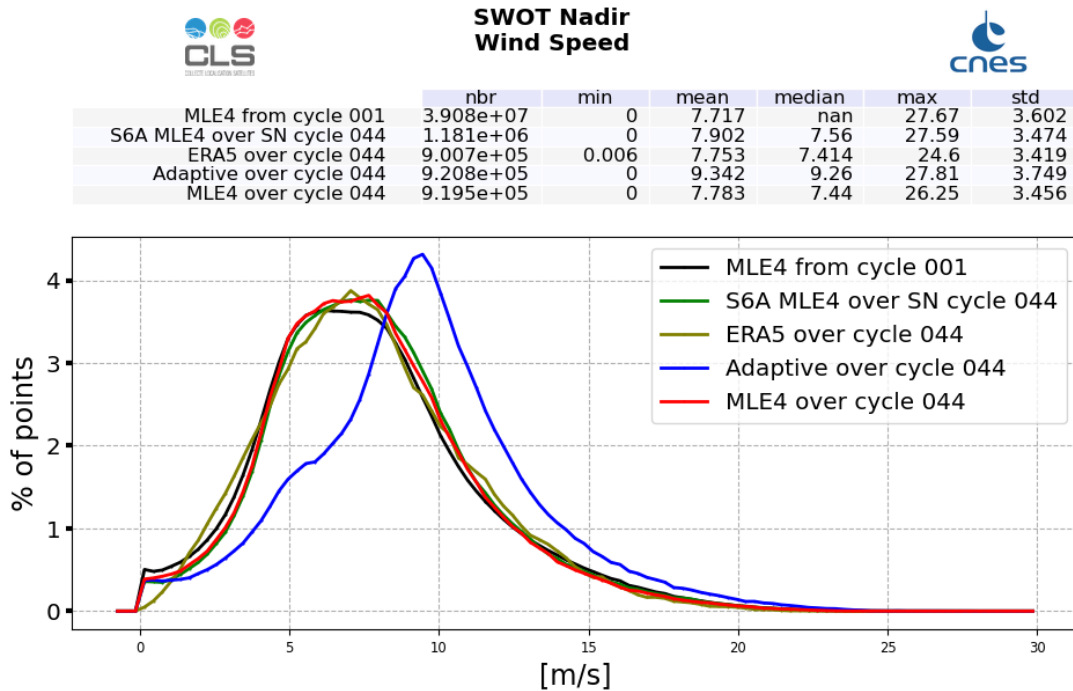
Figure 10: Altimeter Wind Speed histogram computed over cycle 044 (red line for SWOT Nadir MLE4 and blue line for SWOT Nadir Adaptive, green for Sentinel-6A-MF (LR MLE4)) and from cycle 001 (SWOT Nadir, MLE4 only, black line)
