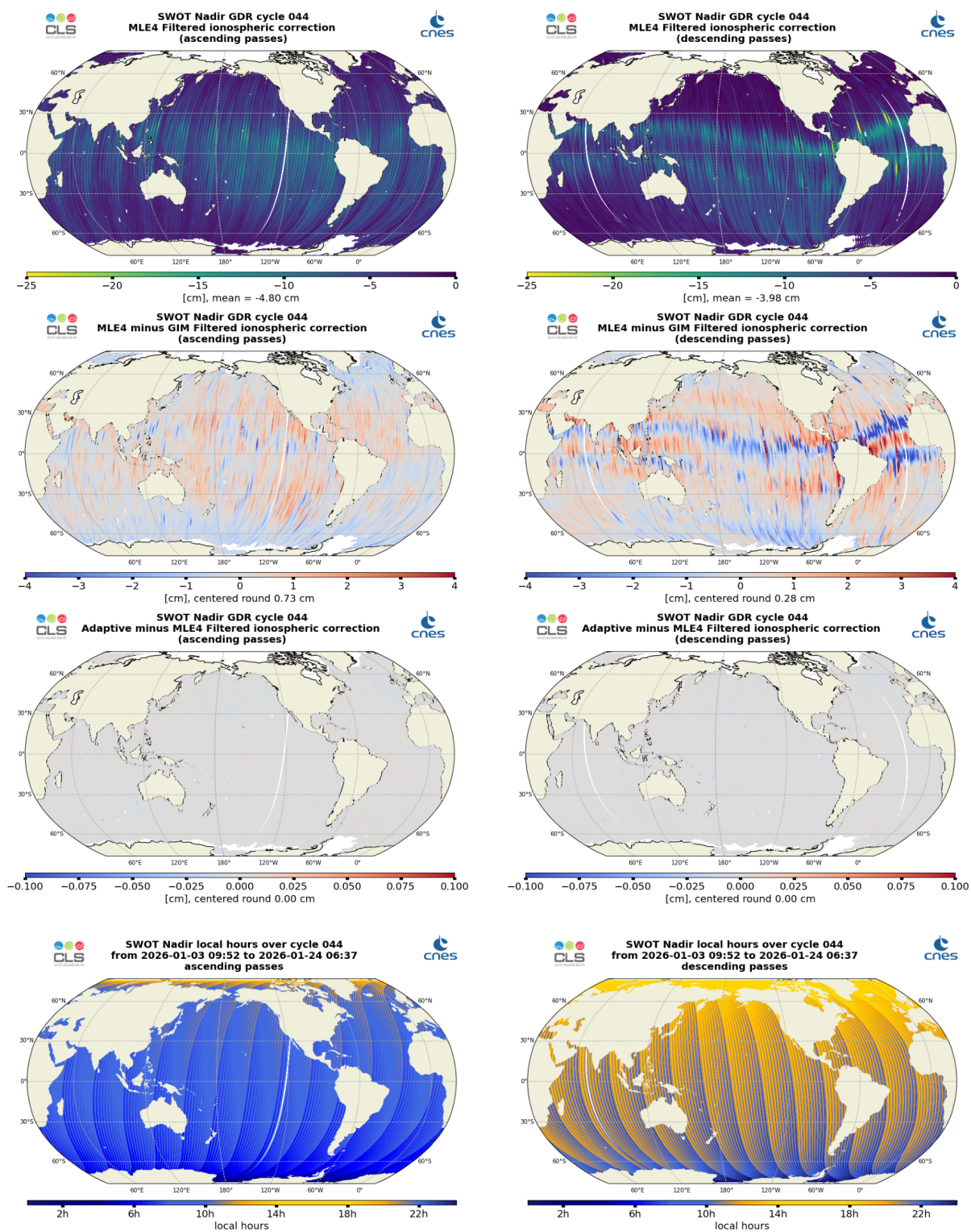
Figure 14: Along-track maps of filtered ionosphere correction over cycle 044 for SWOT Nadir MLE4 (top), MLE4 minus GIM (middle top) or Adaptive minus MLE4 (middle bottom), and local hours (bottom), for ascending passes (left) and descending passes (right)
