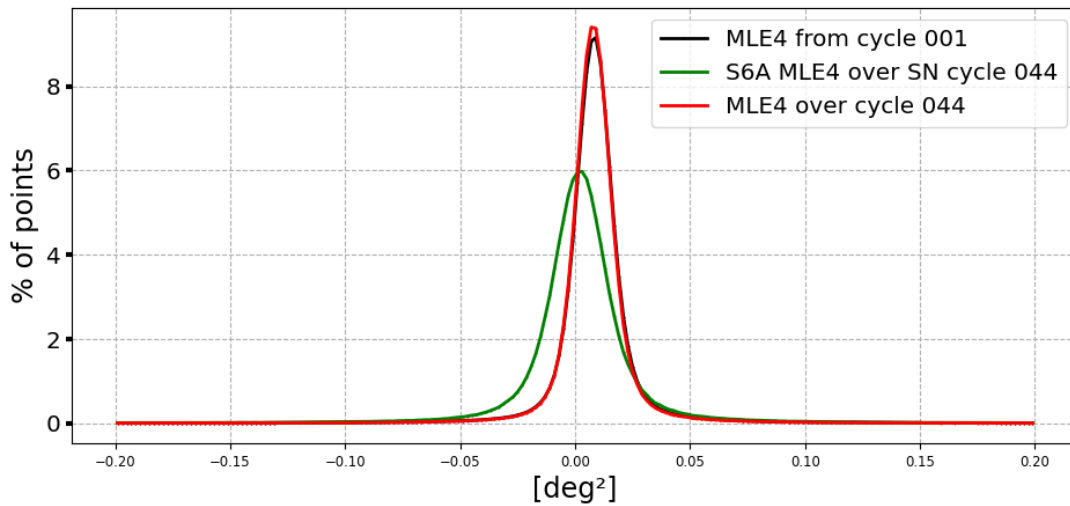
Figure 16: Mispointing histogram computed over cycle 044 (solid line) and from cycle 4 (dashed line)
