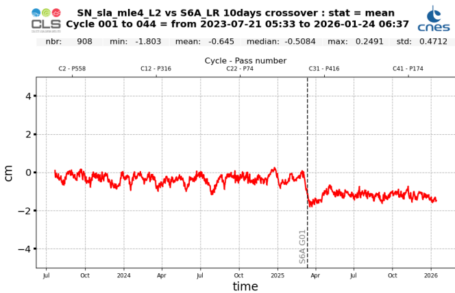
Figure 31: Daily monitoring of SSH difference at crossovers between SWOT Nadir MLE4 and Sentinel-6 MF LR MLE4 from cycle 001 onwards : mean (left) and standard deviation (right)
