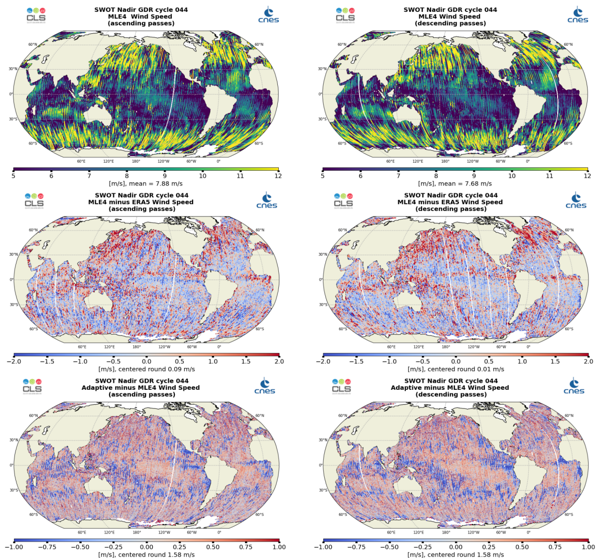
Figure 11: Along-track maps of Altimeter Wind Speed over cycle 044 for SWOT Nadir MLE4 (top), MLE4 minus ERA5 (middle) or Adaptive minus MLE4 (bottom), ascending passes (left) and descending passes (right)
