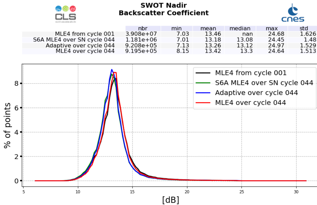
Figure 7: Ku-band Backscattering coefficient histogram computed over cycle 044 (red line for SWOT Nadir MLE4 and blue line for SWOT Nadir Adaptive, green for Sentinel-6A-MF (LR MLE4)) and from cycle 001 (SWOT Nadir, MLE4 only, black line)
