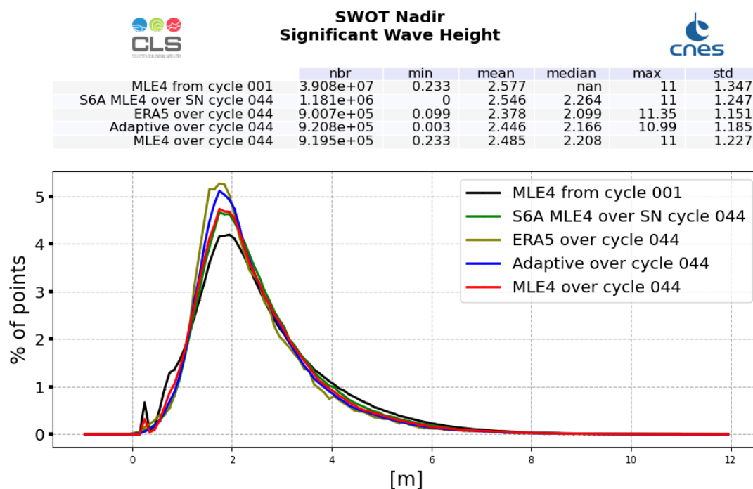
Figure 4: Ku-band Significant Wave Height histogram computed over cycle 044 (red line for SWOT Nadir MLE4 and blue line for SWOT Nadir Adaptive, green for Sentinel-6A-MF (LR MLE4) and dark green for ERA5) and from cycle 001 (SWOT Nadir, MLE4 only, black line)
