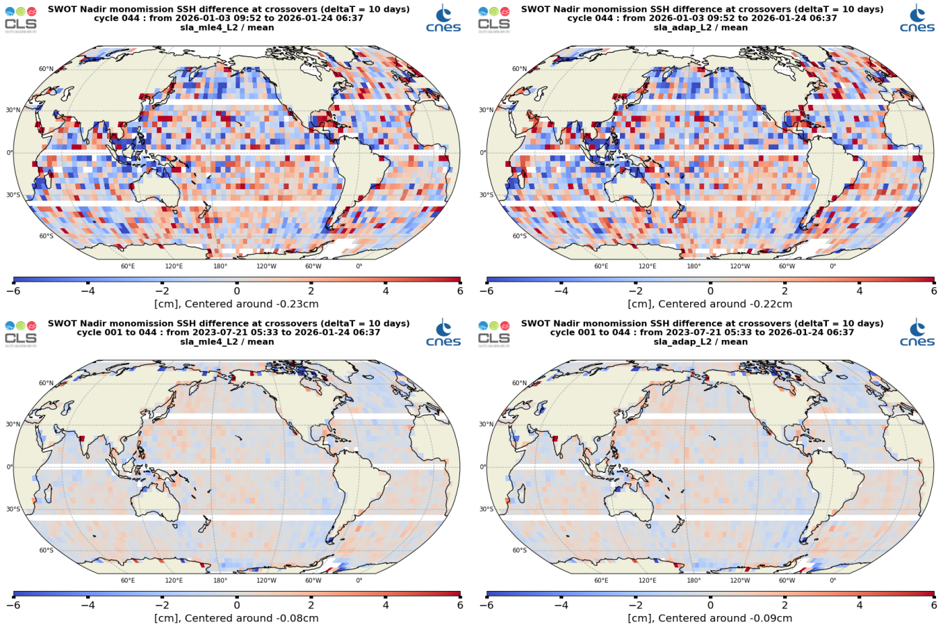
Figure 28: Mean SSH difference at crossovers for SWOT Nadir MLE4 (left) and Adaptive (right) cycle 044(top) and from cycle 001 to cycle 044 (bottom)
