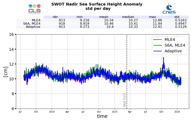
Figure 27: SSHA daily monitoring from cycle 001 to 044, for SWOT Nadir GDR
