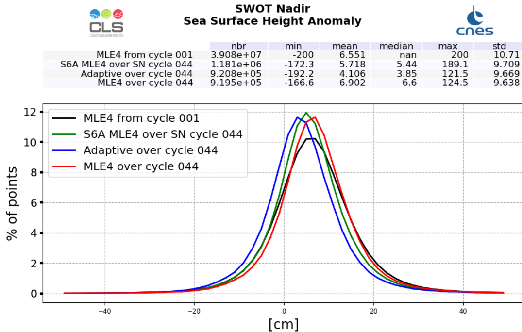
Figure 25: SSHA histogram computed over cycle 044 (red line for SWOT Nadir MLE4 and blue line for SWOT Nadir Adaptive, green for Sentinel-6A-MF (LR MLE4)) and from cycle 001 (SWOT Nadir, MLE4 only, black line)
