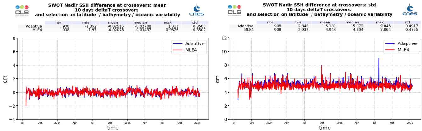
Figure 29: Monitoring of SSH difference at crossovers for SWOT Nadir MLE4 (red) and Adaptive (blue) : mean (left) and standard deviation (right), from cycle 001 to 044
