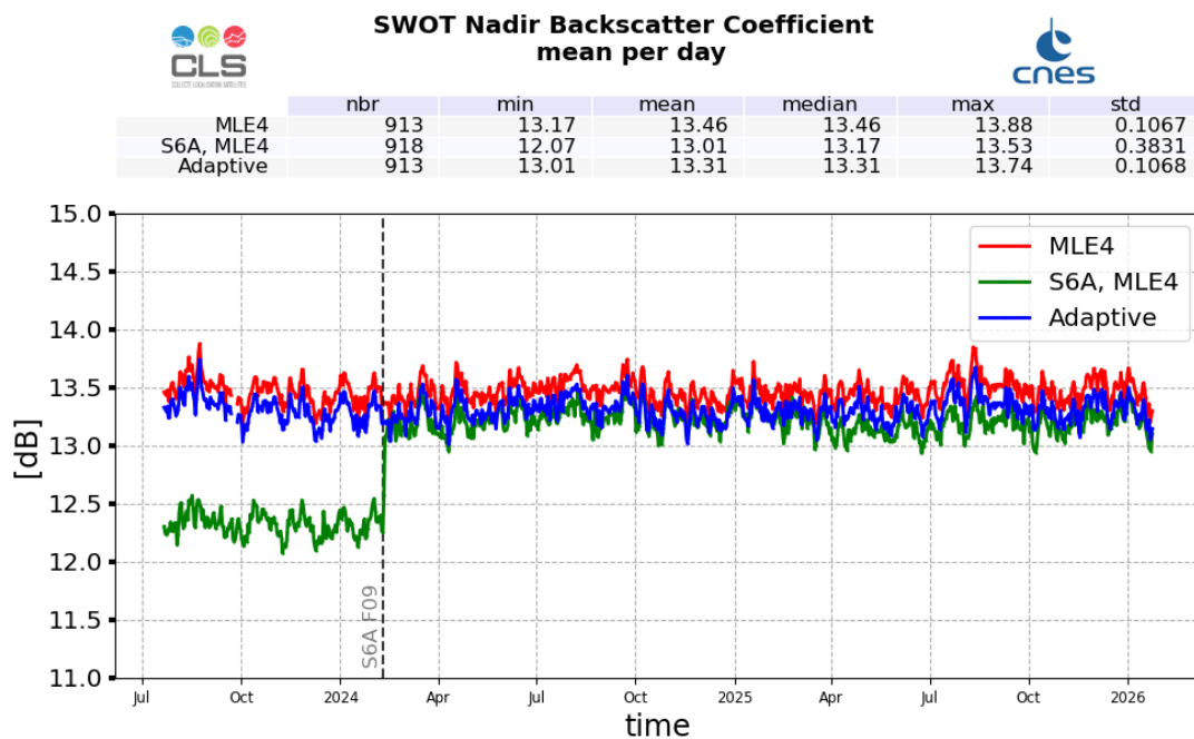
Figure 9: Ku-band Backscattering coefficient daily monitoring from cycle 001 to 044, for SWOT Nadir and Sentinel-6A-MF
