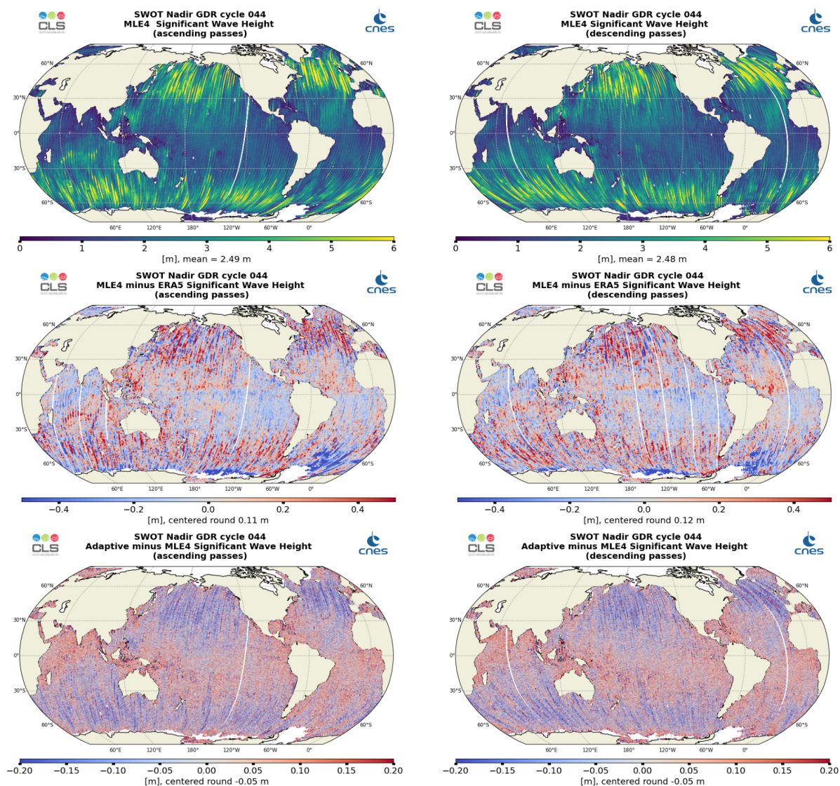
Figure 5: Along-track maps of Ku-band Significant Wave Height over cycle 044 for SWOT Nadir MLE4 (top), MLE4 minus model (middle) or Adaptive minus MLE4 (bottom), ascending passes (left) and descending passes (right)
