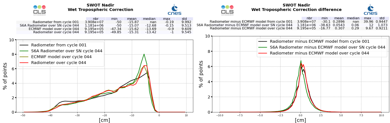
Figure 21: Histogram of wet troposphere corrections : SWOT Nadir radiometer (left) and difference with ECMWF model (right), computed over cycle 044 and from cycle 001 (black line)
