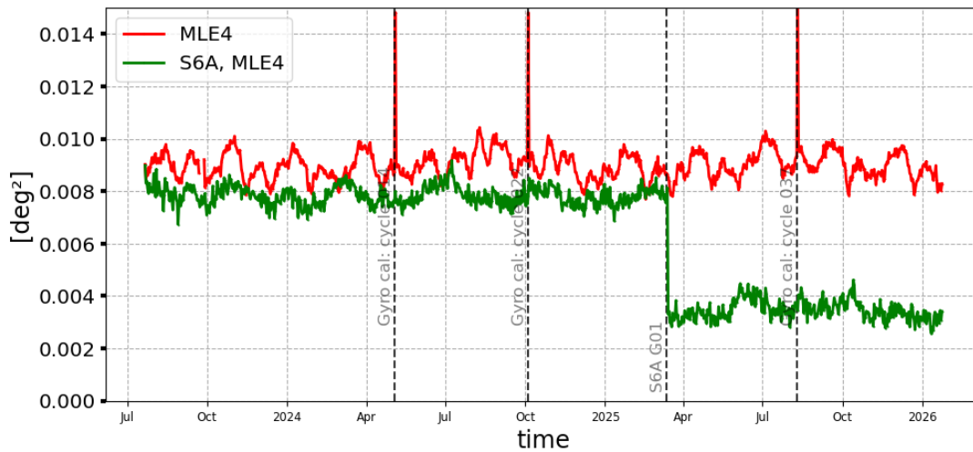
Figure 18: Mispointing daily monitoring from SWOT cycle 001 to 044 for SWOT Nadir GDR (red) and Sentinel-6A-MF (green)
