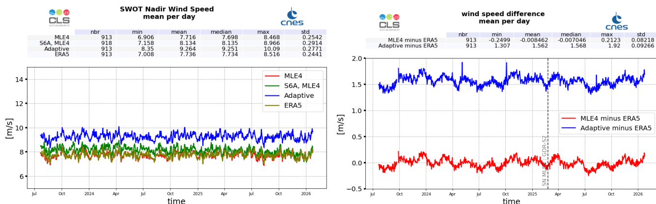
Figure 12: Wind Speed daily monitoring from cycle 001 to 044 for SWOT Nadir GDR, ERA5 model, and Sentinel-6A-MF (LR MLE4) (left), and daily mean difference with ERA5 (right)
