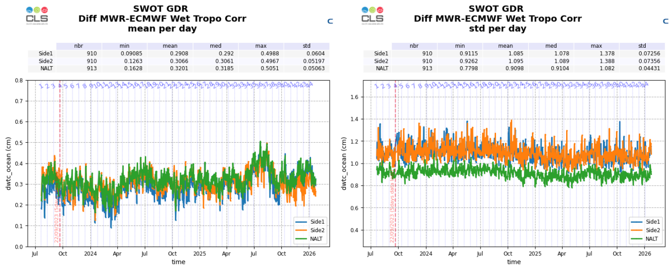
Figure 19: Daily monitoring of mean (left) and standard deviation (right) of the difference between AMRs wet tropospheric correction and ECMWF wet tropospheric correction for the side 1 (blue), the side 2 (orange) and the Nadir (green), computed from cycle 001 to cycle 044
