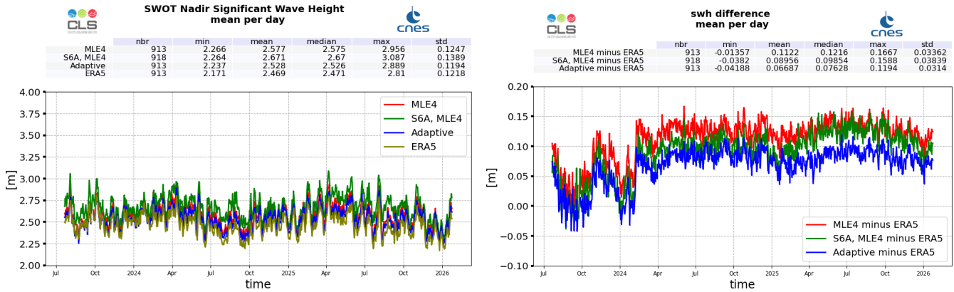
Figure 6: Ku-band Significant Wave Height daily monitoring from cycle 001 to 044, for SWOT Nadir, ERA5 model estimated at SWOT locations, and Sentinel-6A-MF (LR MLE4) (left), and difference with ERA5 model (right)
