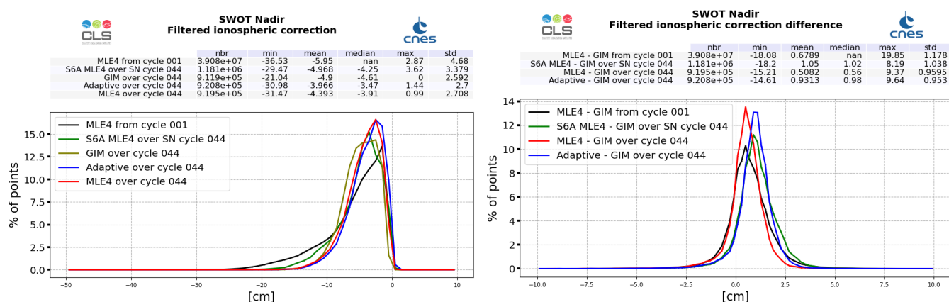
Figure 13: GIM model (dark green) and altimeter filtered ionosphere correction histogram computed over cycle 044 (red line for SWOT Nadir MLE4 and blue line for SWOT Nadir Adaptive, green for Sentinel-6A-MF (LR MLE4)) and from cycle 001 (SWOT Nadir, MLE4 only, black line) (left). Difference between filtered altimeter and GIM model (right).
