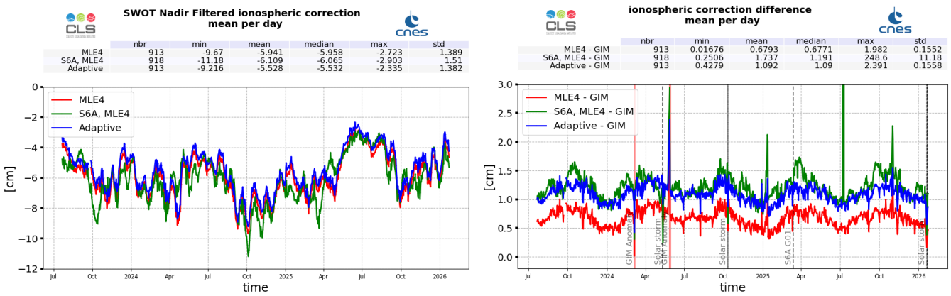
Figure 15: SWOT Nadir MLE4 (red), Adaptive (blue) and Sentinel-6A-MF (LR MLE4) (green) filtered ionosphere correction daily monitoring from cycle 001 to 044 (left) and difference with GIM model (right)
