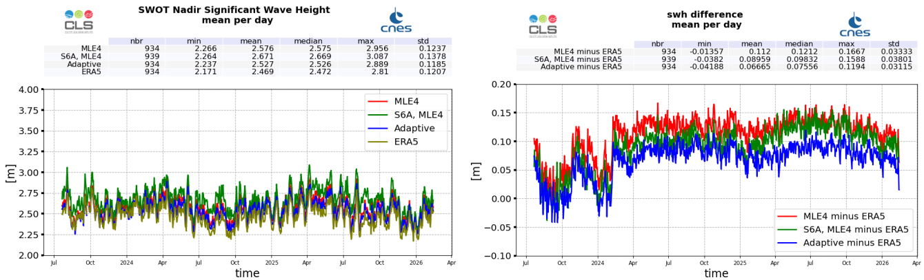
Figure 6: Ku-band Significant Wave Height daily monitoring from cycle 001 to 045, for SWOT Nadir, ERA5 model estimated at SWOT locations, and Sentinel-6A-MF (LR MLE4) (left), and difference with ERA5 model (right)
