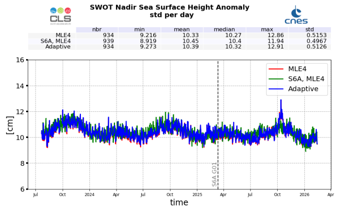
Figure 27: SSHA daily monitoring from cycle 001 to 045, for SWOT Nadir GDR
