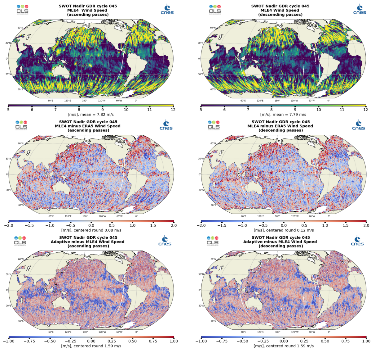
Figure 11: Along-track maps of Altimeter Wind Speed over cycle 045 for SWOT Nadir MLE4 (top), MLE4 minus ERA5 (middle) or Adaptive minus MLE4 (bottom), ascending passes (left) and descending passes (right)
