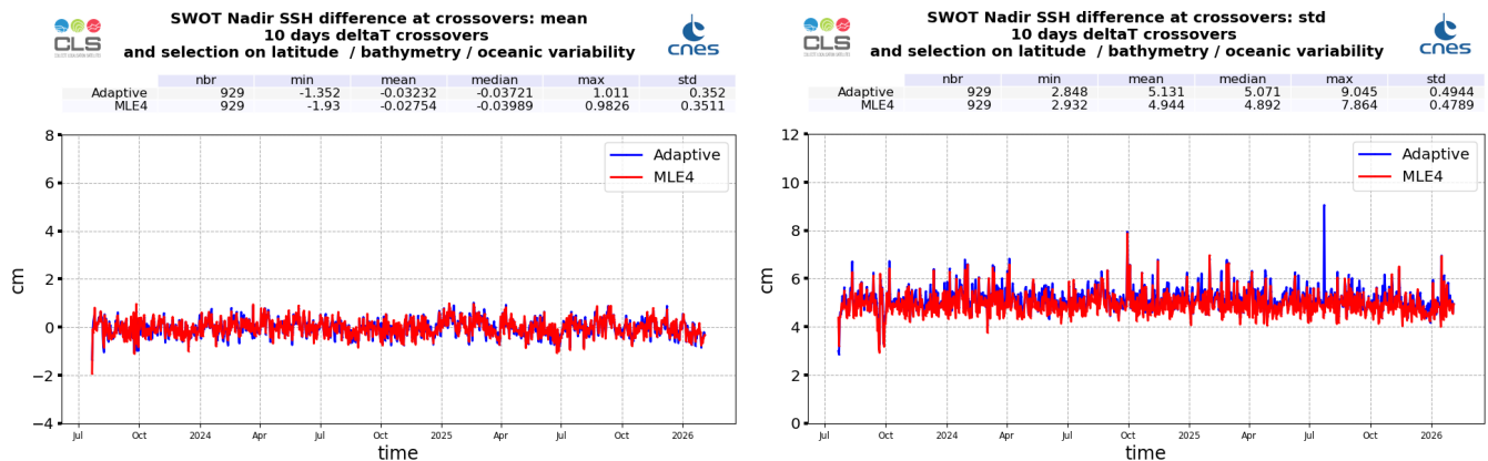
Figure 29: Monitoring of SSH difference at crossovers for SWOT Nadir MLE4 (red) and Adaptive (blue) : mean (left) and standard deviation (right), from cycle 001 to 045
