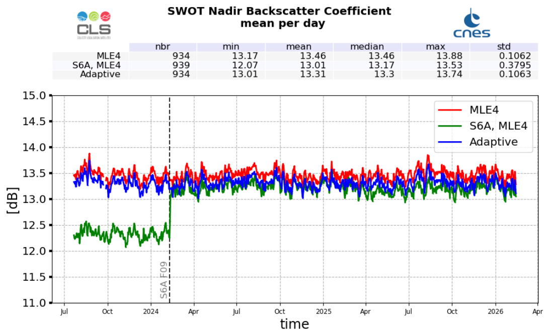
Figure 9: Ku-band Backscattering coefficient daily monitoring from cycle 001 to 045, for SWOT Nadir and Sentinel-6A-MF
