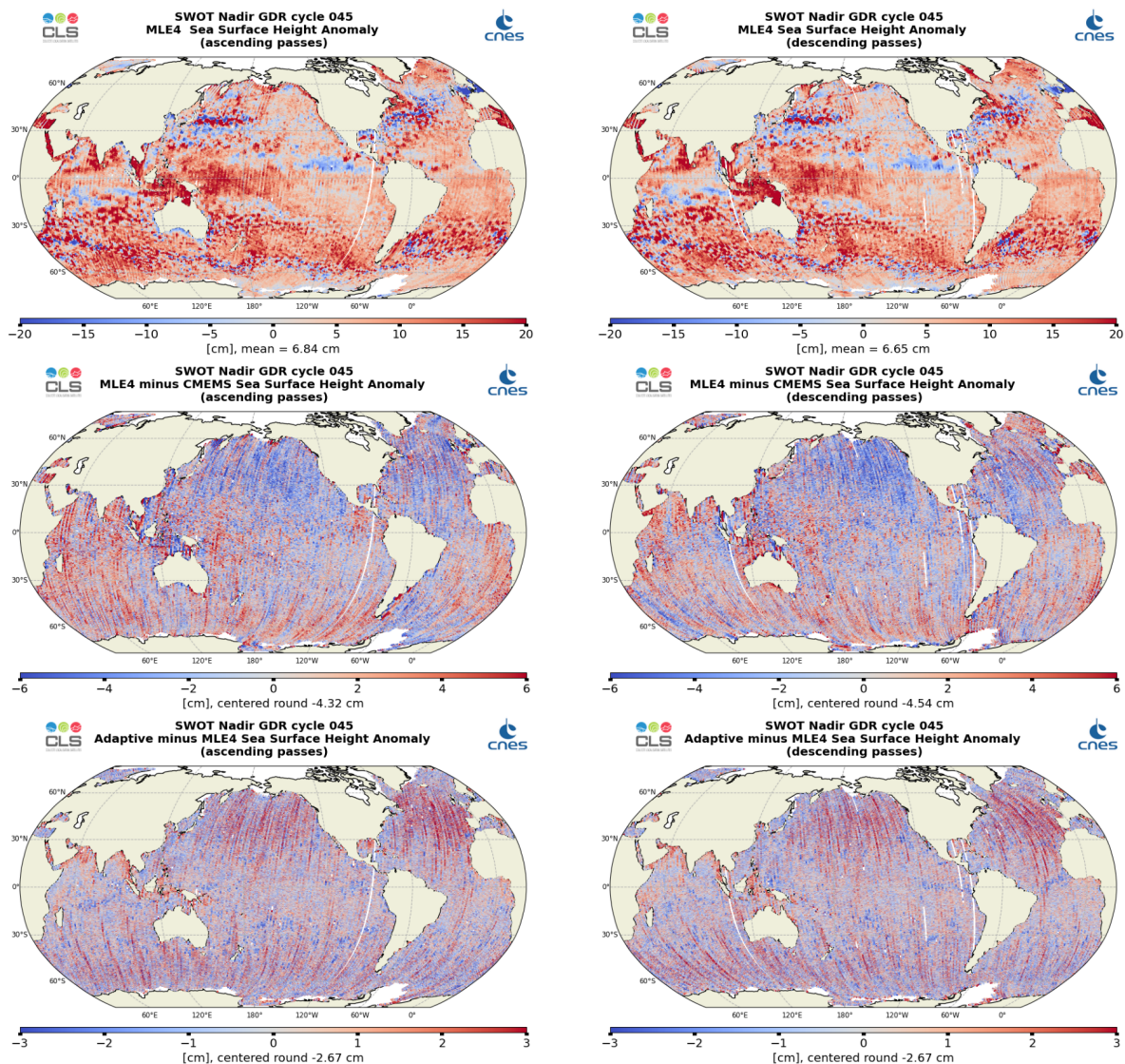
Figure 26: Along-track maps of SSHA over cycle 045 for SWOT Nadir MLE4 (top), MLE4 minus CMEMS (middle) or Adaptive minus MLE4 (bottom), ascending passes (left) and descending passes (right)
