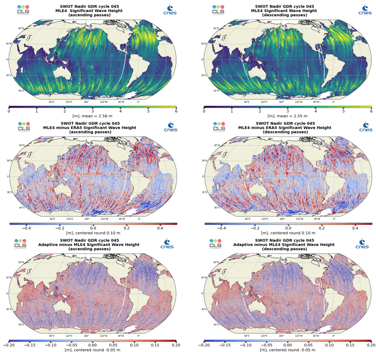
Figure 5: Along-track maps of Ku-band Significant Wave Height over cycle 045 for SWOT Nadir MLE4 (top), MLE4 minus model (middle) or Adaptive minus MLE4 (bottom), ascending passes (left) and descending passes (right)
