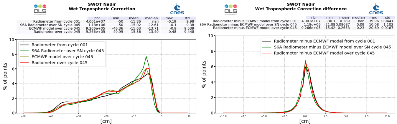
Figure 21: Histogram of wet troposphere corrections : SWOT Nadir radiometer (left) and difference with ECMWF model (right), computed over cycle 045 and from cycle 001 (black line)
