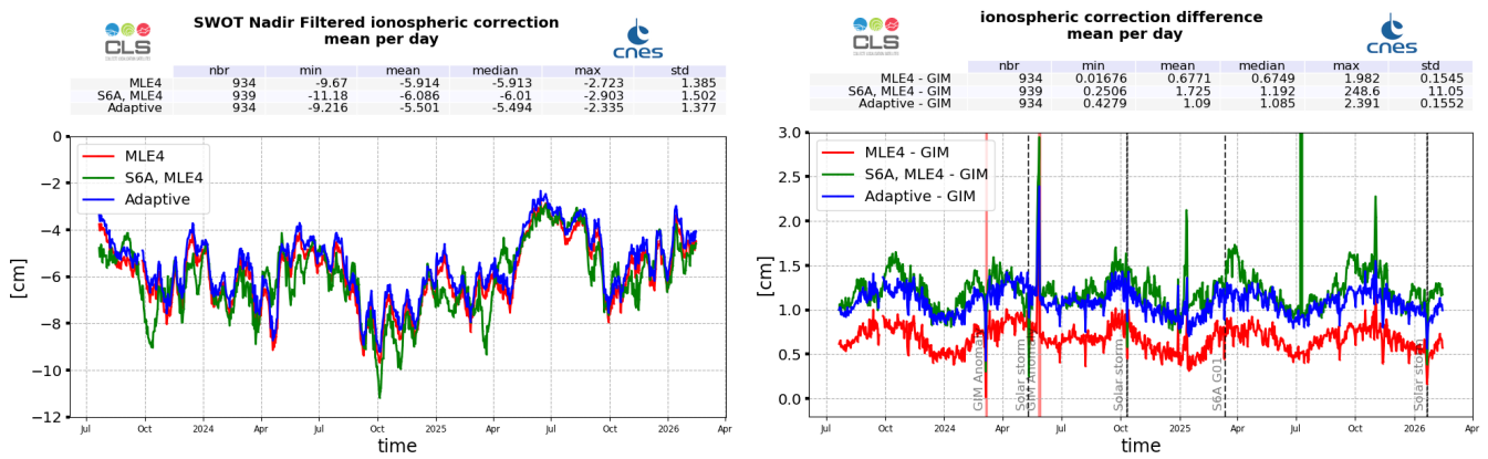
Figure 15: SWOT Nadir MLE4 (red), Adaptive (blue) and Sentinel-6A-MF (LR MLE4) (green) filtered ionosphere correction daily monitoring from cycle 001 to 045 (left) and difference with GIM model (right)
