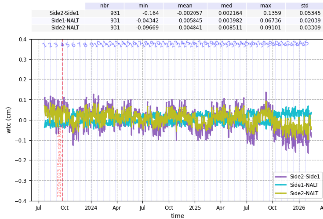
Figure 20: Daily monitoring of the wet tropospheric correction gradient between AMR Side 1 and AMR Side 2 (purple), AMR Side 1 and Nadir (cyan), and AMR Side 2 and Nadir (yellow), from Cycle 001 to 045
