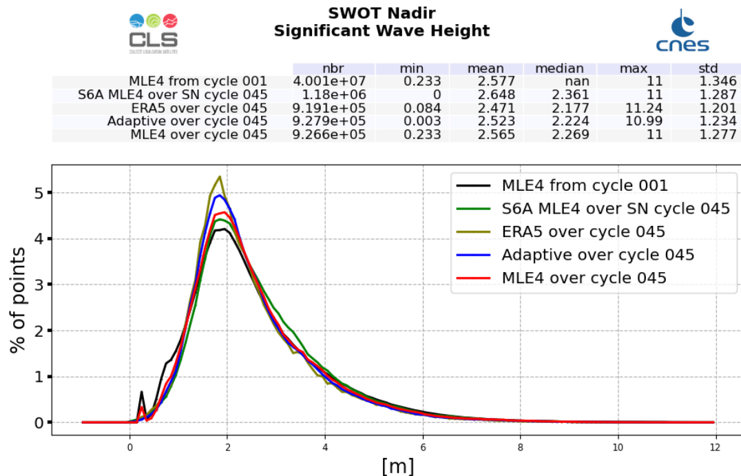
Figure 4: Ku-band Significant Wave Height histogram computed over cycle 045 (red line for SWOT Nadir MLE4 and blue line for SWOT Nadir Adaptive, green for Sentinel-6A-MF (LR MLE4) and dark green for ERA5) and from cycle 001 (SWOT Nadir, MLE4 only, black line)
