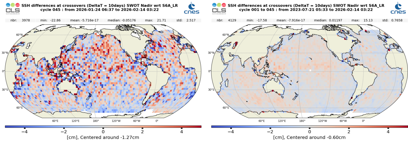
Figure 30: Mean SSH difference at crossovers between SWOT Nadir MLE4 and Sentinel-6 MF LR MLE4 over cycle 045 (left) and from cycle 001 onwards (right)
