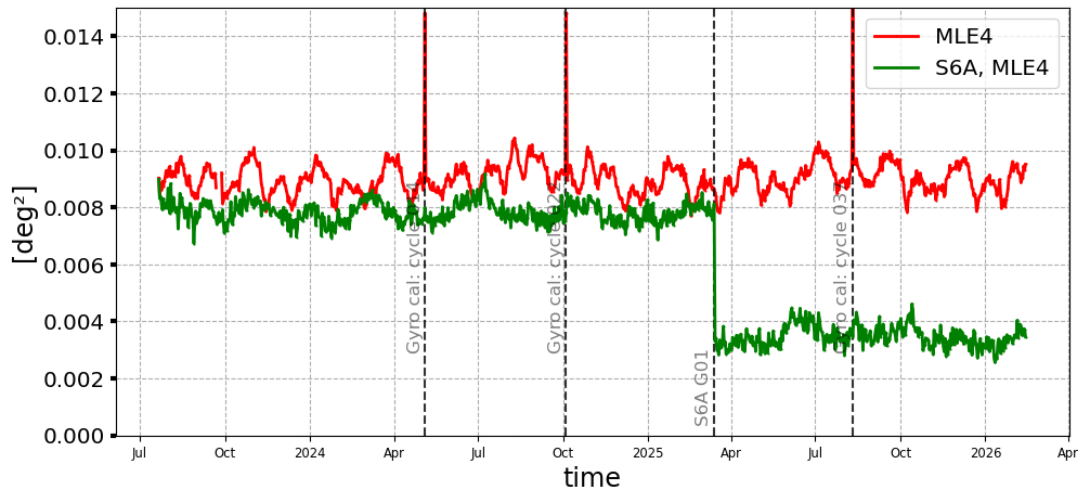
Figure 18: Mispointing daily monitoring from SWOT cycle 001 to 045 for SWOT Nadir GDR (red) and Sentinel-6A-MF (green)
