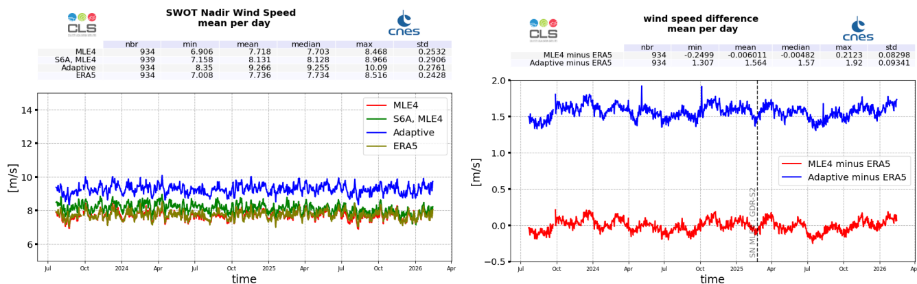
Figure 12: Wind Speed daily monitoring from cycle 001 to 045 for SWOT Nadir GDR, ERA5 model, and Sentinel-6A-MF (LR MLE4) (left), and daily mean difference with ERA5 (right)
