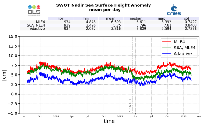
Figure 27: SSHA daily monitoring from cycle 001 to 045, for SWOT Nadir GDR
