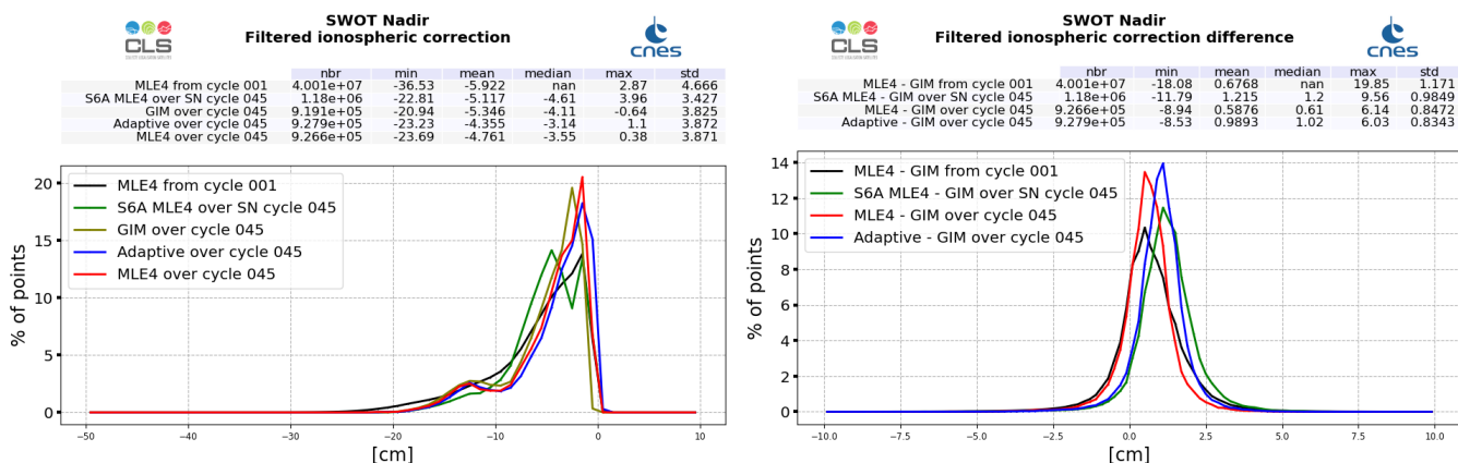
Figure 13: GIM model (dark green) and altimeter filtered ionosphere correction histogram computed over cycle 045 (red line for SWOT Nadir MLE4 and blue line for SWOT Nadir Adaptive, green for Sentinel-6A-MF (LR MLE4)) and from cycle 001 (SWOT Nadir, MLE4 only, black line) (left). Difference between filtered altimeter and GIM model (right).
