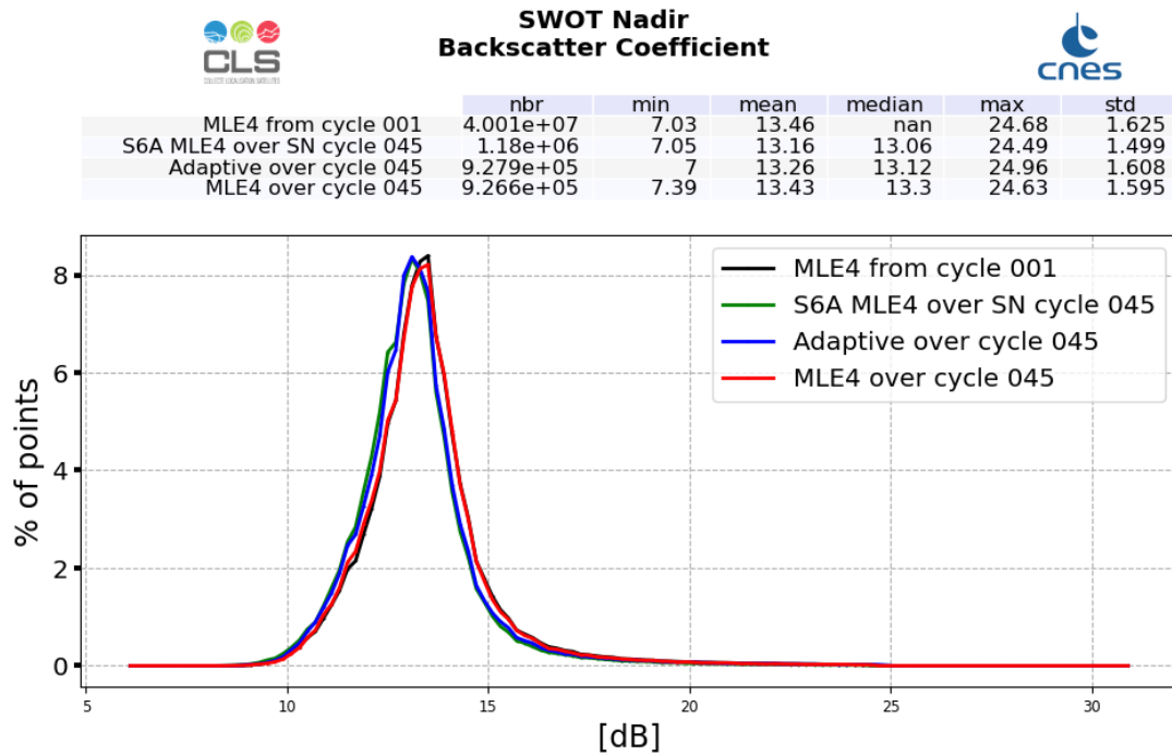
Figure 7: Ku-band Backscattering coefficient histogram computed over cycle 045 (red line for SWOT Nadir MLE4 and blue line for SWOT Nadir Adaptive, green for Sentinel-6A-MF (LR MLE4)) and from cycle 001 (SWOT Nadir, MLE4 only, black line)
