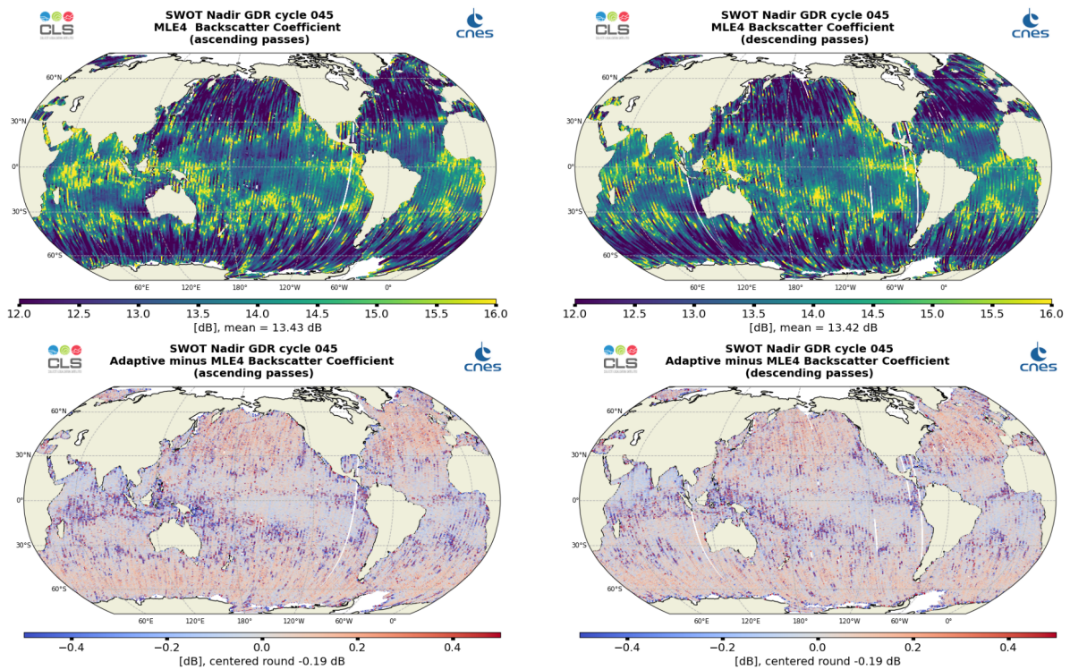
Figure 8: Along-track maps of Ku-band backscatter coefficient \sigma_0 over cycle 045 for SWOT Nadir MLE4 (top) or Adaptive minus MLE4 difference (bottom), ascending passes (left) and descending passes (right)
