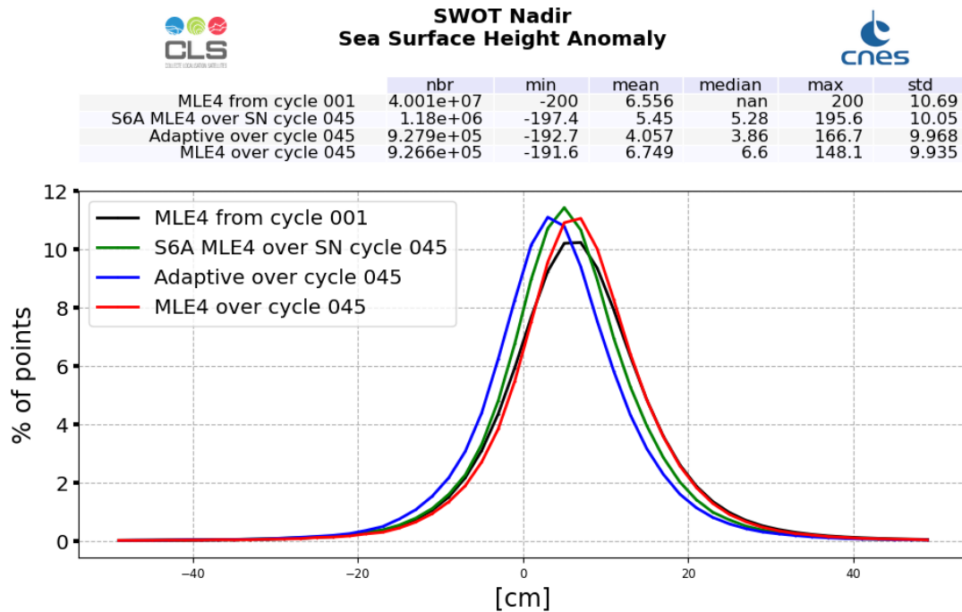
Figure 25: SSHA histogram computed over cycle 045 (red line for SWOT Nadir MLE4 and blue line for SWOT Nadir Adaptive, green for Sentinel-6A-MF (LR MLE4)) and from cycle 001 (SWOT Nadir, MLE4 only, black line)
