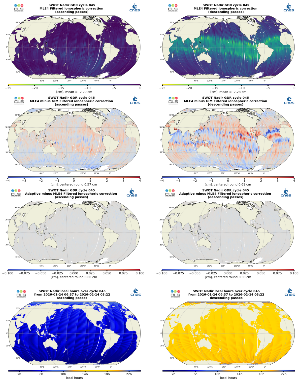
Figure 14: Along-track maps of filtered ionosphere correction over cycle 045 for SWOT Nadir MLE4 (top), MLE4 minus GIM (middle top) or Adaptive minus MLE4 (middle bottom), and local hours (bottom), for ascending passes (left) and descending passes (right)
