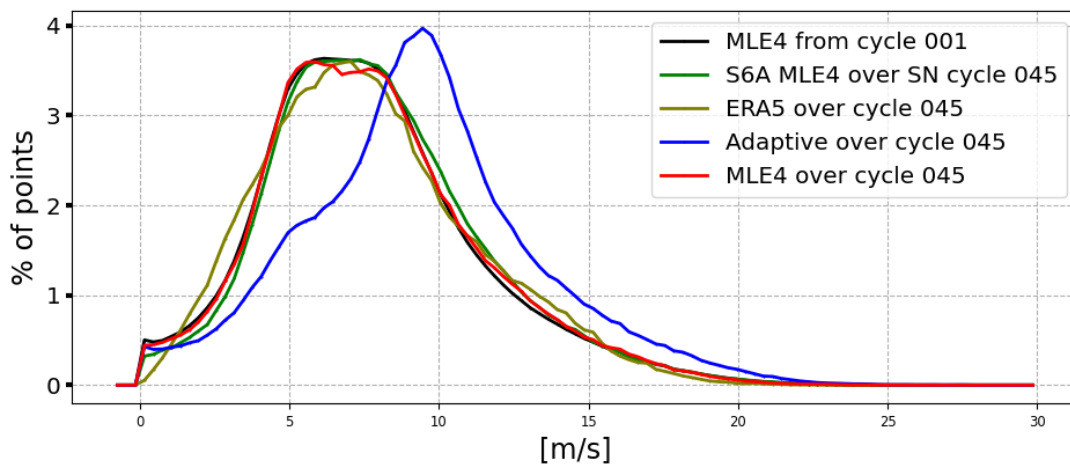
Figure 10: Altimeter Wind Speed histogram computed over cycle 045 (red line for SWOT Nadir MLE4 and blue line for SWOT Nadir Adaptive, green for Sentinel-6A-MF (LR MLE4)) and from cycle 001 (SWOT Nadir, MLE4 only, black line)
