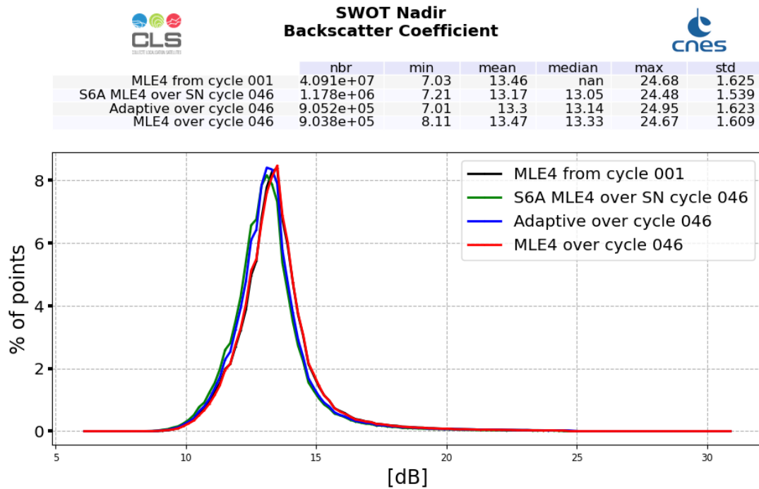
Figure 7: Ku-band Backscattering coefficient histogram computed over cycle 046 (red line for SWOT Nadir MLE4 and blue line for SWOT Nadir Adaptive, green for Sentinel-6A-MF (LR MLE4)) and from cycle 001 (SWOT Nadir, MLE4 only, black line)
