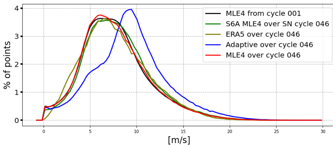
Figure 10: Altimeter Wind Speed histogram computed over cycle 046 (red line for SWOT Nadir MLE4 and blue line for SWOT Nadir Adaptive, green for Sentinel-6A-MF (LR MLE4)) and from cycle 001 (SWOT Nadir, MLE4 only, black line)
