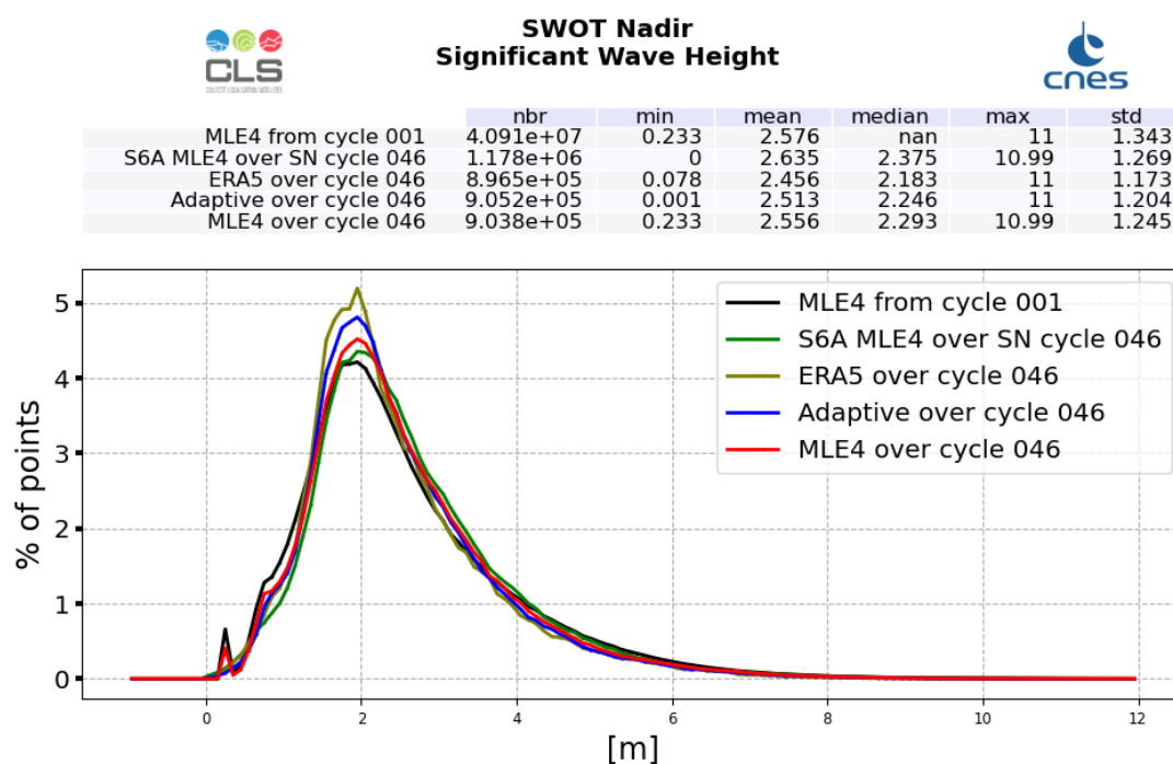
Figure 4: Ku-band Significant Wave Height histogram computed over cycle 046 (red line for SWOT Nadir MLE4 and blue line for SWOT Nadir Adaptive, green for Sentinel-6A-MF (LR MLE4) and dark green for ERA5) and from cycle 001 (SWOT Nadir, MLE4 only, black line)
