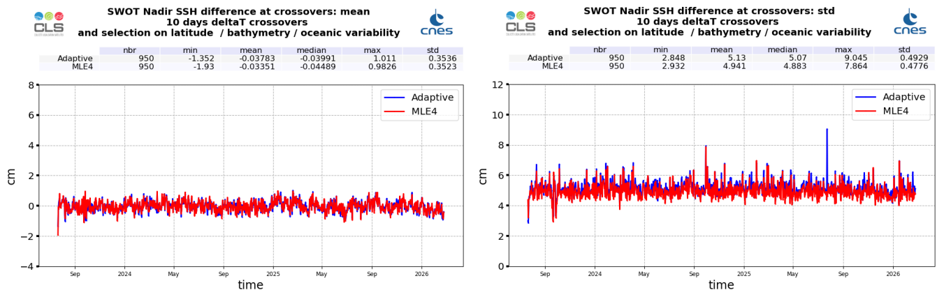
Figure 29: Monitoring of SSH difference at crossovers for SWOT Nadir MLE4 (red) and Adaptive (blue) : mean (left) and standard deviation (right), from cycle 001 to 046
