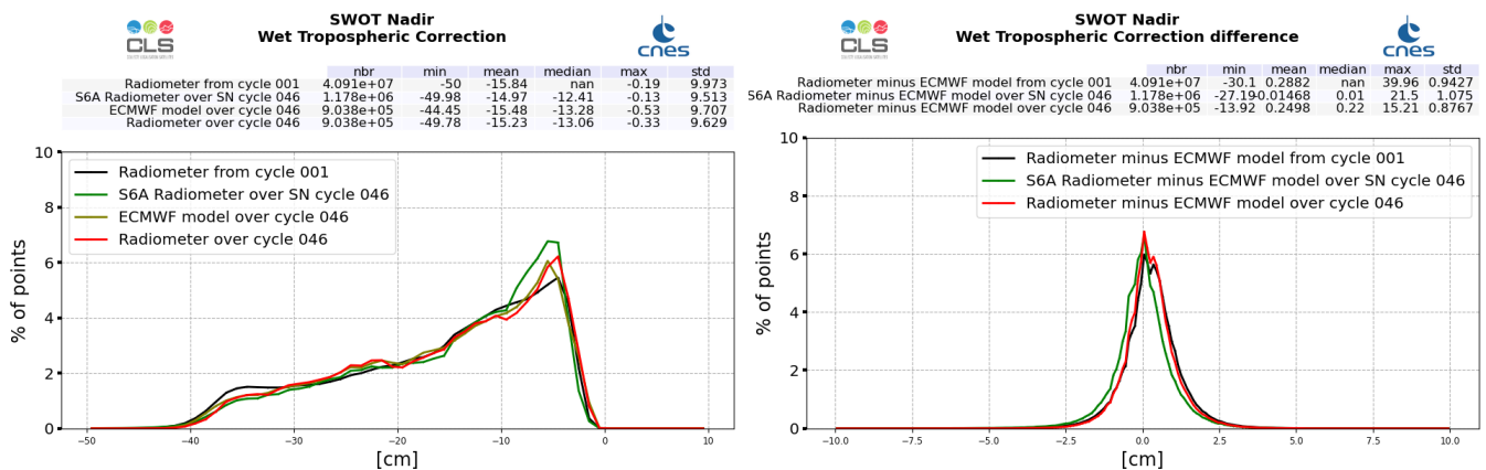
Figure 21: Histogram of wet troposphere corrections : SWOT Nadir radiometer (left) and difference with ECMWF model (right), computed over cycle 046 and from cycle 001 (black line)
