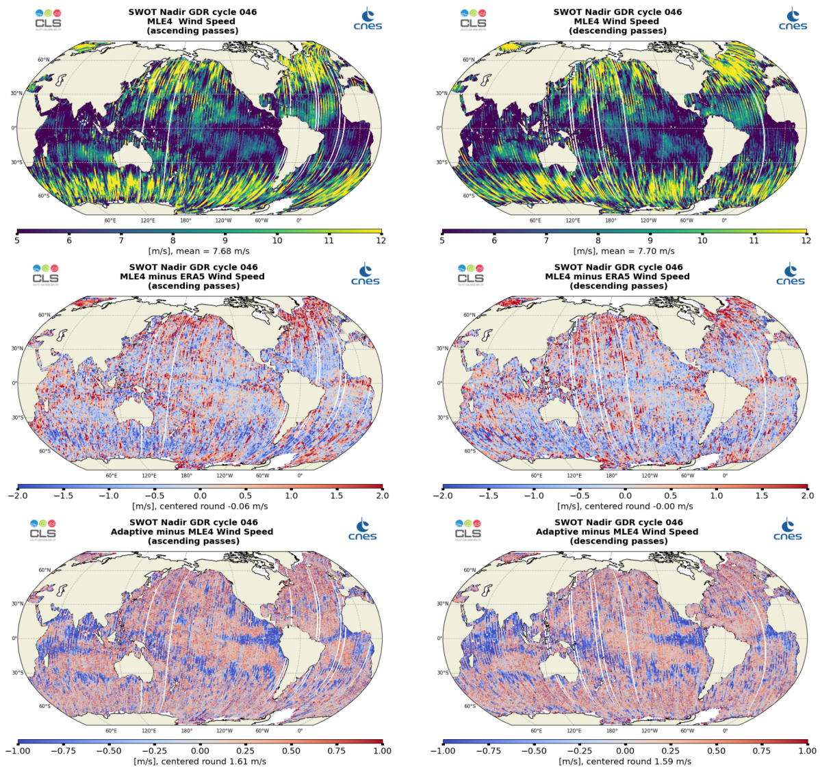
Figure 11: Along-track maps of Altimeter Wind Speed over cycle 046 for SWOT Nadir MLE4 (top), MLE4 minus ERA5 (middle) or Adaptive minus MLE4 (bottom), ascending passes (left) and descending passes (right)
