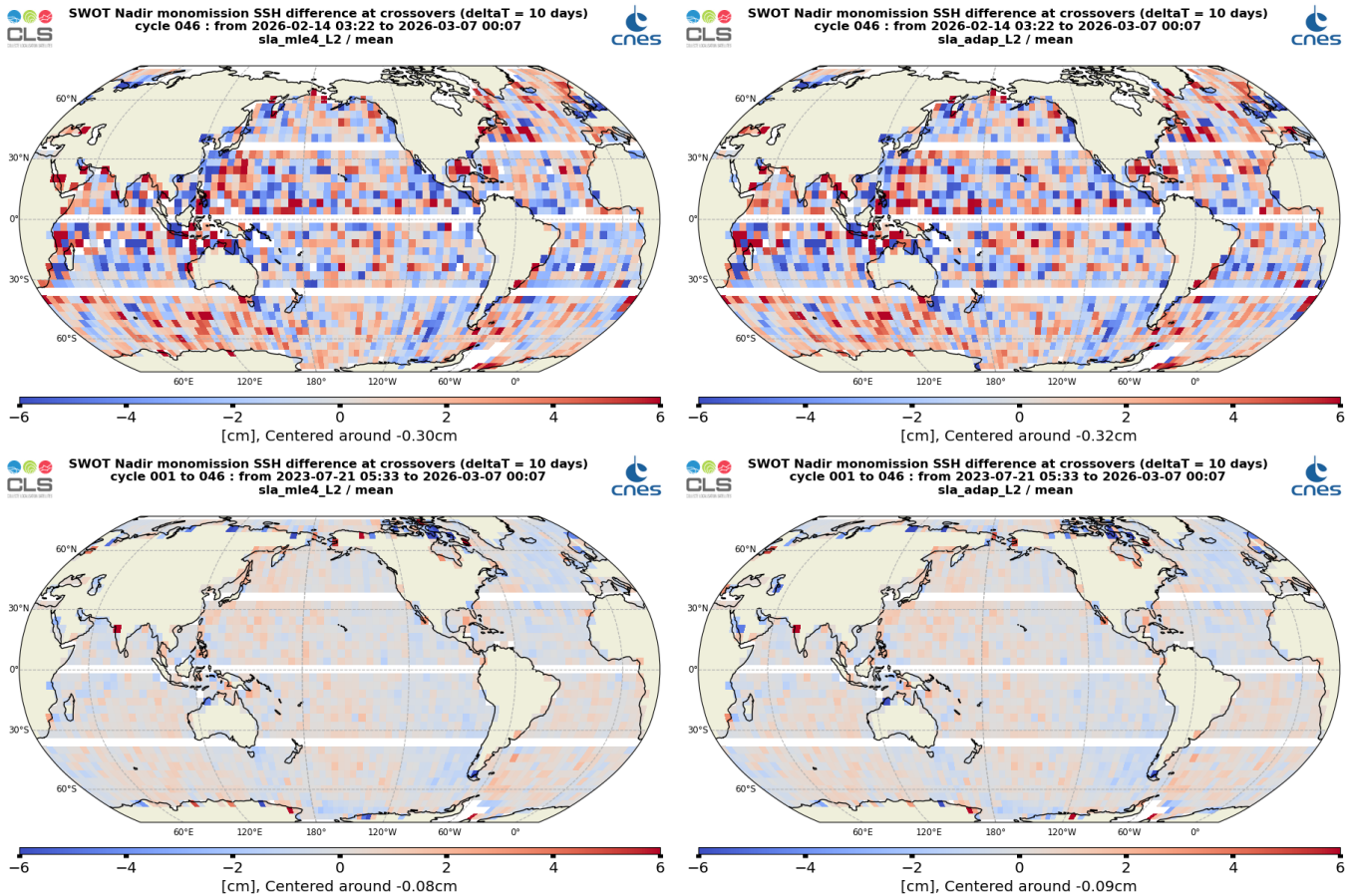
Figure 28: Mean SSH difference at crossovers for SWOT Nadir MLE4 (left) and Adaptive (right) cycle 046(top) and from cycle 001 to cycle 046 (bottom)
