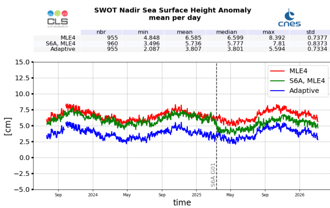
Figure 27: SSHA daily monitoring from cycle 001 to 046, for SWOT Nadir GDR
