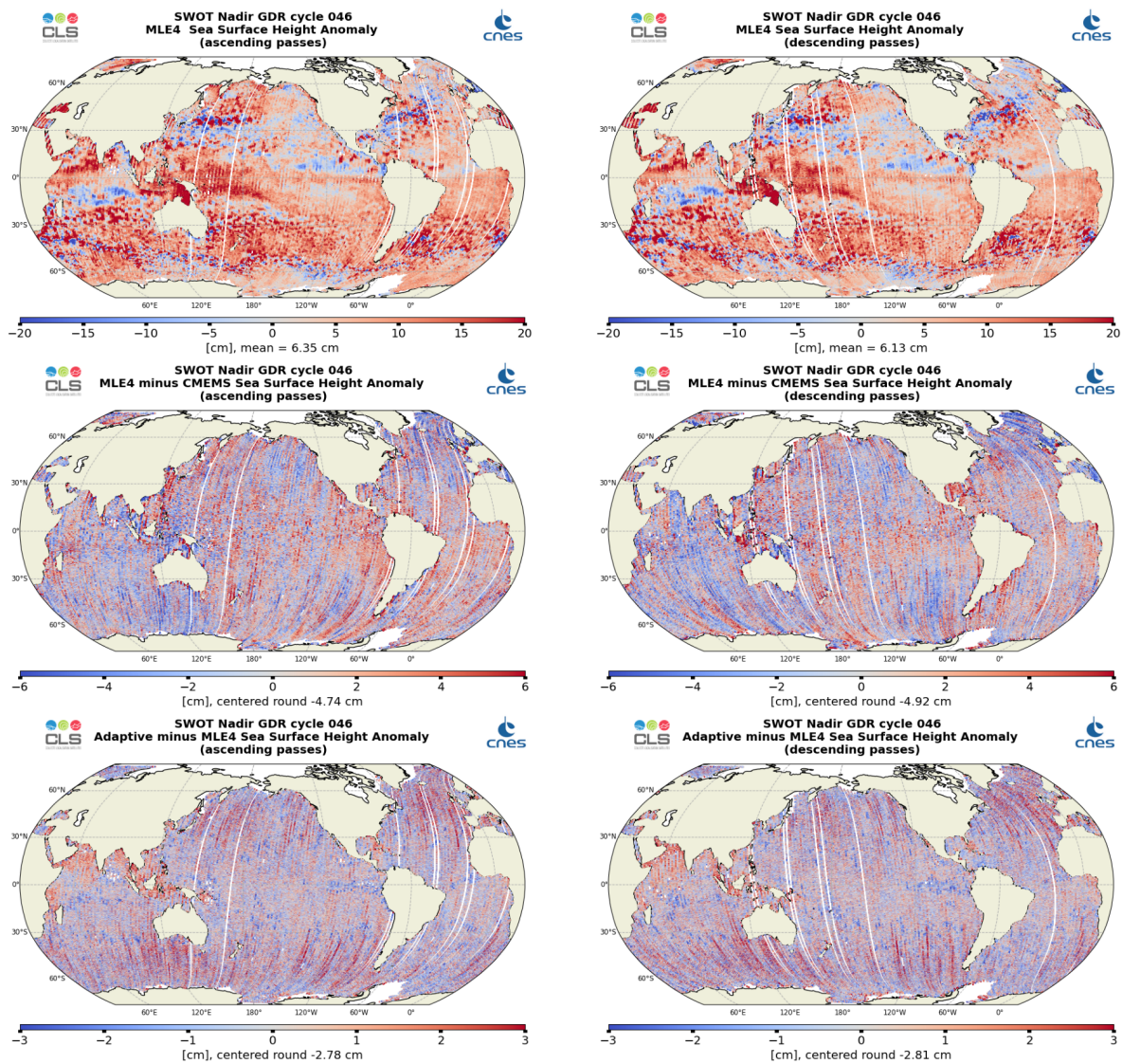
Figure 26: Along-track maps of SSHA over cycle 046 for SWOT Nadir MLE4 (top), MLE4 minus CMEMS (middle) or Adaptive minus MLE4 (bottom), ascending passes (left) and descending passes (right)
