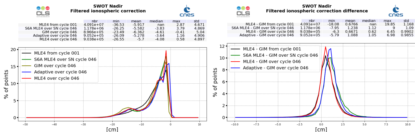
Figure 13: GIM model (dark green) and altimeter filtered ionosphere correction histogram computed over cycle 046 (red line for SWOT Nadir MLE4 and blue line for SWOT Nadir Adaptive, green for Sentinel-6A-MF (LR MLE4)) and from cycle 001 (SWOT Nadir, MLE4 only, black line) (left). Difference between filtered altimeter and GIM model (right).
