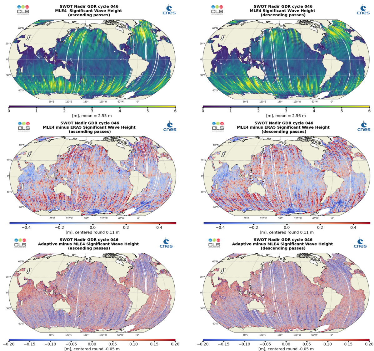
Figure 5: Along-track maps of Ku-band Significant Wave Height over cycle 046 for SWOT Nadir MLE4 (top), MLE4 minus model (middle) or Adaptive minus MLE4 (bottom), ascending passes (left) and descending passes (right)
