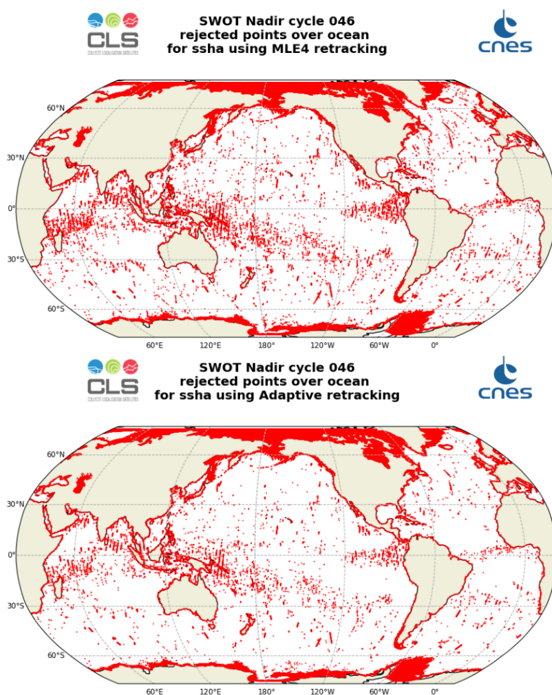
Figure 3: Edited measurements for SWOT Nadir over cycle 046
