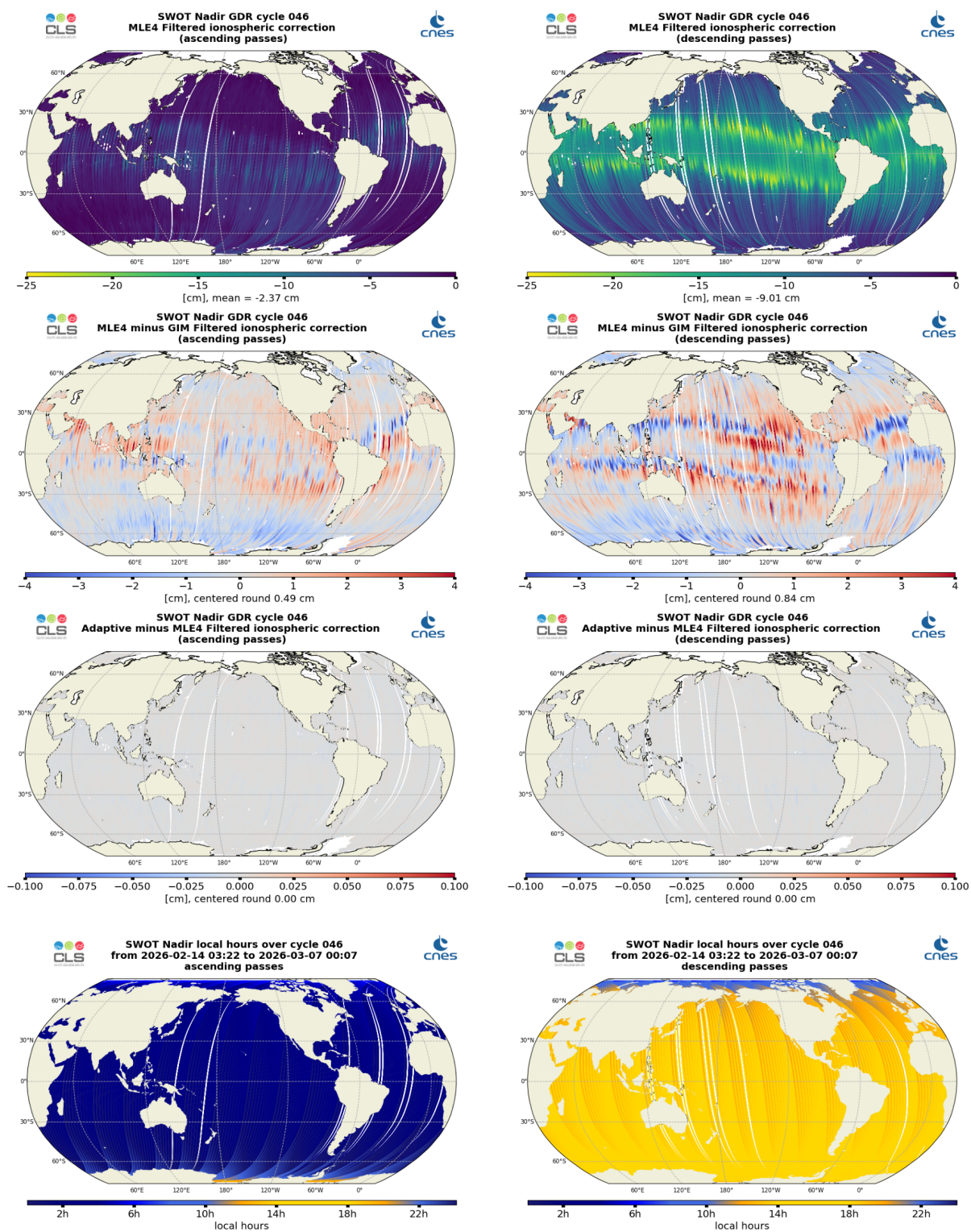
Figure 14: Along-track maps of filtered ionosphere correction over cycle 046 for SWOT Nadir MLE4 (top), MLE4 minus GIM (middle top) or Adaptive minus MLE4 (middle bottom), and local hours (bottom), for ascending passes (left) and descending passes (right)
