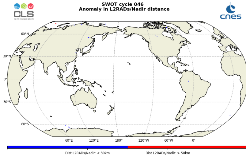
Figure 24: Map of the anomalies detected in the L2RADs/Nadir distance over the cycle 046
