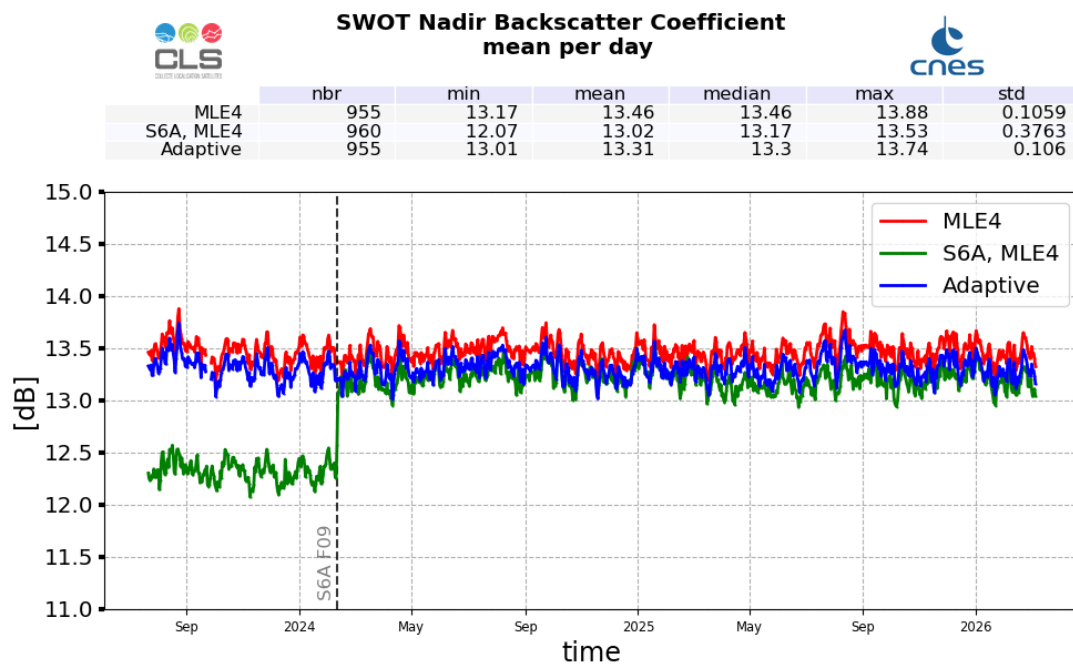
Figure 9: Ku-band Backscattering coefficient daily monitoring from cycle 001 to 046, for SWOT Nadir and Sentinel-6A-MF
