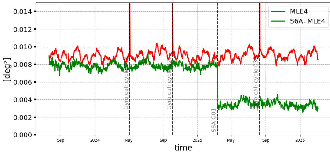
Figure 18: Mispointing daily monitoring from SWOT cycle 001 to 046 for SWOT Nadir GDR (red) and Sentinel-6A-MF (green)
