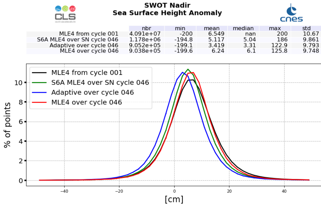
Figure 25: SSHA histogram computed over cycle 046 (red line for SWOT Nadir MLE4 and blue line for SWOT Nadir Adaptive, green for Sentinel-6A-MF (LR MLE4)) and from cycle 001 (SWOT Nadir, MLE4 only, black line)
