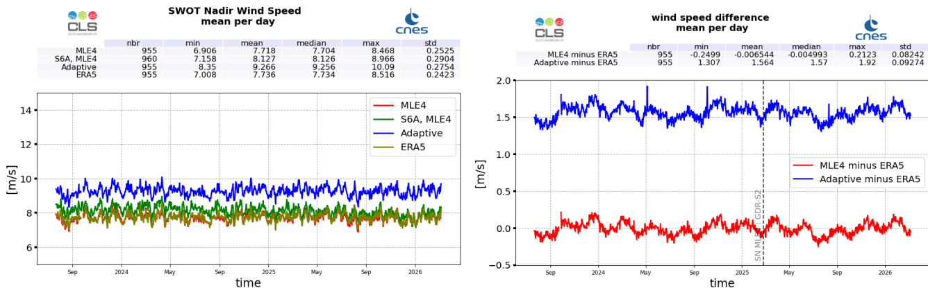
Figure 12: Wind Speed daily monitoring from cycle 001 to 046 for SWOT Nadir GDR, ERA5 model, and Sentinel-6A-MF (LR MLE4) (left), and daily mean difference with ERA5 (right)
