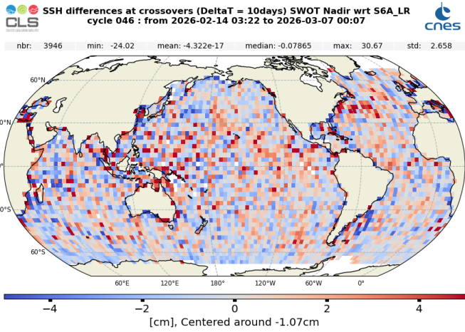
Figure 30: Mean SSH difference at crossovers between SWOT Nadir MLE4 and Sentinel-6 MF LR MLE4 over cycle 046 (left) and from cycle 001 onwards (right)
