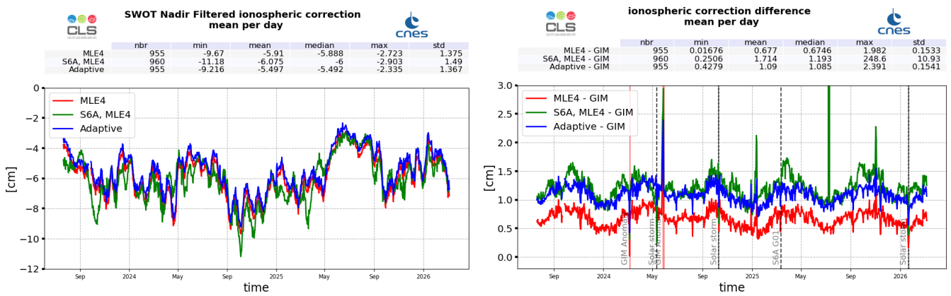
Figure 15: SWOT Nadir MLE4 (red), Adaptive (blue) and Sentinel-6A-MF (LR MLE4) (green) filtered ionosphere correction daily monitoring from cycle 001 to 046 (left) and difference with GIM model (right)
