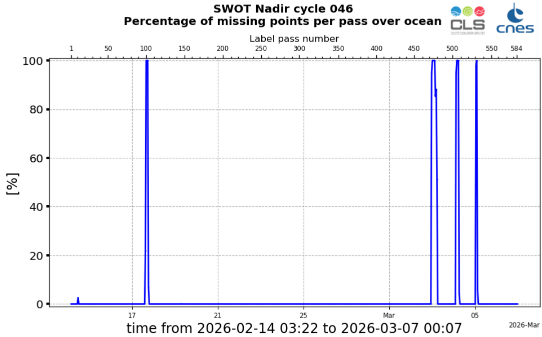
Figure 2: Monitoring of the percentage per pass of missing data over ocean, for SWOT Nadir GDR cycle 046
