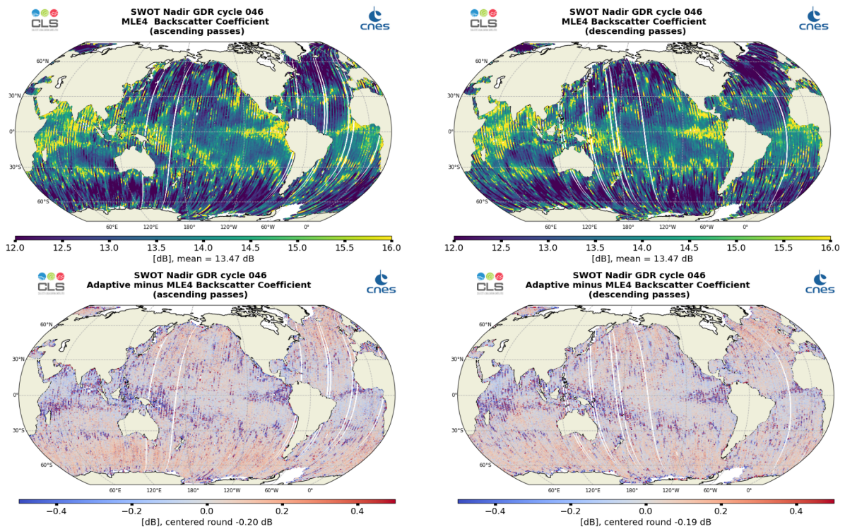
Figure 8: Along-track maps of Ku-band backscatter coefficient \sigma_0 over cycle 046 for SWOT Nadir MLE4 (top) or Adaptive minus MLE4 difference (bottom), ascending passes (left) and descending passes (right)
