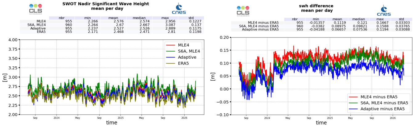
Figure 6: Ku-band Significant Wave Height daily monitoring from cycle 001 to 046, for SWOT Nadir, ERA5 model estimated at SWOT locations, and Sentinel-6A-MF (LR MLE4) (left), and difference with ERA5 model (right)
