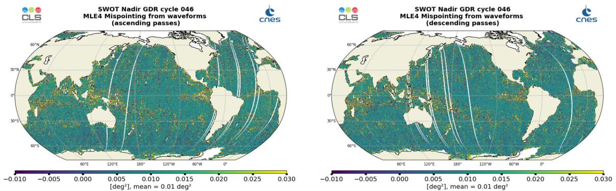
Figure 17: Along-track maps of mispointing over cycle 046 for SWOT Nadir MLE4, ascending passes (left) and descending passes (right)
