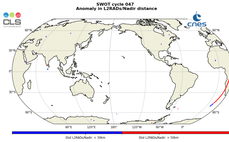
Figure 24: Map of the anomalies detected in the L2RADs/Nadir distance over the cycle 047
