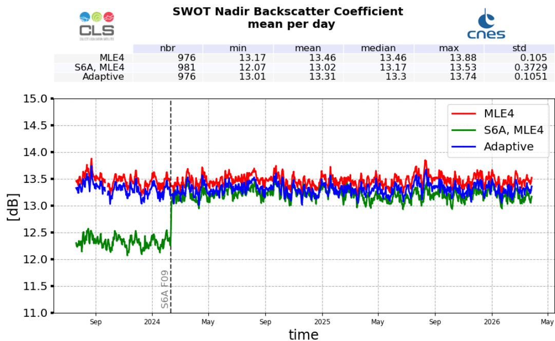
Figure 9: Ku-band Backscattering coefficient daily monitoring from cycle 001 to 047, for SWOT Nadir and Sentinel-6A-MF
