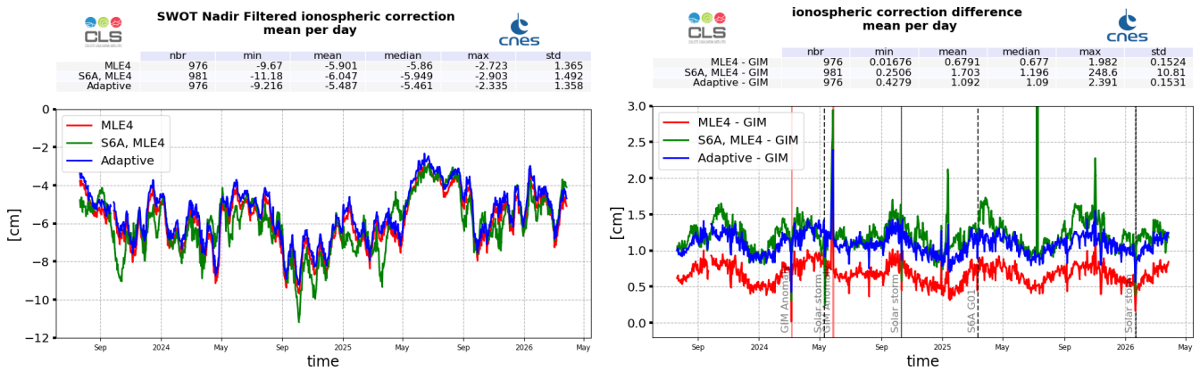
Figure 15: SWOT Nadir MLE4 (red), Adaptive (blue) and Sentinel-6A-MF (LR MLE4) (green) filtered ionosphere correction daily monitoring from cycle 001 to 047 (left) and difference with GIM model (right)
