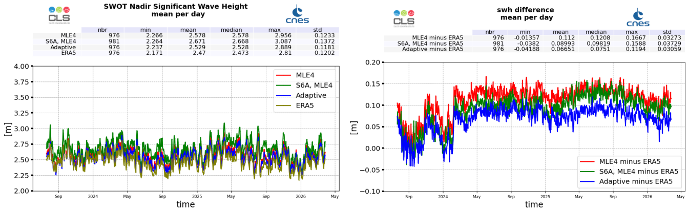
Figure 6: Ku-band Significant Wave Height daily monitoring from cycle 001 to 047, for SWOT Nadir, ERA5 model estimated at SWOT locations, and Sentinel-6A-MF (LR MLE4) (left), and difference with ERA5 model (right)
