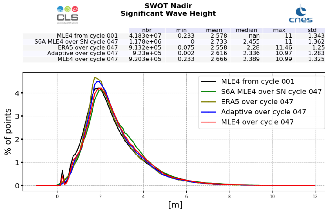
Figure 4: Ku-band Significant Wave Height histogram computed over cycle 047 (red line for SWOT Nadir MLE4 and blue line for SWOT Nadir Adaptive, green for Sentinel-6A-MF (LR MLE4) and dark green for ERA5) and from cycle 001 (SWOT Nadir, MLE4 only, black line)
