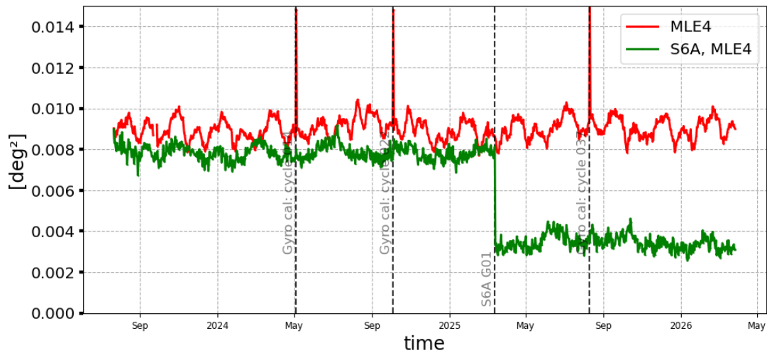
Figure 18: Mispointing daily monitoring from SWOT cycle 001 to 047 for SWOT Nadir GDR (red) and Sentinel-6A-MF (green)
