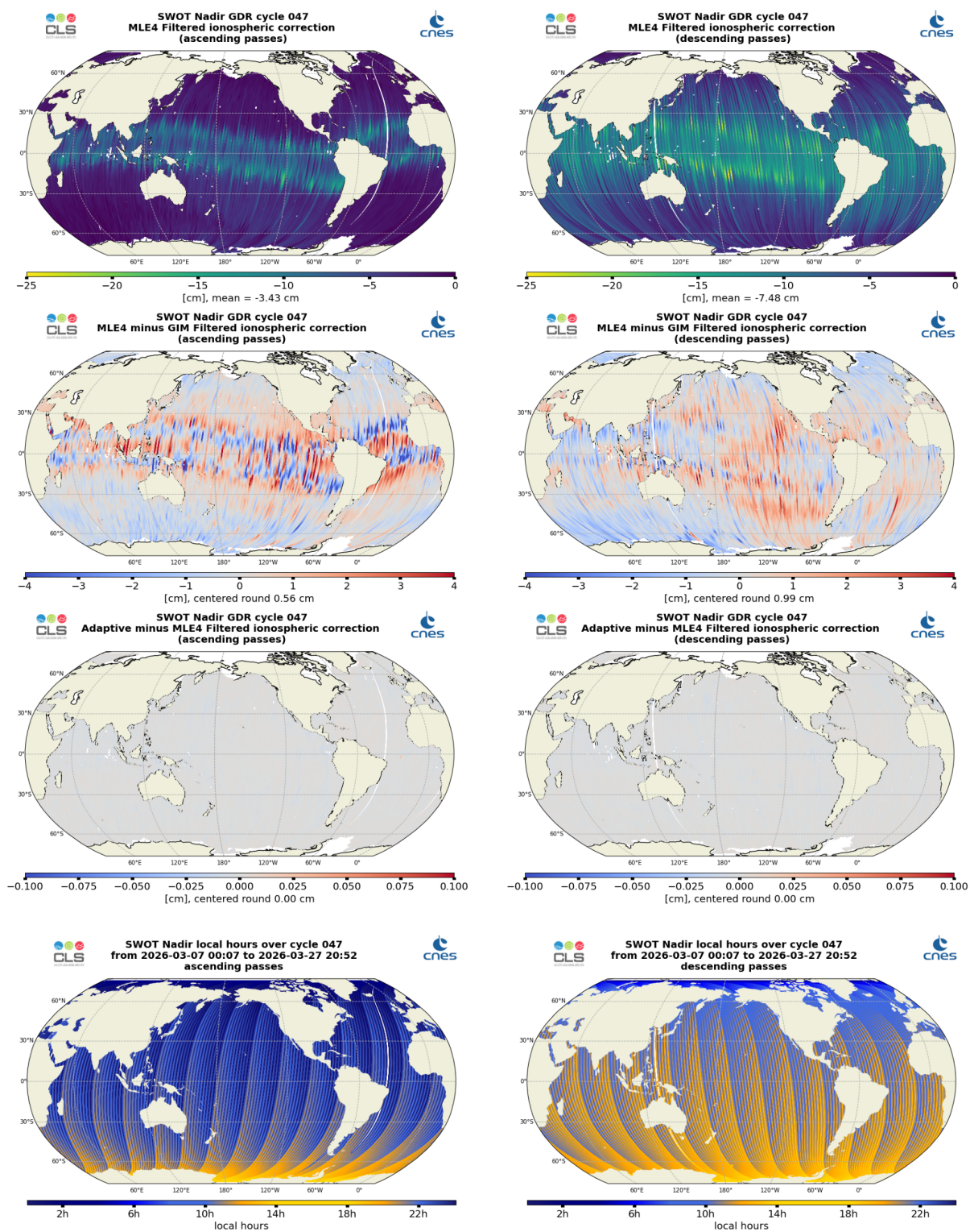
Figure 14: Along-track maps of filtered ionosphere correction over cycle 047 for SWOT Nadir MLE4 (top), MLE4 minus GIM (middle top) or Adaptive minus MLE4 (middle bottom), and local hours (bottom), for ascending passes (left) and descending passes (right)
