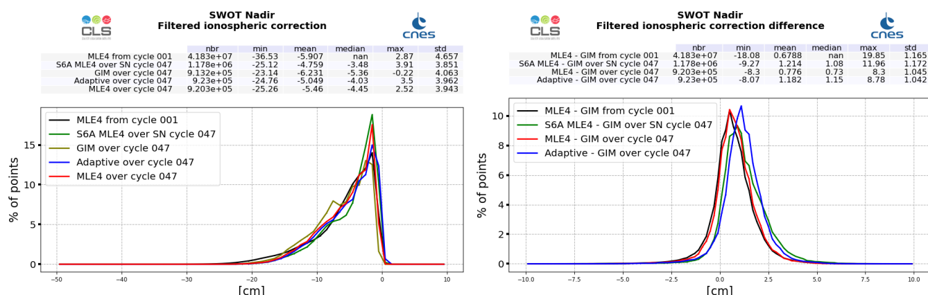
Figure 13: GIM model (dark green) and altimeter filtered ionosphere correction histogram computed over cycle 047 (red line for SWOT Nadir MLE4 and blue line for SWOT Nadir Adaptive, green for Sentinel-6A-MF (LR MLE4)) and from cycle 001 (SWOT Nadir, MLE4 only, black line) (left). Difference between filtered altimeter and GIM model (right).
