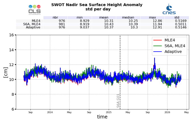
Figure 27: SSHA daily monitoring from cycle 001 to 047, for SWOT Nadir GDR
