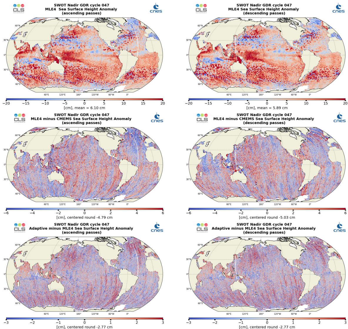
Figure 26: Along-track maps of SSHA over cycle 047 for SWOT Nadir MLE4 (top), MLE4 minus CMEMS (middle) or Adaptive minus MLE4 (bottom), ascending passes (left) and descending passes (right)
