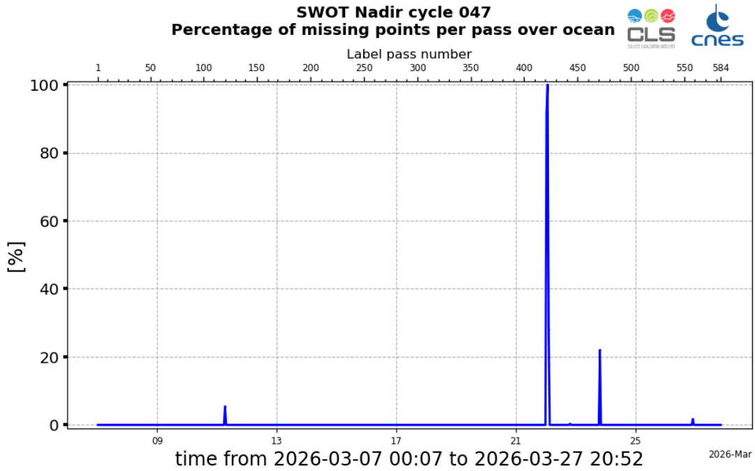
Figure 2: Monitoring of the percentage per pass of missing data over ocean, for SWOT Nadir GDR cycle 047
