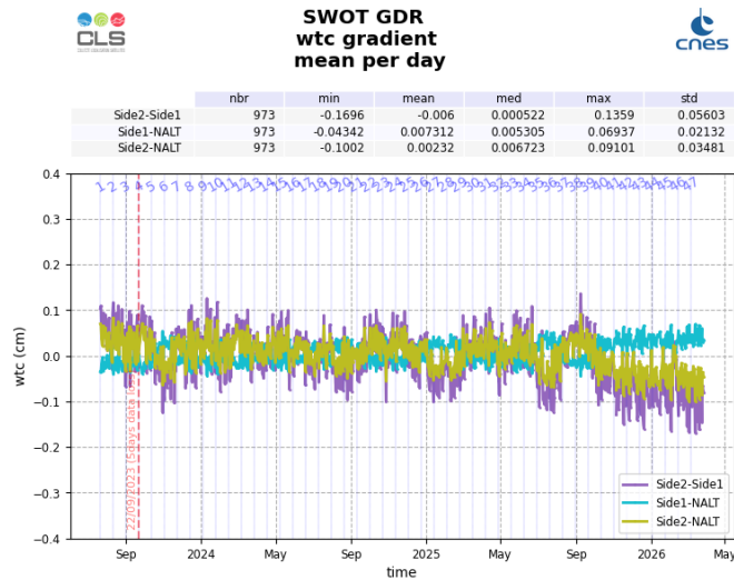
Figure 20: Daily monitoring of the wet tropospheric correction gradient between AMR Side 1 and AMR Side 2 (purple), AMR Side 1 and Nadir (cyan), and AMR Side 2 and Nadir (yellow), from Cycle 001 to 047
