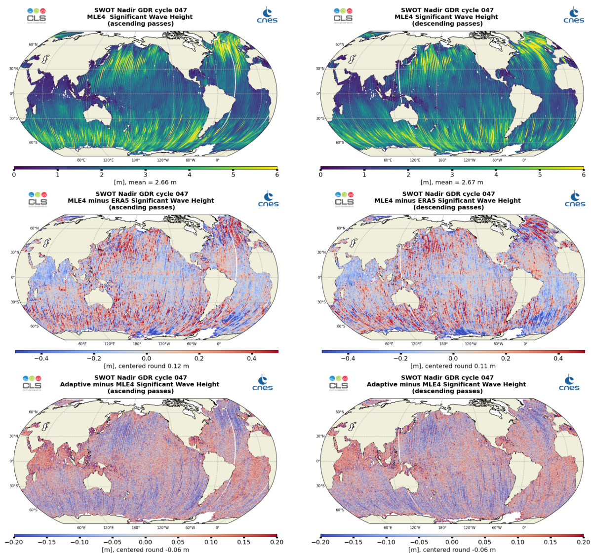
Figure 5: Along-track maps of Ku-band Significant Wave Height over cycle 047 for SWOT Nadir MLE4 (top), MLE4 minus model (middle) or Adaptive minus MLE4 (bottom), ascending passes (left) and descending passes (right)
