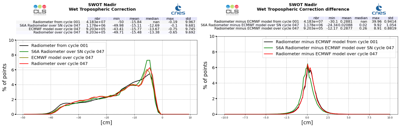
Figure 21: Histogram of wet troposphere corrections : SWOT Nadir radiometer (left) and difference with ECMWF model (right), computed over cycle 047 and from cycle 001 (black line)
