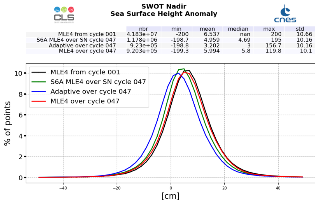
Figure 25: SSHA histogram computed over cycle 047 (red line for SWOT Nadir MLE4 and blue line for SWOT Nadir Adaptive, green for Sentinel-6A-MF (LR MLE4)) and from cycle 001 (SWOT Nadir, MLE4 only, black line)
