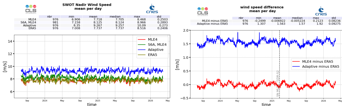
Figure 12: Wind Speed daily monitoring from cycle 001 to 047 for SWOT Nadir GDR, ERA5 model, and Sentinel-6A-MF (LR MLE4) (left), and daily mean difference with ERA5 (right)
