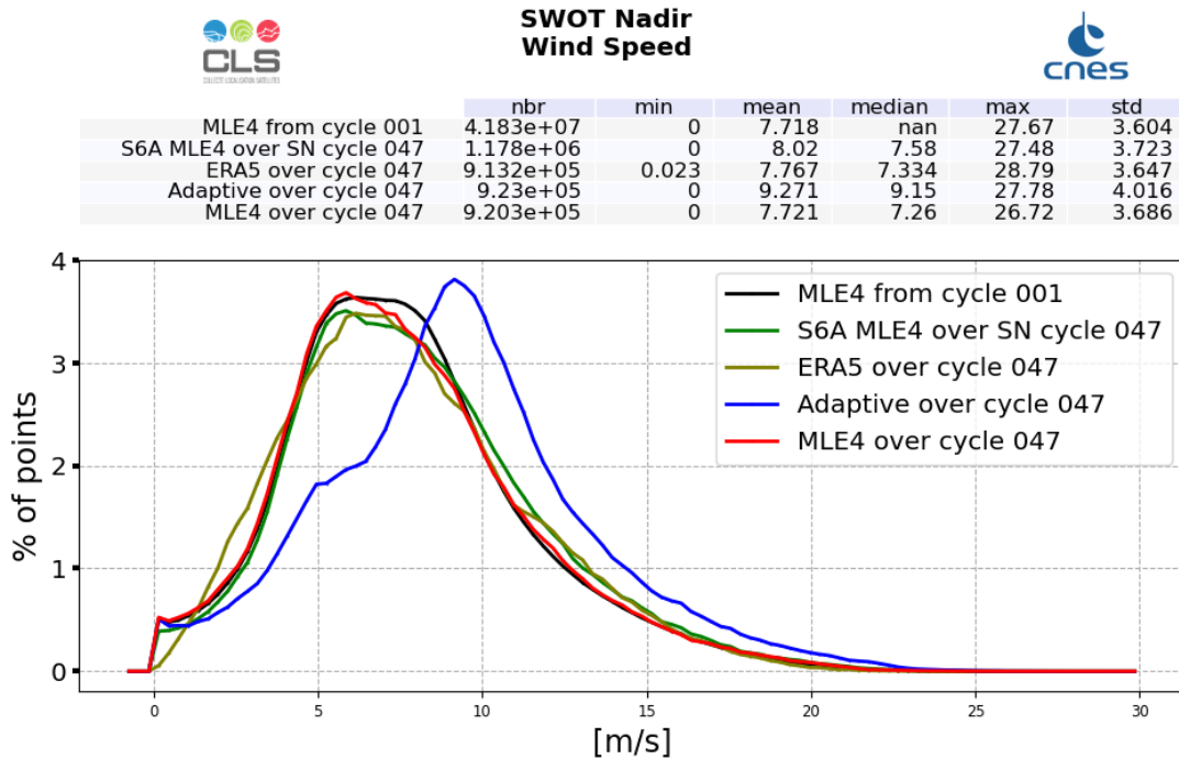
Figure 10: Altimeter Wind Speed histogram computed over cycle 047 (red line for SWOT Nadir MLE4 and blue line for SWOT Nadir Adaptive, green for Sentinel-6A-MF (LR MLE4)) and from cycle 001 (SWOT Nadir, MLE4 only, black line)
