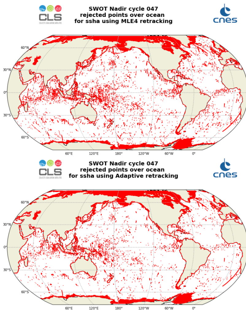
Figure 3: Edited measurements for SWOT Nadir over cycle 047
