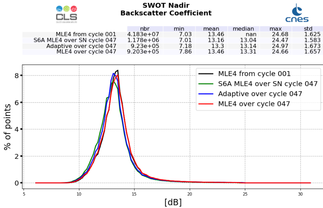
Figure 7: Ku-band Backscattering coefficient histogram computed over cycle 047 (red line for SWOT Nadir MLE4 and blue line for SWOT Nadir Adaptive, green for Sentinel-6A-MF (LR MLE4)) and from cycle 001 (SWOT Nadir, MLE4 only, black line)
