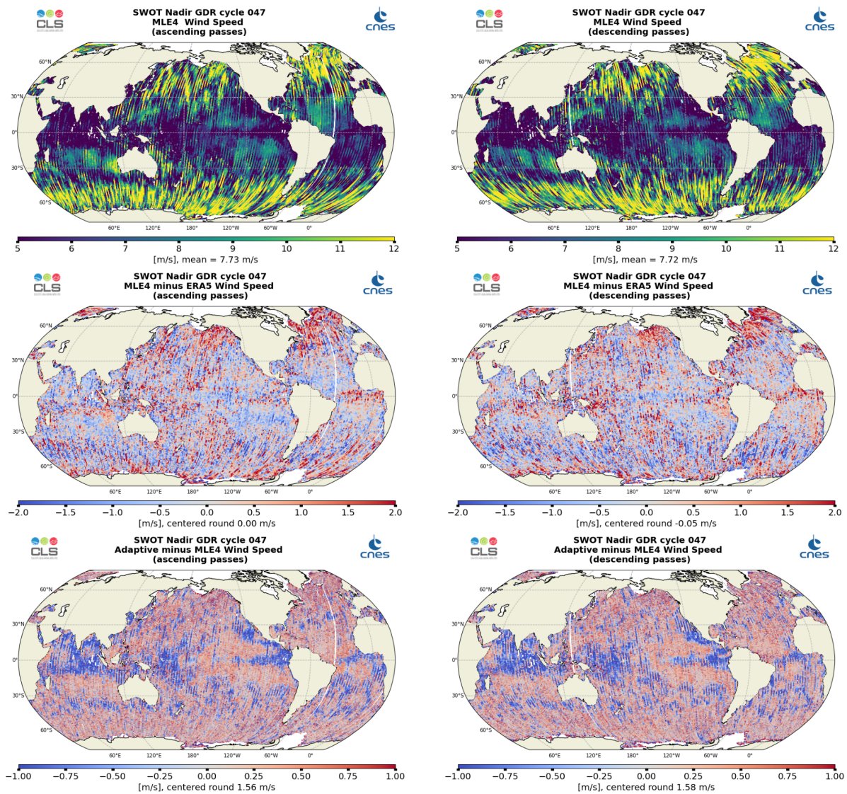
Figure 11: Along-track maps of Altimeter Wind Speed over cycle 047 for SWOT Nadir MLE4 (top), MLE4 minus ERA5 (middle) or Adaptive minus MLE4 (bottom), ascending passes (left) and descending passes (right)
