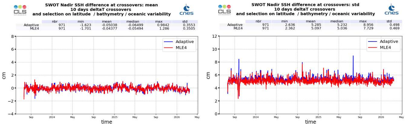
Figure 29: Monitoring of SSH difference at crossovers for SWOT Nadir MLE4 (red) and Adaptive (blue) : mean (left) and standard deviation (right), from cycle 001 to 047
