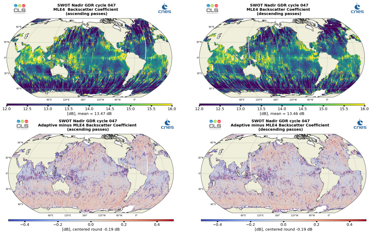
Figure 8: Along-track maps of Ku-band backscatter coefficient \sigma_0 over cycle 047 for SWOT Nadir MLE4 (top) or Adaptive minus MLE4 difference (bottom), ascending passes (left) and descending passes (right)
