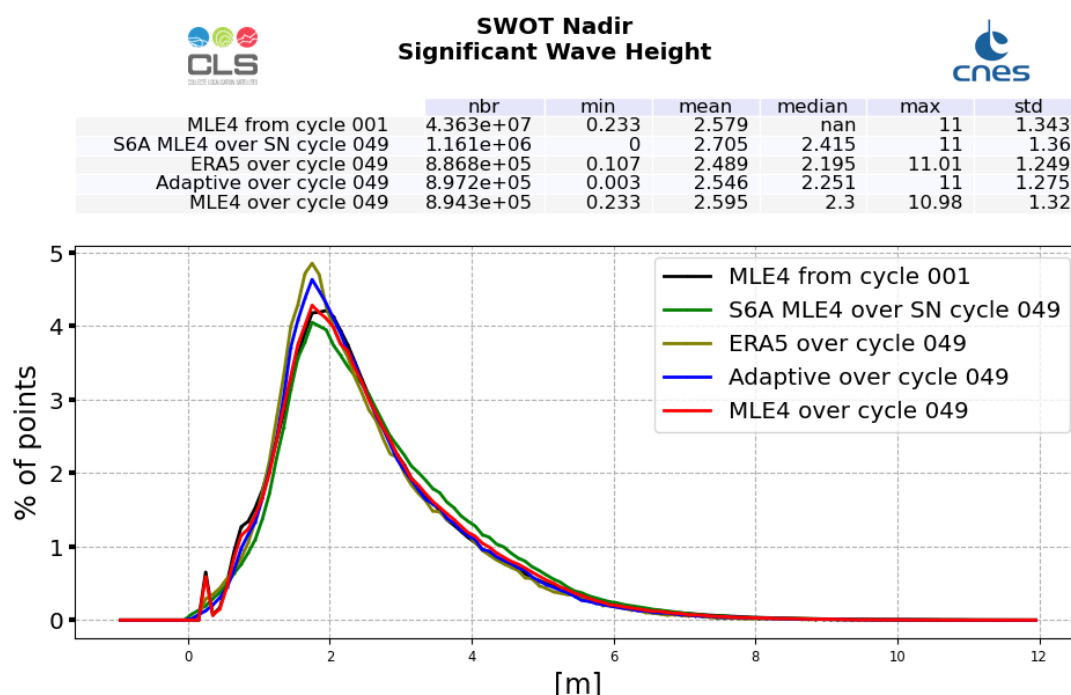
Figure 4: Ku-band Significant Wave Height histogram computed over cycle 049 (red line for SWOT Nadir MLE4 and blue line for SWOT Nadir Adaptive, green for Sentinel-6A-MF (LR MLE4) and dark green for ERA5) and from cycle 001 (SWOT Nadir, MLE4 only, black line)
