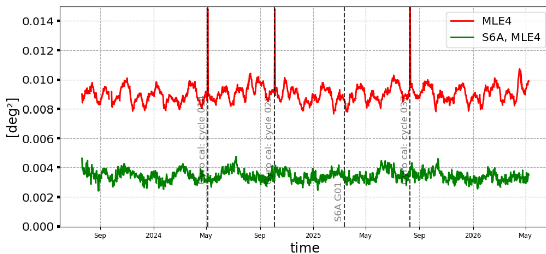
Figure 18: Mispointing daily monitoring from SWOT cycle 001 to 049 for SWOT Nadir GDR (red) and Sentinel-6A-MF (green)
