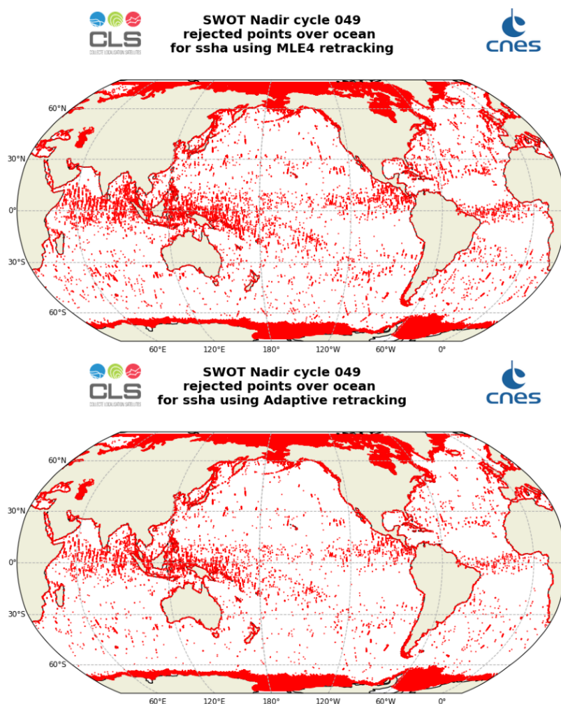
Figure 3: Edited measurements for SWOT Nadir over cycle 049
