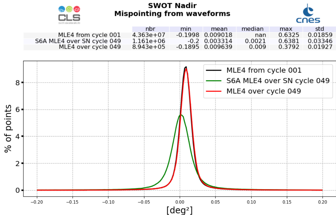
Figure 16: Mispointing histogram computed over cycle 049 (solid line) and from cycle 4 (dashed line)
