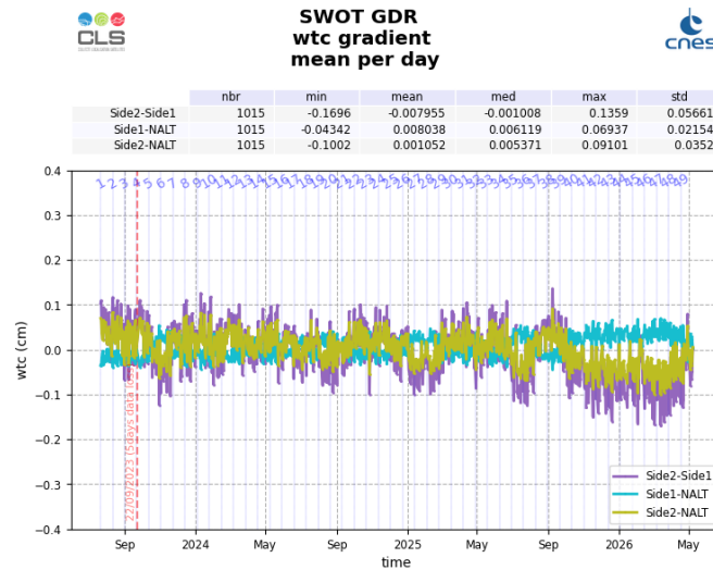
Figure 20: Daily monitoring of the wet tropospheric correction gradient between AMR Side 1 and AMR Side 2 (purple), AMR Side 1 and Nadir (cyan), and AMR Side 2 and Nadir (yellow), from Cycle 001 to 049
