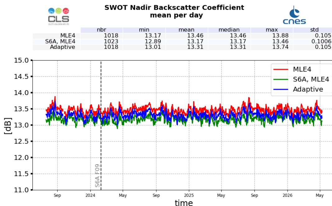
Figure 9: Ku-band Backscattering coefficient daily monitoring from cycle 001 to 049, for SWOT Nadir and Sentinel-6A-MF
