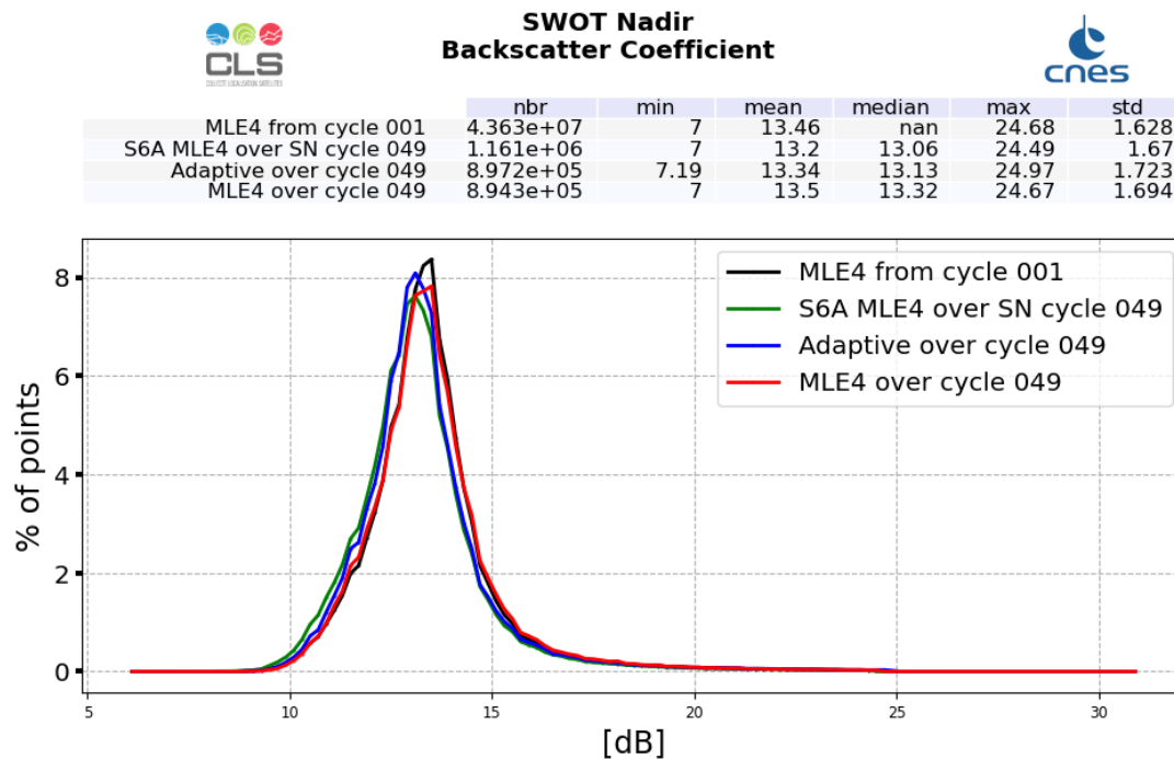
Figure 7: Ku-band Backscattering coefficient histogram computed over cycle 049 (red line for SWOT Nadir MLE4 and blue line for SWOT Nadir Adaptive, green for Sentinel-6A-MF (LR MLE4)) and from cycle 001 (SWOT Nadir, MLE4 only, black line)
