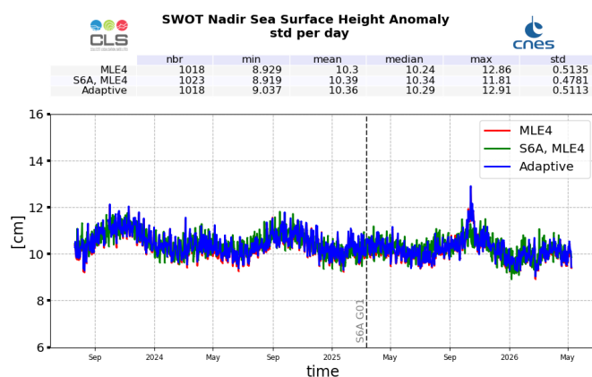
Figure 27: SSHA daily monitoring from cycle 001 to 049, for SWOT Nadir GDR
