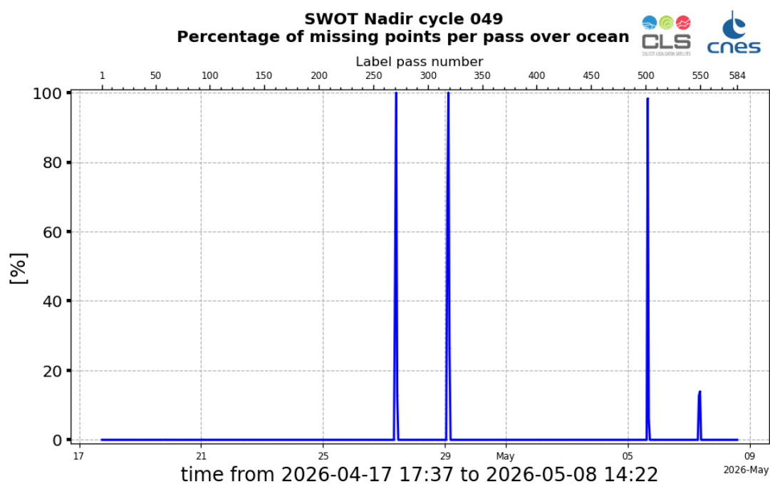
Figure 2: Monitoring of the percentage per pass of missing data over ocean, for SWOT Nadir GDR cycle 049
