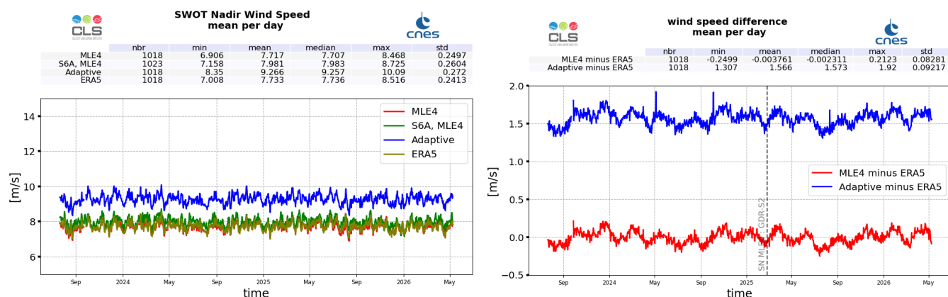
Figure 12: Wind Speed daily monitoring from cycle 001 to 049 for SWOT Nadir GDR, ERA5 model, and Sentinel-6A-MF (LR MLE4) (left), and daily mean difference with ERA5 (right)
