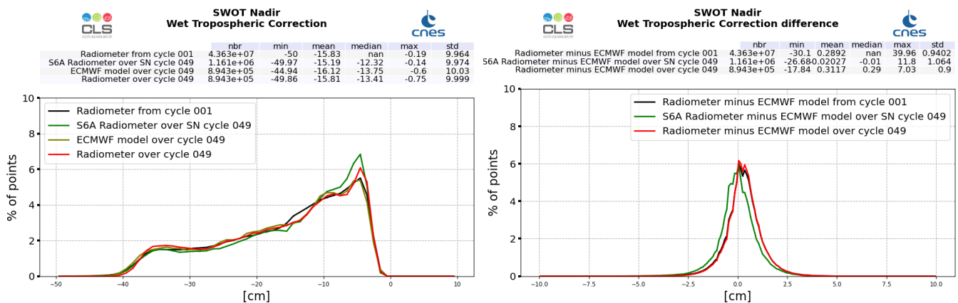
Figure 21: Histogram of wet troposphere corrections : SWOT Nadir radiometer (left) and difference with ECMWF model (right), computed over cycle 049 and from cycle 001 (black line)
