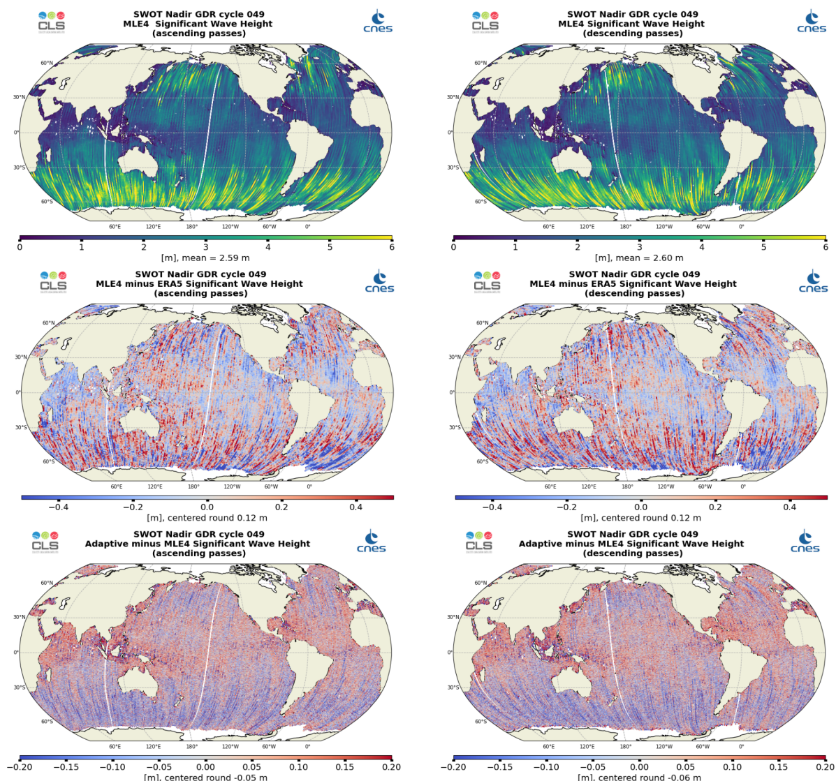
Figure 5: Along-track maps of Ku-band Significant Wave Height over cycle 049 for SWOT Nadir MLE4 (top), MLE4 minus model (middle) or Adaptive minus MLE4 (bottom), ascending passes (left) and descending passes (right)
