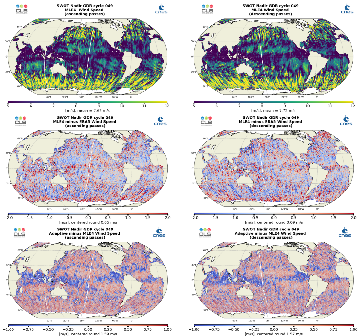
Figure 11: Along-track maps of Altimeter Wind Speed over cycle 049 for SWOT Nadir MLE4 (top), MLE4 minus ERA5 (middle) or Adaptive minus MLE4 (bottom), ascending passes (left) and descending passes (right)
