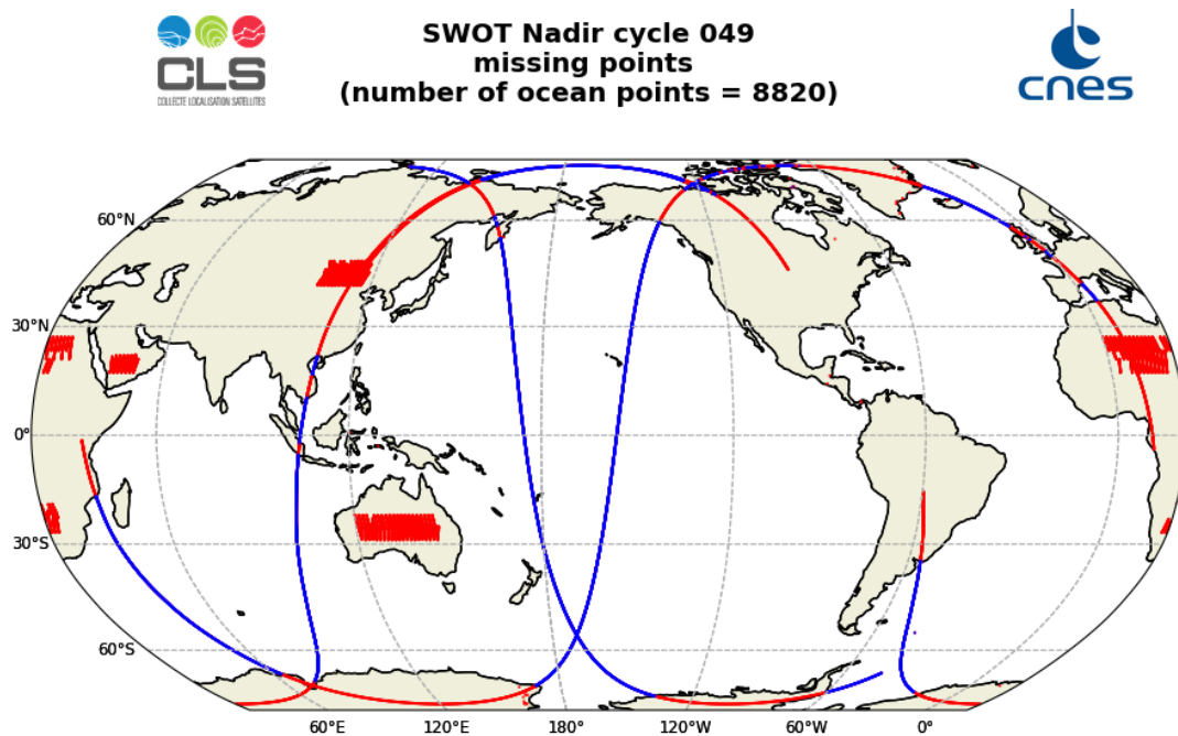
Figure 1: Map of missing measurements for SWOT Nadir GDR cycle 049
