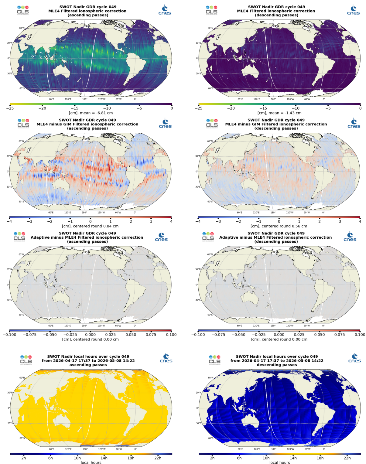
Figure 14: Along-track maps of filtered ionosphere correction over cycle 049 for SWOT Nadir MLE4 (top), MLE4 minus GIM (middle top) or Adaptive minus MLE4 (middle bottom), and local hours (bottom), for ascending passes (left) and descending passes (right)
