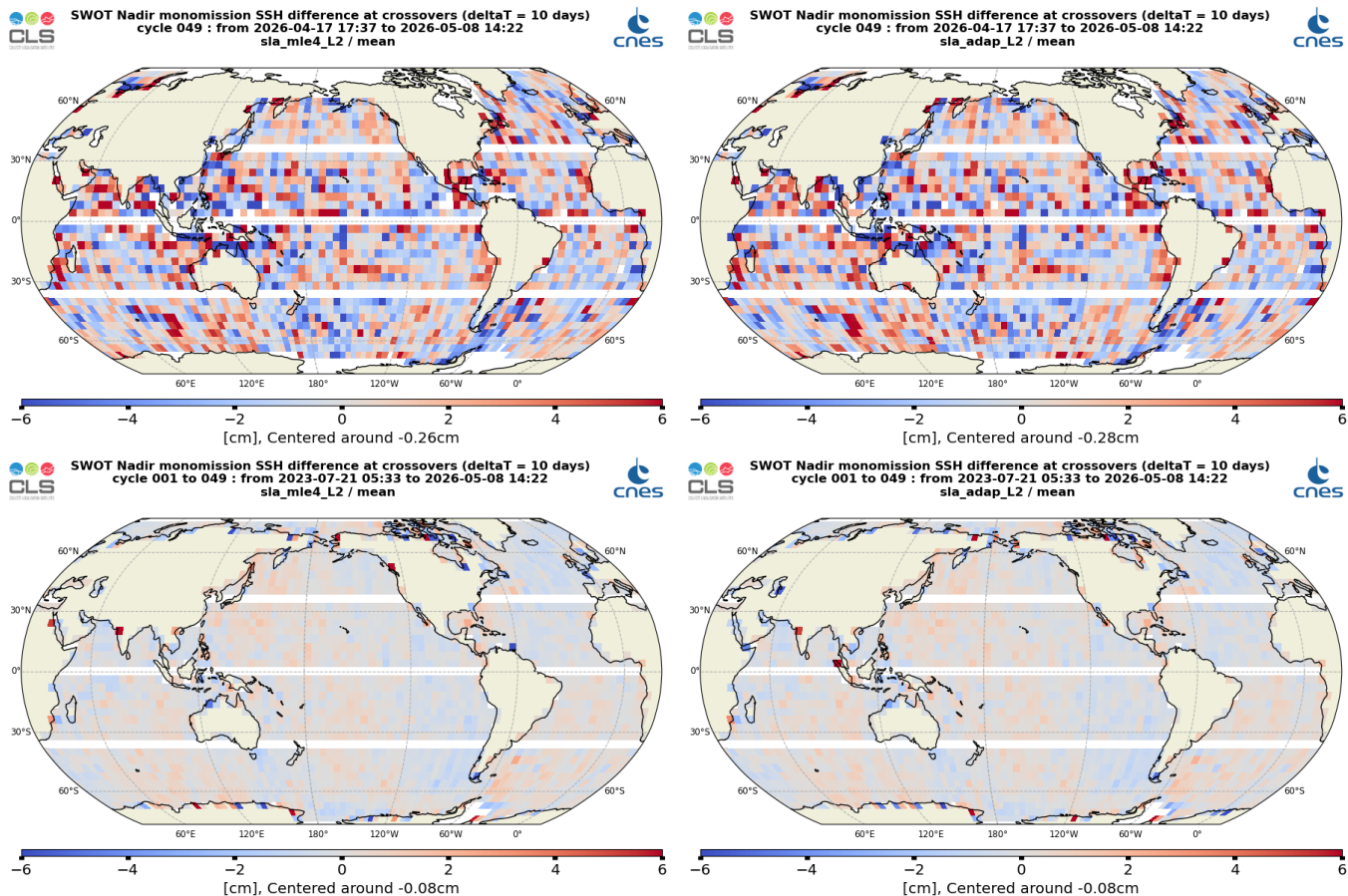
Figure 28: Mean SSH difference at crossovers for SWOT Nadir MLE4 (left) and Adaptive (right) cycle 049(top) and from cycle 001 to cycle 049 (bottom)
