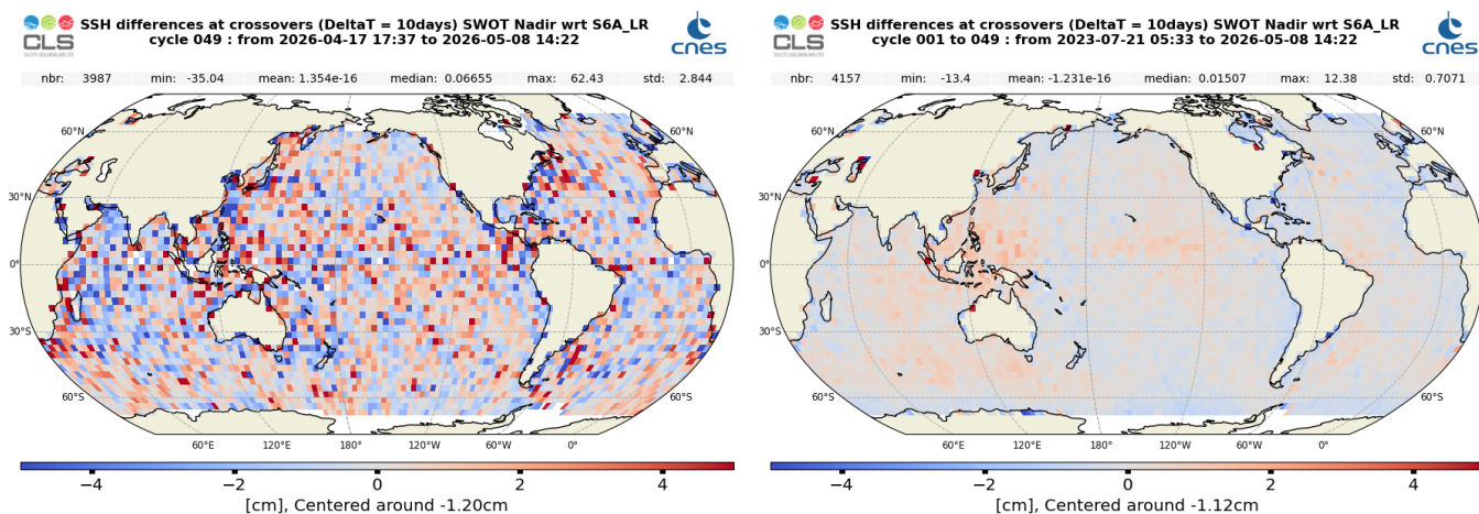
Figure 30: Mean SSH difference at crossovers between SWOT Nadir MLE4 and Sentinel-6 MF LR MLE4 over cycle 049 (left) and from cycle 001 onwards (right)
