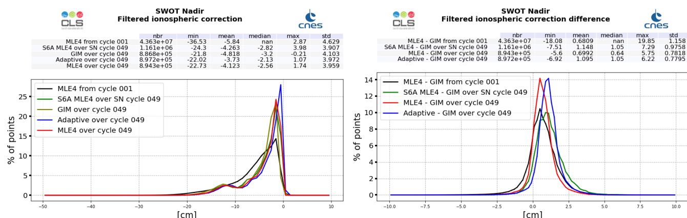
Figure 13: GIM model (dark green) and altimeter filtered ionosphere correction histogram computed over cycle 049 (red line for SWOT Nadir MLE4 and blue line for SWOT Nadir Adaptive, green for Sentinel-6A-MF (LR MLE4)) and from cycle 001 (SWOT Nadir, MLE4 only, black line) (left). Difference between filtered altimeter and GIM model (right).
