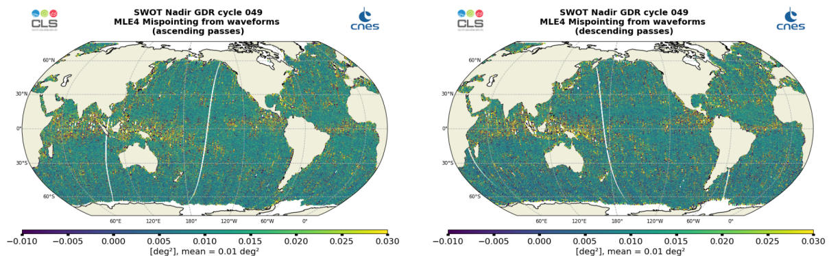
Figure 17: Along-track maps of mispointing over cycle 049 for SWOT Nadir MLE4, ascending passes (left) and descending passes (right)
