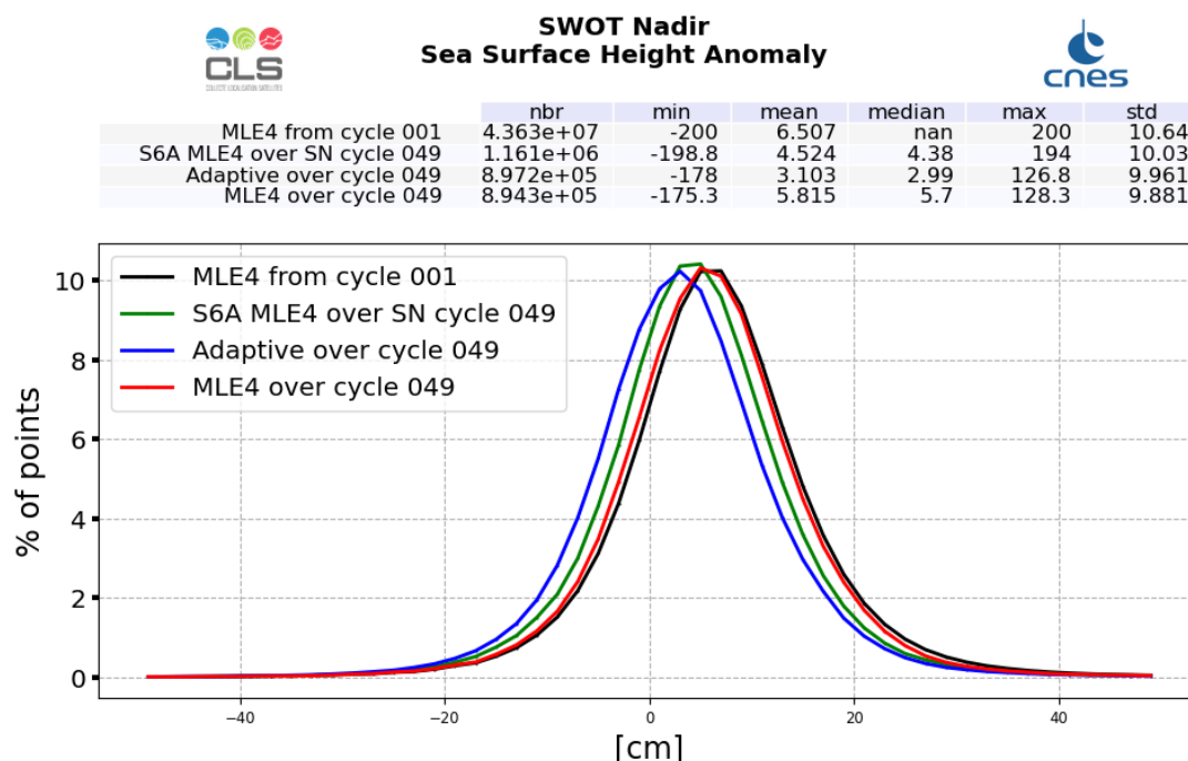
Figure 25: SSHA histogram computed over cycle 049 (red line for SWOT Nadir MLE4 and blue line for SWOT Nadir Adaptive, green for Sentinel-6A-MF (LR MLE4)) and from cycle 001 (SWOT Nadir, MLE4 only, black line)
