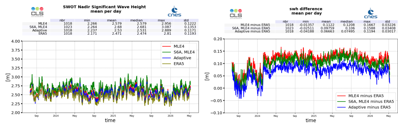
Figure 6: Ku-band Significant Wave Height daily monitoring from cycle 001 to 049, for SWOT Nadir, ERA5 model estimated at SWOT locations, and Sentinel-6A-MF (LR MLE4) (left), and difference with ERA5 model (right)
