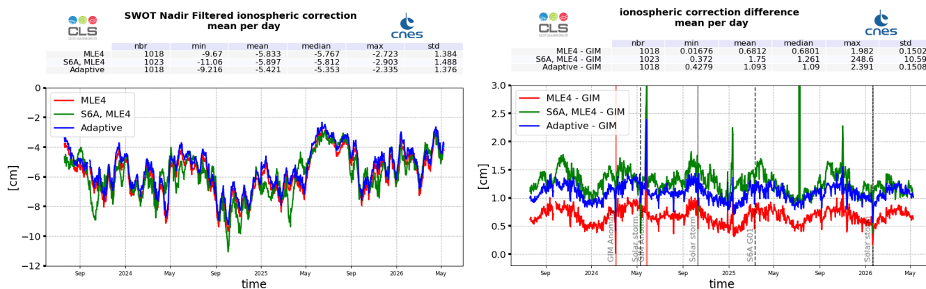
Figure 15: SWOT Nadir MLE4 (red), Adaptive (blue) and Sentinel-6A-MF (LR MLE4) (green) filtered ionosphere correction daily monitoring from cycle 001 to 049 (left) and difference with GIM model (right)
