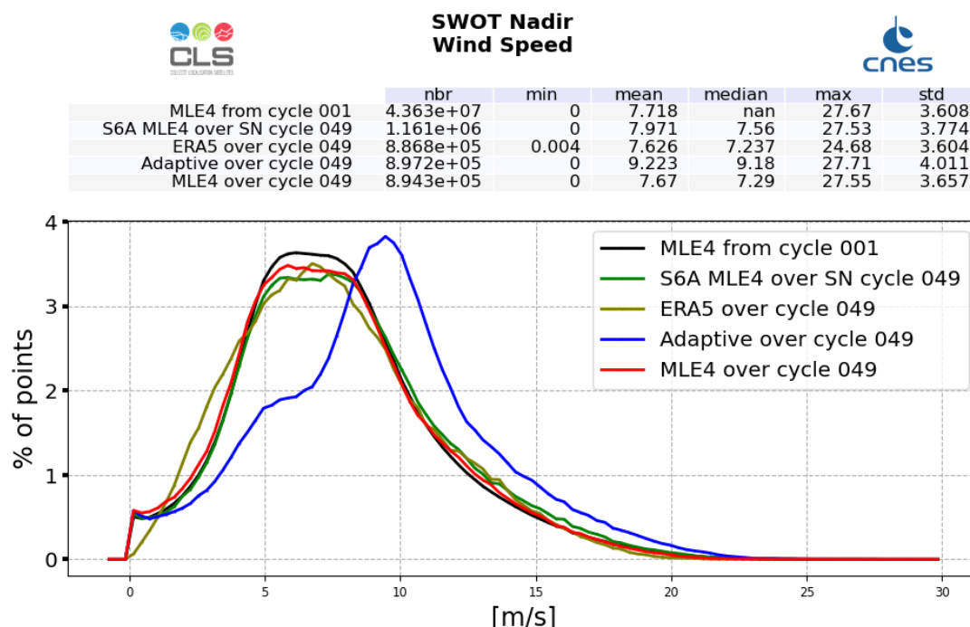
Figure 10: Altimeter Wind Speed histogram computed over cycle 049 (red line for SWOT Nadir MLE4 and blue line for SWOT Nadir Adaptive, green for Sentinel-6A-MF (LR MLE4)) and from cycle 001 (SWOT Nadir, MLE4 only, black line)
