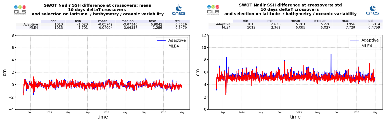
Figure 29: Monitoring of SSH difference at crossovers for SWOT Nadir MLE4 (red) and Adaptive (blue) : mean (left) and standard deviation (right), from cycle 001 to 049
