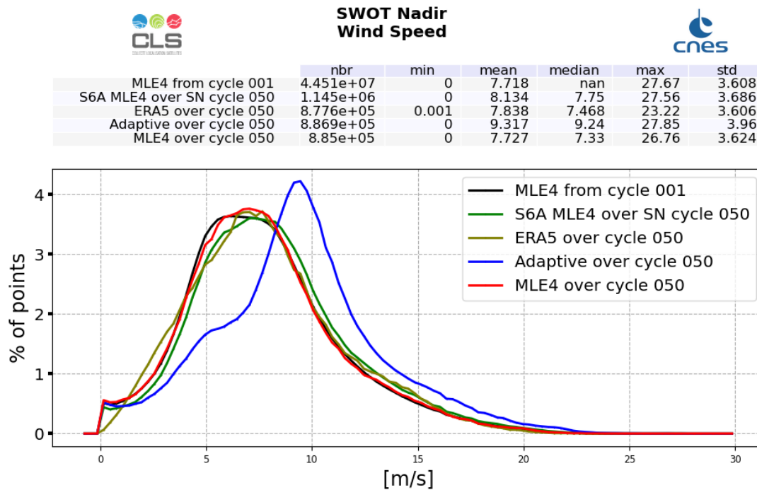
Figure 10: Altimeter Wind Speed histogram computed over cycle 050 (red line for SWOT Nadir MLE4 and blue line for SWOT Nadir Adaptive, green for Sentinel-6A-MF (LR MLE4)) and from cycle 001 (SWOT Nadir, MLE4 only, black line)
