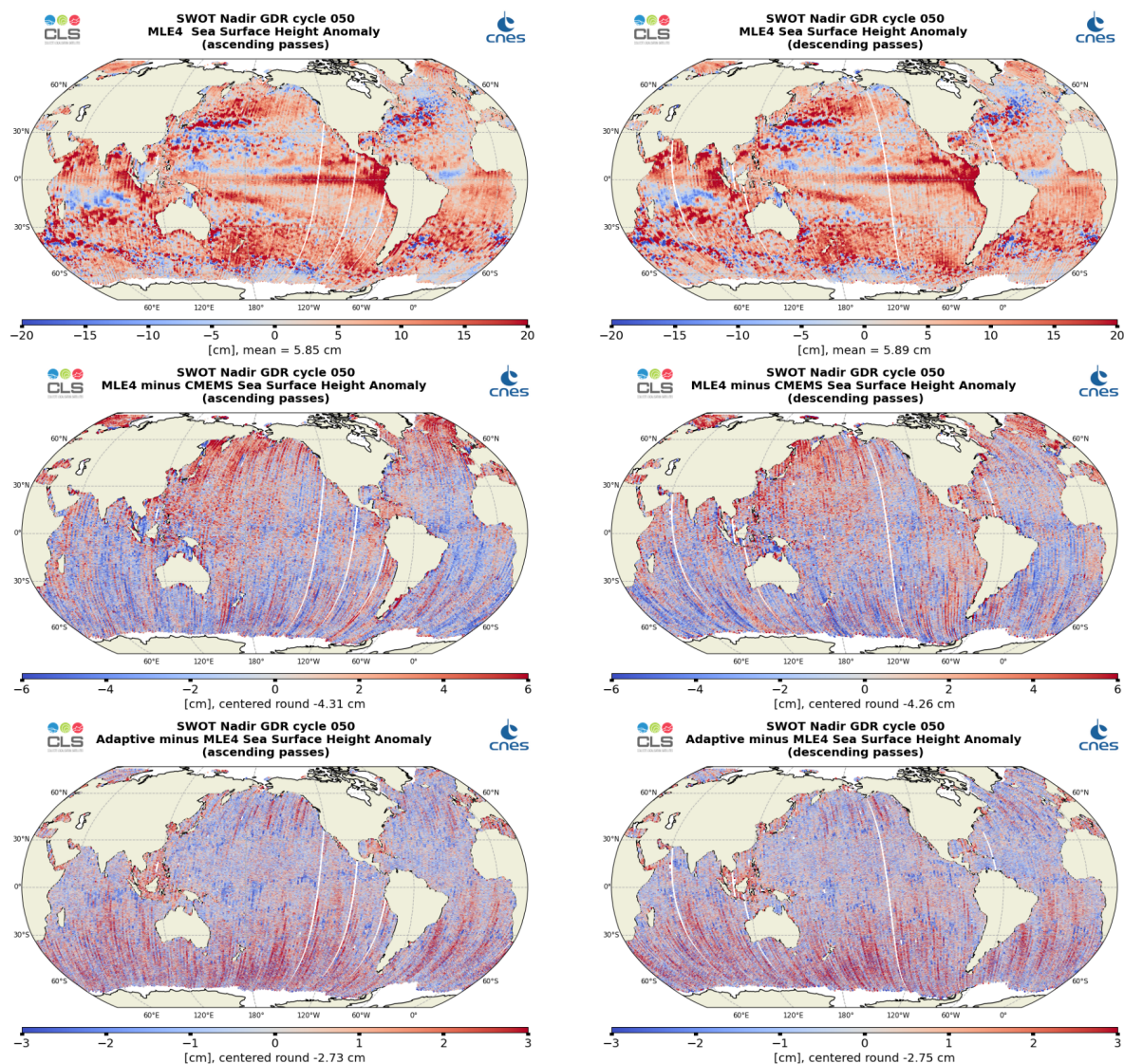
Figure 26: Along-track maps of SSHA over cycle 050 for SWOT Nadir MLE4 (top), MLE4 minus CMEMS (middle) or Adaptive minus MLE4 (bottom), ascending passes (left) and descending passes (right)
