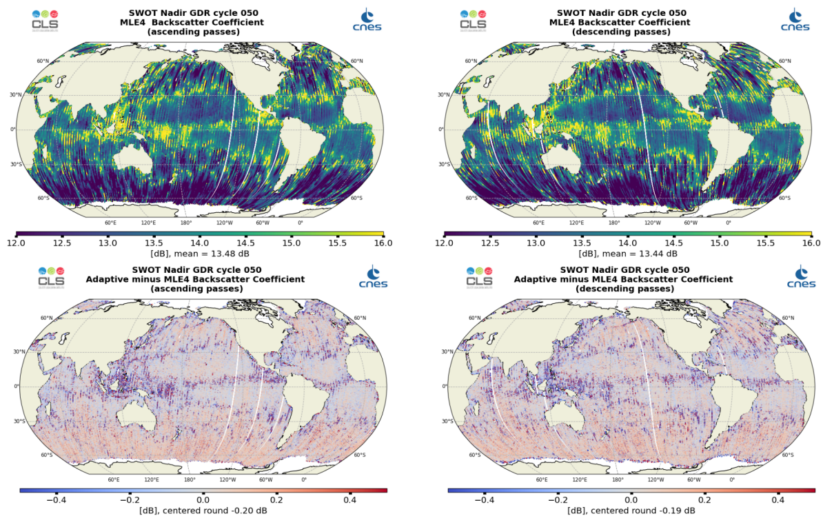
Figure 8: Along-track maps of Ku-band backscatter coefficient \sigma_0 over cycle 050 for SWOT Nadir MLE4 (top) or Adaptive minus MLE4 difference (bottom), ascending passes (left) and descending passes (right)
