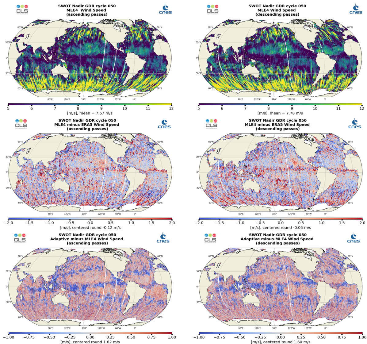
Figure 11: Along-track maps of Altimeter Wind Speed over cycle 050 for SWOT Nadir MLE4 (top), MLE4 minus ERA5 (middle) or Adaptive minus MLE4 (bottom), ascending passes (left) and descending passes (right)
