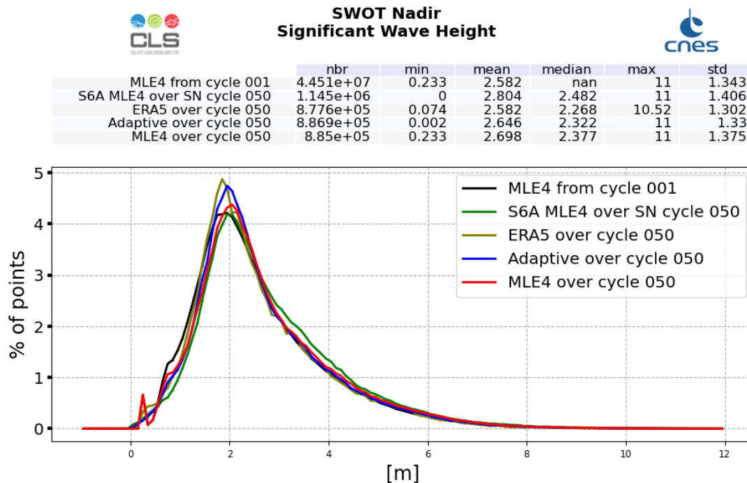
Figure 4: Ku-band Significant Wave Height histogram computed over cycle 050 (red line for SWOT Nadir MLE4 and blue line for SWOT Nadir Adaptive, green for Sentinel-6A-MF (LR MLE4) and dark green for ERA5) and from cycle 001 (SWOT Nadir, MLE4 only, black line)
