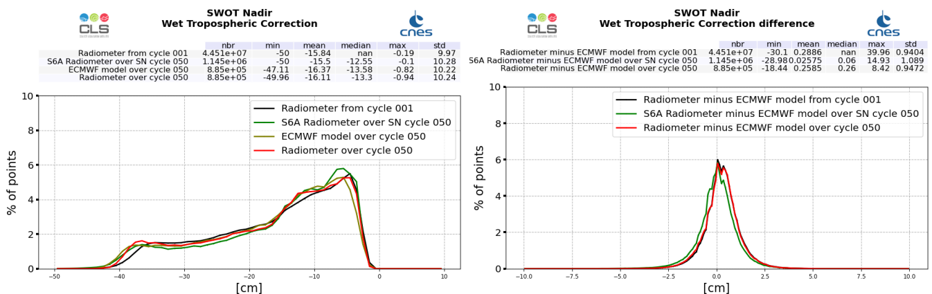
Figure 21: Histogram of wet troposphere corrections : SWOT Nadir radiometer (left) and difference with ECMWF model (right), computed over cycle 050 and from cycle 001 (black line)
