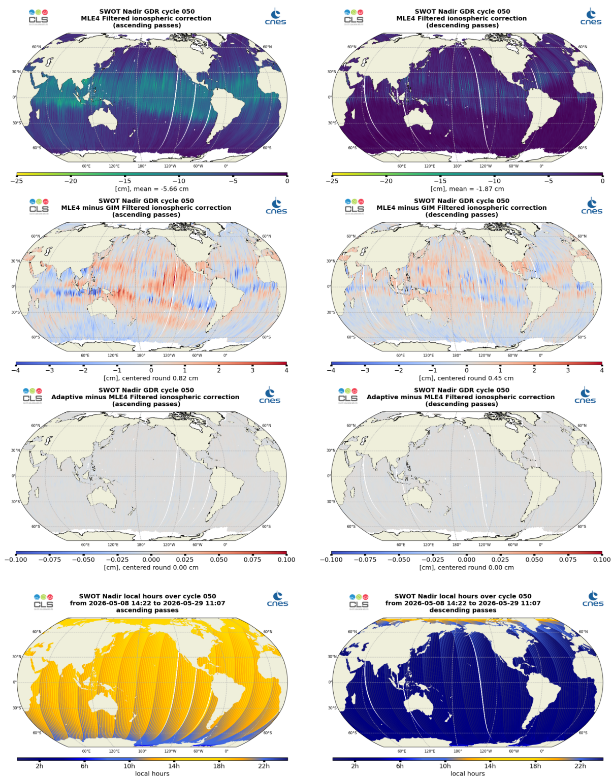
Figure 14: Along-track maps of filtered ionosphere correction over cycle 050 for SWOT Nadir MLE4 (top), MLE4 minus GIM (middle top) or Adaptive minus MLE4 (middle bottom), and local hours (bottom), for ascending passes (left) and descending passes (right)
