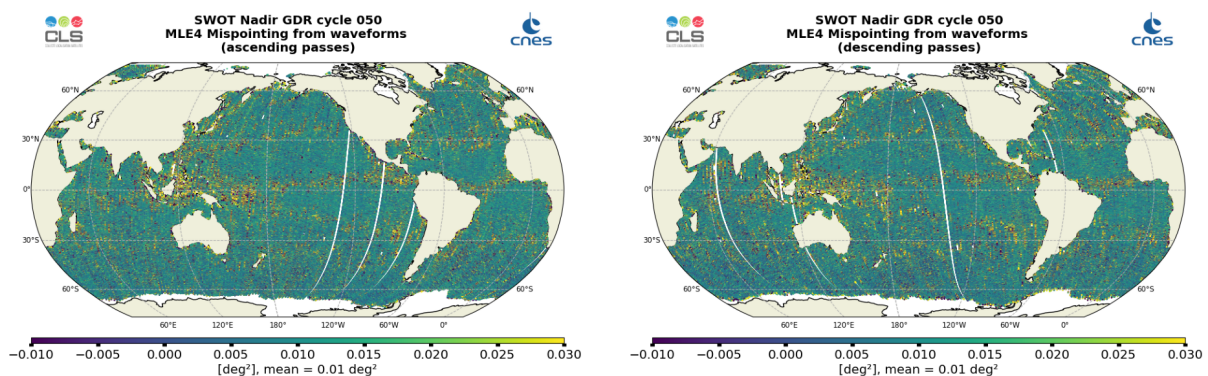
Figure 17: Along-track maps of mispointing over cycle 050 for SWOT Nadir MLE4, ascending passes (left) and descending passes (right)
