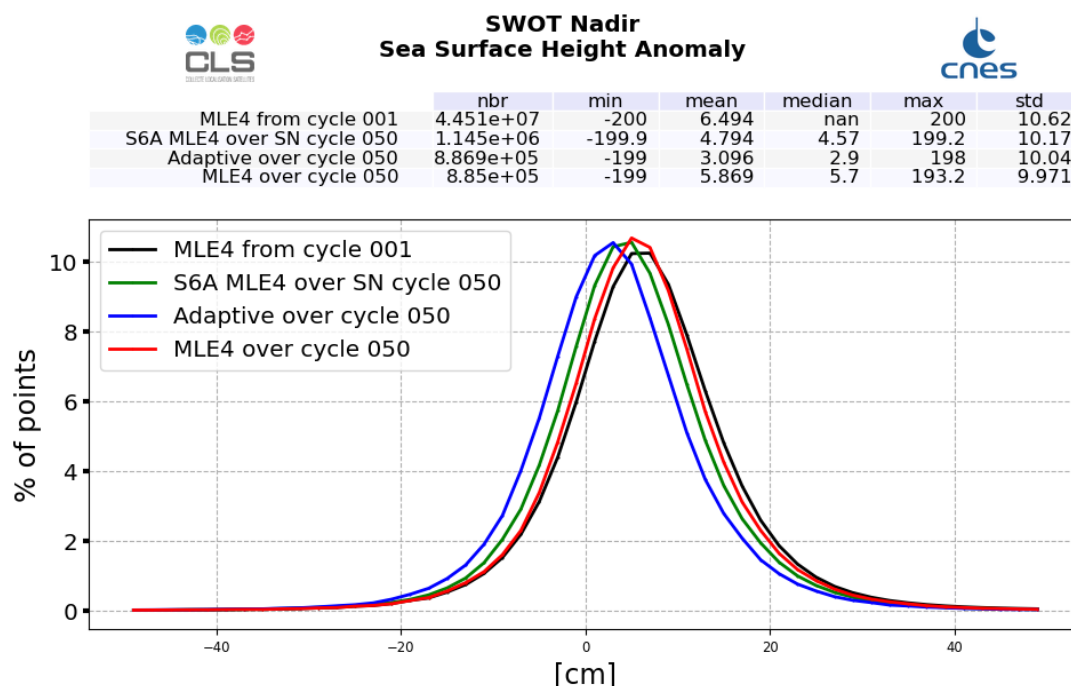
Figure 25: SSHA histogram computed over cycle 050 (red line for SWOT Nadir MLE4 and blue line for SWOT Nadir Adaptive, green for Sentinel-6A-MF (LR MLE4)) and from cycle 001 (SWOT Nadir, MLE4 only, black line)
