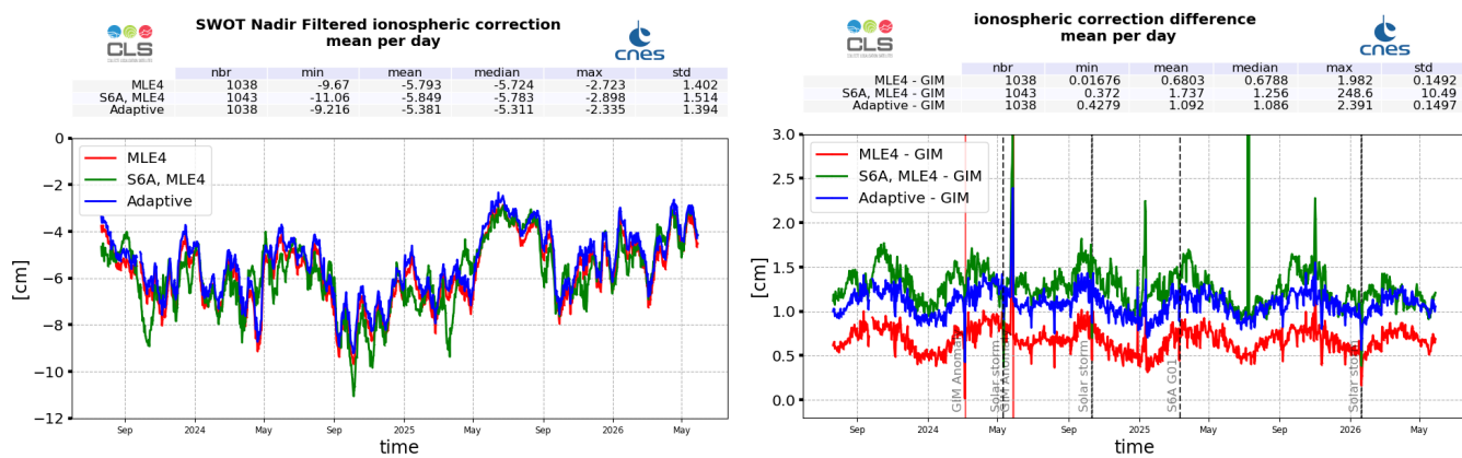
Figure 15: SWOT Nadir MLE4 (red), Adaptive (blue) and Sentinel-6A-MF (LR MLE4) (green) filtered ionosphere correction daily monitoring from cycle 001 to 050 (left) and difference with GIM model (right)
