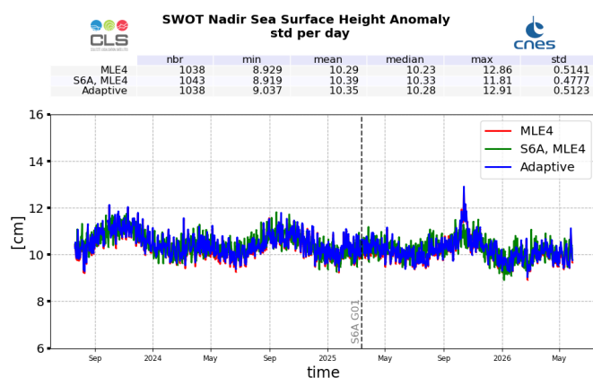
Figure 27: SSHA daily monitoring from cycle 001 to 050, for SWOT Nadir GDR
