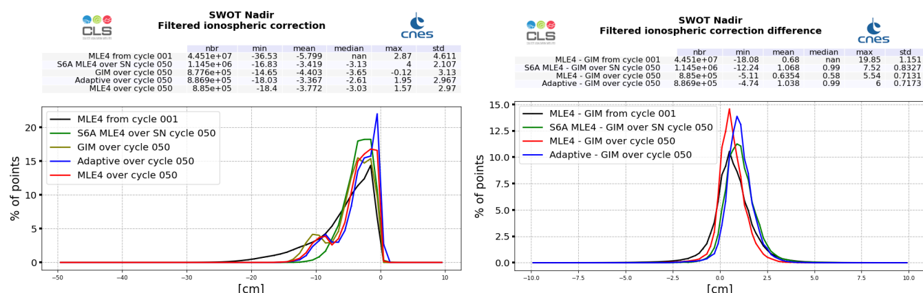
Figure 13: GIM model (dark green) and altimeter filtered ionosphere correction histogram computed over cycle 050 (red line for SWOT Nadir MLE4 and blue line for SWOT Nadir Adaptive, green for Sentinel-6A-MF (LR MLE4)) and from cycle 001 (SWOT Nadir, MLE4 only, black line) (left). Difference between filtered altimeter and GIM model (right).
