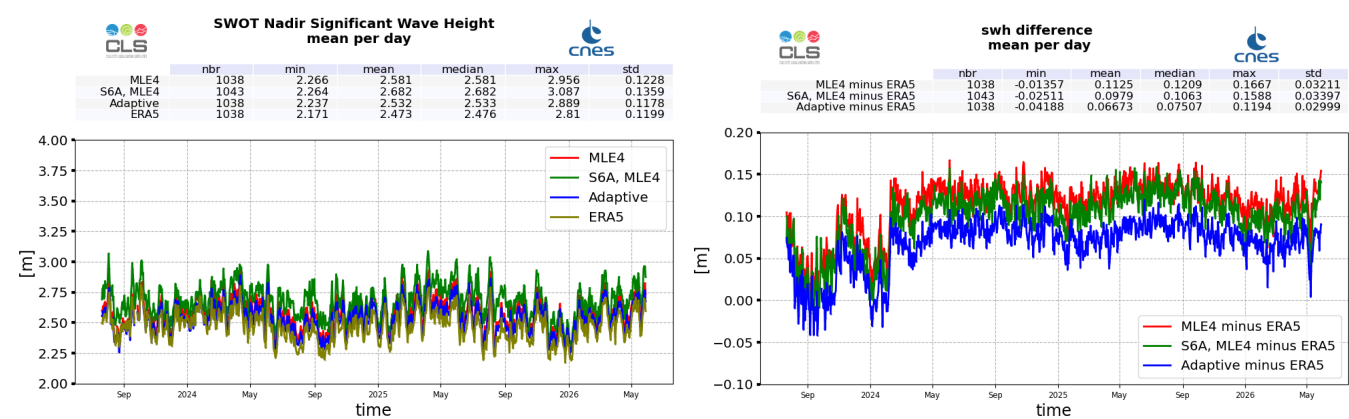
Figure 6: Ku-band Significant Wave Height daily monitoring from cycle 001 to 050, for SWOT Nadir, ERA5 model estimated at SWOT locations, and Sentinel-6A-MF (LR MLE4) (left), and difference with ERA5 model (right)
