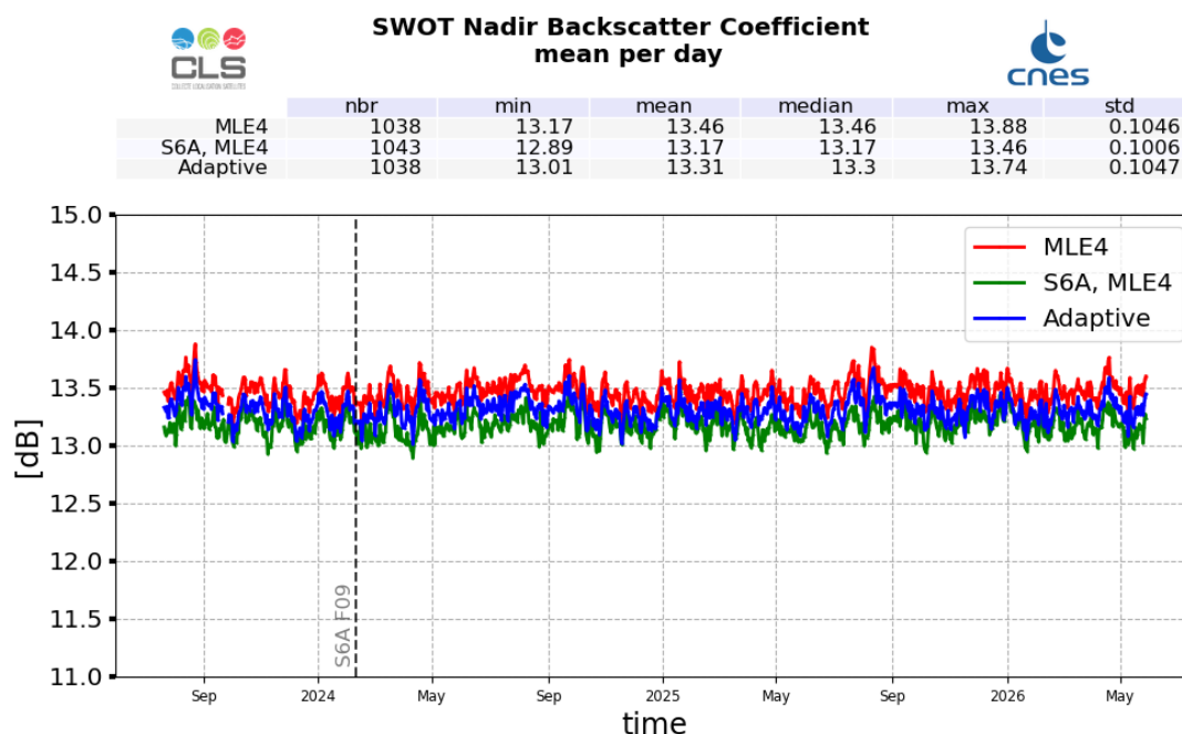
Figure 9: Ku-band Backscattering coefficient daily monitoring from cycle 001 to 050, for SWOT Nadir and Sentinel-6A-MF
