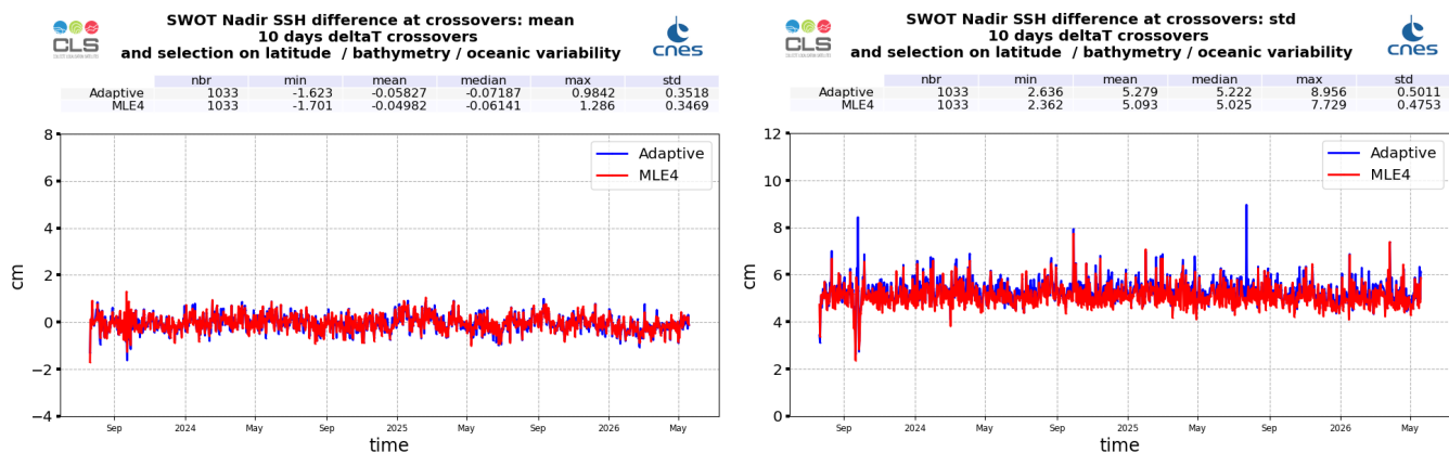
Figure 29: Monitoring of SSH difference at crossovers for SWOT Nadir MLE4 (red) and Adaptive (blue) : mean (left) and standard deviation (right), from cycle 001 to 050
