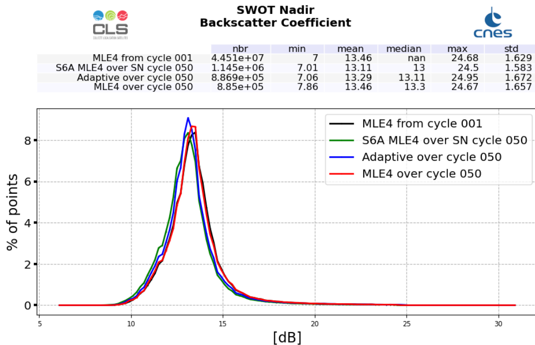
Figure 7: Ku-band Backscattering coefficient histogram computed over cycle 050 (red line for SWOT Nadir MLE4 and blue line for SWOT Nadir Adaptive, green for Sentinel-6A-MF (LR MLE4)) and from cycle 001 (SWOT Nadir, MLE4 only, black line)
