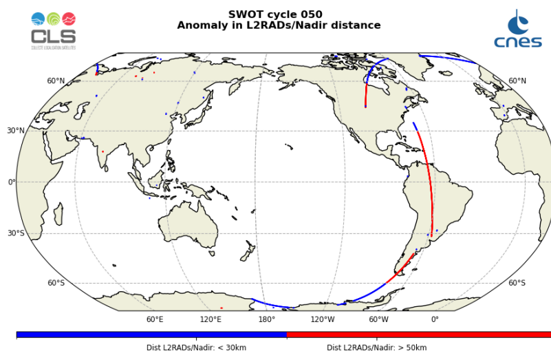
Figure 24: Map of the anomalies detected in the L2RADs/Nadir distance over the cycle 050
