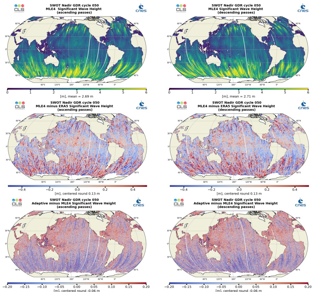
Figure 5: Along-track maps of Ku-band Significant Wave Height over cycle 050 for SWOT Nadir MLE4 (top), MLE4 minus model (middle) or Adaptive minus MLE4 (bottom), ascending passes (left) and descending passes (right)
