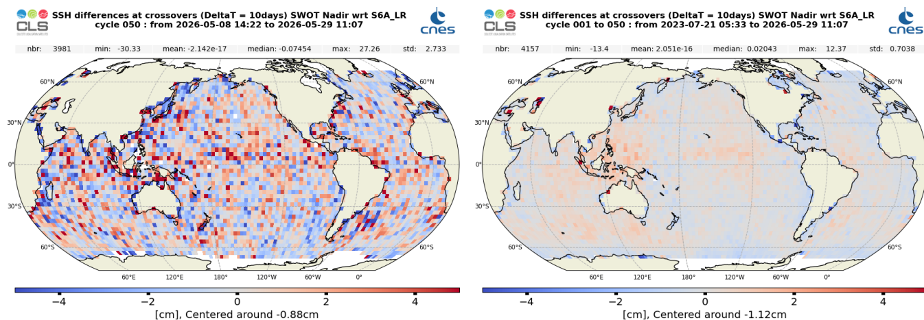
Figure 30: Mean SSH difference at crossovers between SWOT Nadir MLE4 and Sentinel-6 MF LR MLE4 over cycle 050 (left) and from cycle 001 onwards (right)
