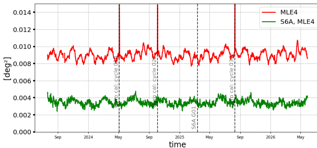
Figure 18: Mispointing daily monitoring from SWOT cycle 001 to 050 for SWOT Nadir GDR (red) and Sentinel-6A-MF (green)
