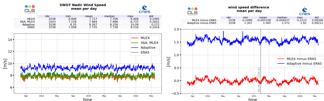
Figure 12: Wind Speed daily monitoring from cycle 001 to 050 for SWOT Nadir GDR, ERA5 model, and Sentinel-6A-MF (LR MLE4) (left), and daily mean difference with ERA5 (right)
