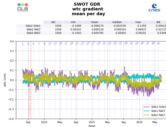
Figure 20: Daily monitoring of the wet tropospheric correction gradient between AMR Side 1 and AMR Side 2 (purple), AMR Side 1 and Nadir (cyan), and AMR Side 2 and Nadir (yellow), from Cycle 001 to 051
