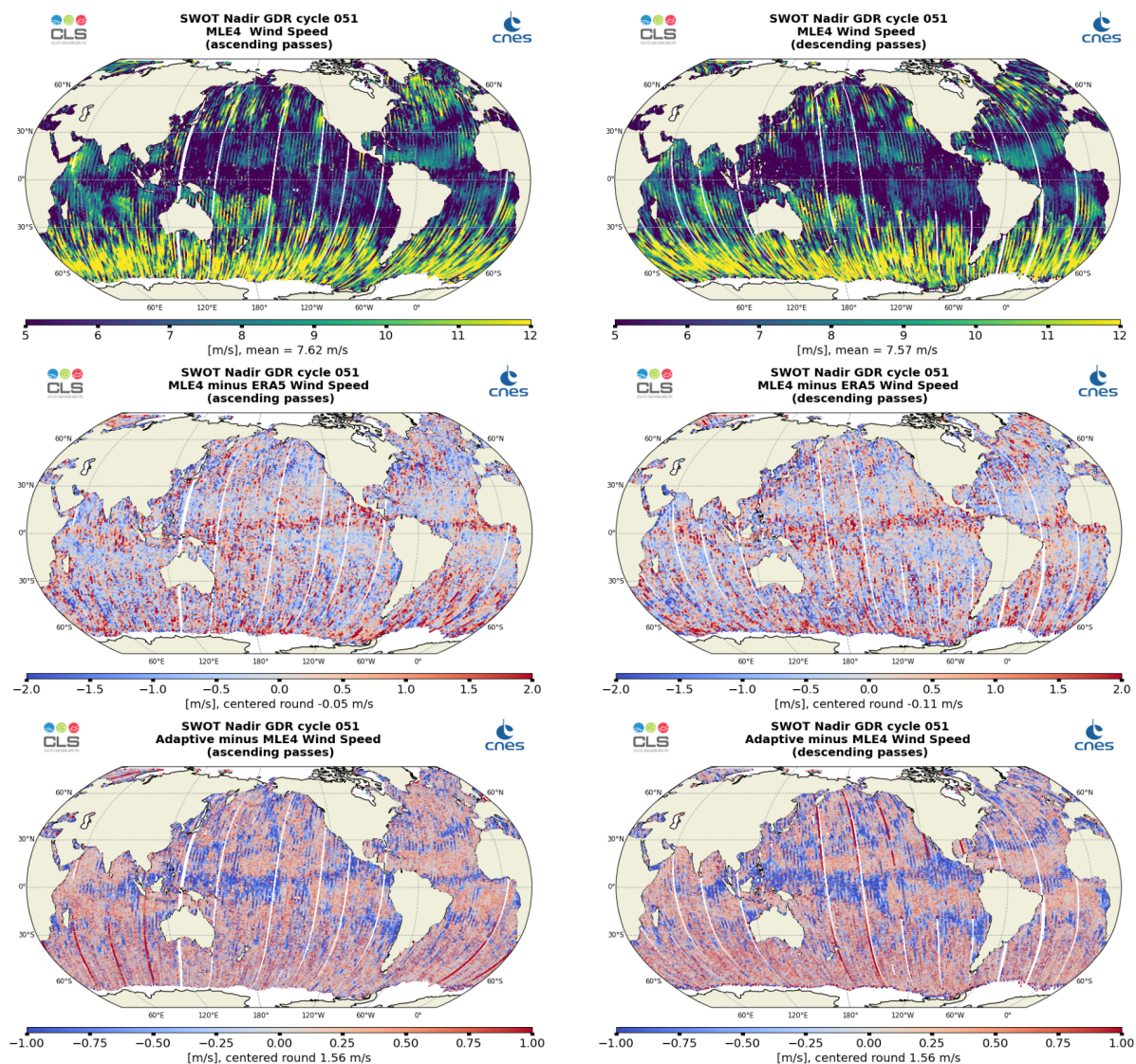
Figure 11: Along-track maps of Altimeter Wind Speed over cycle 051 for SWOT Nadir MLE4 (top), MLE4 minus ERA5 (middle) or Adaptive minus MLE4 (bottom), ascending passes (left) and descending passes (right)
