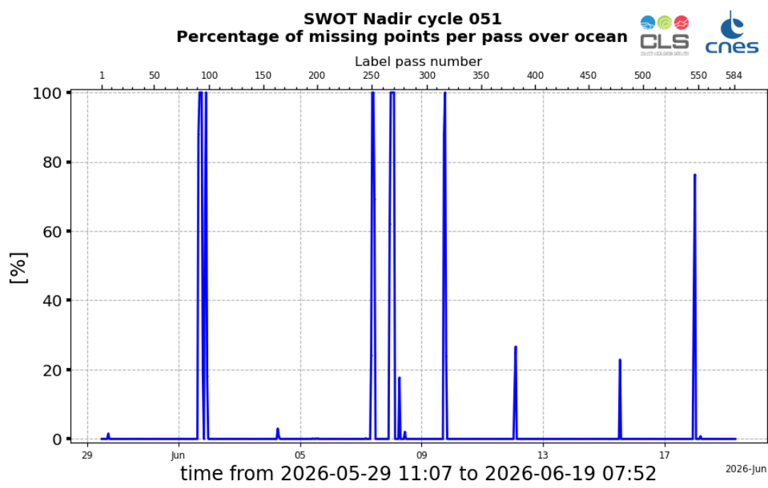
Figure 2: Monitoring of the percentage per pass of missing data over ocean, for SWOT Nadir GDR cycle 051
