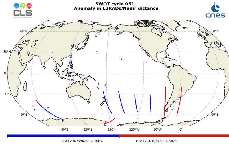
Figure 24: Map of the anomalies detected in the L2RADs/Nadir distance over the cycle 051
