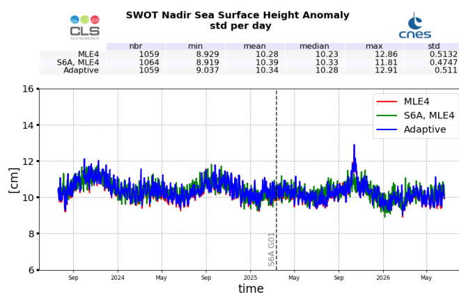
Figure 27: SSHA daily monitoring from cycle 001 to 051, for SWOT Nadir GDR
