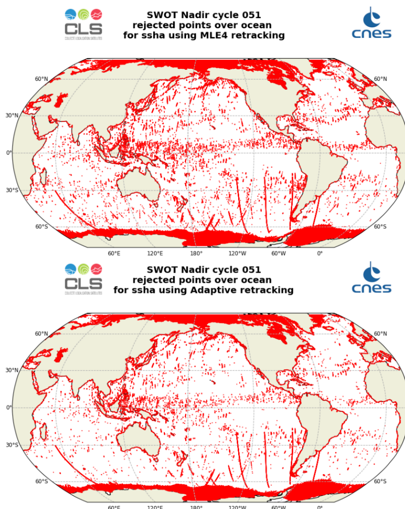
Figure 3: Edited measurements for SWOT Nadir over cycle 051
