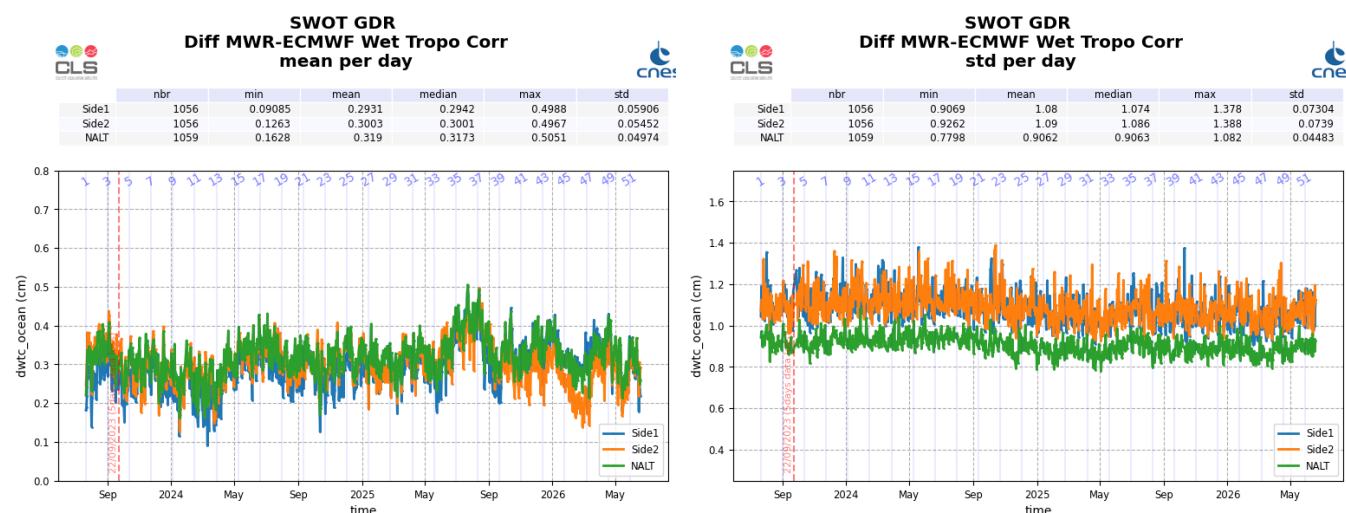
Figure 19: Daily monitoring of mean (left) and standard deviation (right) of the difference between AMRs wet tropospheric correction and ECMWF wet tropospheric correction for the side 1 (blue), the side 2 (orange) and the Nadir (green), computed from cycle 001 to cycle 051
