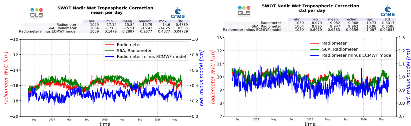
Figure 23: Daily monitoring of mean (left) and standard deviation (right) of the interpolated to Nadir AMRs wet tropospheric corrections (red) and radiometer minus ECMWF model difference of wet tropospheric corrections (blue), computed from cycle 001 to 051. Sentinel-6A-MF radiometer monitoring in green.
