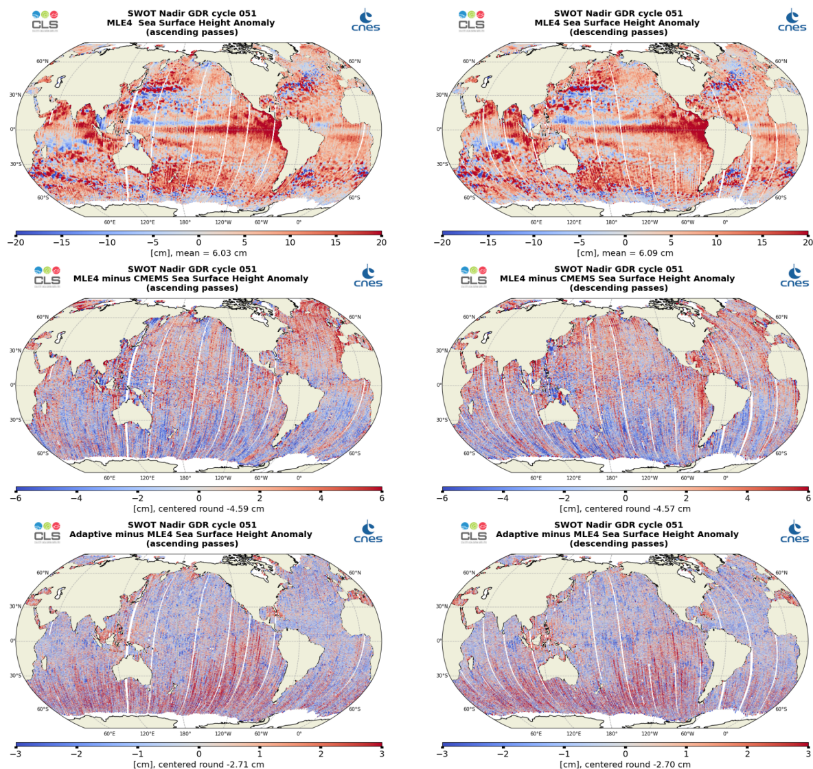
Figure 26: Along-track maps of SSHA over cycle 051 for SWOT Nadir MLE4 (top), MLE4 minus CMEMS (middle) or Adaptive minus MLE4 (bottom), ascending passes (left) and descending passes (right)
