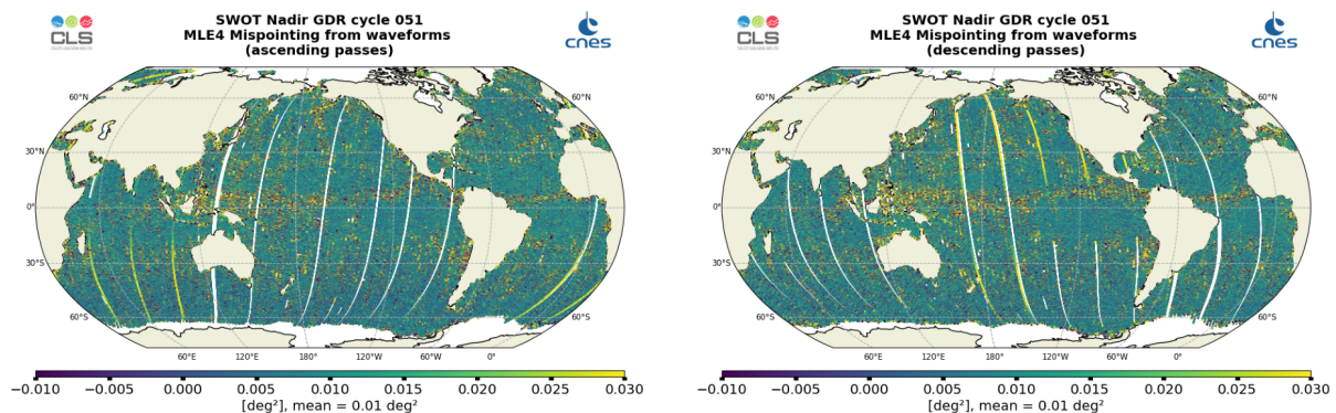
Figure 17: Along-track maps of mispointing over cycle 051 for SWOT Nadir MLE4, ascending passes (left) and descending passes (right)
