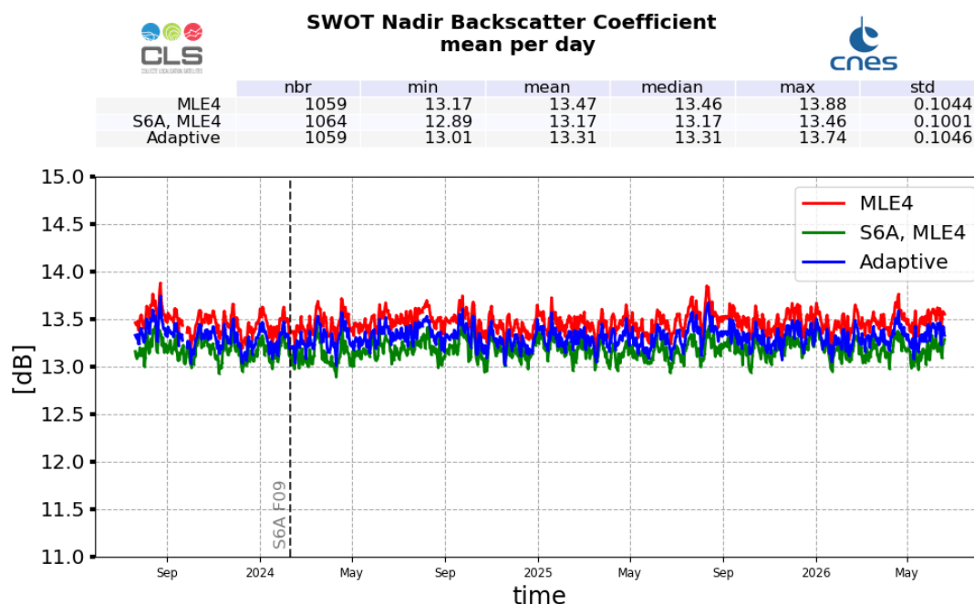
Figure 9: Ku-band Backscattering coefficient daily monitoring from cycle 001 to 051, for SWOT Nadir and Sentinel-6A-MF
