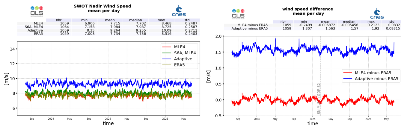
Figure 12: Wind Speed daily monitoring from cycle 001 to 051 for SWOT Nadir GDR, ERA5 model, and Sentinel-6A-MF (LR MLE4) (left), and daily mean difference with ERA5 (right)
