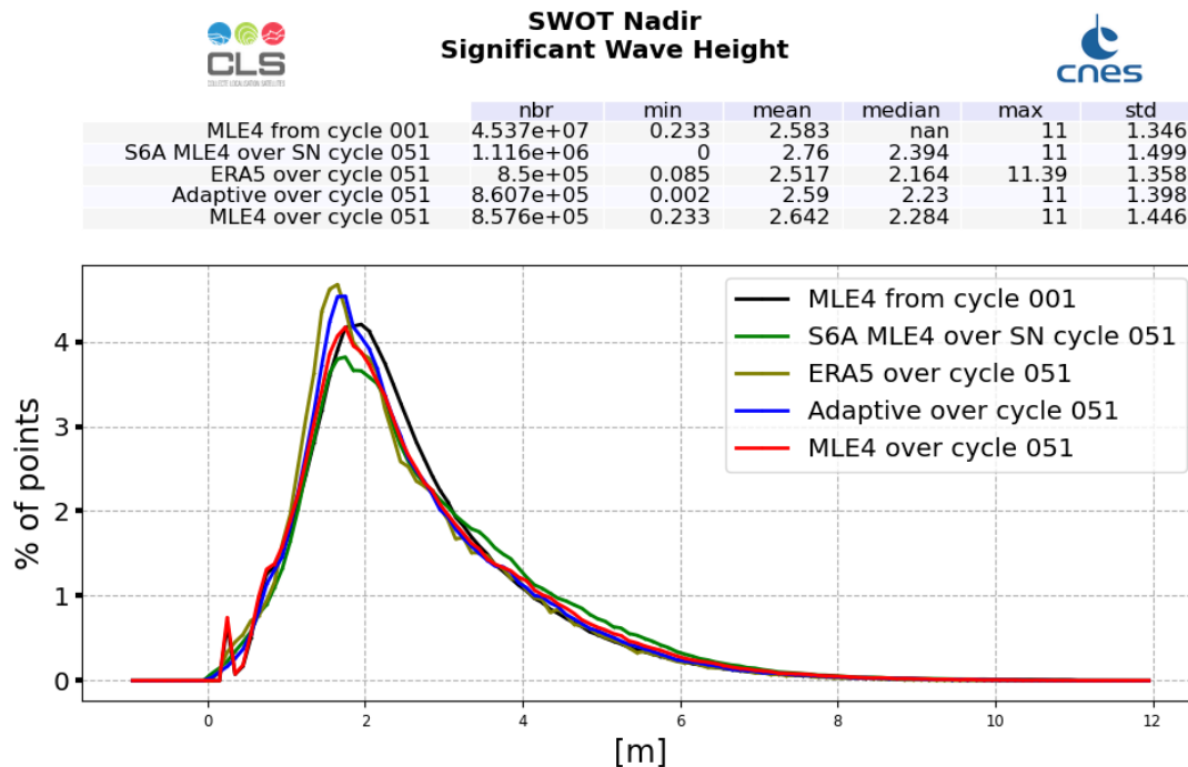
Figure 4: Ku-band Significant Wave Height histogram computed over cycle 051 (red line for SWOT Nadir MLE4 and blue line for SWOT Nadir Adaptive, green for Sentinel-6A-MF (LR MLE4) and dark green for ERA5) and from cycle 001 (SWOT Nadir, MLE4 only, black line)
