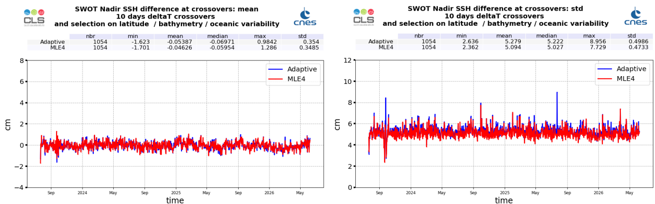
Figure 29: Monitoring of SSH difference at crossovers for SWOT Nadir MLE4 (red) and Adaptive (blue) : mean (left) and standard deviation (right), from cycle 001 to 051
