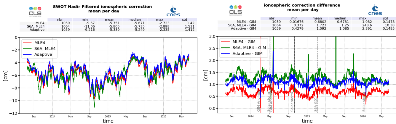
Figure 15: SWOT Nadir MLE4 (red), Adaptive (blue) and Sentinel-6A-MF (LR MLE4) (green) filtered ionosphere correction daily monitoring from cycle 001 to 051 (left) and difference with GIM model (right)
