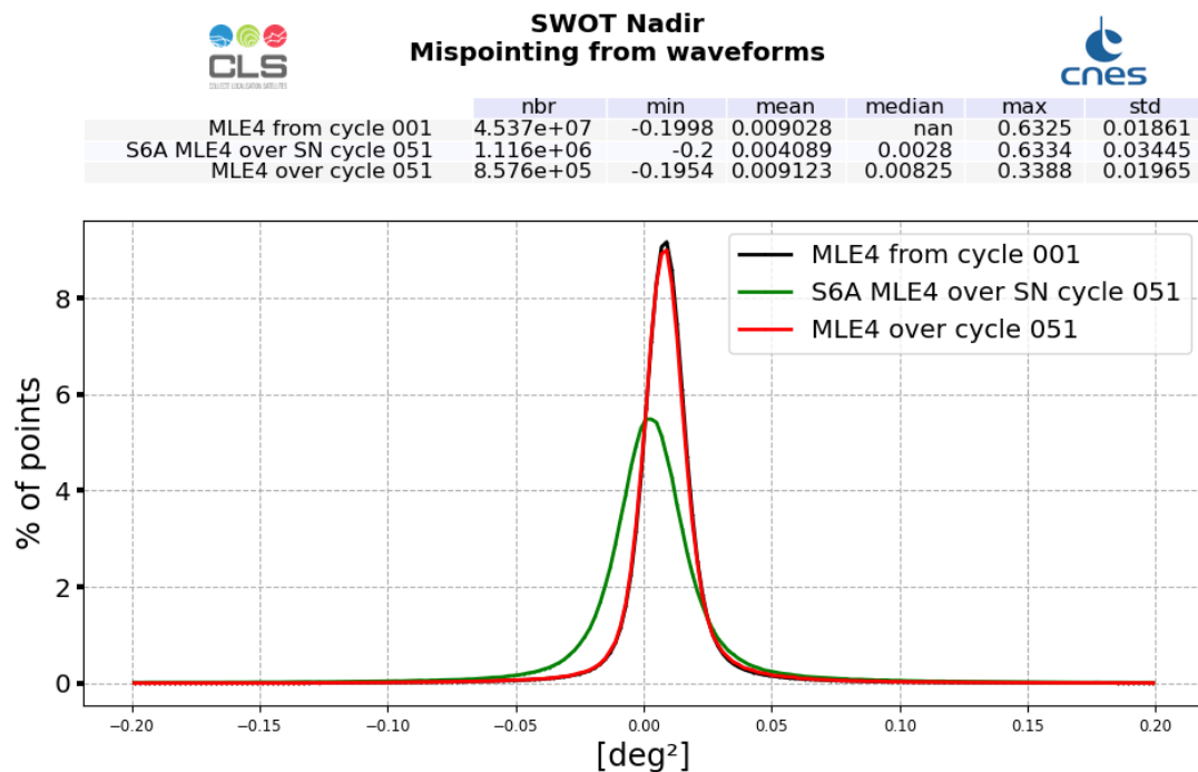
Figure 16: Mispointing histogram computed over cycle 051 (solid line) and from cycle 4 (dashed line)
