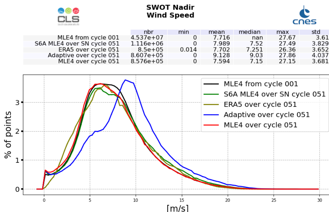
Figure 10: Altimeter Wind Speed histogram computed over cycle 051 (red line for SWOT Nadir MLE4 and blue line for SWOT Nadir Adaptive, green for Sentinel-6A-MF (LR MLE4)) and from cycle 001 (SWOT Nadir, MLE4 only, black line)
