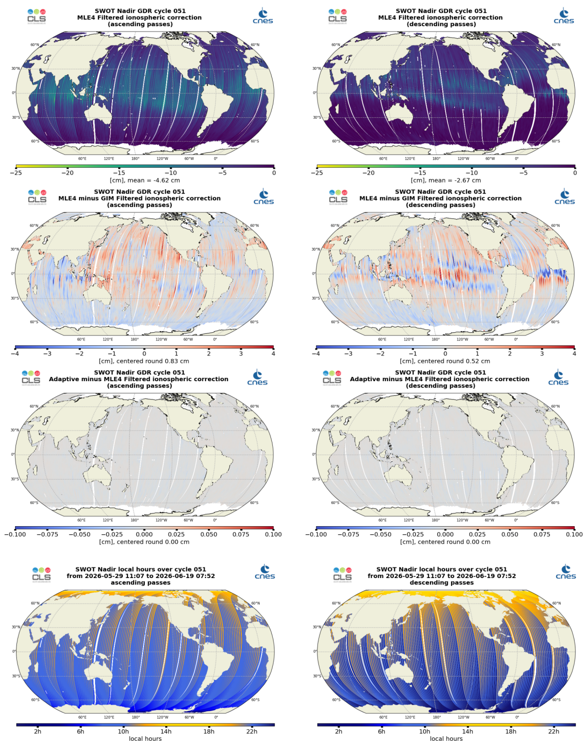
Figure 14: Along-track maps of filtered ionosphere correction over cycle 051 for SWOT Nadir MLE4 (top), MLE4 minus GIM (middle top) or Adaptive minus MLE4 (middle bottom), and local hours (bottom), for ascending passes (left) and descending passes (right)
