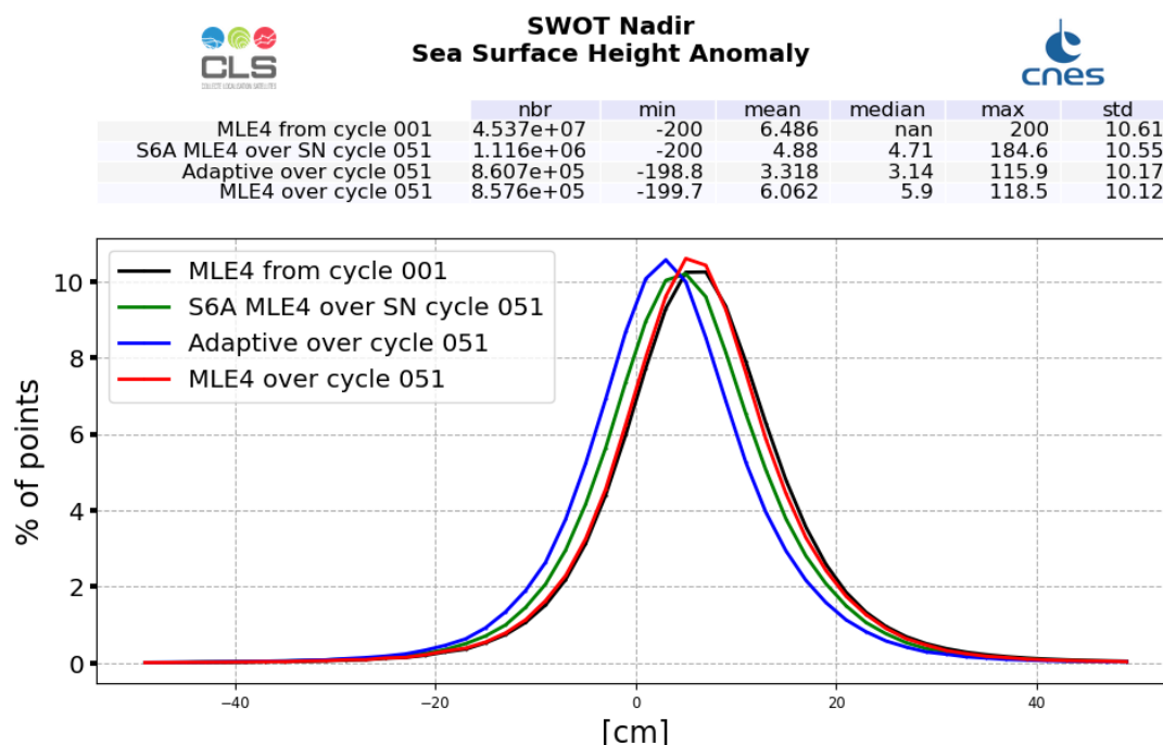
Figure 25: SSHA histogram computed over cycle 051 (red line for SWOT Nadir MLE4 and blue line for SWOT Nadir Adaptive, green for Sentinel-6A-MF (LR MLE4)) and from cycle 001 (SWOT Nadir, MLE4 only, black line)
