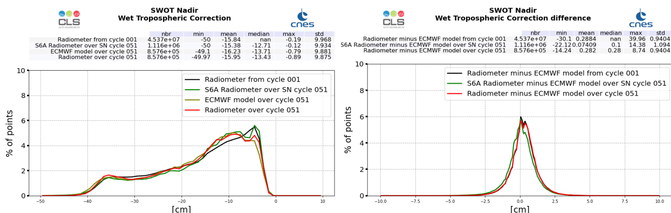
Figure 21: Histogram of wet troposphere corrections : SWOT Nadir radiometer (left) and difference with ECMWF model (right), computed over cycle 051 and from cycle 001 (black line)
