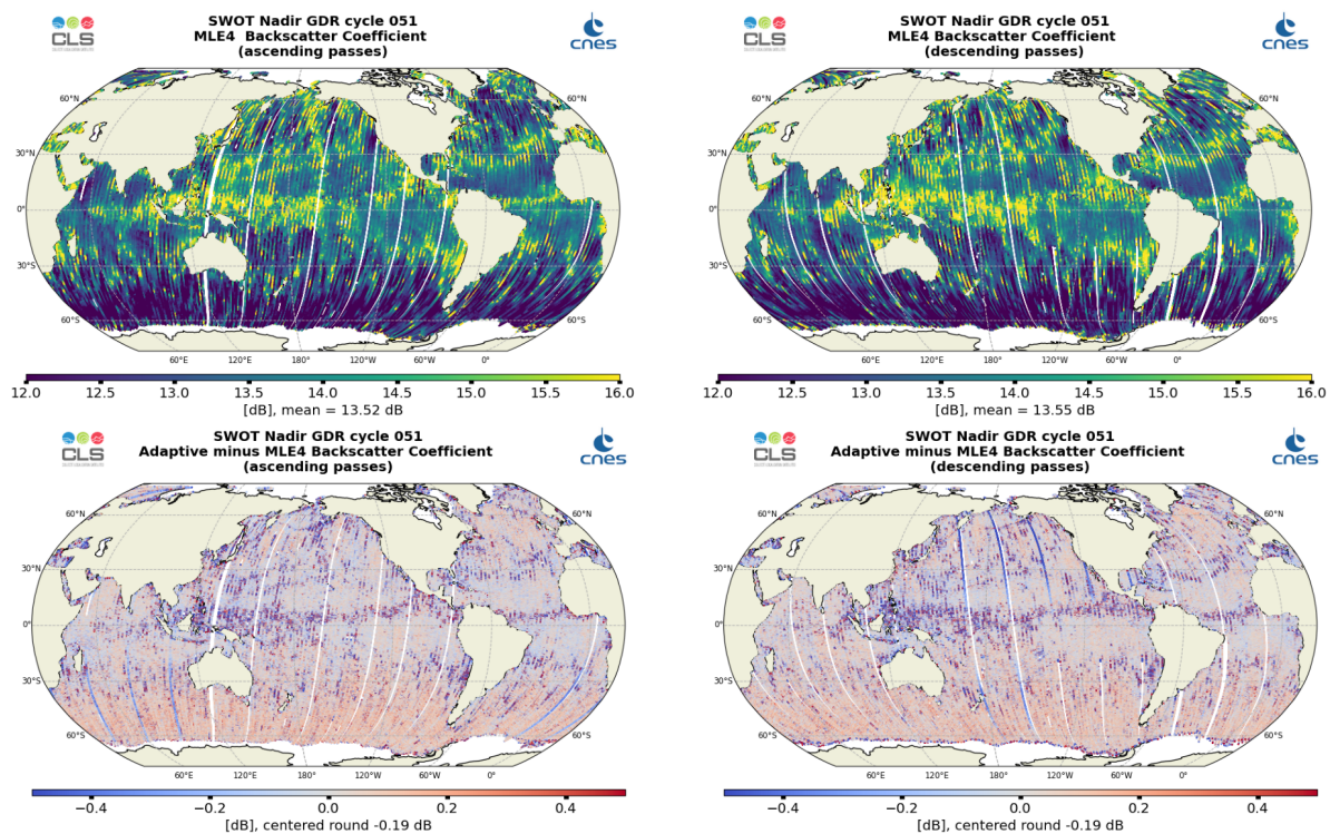
Figure 8: Along-track maps of Ku-band backscatter coefficient \sigma_0 over cycle 051 for SWOT Nadir MLE4 (top) or Adaptive minus MLE4 difference (bottom), ascending passes (left) and descending passes (right)
