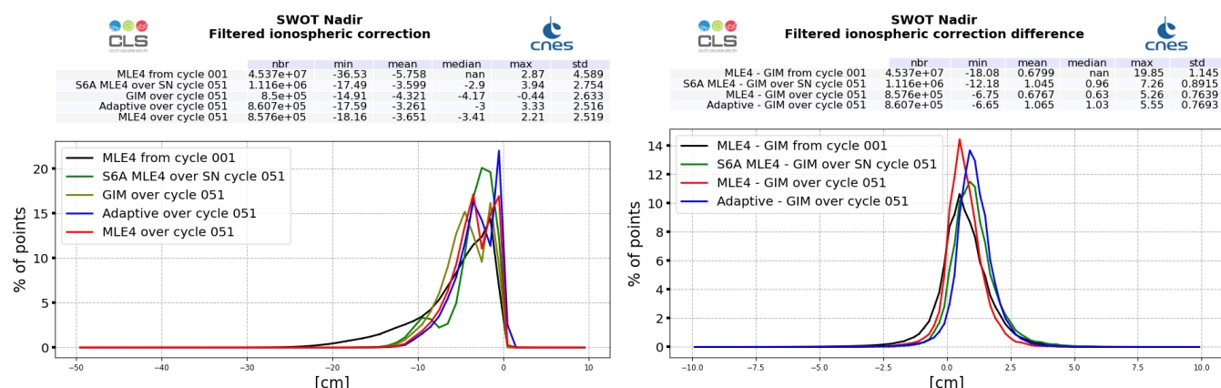
Figure 13: GIM model (dark green) and altimeter filtered ionosphere correction histogram computed over cycle 051 (red line for SWOT Nadir MLE4 and blue line for SWOT Nadir Adaptive, green for Sentinel-6A-MF (LR MLE4)) and from cycle 001 (SWOT Nadir, MLE4 only, black line) (left). Difference between filtered altimeter and GIM model (right).
