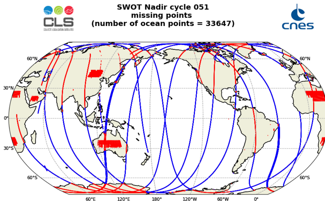
Figure 1: Map of missing measurements for SWOT Nadir GDR cycle 051
