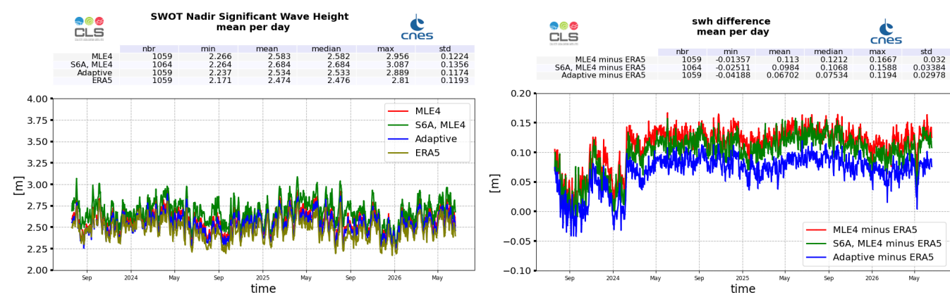
Figure 6: Ku-band Significant Wave Height daily monitoring from cycle 001 to 051, for SWOT Nadir, ERA5 model estimated at SWOT locations, and Sentinel-6A-MF (LR MLE4) (left), and difference with ERA5 model (right)
