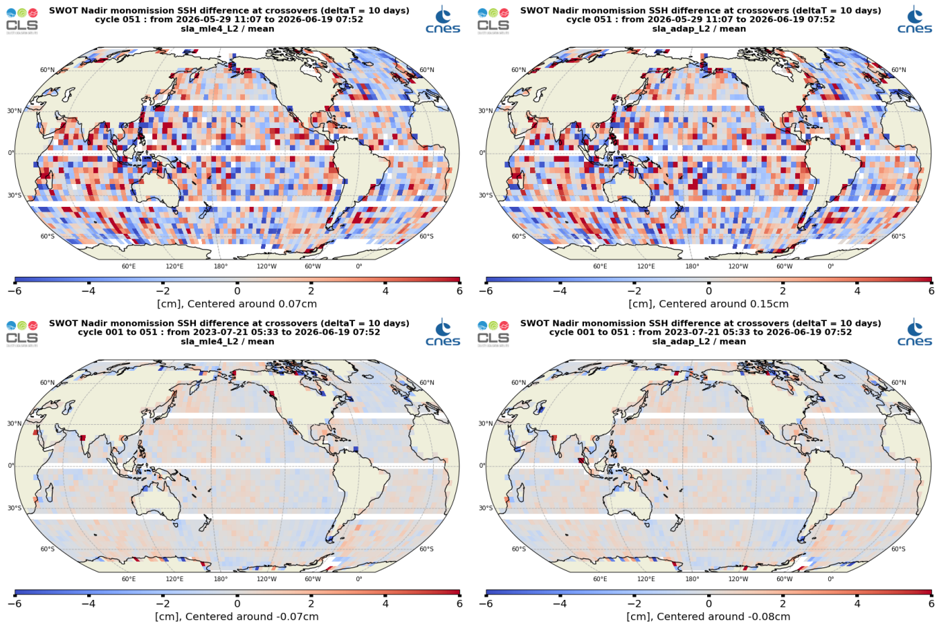
Figure 28: Mean SSH difference at crossovers for SWOT Nadir MLE4 (left) and Adaptive (right) cycle 051(top) and from cycle 001 to cycle 051 (bottom)
