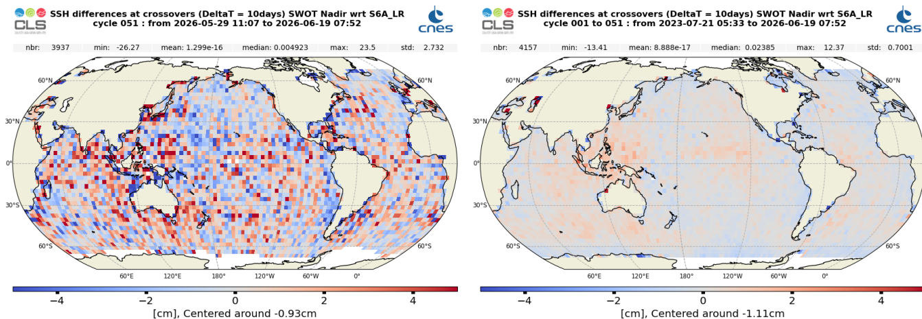
Figure 30: Mean SSH difference at crossovers between SWOT Nadir MLE4 and Sentinel-6 MF LR MLE4 over cycle 051 (left) and from cycle 001 onwards (right)
