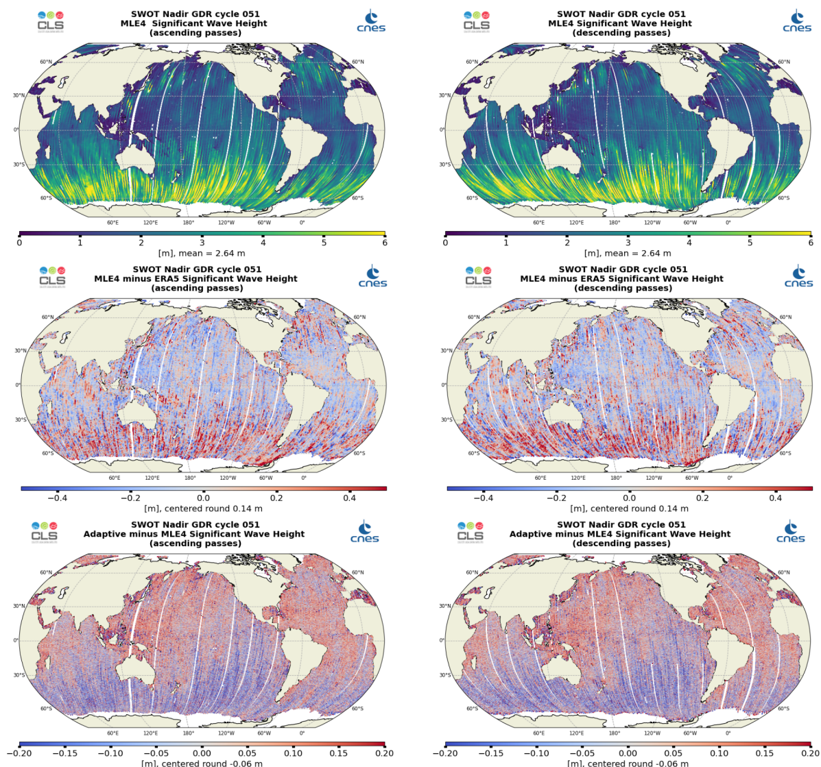
Figure 5: Along-track maps of Ku-band Significant Wave Height over cycle 051 for SWOT Nadir MLE4 (top), MLE4 minus model (middle) or Adaptive minus MLE4 (bottom), ascending passes (left) and descending passes (right)
