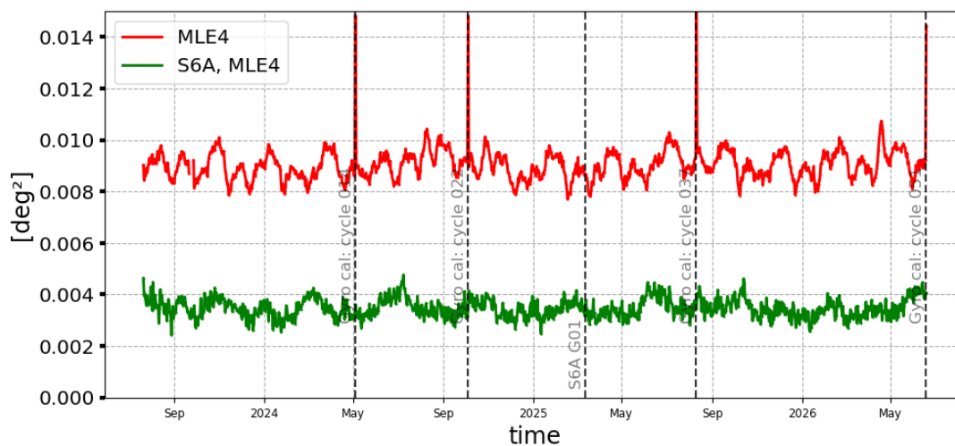
Figure 18: Mispointing daily monitoring from SWOT cycle 001 to 051 for SWOT Nadir GDR (red) and Sentinel-6A-MF (green)
