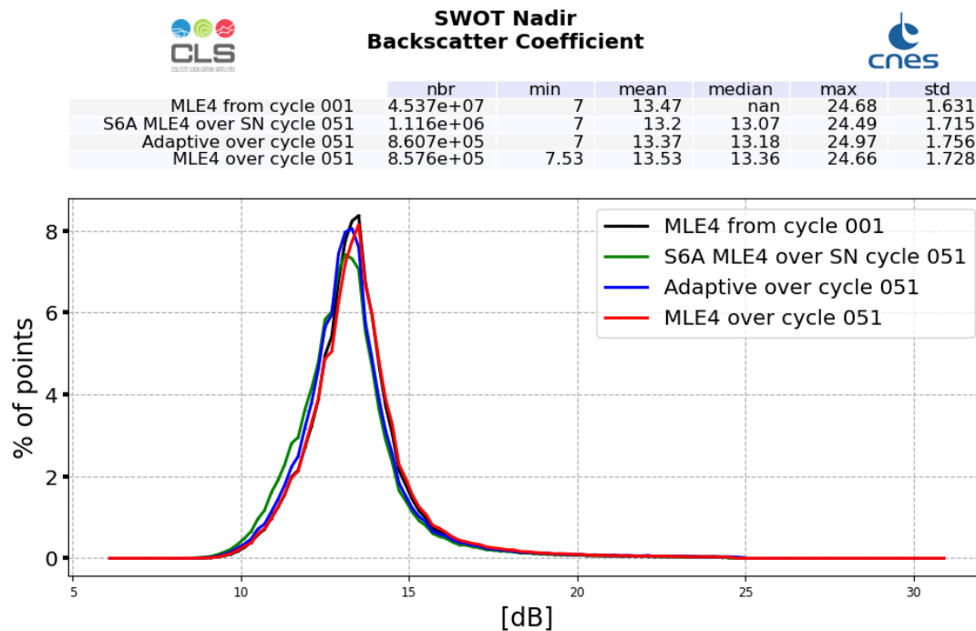
Figure 7: Ku-band Backscattering coefficient histogram computed over cycle 051 (red line for SWOT Nadir MLE4 and blue line for SWOT Nadir Adaptive, green for Sentinel-6A-MF (LR MLE4)) and from cycle 001 (SWOT Nadir, MLE4 only, black line)
