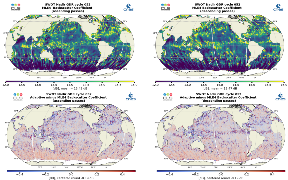
Figure 8: Along-track maps of Ku-band backscatter coefficient \sigma_0 over cycle 052 for SWOT Nadir MLE4 (top) or Adaptive minus MLE4 difference (bottom), ascending passes (left) and descending passes (right)
