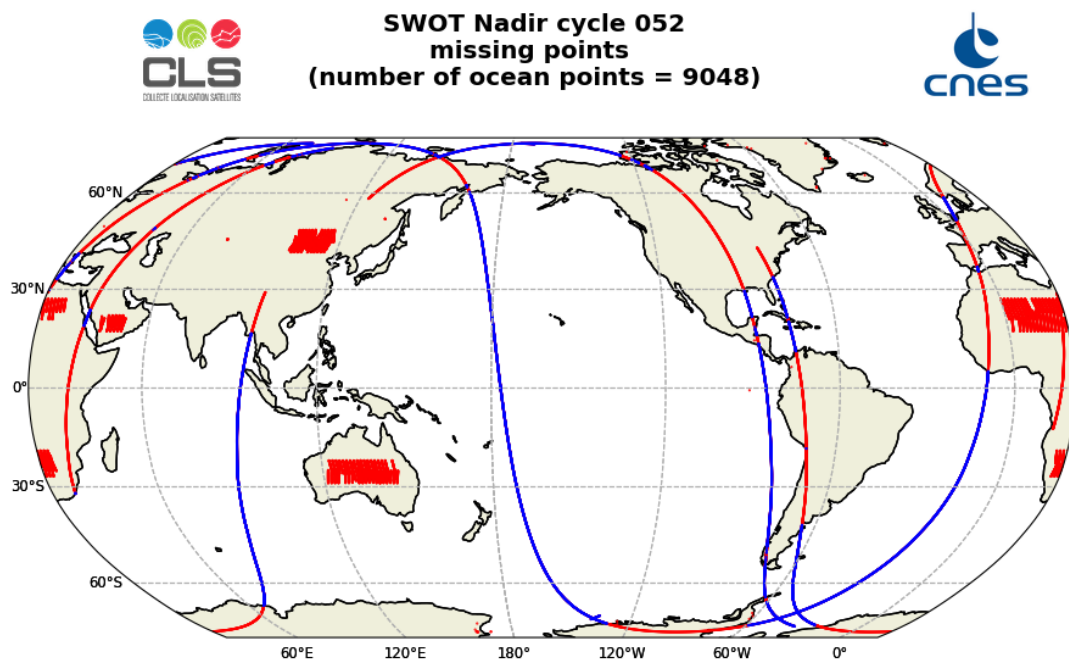
Figure 1: Map of missing measurements for SWOT Nadir GDR cycle 052
