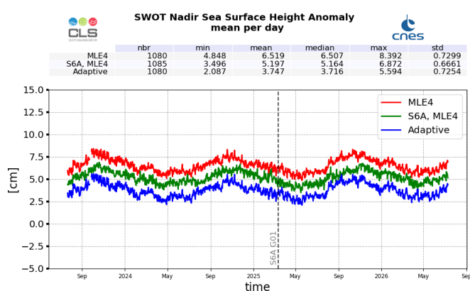
Figure 27: SSHA daily monitoring from cycle 001 to 052, for SWOT Nadir GDR
