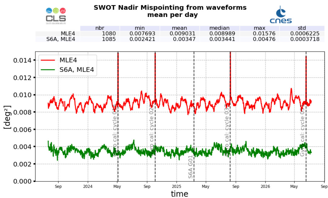
Figure 18: Mispointing daily monitoring from SWOT cycle 001 to 052 for SWOT Nadir GDR (red) and Sentinel-6A-MF (green)
