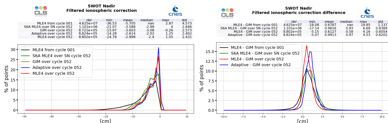
Figure 13: GIM model (dark green) and altimeter filtered ionosphere correction histogram computed over cycle 052 (red line for SWOT Nadir MLE4 and blue line for SWOT Nadir Adaptive, green for Sentinel-6A-MF (LR MLE4)) and from cycle 001 (SWOT Nadir, MLE4 only, black line) (left). Difference between filtered altimeter and GIM model (right).
