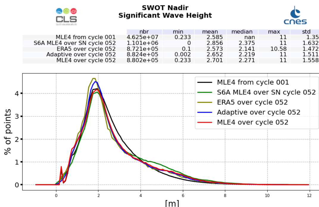
Figure 4: Ku-band Significant Wave Height histogram computed over cycle 052 (red line for SWOT Nadir MLE4 and blue line for SWOT Nadir Adaptive, green for Sentinel-6A-MF (LR MLE4) and dark green for ERA5) and from cycle 001 (SWOT Nadir, MLE4 only, black line)
