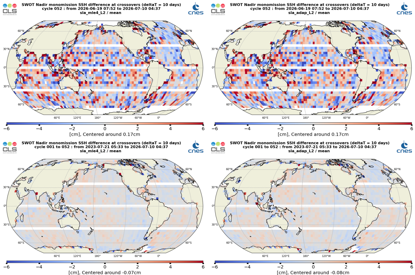
Figure 28: Mean SSH difference at crossovers for SWOT Nadir MLE4 (left) and Adaptive (right) cycle 052(top) and from cycle 001 to cycle 052 (bottom)
