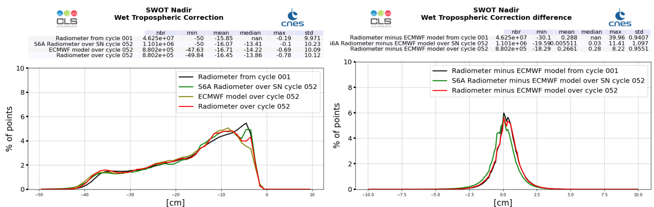
Figure 21: Histogram of wet troposphere corrections : SWOT Nadir radiometer (left) and difference with ECMWF model (right), computed over cycle 052 and from cycle 001 (black line)
