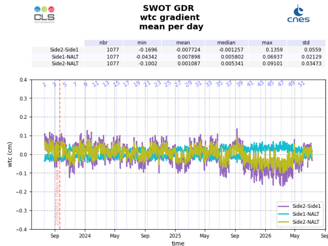
Figure 20: Daily monitoring of the wet tropospheric correction gradient between AMR Side 1 and AMR Side 2 (purple), AMR Side 1 and Nadir (cyan), and AMR Side 2 and Nadir (yellow), from Cycle 001 to 052
