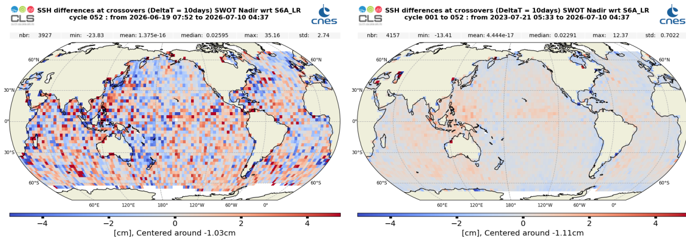
Figure 30: Mean SSH difference at crossovers between SWOT Nadir MLE4 and Sentinel-6 MF LR MLE4 over cycle 052 (left) and from cycle 001 onwards (right)
