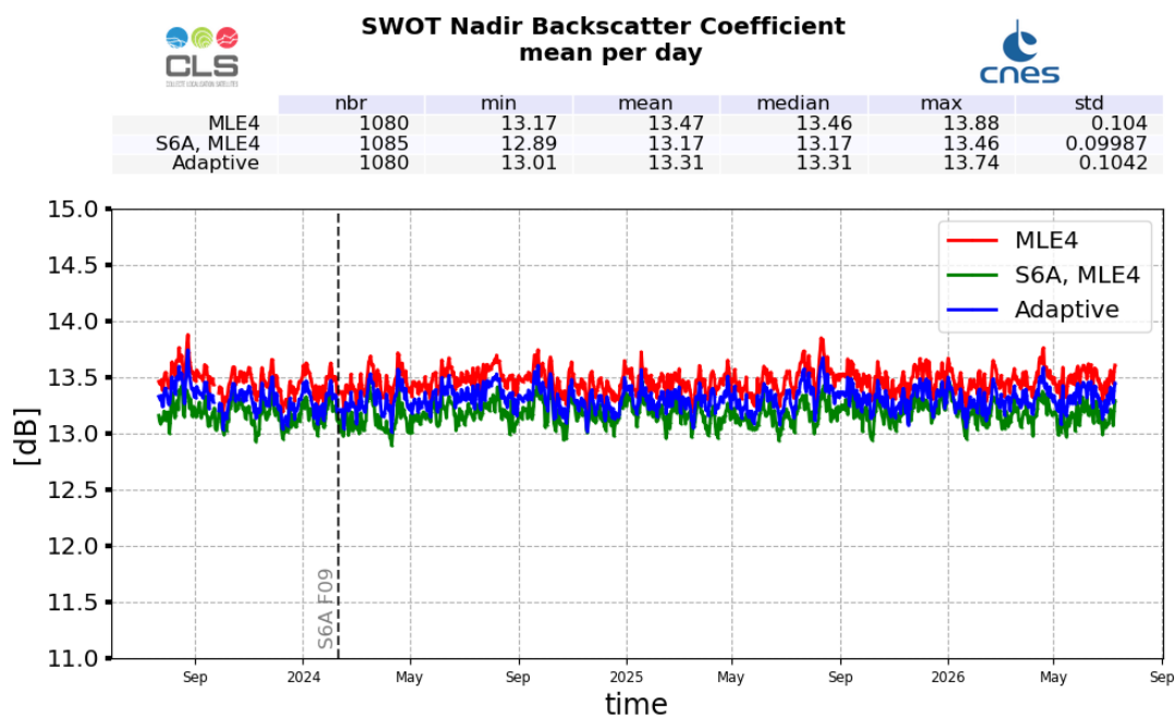
Figure 9: Ku-band Backscattering coefficient daily monitoring from cycle 001 to 052, for SWOT Nadir and Sentinel-6A-MF
