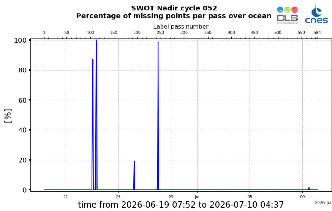
Figure 2: Monitoring of the percentage per pass of missing data over ocean, for SWOT Nadir GDR cycle 052
