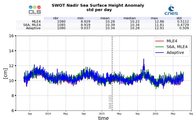
Figure 27: SSHA daily monitoring from cycle 001 to 052, for SWOT Nadir GDR
