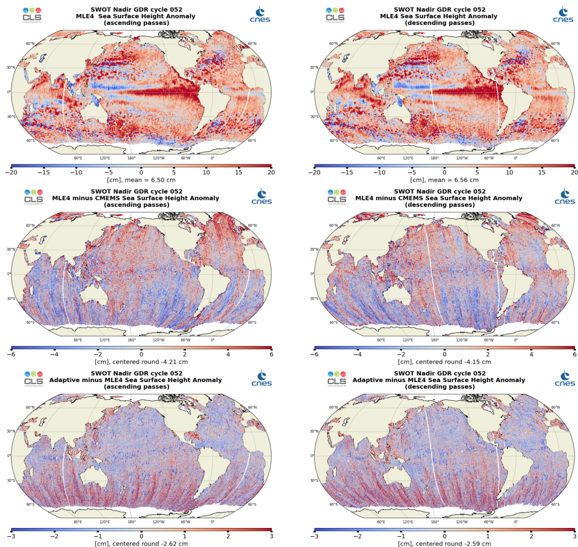
Figure 26: Along-track maps of SSHA over cycle 052 for SWOT Nadir MLE4 (top), MLE4 minus CMEMS (middle) or Adaptive minus MLE4 (bottom), ascending passes (left) and descending passes (right)
