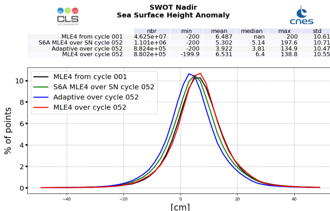
Figure 25: SSHA histogram computed over cycle 052 (red line for SWOT Nadir MLE4 and blue line for SWOT Nadir Adaptive, green for Sentinel-6A-MF (LR MLE4)) and from cycle 001 (SWOT Nadir, MLE4 only, black line)
