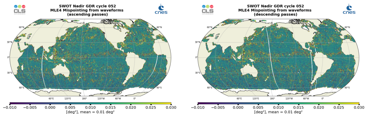
Figure 17: Along-track maps of mispointing over cycle 052 for SWOT Nadir MLE4, ascending passes (left) and descending passes (right)
