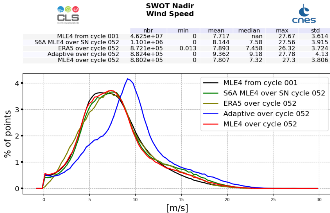
Figure 10: Altimeter Wind Speed histogram computed over cycle 052 (red line for SWOT Nadir MLE4 and blue line for SWOT Nadir Adaptive, green for Sentinel-6A-MF (LR MLE4)) and from cycle 001 (SWOT Nadir, MLE4 only, black line)
