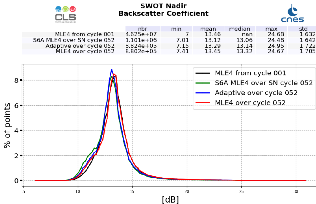
Figure 7: Ku-band Backscattering coefficient histogram computed over cycle 052 (red line for SWOT Nadir MLE4 and blue line for SWOT Nadir Adaptive, green for Sentinel-6A-MF (LR MLE4)) and from cycle 001 (SWOT Nadir, MLE4 only, black line)
