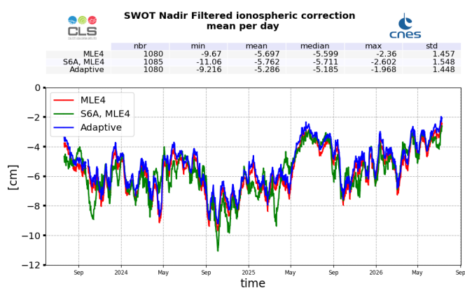
Figure 15: SWOT Nadir MLE4 (red), Adaptive (blue) and Sentinel-6A-MF (LR MLE4) (green) filtered ionosphere correction daily monitoring from cycle 001 to 052 (left) and difference with GIM model (right)
