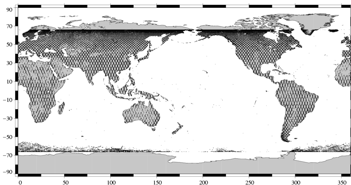
Missing measurements Jason-1 Cycle 060 (23/08/2003 / 02/09/2003)
