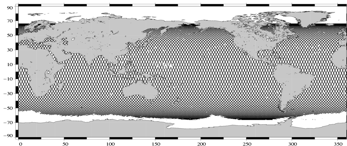
Valid data Jason-1 Cycle 060 (23/08/2003 / 02/09/2003)
