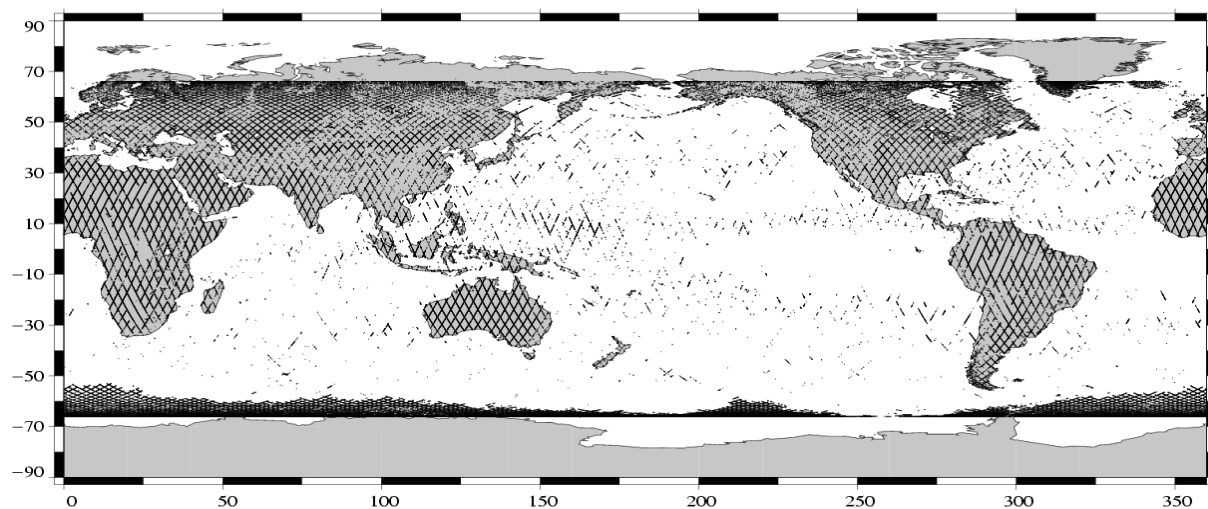
Edited measurements Jason-1 Cycle 060 (23/08/2003 / 02/09/2003)
