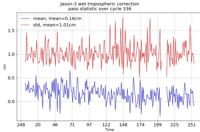
FIGURE 11 – Pass monitoring of wet troposphere differences between radiometer and ECMWF model for Jason-3 cycle 336
