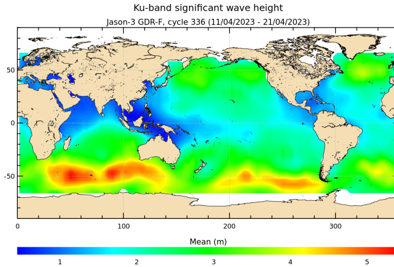
FIGURE 5 – Significant wave height for cycle 336.
