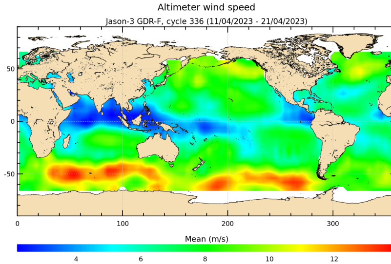
FIGURE 9 – Altimeter wind speed for cycle 336.
