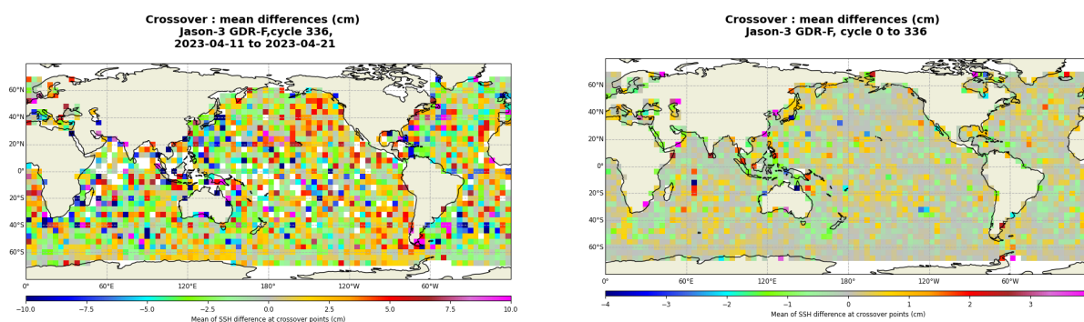
FIGURE 13 – Mean SSH at crossovers for cycle 336 (left) and over the whole Jason-3 period (right).
