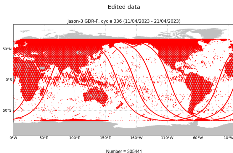
FIGURE 2 – Edited measurements for cycle 336.
