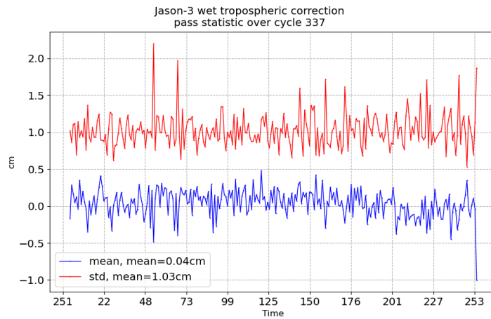
FIGURE 11 – Pass monitoring of wet troposphere differences between radiometer and ECMWF model for Jason-3 cycle 337
