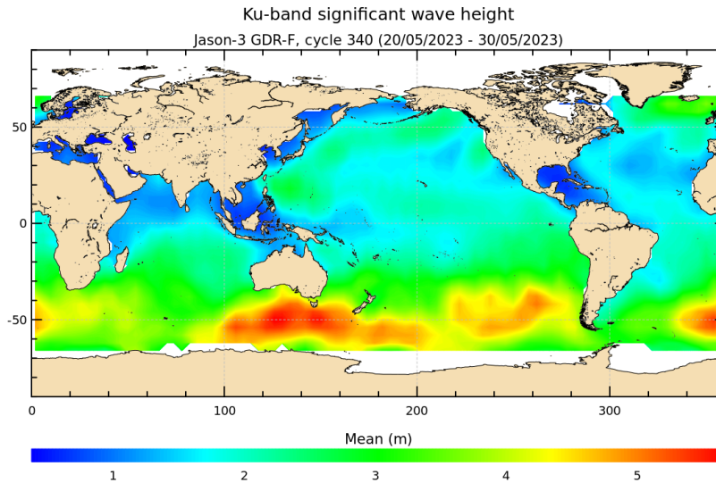
FIGURE 5 – Significant wave height for cycle 340.
