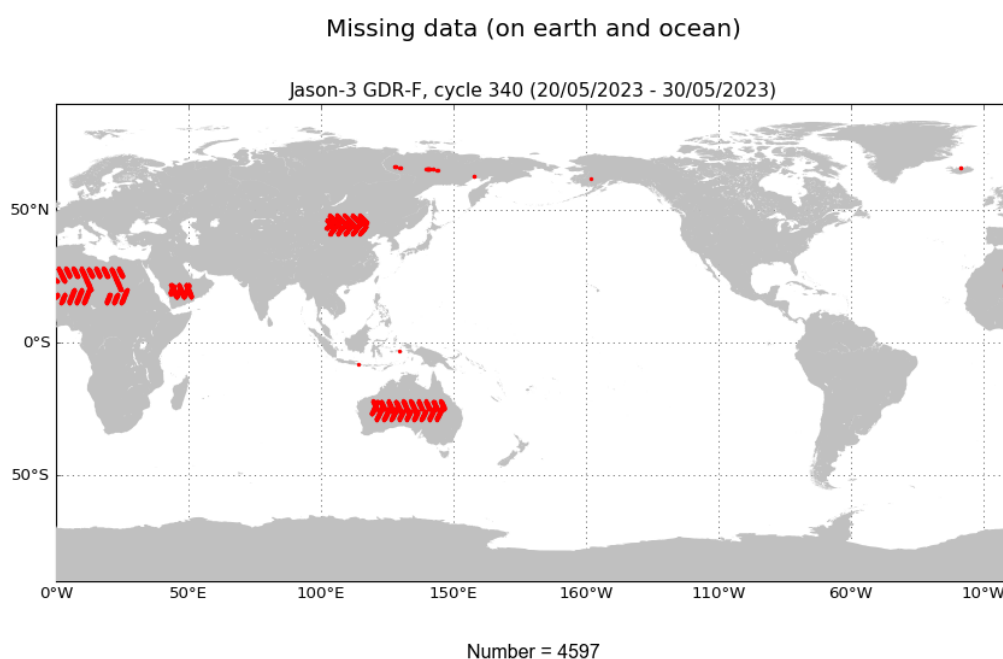
FIGURE 1 – Missing measurements for cycle 340.
