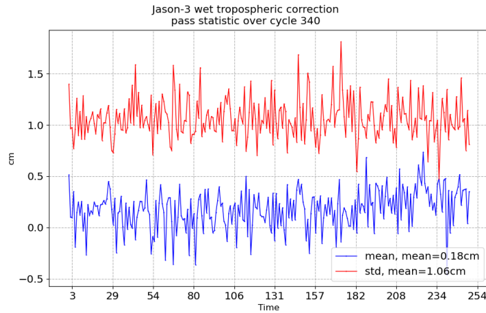
FIGURE 11 – Pass monitoring of wet troposphere differences between radiometer and ECMWF model for Jason-3 cycle 340
