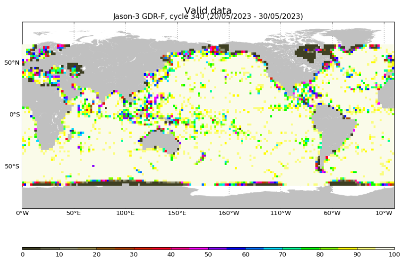
FIGURE 3 – Percentage of valid measurements for cycle 340.
