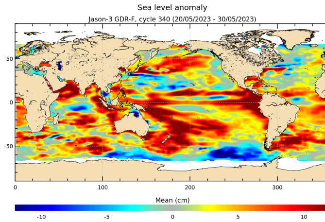
FIGURE 18 – Sea level anomaly relative to MSS for cycle 340.
