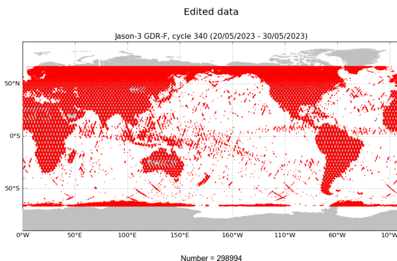
FIGURE 2 – Edited measurements for cycle 340.
