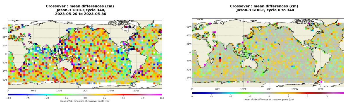
FIGURE 13 – Mean SSH at crossovers for cycle 340 (left) and over the whole Jason-3 period (right).
