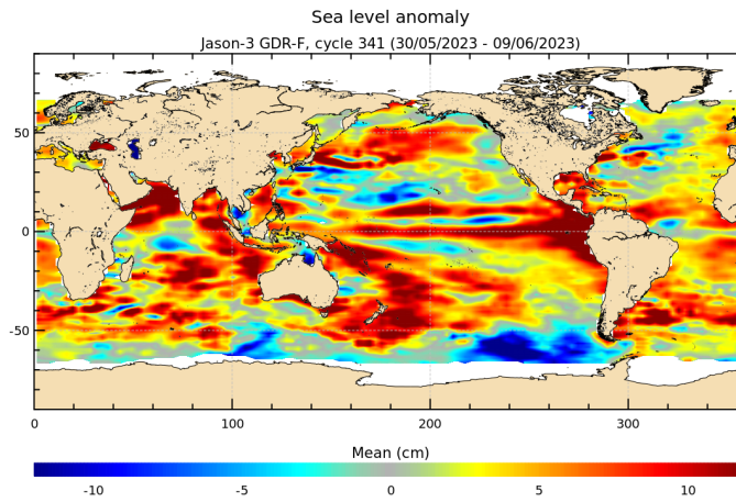
FIGURE 18 – Sea level anomaly relative to MSS for cycle 341.
