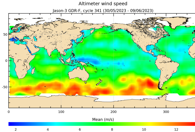
FIGURE 9 – Altimeter wind speed for cycle 341.
