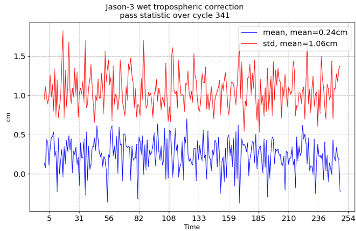
FIGURE 11 – Pass monitoring of wet troposphere differences between radiometer and ECMWF model for Jason-3 cycle 341
