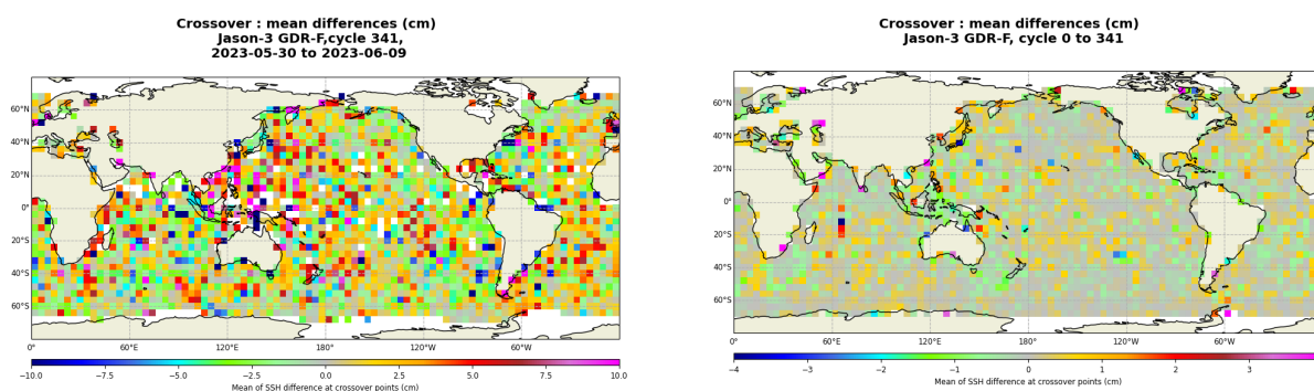
FIGURE 13 – Mean SSH at crossovers for cycle 341 (left) and over the whole Jason-3 period (right).
