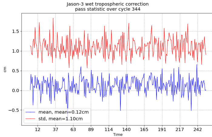
FIGURE 11 – Pass monitoring of wet troposphere differences between radiometer and ECMWF model for Jason-3 cycle 344
