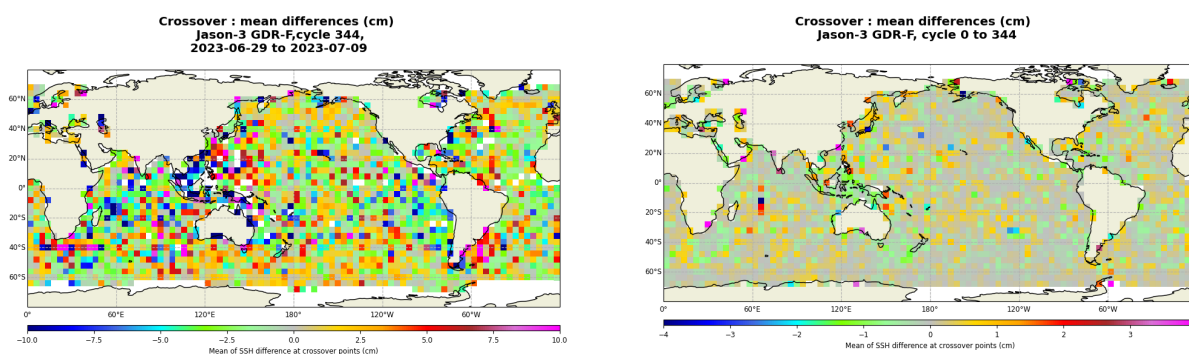
FIGURE 13 – Mean SSH at crossovers for cycle 344 (left) and over the whole Jason-3 period (right).
