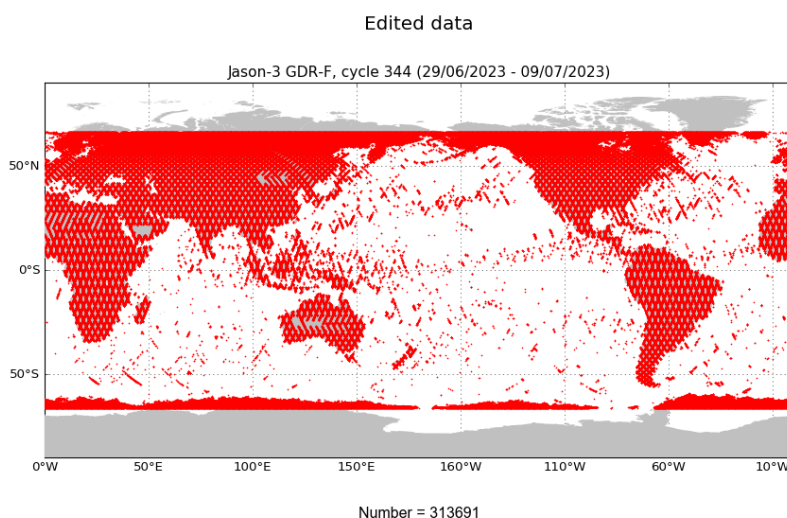
FIGURE 2 – Edited measurements for cycle 344.
