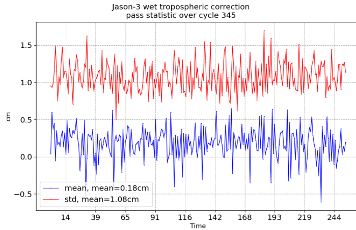
FIGURE 11 – Pass monitoring of wet troposphere differences between radiometer and ECMWF model for Jason-3 cycle 345
