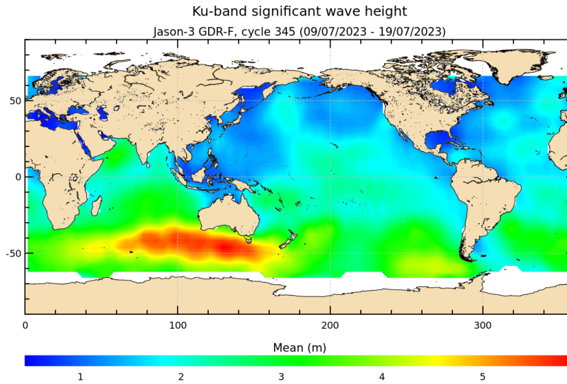
FIGURE 5 – Significant wave height for cycle 345.
