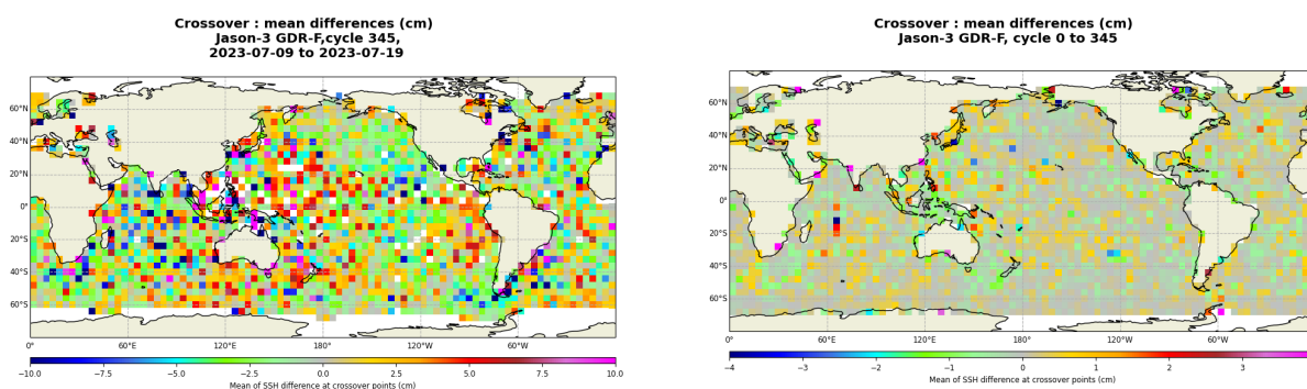
FIGURE 13 – Mean SSH at crossovers for cycle 345 (left) and over the whole Jason-3 period (right).
