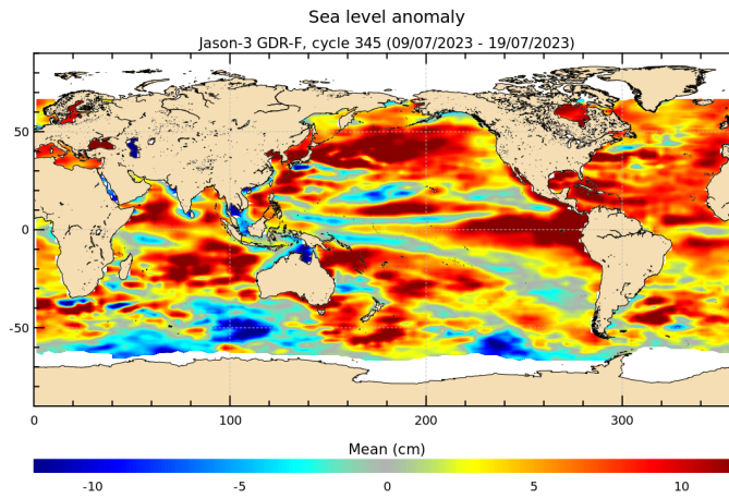
FIGURE 18 – Sea level anomaly relative to MSS for cycle 345.
