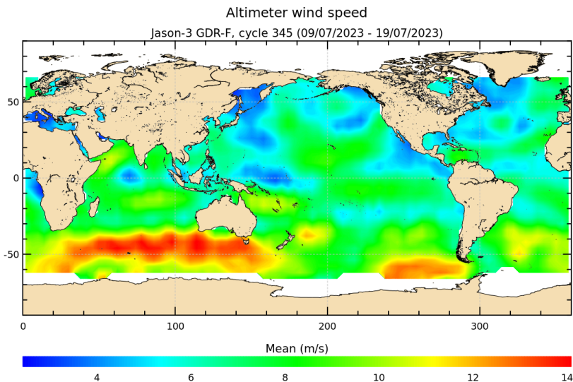
FIGURE 9 – Altimeter wind speed for cycle 345.
