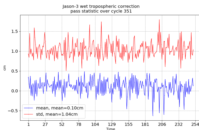
FIGURE 11 – Pass monitoring of wet troposphere differences between radiometer and ECMWF model for Jason-3 cycle 351
