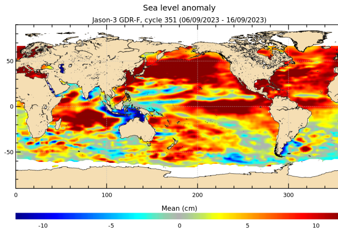
FIGURE 18 – Sea level anomaly relative to MSS for cycle 351.
