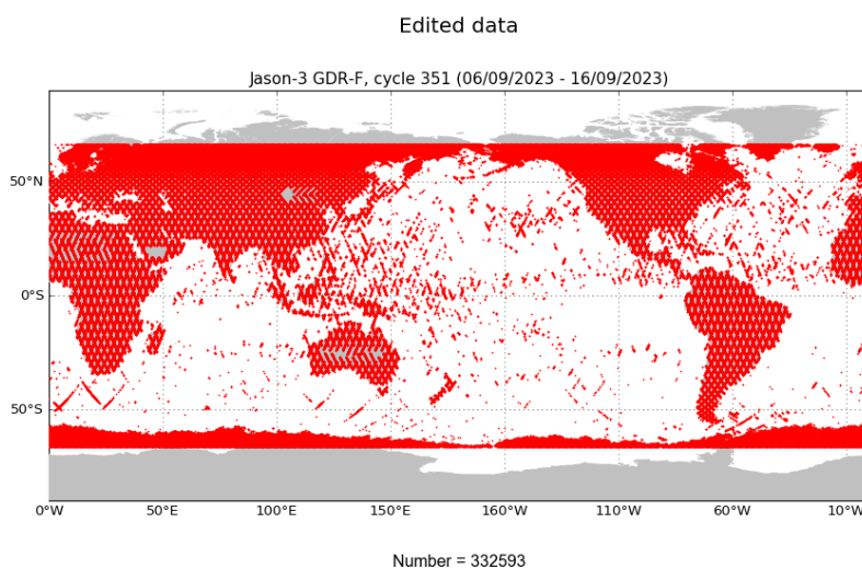
FIGURE 2 – Edited measurements for cycle 351.
