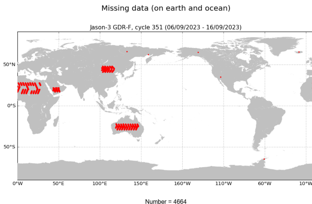
FIGURE 1 – Missing measurements for cycle 351.
