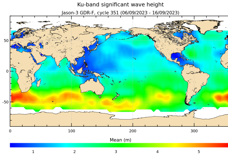
FIGURE 5 – Significant wave height for cycle 351.
