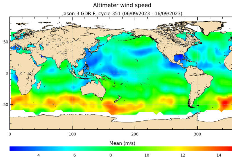
FIGURE 9 – Altimeter wind speed for cycle 351.
