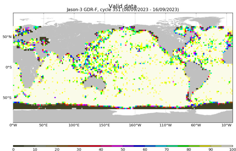
FIGURE 3 – Percentage of valid measurements for cycle 351.
