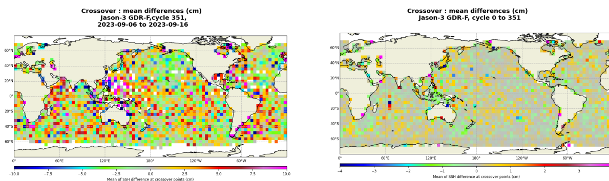
FIGURE 13 – Mean SSH at crossovers for cycle 351 (left) and over the whole Jason-3 period (right).
