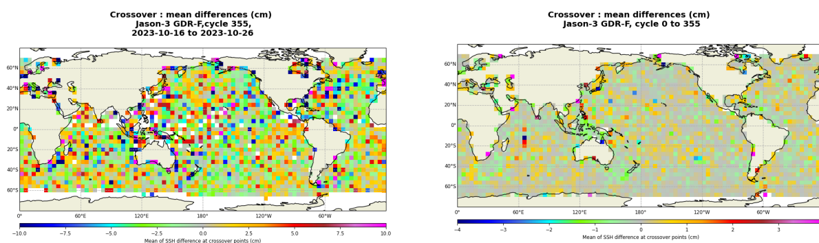
FIGURE 13 – Mean SSH at crossovers for cycle 355 (left) and over the whole Jason-3 period (right).
