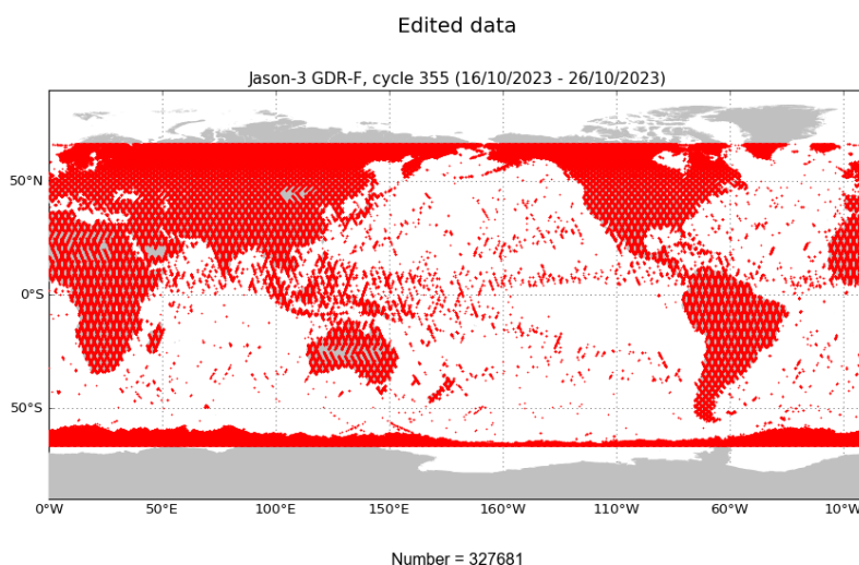
FIGURE 2 – Edited measurements for cycle 355.
