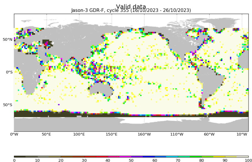
FIGURE 3 – Percentage of valid measurements for cycle 355.
