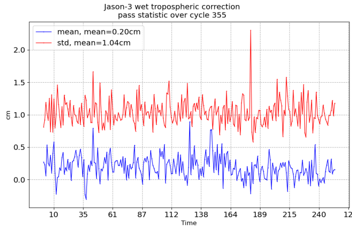
FIGURE 11 – Pass monitoring of wet troposphere differences between radiometer and ECMWF model for Jason-3 cycle 355
