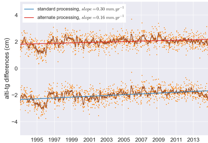
Figure 22: Global mean differences between SSALTO/DUACS grids and tide gauges using two different averaging schemes
