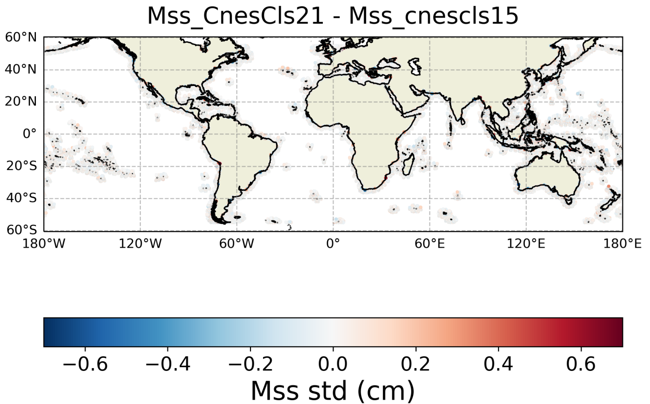
FIGURE 11 – Spatial coherence analysis of the Difference in Mss 's std between Mss_CnesCls21 and Mss_cnescls15
