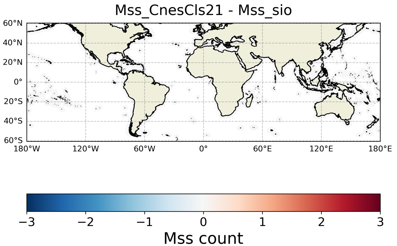
FIGURE 6 – Spatial coherence analysis of the Difference in Mss 's count between Mss_CnesCls21 and Mss_sio
