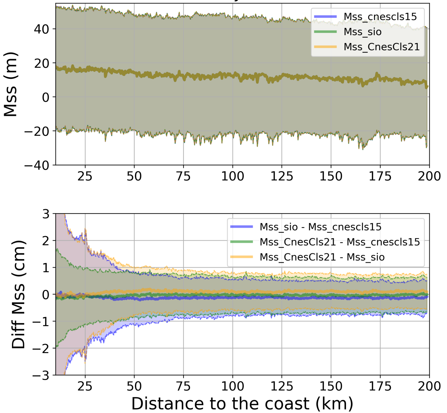
FIGURE 28 – Along-track analysis of Mss 's mean
