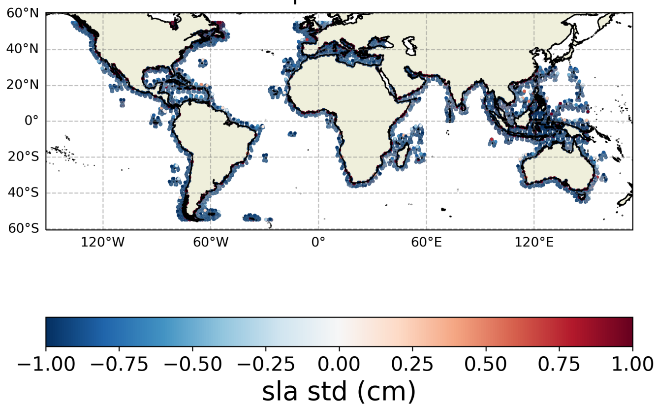
FIGURE 16 – Spatial coherence analysis of the Difference in sla 's std between Adaptive and Mle4
