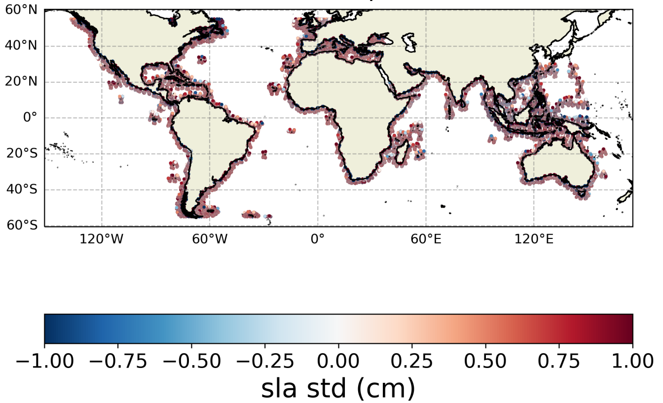
FIGURE 18 – Spatial coherence analysis of the Difference in sla 's std between Ales and Adaptive
