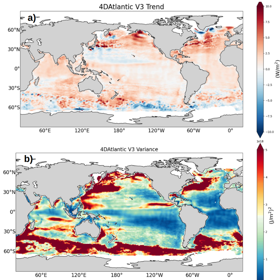
Figure 1: Anomalies in the Ocean Heat Content Trends (a) and variance (b) estimated using the 4DAtlantic v3 dataset for the period April 2002–December 2022.
