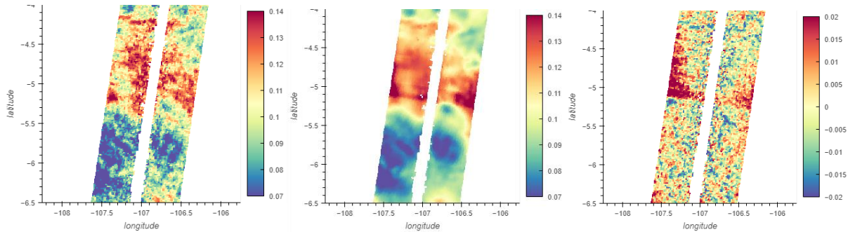
Figure 31: Example of a discontinuity visible in filtered swath. Left: unfiltered ssha variable. Middle: noise filtered ssha. Right: residuals (difference between left and middle)
