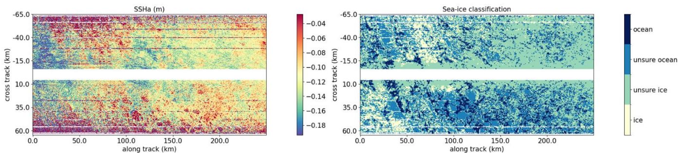
Figure 22: Same as previously, but for C577 P24
