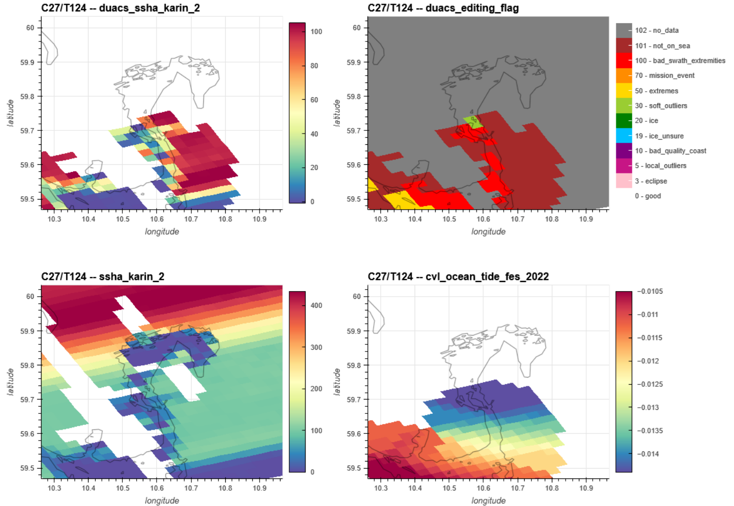
Figure 28: Missing points in L3 are observed when comparing the Sea Level Anomaly from Level-3 (top left) and Level-2 (bottom left) products. The quality flag (top right) indicates missing data in gray that are explained by missing data in the ocean tide correction (bottom right)
