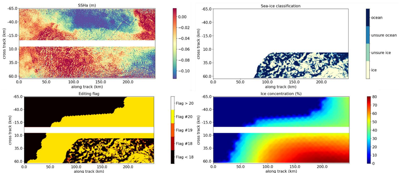
Figure 23: Raw SSHa (top left), sea-ice classification (top right), editing flag (bottom left) and sea ice concentration (bottom right) for KaRIn C500 P2.
