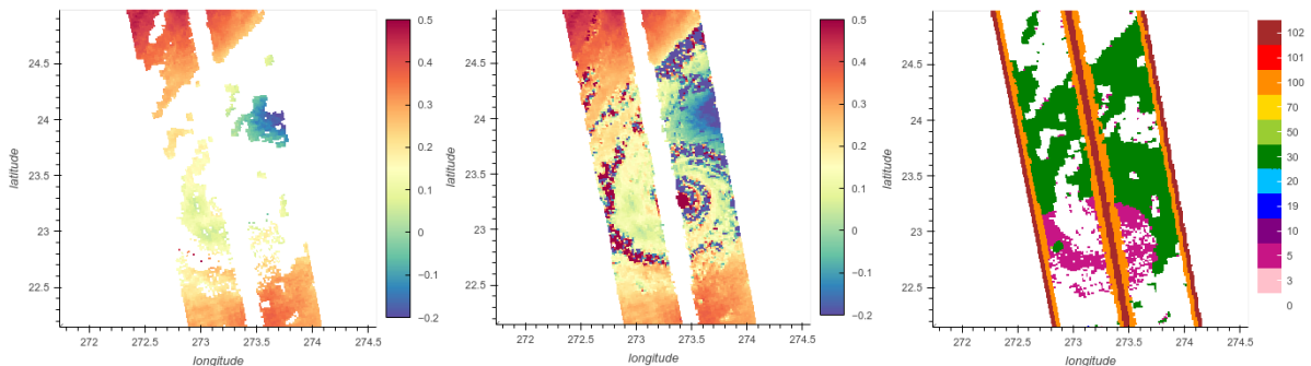
Figure 32: Example of Hurricane Milton. Left: ssha variable i.e. ssha with all flags applied. Middle: ssha with only flags > 30 applied. Right: quality flag
