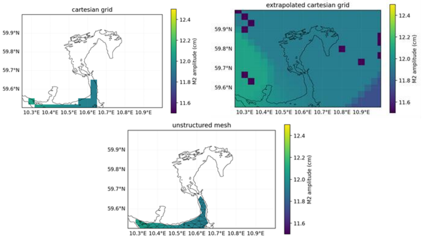
Figure 29: Difference in the definition of the FES2022 source data with (bottom) the original unstructured mesh used in the Level-3 product (top left) the cartesian grid interpolated from the mesh and (top right) the extrapolated cartesian grid used in the Level-2 product
