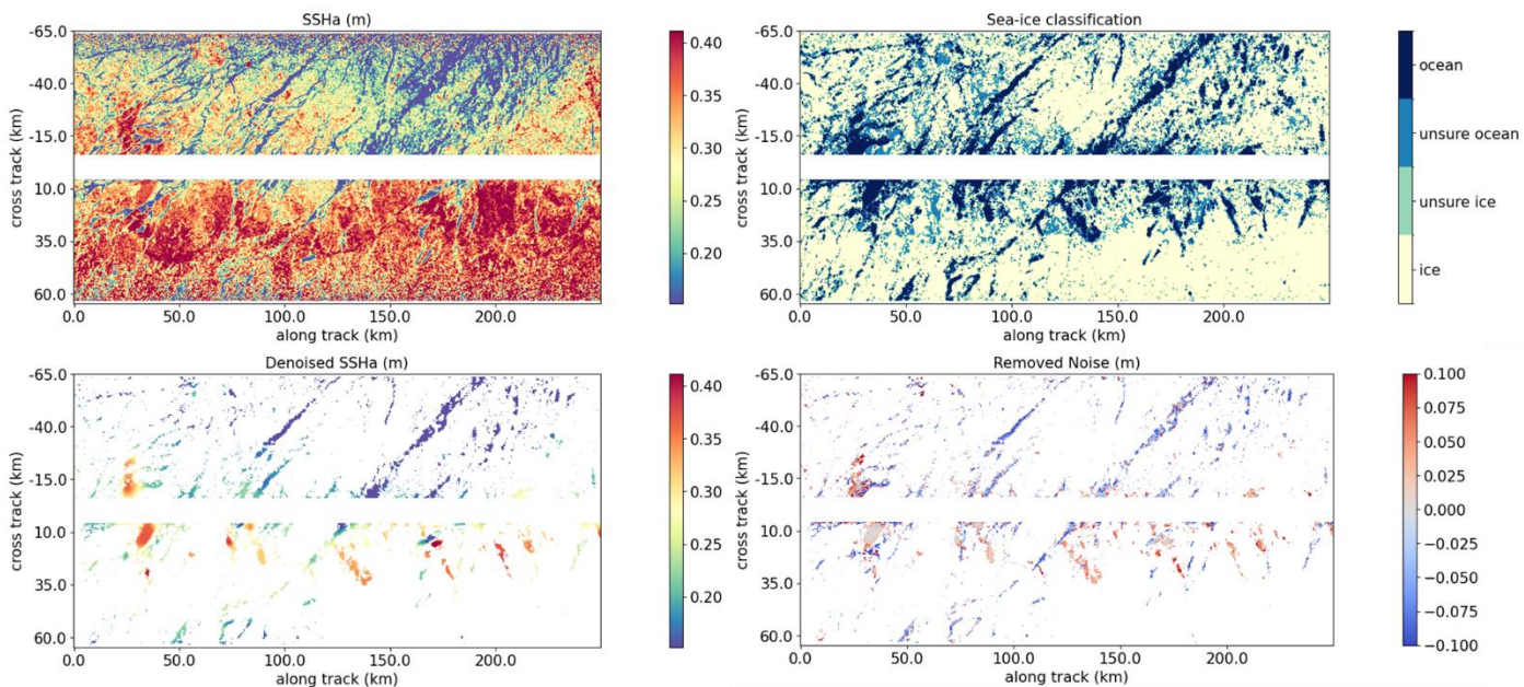
Figure 26: Same as Figure 2524, but for C474 P26
