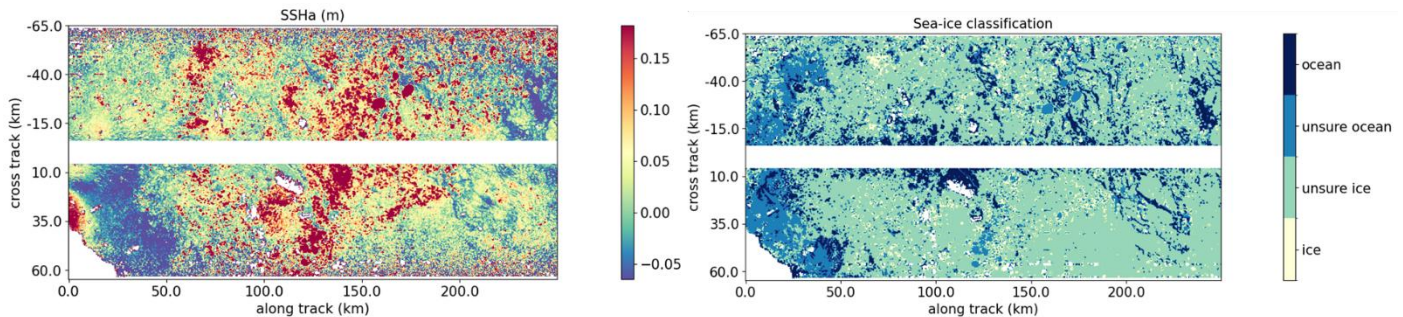
Figure 21: Raw SSHa (left) and sea-ice classification (right) for KaRIn C484 P9
