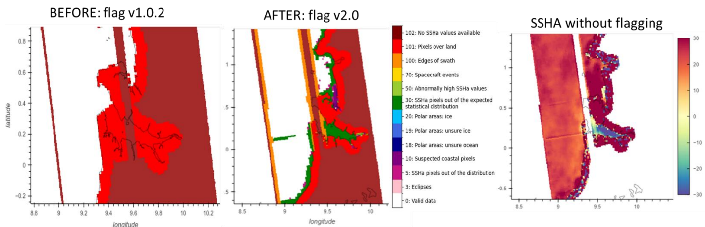
Figure 15: Example of data selection over the Gabon estuary. SSHa before selection (right), after selection in v1.0.2 version (left) and in v2.0 (middle). In that example, main part of the SSHa in the estuary is rejected on statistical criteria on SSHa (flag value 30: SSHa pixels out of the expected statistical distribution)
