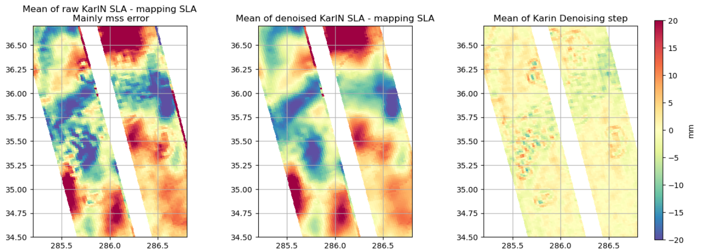
Figure 30: Mean structures remaining on SSHA during the CalVal phase period, before denoising (left) and after denoising (center). In this example, the mean content of the noise removed by the denoising processing (right) is dominated small scale static structures that are not corrected by the MSS used.
