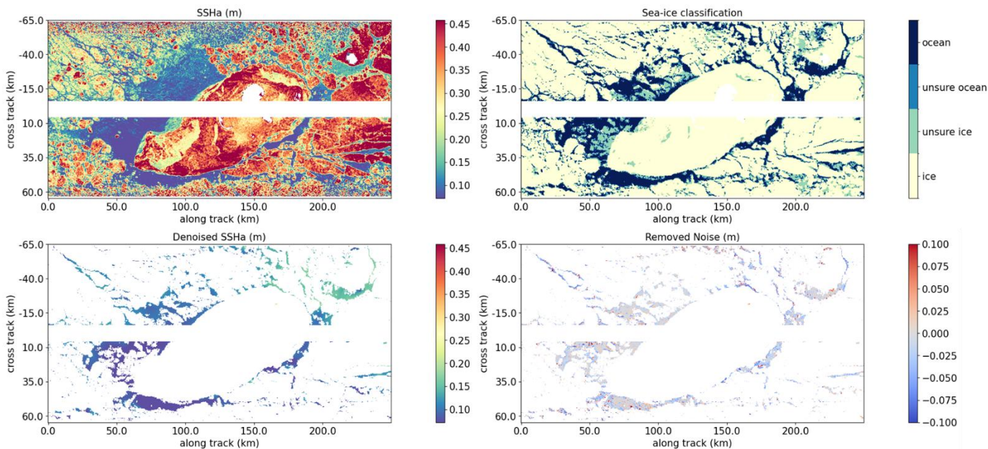
Figure 25: Raw SSHa (top left), sea-ice classification (top right), Denoised SSHa over ocean (bottom left) and Noise removed by denoising processing (bottom right) for KaRIn C507 P1
