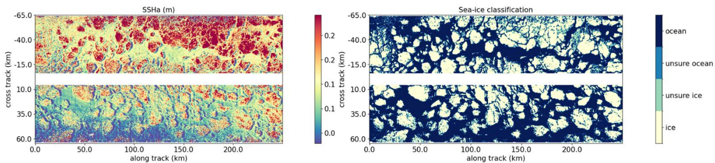
Figure 24: Same as Figure 2120, but for C474 P5
