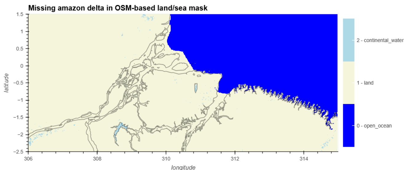
Figure 27: OpenStreetMap-derived land sea mask shows may classify some estuaries a land (yellow)
