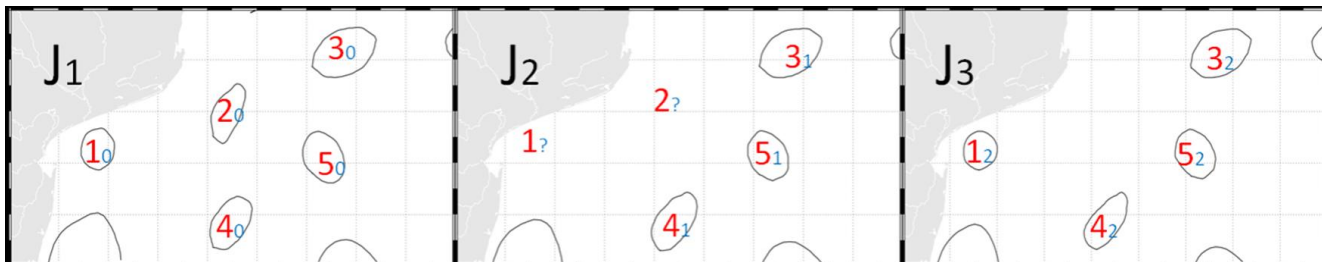
Figure 5: procedure to detect a tracking on a particular eddy: the eddy number 1 is kept because an association has been found on map D+3, contrary to the eddy number 2 where no association is found on the last map.
