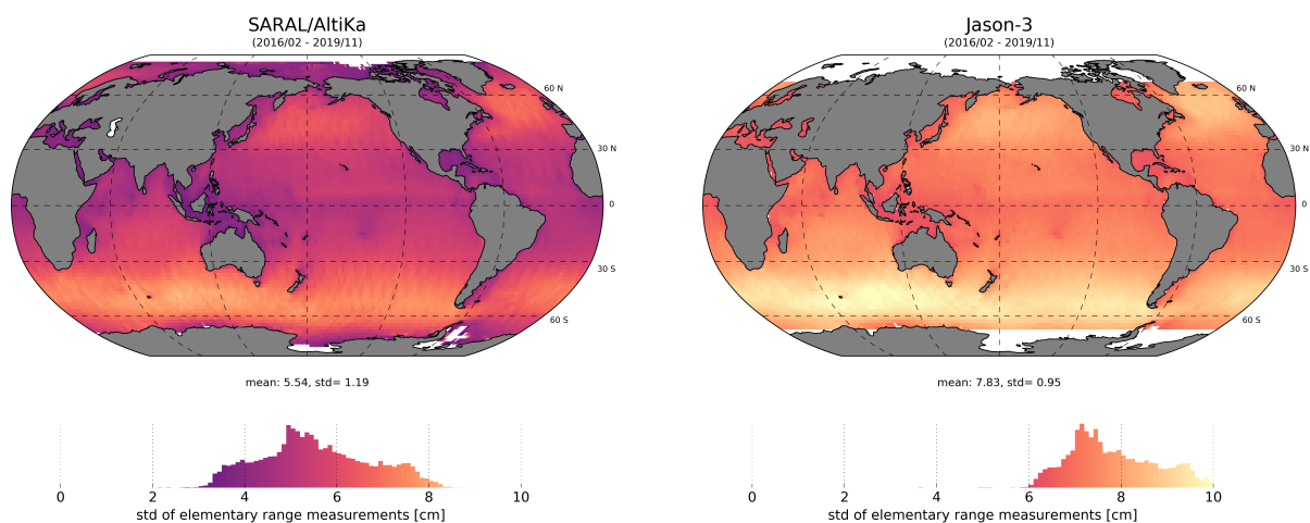
Figure 28: Average map of rms of SARAL/AltiKa elementary 40 Hz range measurements (left) and Jason-3 elementary 20 Hz range measurement (right).
