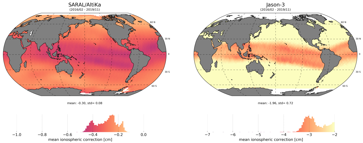
Figure 41: Average map of ionosphere correction for SARAL/Altika (GIM, left) and Jason-3 (filtered dual-frequency ionosphere correction, right). Note that color scales are different for SARAL/Altika and Jason-3.
