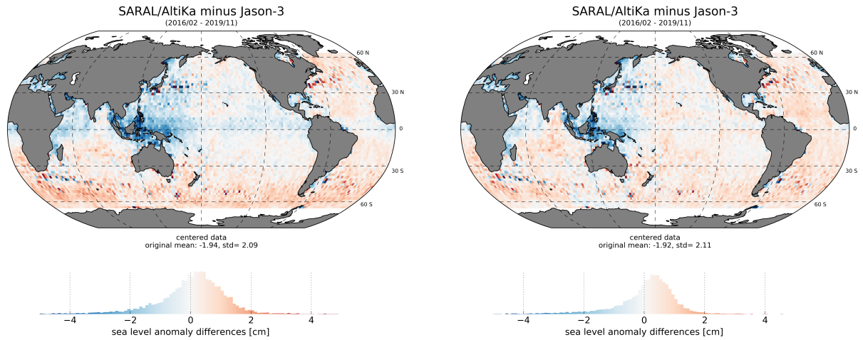
Figure 64: Map of mean SLA differences between SARAL/AltiKa and Jason-3 using (left) the radiometer and (right) model wet tropospheric correction.
