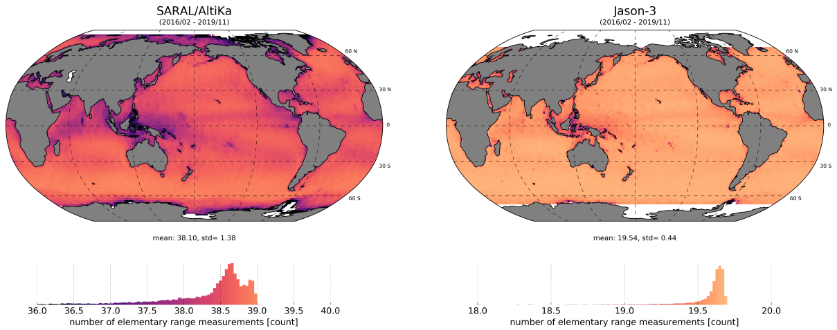
Figure 26: Average map of number of SARAL/AltiKa elementary 40 Hz range measurements (left) and Jason-3 elementary 20 Hz range measurements (right).
