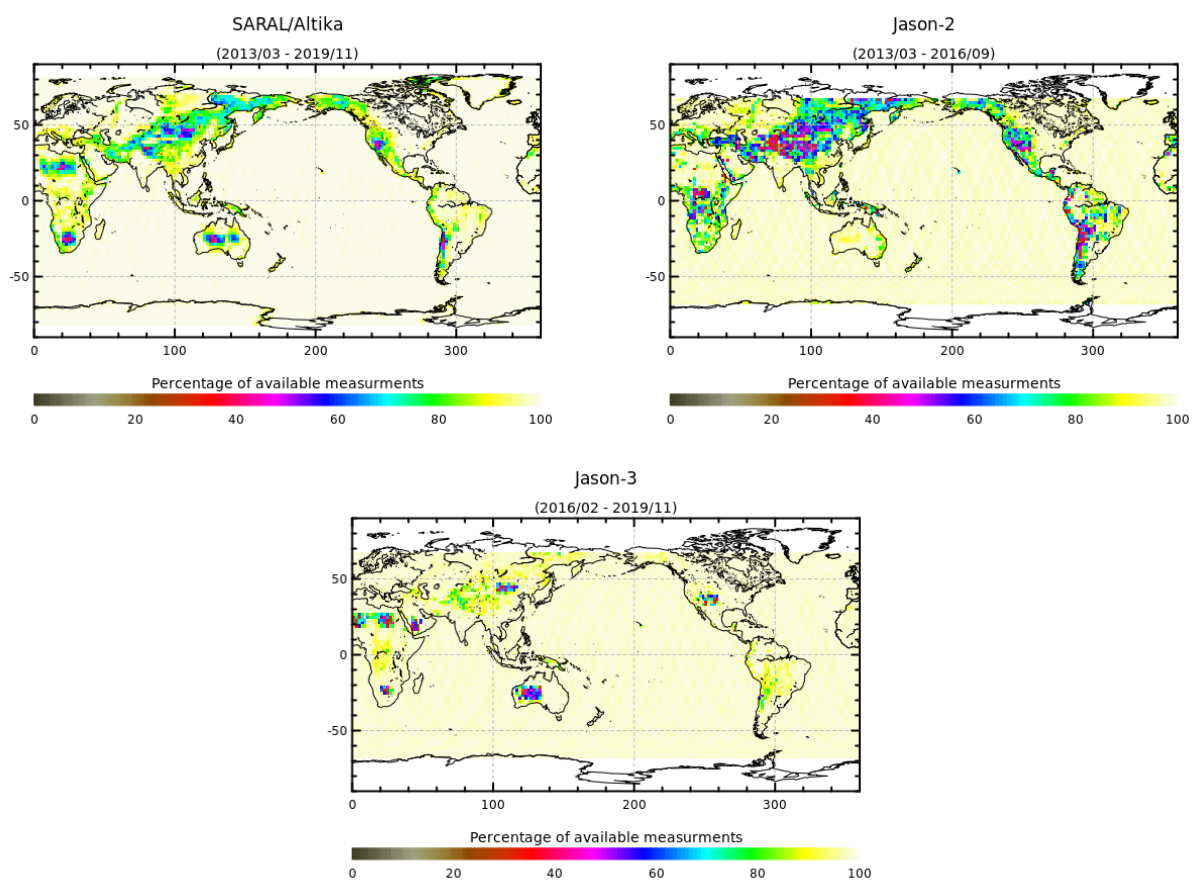
Figure 2: Map of the percentage of available measurements over land for SARAL/Altika (left) Jason-2 (right) and Jason-3 (bottom).
