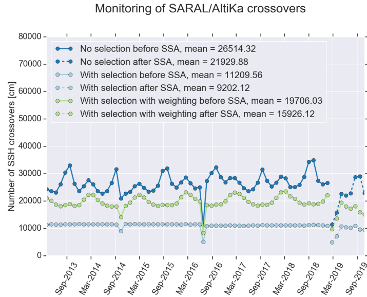
Figure 53: Monitoring of SARAL/AltiKa's number of valid crossovers per cycle.
