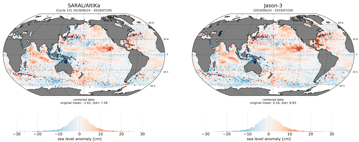
Figure 63: SLA map for SARAL/AltiKa 131 cycle using the radiometer wet tropospheric correction (left) from SARAL/AltiKa data, and (right) from Jason-3 data over the same period.
