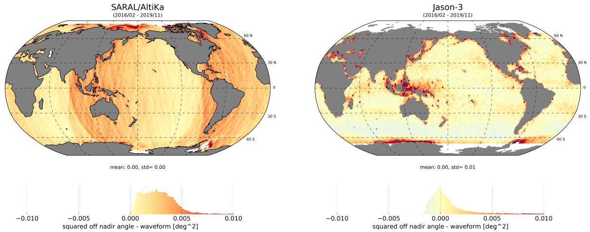
Figure 30: Average map of off-nadir angle from waveforms for SARAL/AltiKa (left) and Jason-3 (right).
