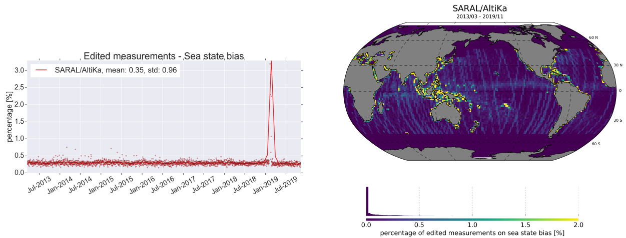
Figure 19: Percentage of edited measurements by sea state bias criterion. [top] monitoring for GDR data and [bottom] map since the beginning of the mission (cycles 1 to 134). Dots are daily averages while solid lines correspond to cycle averages.
