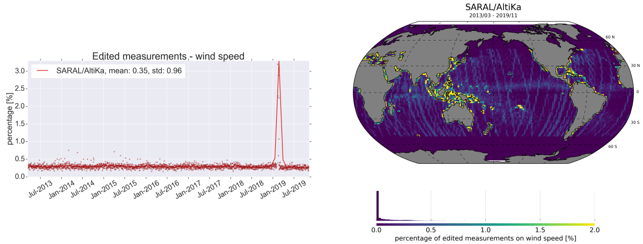
Figure 20: Percentage of edited measurements by wind speed criterion. [top] monitoring for GDR data and [bottom] map since the beginning of the mission (cycles 1 to 134). Dots are daily averages while solid lines correspond to cycle averages.
