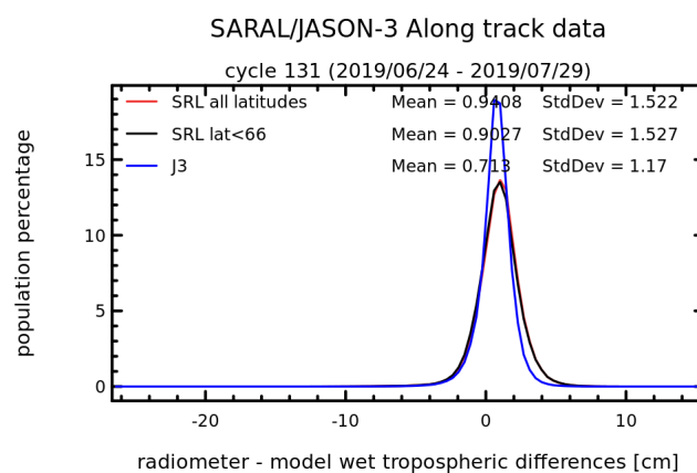
Figure 46: Histogram (of along-track data) of radiometer minus ECMWF model wet troposphere correction between SARAL/AltiKa and Jason-3 computed for SARAL/AltiKa cycle 131.
