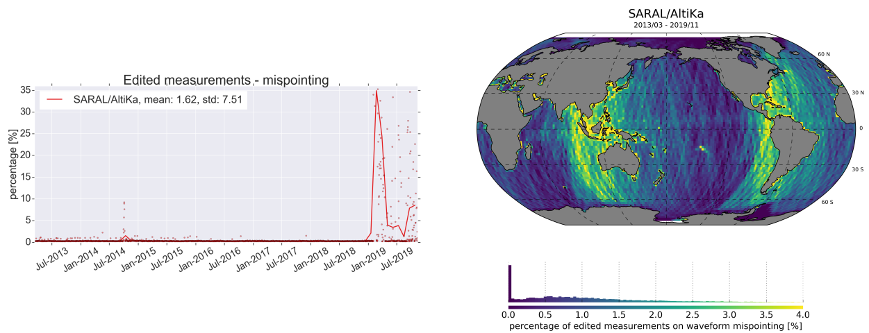
Figure 18: Percentage of edited measurements by square off-nadir angle criterion. [top] monitoring for GDR data and [bottom] map since the beginning of the mission (cycles 1 to 134). Dots are daily averages while solid lines correspond to cycle averages.
