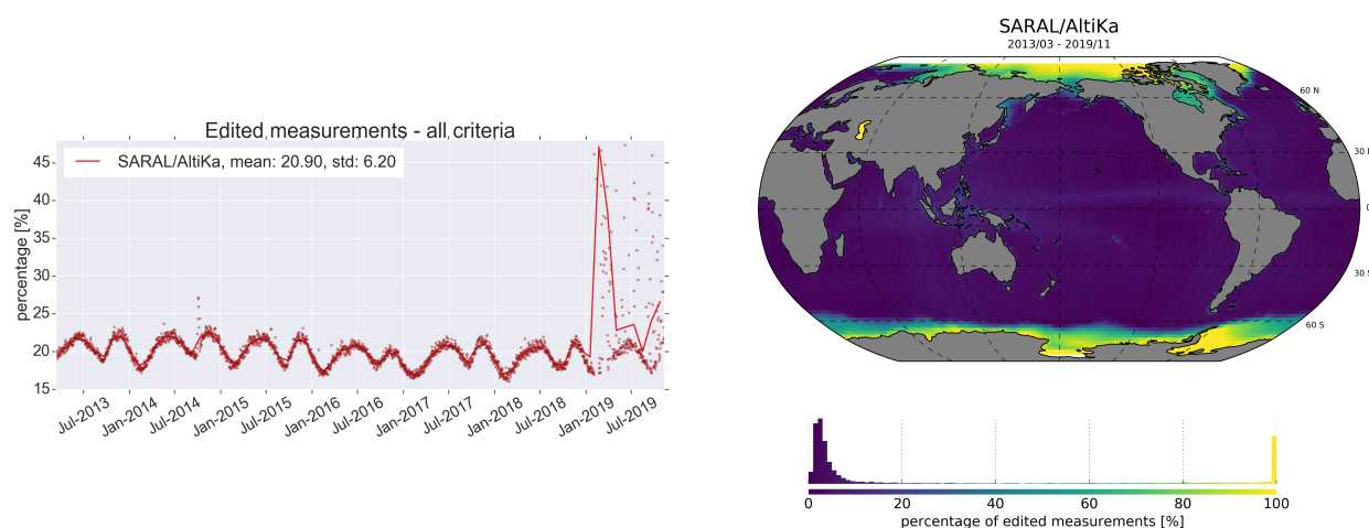
Figure 5: Total percentage of SARAL/AltiKa edited measurements. [top] monitoring for GDR data and [bottom] map since the beginning of mission (cycles 1 to 134). Dots are daily averages while solid lines correspond to cycle averages.
