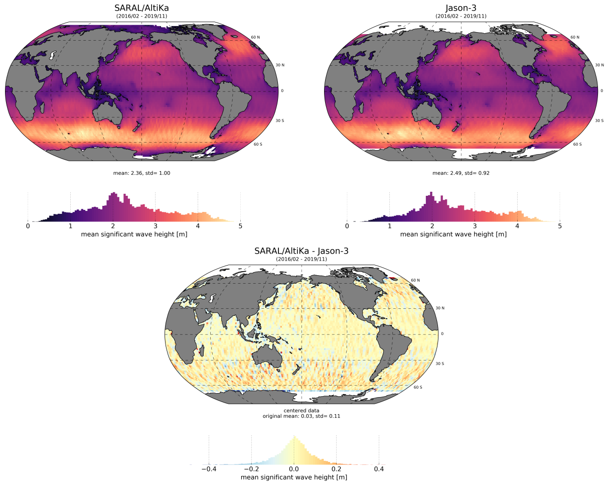
Figure 38: Average map of significant wave height for SARAL/AltiKa (left) and Jason-3 (right). Difference map of SARAL/AltiKa and Jason-3 significant wave height.
