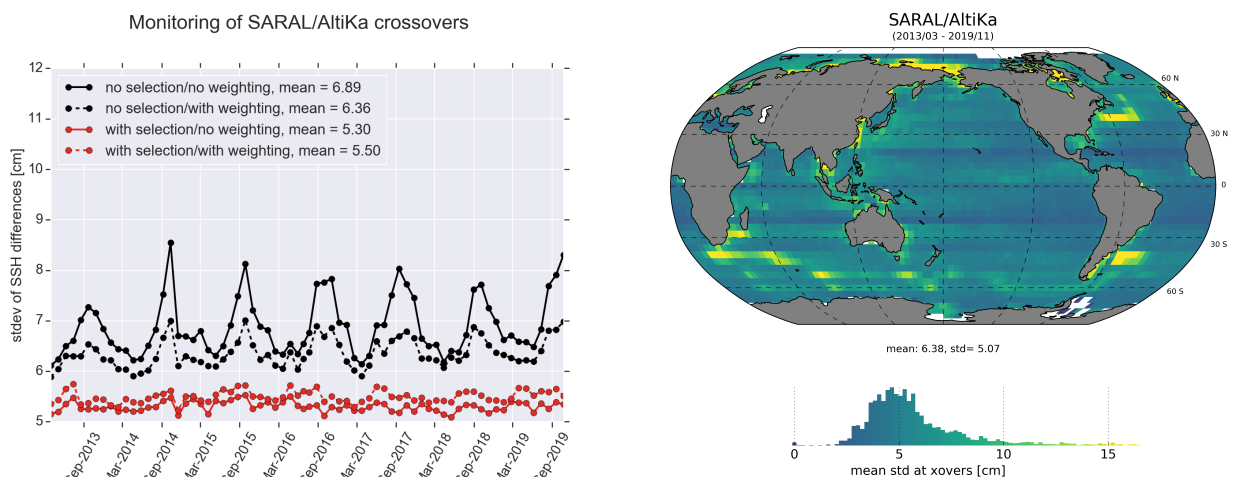
Figure 59: Cycle by cycle standard deviation of SSH crossover differences for SARAL/AltiKa using different selections and averaging methods (left) and map of standard deviation at crossover points. In both cases the radiometer wet tropospheric correction is used.
