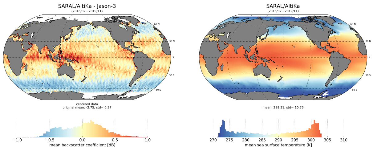
Figure 35: Difference map of SARAL/AltiKa and Jason-3 backscattering coefficient (left) and map of sea surface temperature (right) .
