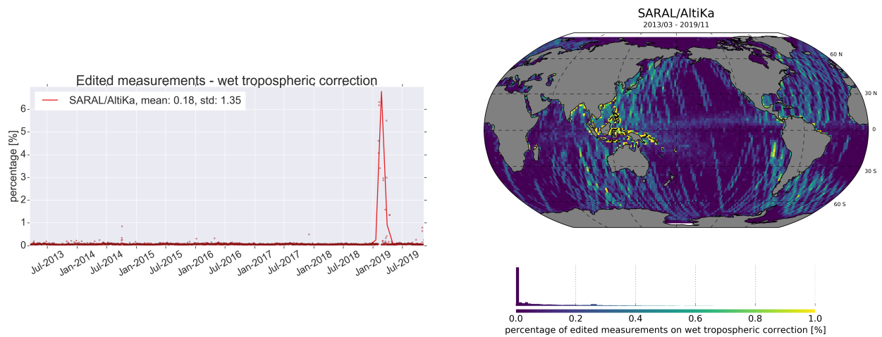
Figure 17: Percentage of edited measurements due to radiometer wet tropospheric correction out of thresholds. [top] monitoring for GDR data and [bottom] map since the beginning of mission (cycles 1 to 134). Dots are daily averages while solid lines correspond to cycle averages.
