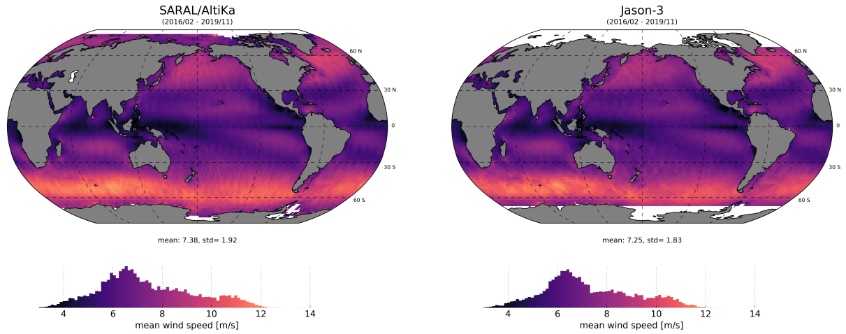
Figure 48: Average map of altimeter wind speed for SARAL/AltiKa (left) and Jason-3 (right).
