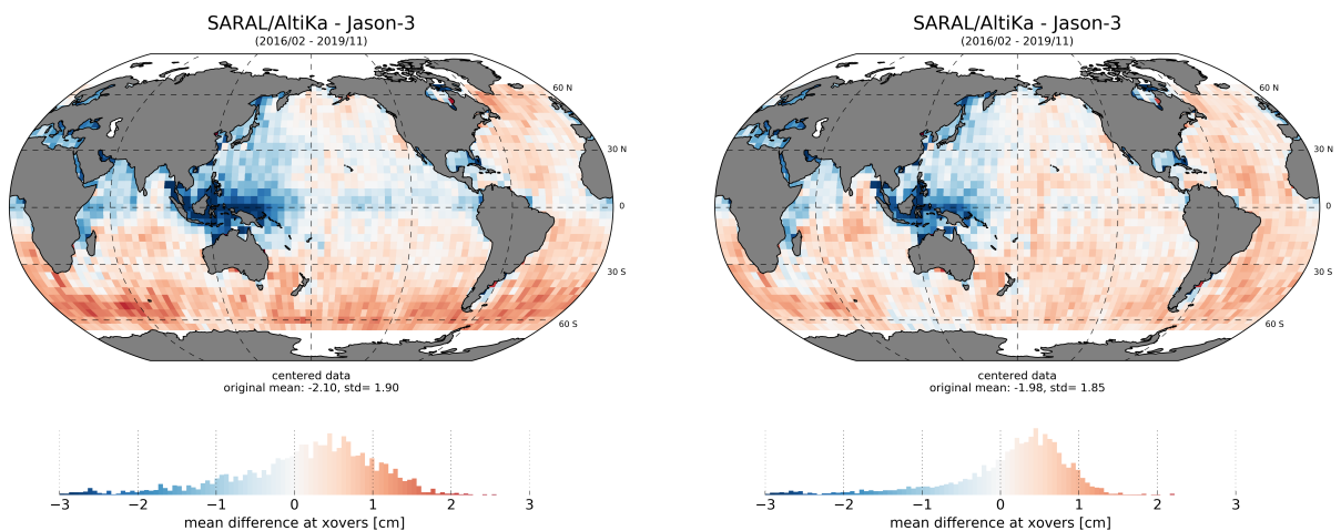
Figure 58: Map of mean of SSH crossovers differences between SARAL/AltiKa and Jason-3 using the radiometer wet tropospheric correction (left) or the ECMWF model wet troposphere correction (right) for both missions. The maps are centered around the mean.
