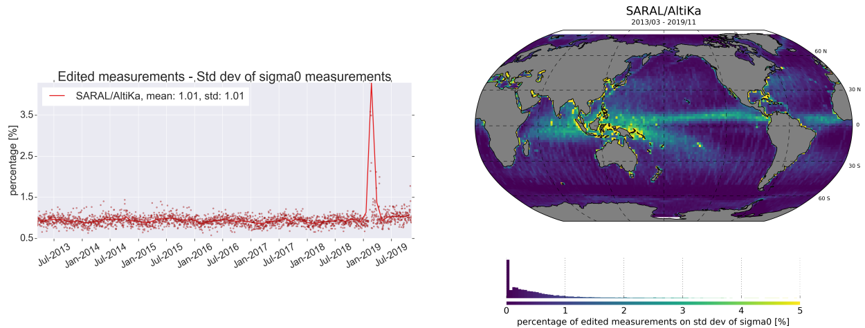
Figure 16: Percentage of edited measurements by 40 Hz Sigma0 standard deviation criterion. [top] monitoring for GDR data and [bottom] map since the beginning of mission (cycles 1 to 134). Dots are daily averages while solid lines correspond to cycle averages.
