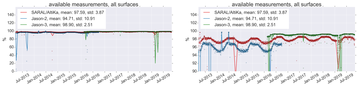
Figure 1: Percentage of available measurements over all surfaces for SARAL/AltiKa, Jason-2 and Jason-3. Dots are daily averages while solid lines correspond to cycle averages.
