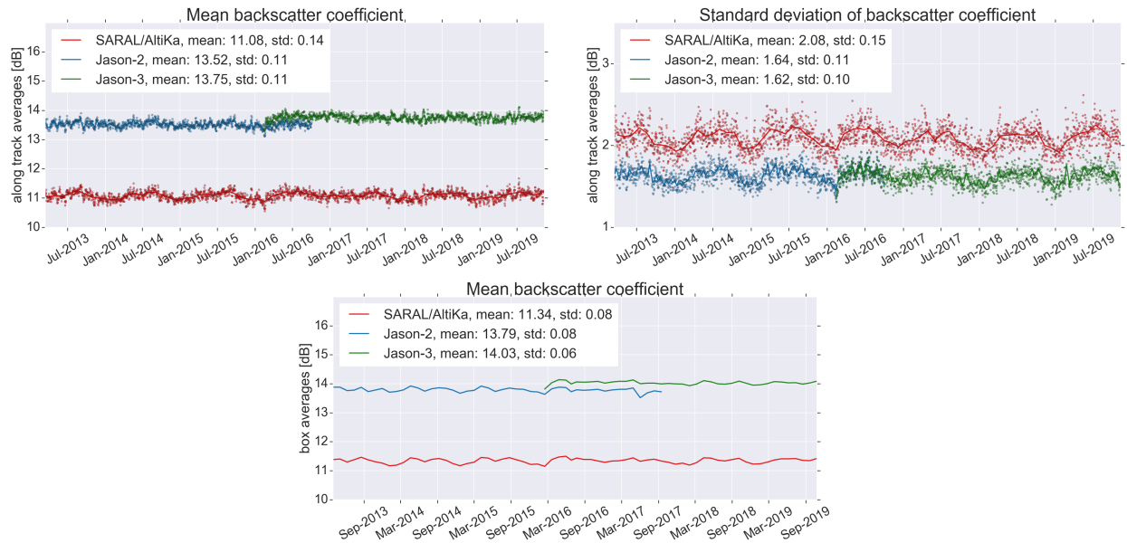
Figure 33: Daily monitoring of mean (top) and standard deviation (center) of SARAL/AltiKa, Jason-2 and Jason-3 backscattering coefficient and cyclic monitoring of box averaged latitude weighted mean (bottom). Dots are daily averages while solid lines correspond to cycle averages.
