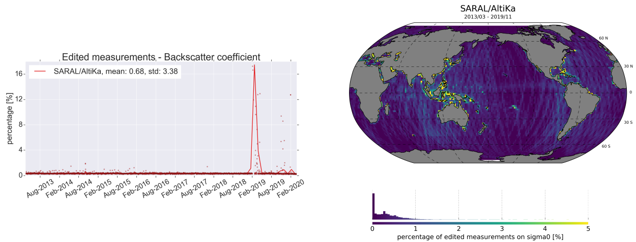
Figure 14: Percentage of edited measurements by Sigma0 criterion. [top] monitoring for GDR data and [bottom] map since the beginning of mission (cycles 1 to 134). Dots are daily averages while solid lines correspond to cycle averages.
