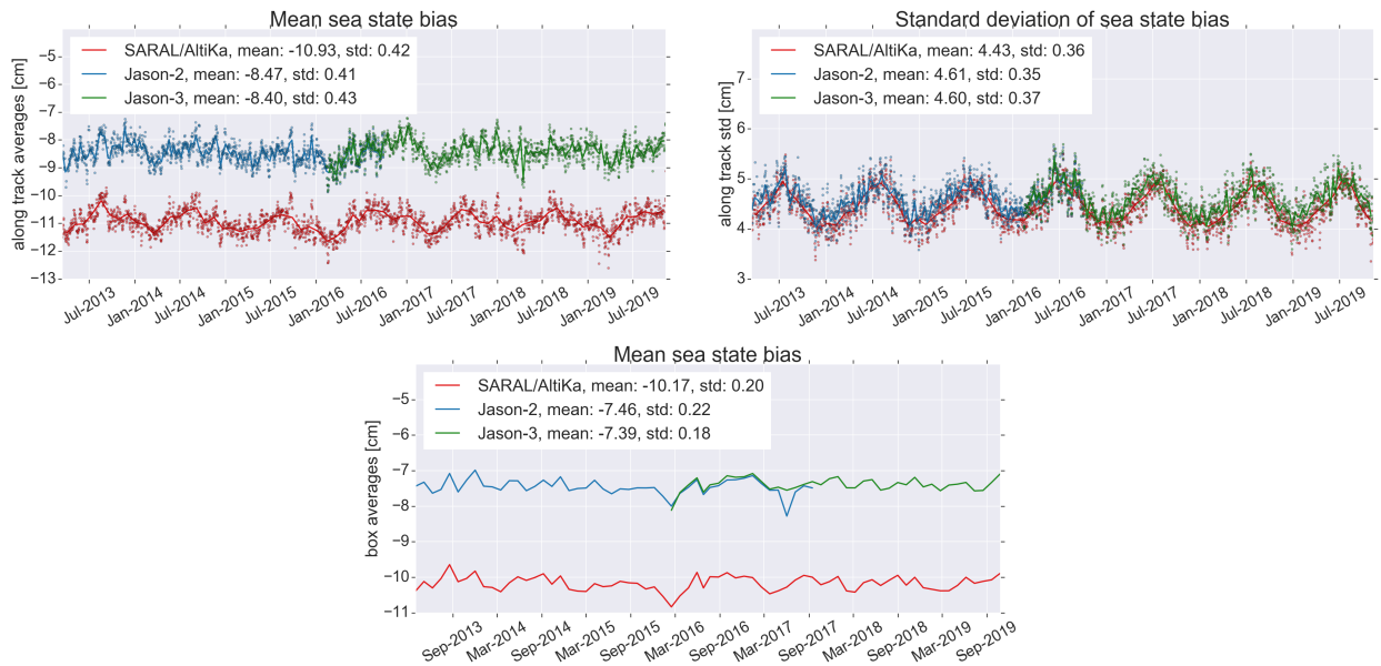
Figure 50: Monitoring of mean (top) and standard deviation (center) of (along-track) sea state bias of SARAL/AltiKa Jason-2 and Jason-3. Cycle per cycle monitoring of latitude weighted box averaged mean (bottom). Dots are daily averages while solid lines correspond to cycle averages.
