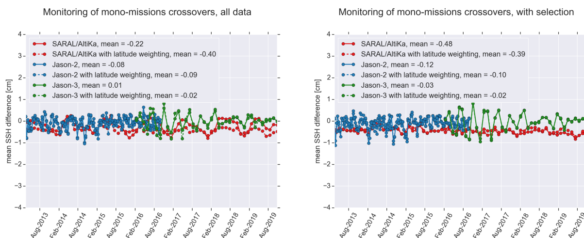
Figure 56: Cycle per cycle monitoring of ascending/descending SSH differences at mono-mission crossovers for SARAL/AltiKa Jason-2 and Jason-3 for Saral cycles 1 to 134.
