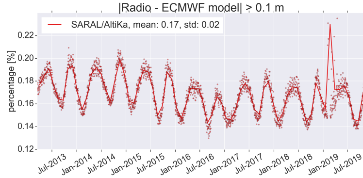
Figure 7: Percentage of measurements for which the absolute value of the difference between the model wet tropospheric correction and the dual frequency wet tropospheric correction exceeds 0,1m . Dots are daily averages while solid lines correspond to cycle averages.
