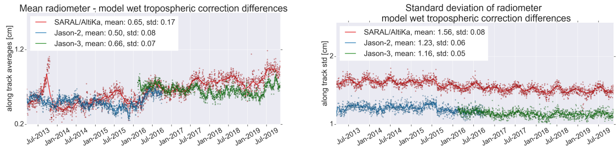
Figure 44: Monitoring of mean and standard deviation of radiometer minus model wet troposphere correction differences for SARAL/AltiKa Jason-2 and Jason-3. Dots are daily averages while solid lines correspond to cycle averages.
