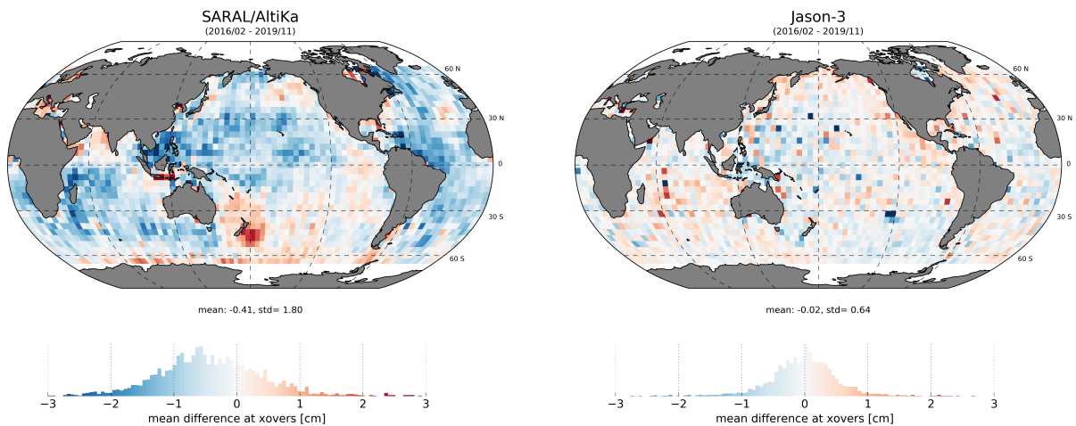
Figure 55: Map of mean of SSH crossovers differences for [left] SARAL/AltiKa and [right] Jason-3.
