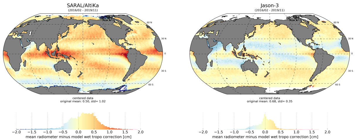
Figure 45: Average map of radiometer minus ECMWF model wet troposphere correction for SARAL/AltiKa (left) and Jason-3 (right).
