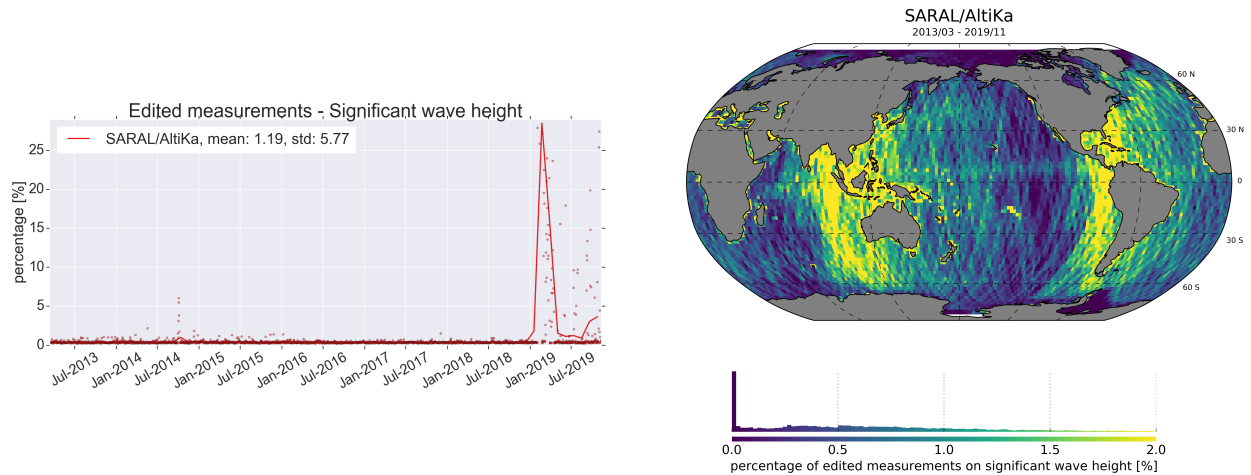
Figure 13: Percentage of edited measurements by SWH criterion. [top] monitoring for GDR data and [botom] map since the beginning of mission (cycles 1 to 134). Dots are daily averages while solid lines correspond to cycle averages.
