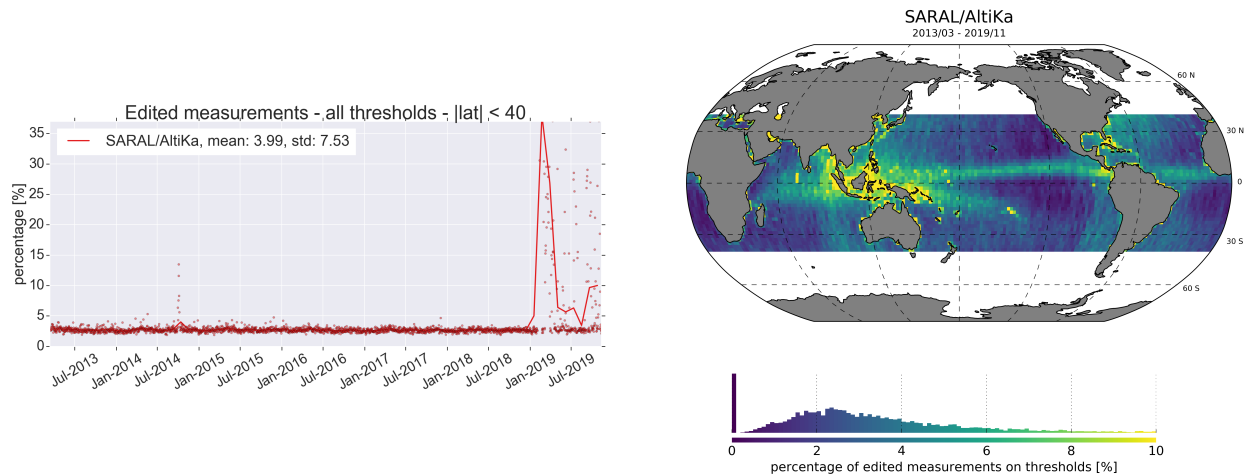
Figure 10: Percentage of edited measurements on all thresholds combined, for |\text{latitudes}| < 40^\circ . [top] monitoring for GDR data and [bottom] map since the beginning of mission (cycles 1 to 134). Dots are daily averages while solid lines correspond to cycle averages.
