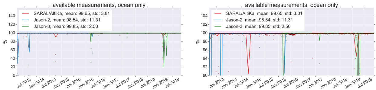
Figure 3: Percentage of available measurements over ocean for SARAL/AltiKa Jason-2 and Jason-3. Dots are daily averages while solid lines correspond to cycle averages.
