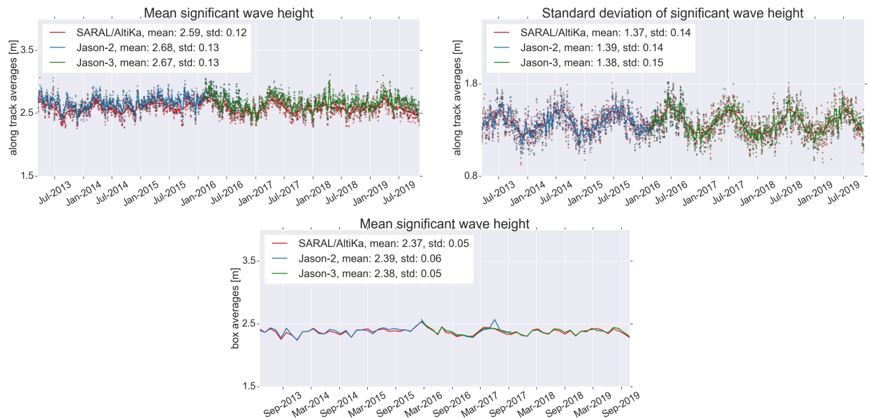
Figure 37: Daily monitoring of mean (top) and standard deviation (center) of significant wave height for SARAL/AltiKa, Jason-2 and Jason-3 and cycle per cycle monitoring of box averaged latitude weighted mean (bottom). Dots are daily averages while solid lines correspond to cycle averages.
