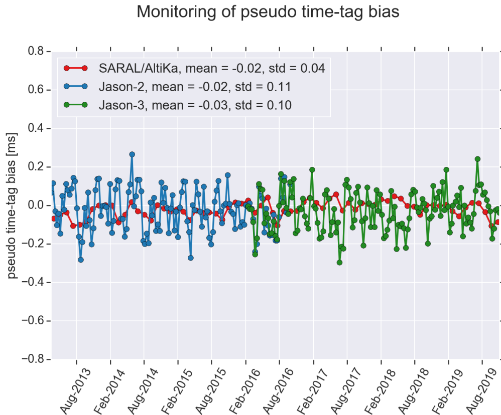
Figure 62: Cycle per cycle monitoring of the pseudo time tag bias for SARAL/AltiKa and Jason-2
