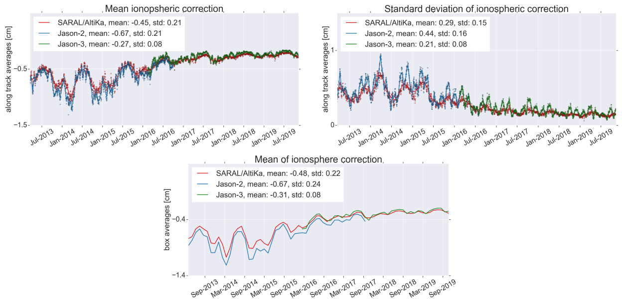
Figure 40: Daily monitoring of mean and standard deviation ionosphere correction for SARAL/AltiKa (GIM), Jason-2 and Jason-3 (filtered dual-frequency ionosphere correction with scale factor 0.14418 for mean computation). Dots are daily averages while solid lines correspond to cycle averages.
