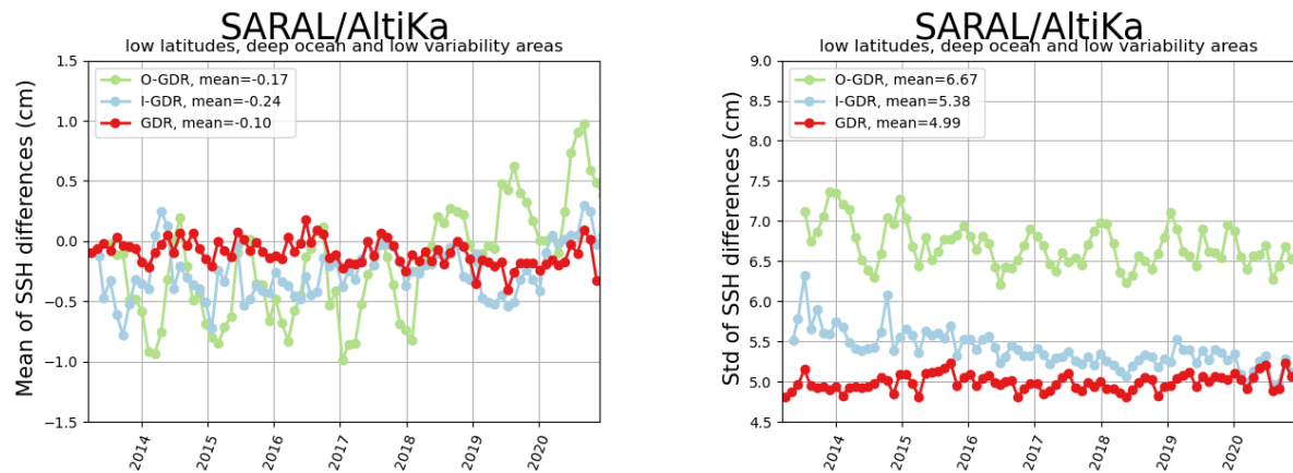
Figure 61: Cycle per cycle monitoring of mean and standard deviation of SSH crossover differences for SARAL/AltiKa using radiometer wet troposphere correction and geographical selection ( |\text{latitude}| < 50^\circ , bathymetry < -1000 m and ocean variability < 20 cm rms).
