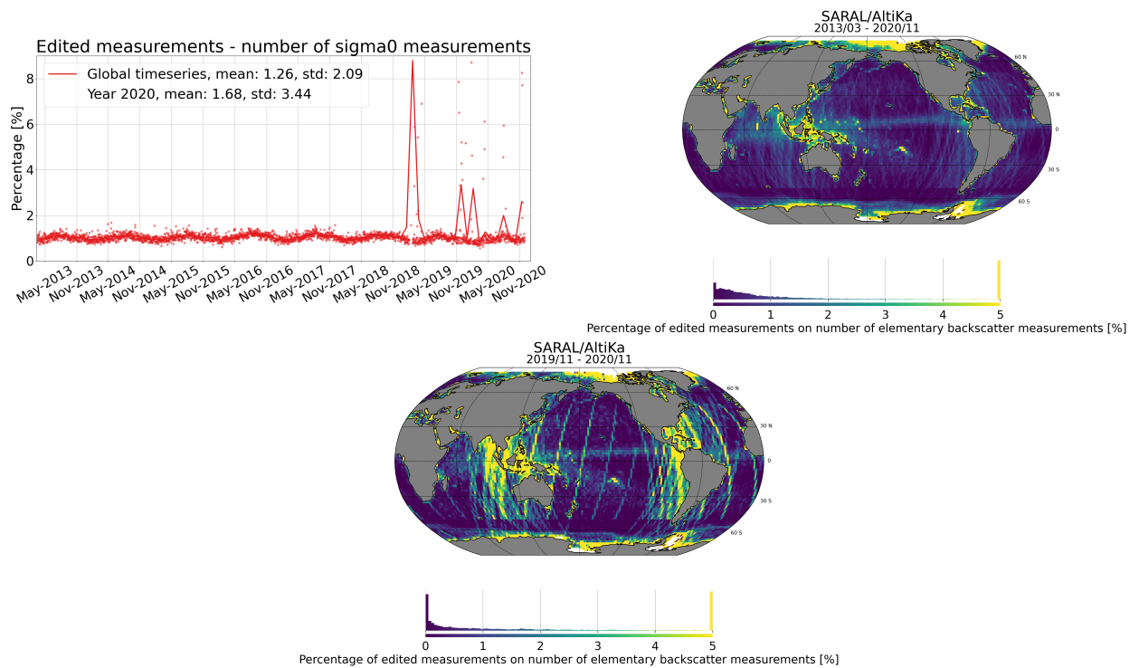
Figure 15: Percentage of edited measurements by number of high rate backscatter coefficient measurements. [left] monitoring for GDR data, [right] map since the beginning of mission (cycles 1 to 145) and [bottom] map over the past year (2020). Dots are daily averages while solid lines correspond to cycle averages.
