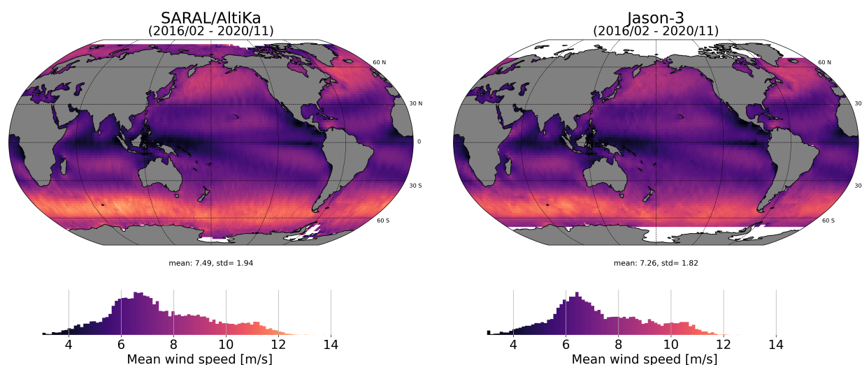
Figure 48: Average map of altimeter wind speed for SARAL/AltiKa (left) and Jason-3 (right).
