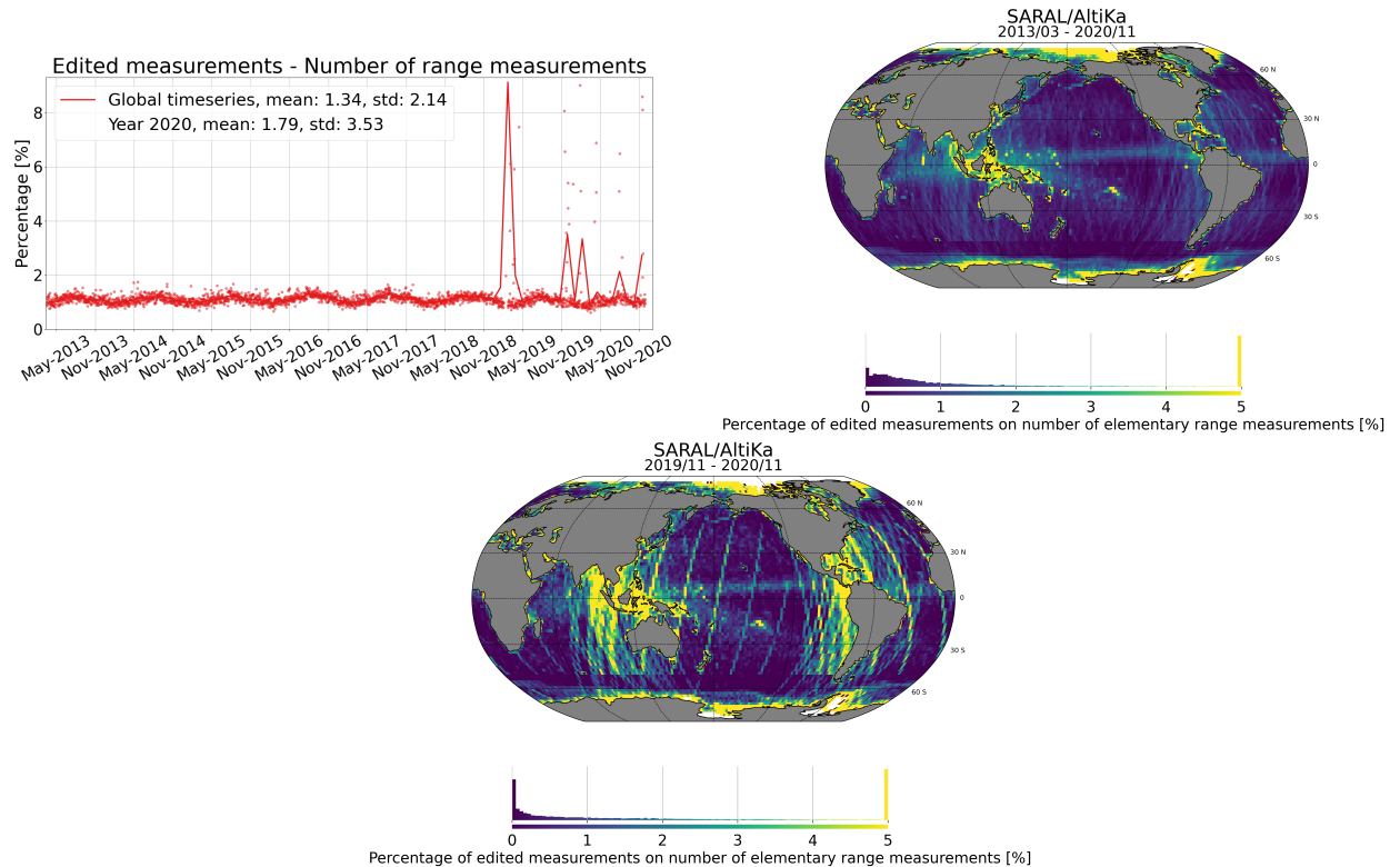
Figure 11: Percentage of edited measurements on the number of 40-Hz measurements criterion. [left] monitoring for GDR data, [right] map since the beginning of mission (cycles 1 to 145) and [bottom] map over the past year (2020). Dots are daily averages while solid lines correspond to cycle averages.
