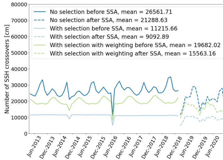
Figure 53: Monitoring of SARAL/AltiKa's number of valid crossovers per cycle.
