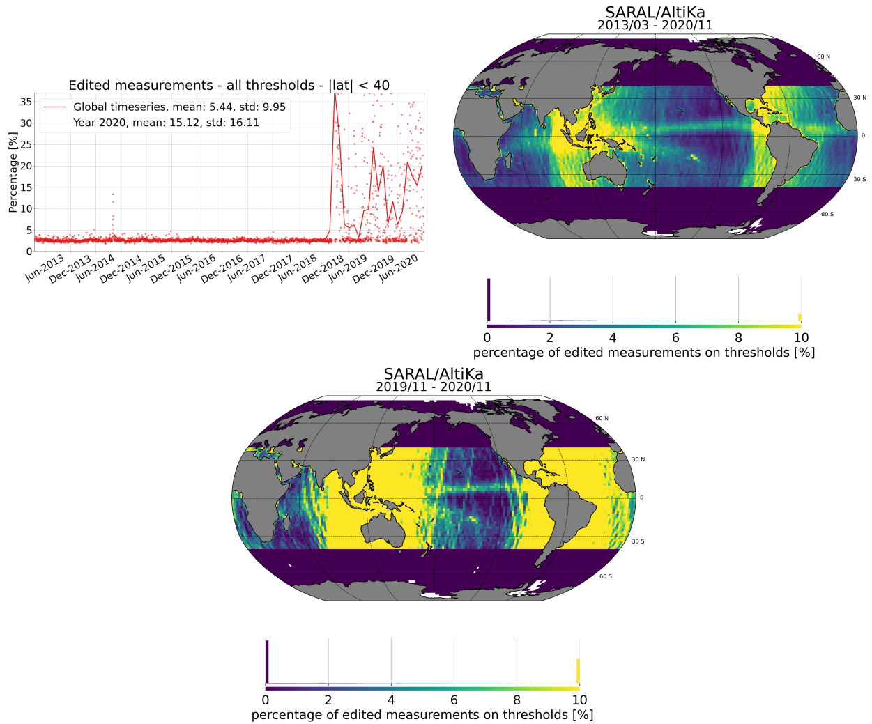
Figure 10: Percentage of edited measurements on all thresholds combined, for |latitudes| < 40^\circ . [left] monitoring for GDR data, [right] map since the beginning of mission (cycles 1 to 145) and [bottom] map over the past year (2020). Dots are daily averages while solid lines correspond to cycle averages.
