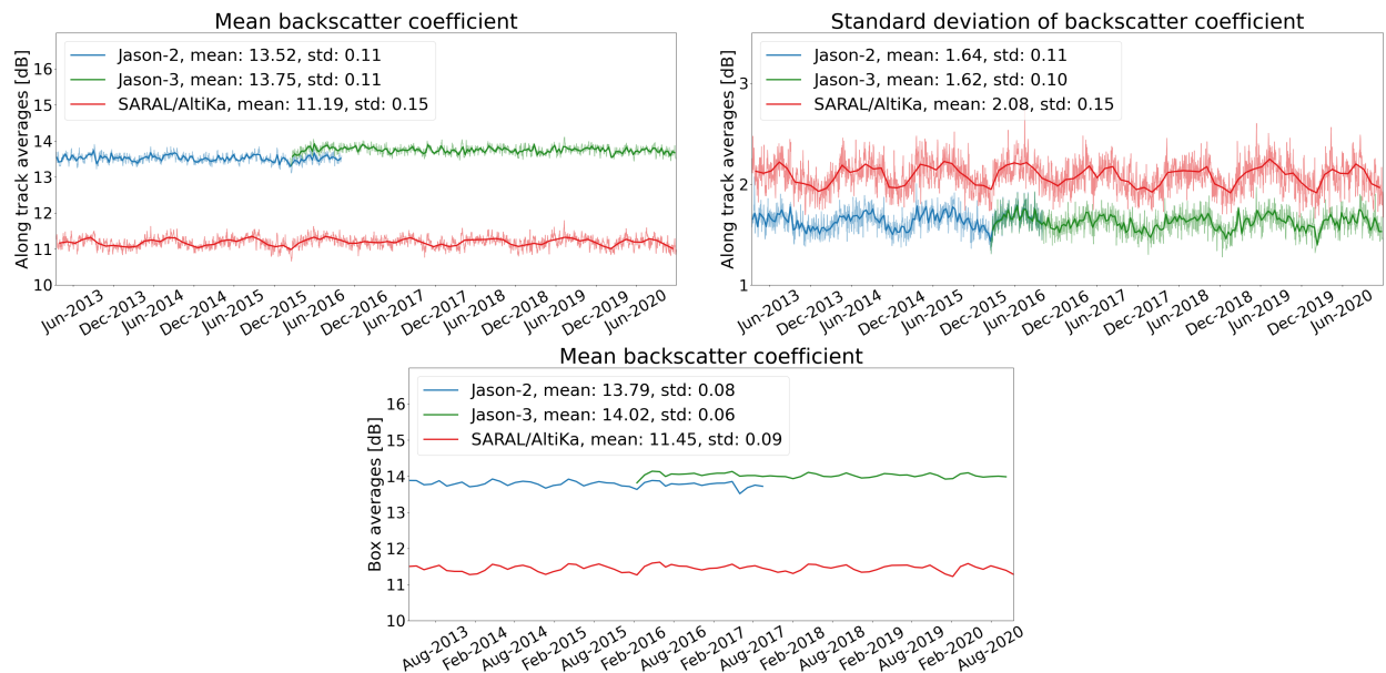
Figure 33: Daily monitoring of mean (top) and standard deviation (center) of SARAL/AltiKa, Jason-2 and Jason-3 backscattering coefficient and cyclic monitoring of box averaged latitude weighted mean (bottom). Dots are daily averages while solid lines correspond to cycle averages.
