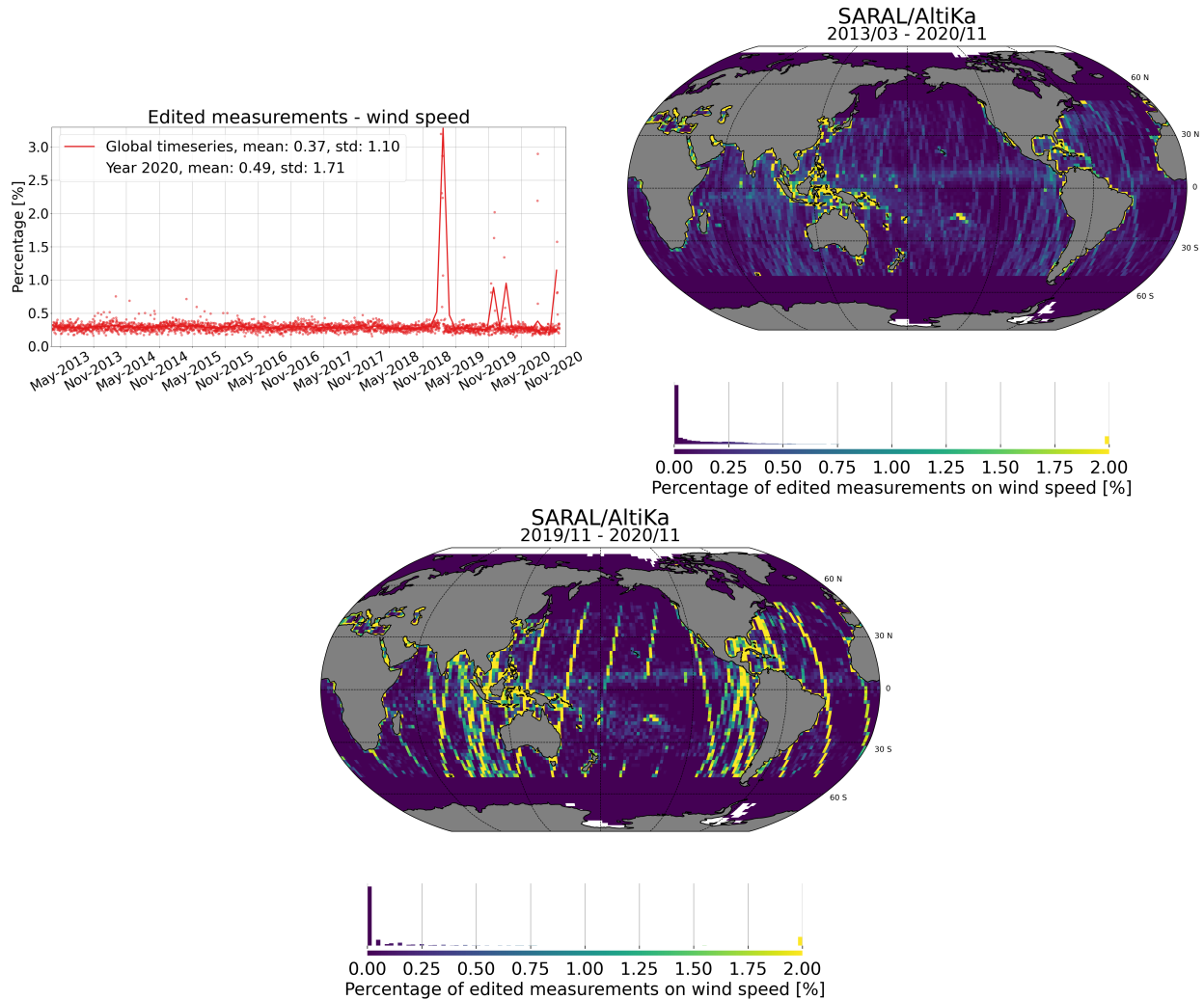
Figure 20: Percentage of edited measurements by wind speed criterion. [left] monitoring for GDR data, [right] map since the beginning of the mission (cycles 1 to 145) and [bottom] map over the past year (2020). Dots are daily averages while solid lines correspond to cycle averages.
