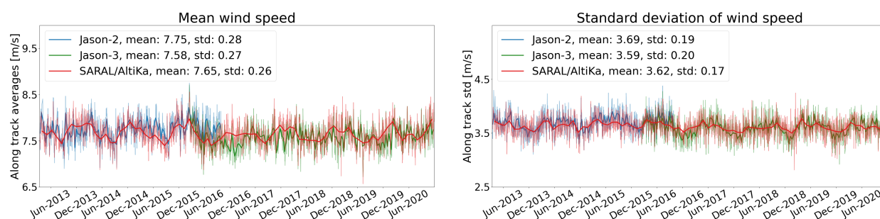
Figure 47: Monitoring of mean and standard deviation of altimeter wind speed for SARAL/AltiKa and Jason-3. Dots are daily averages while solid lines correspond to cycle averages.
