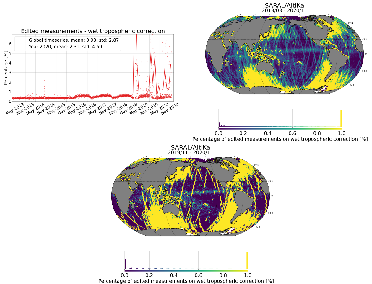
Figure 17: Percentage of edited measurements due to radiometer wet tropospheric correction out of thresholds. [left] monitoring for GDR data, [right] map since the beginning of mission (cycles 1 to 145) and [bottom] map over the past year (2020). Dots are daily averages while solid lines correspond to cycle averages.
