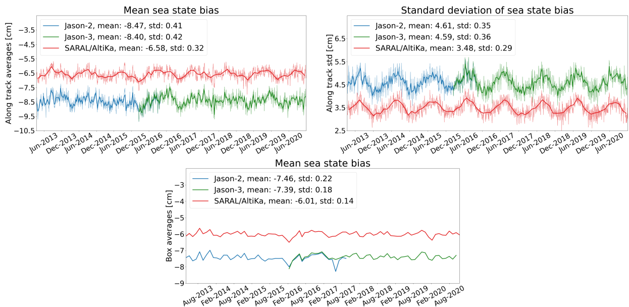
Figure 50: Monitoring of mean (top) and standard deviation (center) of (along-track) sea state bias of SARAL/AltiKa Jason-2 and Jason-3. Cycle per cycle monitoring of latitude weighted box averaged mean (bottom). Dots are daily averages while solid lines correspond to cycle averages.
