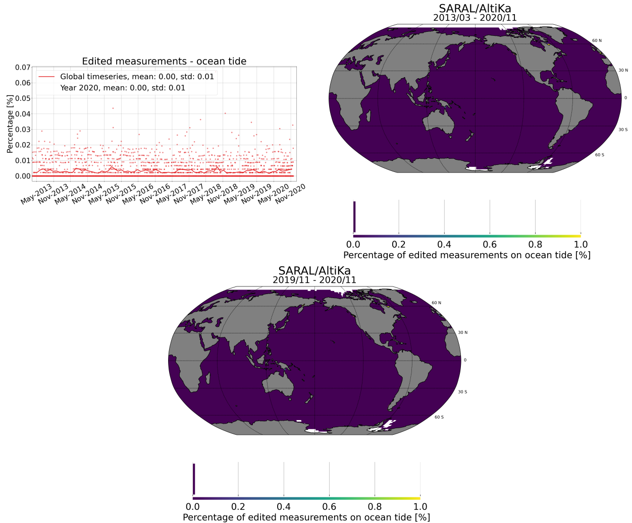
Figure 21: Percentage of edited measurements by ocean tide criterion. [top] monitoring for GDR data, [right] map since the beginning of the mission (cycles 1 to 145) and [bottom] map over the past year (2020). Dots are daily averages while solid lines correspond to cycle averages.
