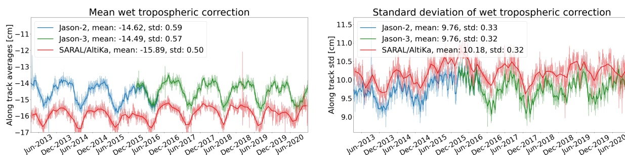
Figure 43: Monitoring of mean and standard deviation of radiometer wet troposphere correction for SARAL/AltiKa (red) Jason-2 (blue) and Jason-3 (green). Dots are daily averages while solid lines correspond to cycle averages.
