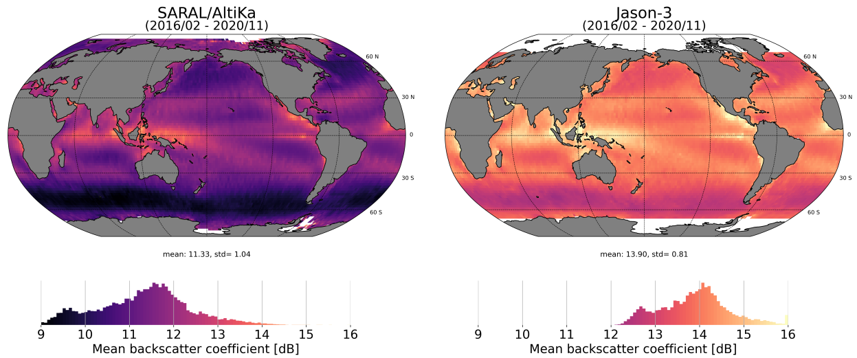
Figure 34: Average map of backscattering coefficient for SARAL/AltiKa (left) and Jason-3 (right).
