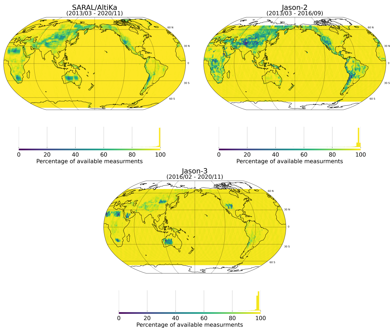
Figure 2: Map of the percentage of available measurements over land for SARAL/Altika (left) Jason-2 (right) and Jason-3 (bottom).
