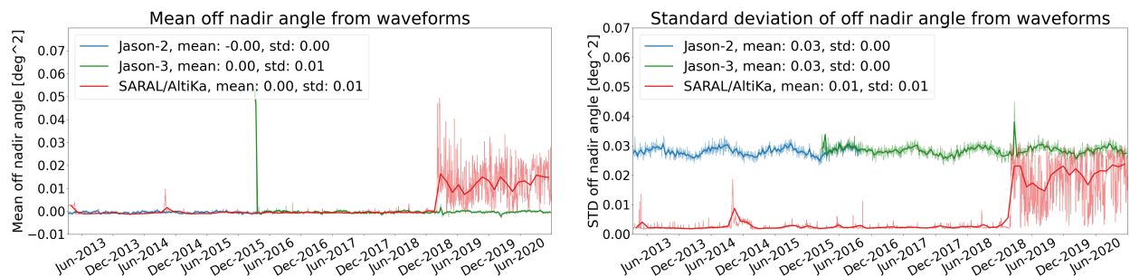
Figure 29: Monitoring of mean (left) and standard deviation (right) of , Jason-2 and Jason-3 off-nadir angle from waveforms. Dots represent daily averages, the lines corresponds to cycle averages.
