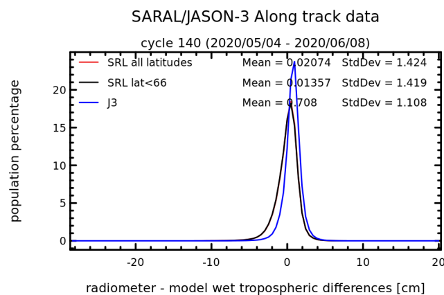
Figure 46: Histogram (of along-track data) of radiometer minus ECMWF model wet troposphere correction between SARAL/Altika and Jason-3 computed for SARAL/Altika cycle 140.
