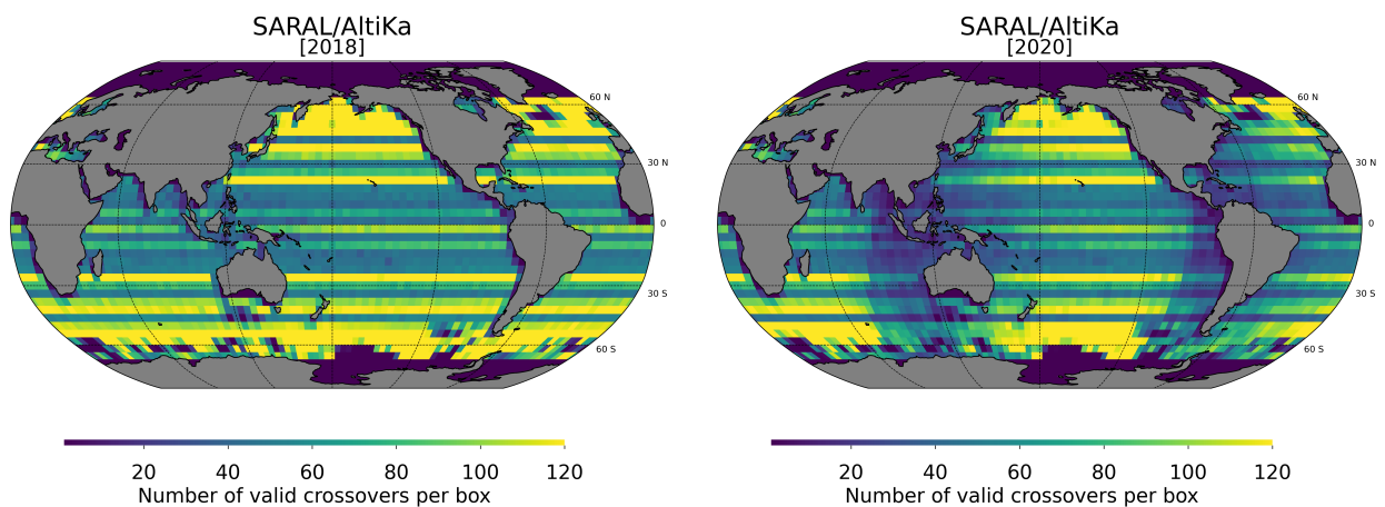
Figure 54: Number of valid crossovers per box for SARAL/AltiKa over (left) 2018, and (right) 2020.
