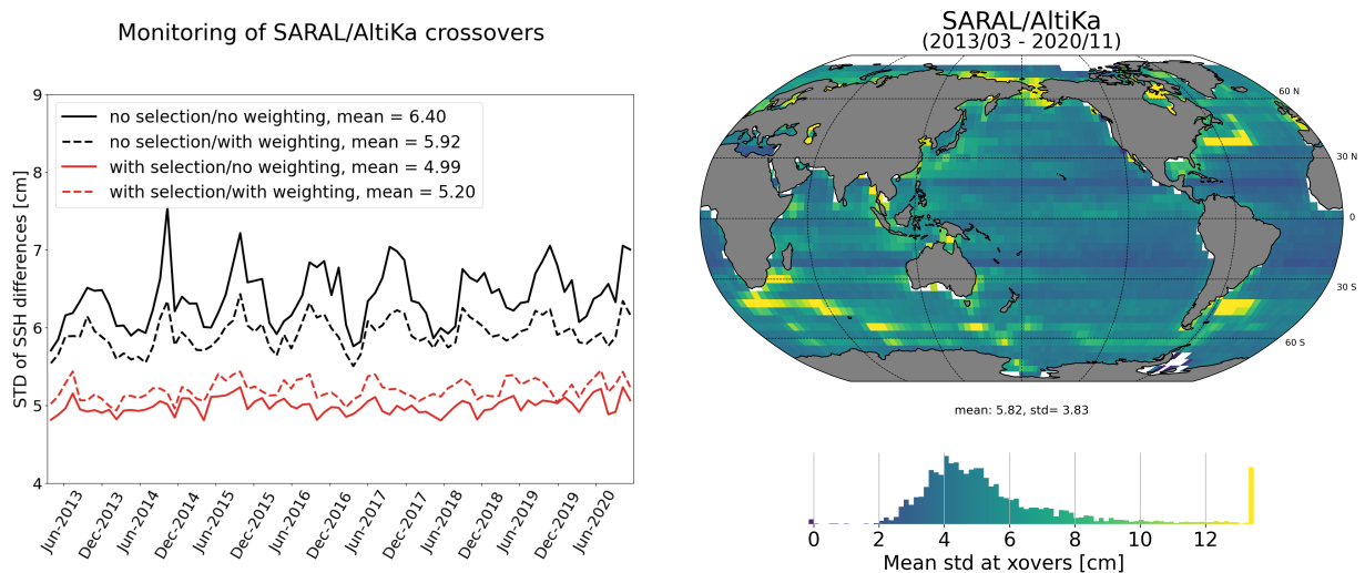
Figure 59: Cycle by cycle standard deviation of SSH crossover differences for SARAL/AltiKa using different selections and averaging methods (left) and map of standard deviation at crossover points. In both cases the radiometer wet tropospheric correction is used.
