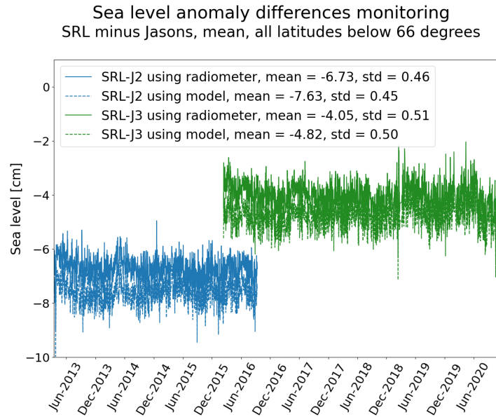
Figure 66: Monitoring of the daily mean SLA difference between SARAL/AltiKa and Jason-2 / SARAL/AltiKa and Jason-3, using the radiometer and model wet tropospheric corrections.
