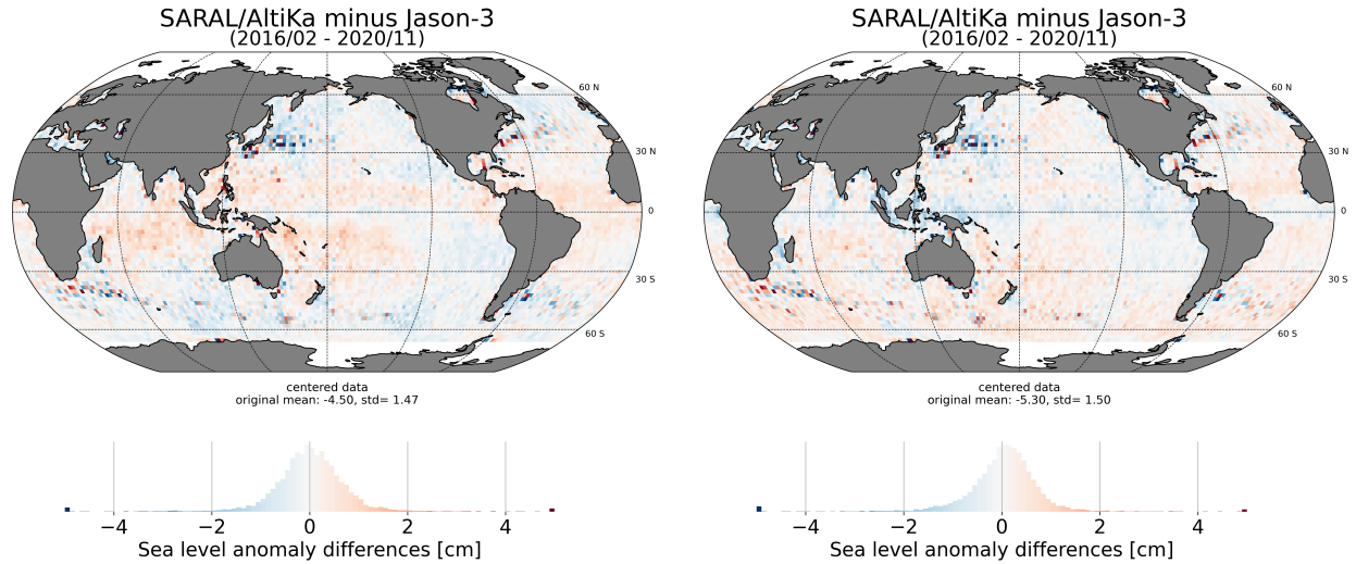
Figure 64: Map of mean SLA differences between SARAL/AltiKa and Jason-3 using (left) the radiometer and (right) model wet tropospheric correction.
