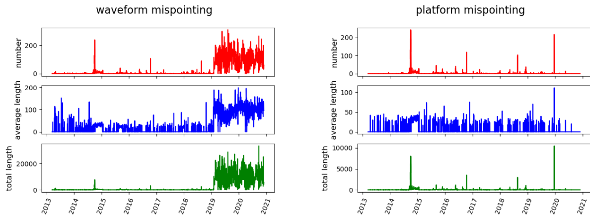
Figure 32: Monitoring of mispointed track sections from waveform (left) and platform (right) data.
