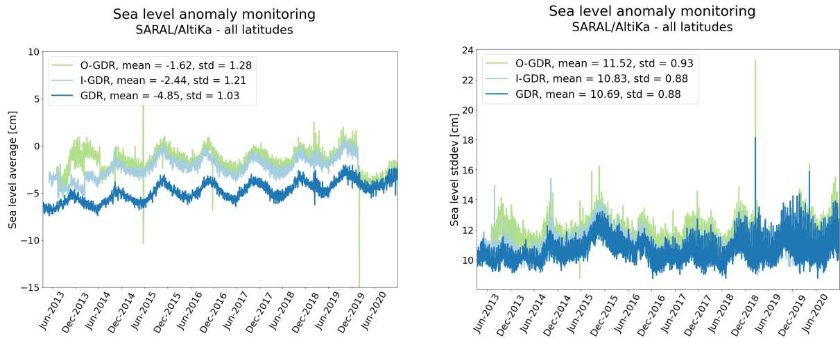
Figure 67: Daily monitoring of the mean (left) and standard deviation [right] of global average SARAL/AltiKa SLA, using the radiometer wet tropospheric correction, for OGDR, IGDR and GDR products.
