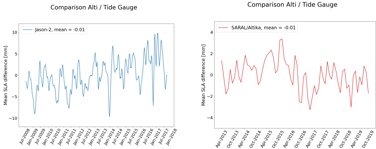
Figure 69: SLA differences between the altimeters and the GLOSS/CLIVAR tide gauge network for Jason-2 (left) and SARAL/AltiKa (right).
