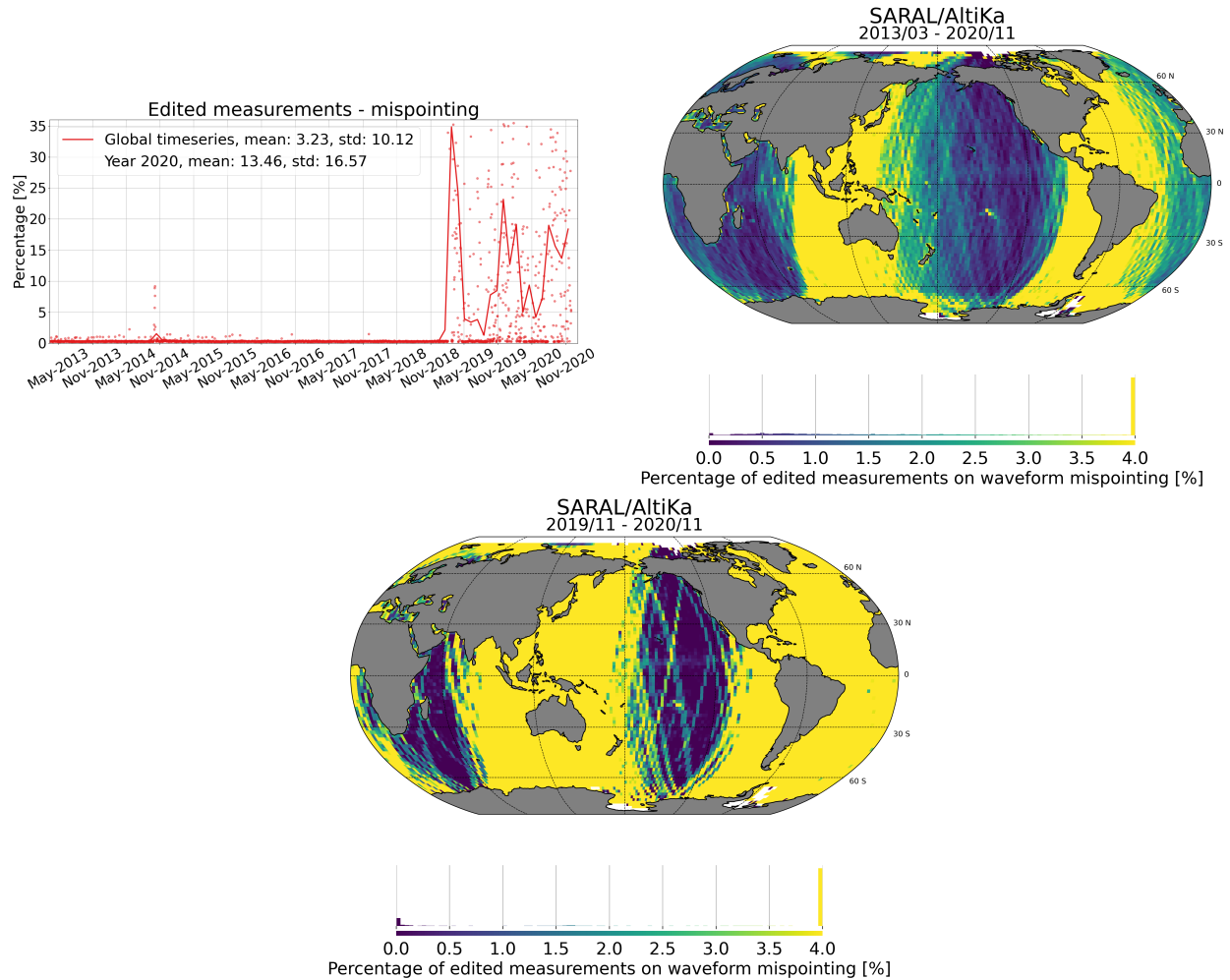
Figure 18: Percentage of edited measurements by square off-nadir angle criterion. [left] monitoring for GDR data, [right] map since the beginning of the mission (cycles 1 to 145) and [bottom] map over the past year (2020). Dots are daily averages while solid lines correspond to cycle averages.
