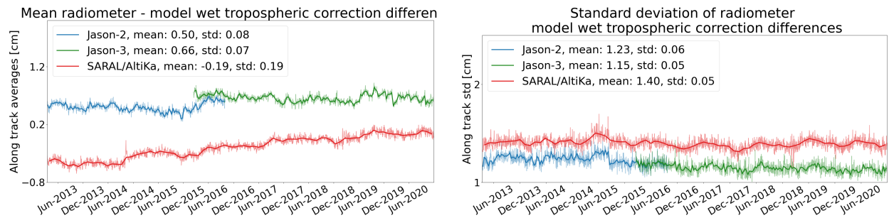
Figure 44: Monitoring of mean and standard deviation of radiometer minus model wet troposphere correction differences for SARAL/AltiKa Jason-2 and Jason-3. Dots are daily averages while solid lines correspond to cycle averages.
