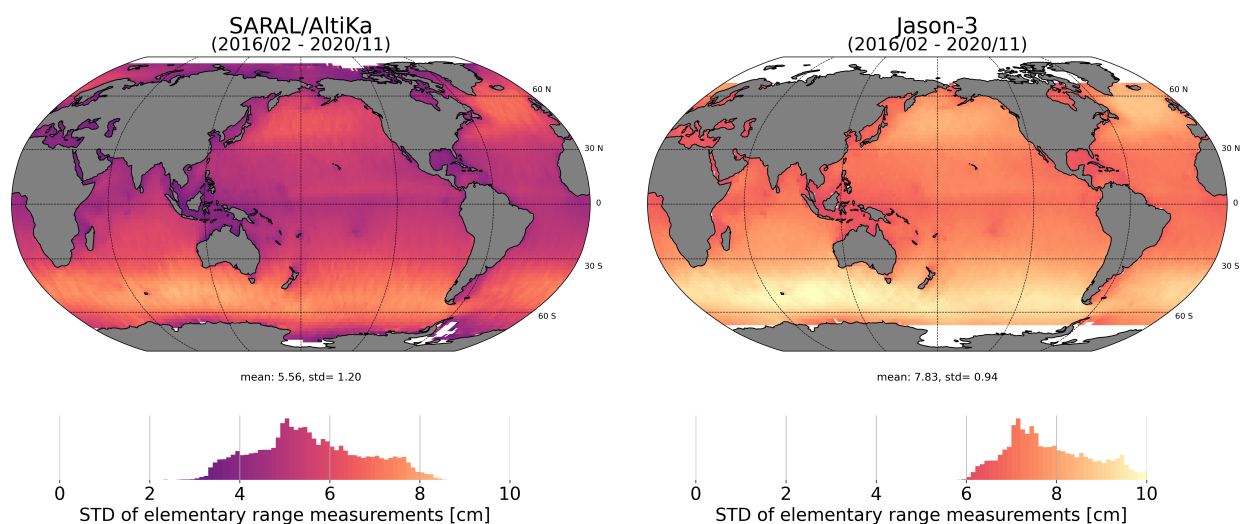
Figure 28: Average map of rms of SARAL/AltiKa elementary 40 Hz range measurements (left) and Jason-3 elementary 20 Hz range measurement (right).
