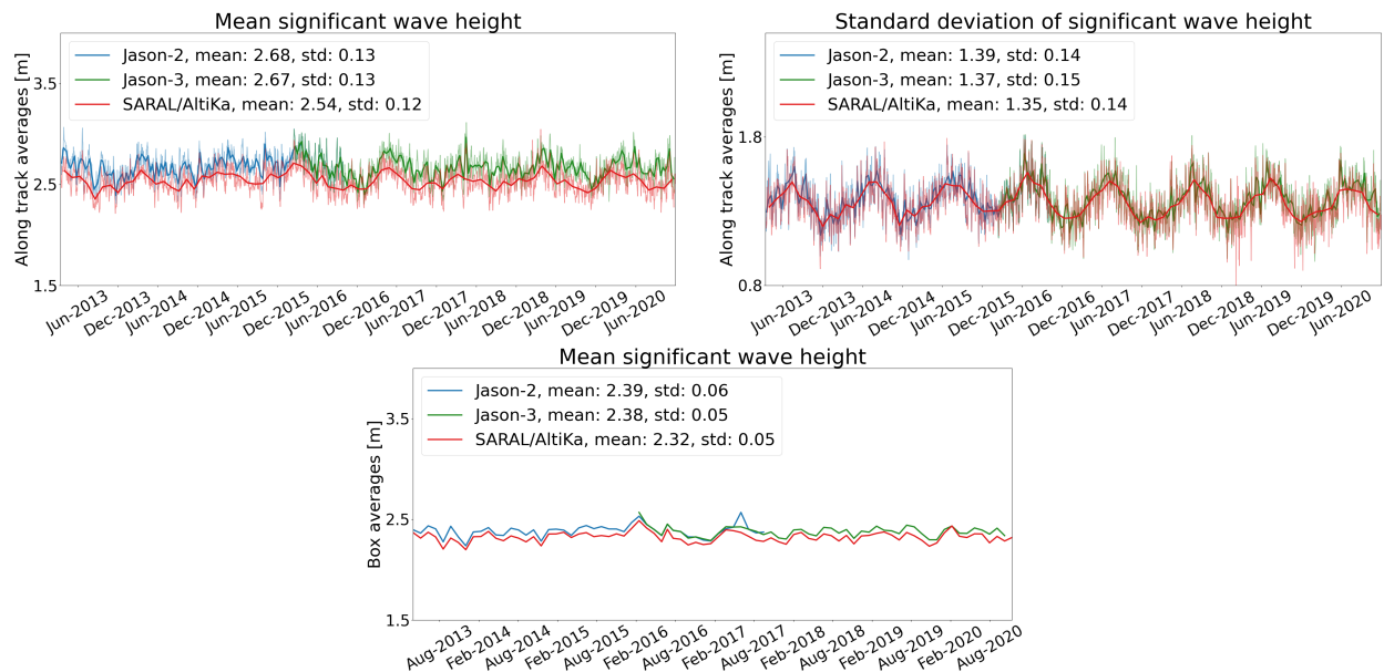
Figure 37: Daily monitoring of mean (top) and standard deviation (center) of significant wave height for SARAL/AltiKa, Jason-2 and Jason-3 and cycle per cycle monitoring of box averaged latitude weighted mean (bottom). Dots are daily averages while solid lines correspond to cycle averages.
