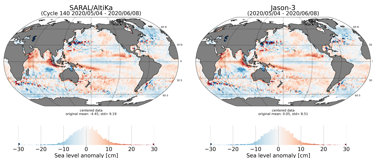
Figure 63: SLA map for SARAL/Altika 140 cycle using the radiometer wet tropospheric correction (left) from SARAL/Altika data, and (right) from Jason-3 data over the same period.
