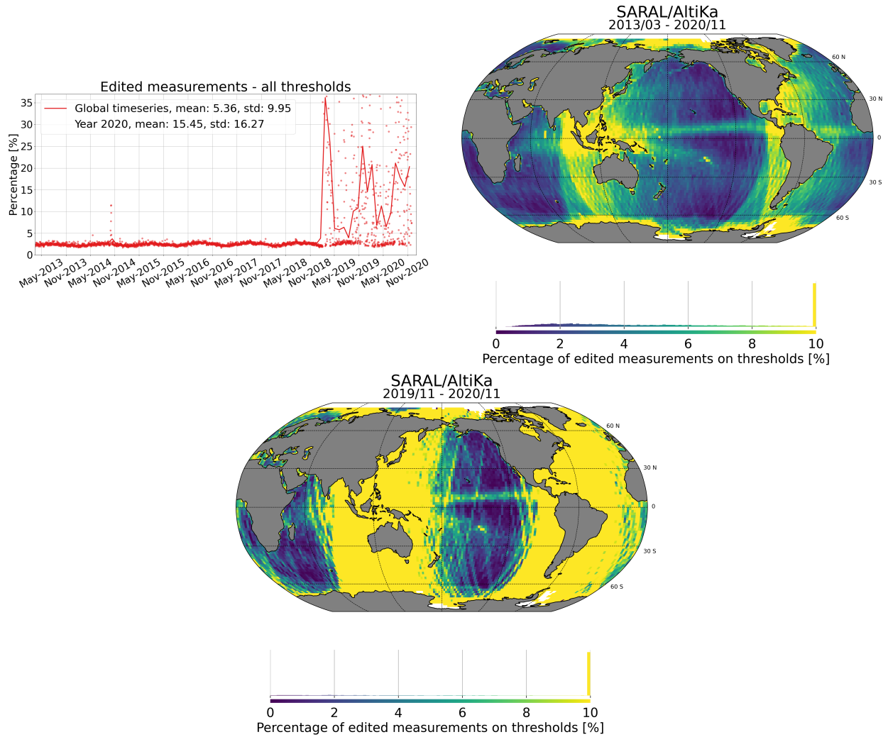
Figure 9: Percentage of edited measurements on all thresholds combined. [left] monitoring for GDR data, [right] map since the beginning of mission (cycles 1 to 145) and [bottom] map over the past year (2020). Dots are daily averages while solid lines correspond to cycle averages.
