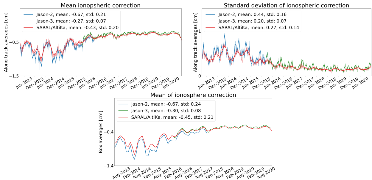
Figure 40: Daily monitoring of mean and standard deviation ionosphere correction for SARAL/AltiKa (GIM), Jason-2 and Jason-3 (filtered dual-frequency ionosphere correction with scale factor 0.14418 for mean computation). Dots are daily averages while solid lines correspond to cycle averages.
