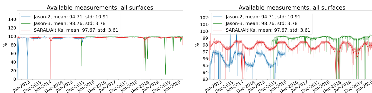
Figure 1: Percentage of available measurements over all surfaces for SARAL/AltiKa, Jason-2 and Jason-3. Dots are daily averages while solid lines correspond to cycle averages.
