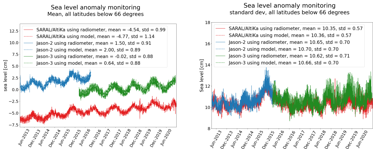
Figure 65: Monitoring of daily mean (left) and daily standard deviation (right) of SLA of GDR data using the radiometer (plain lines) and the model (dotted lines) wet tropospheric corrections. Global statistics are estimated for all latitudes between -66^\circ and 66^\circ .
