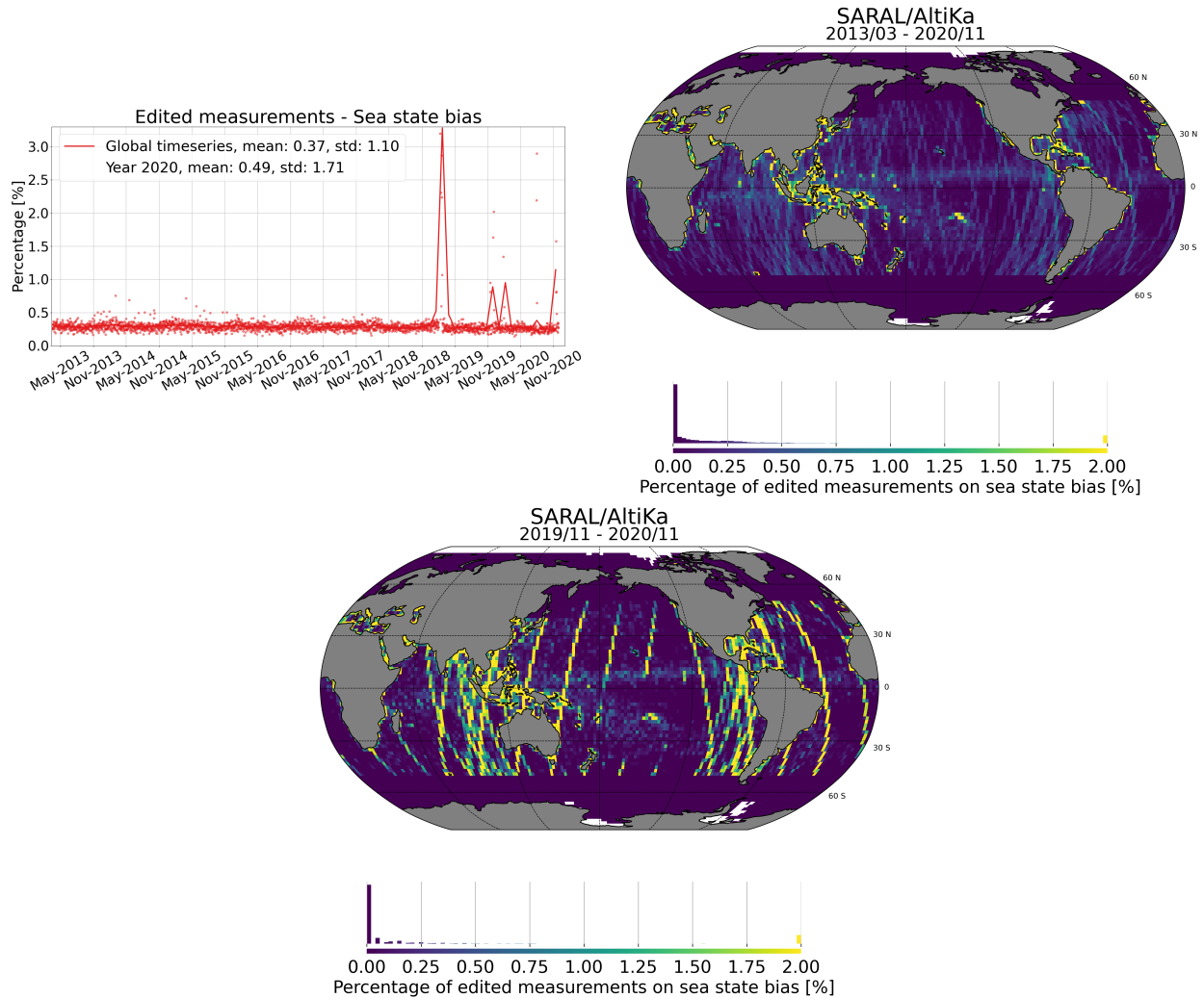
Figure 19: Percentage of edited measurements by sea state bias criterion. [left] monitoring for GDR data, [right] map since the beginning of the mission (cycles 1 to 145) and [bottom] map over the past year (2020). Dots are daily averages while solid lines correspond to cycle averages.
