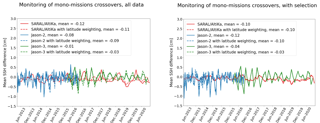
Figure 56: Cycle per cycle monitoring of ascending/descending SSH differences at mono-mission crossovers for SARAL/Altika Jason-2 and Jason-3 for Saral cycles 1 to 145.
