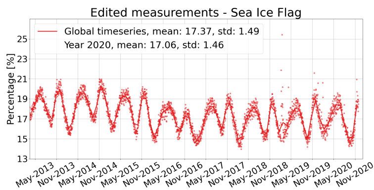
Figure 6: Percentage of edited measurements by ice flag criterion. Monitoring for GDR data (all latitude). Dots are daily averages while solid lines correspond to cycle averages.
