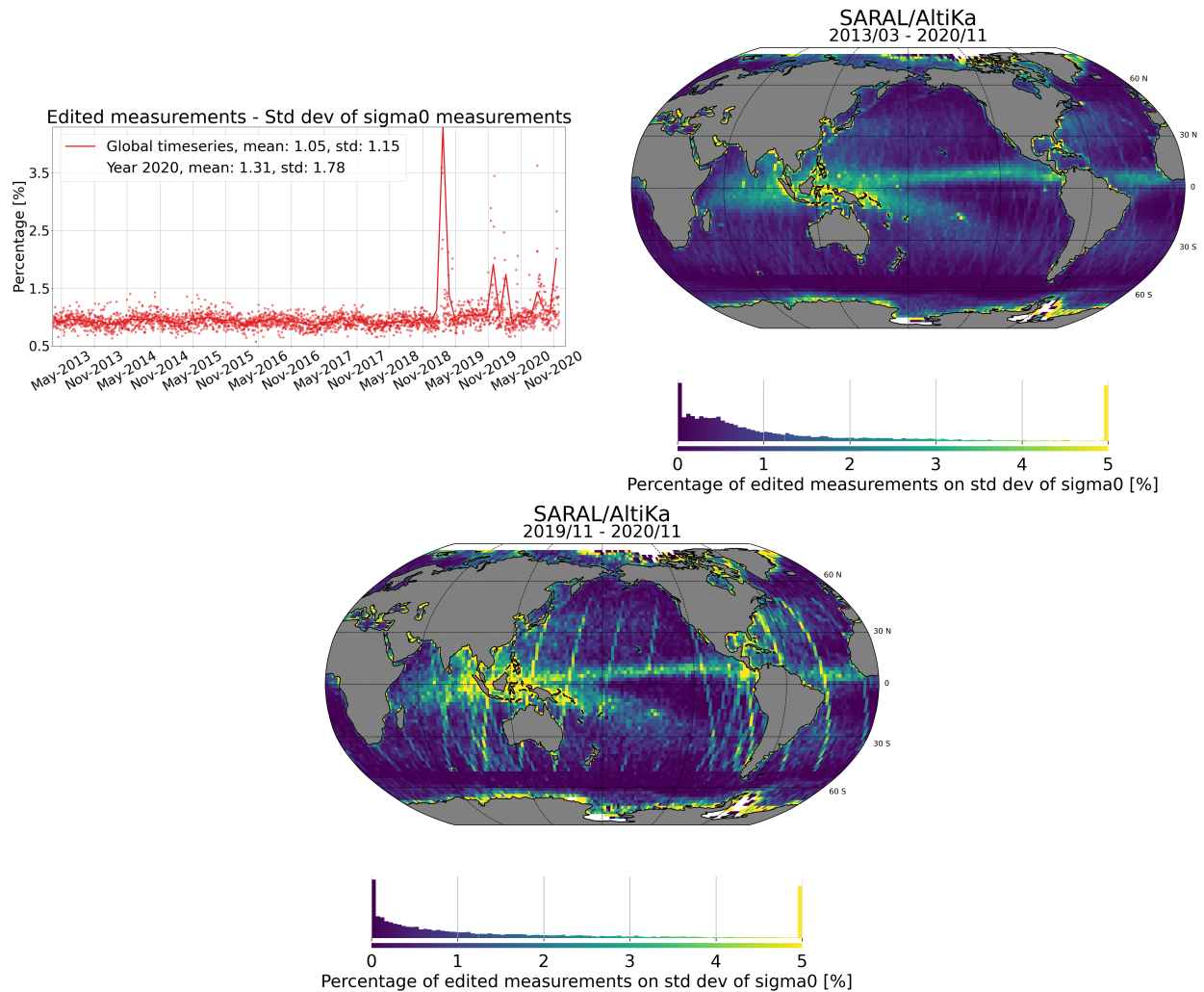
Figure 16: Percentage of edited measurements by 40 Hz Sigma0 standard deviation criterion. [left] monitoring for GDR data, [right] map since the beginning of mission (cycles 1 to 145) and [bottom] map over the past year (2020). Dots are daily averages while solid lines correspond to cycle averages.
