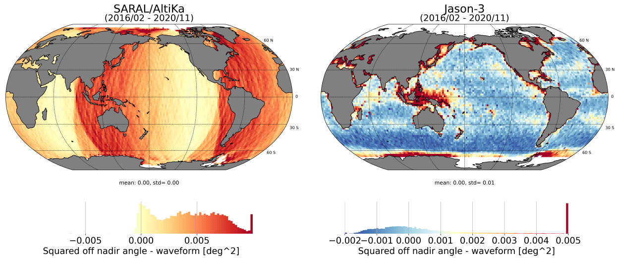
Figure 30: Average map of off-nadir angle from waveforms for SARAL/AltiKa (left) and Jason-3 (right).
