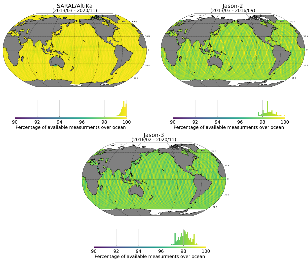
Figure 4: Map of the percentage of available measurements over ocean for SARAL/AltiKa (left) Jason-2 (right) and Jason-3 (bottom).
