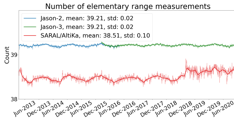
Figure 25: Daily monitoring of mean of number of elementary measurements for SARAL/AltiKa (ref) , Jason-2 (blue) and Jason-3 (green). Dots represent daily averages, the lines corresponds to cycle averages. Jason-2 and Jason-3 data are multiplied by two to account for the 40Hz/20Hz difference between the two missions.
